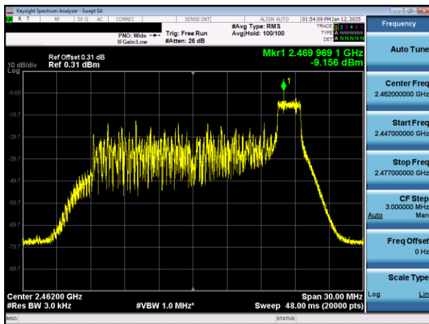
Plot 7-7. Power Spectral Density Plot Antenna WF2b (802.11ax OFDMA – RU26 Index 8 – Ch. 11)
