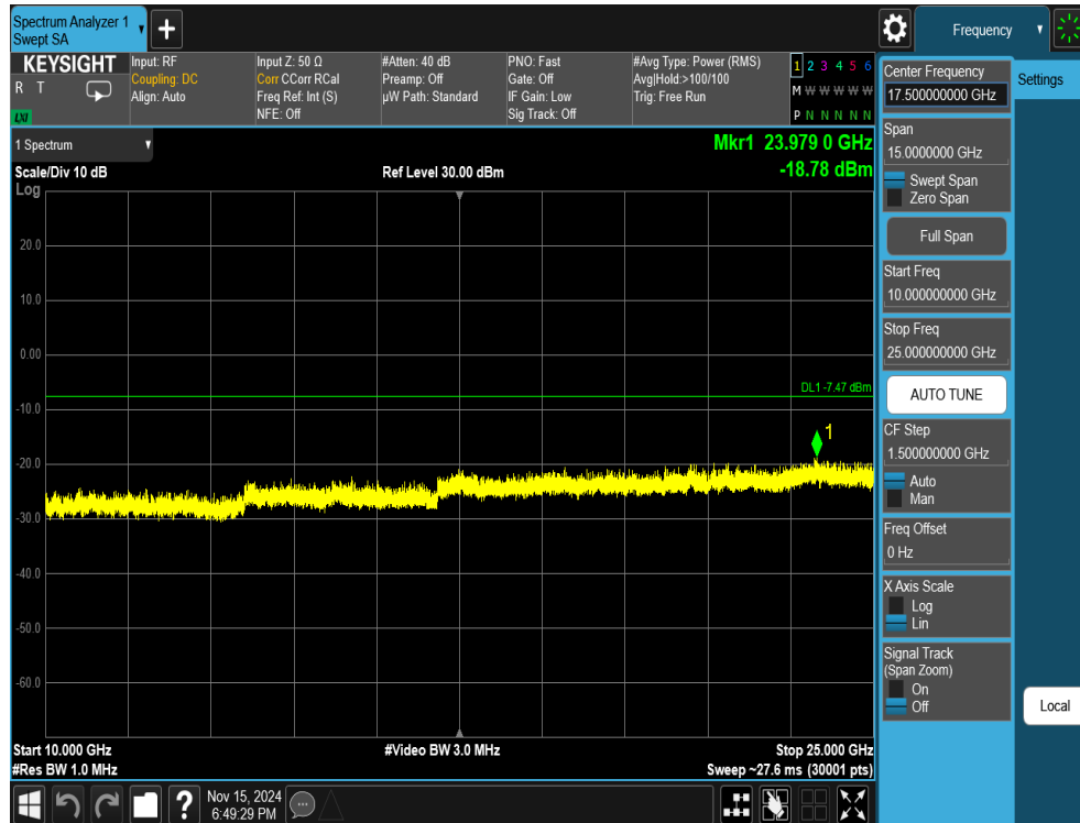
Plot 7-54. Conducted Spurious Plot Antenna WF7b (802.11ax OFDMA – RU242 – Ch. 11)
