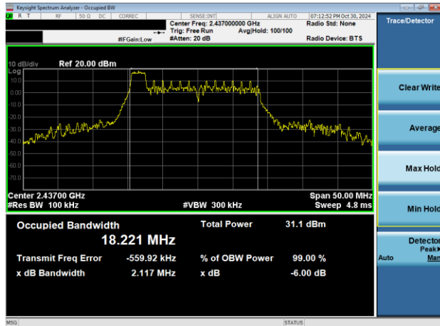
Plot 7-3. 6dB BW & 99% OBW Antenna WF2b (802.11ax OFDMA – RU26 Index 0 – Ch. 6)
