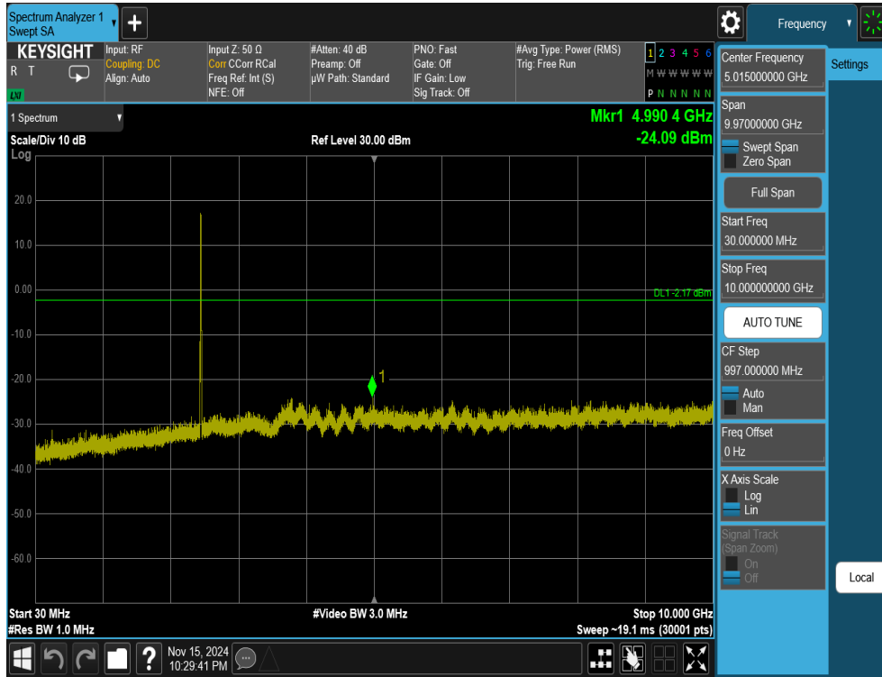
Plot 7-59. Conducted Spurious Plot Antenna WF2b (802.11ax OFDMA – RU26 – Ch. 11)
