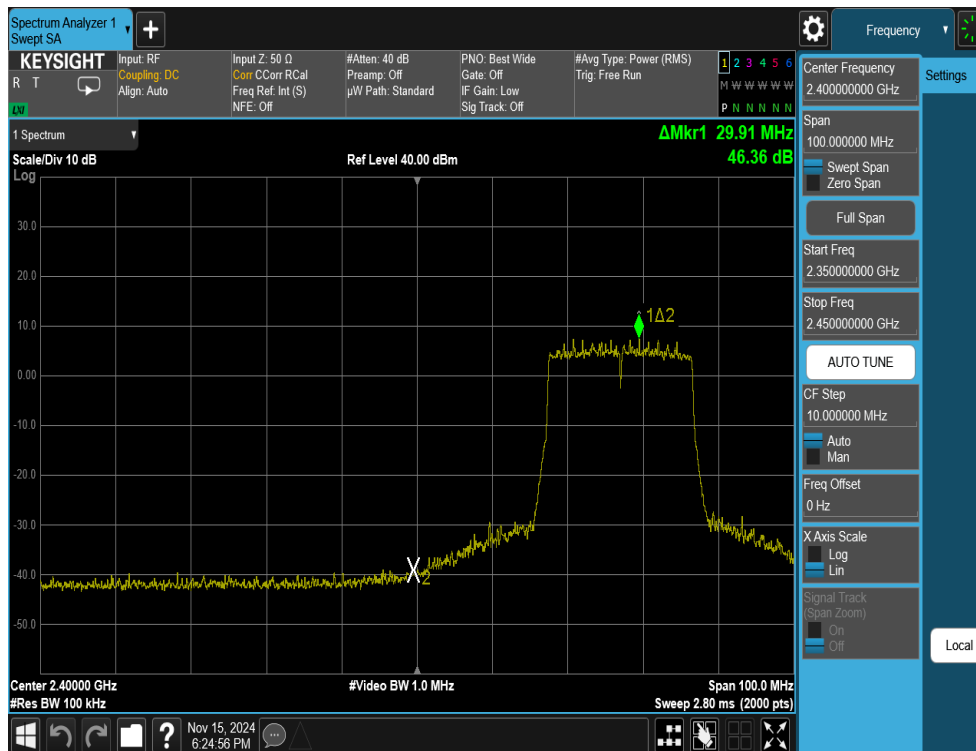
Plot 7-18. Band Edge Antenna WF7b (802.11ax OFDMA – RU242 – Ch. 4)
