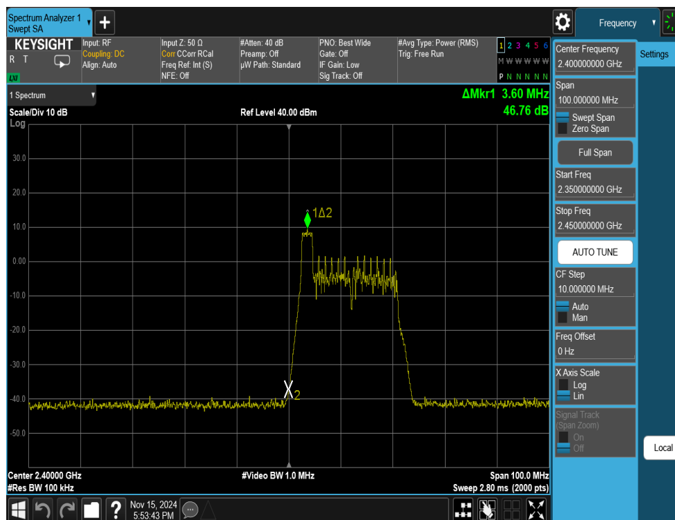
Plot 7-13. Band Edge Antenna WF7b (802.11ax OFDMA – RU26 Index 0 – Ch. 1)
