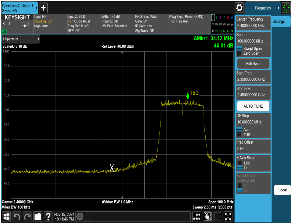
Plot 7-33. Band Edge Antenna WF2b (802.11ax OFDMA – RU242 – Ch. 4)
