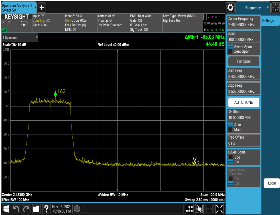
Plot 7-39. Band Edge Antenna WF2b (802.11ax OFDMA – RU242 – Ch. 9)
