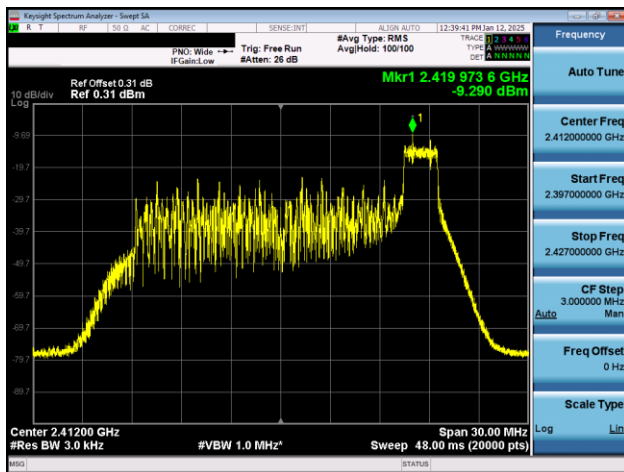
Plot 7-5. Power Spectral Density Plot Antenna WF7b (802.11ax OFDMA – RU26 Index 8 – Ch. 1)
