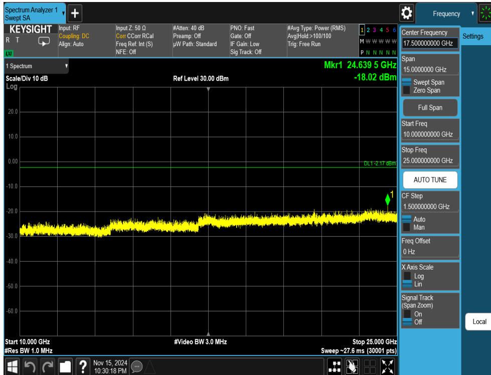
Plot 7-60. Conducted Spurious Plot Antenna WF2b (802.11ax OFDMA – RU26 – Ch. 11)
