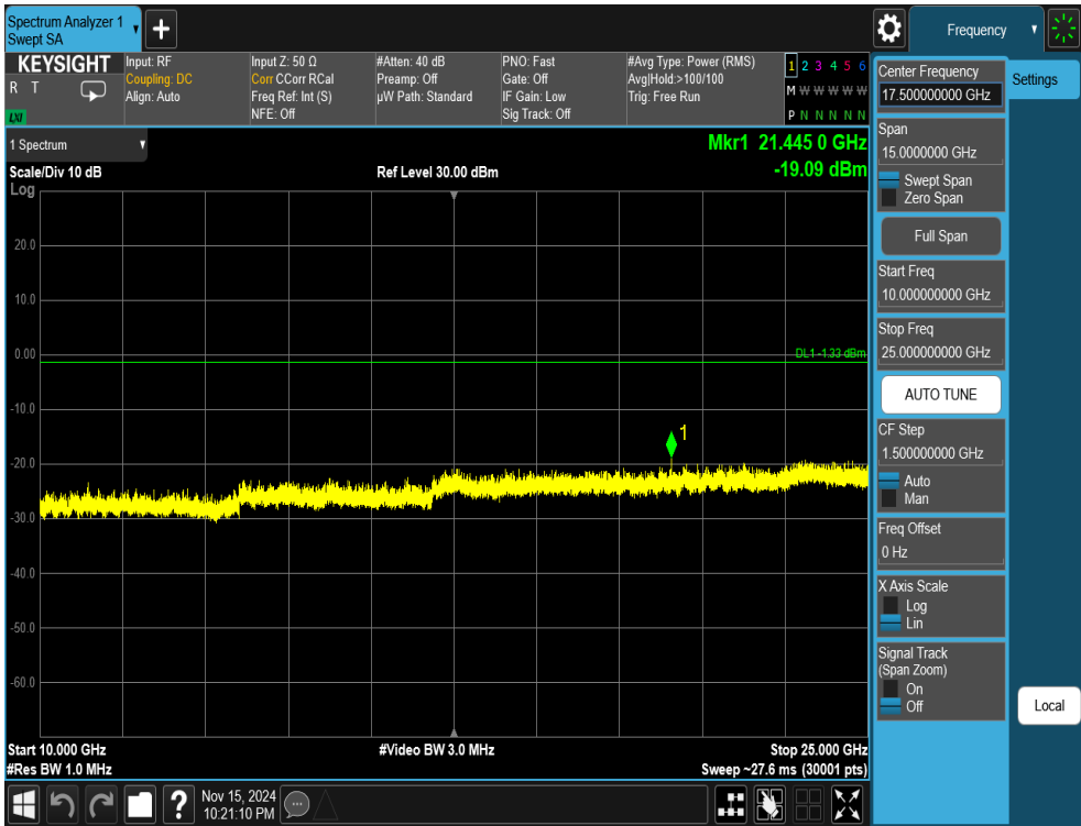
Plot 7-56. Conducted Spurious Plot Antenna WF2b (802.11ax OFDMA – RU26 – Ch. 1)
