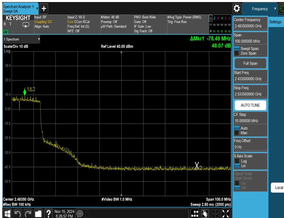
Plot 7-21. Band Edge Antenna WF7b (802.11ax OFDMA – RU242 – Ch. 6(High Channel))
