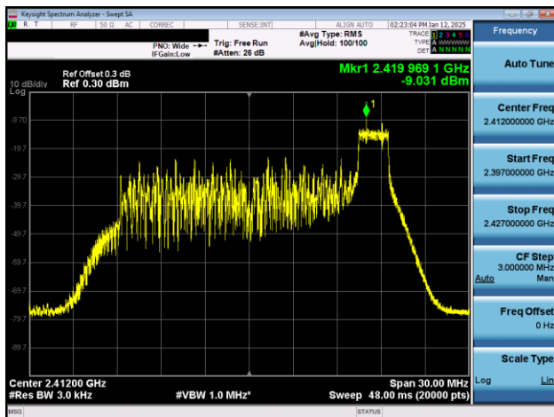
Plot 7-10. Power Spectral Density Plot Antenna WF2b (802.11ax OFDMA – RU26 Index 8 – Ch. 1)
