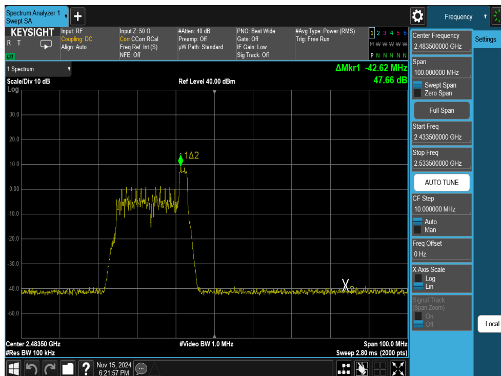
Plot 7-14. Band Edge Antenna WF7b (802.11ax OFDMA – RU26 Index 8 – Ch. 12)
