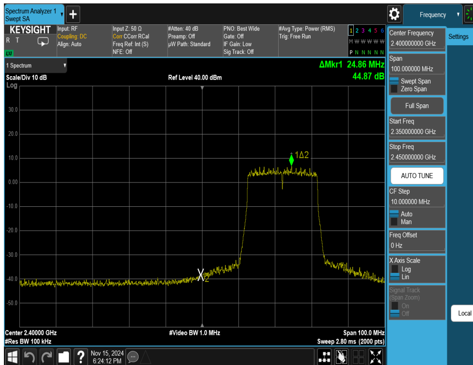
Plot 7-17. Band Edge Antenna WF7b (802.11ax OFDMA – RU242 – Ch. 3)
