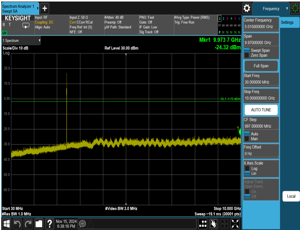
Plot 7-45. Conducted Spurious Plot Antenna WF7b (802.11ax OFDMA – RU26 – Ch. 6)
