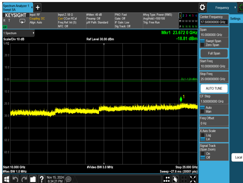
Plot 7-44. Conducted Spurious Plot Antenna WF7b (802.11ax OFDMA – RU26 – Ch. 1)
