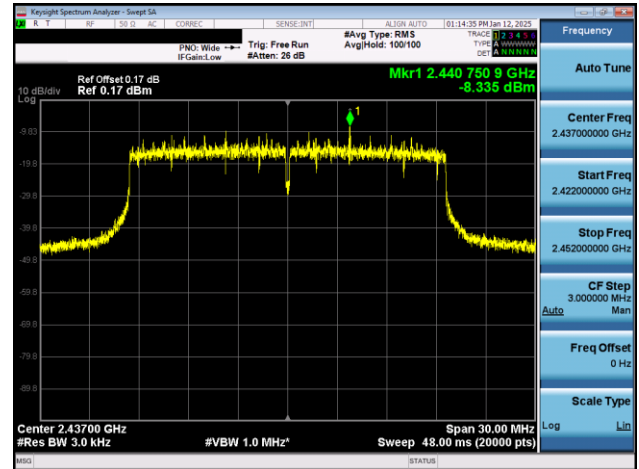
Plot 7-11. Power Spectral Density Plot Antenna WF7b (802.11ax OFDMA – RU242 – Ch. 6)
