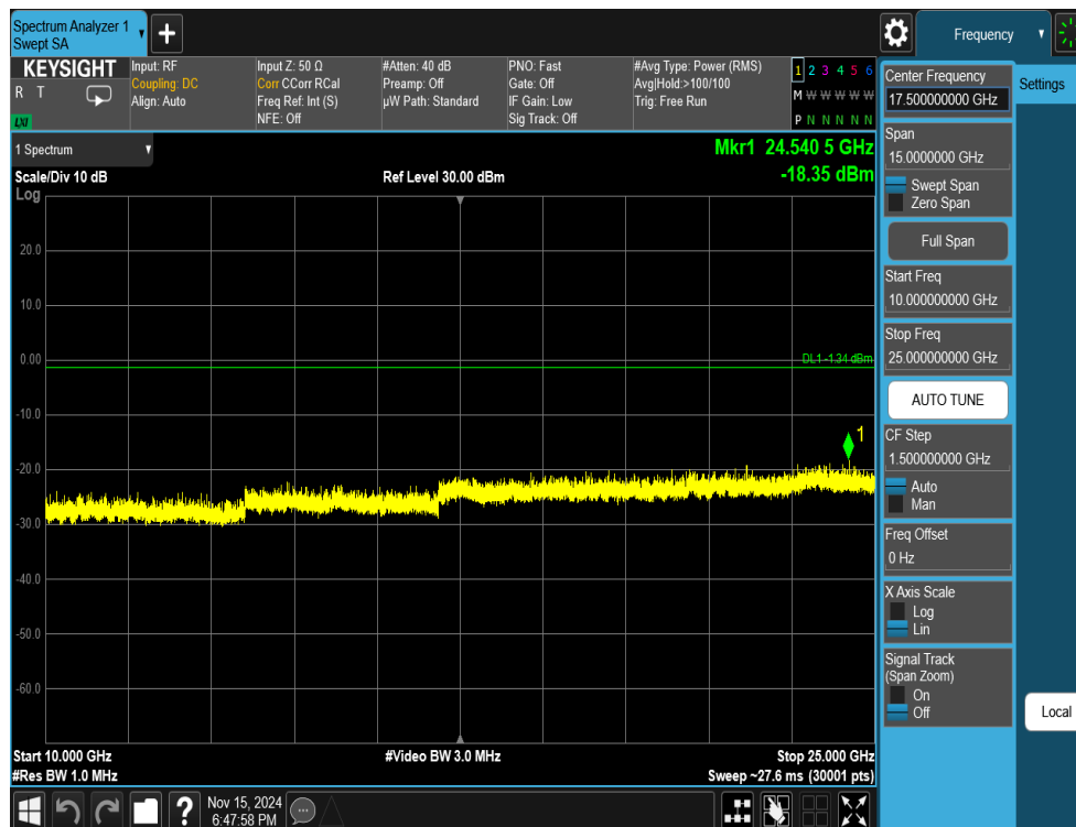
Plot 7-52. Conducted Spurious Plot Antenna WF7b (802.11ax OFDMA – RU242 – Ch. 6)
