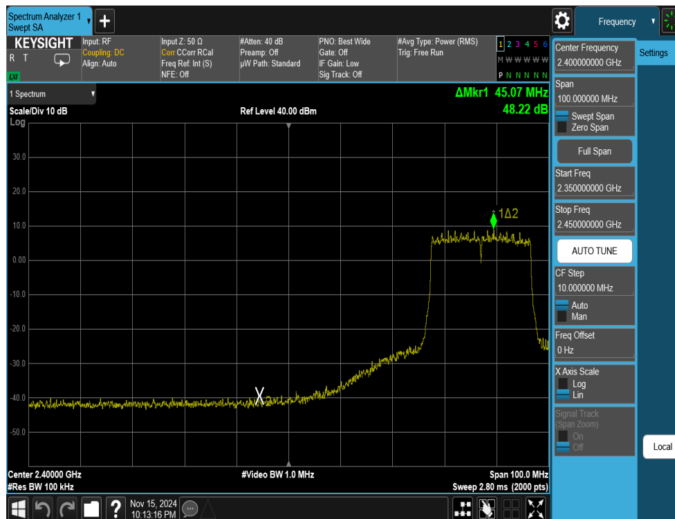
Plot 7-35. Band Edge Antenna WF2b (802.11ax OFDMA – RU242 – Ch. 6(Low Channel))
