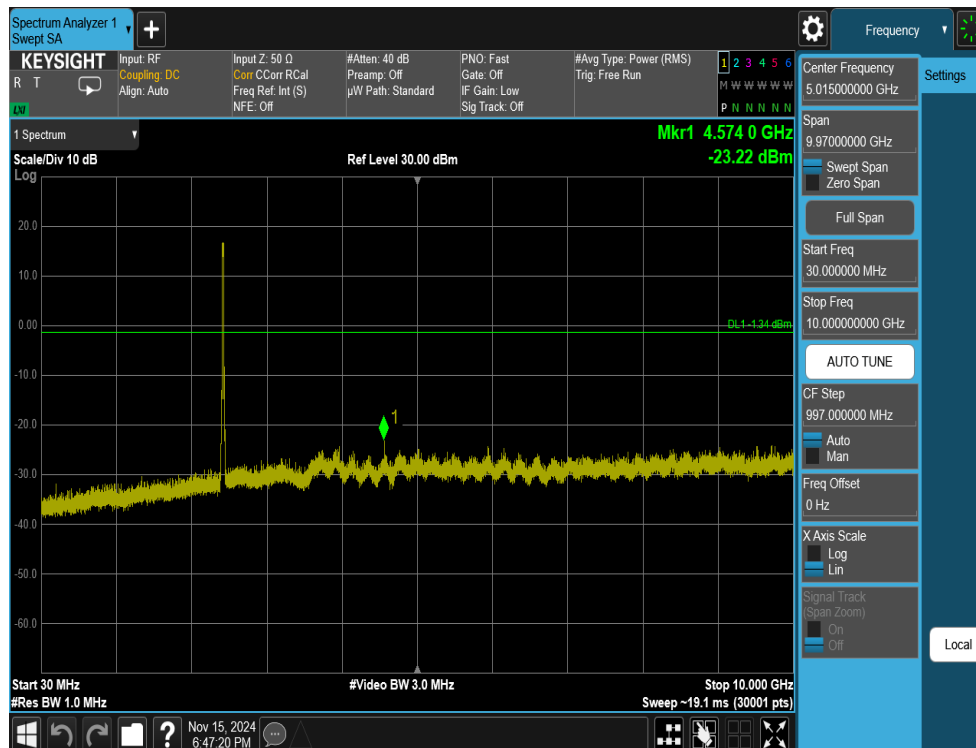
Plot 7-51. Conducted Spurious Plot Antenna WF7b (802.11ax OFDMA – RU242 – Ch. 6)
