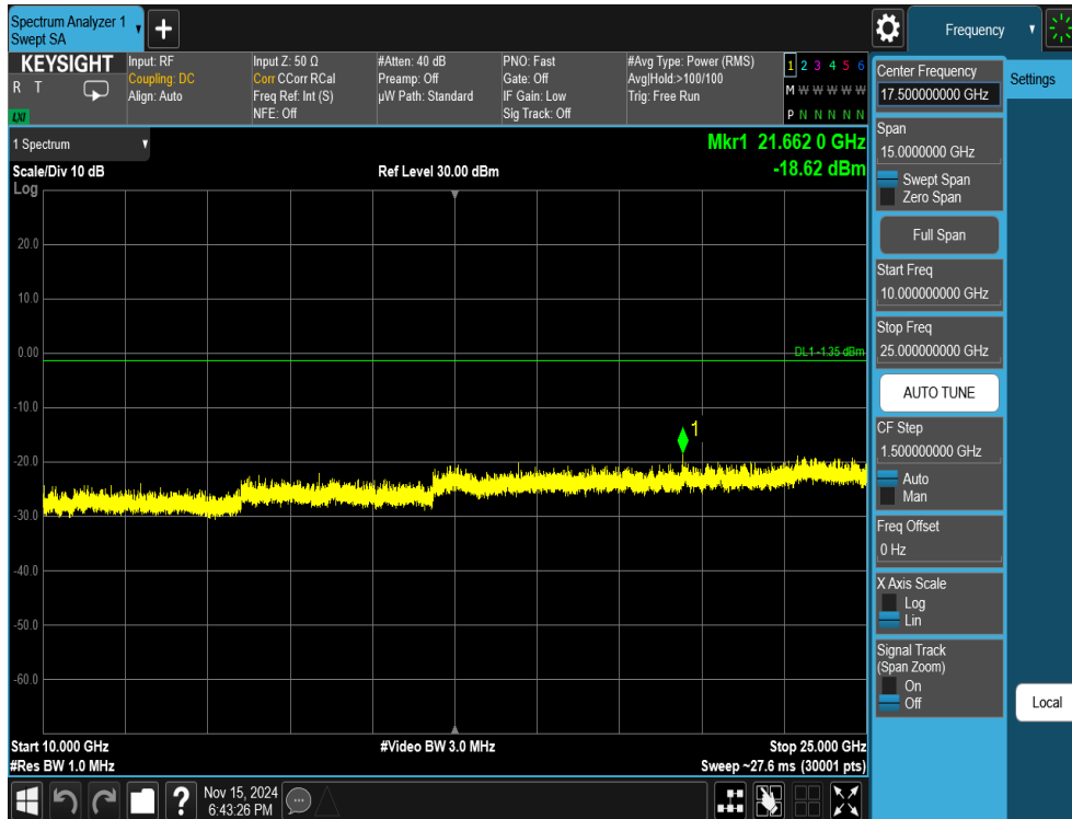
Plot 7-48. Conducted Spurious Plot Antenna WF7b (802.11ax OFDMA – RU26 – Ch. 11)
