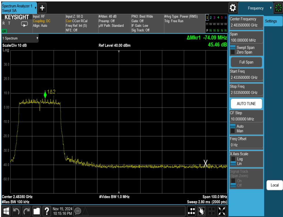
Plot 7-38. Band Edge Antenna WF2b (802.11ax OFDMA – RU242 – Ch. 8)
