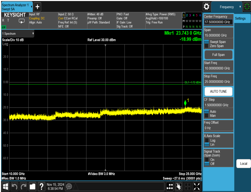
Plot 7-46. Conducted Spurious Plot Antenna WF7b (802.11ax OFDMA – RU26 – Ch. 6)
