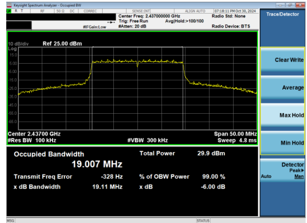
Plot 7-4. 6dB BW & 99% OBW Plot Antenna WF2b (802.11ax OFDMA – RU242 – Ch. 6)
