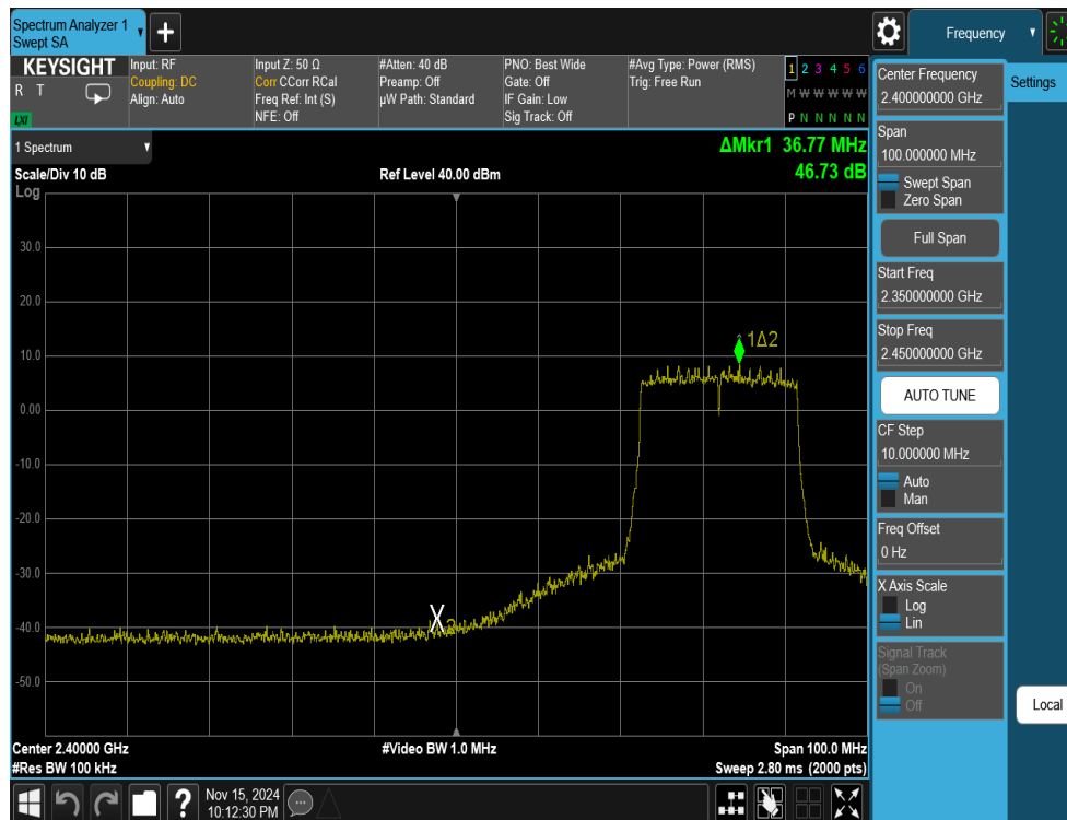
Plot 7-34. Band Edge Antenna WF2b (802.11ax OFDMA – RU242 – Ch. 5)
