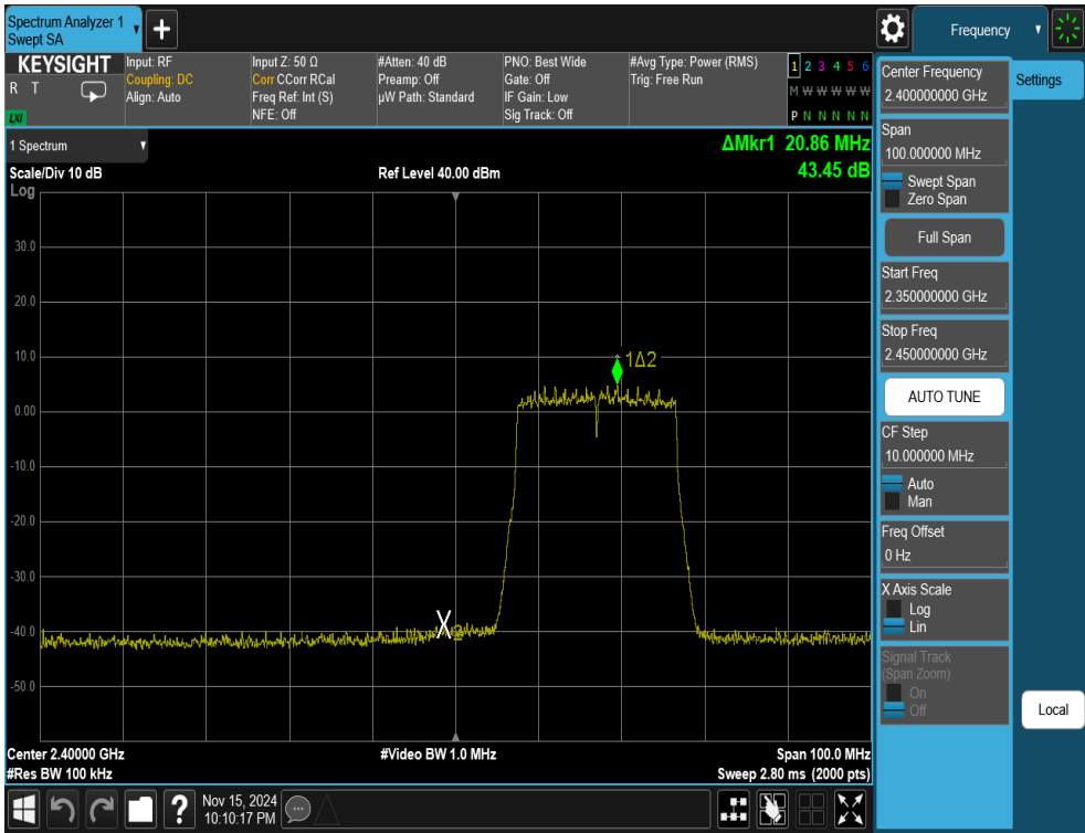
Plot 7-31. Band Edge Antenna WF2b (802.11ax OFDMA – RU242 – Ch. 2)
