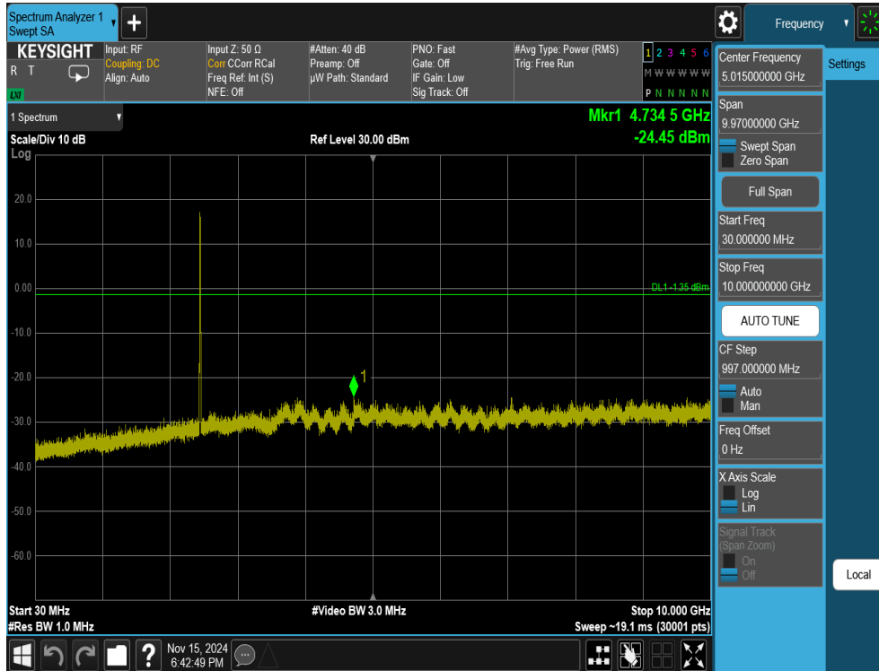
Plot 7-47. Conducted Spurious Plot Antenna WF7b (802.11ax OFDMA – RU26 – Ch. 11)
