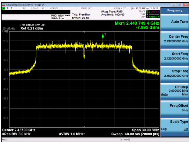
Plot 7-8. Power Spectral Density Plot Antenna WF2b (802.11ax OFDMA – RU242 – Ch. 6)
