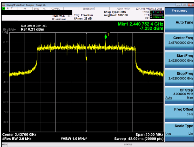
Plot 7-6. Power Spectral Density Plot Antenna WF7b (802.11ax OFDMA – RU242 – Ch. 6)
