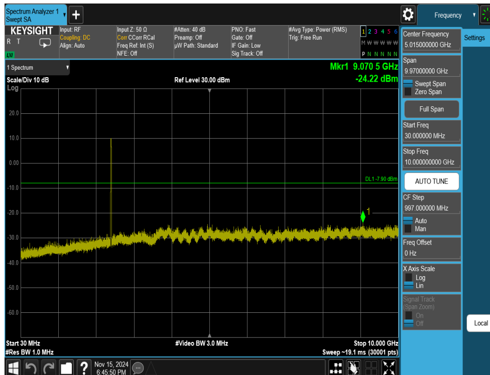
Plot 7-49. Conducted Spurious Plot Antenna WF7b (802.11ax OFDMA – RU242 – Ch. 1)
