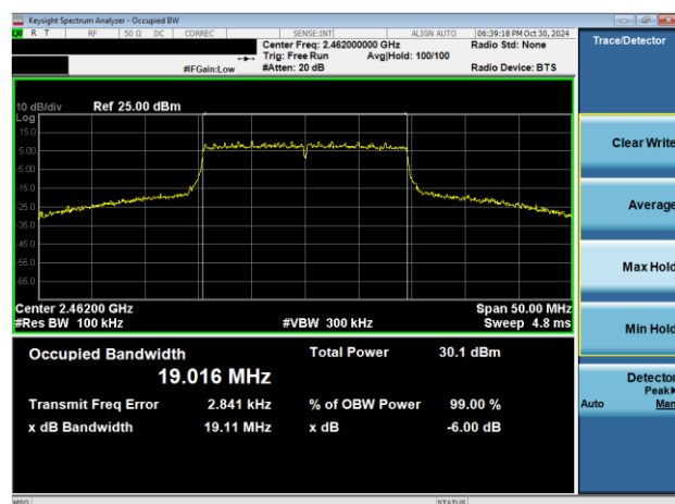
Plot 7-2. 6dB BW & 99% OBW Plot Antenna WF7b (802.11ax OFDMA – RU242 – Ch. 11)
