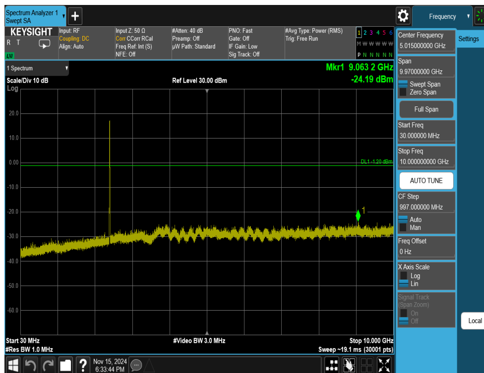
Plot 7-43. Conducted Spurious Plot Antenna WF7b (802.11ax OFDMA – RU26 – Ch. 1)
