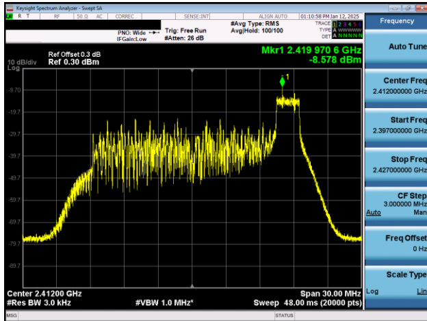
Plot 7-9. Power Spectral Density Plot Antenna WF7b (802.11ax OFDMA – RU26 Index 8 – Ch. 1)
