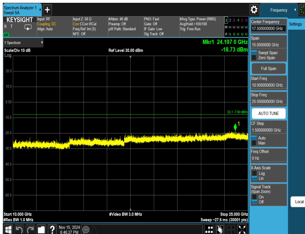
Plot 7-50. Conducted Spurious Plot Antenna WF7b (802.11ax OFDMA – RU242 – Ch. 1)
