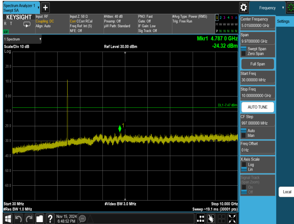
Plot 7-53. Conducted Spurious Plot Antenna WF7b (802.11ax OFDMA – RU242 – Ch. 11)
