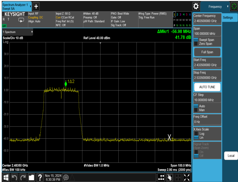
Plot 7-26. Band Edge Antenna WF7b (802.11ax OFDMA – RU242 – Ch. 11)
