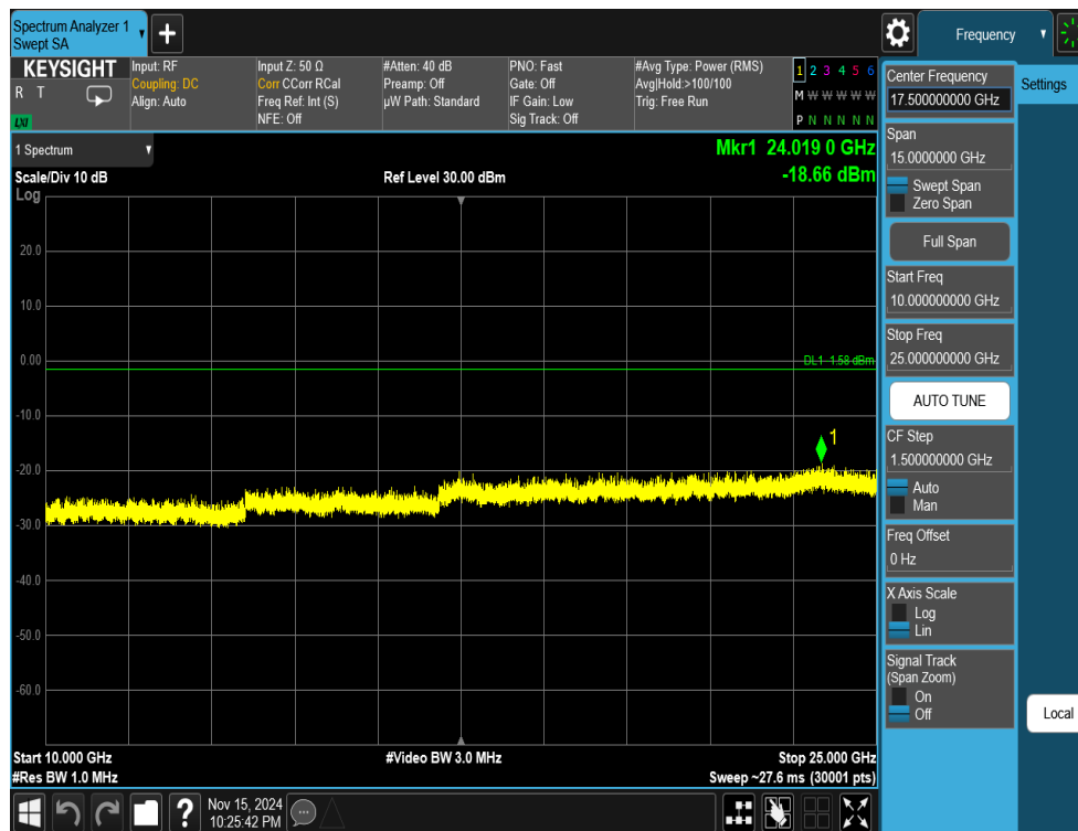
Plot 7-58. Conducted Spurious Plot Antenna WF2b (802.11ax OFDMA – RU26 – Ch. 6)
