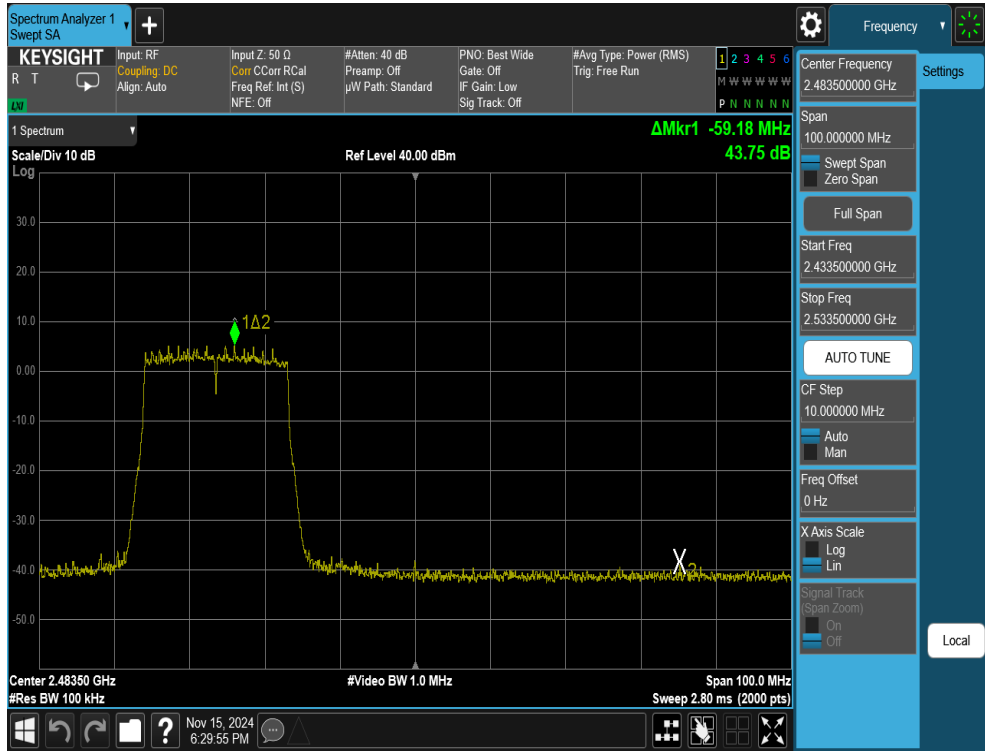
Plot 7-25. Band Edge Antenna WF7b (802.11ax OFDMA – RU242 – Ch. 10)
