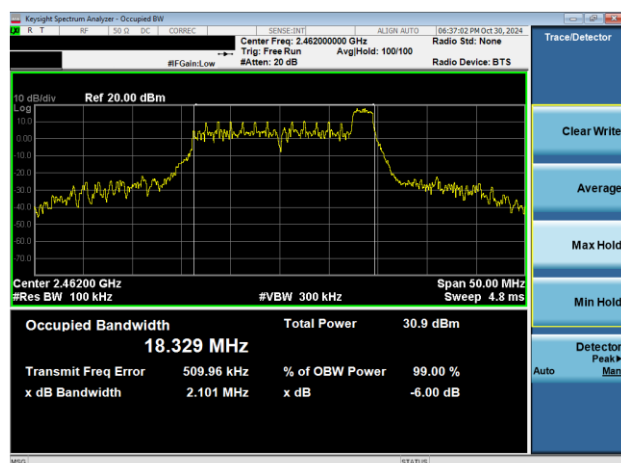
Plot 7-1. 6dB BW & 99% OBW Plot Antenna WF7b (802.11ax OFDMA – RU26 Index 8 – Ch. 11)
