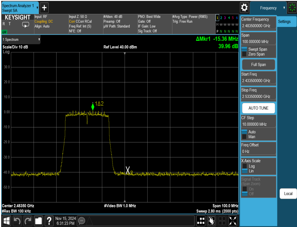
Plot 7-27. Band Edge Antenna WF7b (802.11ax OFDMA – RU242 – Ch. 12)
