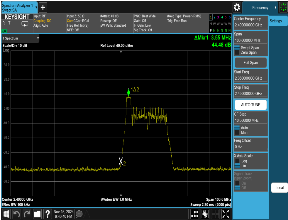
Plot 7-28. Band Edge Antenna WF2b (802.11ax OFDMA – RU26 Index 0 – Ch. 1)
