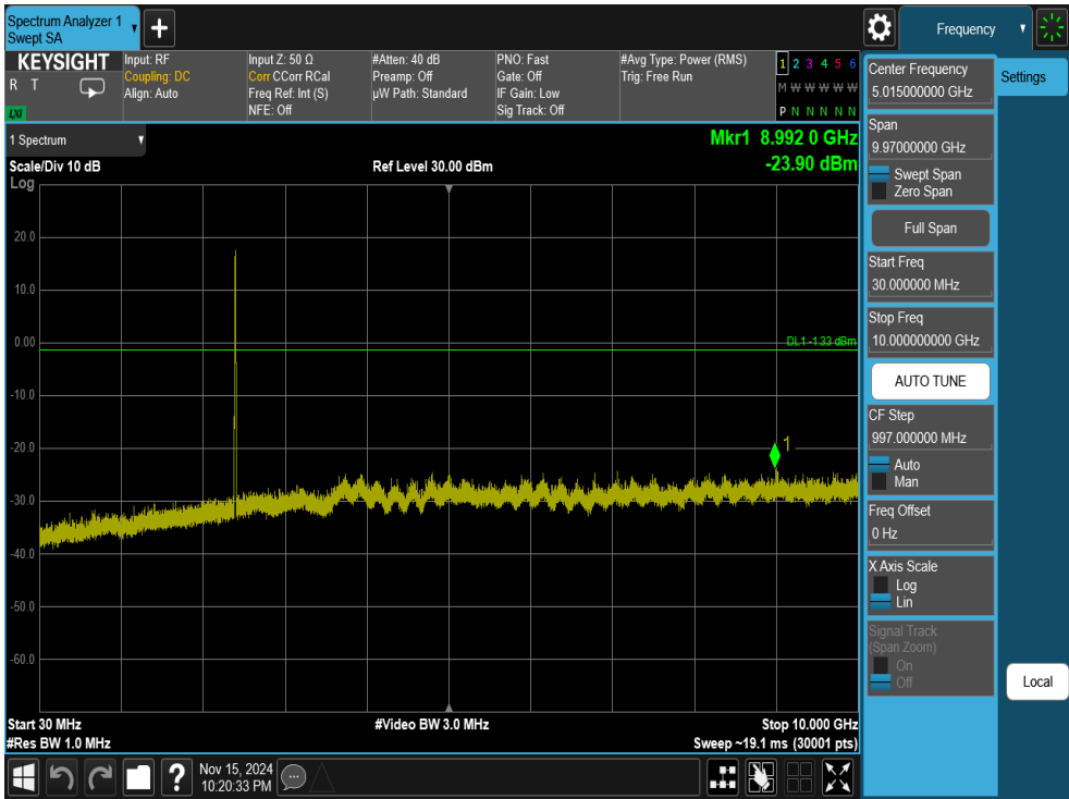
Plot 7-55. Conducted Spurious Plot Antenna WF2b (802.11ax OFDMA – RU26 – Ch. 1)
