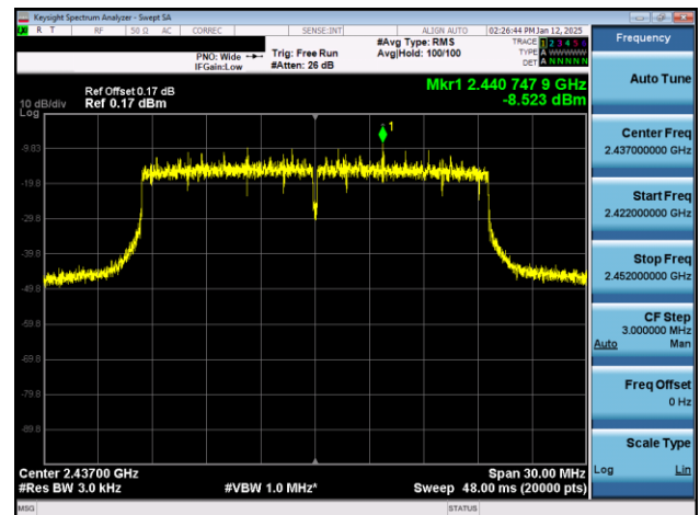
Plot 7-12. Power Spectral Density Plot Antenna WF2b (802.11ax OFDMA – RU242 – Ch. 6)
