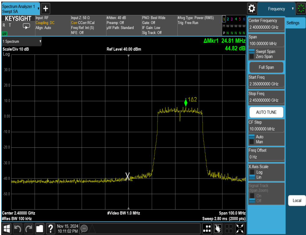
Plot 7-32. Band Edge Antenna WF2b (802.11ax OFDMA – RU242 – Ch. 3)
