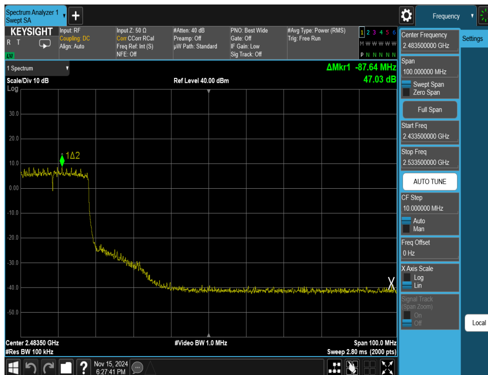
Plot 7-22. Band Edge Antenna WF7b (802.11ax OFDMA – RU242 – Ch. 7)
