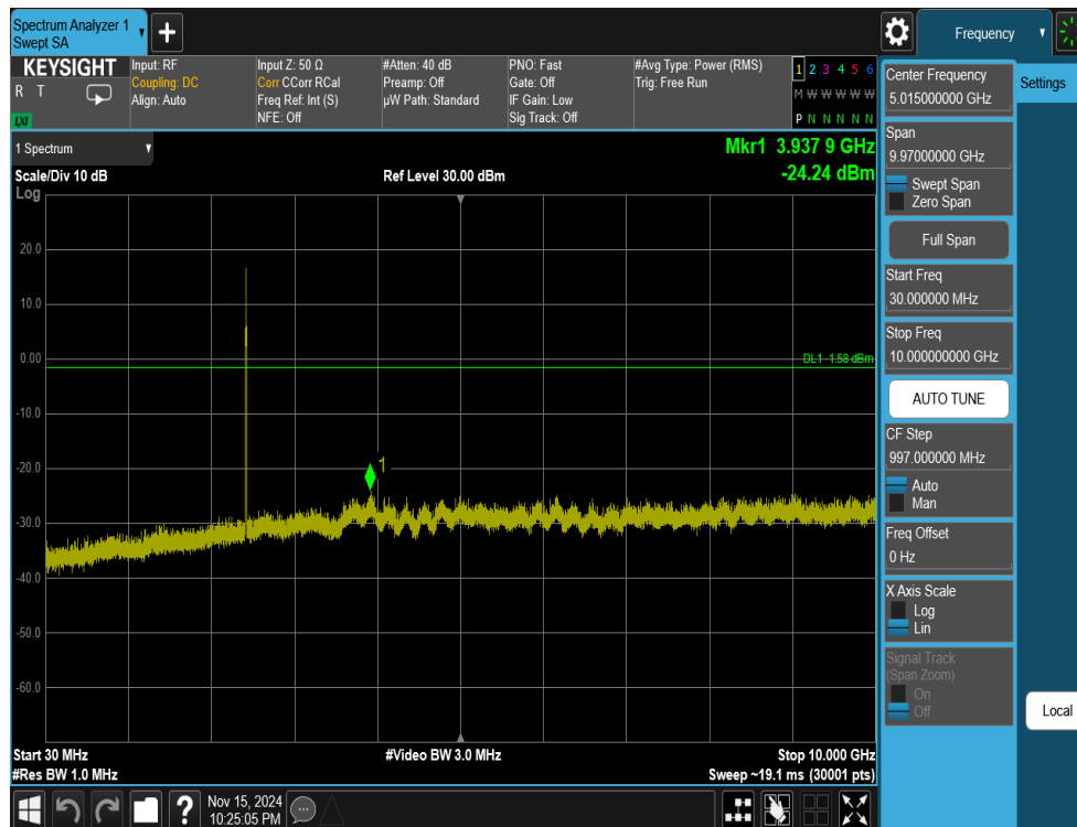
Plot 7-57. Conducted Spurious Plot Antenna WF2b (802.11ax OFDMA – RU26 – Ch. 6)
