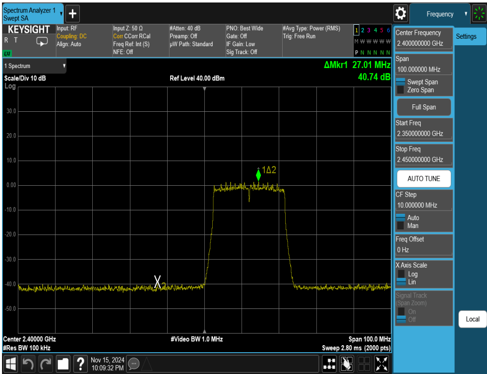
Plot 7-30. Band Edge Antenna WF2b (802.11ax OFDMA – RU242 – Ch. 1)
