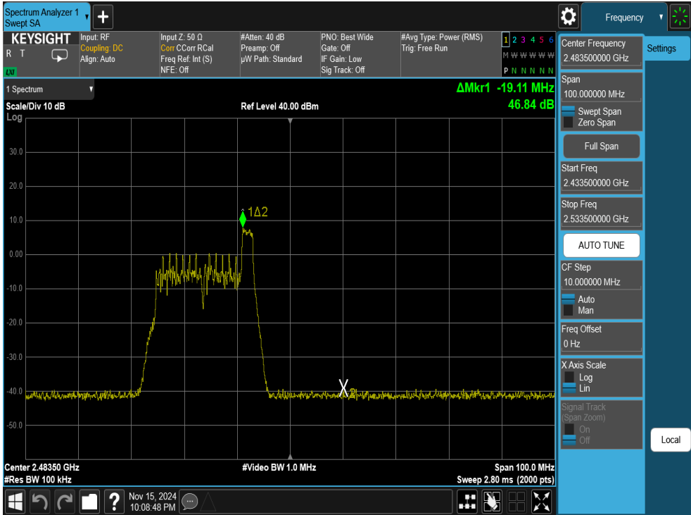
Plot 7-29. Band Edge Antenna WF2b (802.11ax OFDMA – RU26 Index 8 – Ch. 12)
