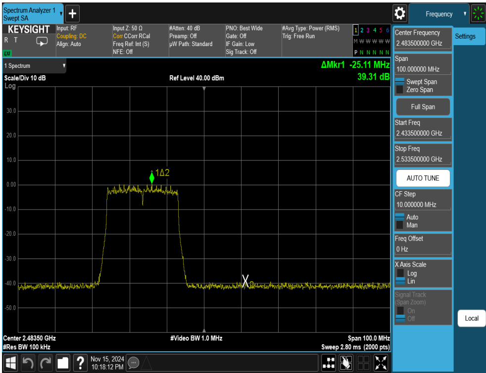
Plot 7-42. Band Edge Antenna WF2b (802.11ax OFDMA – RU242 – Ch. 12)
