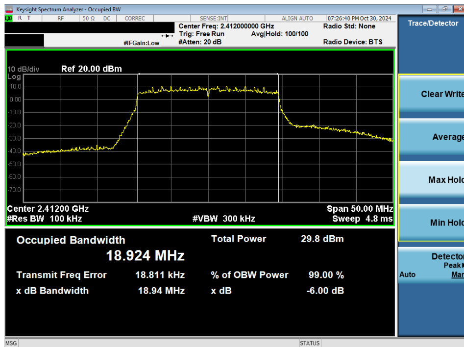
Plot 7-8. 6 dB BW and 99% OBW Plot Antenna WF2b (802.11ax SU – Ch. 1)
