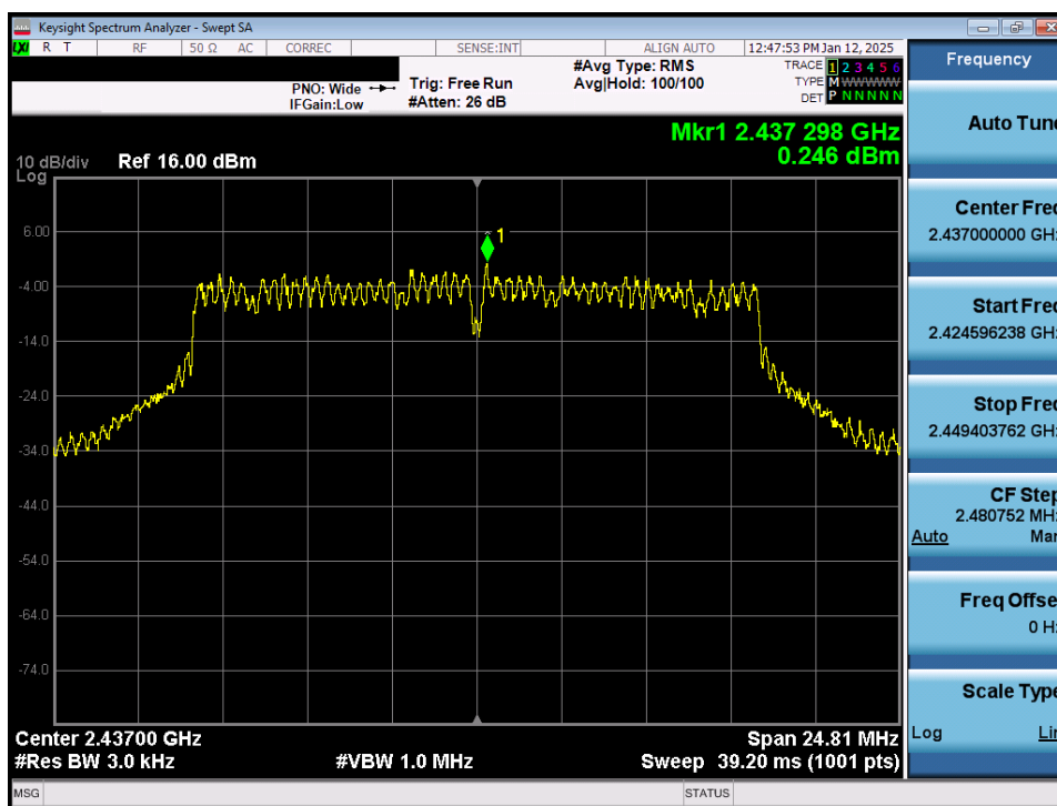
Plot 7-10. Power Spectral Density Plot Antenna WF7b (802.11g – Ch. 6)
