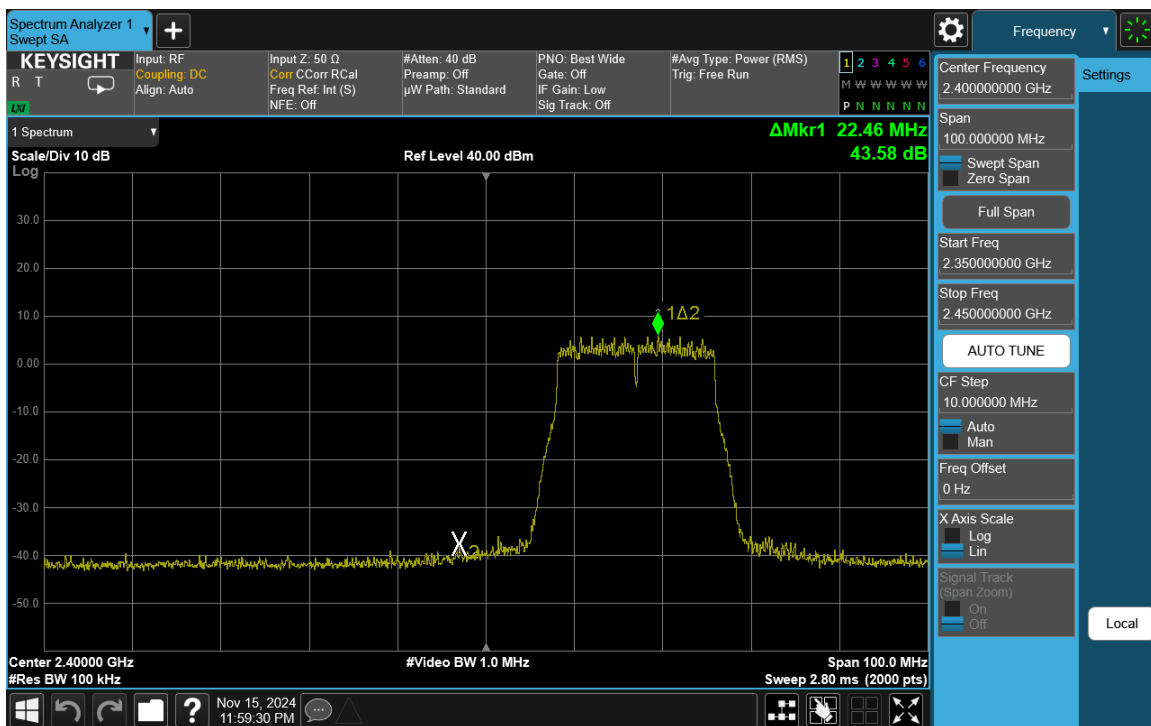
Plot 7-67. Band Edge Plot Antenna WF2b (802.11n (2.4GHz) – Ch. 2)
