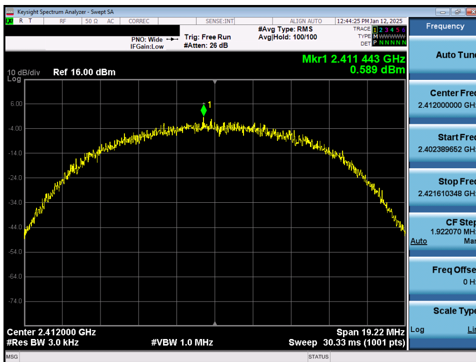
Plot 7-9. Power Spectral Density Plot Antenna WF7b (802.11b – Ch. 1)
