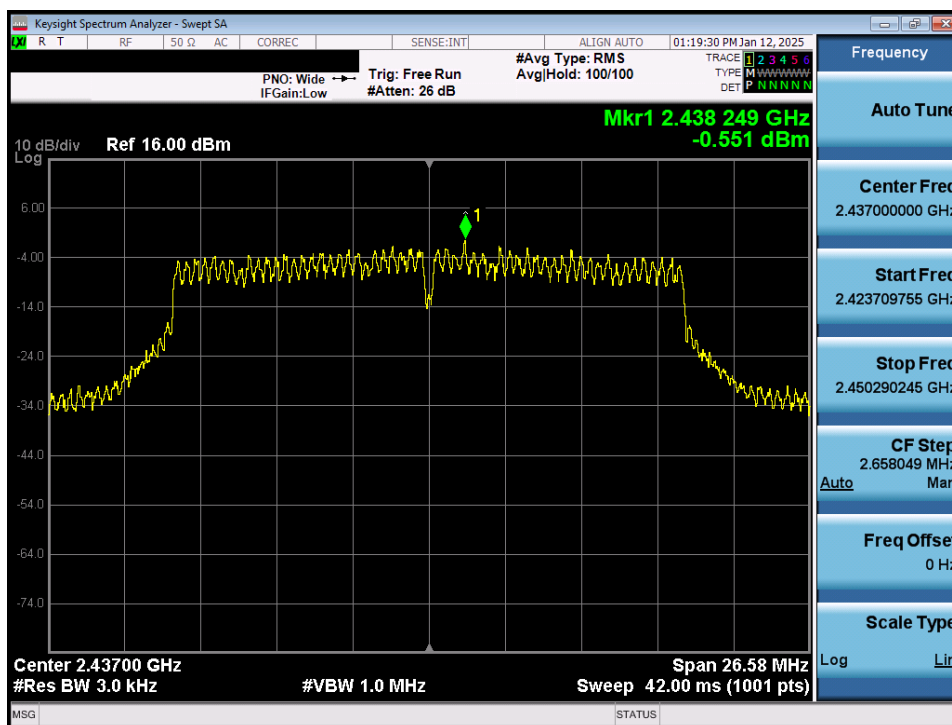
Plot 7-19. Power Spectral Density Plot CDD Antenna WF7b (802.11n – Ch. 6)
