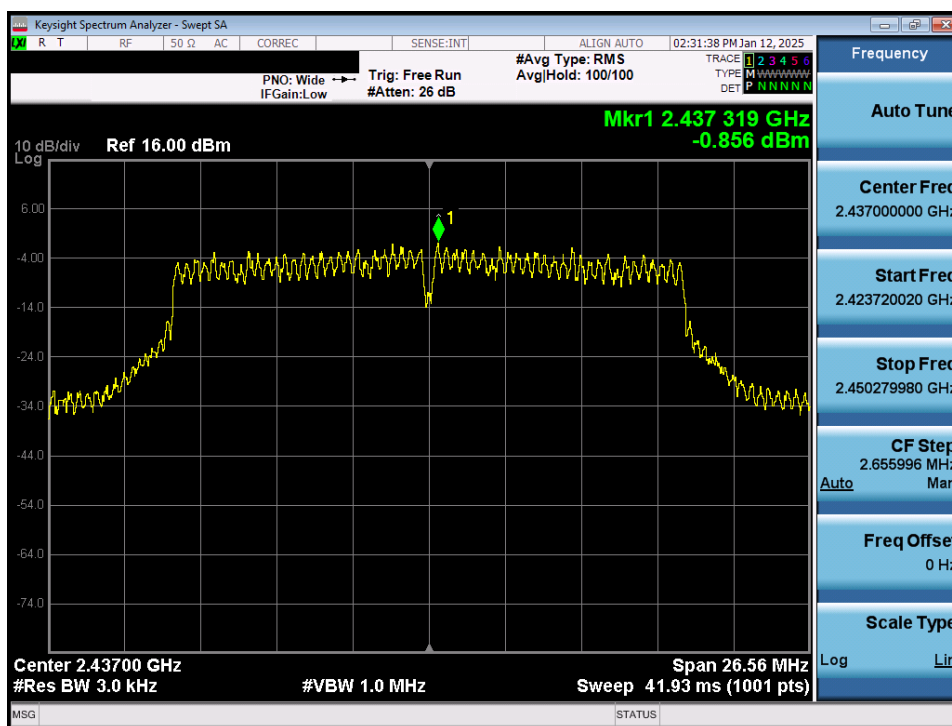
Plot 7-20. Power Spectral Density Plot CDD Antenna WF2b (802.11n – Ch. 6)
