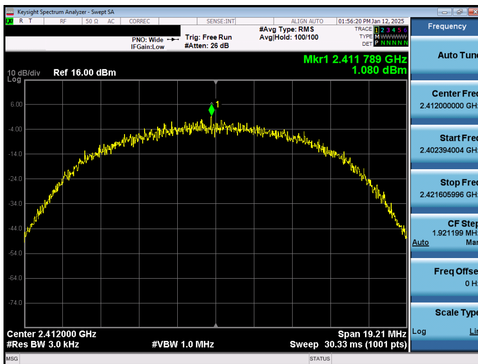
Plot 7-13. Power Spectral Density Plot Antenna WF2b (802.11b – Ch. 1)
