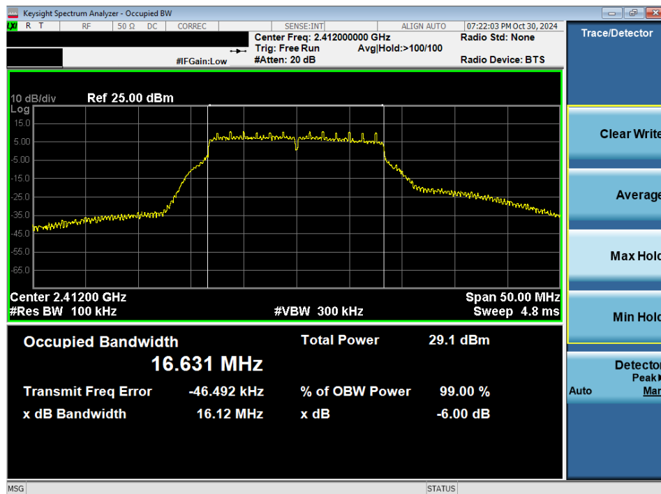
Plot 7-6. 6 dB BW and 99% OBW Plot Antenna WF2b (802.11g – Ch. 1)
