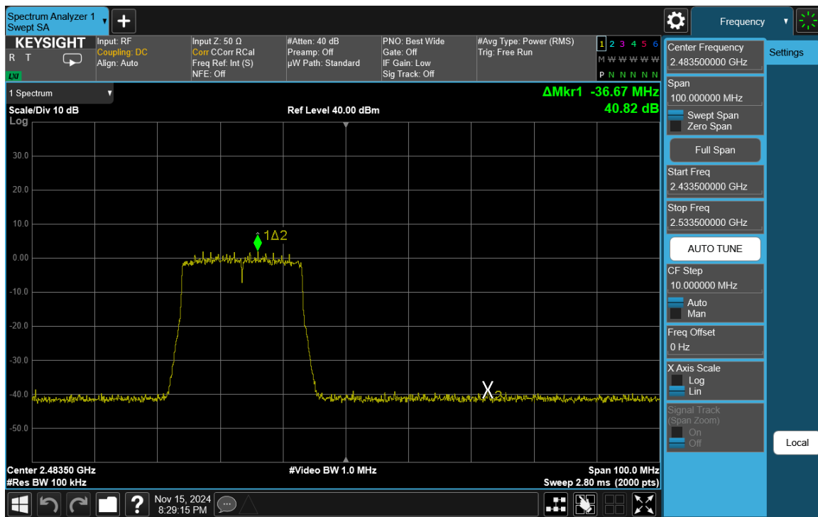
Plot 7-53. Band Edge Plot Antenna WF7b (802.11ax (SU - 2.4GHz) – Ch. 12)
