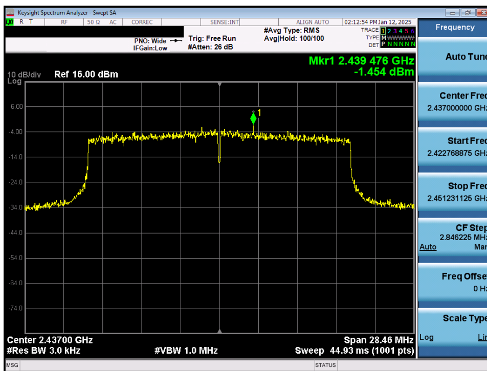
Plot 7-16. Power Spectral Density Plot Antenna WF2b (802.11ax SU – Ch. 6)
