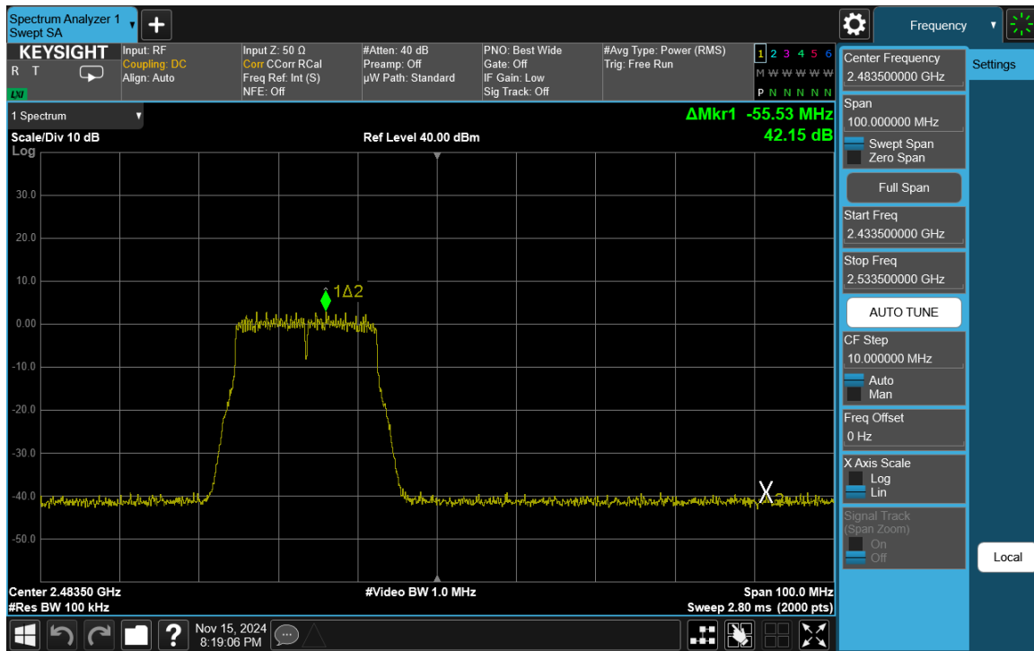
Plot 7-41. Band Edge Plot Antenna WF7b (802.11n (2.4GHz) - Ch. 12)
