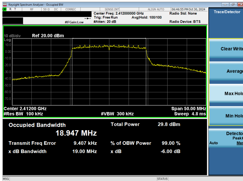
Plot 7-4. 6 dB BW and 99% OBW Plot Antenna WF7b (802.11ax SU – Ch. 1)
