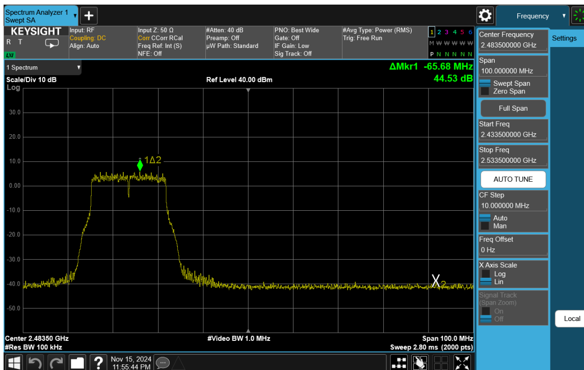
Plot 7-62. Band Edge Plot Antenna WF2b (802.11g – Ch. 10)
