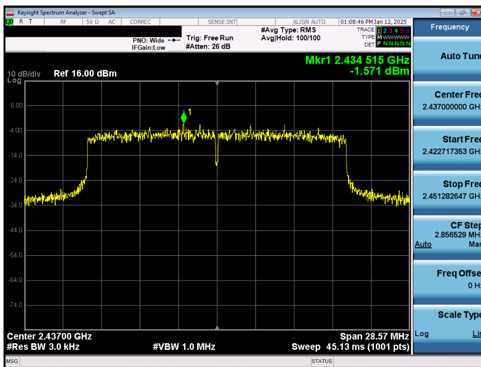
Plot 7-12. Power Spectral Density Plot Antenna WF7b (802.11ax SU – Ch. 6)
