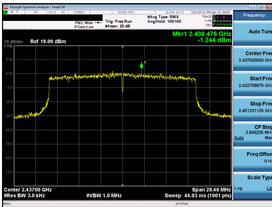
Plot 7-22. Power Spectral Density Plot CDD Antenna WF2b (802.11ax SU – Ch. 6)
