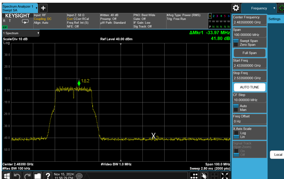
Plot 7-63. Band Edge Plot Antenna WF2b (802.11g – Ch. 11)
