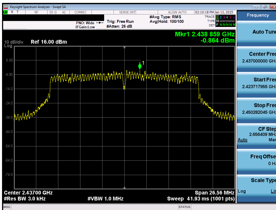
Plot 7-15. Power Spectral Density Plot Antenna WF2b (802.11n – Ch. 6)
