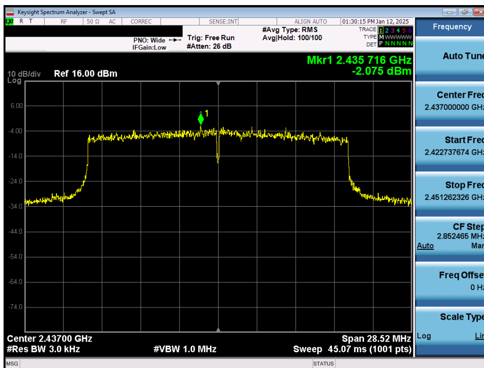
Plot 7-21. Power Spectral Density Plot CDD Antenna WF7b (802.11ax SU – Ch. 6)
