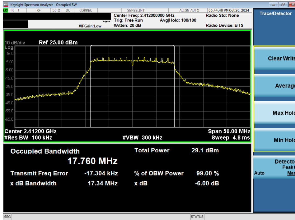
Plot 7-3. 6 dB BW and 99% OBW Plot Antenna WF7b (802.11n – Ch. 1)
