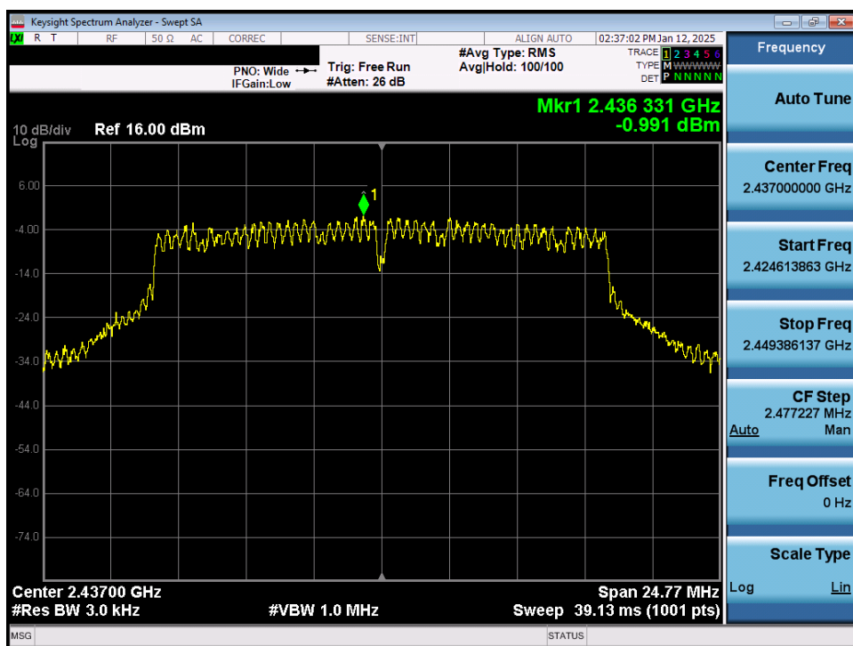
Plot 7-18. Power Spectral Density Plot CDD Antenna WF2b (802.11g – Ch. 6)
