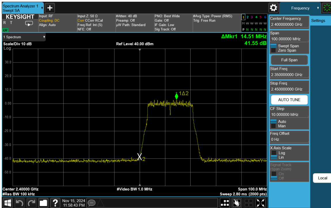
Plot 7-66. Band Edge Plot Antenna WF2b (802.11n (2.4GHz) – Ch. 1)
