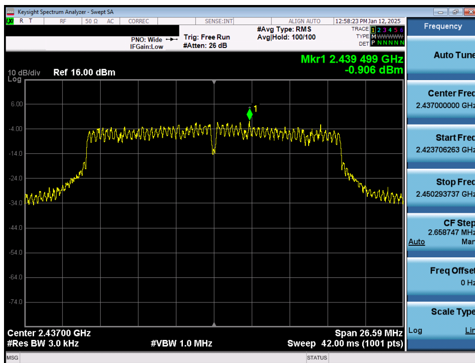
Plot 7-11. Power Spectral Density Plot Antenna WF7b (802.11n – Ch. 6)
