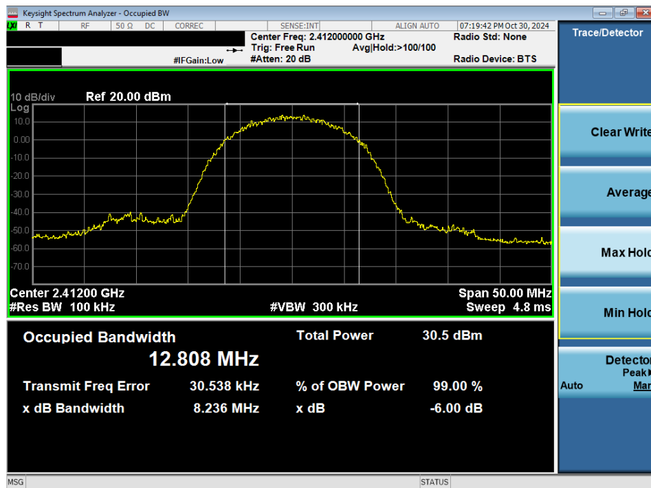
Plot 7-5. 6 dB BW and 99% OBW Plot Antenna WF2b (802.11b – Ch. 1)
