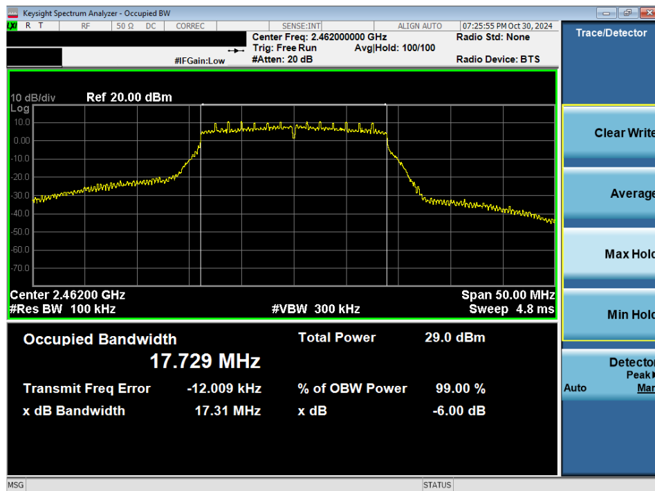
Plot 7-7. 6 dB BW and 99% OBW Plot Antenna WF2b (802.11n – Ch. 11)
