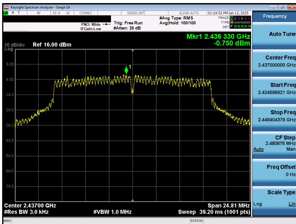
Plot 7-17. Power Spectral Density Plot CDD Antenna WF7b (802.11g – Ch. 6)
