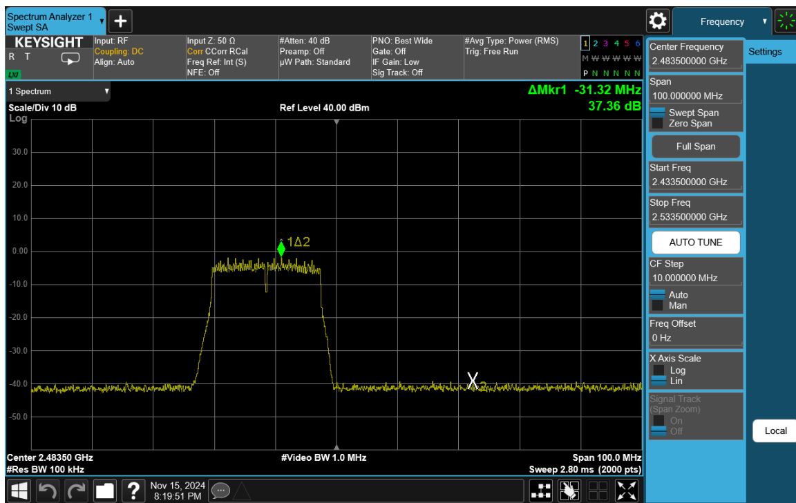
Plot 7-42. Band Edge Plot Antenna WF7b (802.11n (2.4GHz) - Ch. 13)
