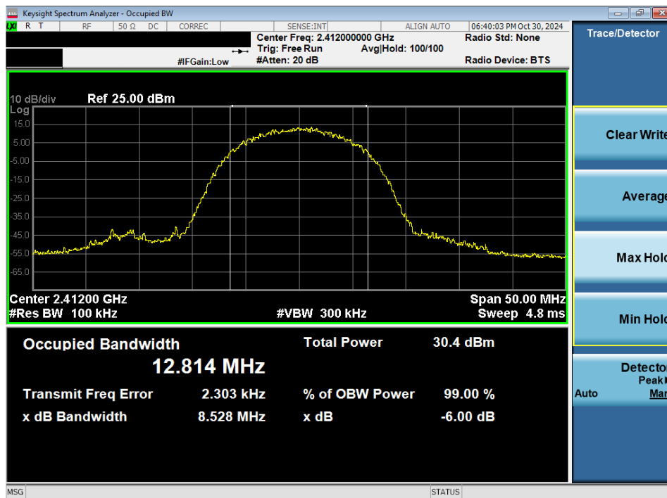
Plot 7-1. 6 dB BW and 99% OBW Plot Antenna WF7b (802.11b – Ch. 1)
