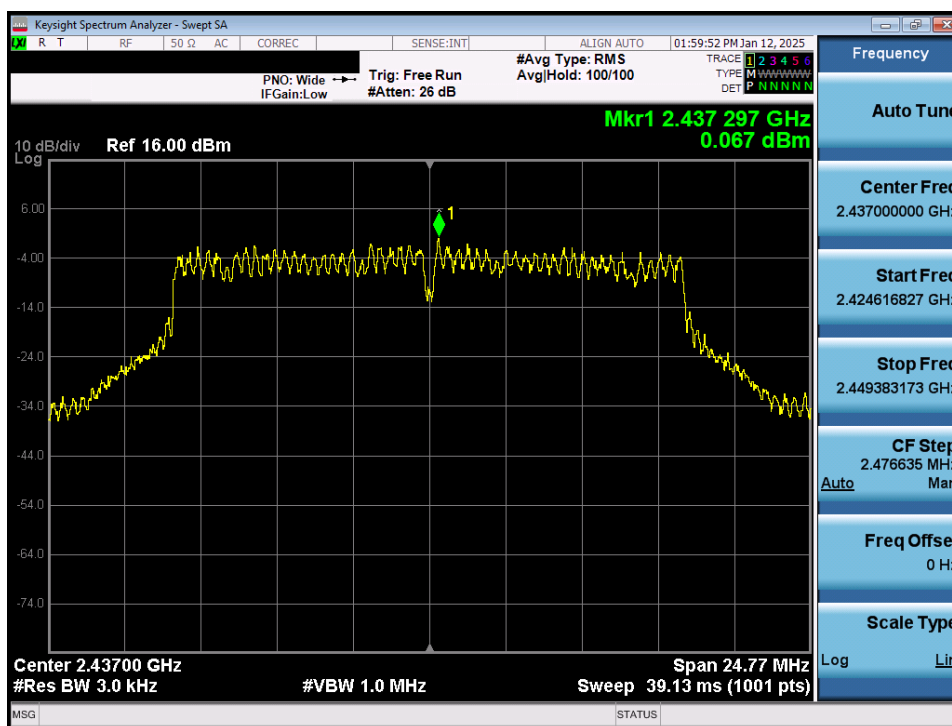
Plot 7-14. Power Spectral Density Plot Antenna WF2b (802.11g – Ch. 6)
