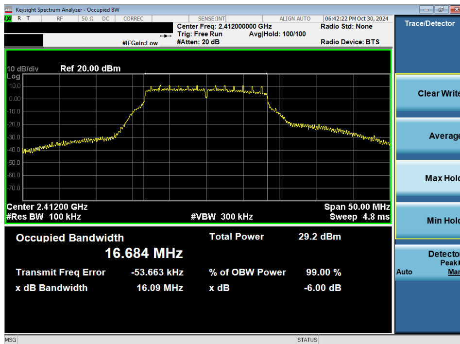
Plot 7-2. 6 dB BW and 99% OBW Plot Antenna WF7b (802.11g – Ch. 1)
