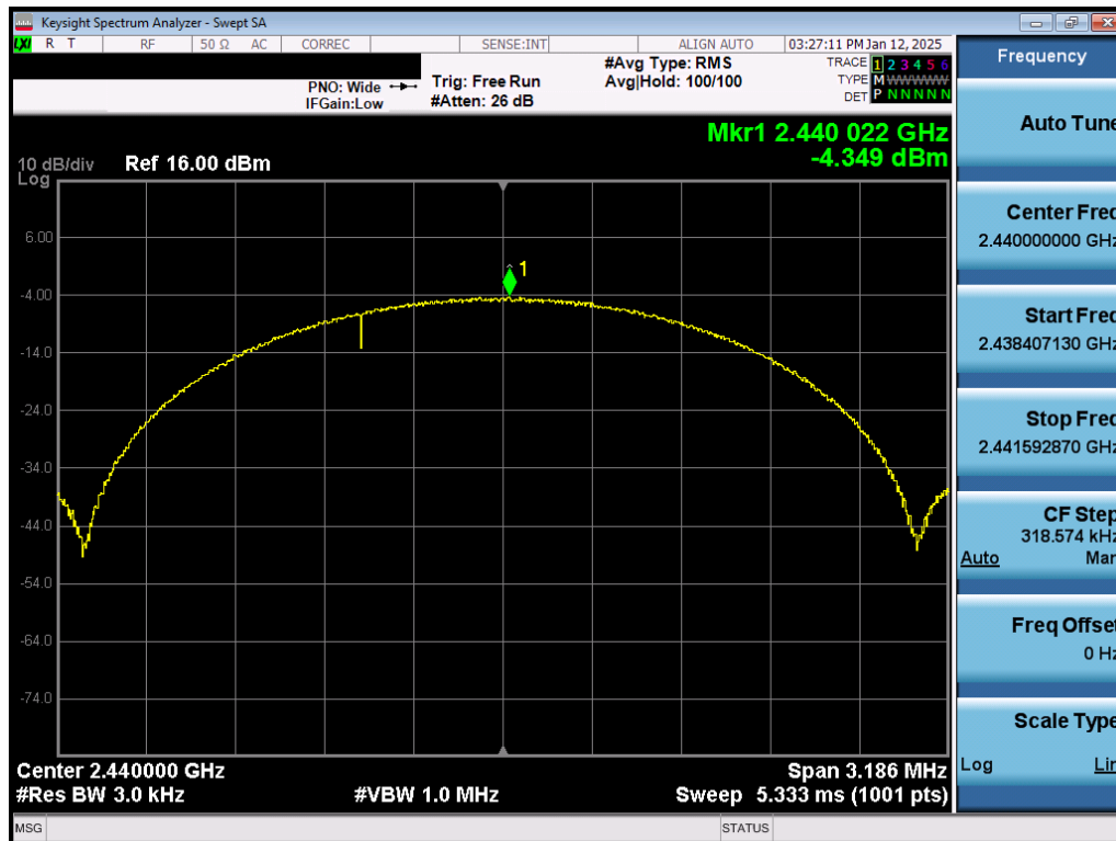
Plot 7-52. Power Spectral Density Plot Antenna WF2b (Bluetooth (LE), 2Mbps, ePA – Ch. 19)
