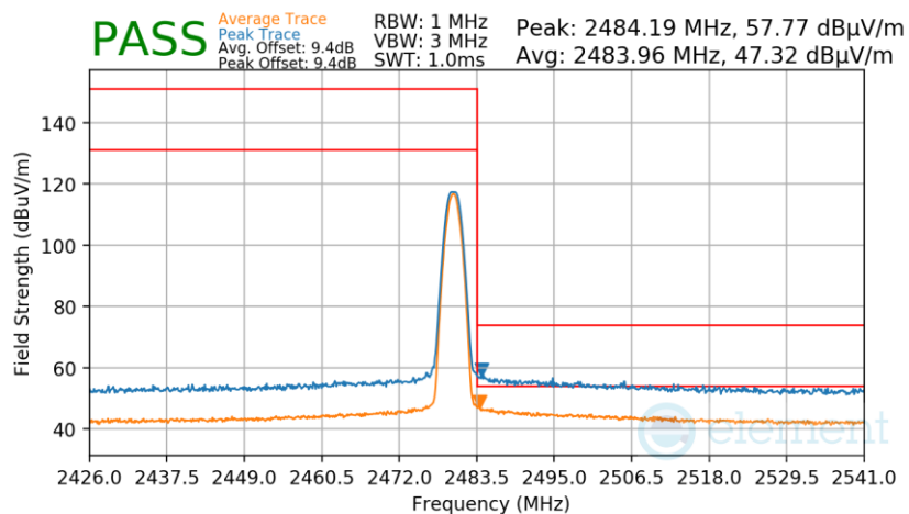
Plot 7-86. Radiated Restricted Upper Band Edge Measurement Antenna WF7b (Average & Peak)
