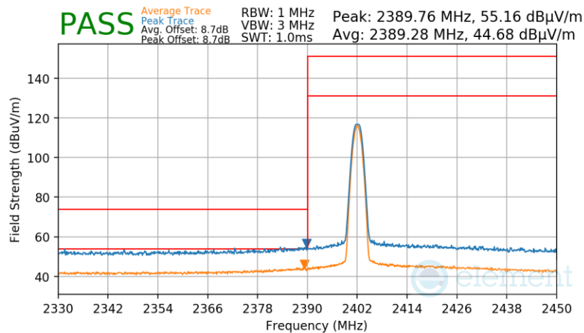
Plot 7-89. Radiated Restricted Lower Band Edge Measurement Antenna WF2b (Average & Peak)
