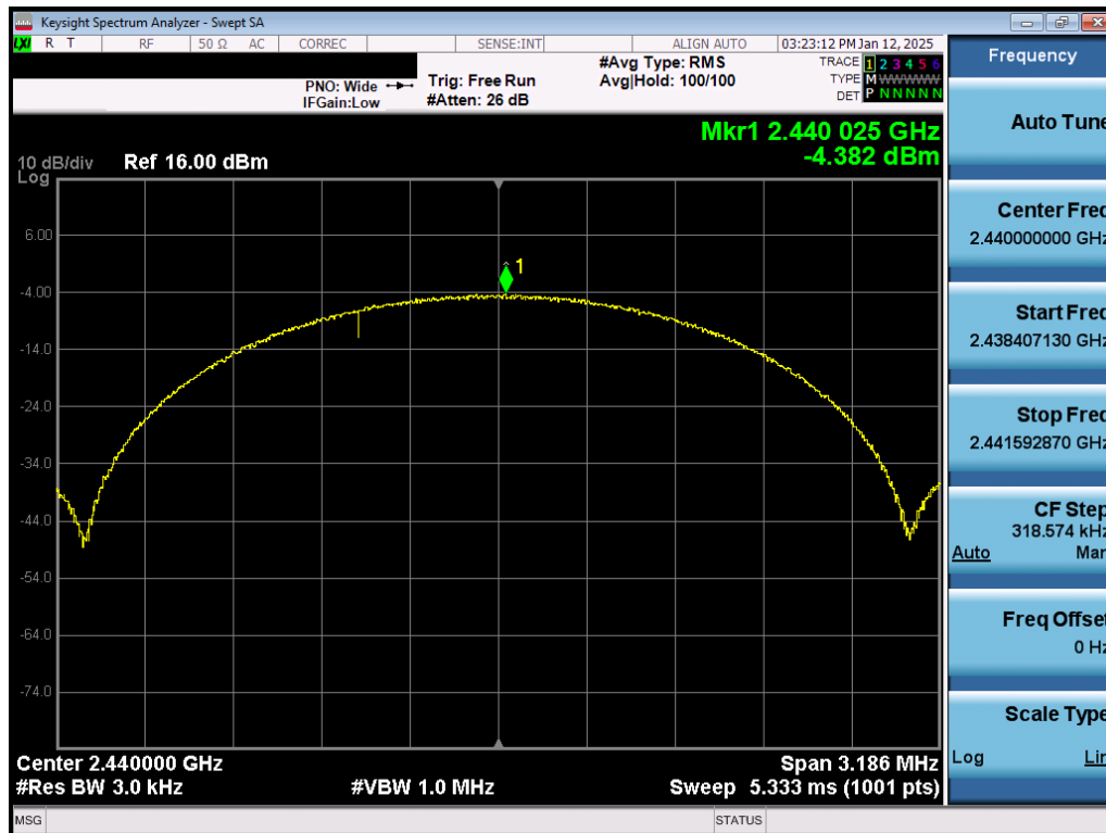
Plot 7-32. Power Spectral Density Plot Antenna WF2b (Bluetooth (LE), 2Mbps, ePA – Ch. 19)
