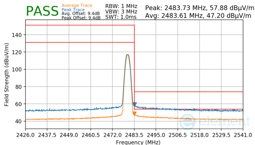
Plot 7-90. Radiated Restricted Upper Band Edge Measurement Antenna WF2b (Average & Peak)
