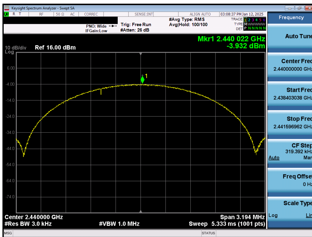
Plot 7-51. Power Spectral Density Plot Antenna WF7b (Bluetooth (LE), 2Mbps, ePA – Ch. 19)
