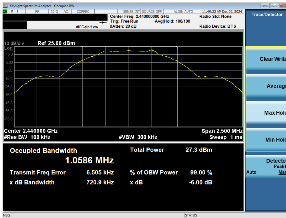
Plot 7-8. 6dB BW & 99% OBW Plot Antenna WF2b (Bluetooth (LE), 1Mbps, ePA – Ch. 19)
