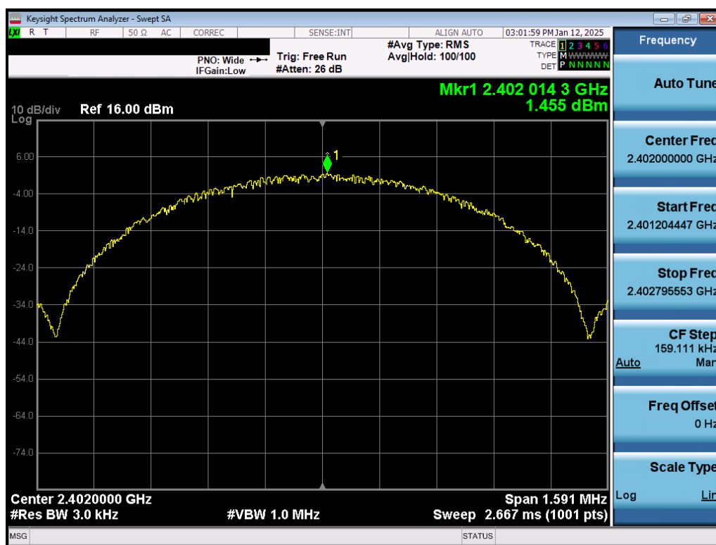
Plot 7-13. Power Spectral Density Plot Antenna WF7b (Bluetooth (LE), 1Mbps, ePA – Ch. 0)
