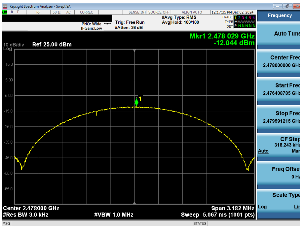
Plot 7-60. Power Spectral Density Plot Antenna WF2b (Bluetooth (LE), 2Mbps, iPA – Ch. 38)
