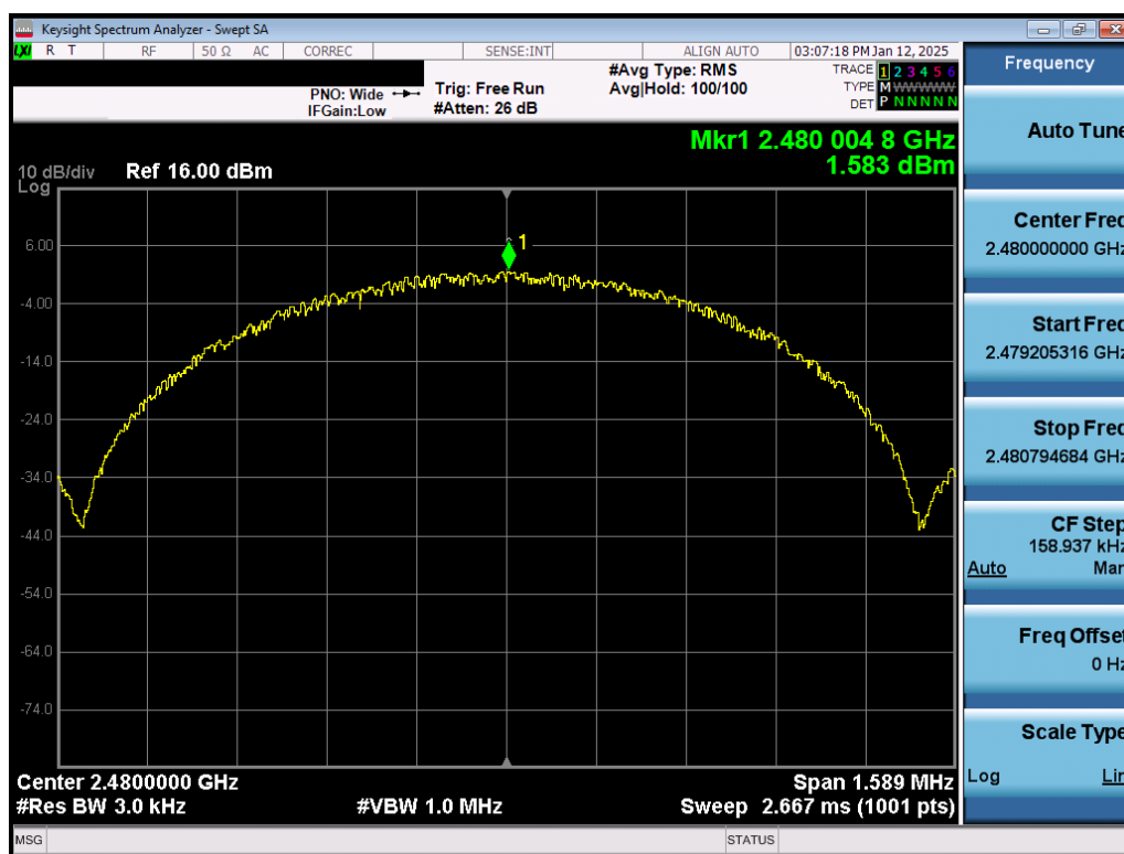
Plot 7-41. Power Spectral Density Plot Antenna WF7b (Bluetooth (LE), 1Mbps, ePA – Ch. 39)
