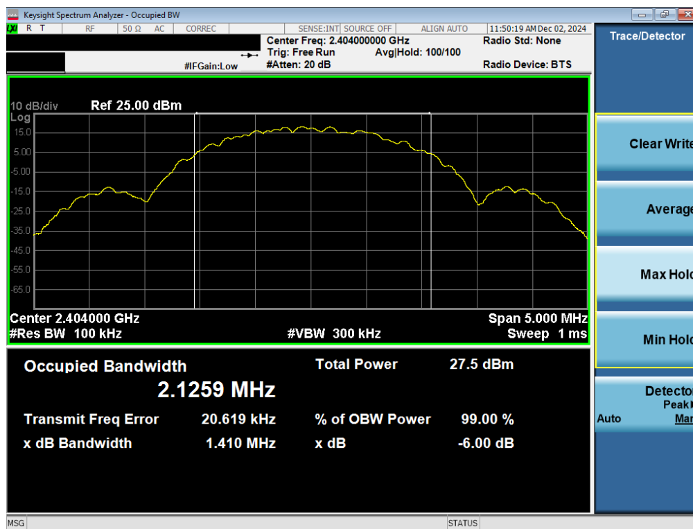
Plot 7-10. 6dB BW & 99% OBW Plot Antenna WF2b (Bluetooth (LE), 2Mbps, ePA – Ch. 1)
