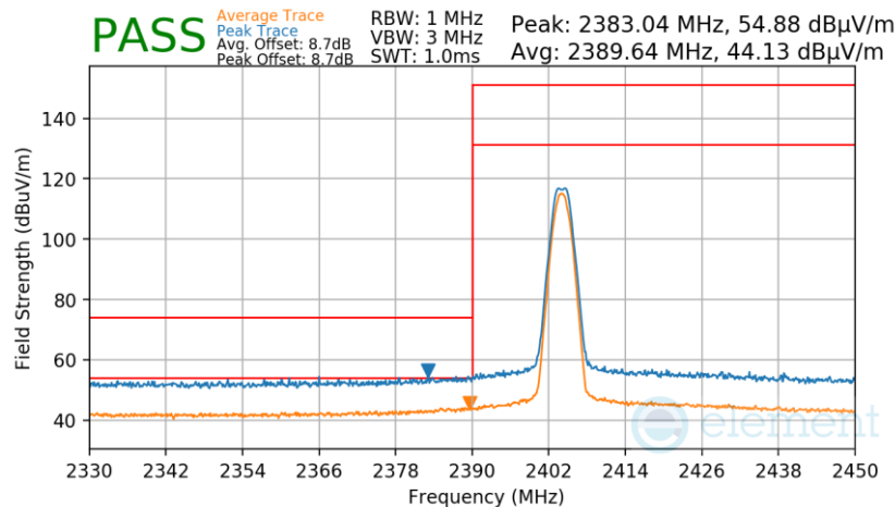
Plot 7-91. Radiated Restricted Lower Band Edge Measurement Antenna WF2b (Average & Peak)
