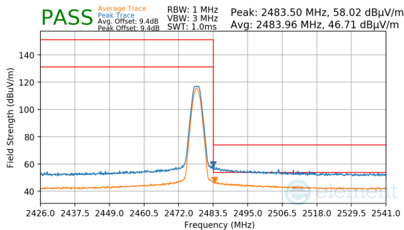
Plot 7-92. Radiated Restricted Upper Band Edge Measurement Antenna WF2b (Average & Peak)
