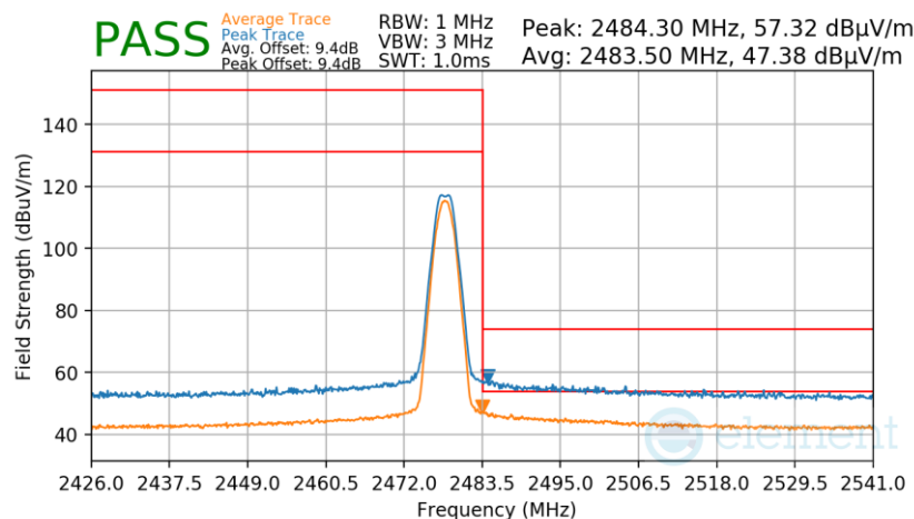
Plot 7-88. Radiated Restricted Upper Band Edge Measurement Antenna WF7b (Average & Peak)
