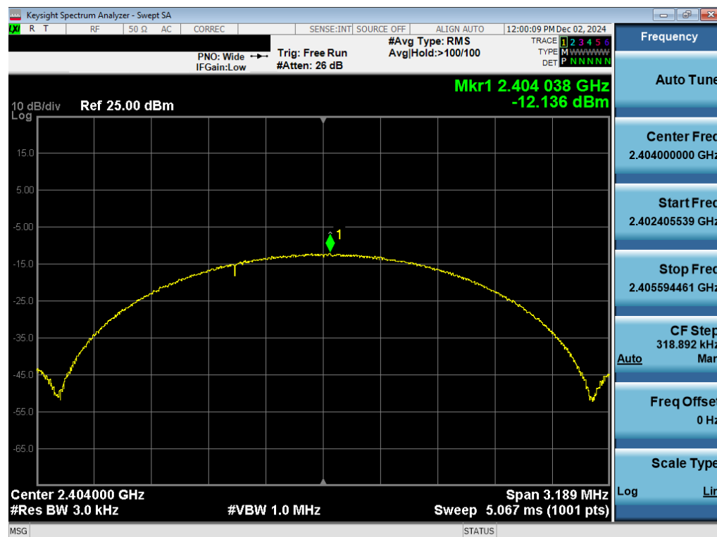
Plot 7-34. Power Spectral Density Plot Antenna WF2b (Bluetooth (LE), 2Mbps, iPA – Ch. 1)
