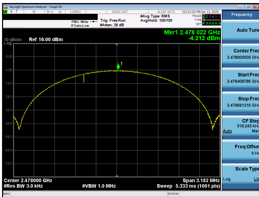
Plot 7-33. Power Spectral Density Plot Antenna WF2b (Bluetooth (LE), 2Mbps, ePA – Ch. 38)
