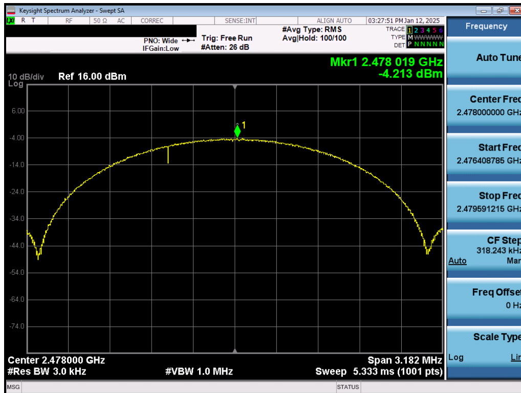
Plot 7-54. Power Spectral Density Plot Antenna WF2b (Bluetooth (LE), 2Mbps, ePA – Ch. 38)
