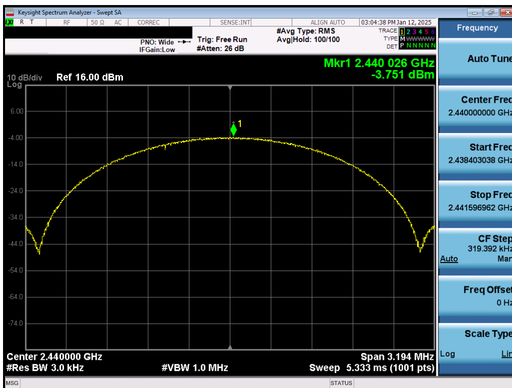
Plot 7-20. Power Spectral Density Plot Antenna WF7b (Bluetooth (LE), 2Mbps, ePA – Ch. 19)
