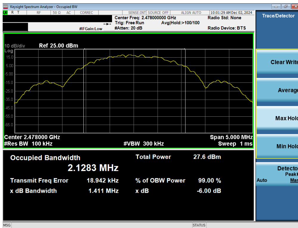
Plot 7-6. 6dB BW & 99% OBW Plot Antenna WF7b (Bluetooth (LE), 2Mbps, ePA – Ch. 38)
