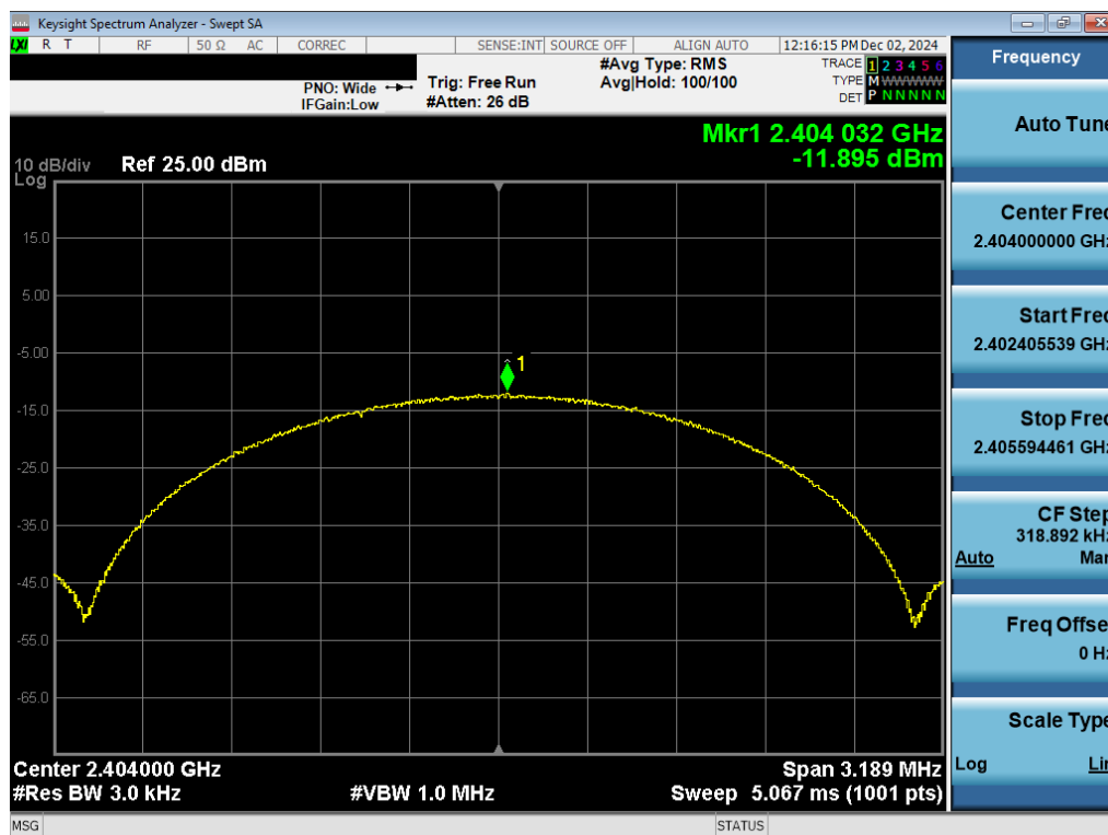
Plot 7-56. Power Spectral Density Plot Antenna WF2b (Bluetooth (LE), 2Mbps, iPA – Ch. 1)
