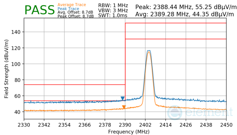
Plot 7-87. Radiated Restricted Lower Band Edge Measurement Antenna WF7b (Average & Peak)
