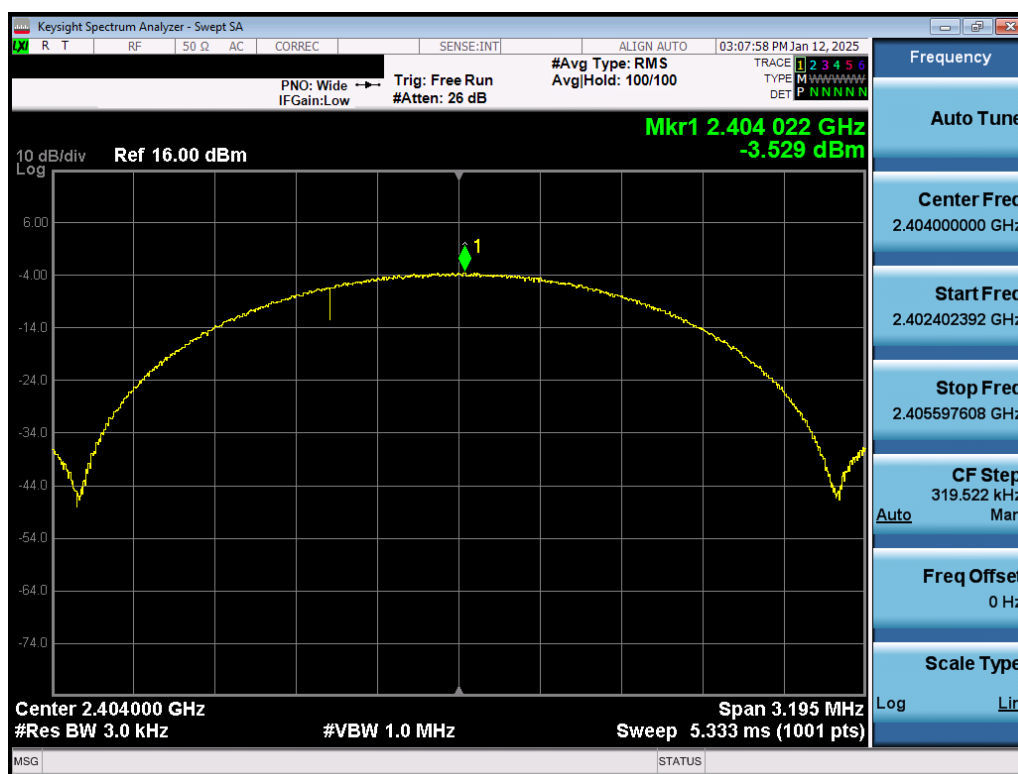
Plot 7-49. Power Spectral Density Plot Antenna WF7b (Bluetooth (LE), 2Mbps, ePA – Ch. 1)
