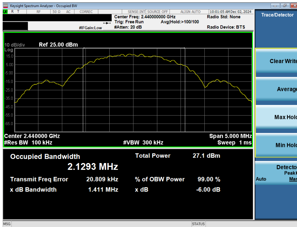
Plot 7-5. 6dB BW & 99% OBW Plot Antenna WF7b (Bluetooth (LE), 2Mbps, ePA – Ch. 19)
