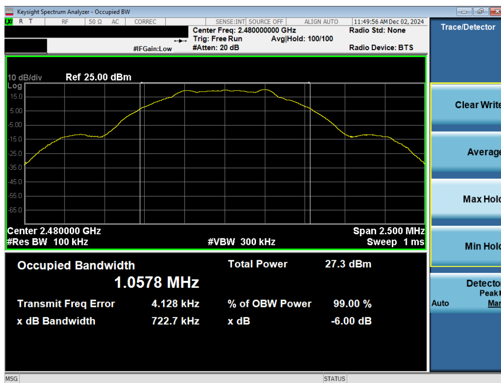
Plot 7-9. 6dB BW & 99% OBW Plot Antenna WF2b (Bluetooth (LE), 1Mbps, ePA – Ch. 39)
