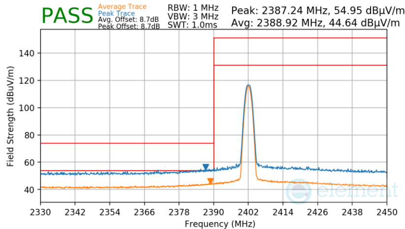
Plot 7-85. Radiated Restricted Lower Band Edge Measurement Antenna WF7b (Average & Peak)
