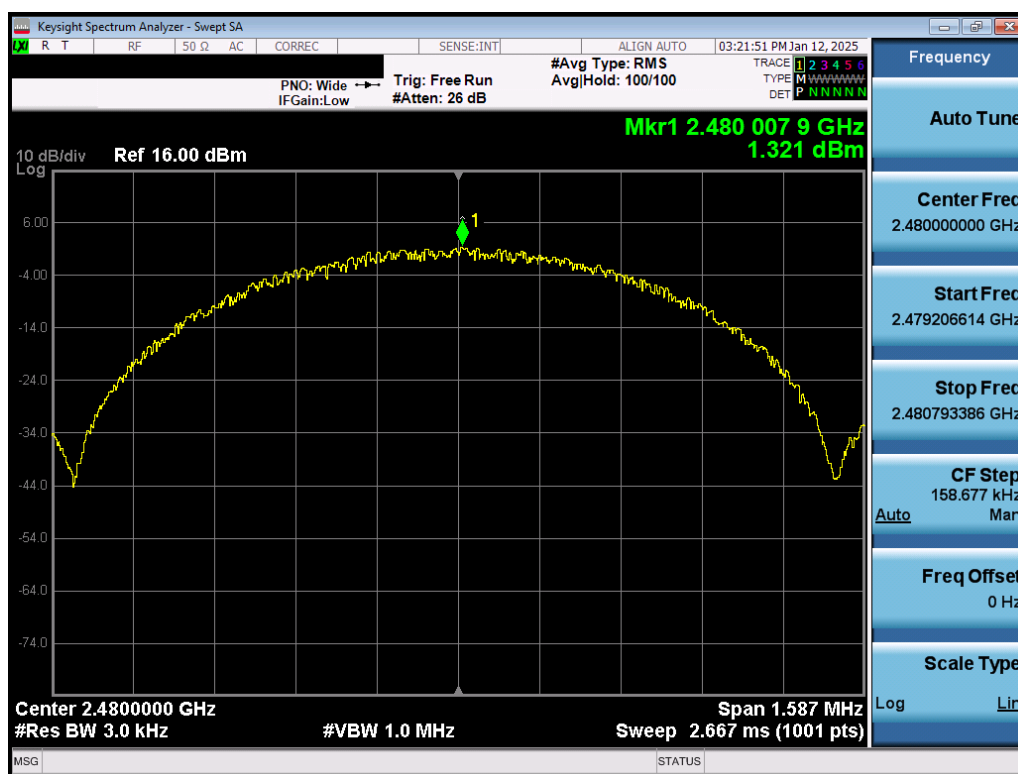
Plot 7-27. Power Spectral Density Plot Antenna WF2b (Bluetooth (LE), 1Mbps, ePA – Ch. 39)
