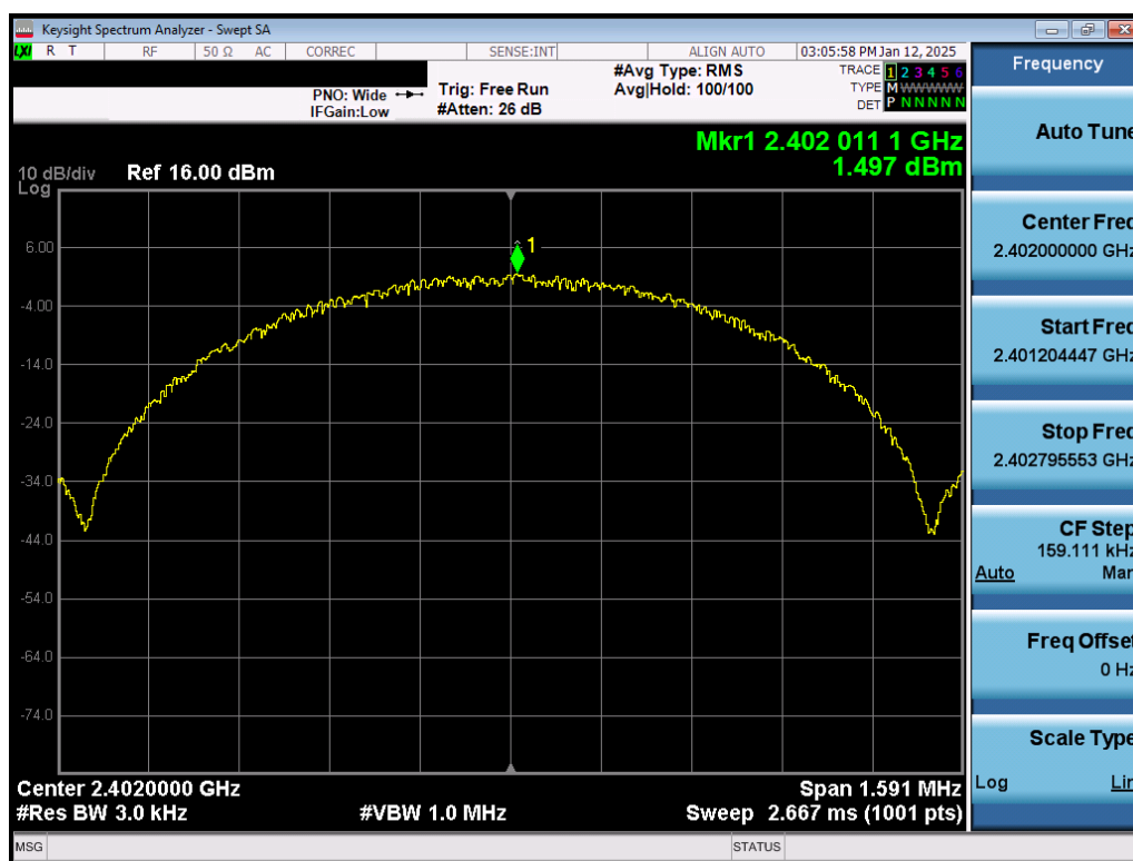
Plot 7-37. Power Spectral Density Plot Antenna WF7b (Bluetooth (LE), 1Mbps, ePA – Ch. 0)
