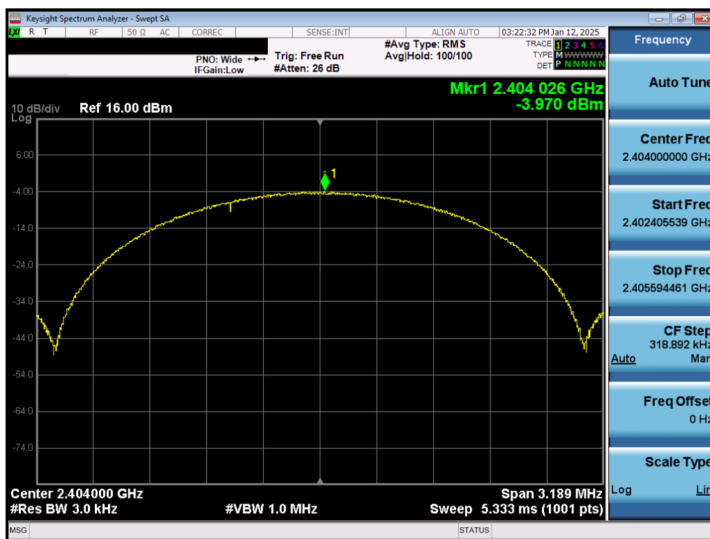
Plot 7-31. Power Spectral Density Plot Antenna WF2b (Bluetooth (LE), 2Mbps, ePA – Ch. 1)
