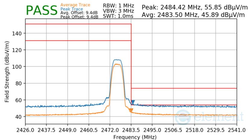
Plot 7-92. Radiated Restricted Upper Band Edge Measurement Antenna WF2b
