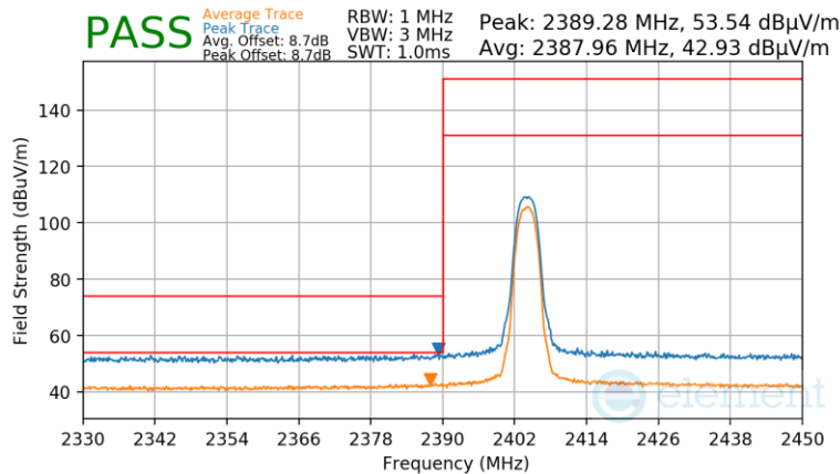
Plot 7-85. Radiated Restricted Lower Band Edge Measurement Antenna WF7b
