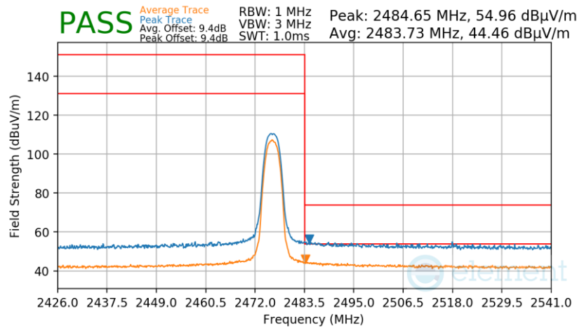
Plot 7-87. Radiated Restricted Upper Band Edge Measurement Antenna WF7b
