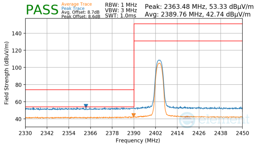
Plot 7-89. Radiated Restricted Lower Band Edge Measurement Antenna WF2b
