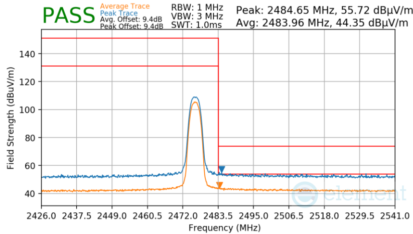
Plot 7-91. Radiated Restricted Upper Band Edge Measurement Antenna WF2b
