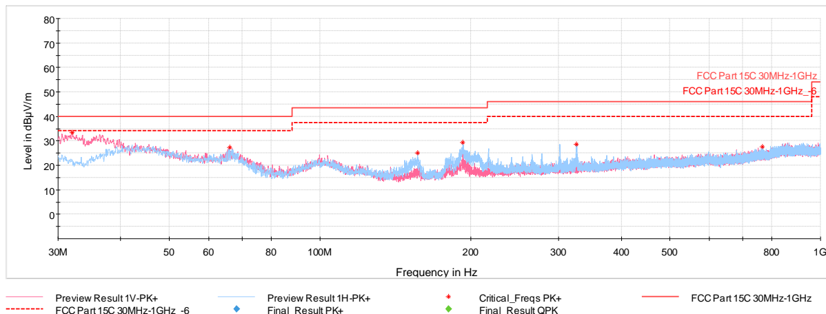
Plot 7-97. Radiated Spurious Emissions Below 1GHz TxBF (4Mbps, ePA – Ch.38 with AC/DC Adapter via USB-C cable with wire charger)
