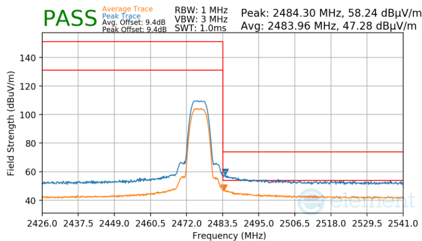
Plot 7-88. Radiated Restricted Upper Band Edge Measurement Antenna WF7b
