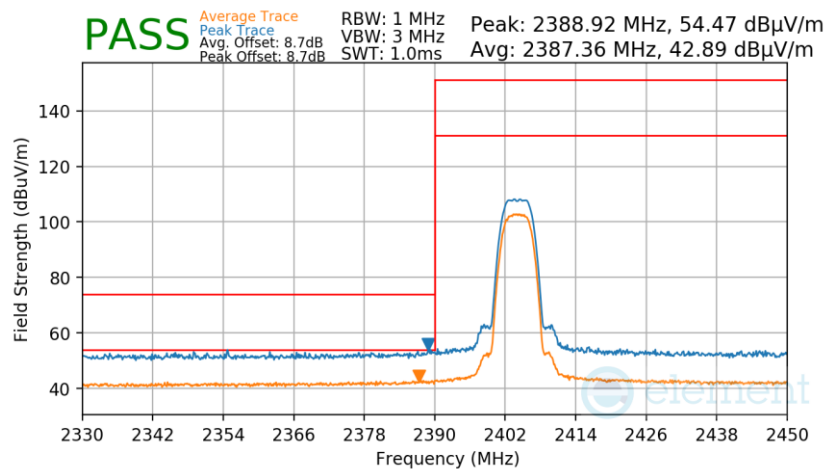
Plot 7-90. Radiated Restricted Lower Band Edge Measurement Antenna WF2b
