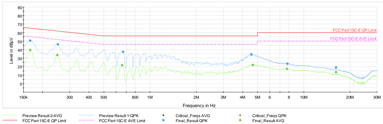
Plot 7-84. AC Line Conducted Plot with Bluetooth HDR TxBF (N, 4Mbps ePA - Ch.38 with AC/DC Adapter via USB-C cable with wire charger)
