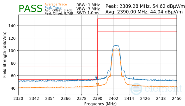
Plot 7-86. Radiated Restricted Lower Band Edge Measurement Antenna WF7b
