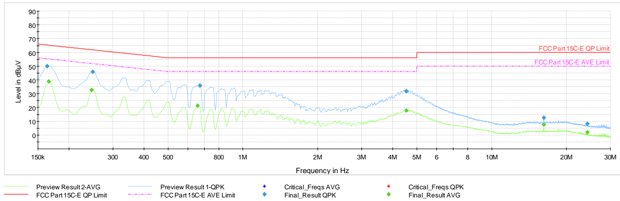
Plot 7-83. AC Line Conducted Plot with Bluetooth HDR Tx BF (L1, 4Mbps ePA - Ch.38 with AC/DC Adapter via USB-C cable with wire charger)
