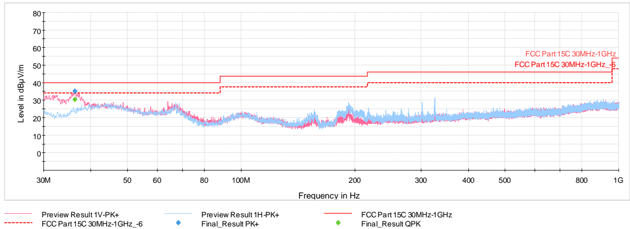
Plot 7-46. Radiated Spurious Emissions 30MHz-1GHz Antenna WF7b (ePA - Ch.25, with AC/DC Adapter via USB-C cable with wire charger)
