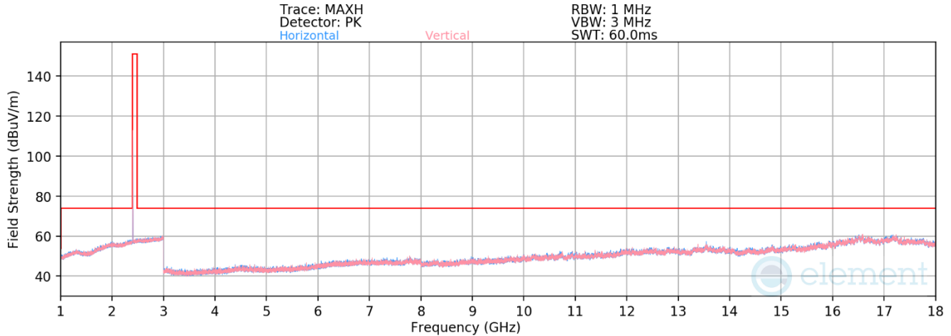
Plot 7-39. Radiated Spurious Emissions 1-18GHz Antenna WF2b (802.15.4 ePA – Ch. 11)
