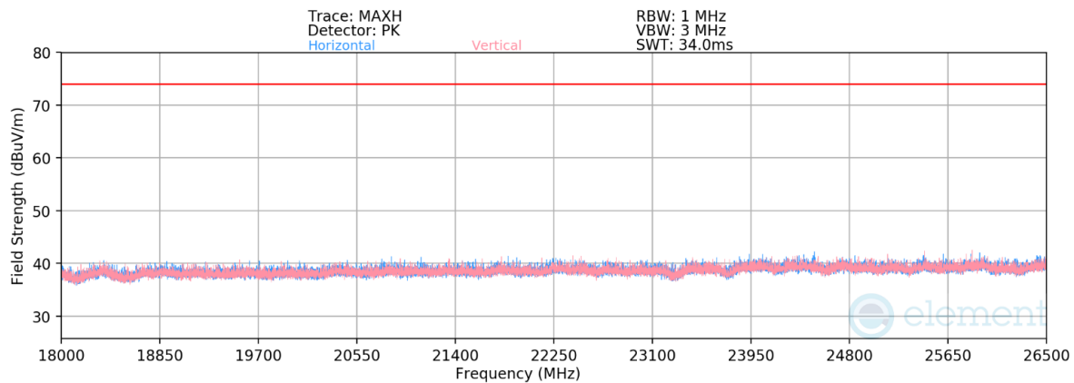
Plot 7-38. Radiated Spurious Emissions Above 18GHz Antenna WF7b (802.15.4 ePA – Ch. 25)
