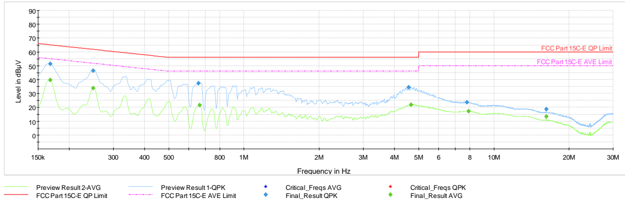
Plot 7-48. AC Line Conducted Emission with 802.15.4 Antenna WF7b (N, Ch.25 - ePA, with AC/DC Adapter via USB-C cable with wire charger)
