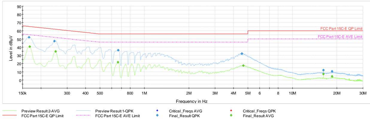
Plot 7-47. AC Line Conducted Emission with 802.15.4 Antenna WF7b (L1, Ch.25 - ePA, with AC/DC Adapter via USB-C cable with wire charger)
