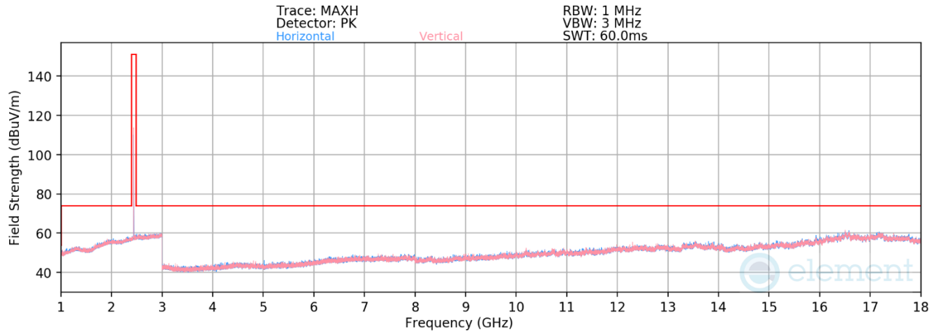
Plot 7-40. Radiated Spurious Emissions 1-18GHz Antenna WF2b (802.15.4 ePA – Ch. 18)
