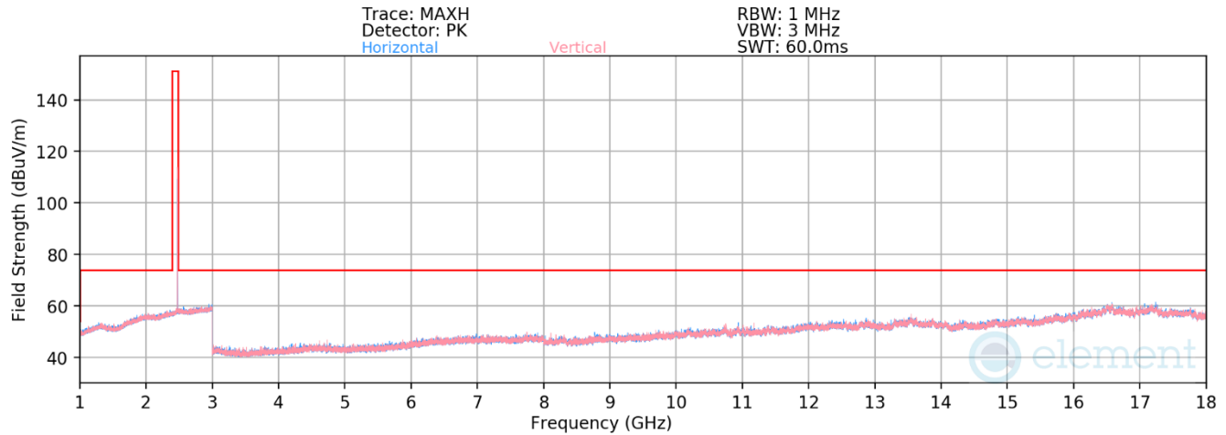
Plot 7-41. Radiated Spurious Emissions 1-18GHz Antenna WF2b (802.15.4 ePA – Ch. 25)
