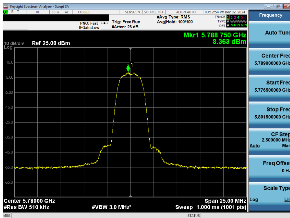
Plot 7-39. PSD Antenna WF2a (NB UNII HDR4, ePA – 5789MHz)
