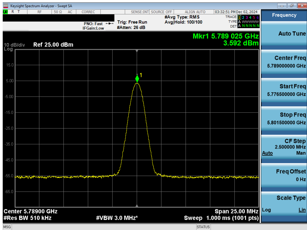
Plot 7-50. PSD Antenna WF7b (NB UNII BDR, iPA – 5789MHz)
