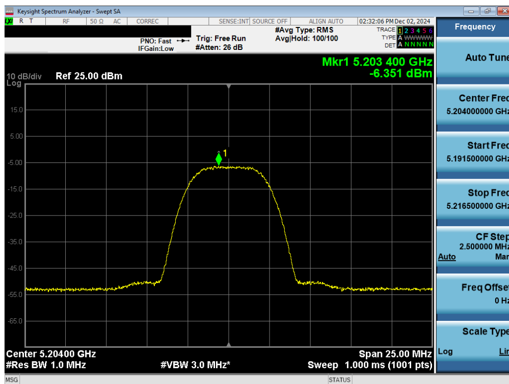
Plot 7-48. PSD Antenna WF7b (NB UNII HDR8, iPA – 5204MHz)
