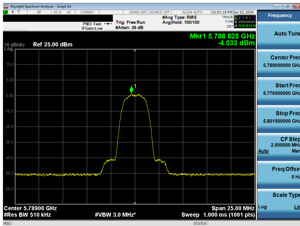
Plot 7-28. PSD Antenna WF7a (NB UNII HDR4, iPA – 5789MHz)
