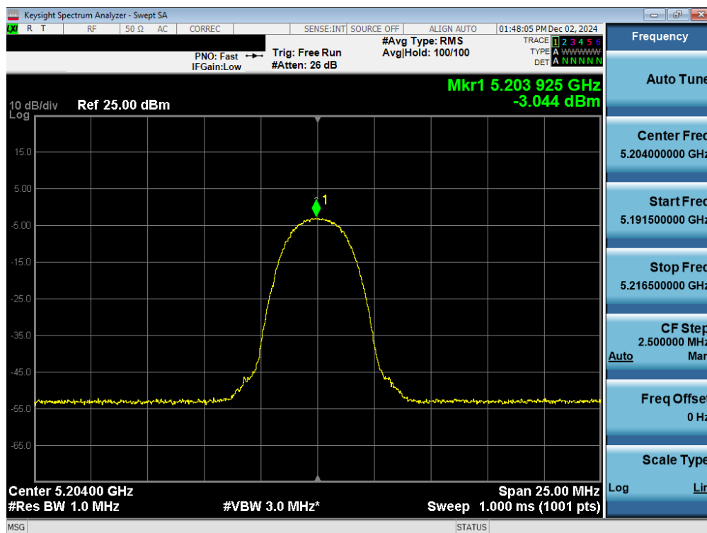
Plot 7-62. PSD TxBF Antenna WF2a (NB UNII HDR4, iPA – 5204MHz)
