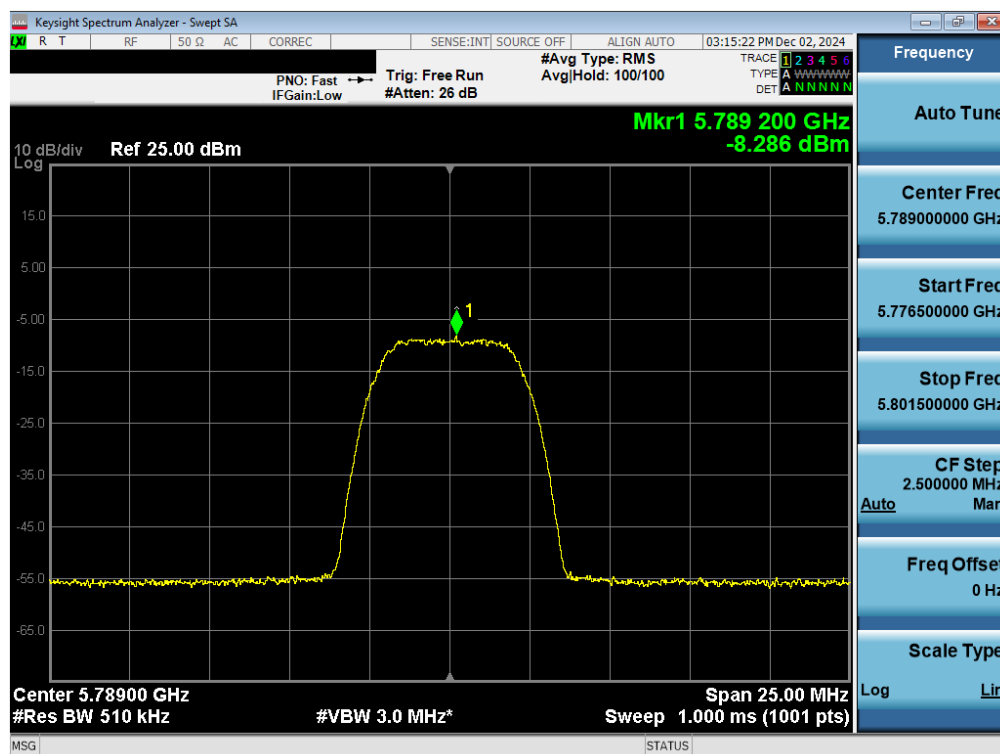
Plot 7-42. PSD Antenna WF2a (NB UNII HDR8, iPA – 5789MHz)
