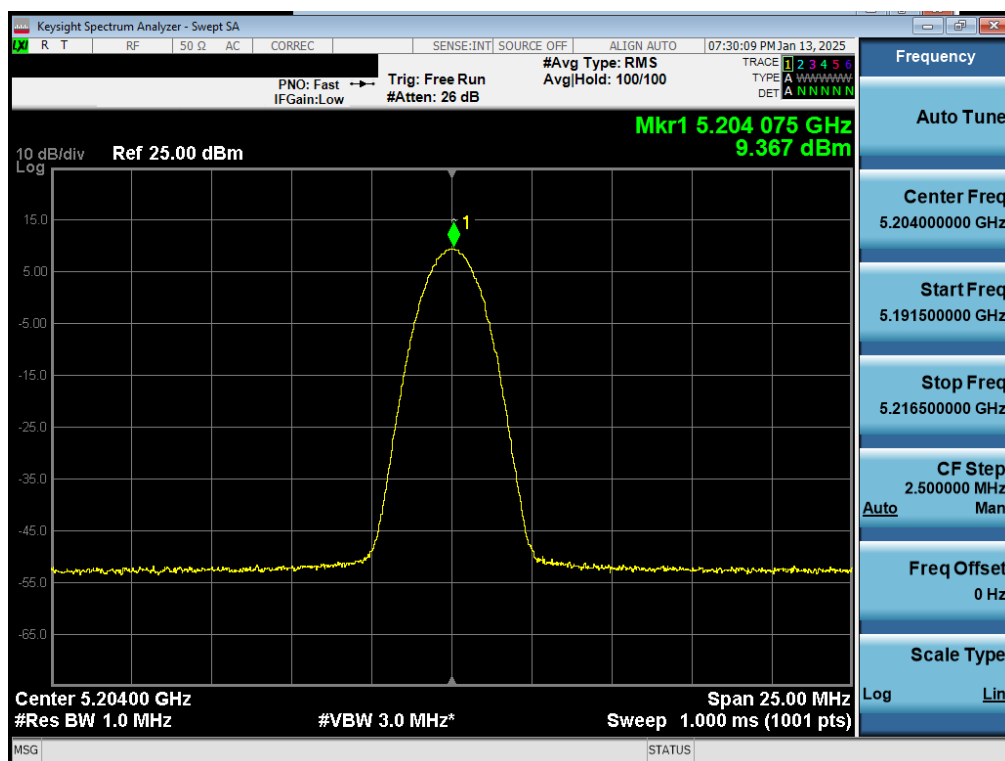
Plot 7-43. PSD Antenna WF7b (NB UNII BDR, ePA – 5204MHz)
