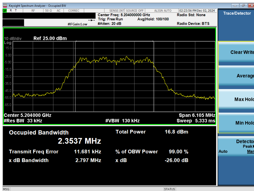
Plot 7-8. 26dB BW & 99% OBW Antenna WF7b (NB UNII HDR4, ePA- 5204MHz)
