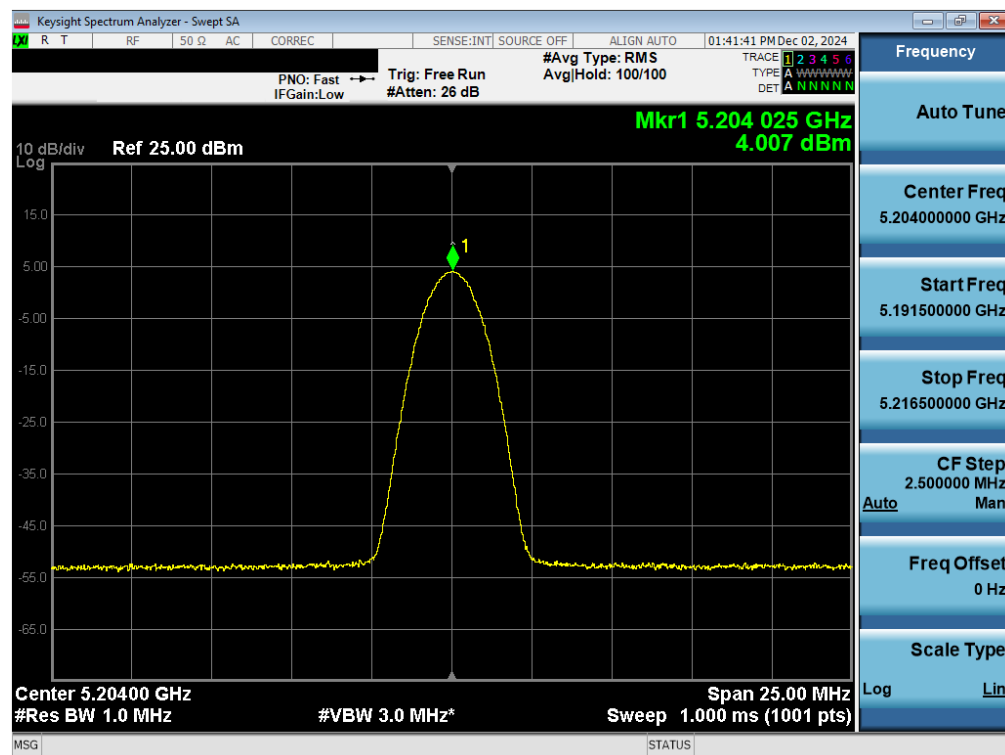
Plot 7-32. PSD Antenna WF2a (NB UNII BDR, iPA – 5204MHz)
