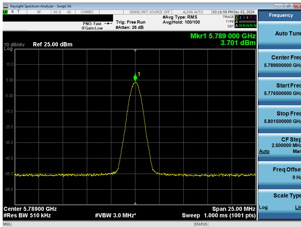
Plot 7-70. PSD TxBF Antenna WF2a (NB UNII BDR, iPA – 5789MHz)
