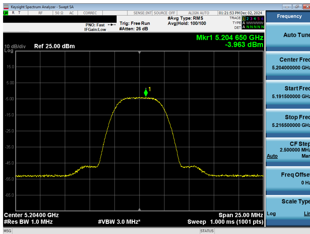
Plot 7-24. PSD Antenna WF7a (NB UNII HDR8, iPA – 5204MHz)
