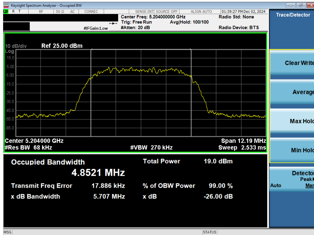
Plot 7-6. 26dB BW & 99% OBW Antenna WF2a (NB UNII HDR8, ePA- 5204MHz)
