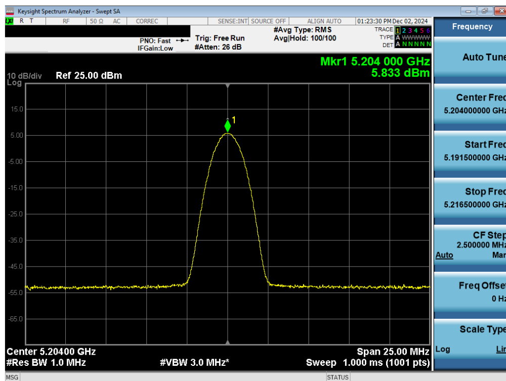
Plot 7-57. PSD TxBF Antenna WF7a (NB UNII BDR, iPA – 5204MHz)
