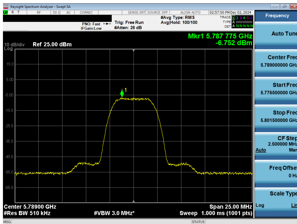
Plot 7-77. PSD TxBF Antenna WF7a (NB UNII HDR8, iPA – 5789MHz)
