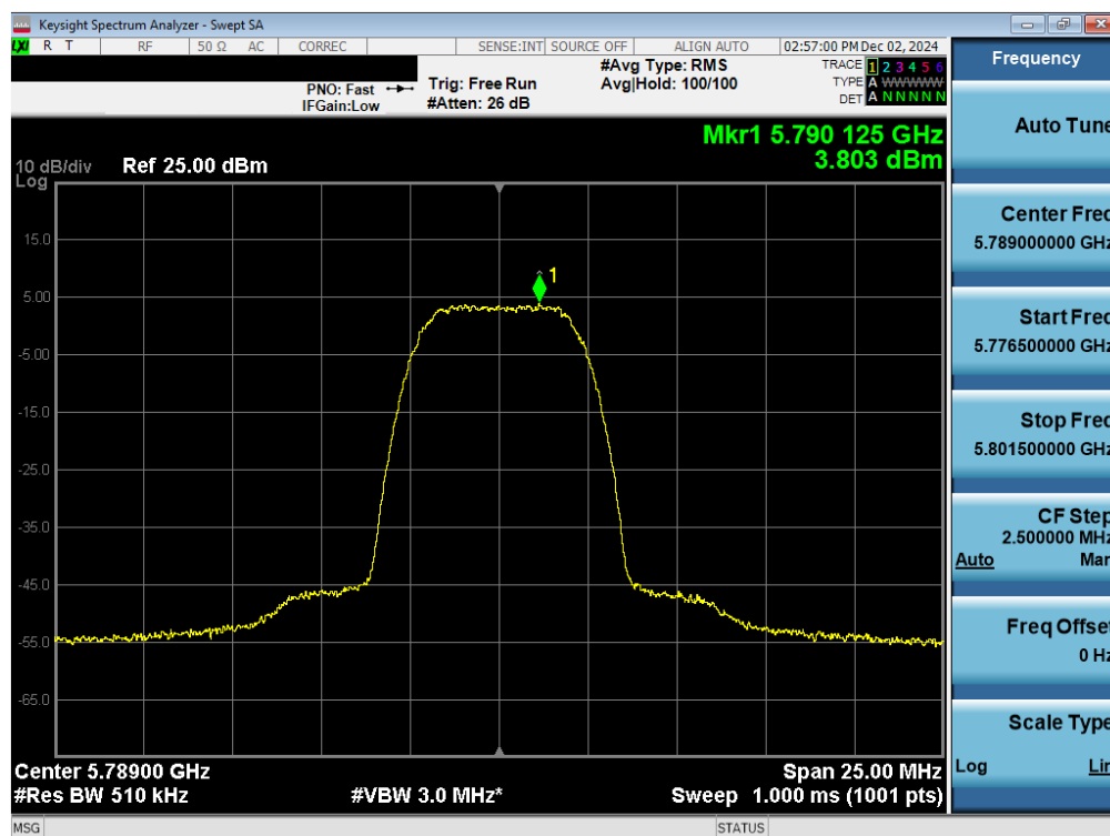
Plot 7-75. PSD TxBF Antenna WF7a (NB UNII HDR8, ePA – 5789MHz)
