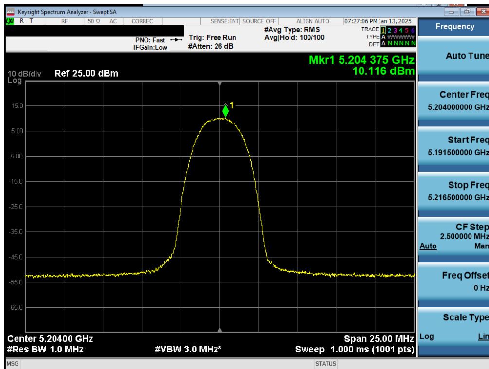
Plot 7-33. PSD Antenna WF2a (NB UNII HDR4, ePA – 5204MHz)
