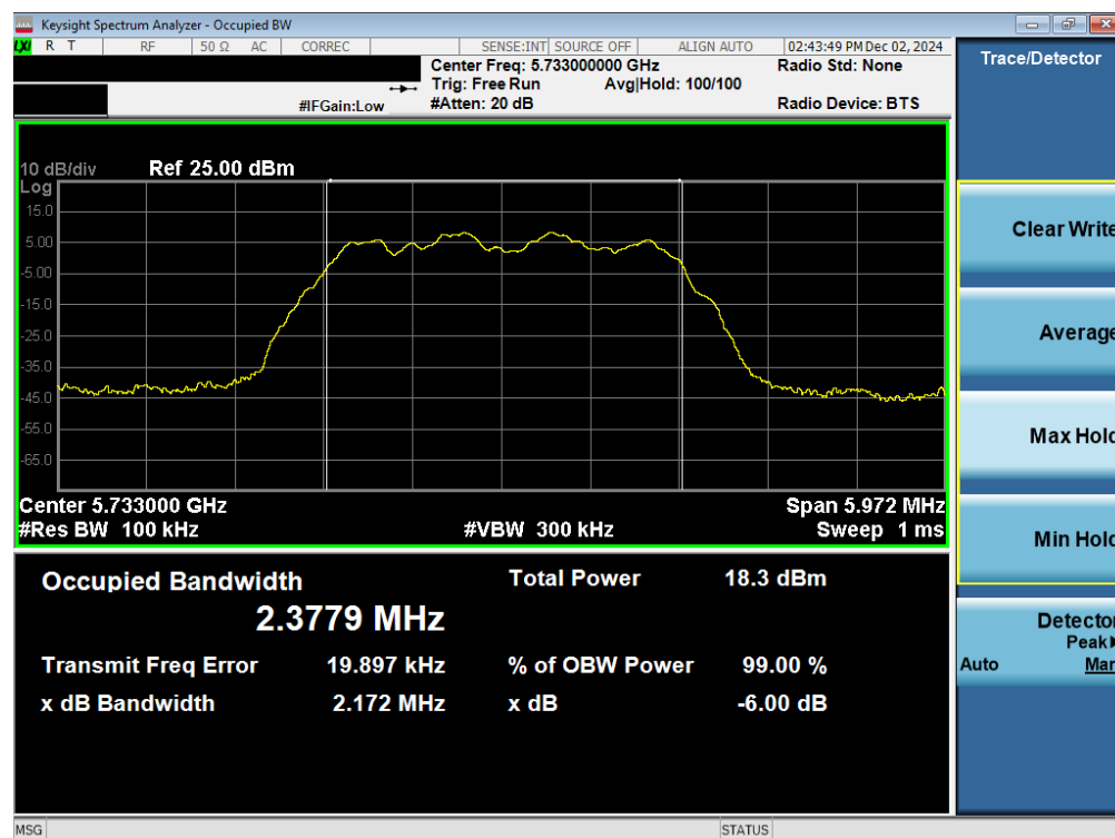
Plot 7-11. 6dB BW & 99% OBW Antenna WF7a (NB UNII HDR4, 5733MHz)
