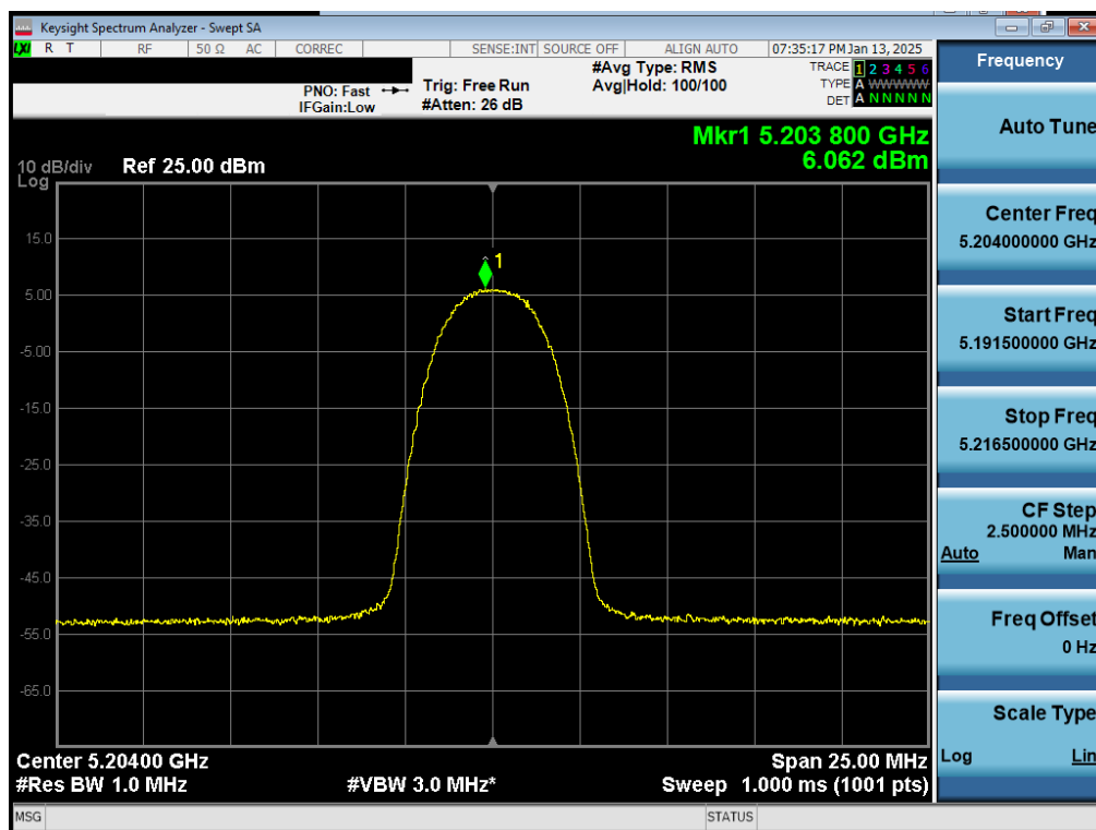
Plot 7-60. PSD TxBF Antenna WF2a (NB UNII HDR4, ePA - 5204MHz)
