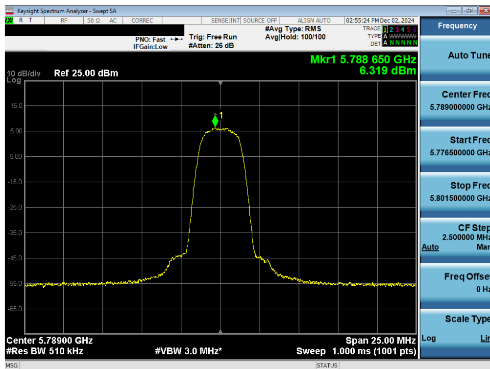
Plot 7-71. PSD TxBF Antenna WF7a (NB UNII HDR4, ePA – 5789MHz)
