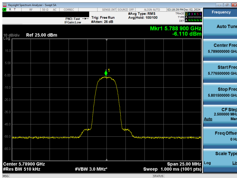
Plot 7-74. PSD TxBF Antenna WF2a (NB UNII HDR4, iPA – 5789MHz)
