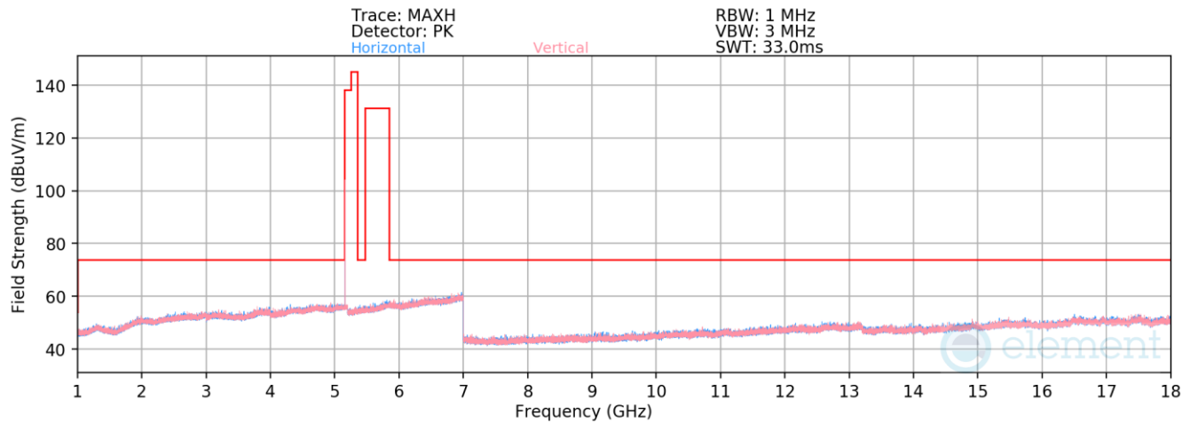
Plot 7-79. Radiated Spurious Emissions 1-18GHz Antenna WF7b (NB UNII BDR ePA – 5162MHz)
