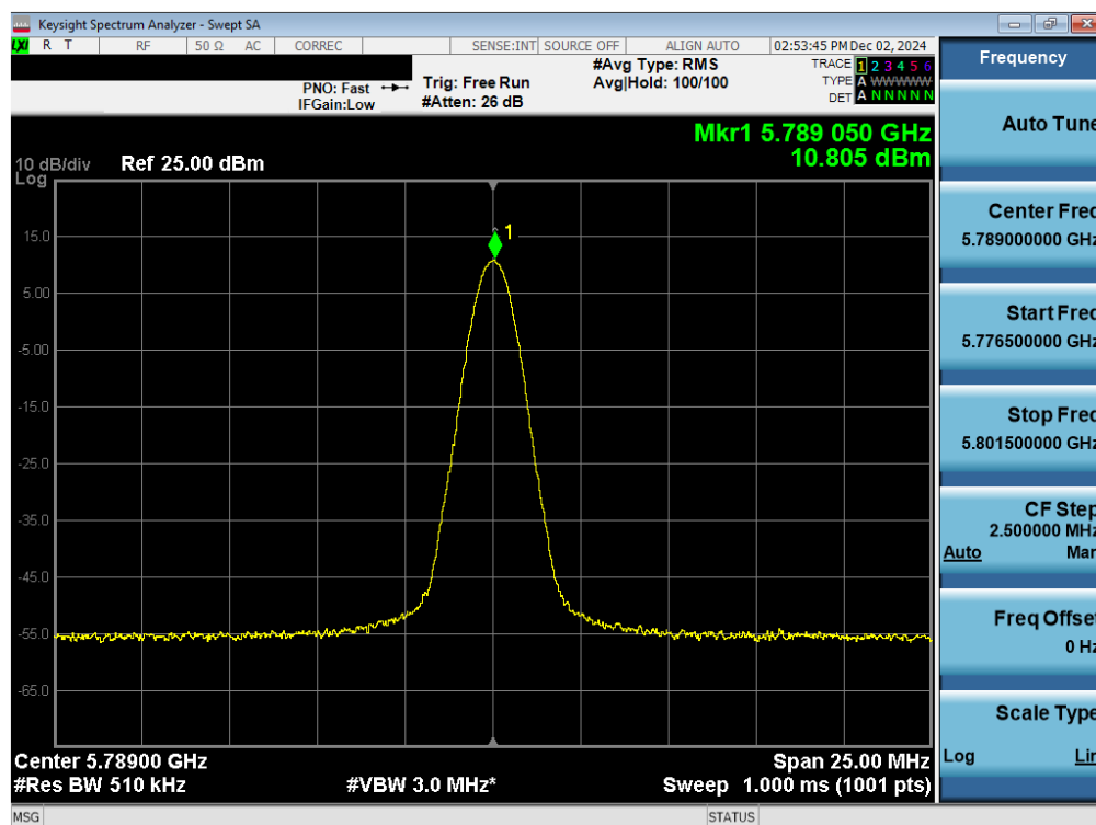
Plot 7-67. PSD TxBF Antenna WF7a (NB UNII BDR, ePA – 5789MHz)
