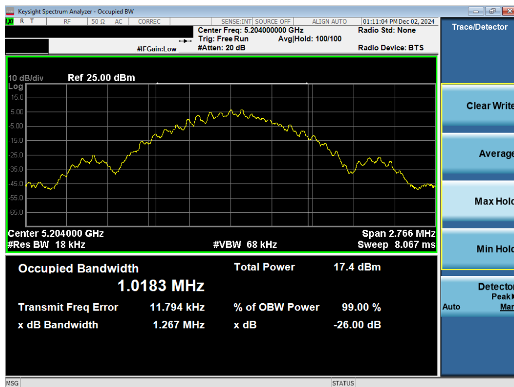
Plot 7-1. 26dB BW & 99% OBW Antenna WF7a (NB UNII BDR, ePA- 5204MHz)
