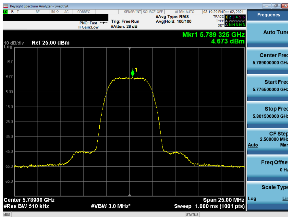
Plot 7-76. PSD TxBF Antenna WF7a (NB UNII HDR8, ePA – 5789MHz)
