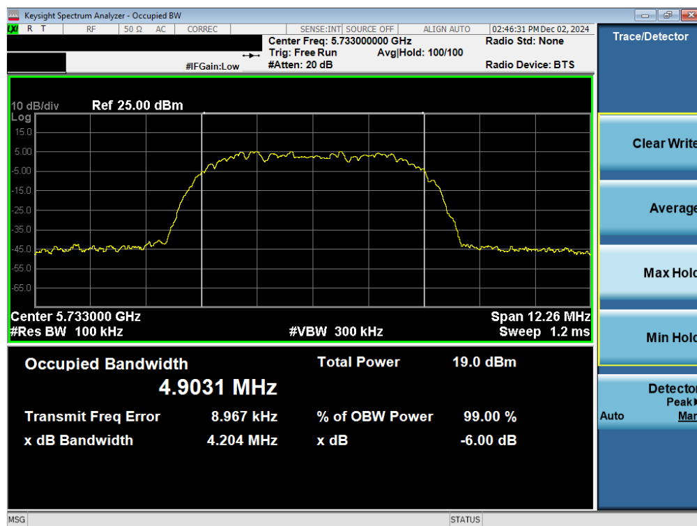
Plot 7-12. 6dB BW & 99% OBW Antenna WF7a (NB UNII HDR8, 5733MHz)
