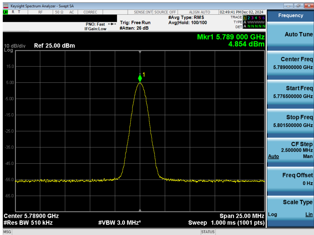
Plot 7-26. PSD Antenna WF7a (NB UNII BDR, iPA – 5789MHz)
