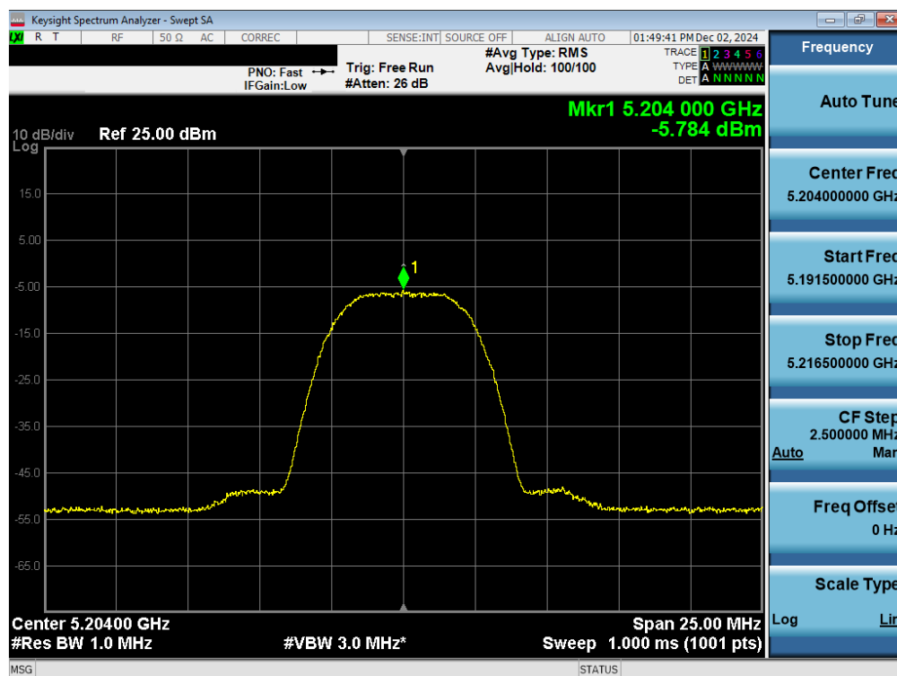
Plot 7-66. PSD TxBF Antenna WF2a (NB UNII HDR8, iPA – 5204MHz)
