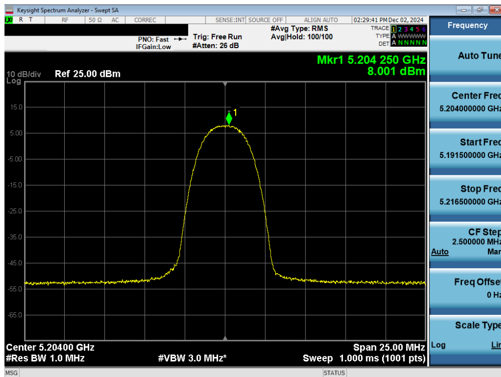
Plot 7-45. PSD Antenna WF7b (NB UNII HDR4, ePA – 5204MHz)
