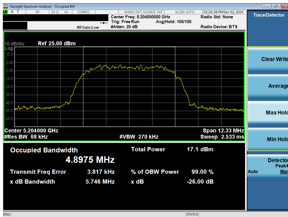
Plot 7-9. 26dB BW & 99% OBW Antenna WF7b (NB UNII HDR8, ePA- 5204MHz)
