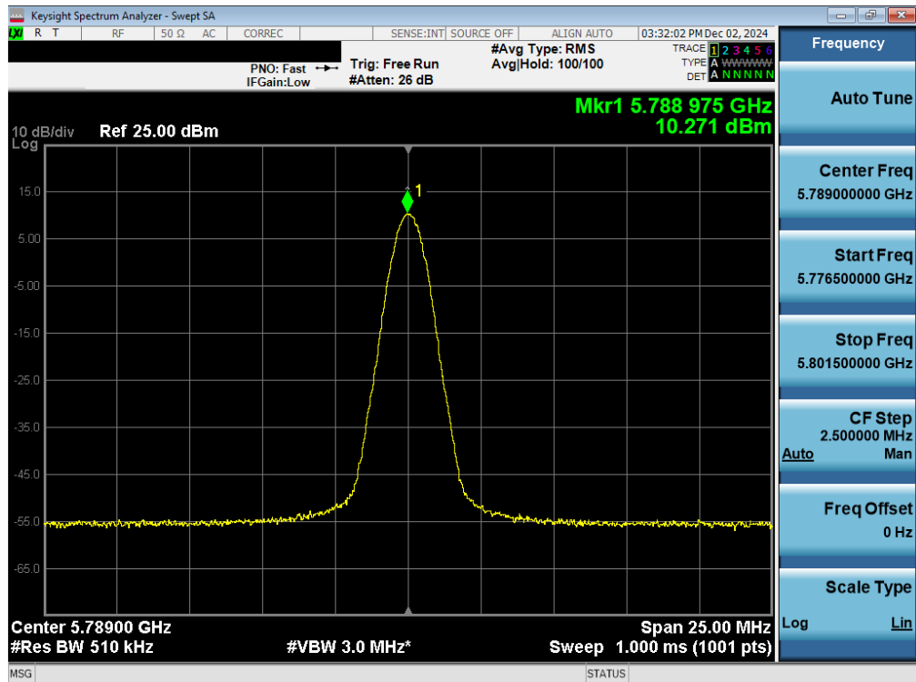
Plot 7-49. PSD Antenna WF7b (NB UNII BDR, ePA – 5789MHz)
