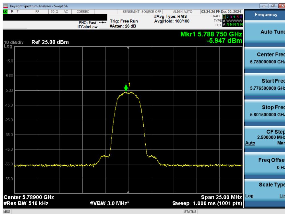
Plot 7-52. PSD Antenna WF7b (NB UNII HDR4, iPA – 5789MHz)
