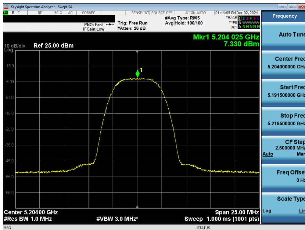
Plot 7-35. PSD Antenna WF2a (NB UNII HDR8, ePA – 5204MHz)
