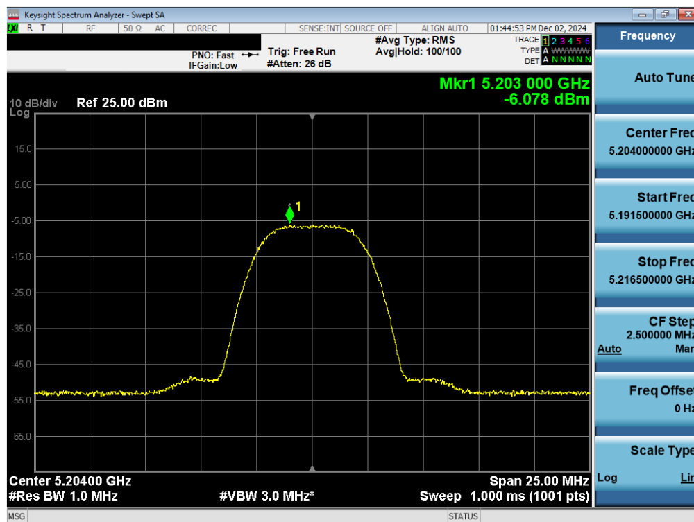
Plot 7-36. PSD Antenna WF2a (NB UNII HDR8, iPA – 5204MHz)
