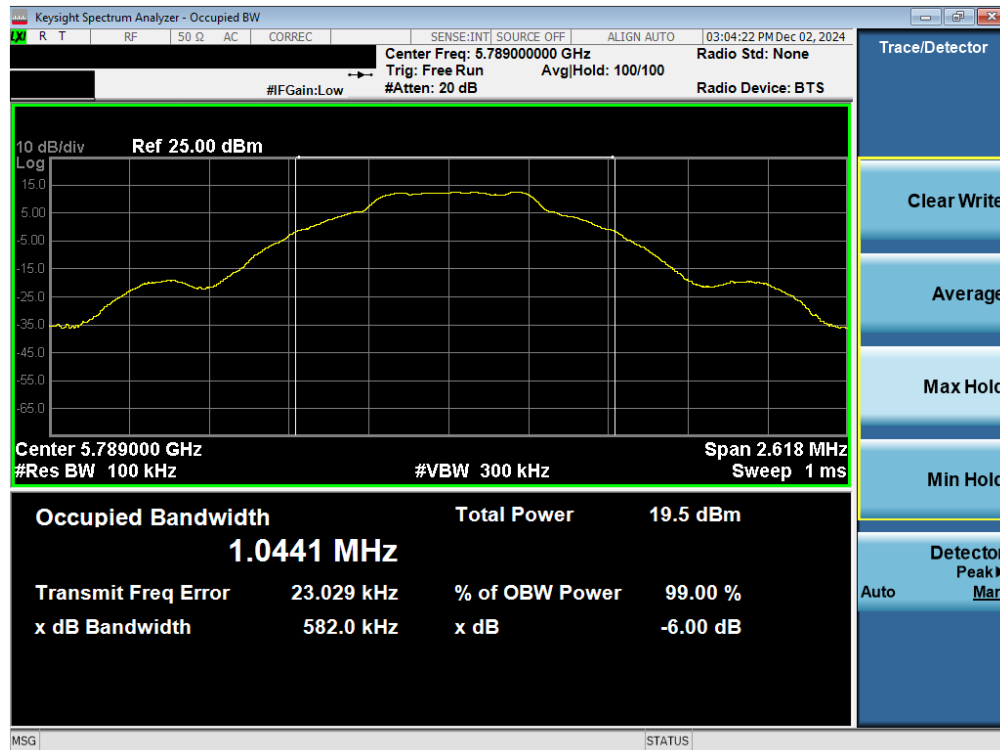
Plot 7-13. 6dB BW & 99% OBW Antenna WF2a (NB UNII BDR, 5789MHz)
