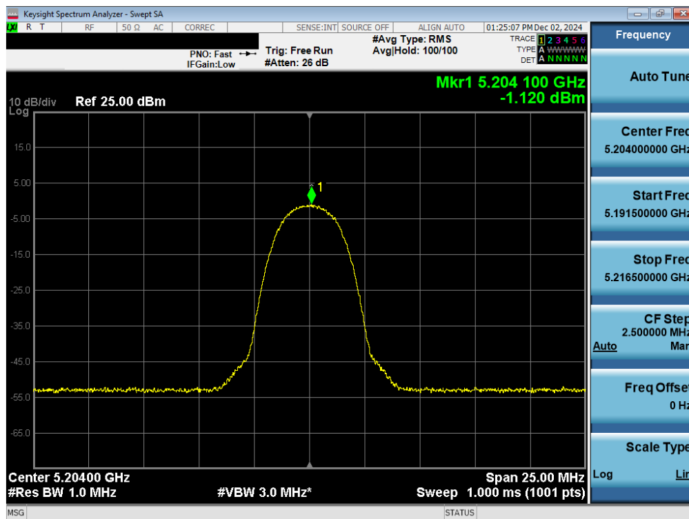
Plot 7-61. PSD TxBF Antenna WF7a (NB UNII HDR4, iPA – 5204MHz)
