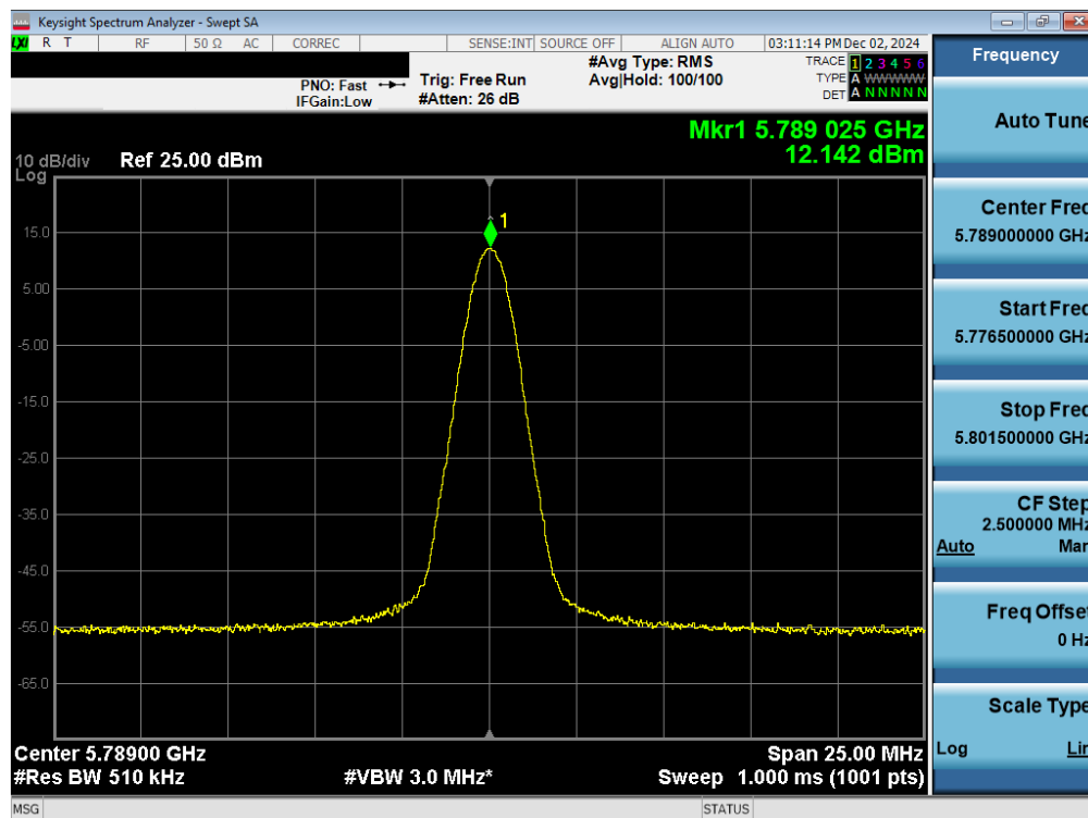
Plot 7-37. PSD Antenna WF2a (NB UNII BDR, ePA – 5789MHz)
