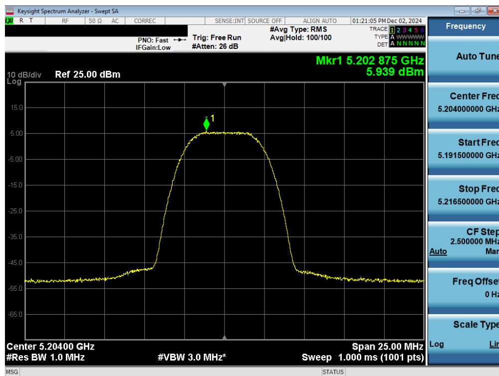
Plot 7-23. PSD Antenna WF7a (NB UNII HDR8, ePA – 5204MHz)
