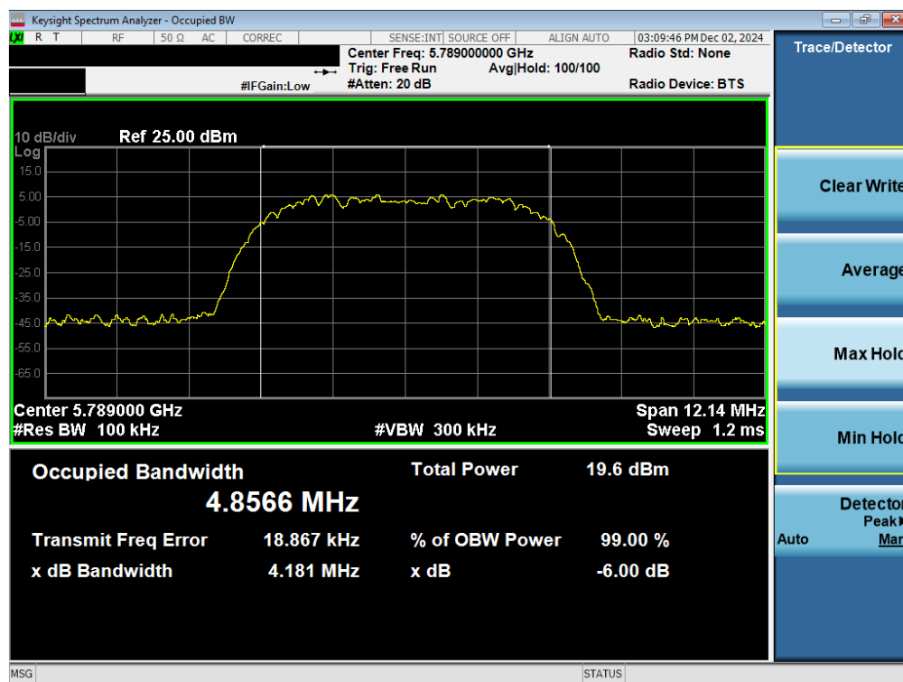
Plot 7-15. 6dB BW & 99% OBW Antenna WF2a (NB UNII HDR8, 5789MHz)
