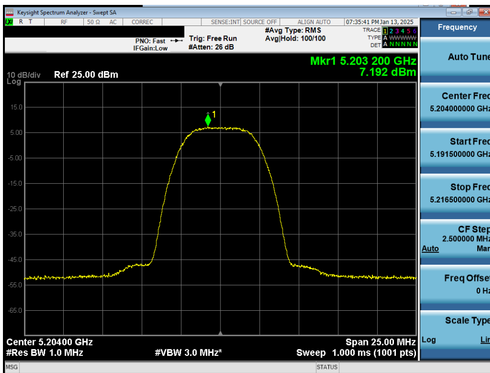
Plot 7-64. PSD TxBF Antenna WF2a (NB UNII HDR8, ePA – 5204MHz)
