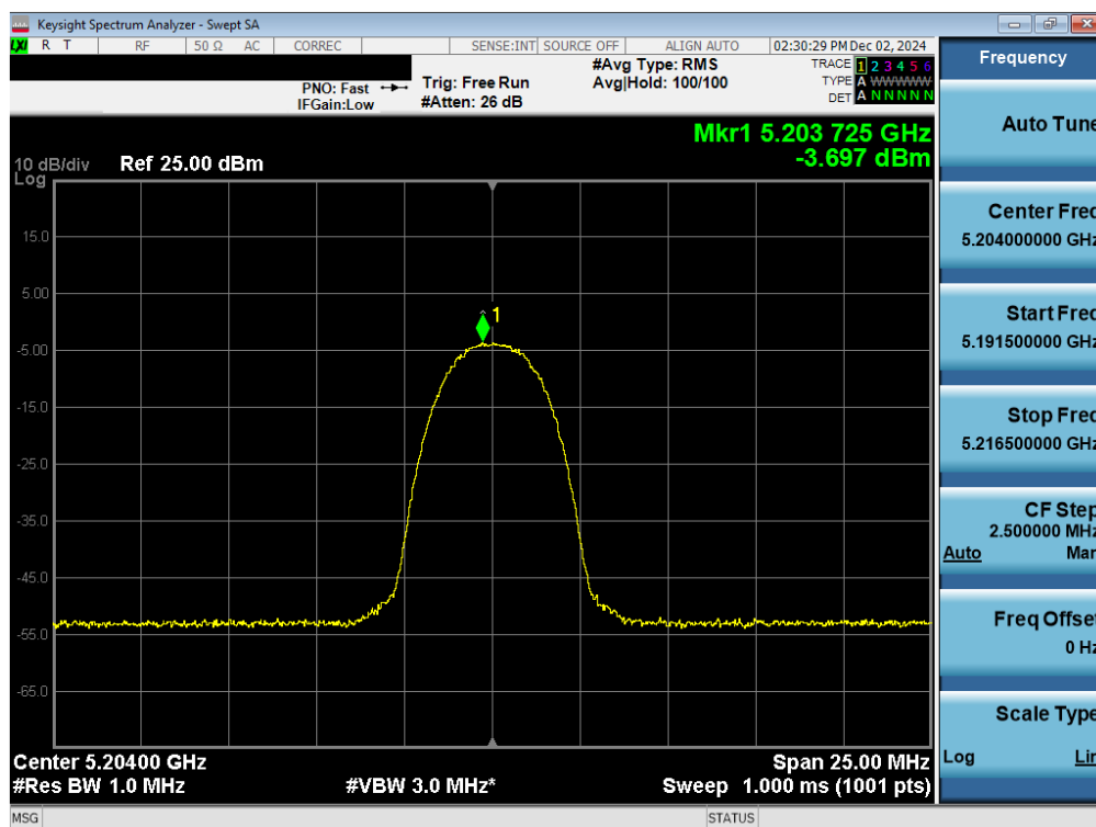
Plot 7-46. PSD Antenna WF7b (NB UNII HDR4, iPA – 5204MHz)
