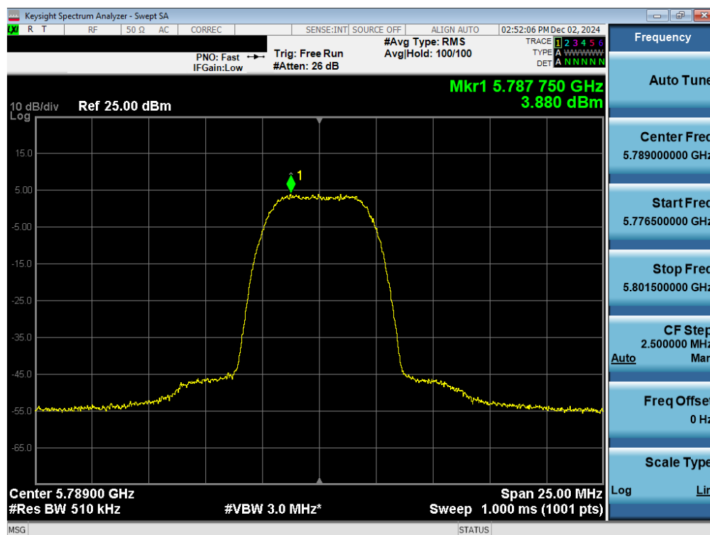
Plot 7-29. PSD Antenna WF7a (NB UNII HDR8, ePA – 5789MHz)
