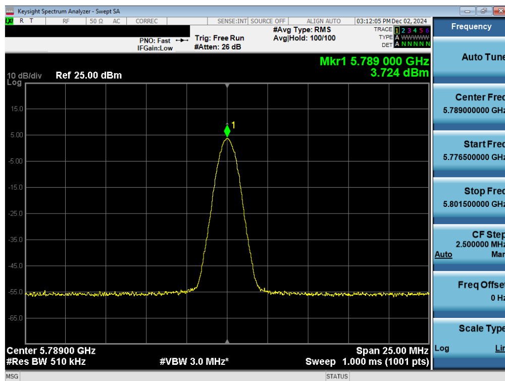
Plot 7-38. PSD Antenna WF2a (NB UNII BDR, iPA – 5789MHz)
