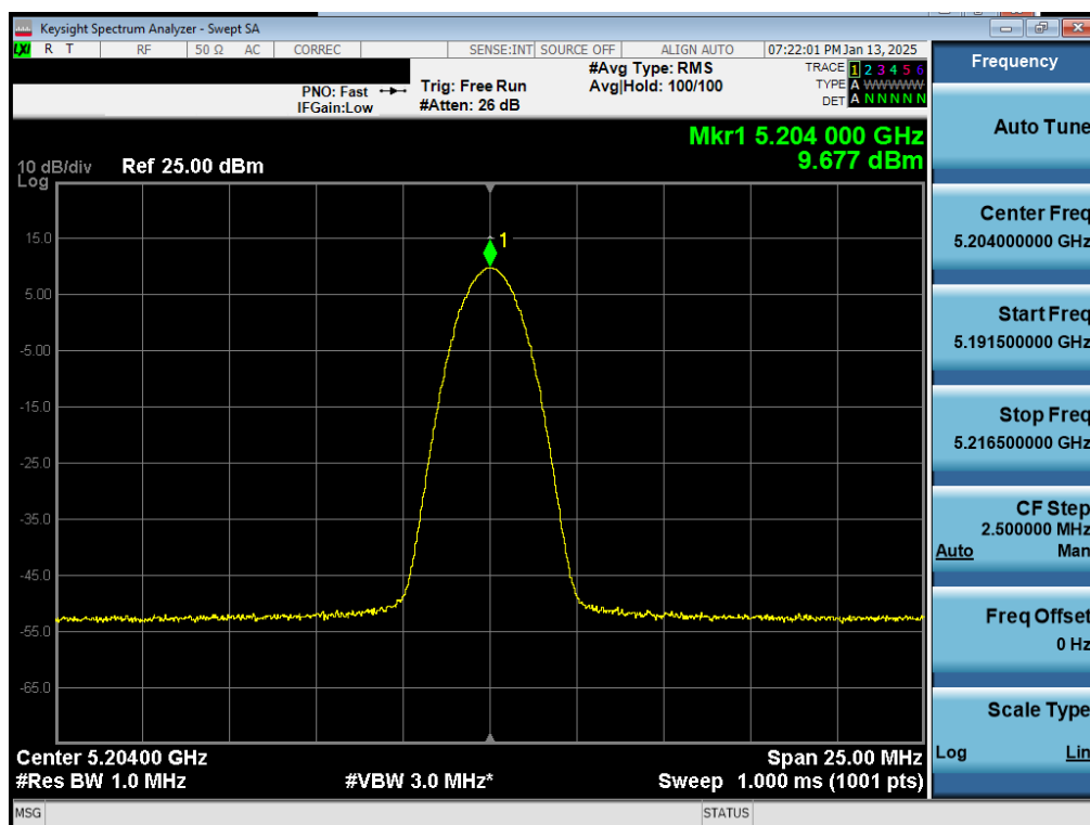
Plot 7-19. PSD Antenna WF7a (NB UNII BDR, ePA – 5204MHz)
