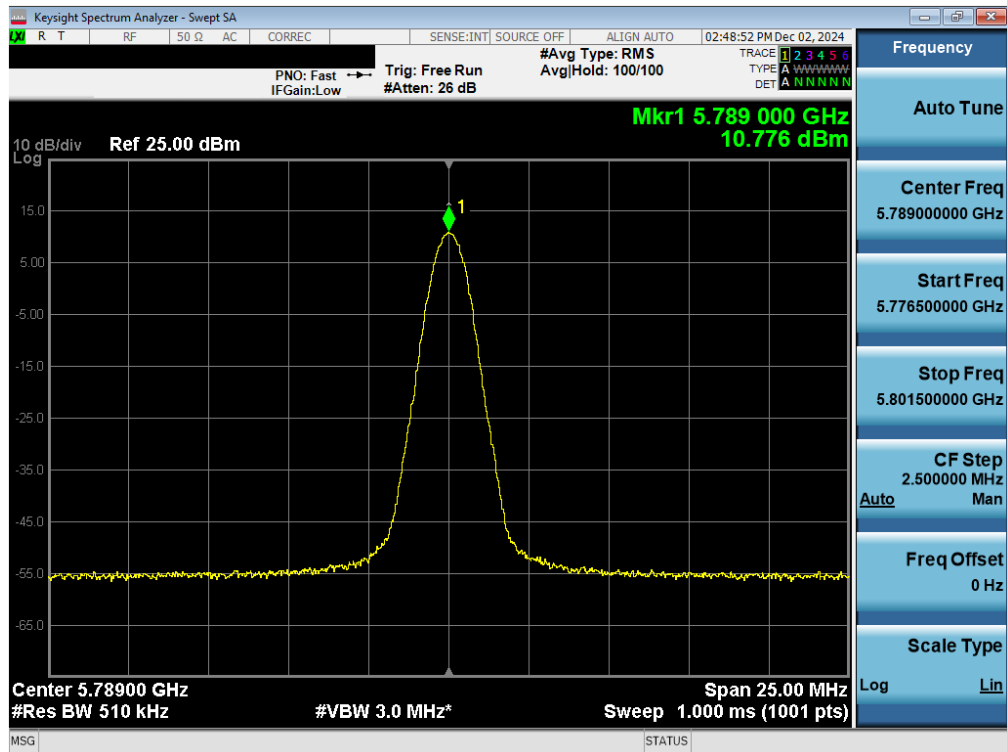
Plot 7-25. PSD Antenna WF7a (NB UNII BDR, ePA – 5789MHz)
