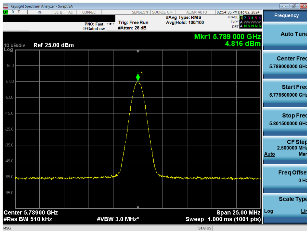
Plot 7-69. PSD TxBF Antenna WF7a (NB UNII BDR, iPA – 5789MHz)
