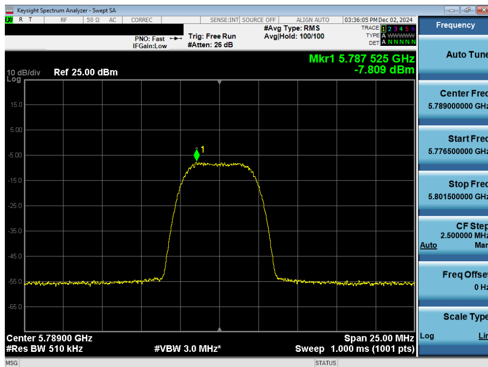
Plot 7-54. PSD Antenna WF7b (NB UNII HDR8, iPA – 5789MHz)
