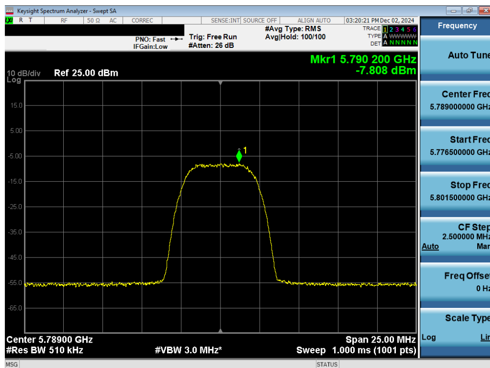
Plot 7-78. PSD TxBF Antenna WF2a (NB UNII HDR8, iPA – 5789MHz)
