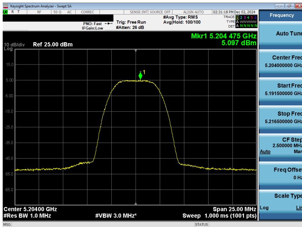
Plot 7-47. PSD Antenna WF7b (NB UNII HDR8, ePA – 5204MHz)
