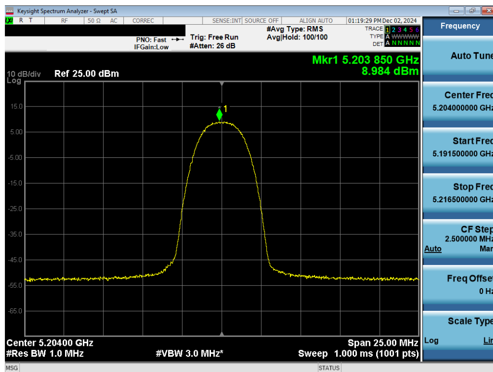
Plot 7-21. PSD Antenna WF7a (NB UNII HDR4, ePA – 5204MHz)
