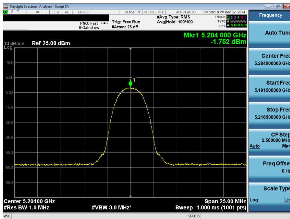
Plot 7-22. PSD Antenna WF7a (NB UNII HDR4, iPA – 5204MHz)
