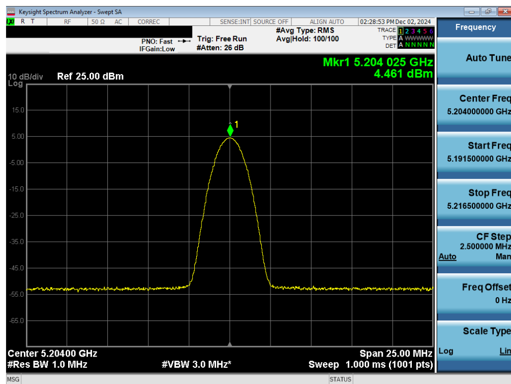
Plot 7-44. PSD Antenna WF7b (NB UNII BDR, iPA – 5204MHz)
