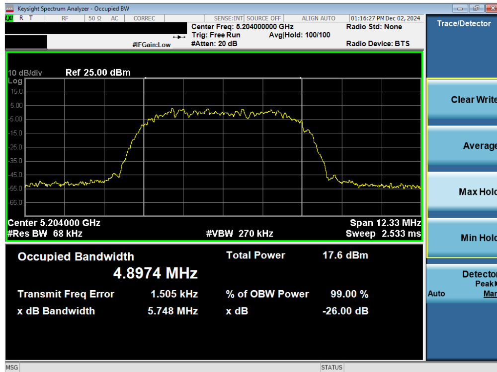
Plot 7-3. 26dB BW & 99% OBW Antenna WF7a (NB UNII HDR8, ePA- 5204MHz)
