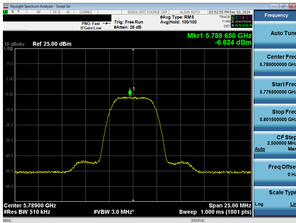
Plot 7-30. PSD Antenna WF7a (NB UNII HDR8, iPA – 5789MHz)
