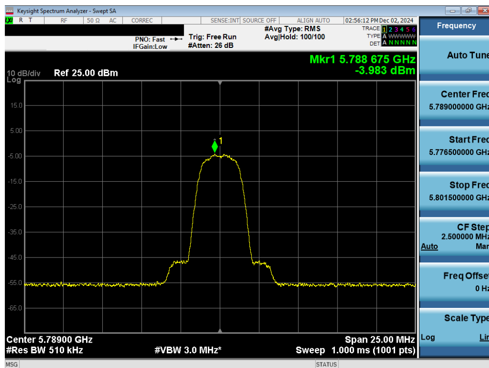
Plot 7-73. PSD TxBF Antenna WF7a (NB UNII HDR4, iPA – 5789MHz)
