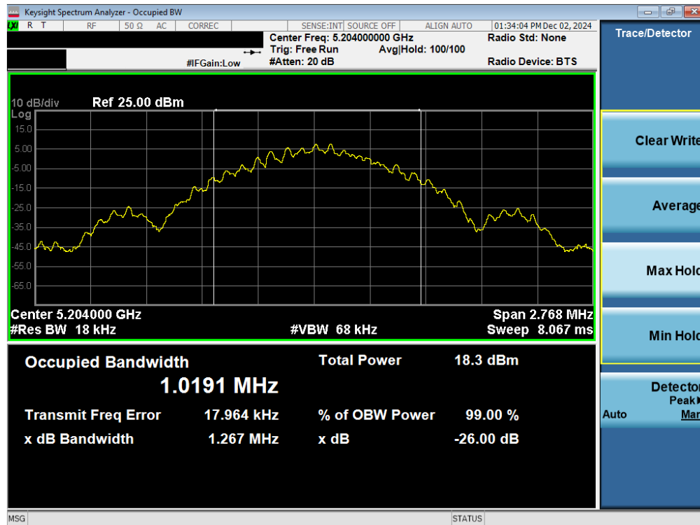
Plot 7-4. 26dB BW & 99% OBW Antenna WF2a (NB UNII BDR, ePA- 5204MHz)
