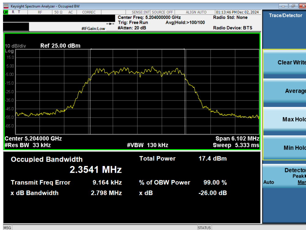
Plot 7-2. 26dB BW & 99% OBW Antenna WF7a (NB UNII HDR4, ePA- 5204MHz)
