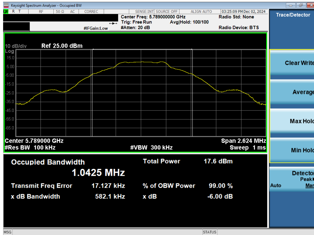
Plot 7-16. 6dB BW & 99% OBW Antenna WF7b (NB UNII BDR, 5789MHz)
