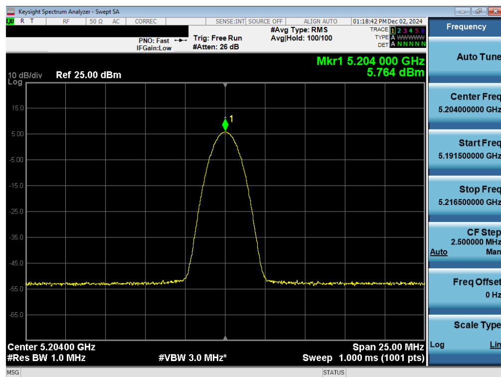
Plot 7-20. PSD Antenna WF7a (NB UNII BDR, iPA – 5204MHz)
