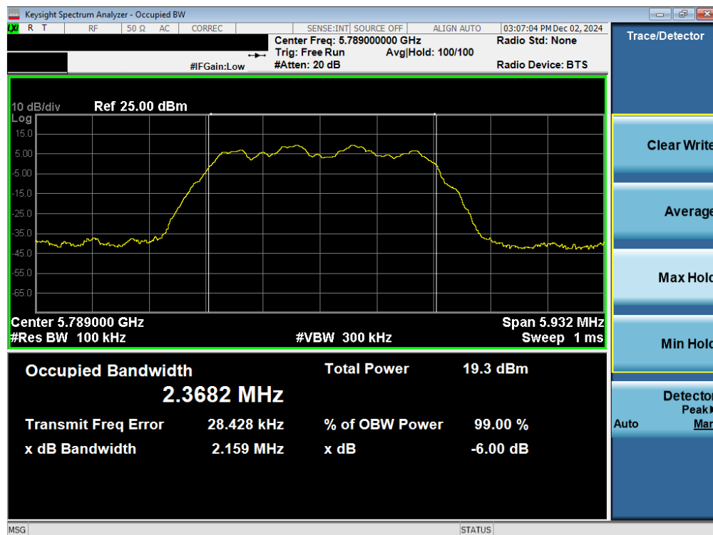
Plot 7-14. 6dB BW & 99% OBW Antenna WF2a (NB UNII HDR4, 5789MHz)
