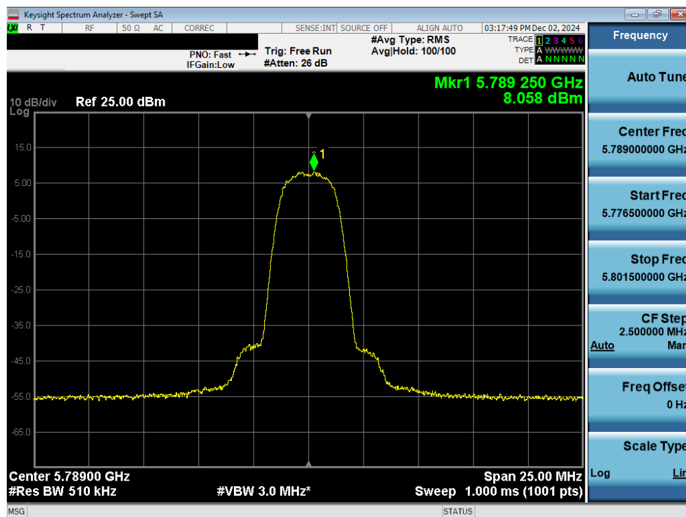
Plot 7-72. PSD TxBF Antenna WF2a (NB UNII HDR4, ePA – 5789MHz)
