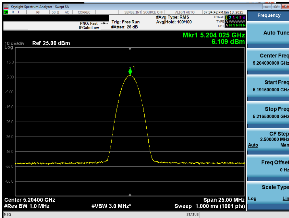
Plot 7-56. PSD TxBF Antenna WF2a (NB UNII BDR, ePA – 5204MHz)
