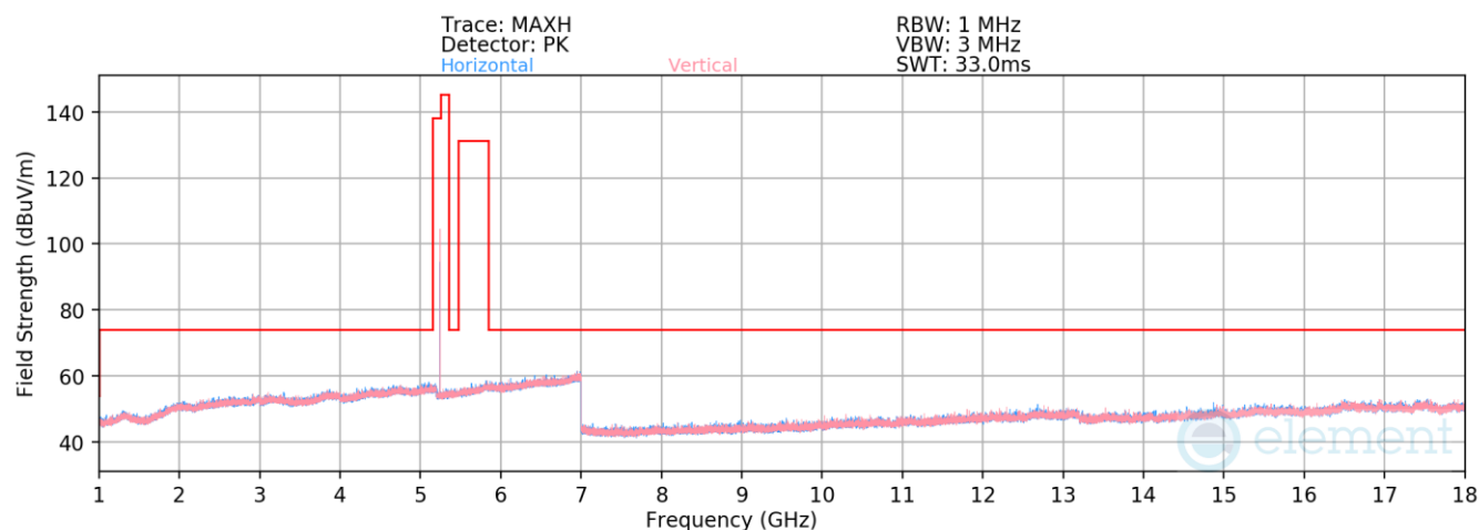
Plot 7-81. Radiated Spurious Emissions 1-18GHz Antenna WF7b (NB UNII BDR ePA – 5245MHz)
