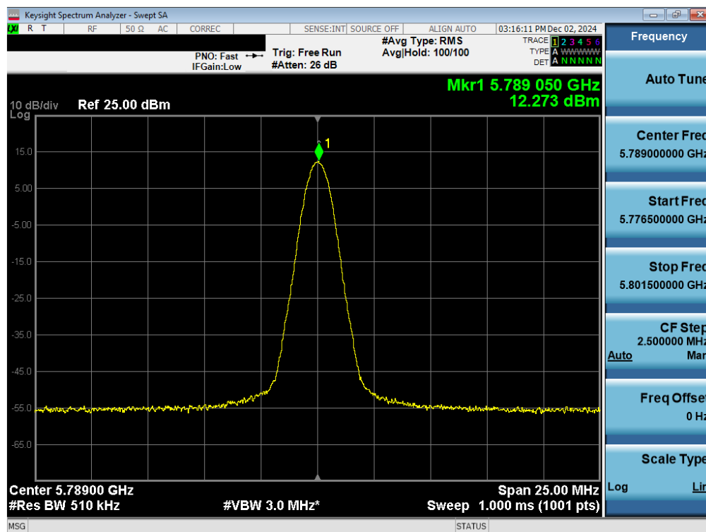
Plot 7-68. PSD TxBF Antenna WF2a (NB UNII BDR, ePA – 5789MHz)
