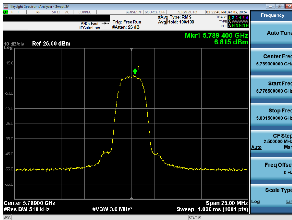
Plot 7-51. PSD Antenna WF7b (NB UNII HDR4, ePA – 5789MHz)
