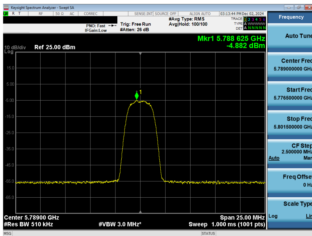
Plot 7-40. PSD Antenna WF2a (NB UNII HDR4, iPA – 5789MHz)
