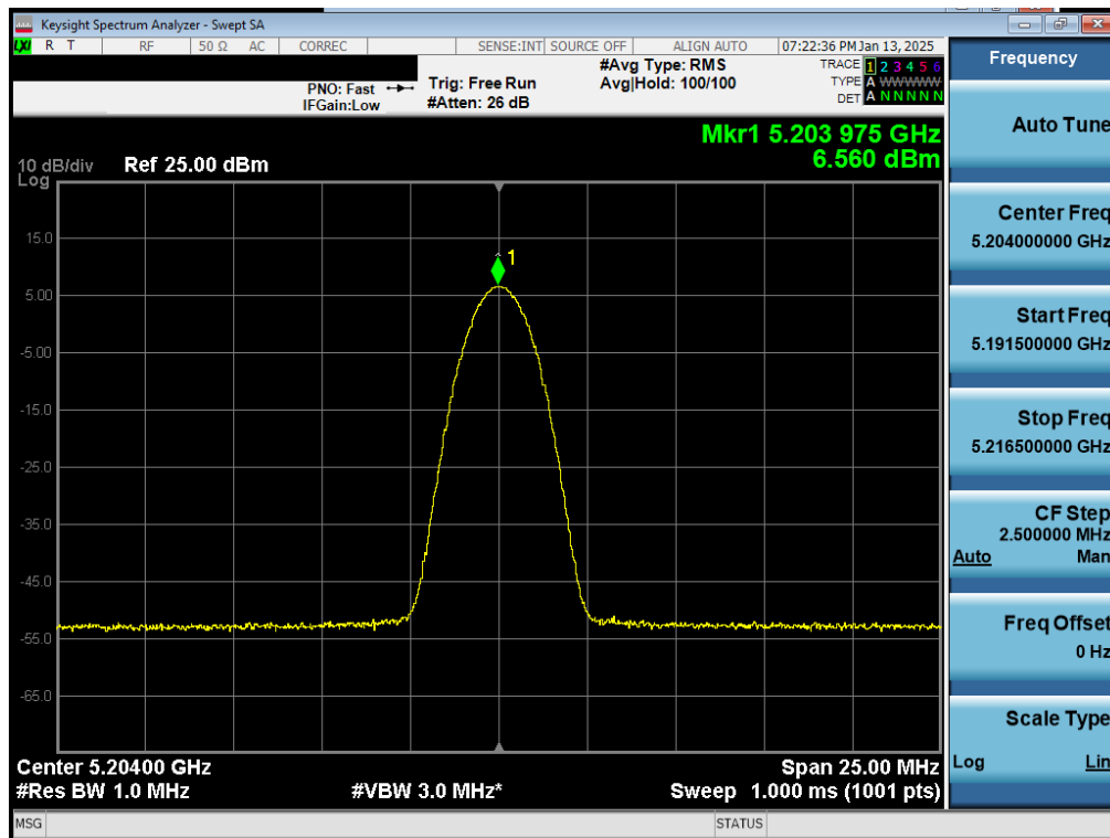
Plot 7-55. PSD TxBF Antenna WF7a (NB UNII BDR, ePA – 5204MHz)
