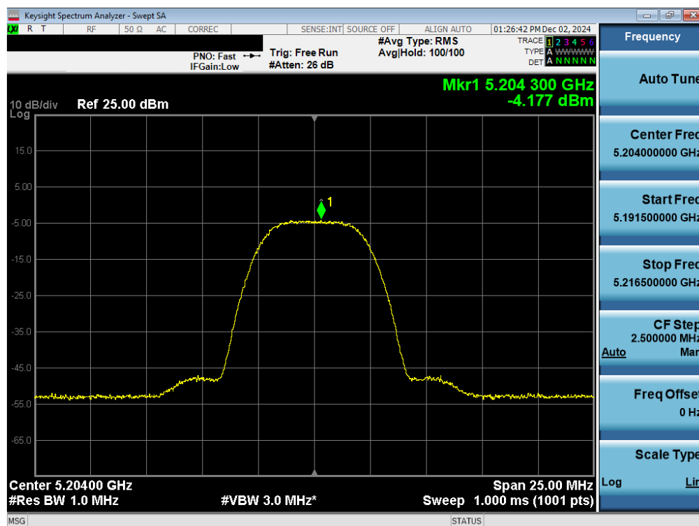
Plot 7-65. PSD TxBF Antenna WF7a (NB UNII HDR8, iPA – 5204MHz)
