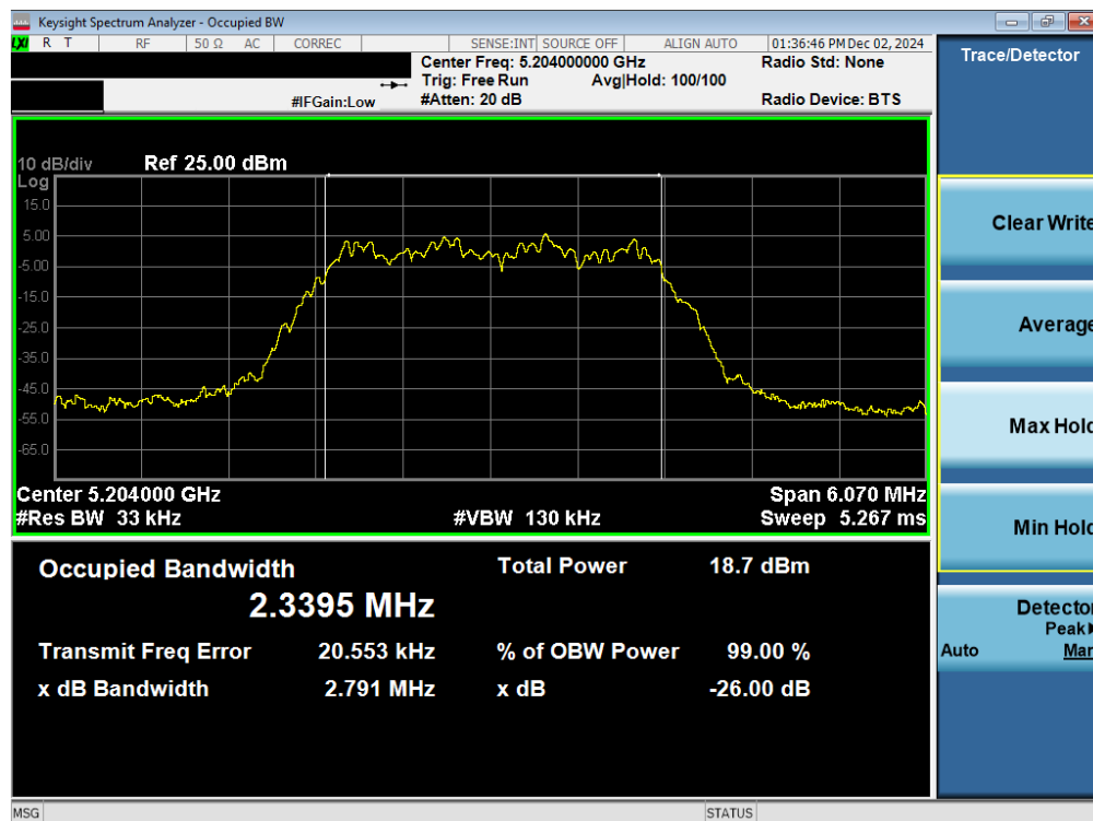
Plot 7-5. 26dB BW & 99% OBW Antenna WF2a (NB UNII HDR4, ePA- 5204MHz)
