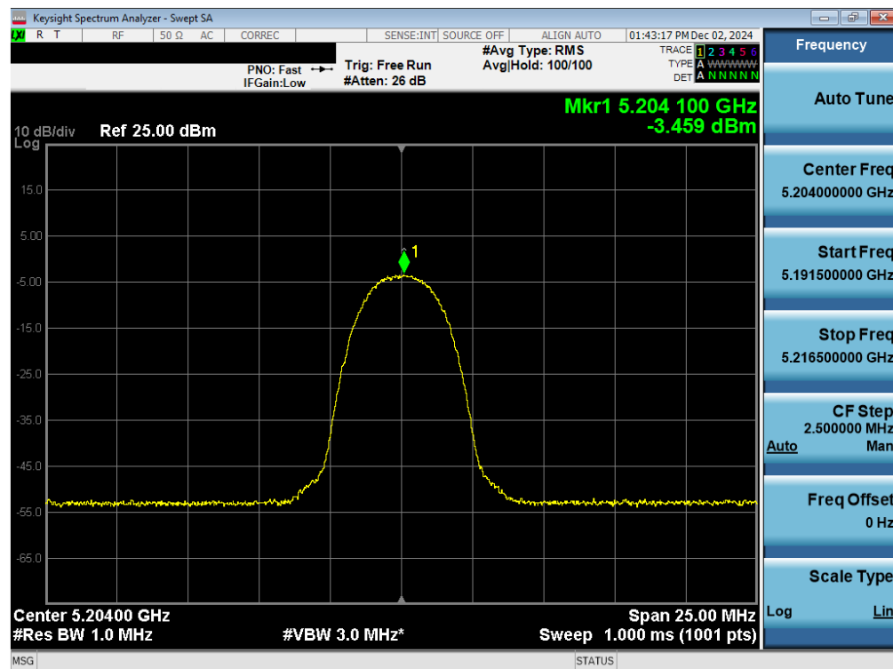
Plot 7-34. PSD Antenna WF2a (NB UNII HDR4, iPA – 5204MHz)
