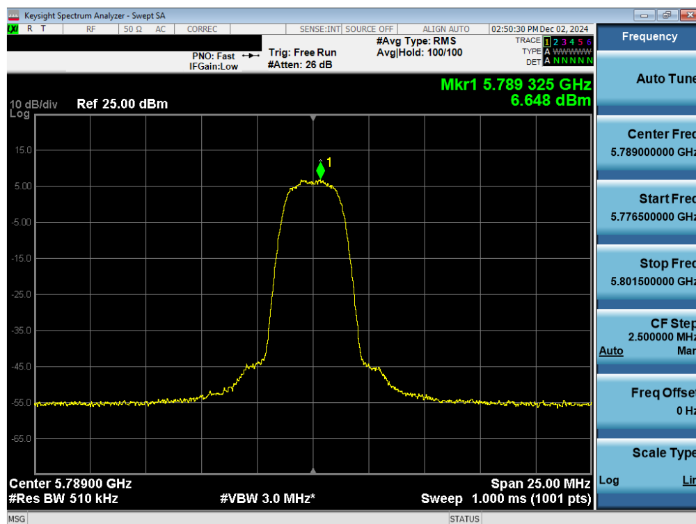
Plot 7-27. PSD Antenna WF7a (NB UNII HDR4, ePA – 5789MHz)
