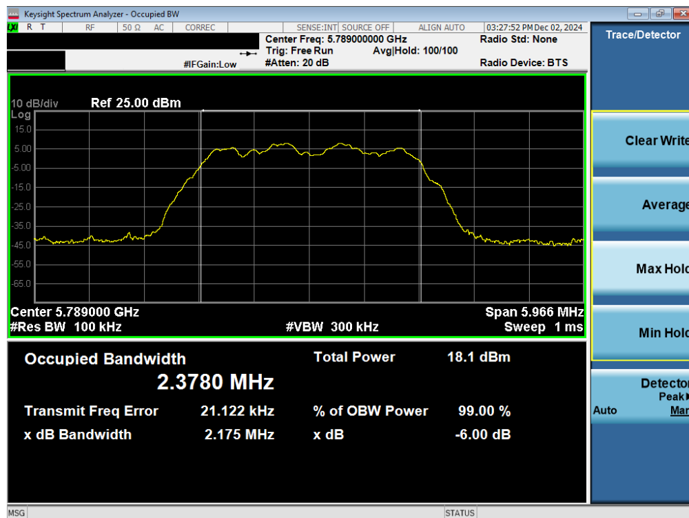
Plot 7-17. 6dB BW & 99% OBW Antenna WF7b (NB UNII HDR4, 5789MHz)
