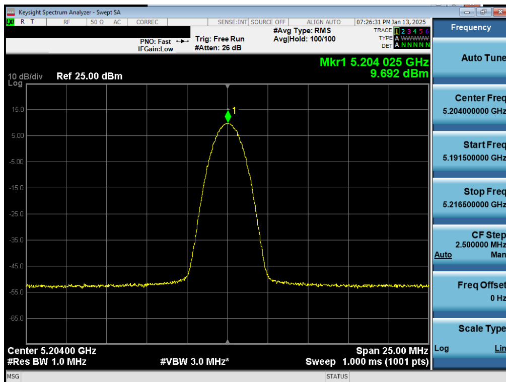
Plot 7-31. PSD Antenna WF2a (NB UNII BDR, ePA – 5204MHz)
