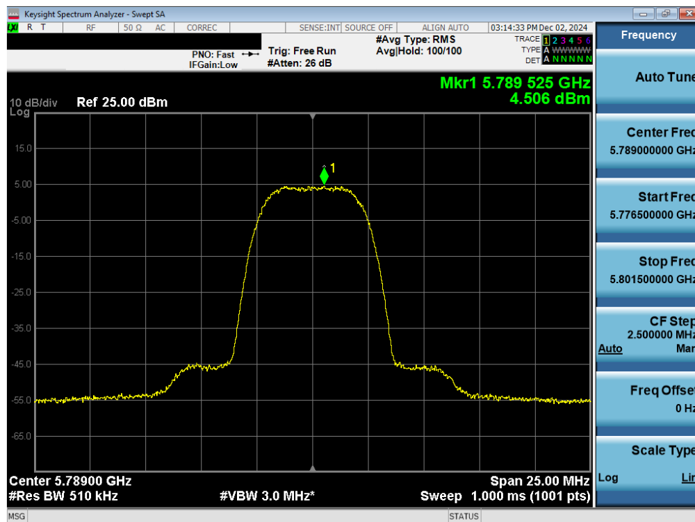
Plot 7-41. PSD Antenna WF2a (NB UNII HDR8, ePA – 5789MHz)
