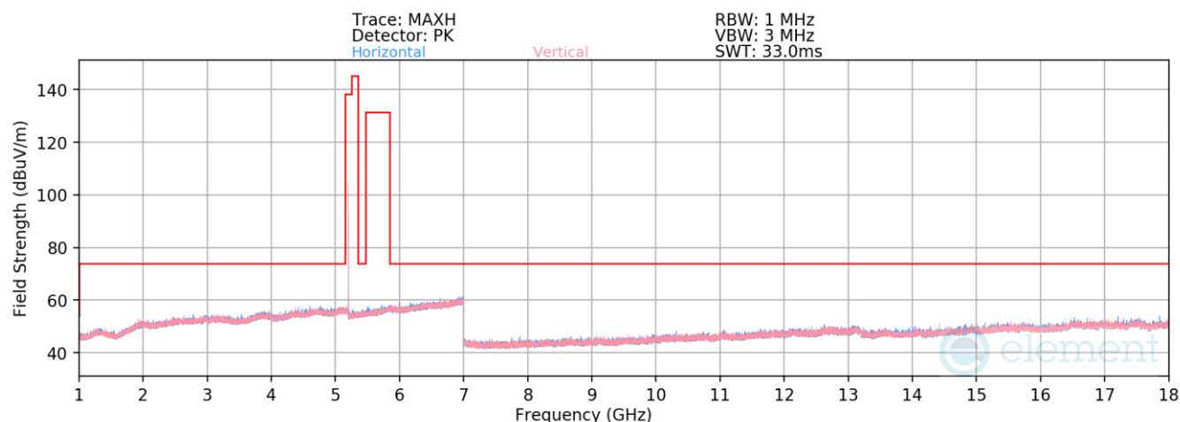
Plot 7-80. Radiated Spurious Emissions 1-18GHz Antenna WF7b (NB UNII BDR ePA – 5204MHz)
