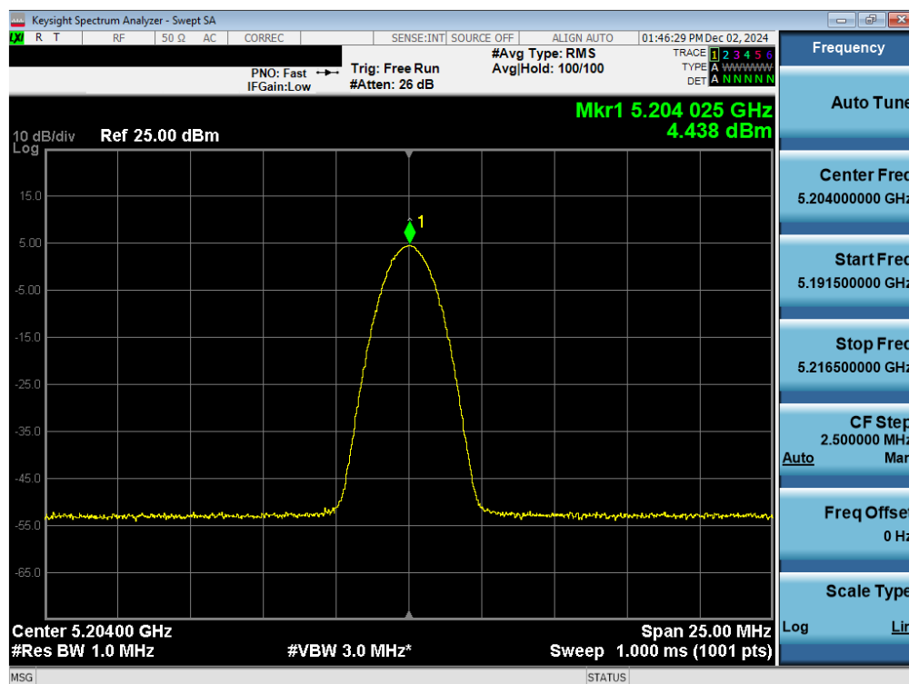
Plot 7-58. PSD TxBF Antenna WF2a (NB UNII BDR, iPA – 5204MHz)
