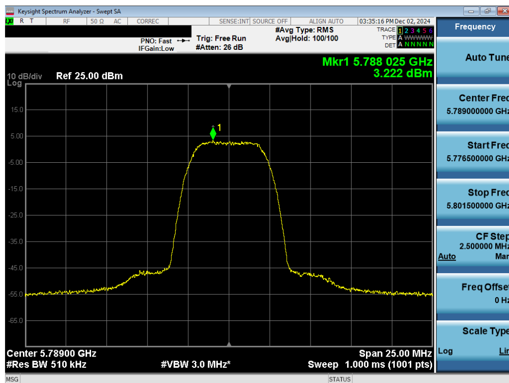
Plot 7-53. PSD Antenna WF7b (NB UNII HDR8, ePA – 5789MHz)
