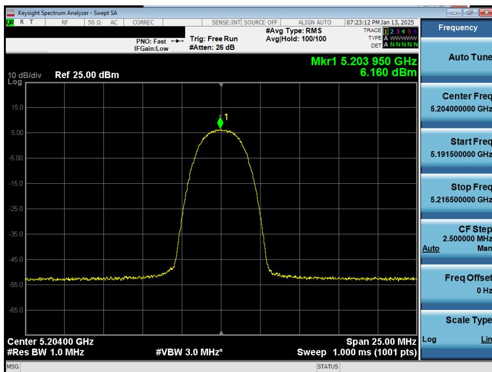
Plot 7-59. PSD TxBF Antenna WF7a (NB UNII HDR4, ePA - 5204MHz)
