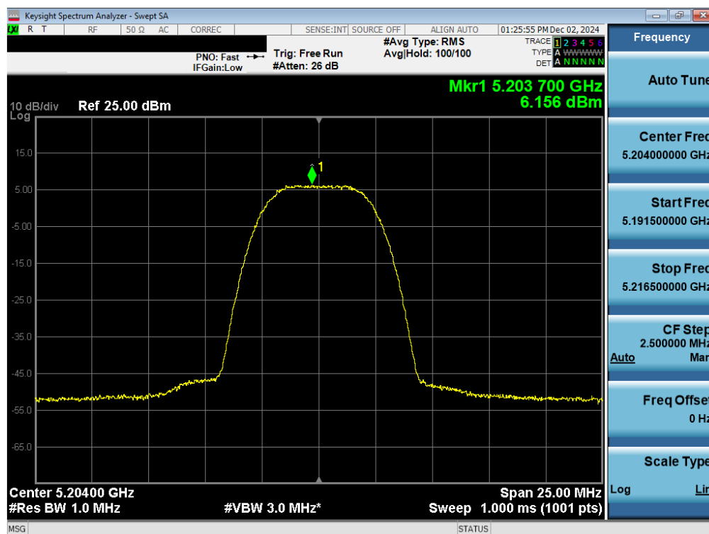
Plot 7-63. PSD TxBF Antenna WF7a (NB UNII HDR8, ePA – 5204MHz)
