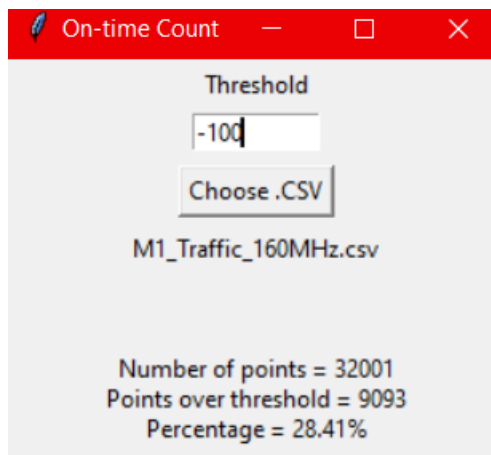
Figure 9-4. 5570MHz - Channel Loading Calculation - Mode 1 (160MHz)
