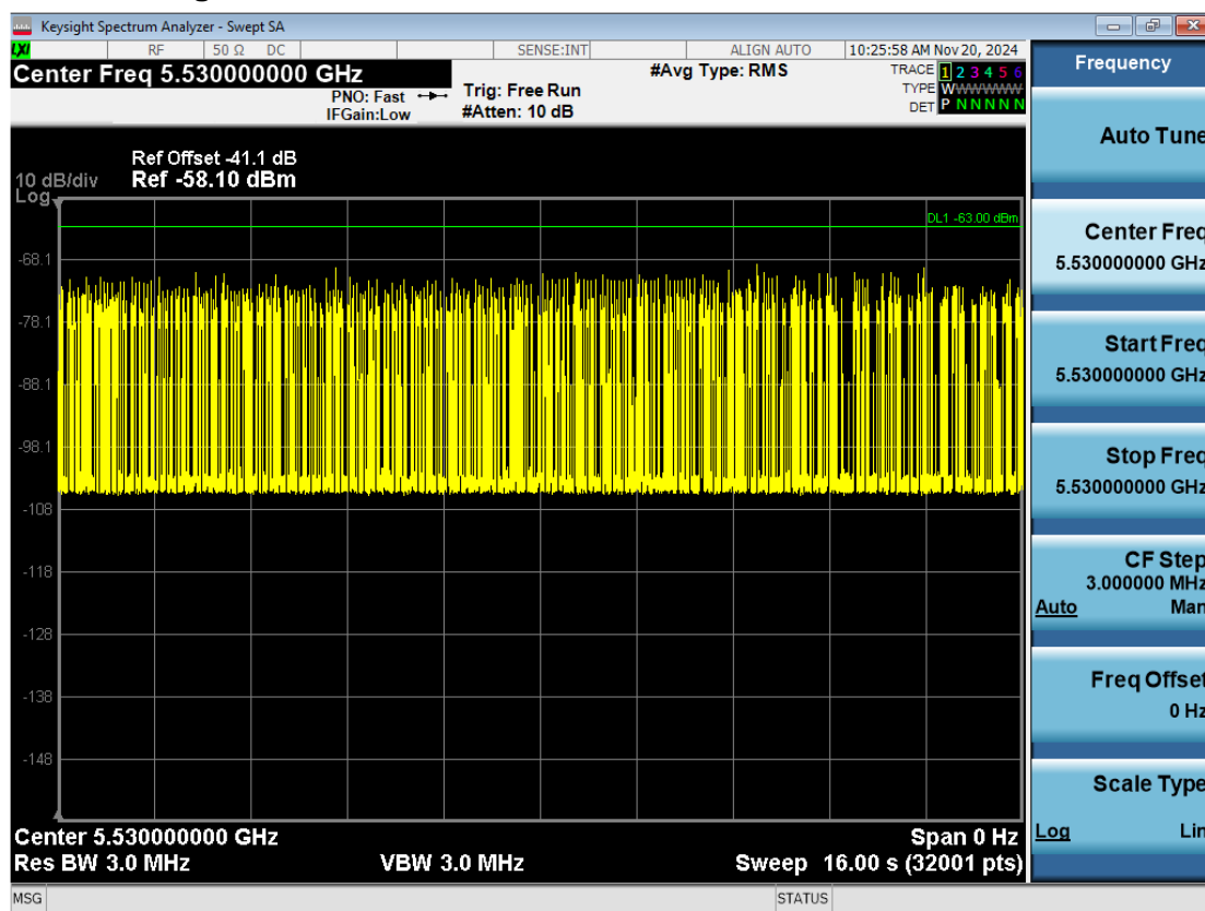
Figure 9-5. 5530MHz - Channel Loading - Mode 2 (80MHz)
