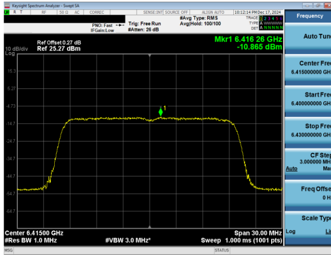
Plot 7-37. PSD Plot Antenna WF8 (20MHz 802.11ax RU242 (UNII Band 5) – Ch. 93)
