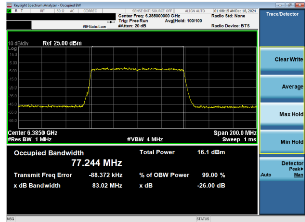
Plot 7-23. 26dB & 99% Bandwidth Plot Antenna WF7a (80MHz 802.11ax RU996 (UNII Band 5) – Ch. 87)
