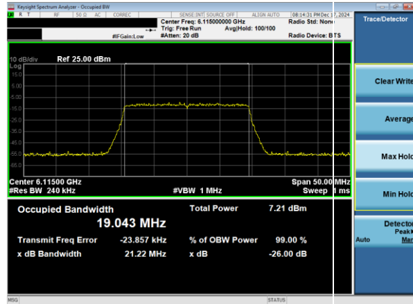
Plot 7-5. 26dB & 99% Bandwidth Plot Antenna WF8 (20MHz 802.11ax RU242 (UNII Band 5) – Ch. 33)
