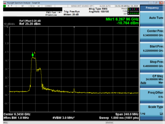
Plot 7-52. PSD Plot Antenna WF7a (160MHz 802.11ax RU106 (UNII Band 5) – Ch. 79)
