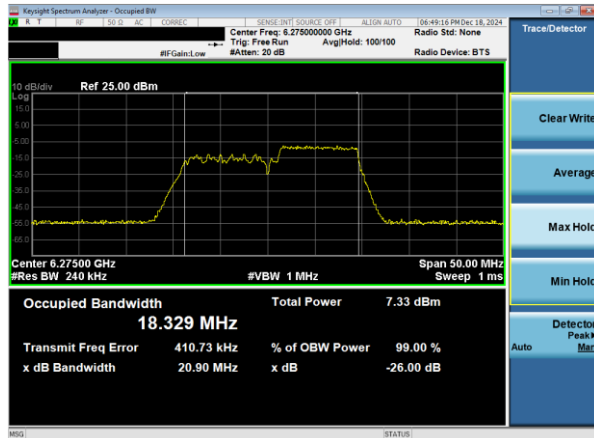
Plot 7-1. 26dB & 99% Bandwidth Plot Antenna WF8 (20MHz 802.11ax RU106 (UNII Band 5) – Ch. 65)
