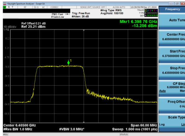
Plot 7-65. PSD Plot Antenna WF8 (40MHz 802.11ax RU242 (UNII Band 5) – Ch. 91)
