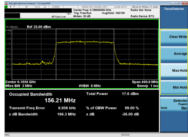
Plot 7-8. 26dB & 99% Bandwidth Plot Antenna WF8 (160MHz 802.11ax RU996x2 (UNII Band 5) – Ch. 47)
