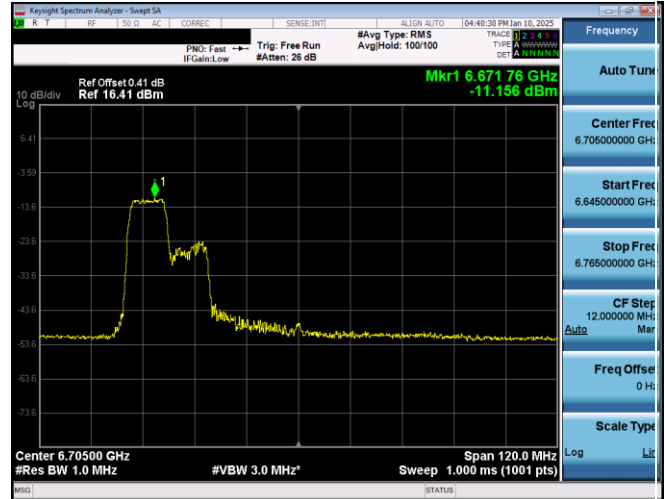
Plot 7-43. PSD Plot Antenna WF8 (80MHz 802.11ax RU106 (UNII Band 7) – Ch. 151)
