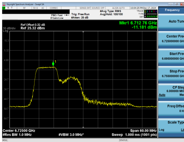
Plot 7-42. PSD Plot Antenna WF8 (40MHz 802.11ax RU106 (UNII Band 7) – Ch. 155)
