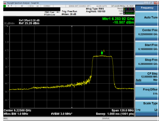
Plot 7-35. PSD Plot Antenna WF8 (80MHz 802.11ax RU106 (UNII Band 5) – Ch. 55)
