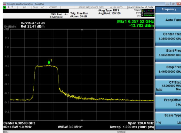
Plot 7-67. PSD Plot Antenna WF8 (80MHz 802.11ax RU242 (UNII Band 5) – Ch. 87)
