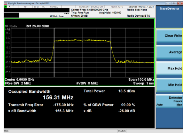
Plot 7-16. 26dB & 99% Bandwidth Plot Antenna WF8 (160MHz 802.11ax RU996x2 (UNII Band 7) – Ch. 143)
