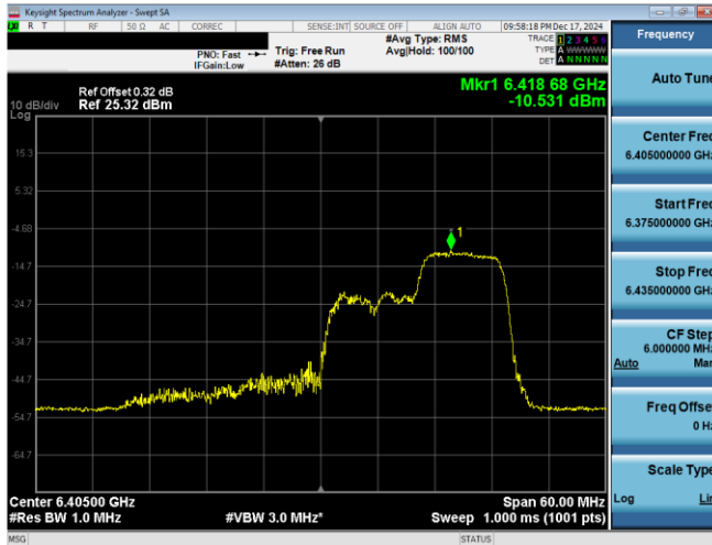
Plot 7-34. PSD Plot Antenna WF8 (40MHz 802.11ax RU106 (UNII Band 5) – Ch. 91)
