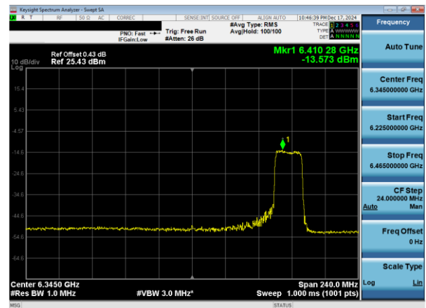
Plot 7-69. PSD Plot Antenna WF8 (160MHz 802.11ax RU242 (UNII Band 5) – Ch. 79)
