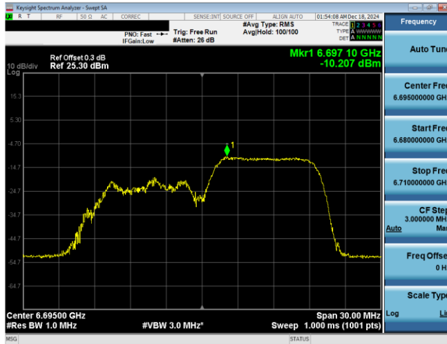
Plot 7-57. PSD Plot Antenna WF7a (20MHz 802.11ax RU106 (UNII Band 7) - Ch. 149)
