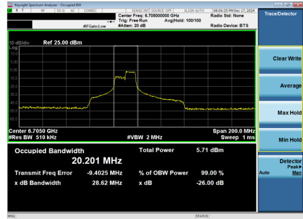
Plot 7-11. 26dB & 99% Bandwidth Plot Antenna WF8 (80MHz 802.11ax RU106 (UNII Band 7) – Ch. 151)
