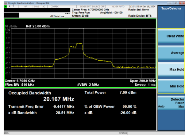
Plot 7-27. 26dB & 99% Bandwidth Plot Antenna WF7a (80MHz 802.11ax RU106 (UNII Band 7) – Ch. 151)
