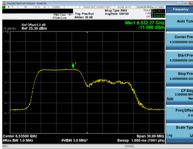
Plot 7-41. PSD Plot Antenna WF8 (20MHz 802.11ax RU106 (UNII Band 7) – Ch. 117)
