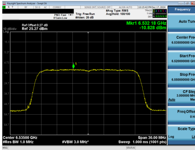
Plot 7-45. PSD Plot Antenna WF8 (20MHz 802.11ax RU242 (UNII Band 7) – Ch. 117)
