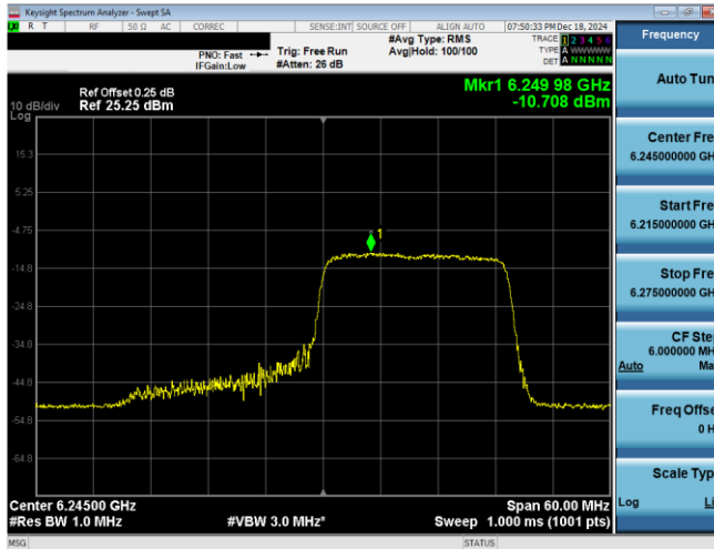
Plot 7-50. PSD Plot Antenna WF7a (40MHz 802.11ax RU242 (UNII Band 5) – Ch. 59)
