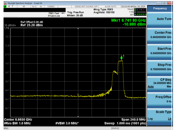
Plot 7-60. PSD Plot Antenna WF7a (160MHz 802.11ax RU106 (UNII Band 7) - Ch. 143)
