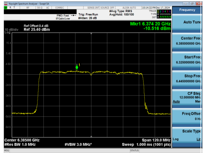
Plot 7-39. PSD Plot Antenna WF8 (80MHz 802.11ax RU996 (UNII Band 5) – Ch. 87)
