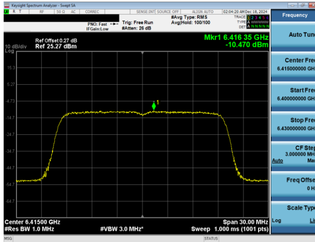
Plot 7-53. PSD Plot Antenna WF7a (20MHz 802.11ax RU242 (UNII Band 5) – Ch. 93)
