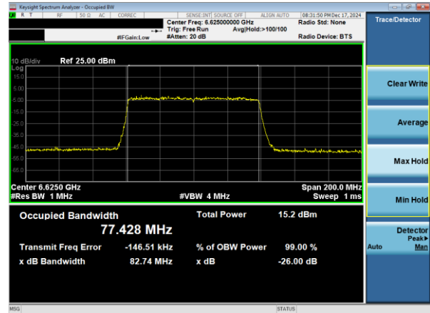
Plot 7-15. 26dB & 99% Bandwidth Plot Antenna WF8 (80MHz 802.11ax RU996 (UNII Band 7) – Ch. 135)
