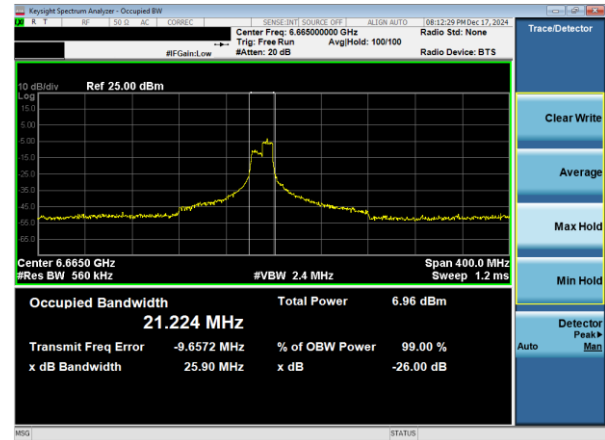
Plot 7-12. 26dB & 99% Bandwidth Plot Antenna WF8 (160MHz 802.11ax RU106 (UNII Band 7) – Ch. 143)
