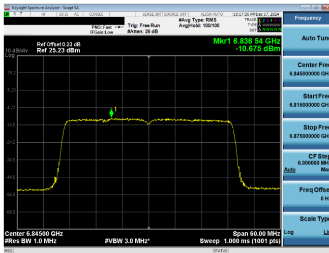
Plot 7-46. PSD Plot Antenna WF8 (40MHz 802.11ax RU484 (UNII Band 7) – Ch. 179)
