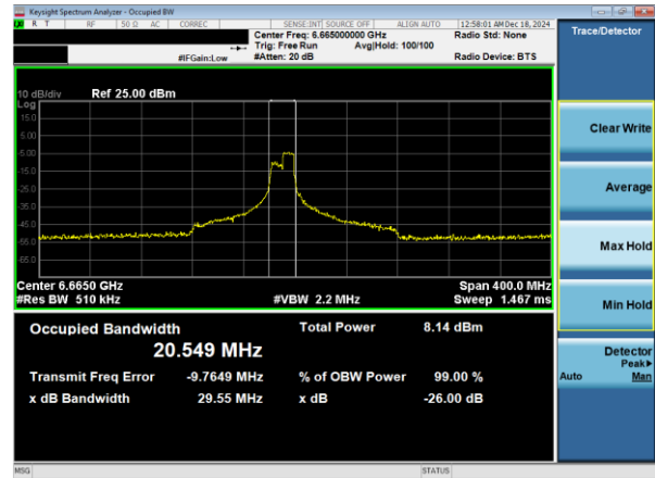
Plot 7-28. 26dB & 99% Bandwidth Plot Antenna WF7a (160MHz 802.11ax RU106 (UNII Band 7) – Ch. 143)
