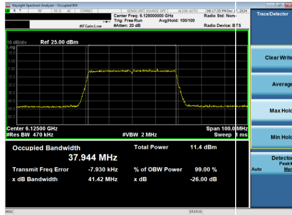
Plot 7-6. 26dB & 99% Bandwidth Plot Antenna WF8 (40MHz 802.11ax RU484 (UNII Band 5) – Ch. 35)
