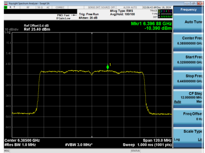
Plot 7-55. PSD Plot Antenna WF7a (80MHz 802.11ax RU996 (UNII Band 5) – Ch. 87)
