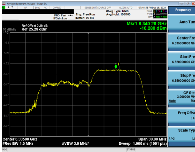
Plot 7-49. PSD Plot Antenna WF7a (20MHz 802.11ax RU106 (UNII Band 5) – Ch. 77)
