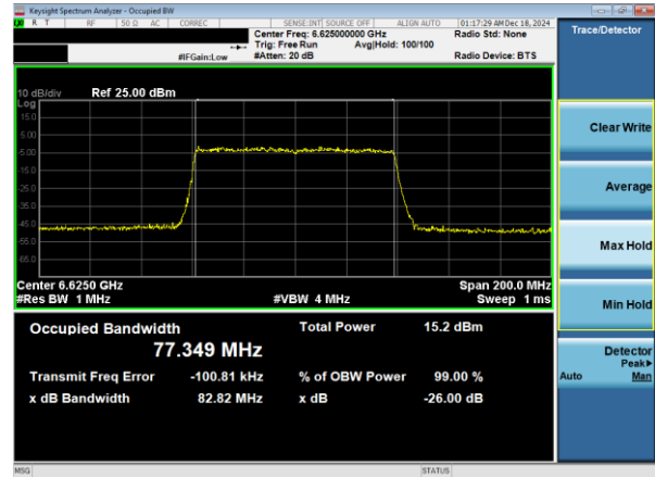
Plot 7-31. 26dB & 99% Bandwidth Plot Antenna WF7a (80MHz 802.11ax RU996 (UNII Band 7) – Ch. 135)
