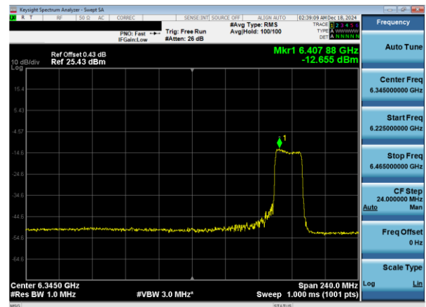
Plot 7-70. PSD Plot Antenna WF7a (160MHz 802.11ax RU242 (UNII Band 5) – Ch. 79)
