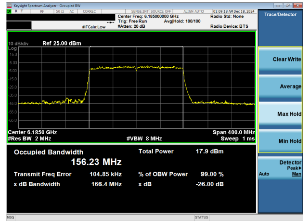
Plot 7-24. 26dB & 99% Bandwidth Plot Antenna WF7a (160MHz 802.11ax RU996x2 (UNII Band 5) – Ch. 47)
