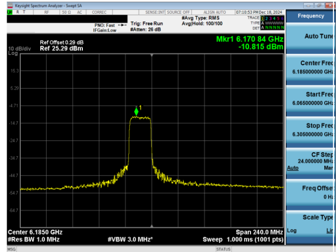
Plot 7-36. PSD Plot Antenna WF8 (160MHz 802.11ax RU242 (UNII Band 5) – Ch. 47)
