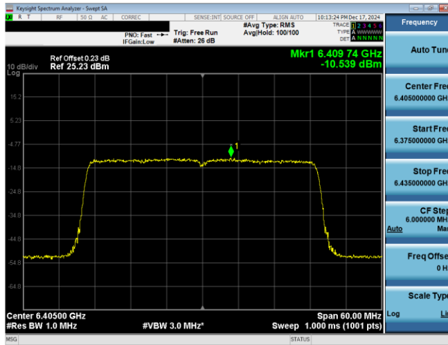
Plot 7-38. PSD Plot Antenna WF8 (40MHz 802.11ax RU484 (UNII Band 5) – Ch. 91)
