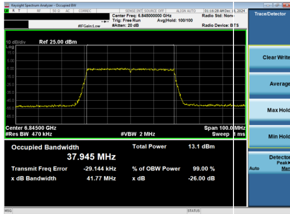
Plot 7-30. 26dB & 99% Bandwidth Plot Antenna WF7a (40MHz 802.11ax RU484 (UNII Band 7) – Ch. 179)
