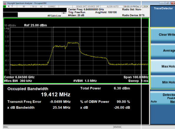
Plot 7-10. 26dB & 99% Bandwidth Plot Antenna WF8 (40MHz 802.11ax RU106 (UNII Band 7) – Ch. 179)
