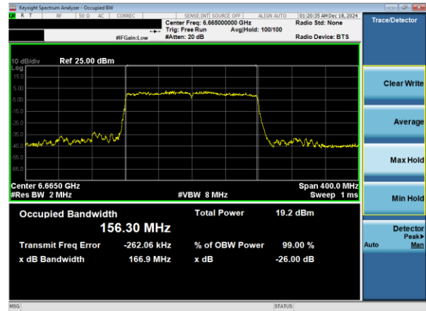
Plot 7-32. 26dB & 99% Bandwidth Plot Antenna WF7a (160MHz 802.11ax RU996x2 (UNII Band 7) – Ch. 143)
