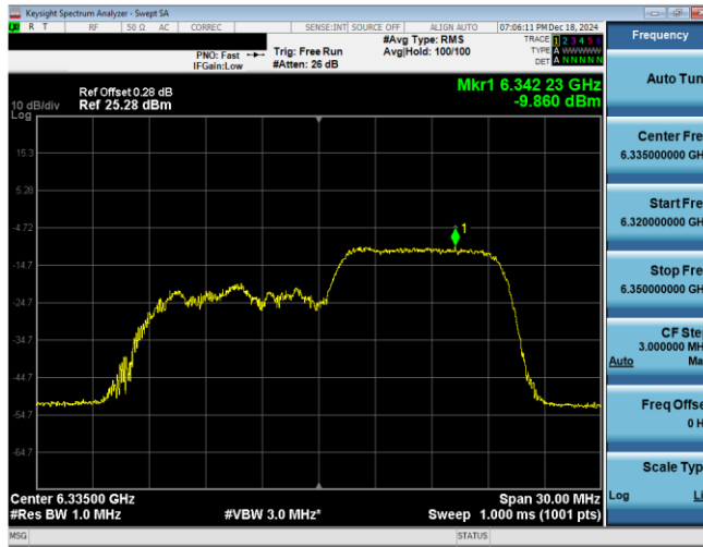
Plot 7-33. PSD Plot Antenna WF8 (20MHz 802.11ax RU106 (UNII Band 5) – Ch. 77)
