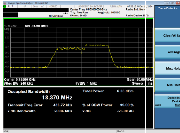
Plot 7-9. 26dB & 99% Bandwidth Plot Antenna WF8 (20MHz 802.11ax RU106 (UNII Band 7) – Ch. 181)
