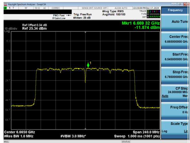
Plot 7-48. PSD Plot Antenna WF8 (160MHz 802.11ax RU996x2 (UNII Band 7) – Ch. 143)
