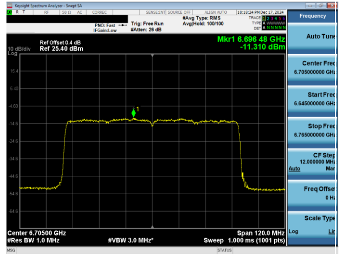
Plot 7-47. PSD Plot Antenna WF8 (80MHz 802.11ax RU996 (UNII Band 7) – Ch. 151)
