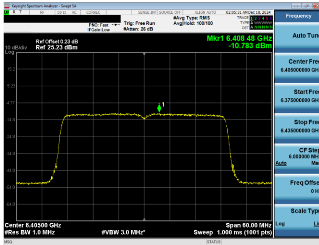
Plot 7-54. PSD Plot Antenna WF7a (40MHz 802.11ax RU484 (UNII Band 5) – Ch. 91)
