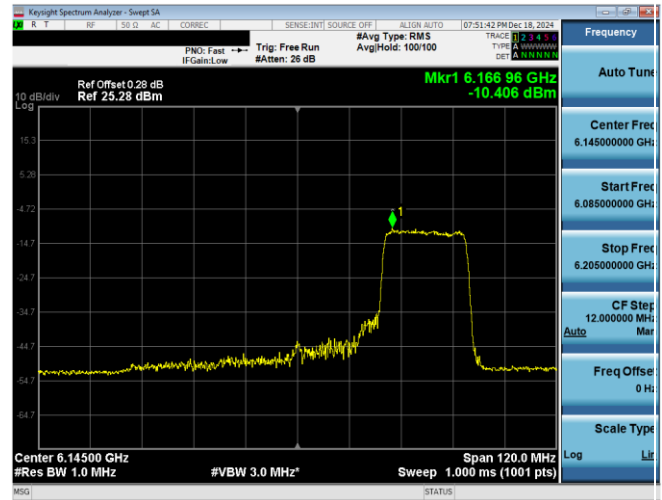
Plot 7-51. PSD Plot Antenna WF7a (80MHz 802.11ax RU242 (UNII Band 5) – Ch. 39)
