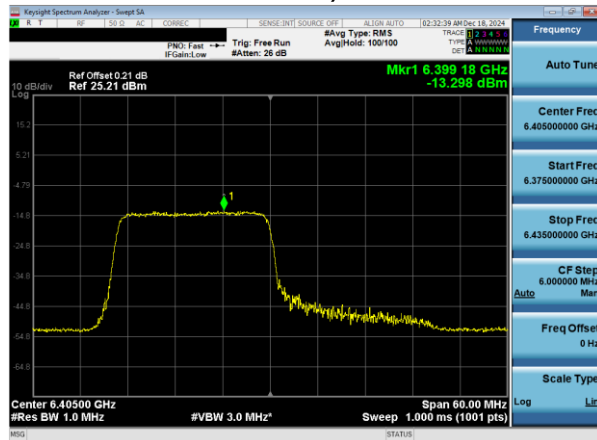
Plot 7-66. PSD Plot Antenna WF7a (40MHz 802.11ax RU242 (UNII Band 5) – Ch. 91)
