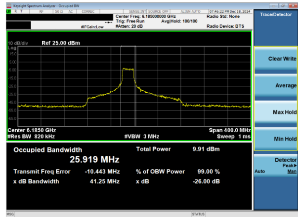
Plot 7-20. 26dB & 99% Bandwidth Plot Antenna WF7a (160MHz 802.11ax RU242 (UNII Band 5) – Ch. 47)
