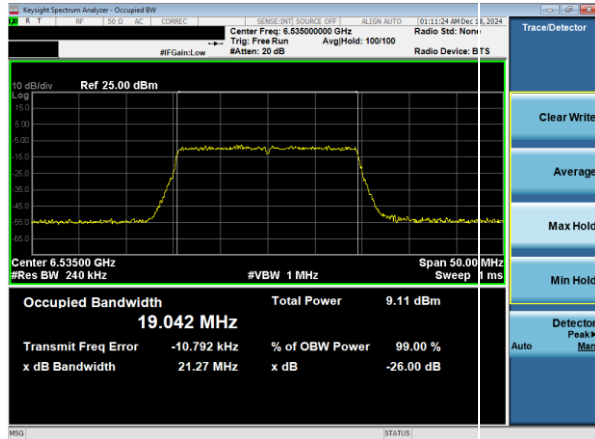
Plot 7-29. 26dB & 99% Bandwidth Plot Antenna WF7a (20MHz 802.11ax RU242 (UNII Band 7) – Ch. 117)
