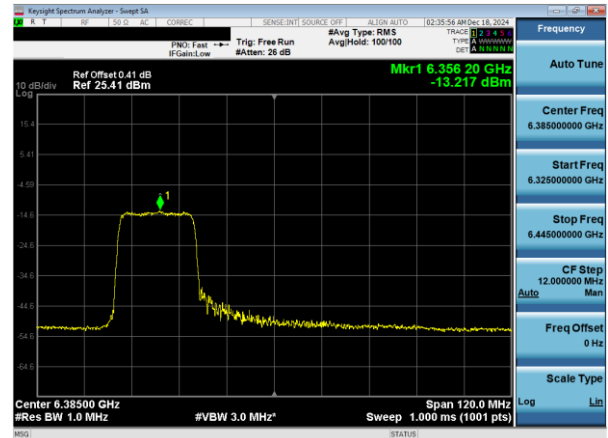
Plot 7-68. PSD Plot Antenna WF7a (80MHz 802.11ax RU106 (UNII Band 5) – Ch. 87)
