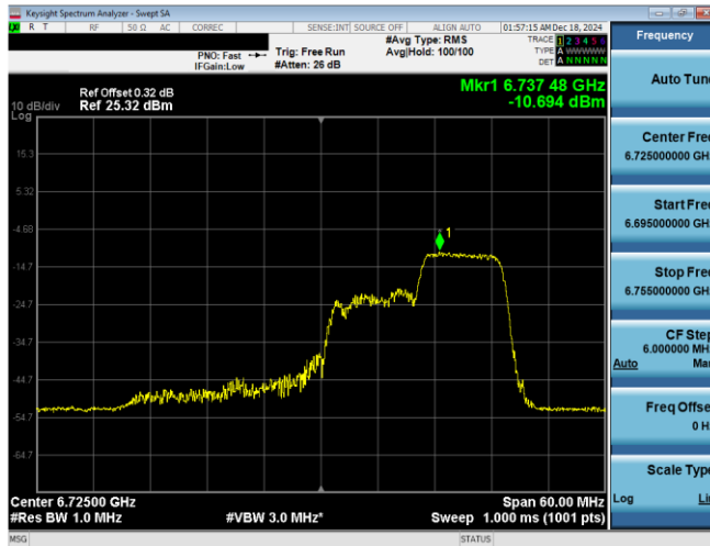
Plot 7-58. PSD Plot Antenna WF7a (40MHz 802.11ax RU106 (UNII Band 7) - Ch. 155)
