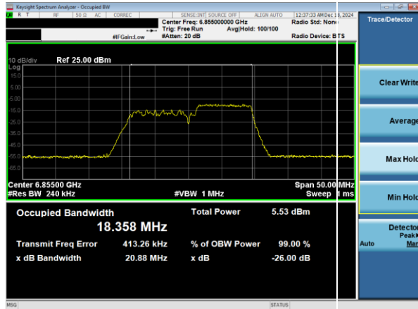
Plot 7-25. 26dB & 99% Bandwidth Plot Antenna WF7a (20MHz 802.11ax RU106 (UNII Band 7) – Ch. 181)
