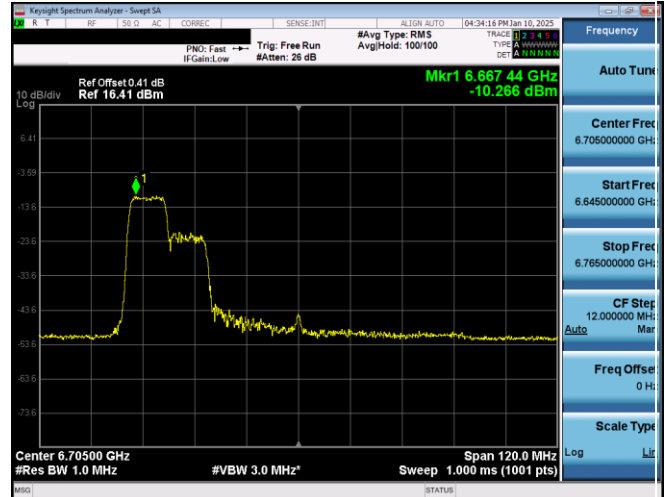
Plot 7-59. PSD Plot Antenna WF7a (80MHz 802.11ax RU106 (UNII Band 7) - Ch. 151)
