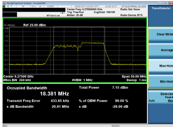
Plot 7-17. 26dB & 99% Bandwidth Plot Antenna WF7a (20MHz 802.11ax RU106 (UNII Band 5) – Ch. 65)
