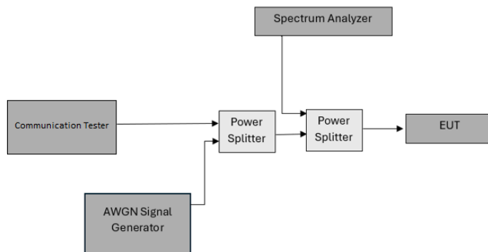
Figure 7-5. Contention-based protocol test setup, conducted method
