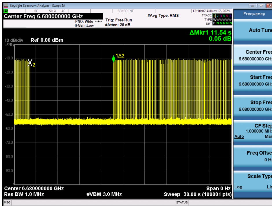
Plot 7-98. Contention Based Protocol Timing Plot – UNII 7 – 160MHz Channel 143 – Low
