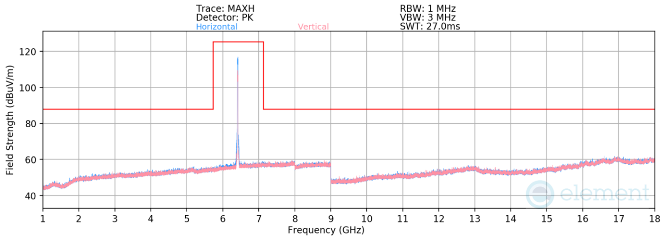
Plot 7-110. Radiated Spurious Emissions 1-18GHz SDM (802.11ax – Ch. 93)
