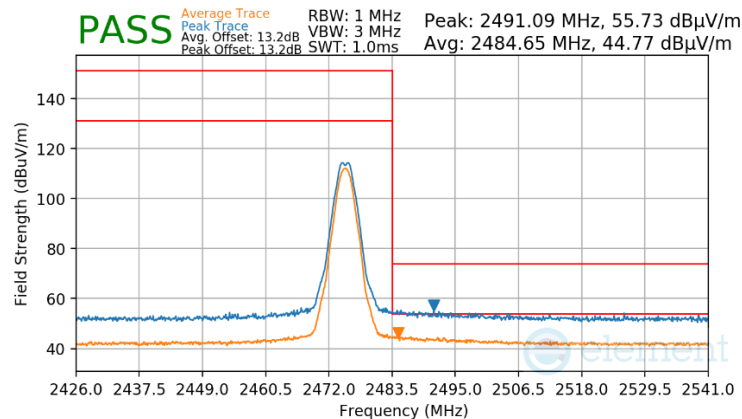
Plot 7-45. Radiated Restricted Upper Band Edge Measurement Antenna WF7b
