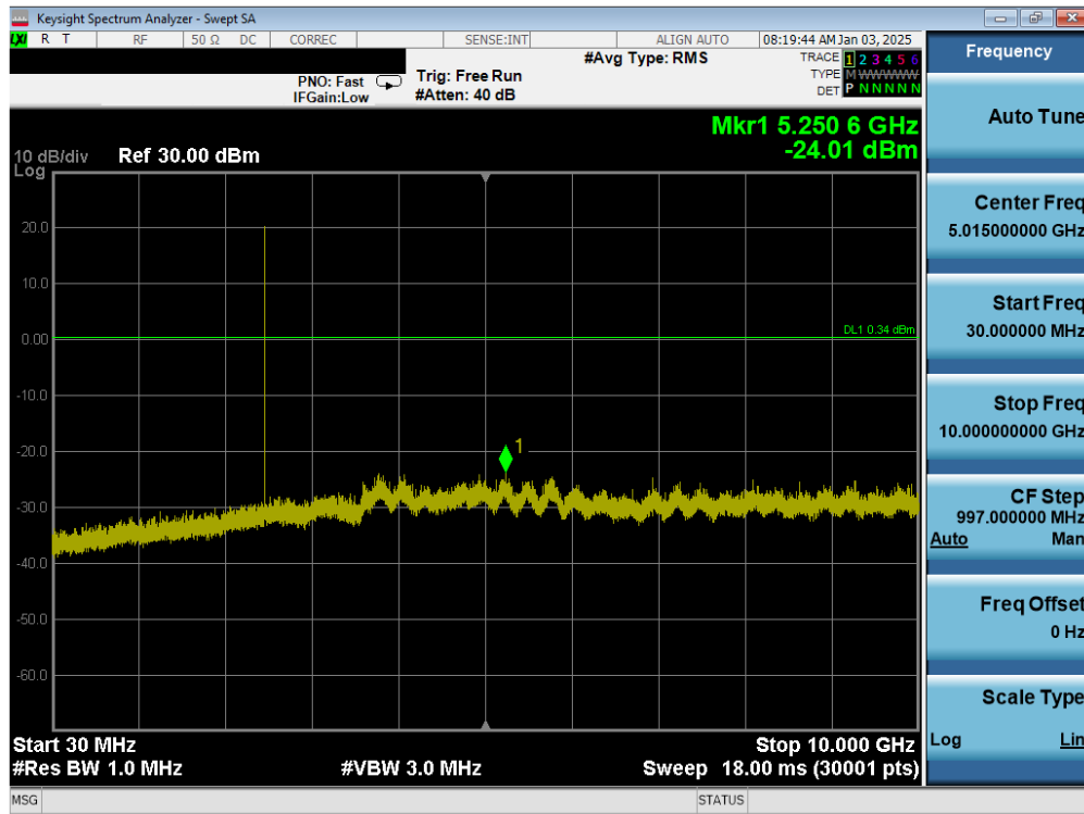
Plot 7-27. Conducted Spurious Antenna WF8 (802.15.4, ePA – Ch. 25)
