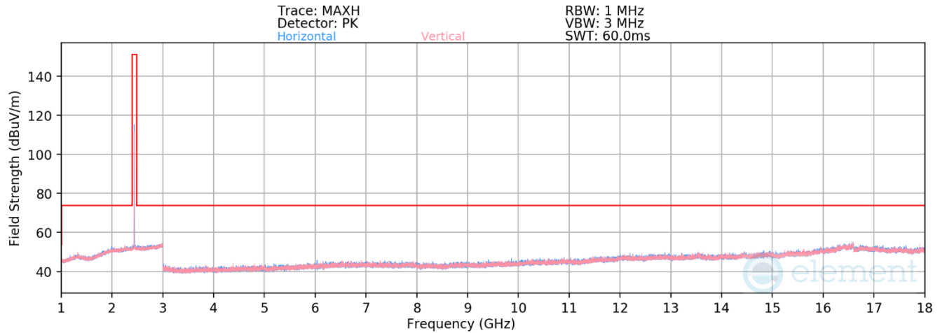
Plot 7-40. Radiated Spurious Emissions 1-18GHz Antenna WF7b (802.15.4 ePA – Ch. 18)
