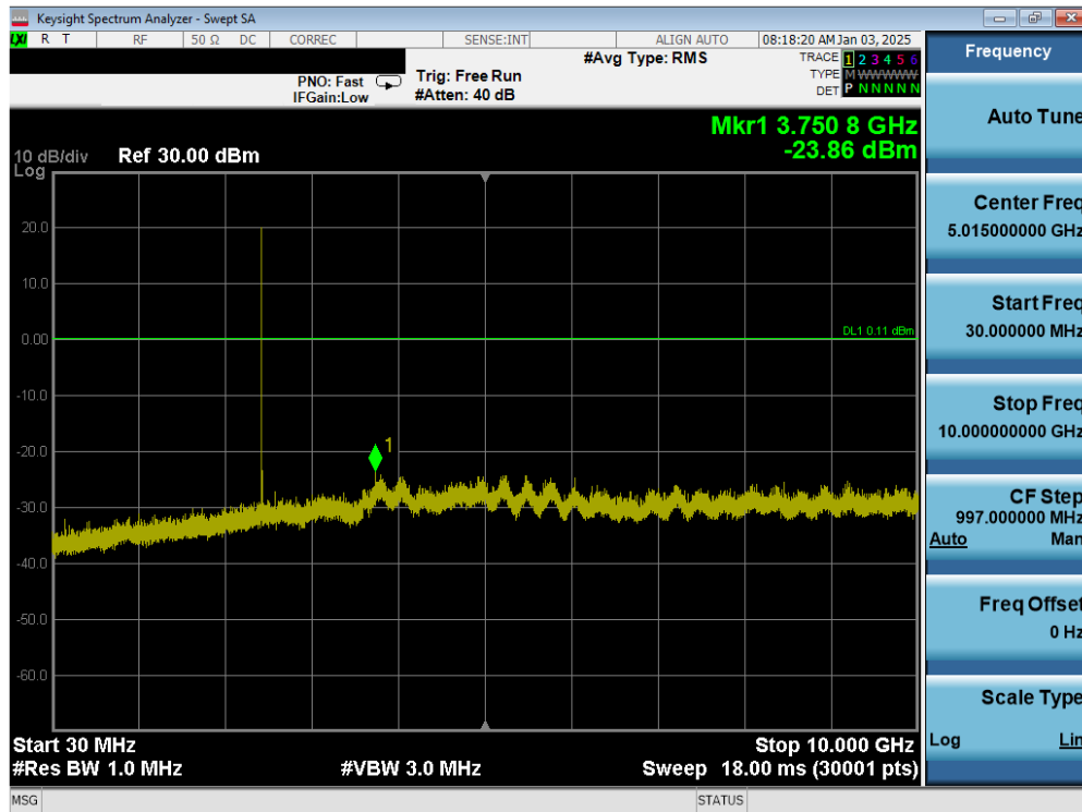
Plot 7-25. Conducted Spurious Antenna WF8 (802.15.4, ePA – Ch. 18)
