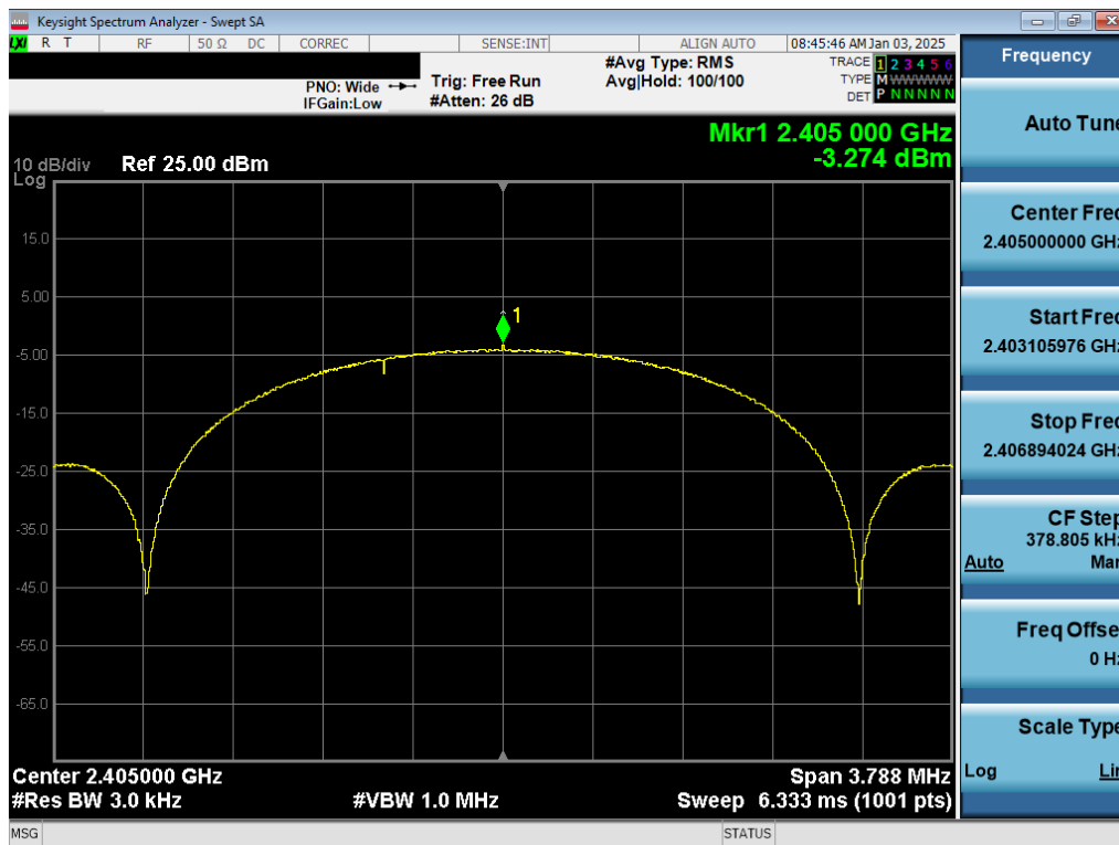
Plot 7-13. Power Spectral Density Antenna WF7b (802.15.4, ePA – Ch. 11)
