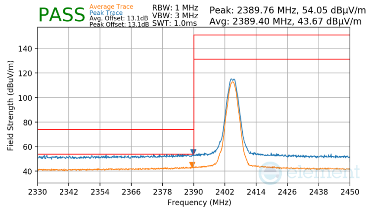
Plot 7-44. Radiated Restricted Lower Band Edge Measurement Antenna WF7b
