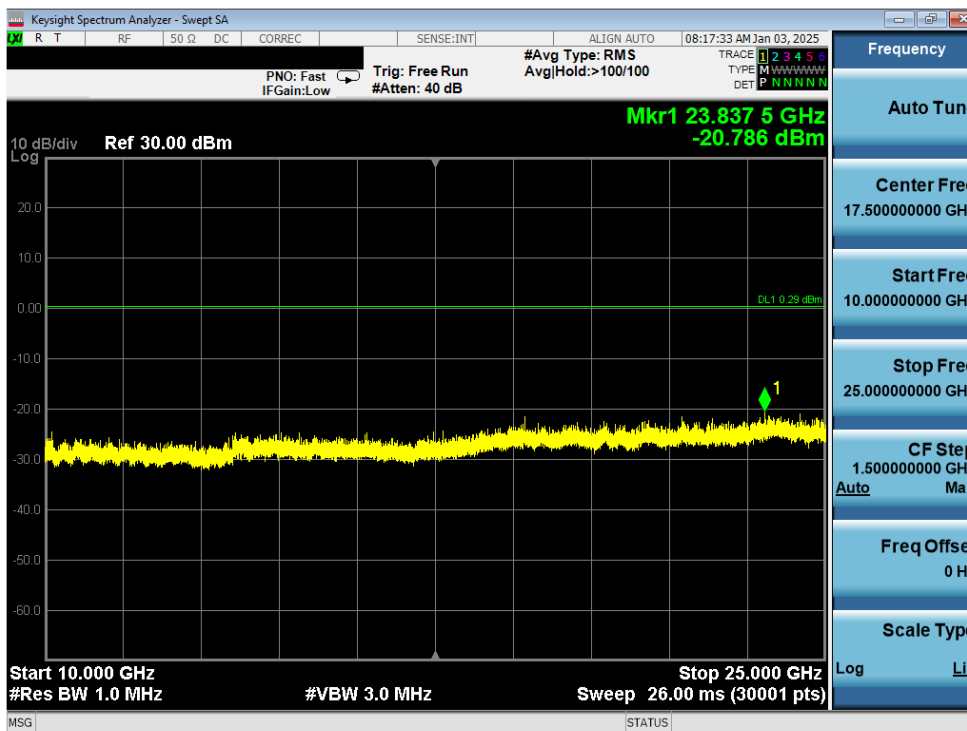
Plot 7-24. Conducted Spurious Antenna WF8 (802.15.4, ePA – Ch. 11)
