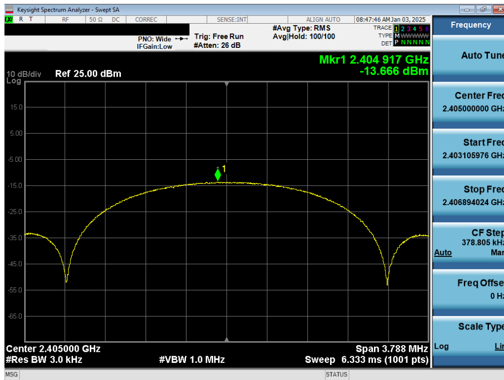
Plot 7-16. Power Spectral Density Antenna WF7b (802.15.4, iPA – Ch. 11)
