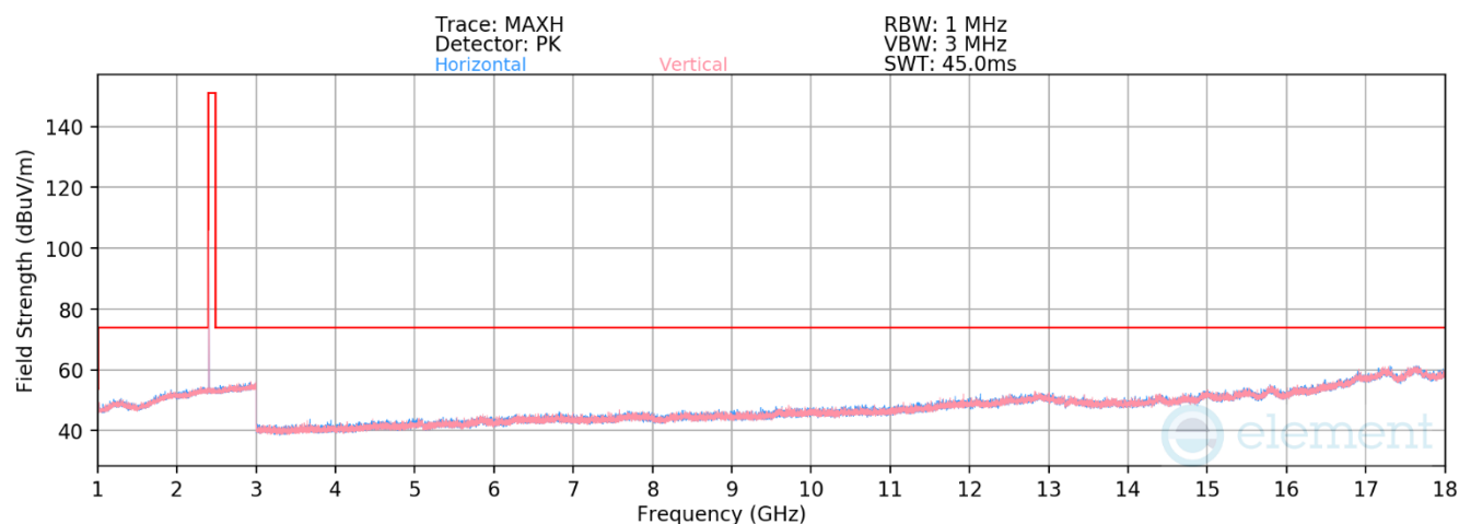
Plot 7-35. Radiated Spurious Emissions 1-18GHz Antenna WF8 (802.15.4 ePA – Ch. 11)
