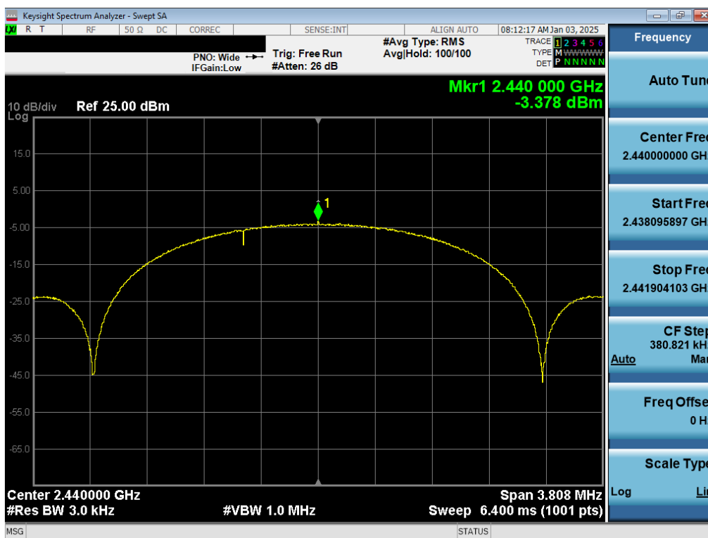
Plot 7-8. Power Spectral Density Antenna WF8 (802.15.4, ePA – Ch. 18)
