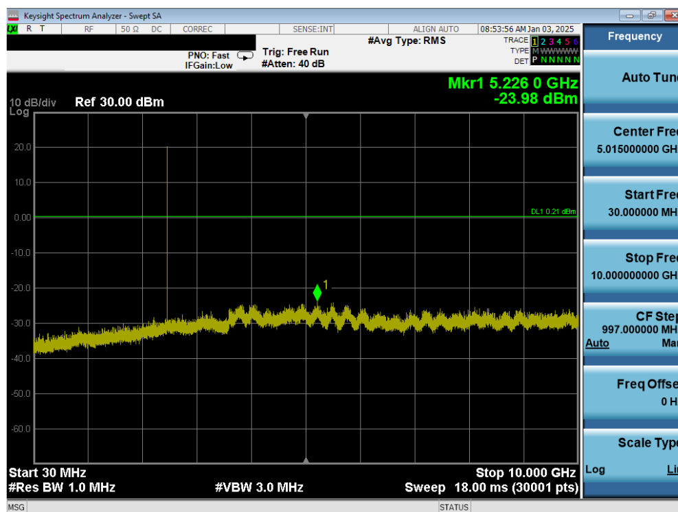
Plot 7-33. Conducted Spurious Antenna WF7b (802.15.4, ePA – Ch. 25)
