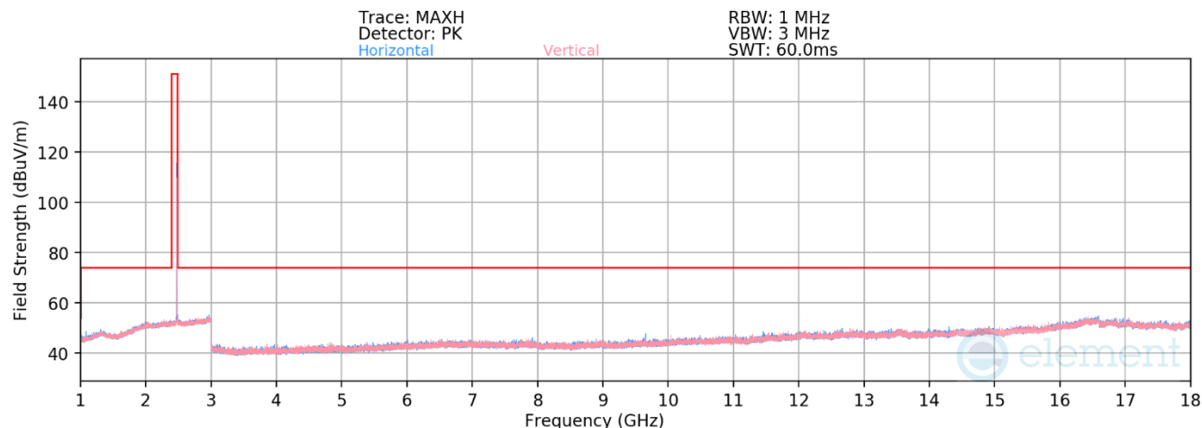
Plot 7-41. Radiated Spurious Emissions 1-18GHz Antenna WF7b (802.15.4 ePA – Ch. 25)
