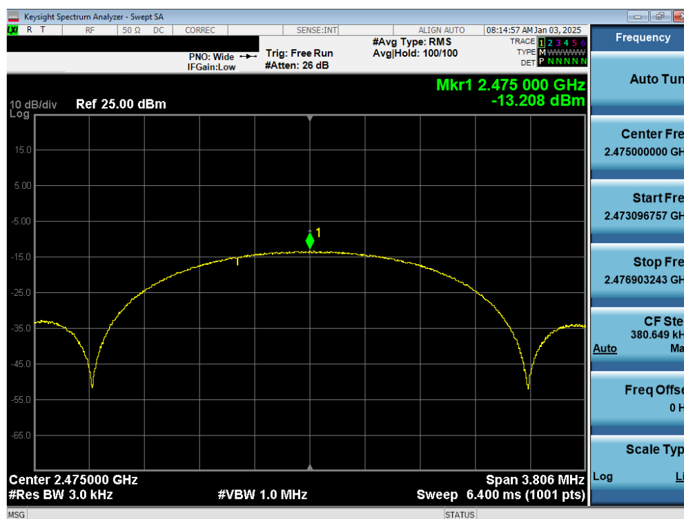
Plot 7-12. Power Spectral Density Antenna WF8 (802.15.4, iPA – Ch. 25)
