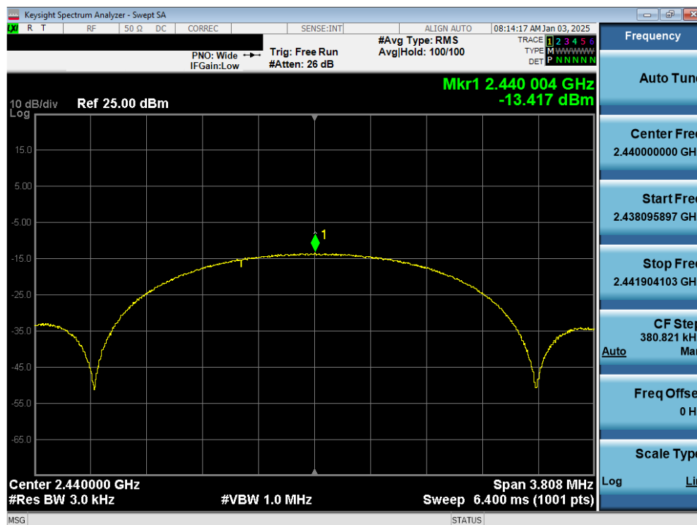
Plot 7-11. Power Spectral Density Antenna WF8 (802.15.4, iPA – Ch. 18)
