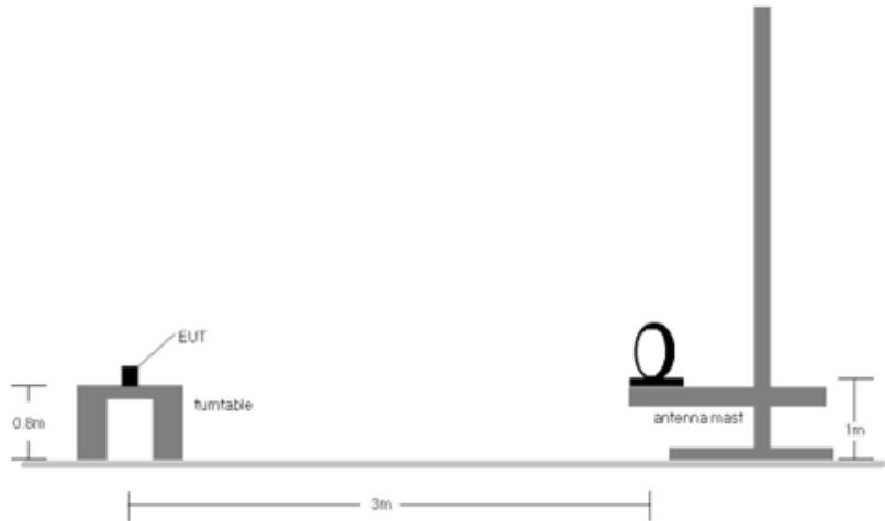
Figure 7-7. Radiated Test Setup < 30Mhz
