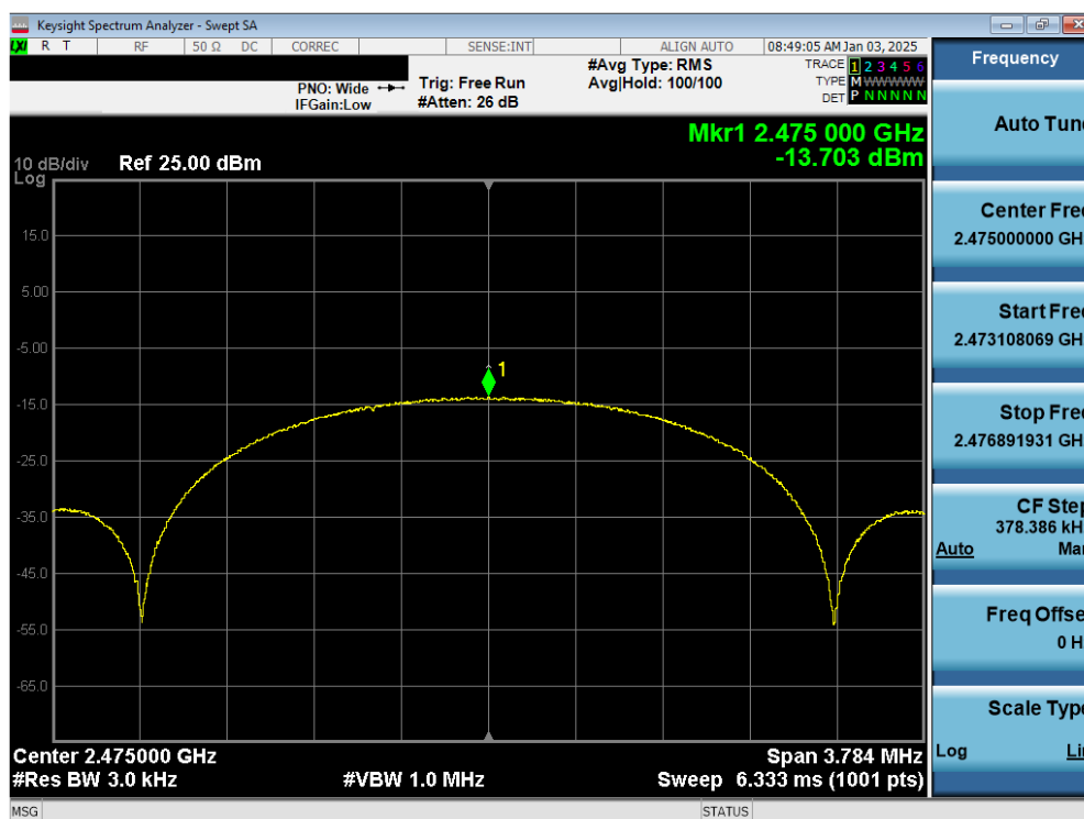
Plot 7-18. Power Spectral Density Antenna WF7b (802.15.4, iPA – Ch. 25)
