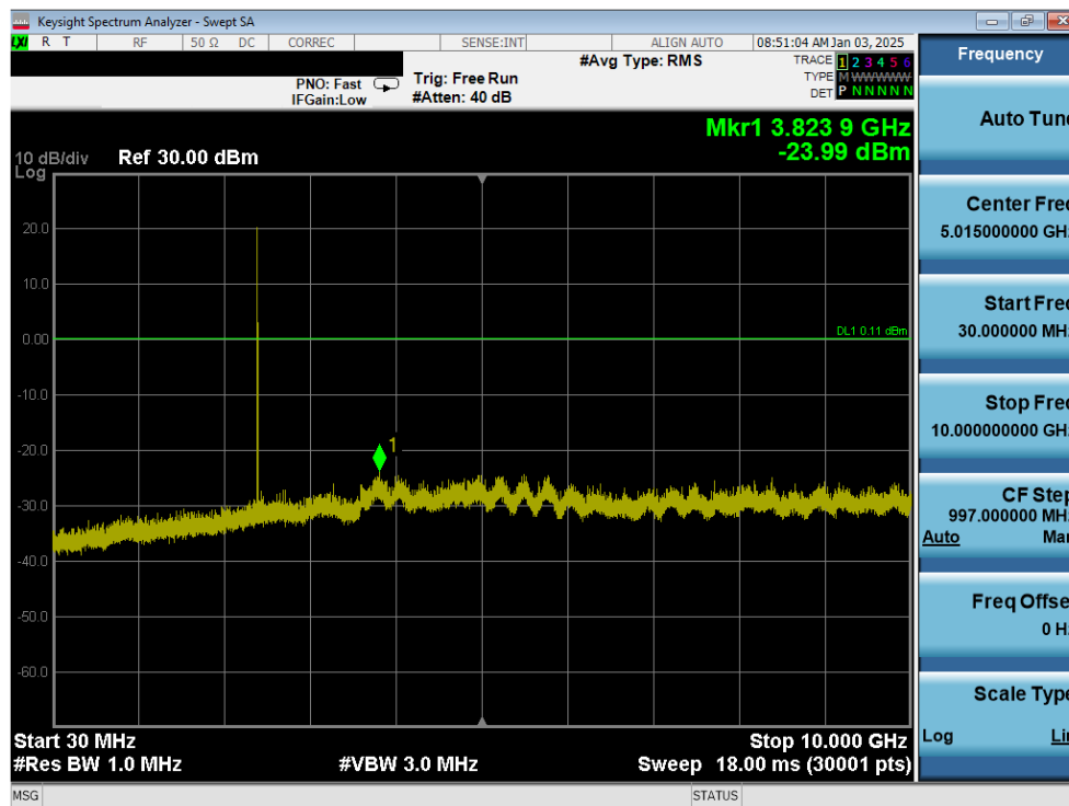
Plot 7-29. Conducted Spurious Antenna WF7b (802.15.4, ePA – Ch. 11)
