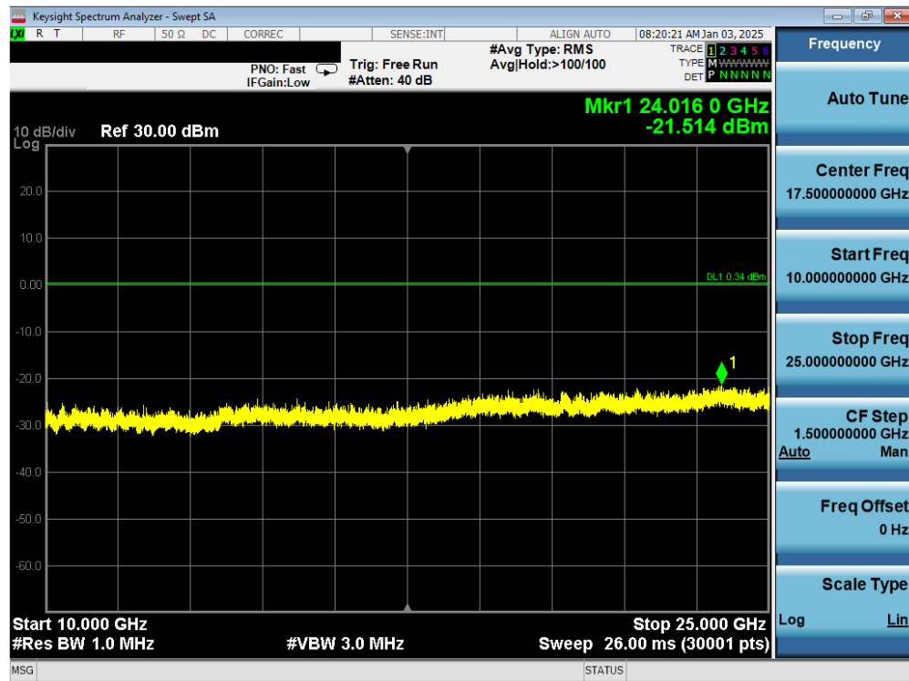
Plot 7-28. Conducted Spurious Antenna WF8 (802.15.4, ePA – Ch. 25)
