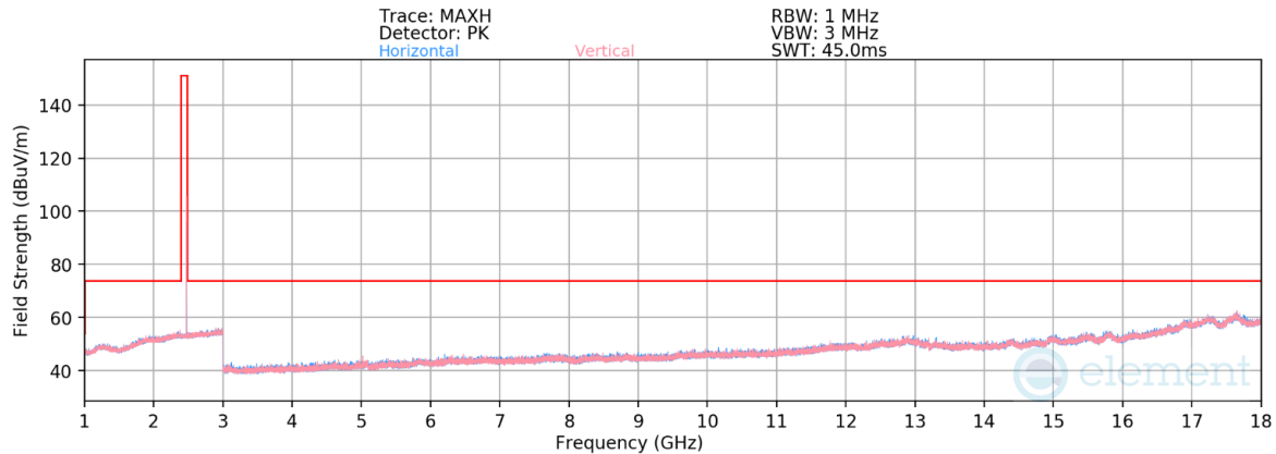
Plot 7-37. Radiated Spurious Emissions 1-18GHz Antenna WF8 (802.15.4 ePA – Ch. 25)
