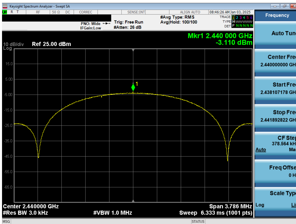
Plot 7-14. Power Spectral Density Antenna WF7b (802.15.4, ePA – Ch. 18)
