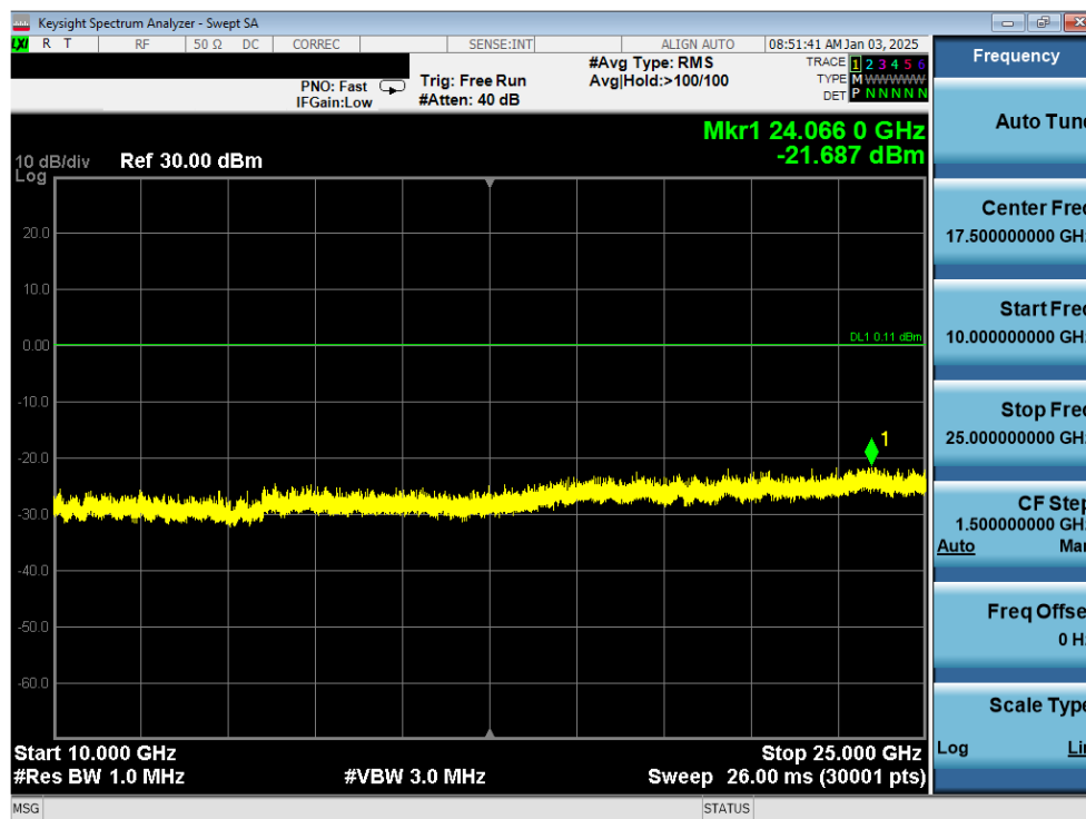
Plot 7-30. Conducted Spurious Antenna WF7b (802.15.4, ePA – Ch. 11)
