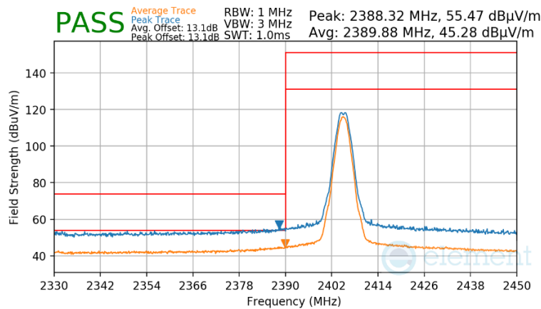
Plot 7-42. Radiated Restricted Lower Band Edge Measurement Antenna WF8
