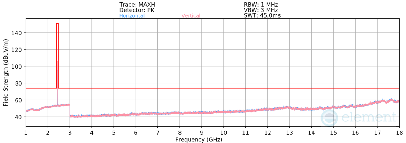
Plot 7-36. Radiated Spurious Emissions 1-18GHz Antenna WF8 (802.15.4 ePA – Ch. 18)
