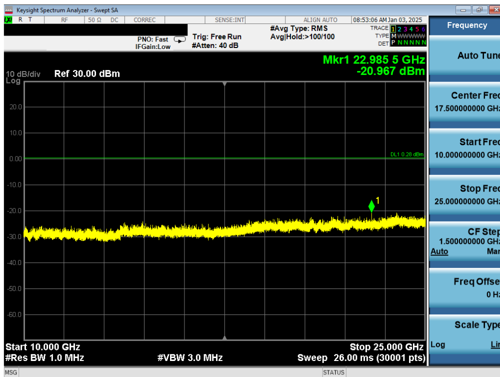
Plot 7-32. Conducted Spurious Antenna WF7b (802.15.4, ePA – Ch. 18)
