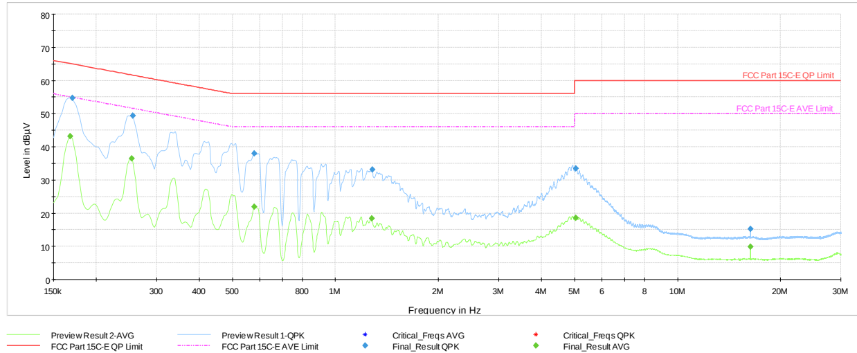
Plot 7-47. AC Line Conducted Emission with 802.15.4 Antenna WF8 (L1, Ch.25 - ePA, with AC/DC Adapter via USB-C cable with wire charger)
