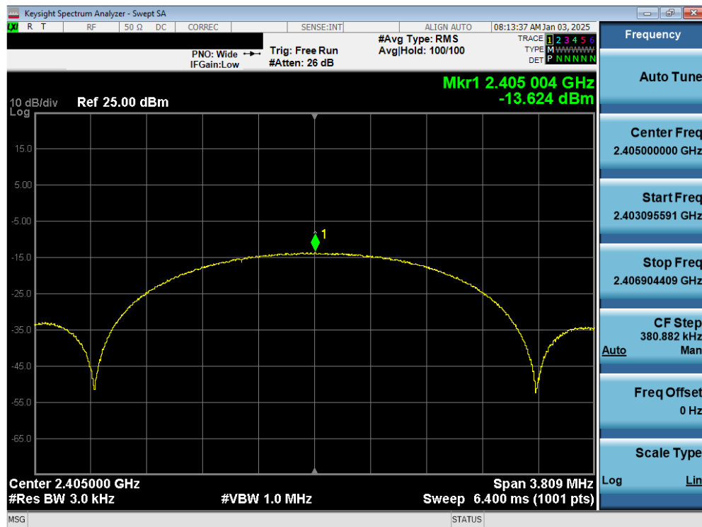
Plot 7-10. Power Spectral Density Antenna WF8 (802.15.4, iPA – Ch. 11)
