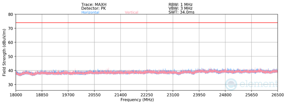
Plot 7-38. Radiated Spurious Emissions Above 18GHz Antenna WF8 (802.15.4 ePA – Ch. 25)
