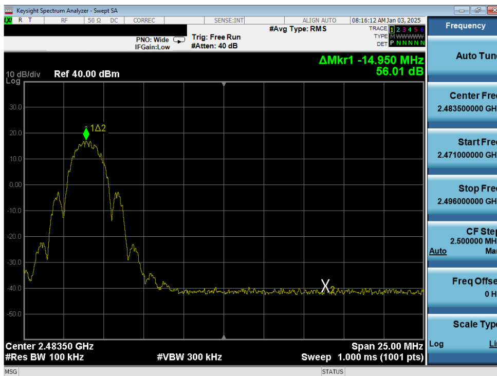
Plot 7-20. Band Edge Antenna WF8 (802.15.4, ePA – Ch. 25)
