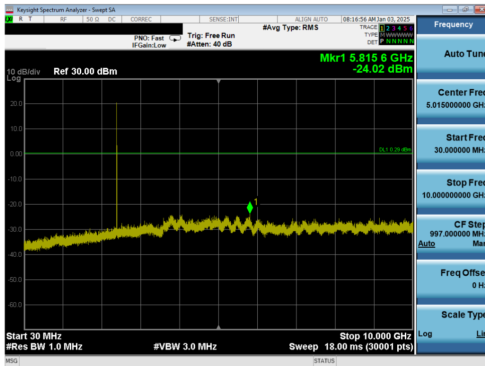
Plot 7-23. Conducted Spurious Antenna WF8 (802.15.4, ePA – Ch. 11)
