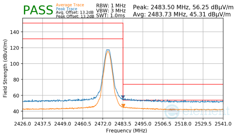
Plot 7-43. Radiated Restricted Upper Band Edge Measurement Antenna WF8
