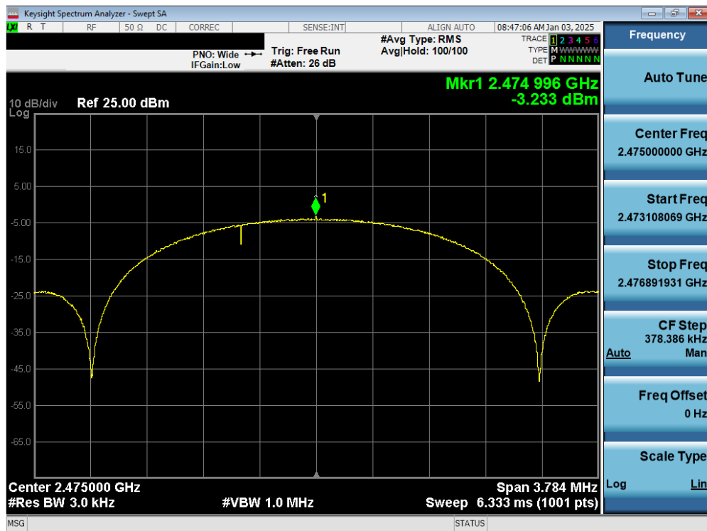
Plot 7-15. Power Spectral Density Antenna WF7b (802.15.4, ePA – Ch. 25)
