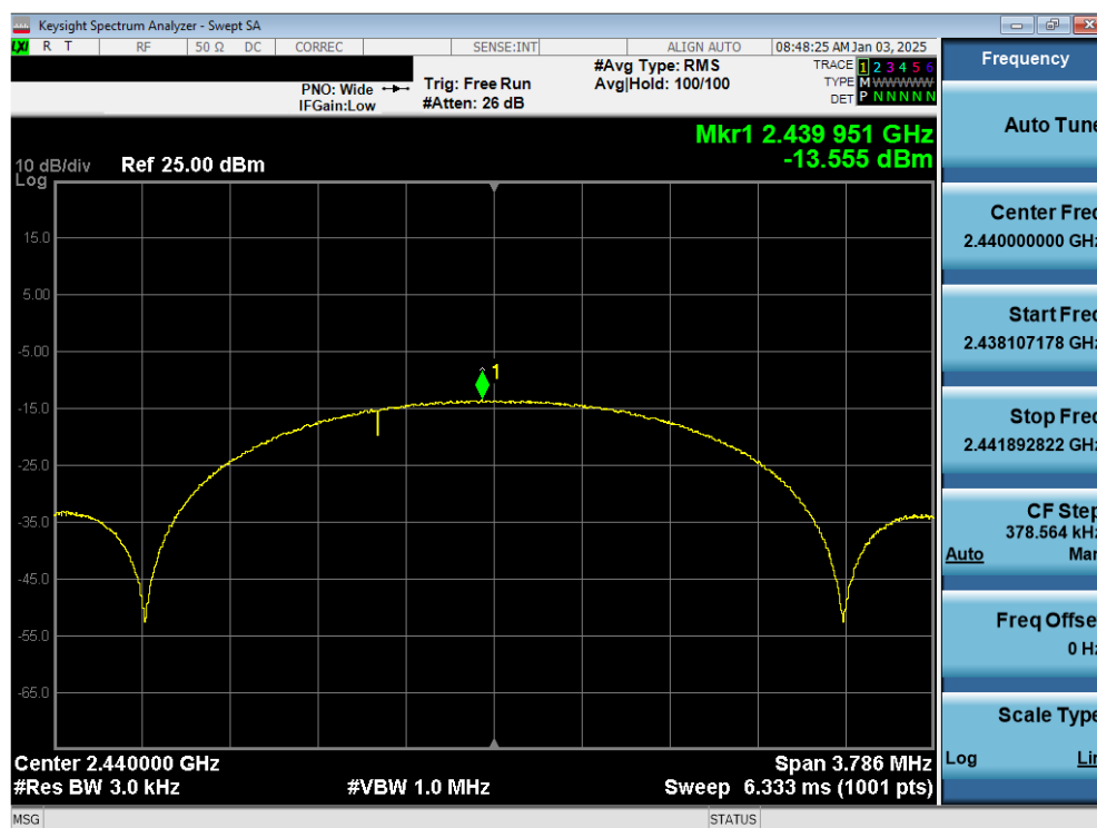
Plot 7-17. Power Spectral Density Antenna WF7b (802.15.4, iPA – Ch. 18)
