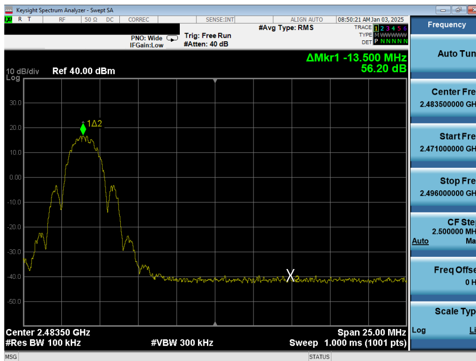
Plot 7-22. Band Edge Antenna WF7b (802.15.4, ePA – Ch. 25)
