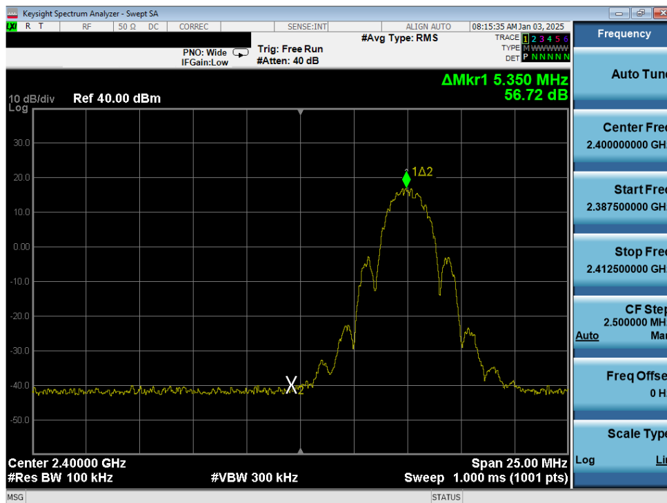
Plot 7-19. Band Edge Antenna WF8 (802.15.4, ePA – Ch. 11)
