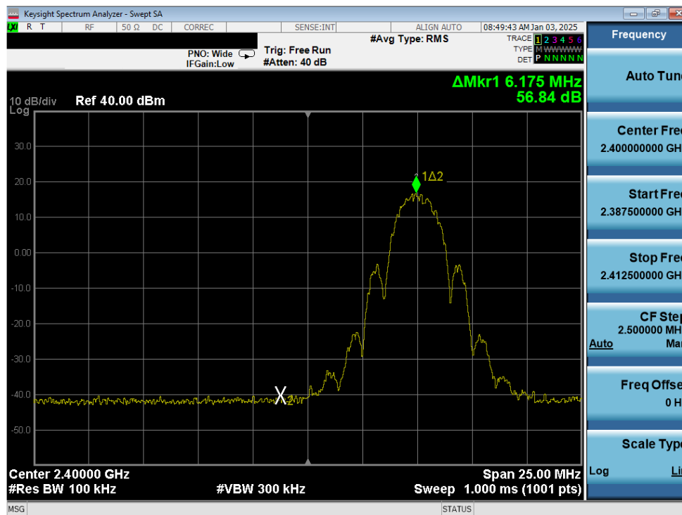
Plot 7-21. Band Edge Antenna WF7b (802.15.4, ePA – Ch. 11)
