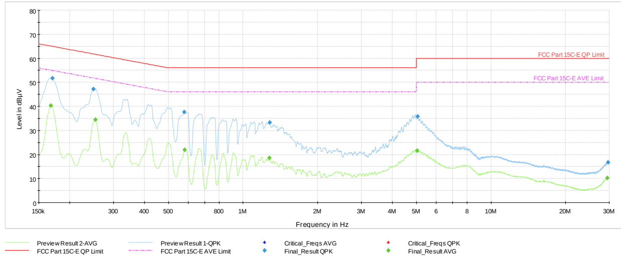
Plot 7-48. AC Line Conducted Emission with 802.15.4 Antenna WF8 (N, Ch.25 - ePA, with AC/DC Adapter via USB-C cable with wire charger)
