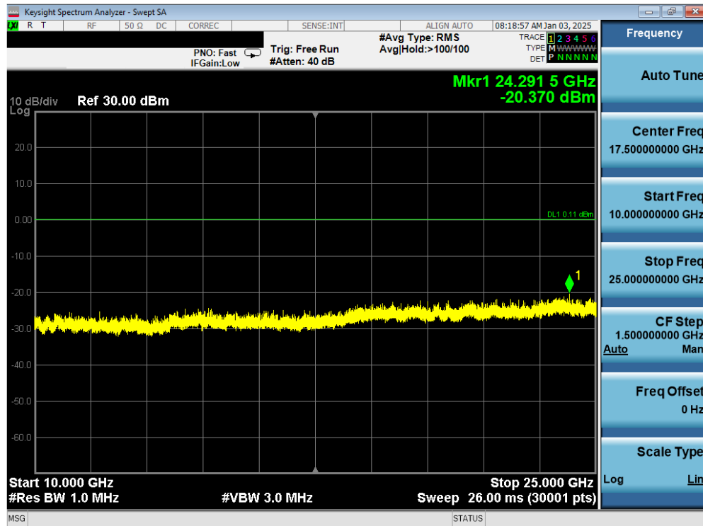
Plot 7-26. Conducted Spurious Antenna WF8 (802.15.4, ePA – Ch. 18)
