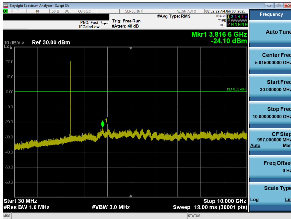
Plot 7-31. Conducted Spurious Antenna WF7b (802.15.4, ePA – Ch. 18)
