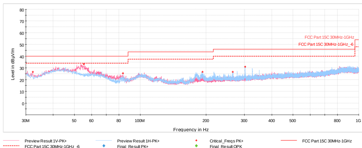
Plot 7-46. Radiated Spurious Emissions 30MHz-1GHz Antenna WF8 (ePA - Ch.25, with AC/DC Adapter via USB-C cable with wire charger)
