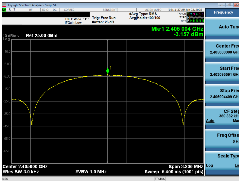
Plot 7-7. Power Spectral Density Antenna WF8 (802.15.4, ePA – Ch. 11)
