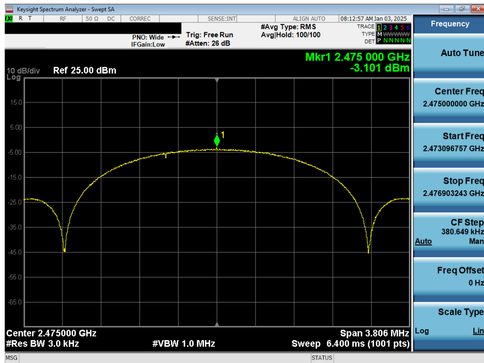
Plot 7-9. Power Spectral Density Antenna WF8 (802.15.4, ePA – Ch. 25)
