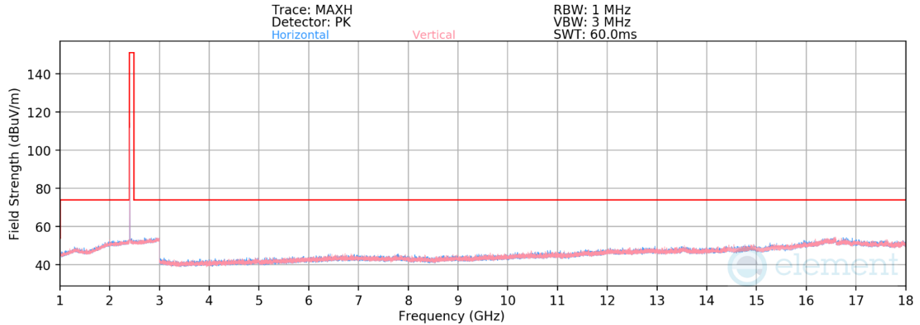
Plot 7-39. Radiated Spurious Emissions 1-18GHz Antenna WF7b (802.15.4 ePA – Ch. 11)
