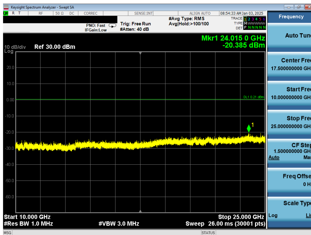
Plot 7-34. Conducted Spurious Antenna WF7b (802.15.4, ePA – Ch. 25)
