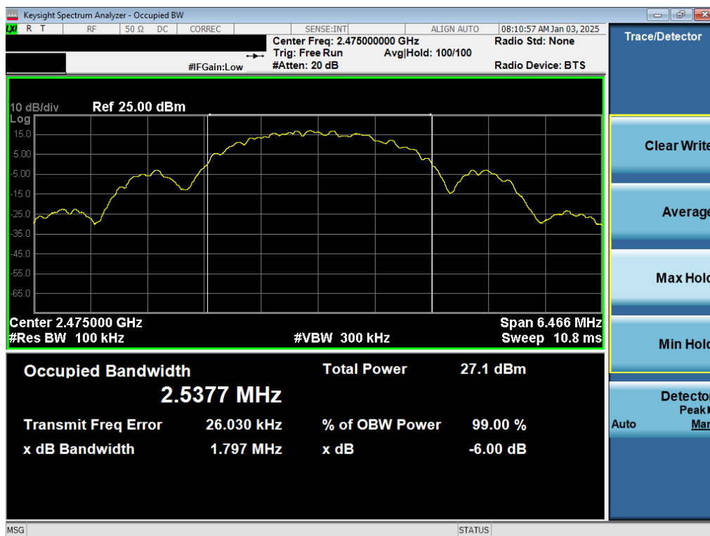
Plot 7-3. 6dB BW & 99% OBW Antenna WF8 (802.15.4, Ch. 25)
