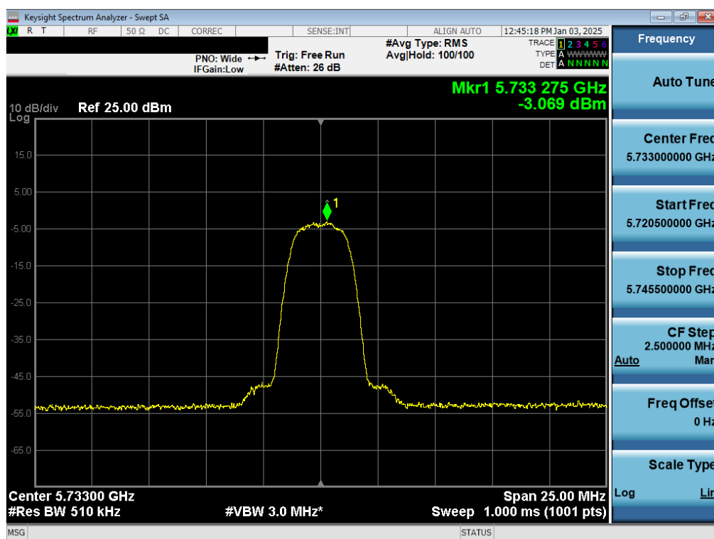
Plot 7-56. PSD TxBF Antenna WF7a (NB UNII HDR4, iPA – 5733MHz)
