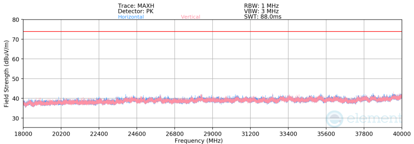
Plot 7-67. Radiated Spurious Emissions Above 18GHz (NB UNII BDR, ePA - 5789MHz)
