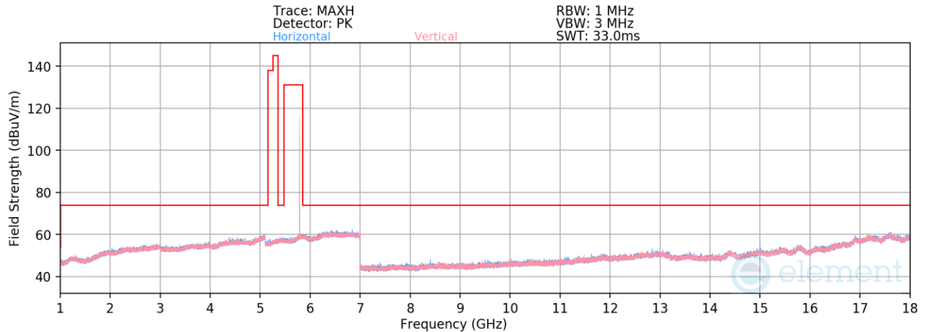
Plot 7-66. Radiated Spurious Emissions 1-18GHz TxBF (NB UNII BDR, ePA - 5789MHz)
