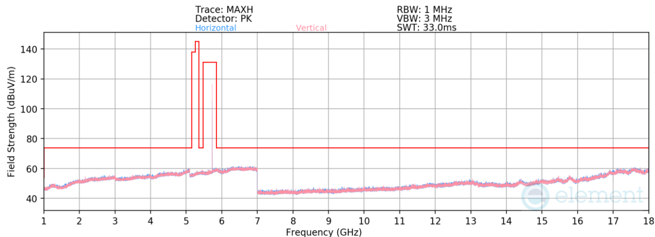
Plot 7-65. Radiated Spurious Emissions 1-18GHz TxBF (NB UNII BDR, ePA - 5733MHz)
