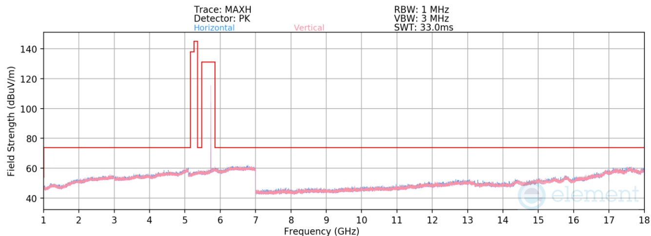
Plot 7-73. Radiated Spurious Emissions 1-18GHz TxBF (NB UNII HDR4, ePA - 5733MHz)
