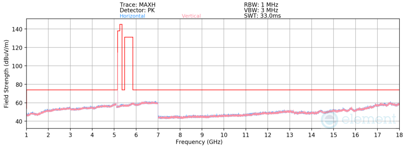
Plot 7-61. Radiated Spurious Emissions 1-18GHz TxBF (NB UNII BDR, ePA – 5162MHz)
