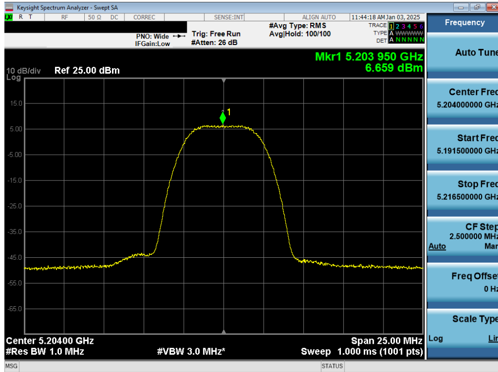
Plot 7-45. PSD TxBF Antenna WF8 (NB UNII HDR8, ePA – 5204MHz)
