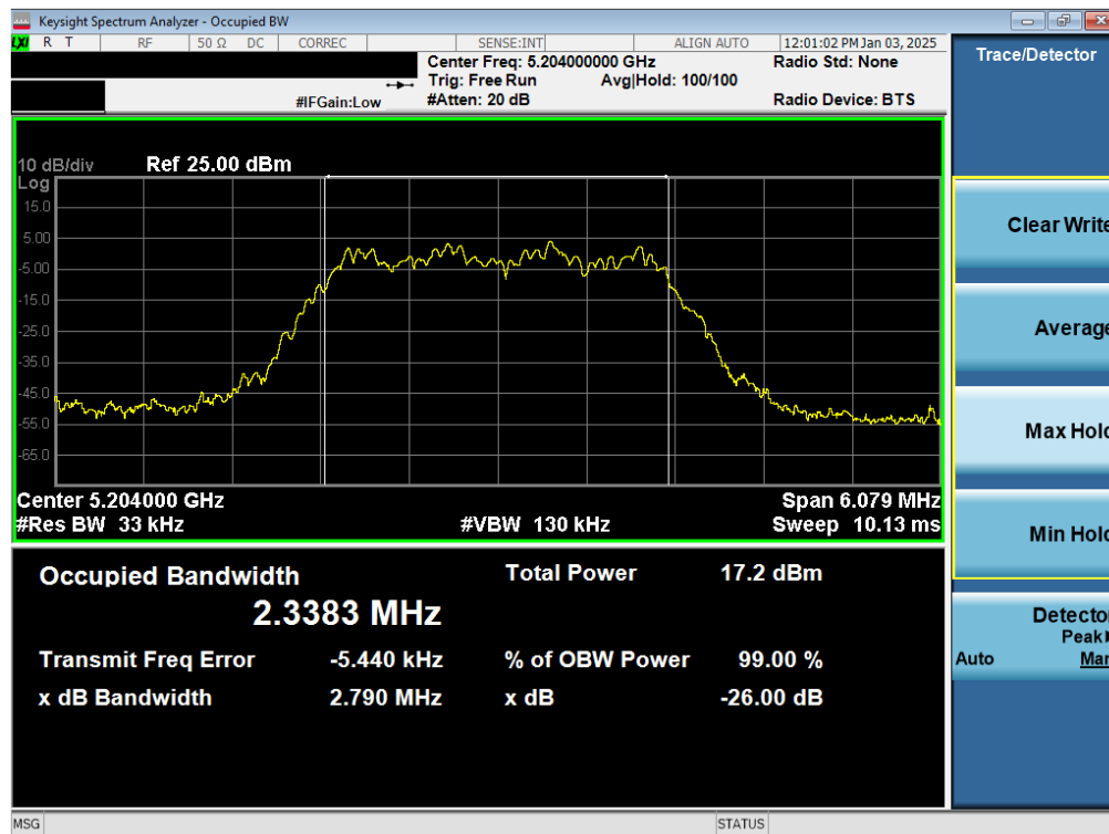
Plot 7-5. 26dB BW & 99% OBW Antenna WF7a (NB UNII HDR4, ePA- 5204MHz)
