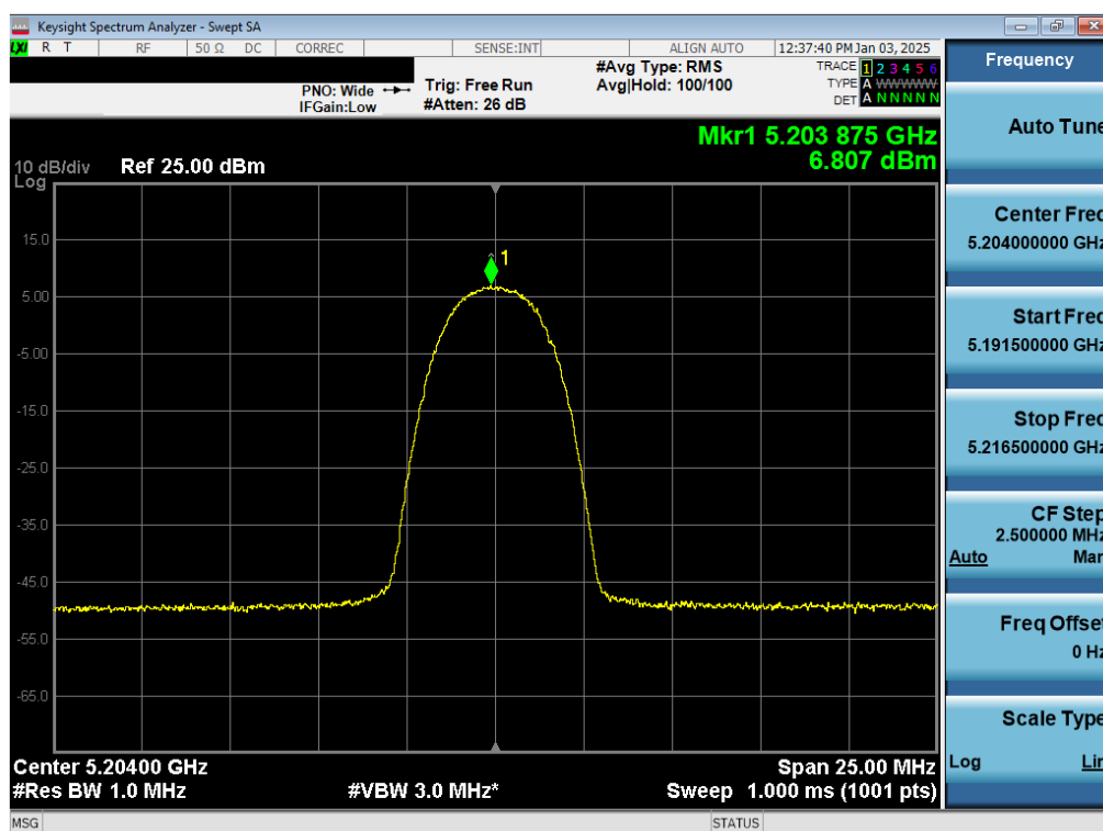
Plot 7-42. PSD TxBF Antenna WF7a (NB UNII HDR4, ePA – 5204MHz)
