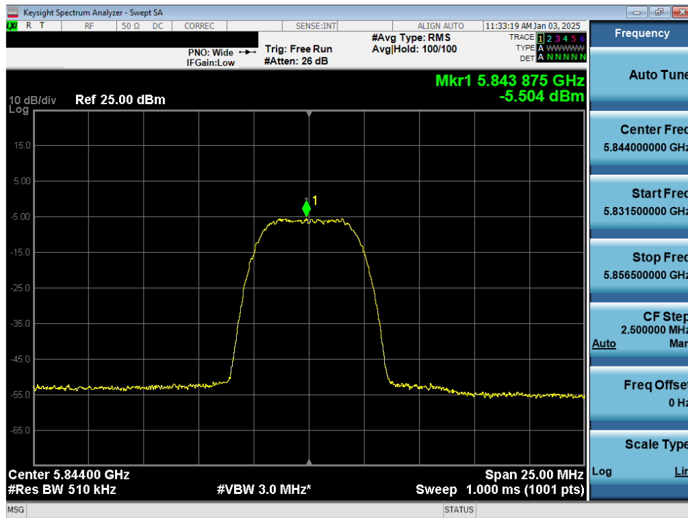
Plot 7-24. PSD Antenna WF8 (NB UNII HDR8, iPA – 5844MHz)
