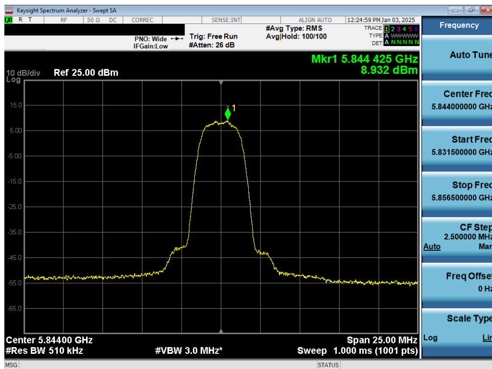
Plot 7-33. PSD Antenna WF7a (NB UNII HDR4, ePA – 5844MHz)
