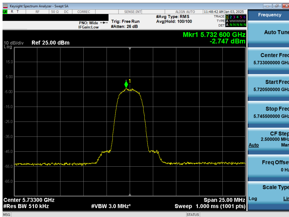
Plot 7-55. PSD TxBF Antenna WF8 (NB UNII HDR4, iPA – 5733MHz)
