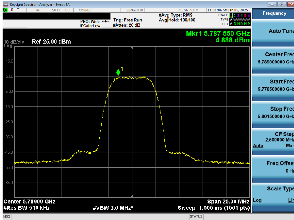
Plot 7-23. PSD Antenna WF8 (NB UNII HDR8, ePA – 5789MHz)
