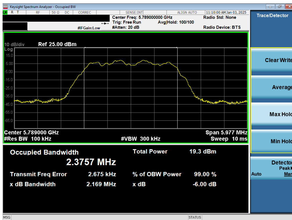
Plot 7-8. 6dB BW & 99% OBW Antenna WF8 (NB UNII HDR4, 5789MHz)
