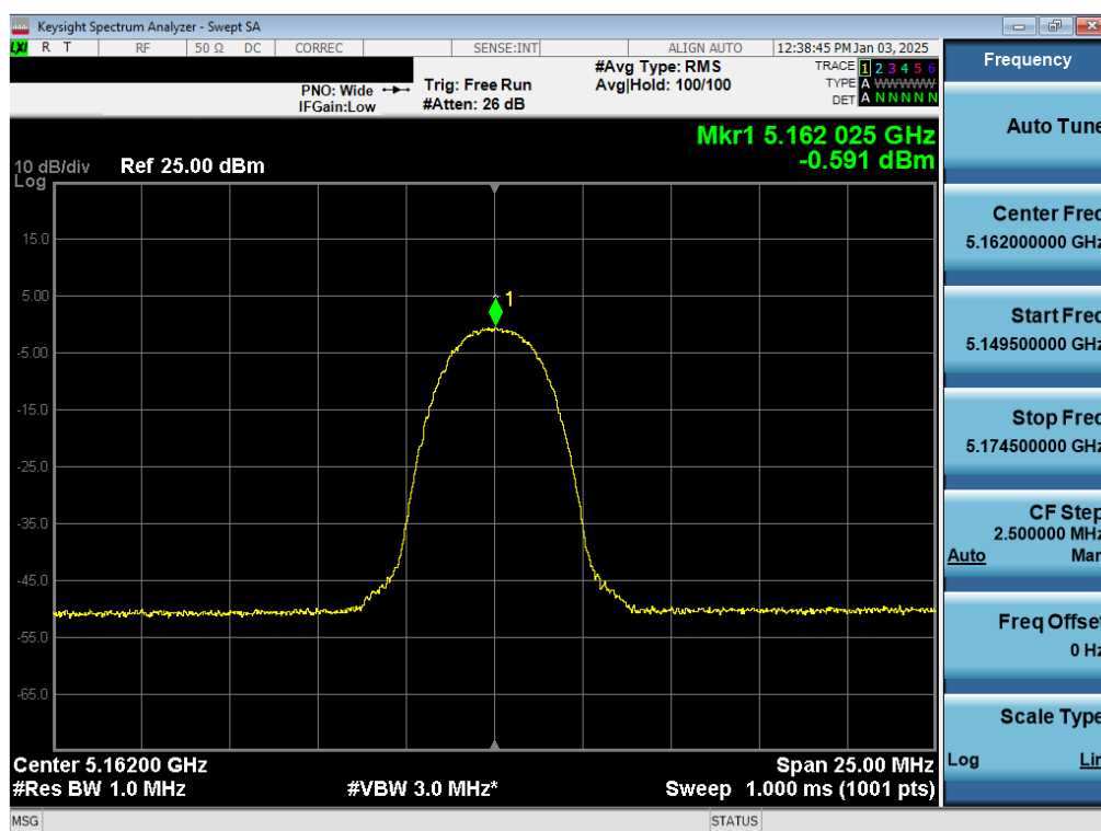
Plot 7-44. PSD TxBF Antenna WF7a (NB UNII HDR4, iPA – 5162MHz)
