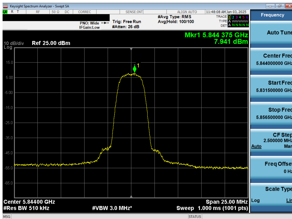
Plot 7-53. PSD TxBF Antenna WF8 (NB UNII HDR4, ePA – 5844MHz)
