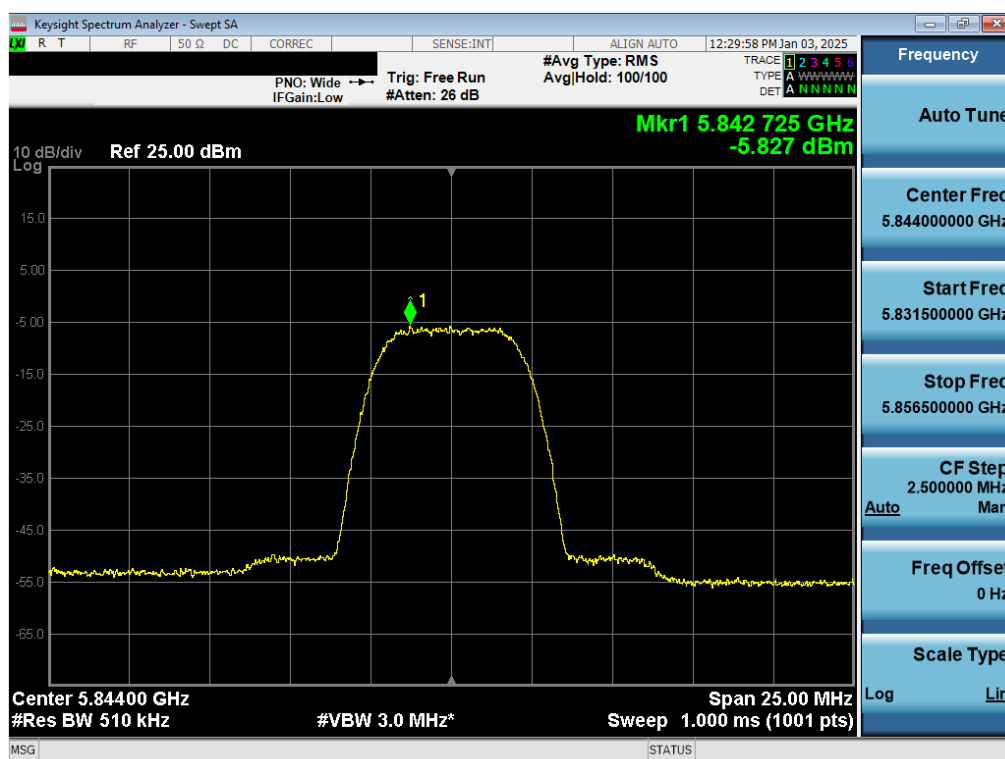
Plot 7-36. PSD Antenna WF7a (NB UNII HDR8, iPA – 5844MHz)
