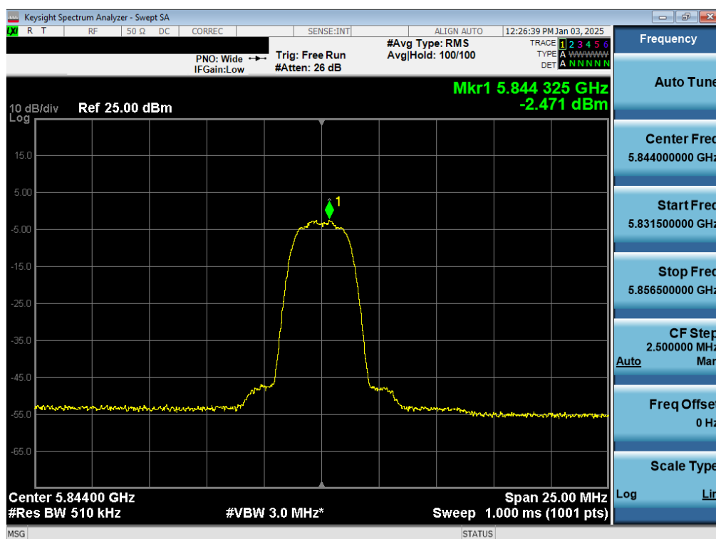
Plot 7-34. PSD Antenna WF7a (NB UNII HDR4, iPA – 5844MHz)
