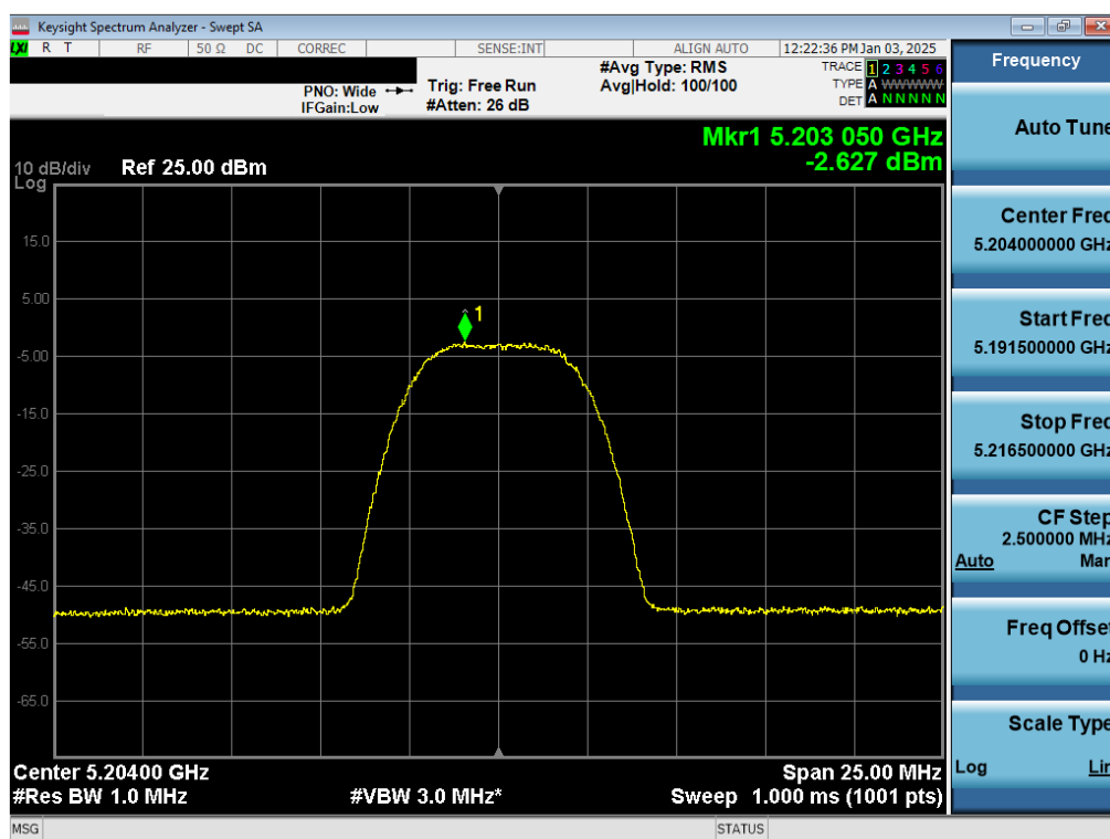
Plot 7-30. PSD Antenna WF7a (NB UNII HDR8, iPA – 5204MHz)
