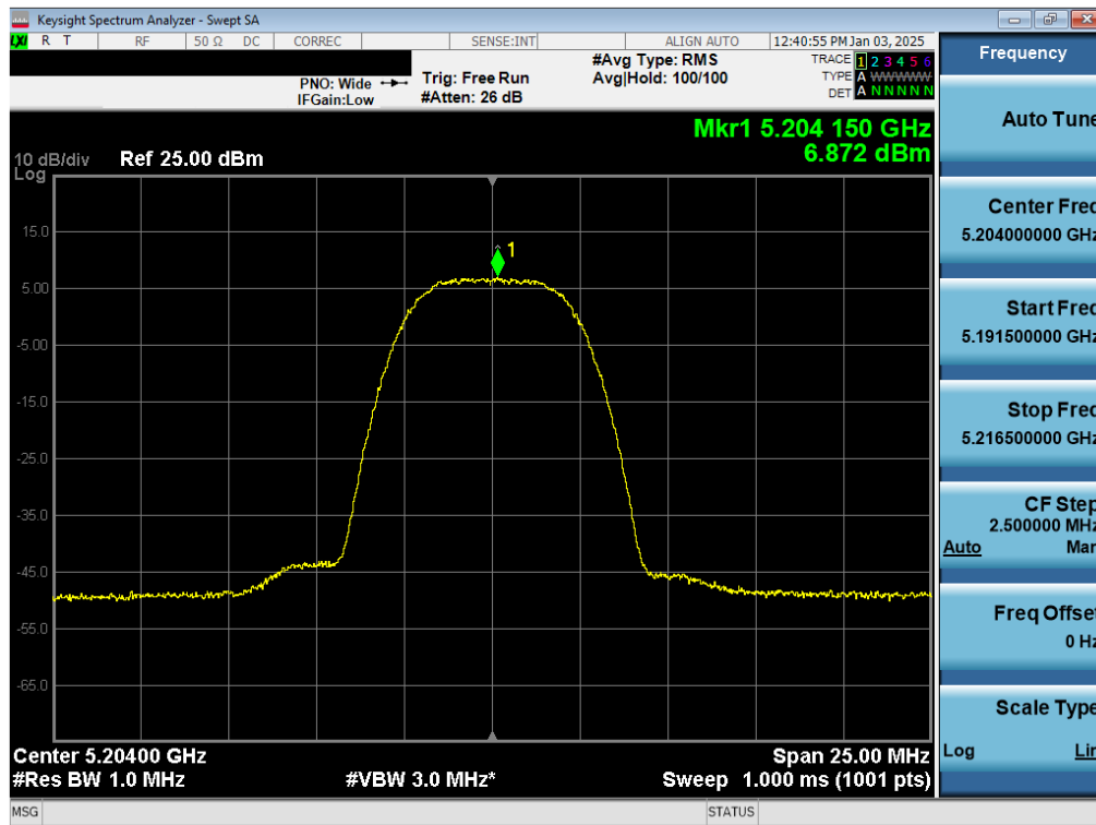
Plot 7-46. PSD TxBF Antenna WF7a (NB UNII HDR8, ePA – 5204MHz)
