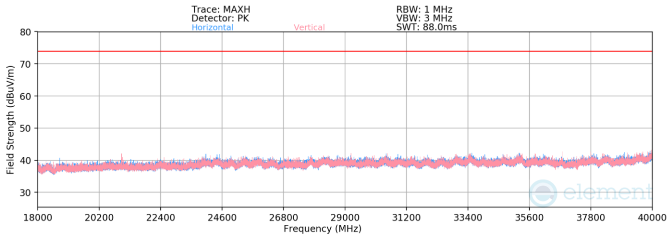
Plot 7-71. Radiated Spurious Emissions Above 18GHz (NB UNII HDR4, ePA – 5204MHz)
