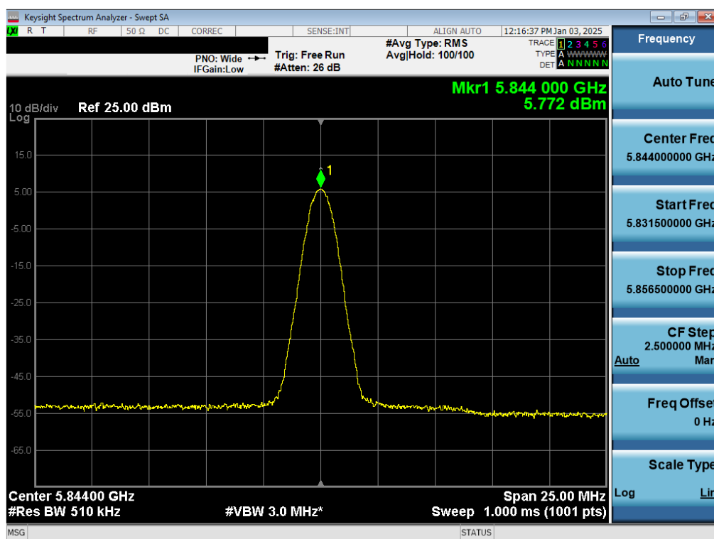
Plot 7-32. PSD Antenna WF7a (NB UNII BDR, iPA – 5844MHz)
