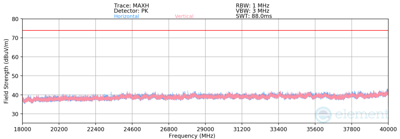
Plot 7-75. Radiated Spurious Emissions Above 18GHz (NB UNII HDR4, ePA – 5789MHz)
