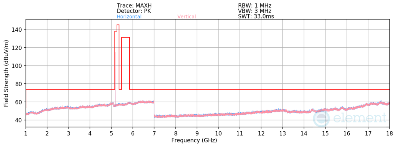
Plot 7-62. Radiated Spurious Emissions 1-18GHz TxBF (NB UNII BDR, ePA – 5204MHz)
