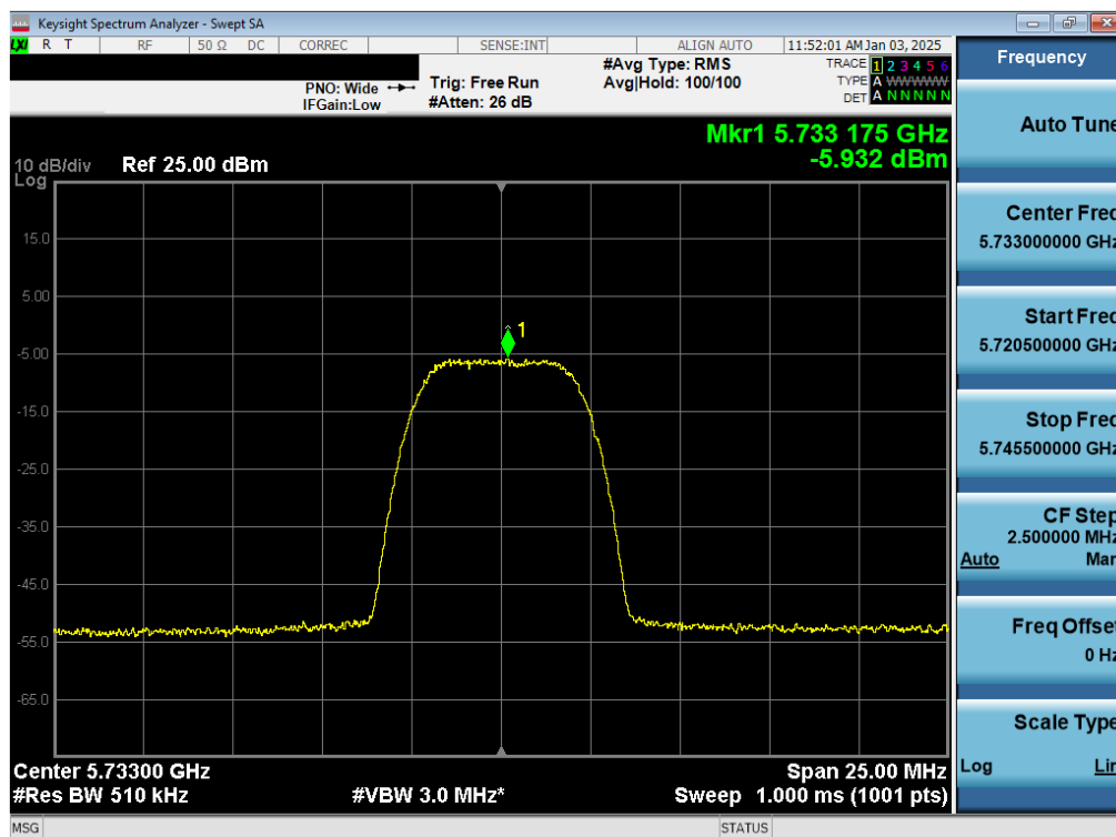
Plot 7-59. PSD TxBF Antenna WF8 (NB UNII HDR8, iPA – 5733MHz)
