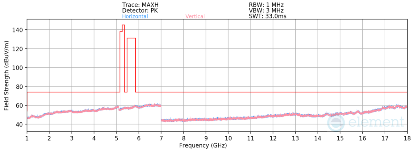
Plot 7-70. Radiated Spurious Emissions 1-18GHz TxBF (NB UNII HDR4, ePA – 5204MHz)
