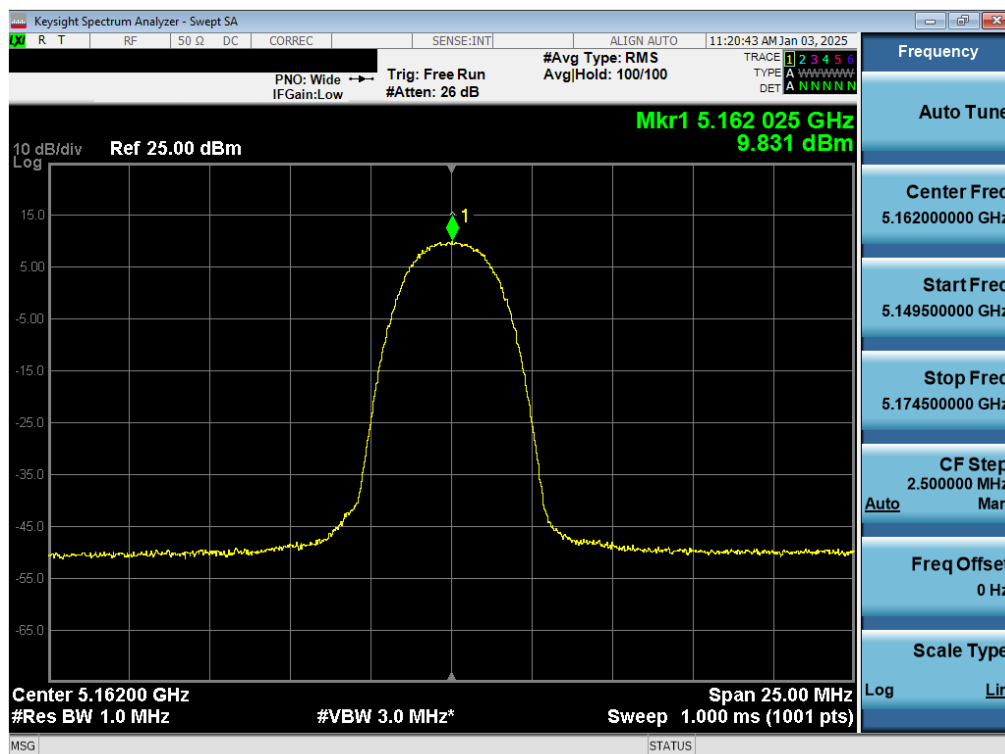
Plot 7-15. PSD Antenna WF8 (NB UNII HDR4, ePA – 5162MHz)
