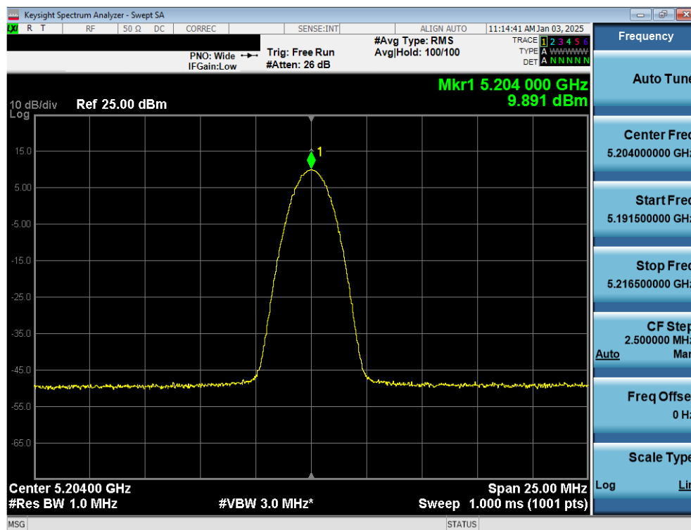
Plot 7-13. PSD Antenna WF8 (NB UNII BDR, ePA – 5204MHz)
