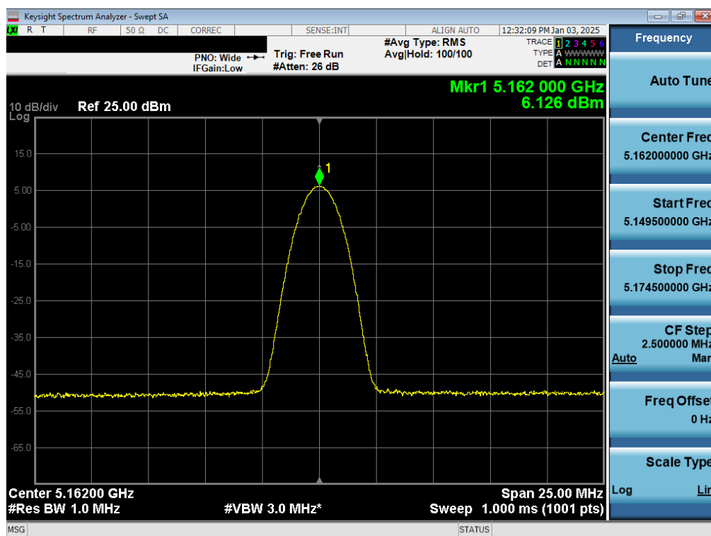
Plot 7-40. PSD TxBF Antenna WF7a (NB UNII BDR, iPA – 5162MHz)
