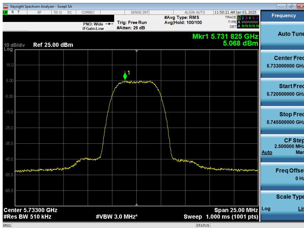
Plot 7-57. PSD TxBF Antenna WF8 (NB UNII HDR8, ePA – 5733MHz)
