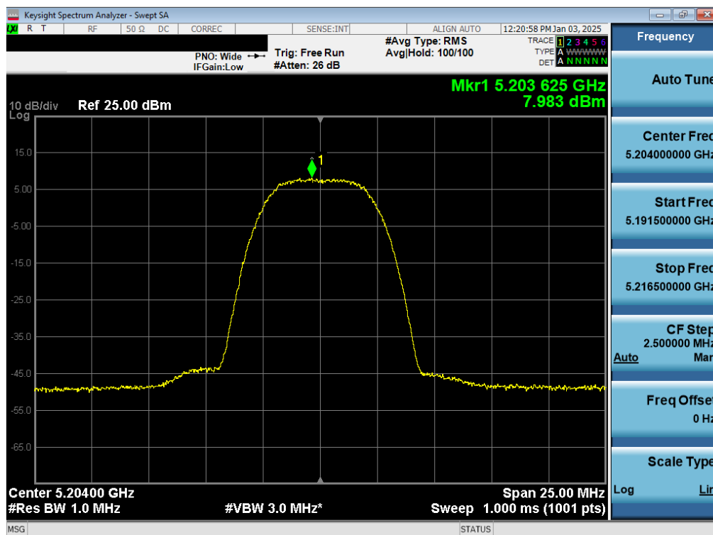
Plot 7-29. PSD Antenna WF7a (NB UNII HDR8, ePA – 5204MHz)
