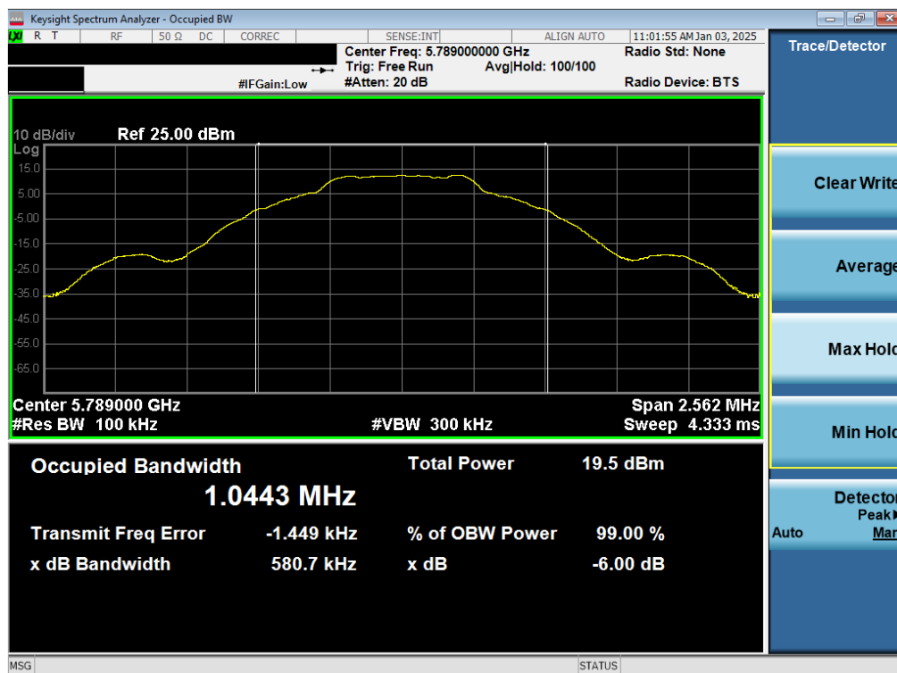
Plot 7-7. 6dB BW & 99% OBW Antenna WF8 (NB UNII BDR, 5789MHz)
