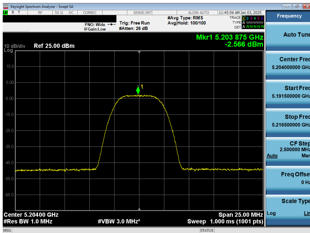
Plot 7-47. PSD TxBF Antenna WF8 (NB UNII HDR8, iPA – 5204MHz)
