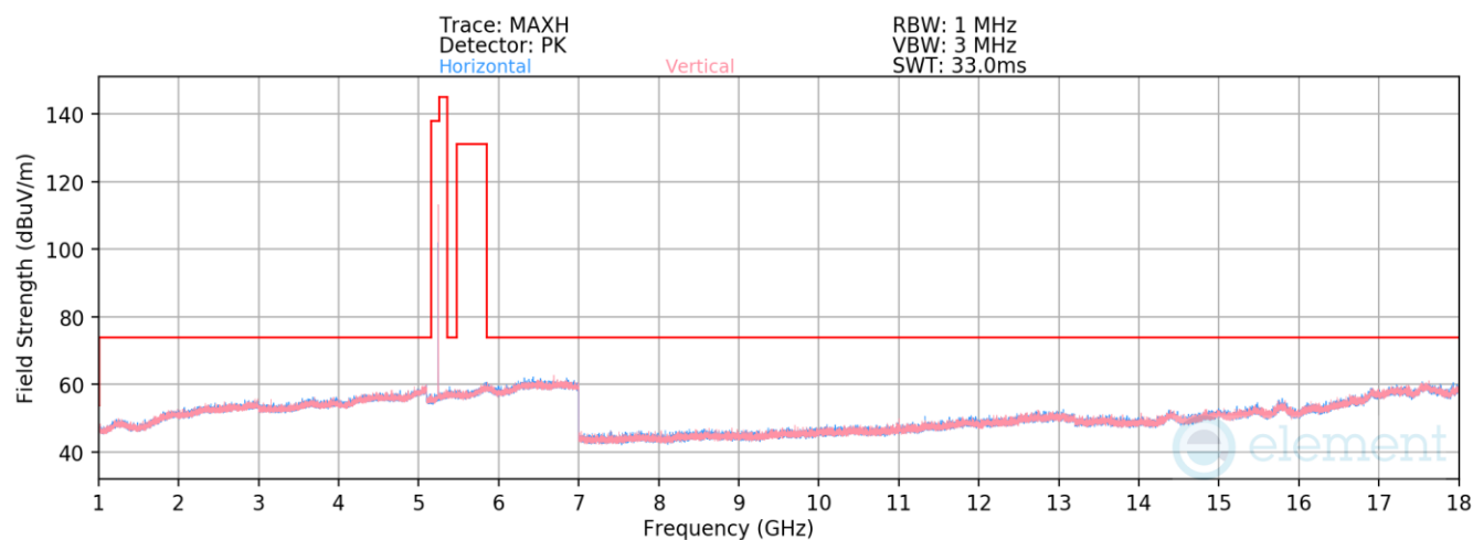
Plot 7-72. Radiated Spurious Emissions 1-18GHz TxBF (NB UNII HDR4, ePA – 5245MHz)
