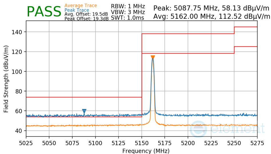
Plot 7-77. Radiated Lower Band Edge Measurement Antenna WF8
