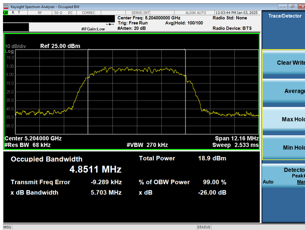
Plot 7-6. 26dB BW & 99% OBW Antenna WF7a (NB UNII HDR8, ePA– 5204MHz)
