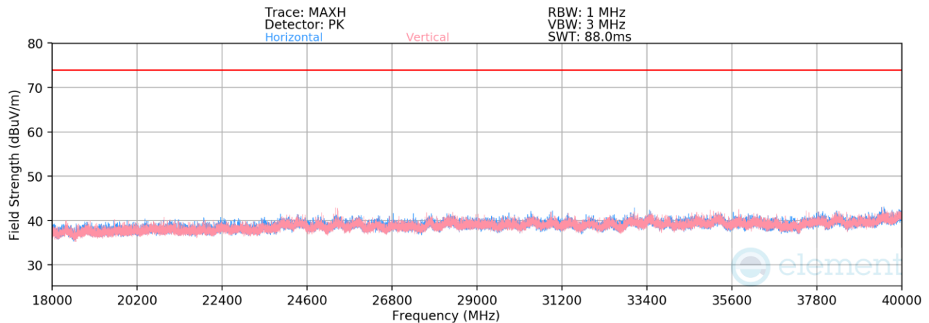
Plot 7-63. Radiated Spurious Emissions Above 18GHz (NB UNII BDR, ePA – 5204MHz)
