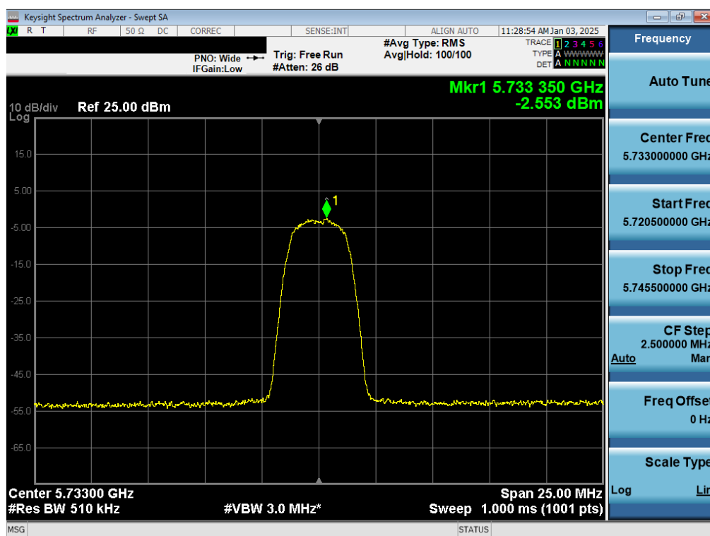
Plot 7-22. PSD Antenna WF8 (NB UNII HDR4, iPA – 5733MHz)
