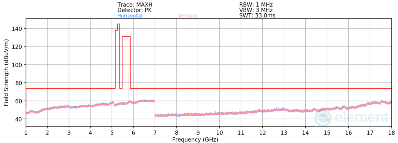
Plot 7-74. Radiated Spurious Emissions 1-18GHz TxBF (NB UNII HDR4, ePA – 5789MHz)
