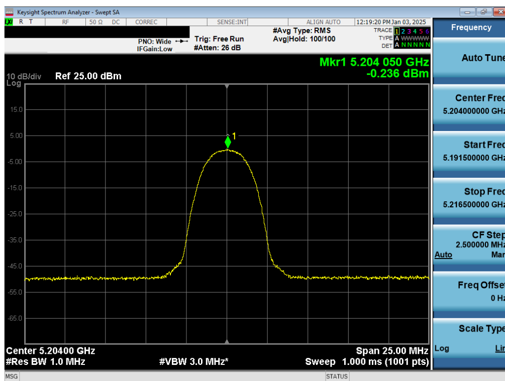
Plot 7-28. PSD Antenna WF7a (NB UNII HDR4, iPA – 5204MHz)
