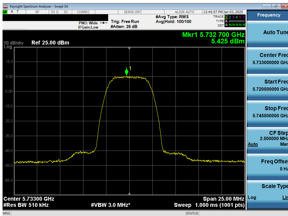
Plot 7-58. PSD TxBF Antenna WF7a (NB UNII HDR8, ePA – 5733MHz)
