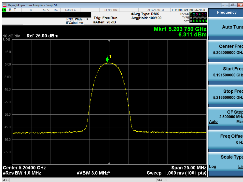
Plot 7-41. PSD TxBF Antenna WF8 (NB UNII HDR4, ePA – 5204MHz)
