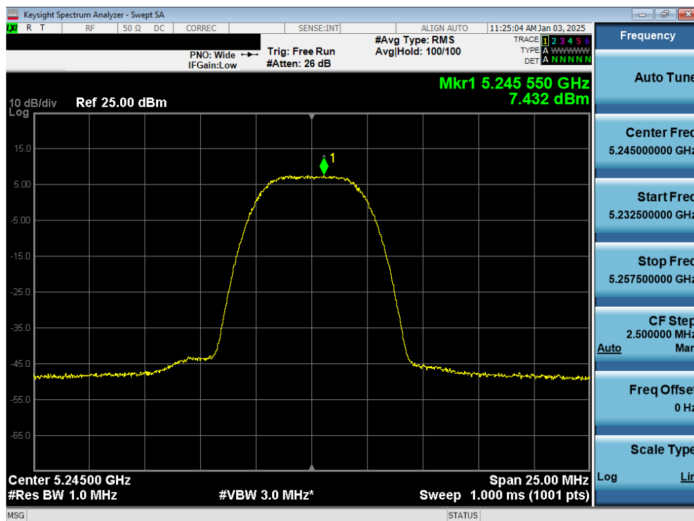
Plot 7-17. PSD Antenna WF8 (NB UNII HDR8, ePA – 5245MHz)
