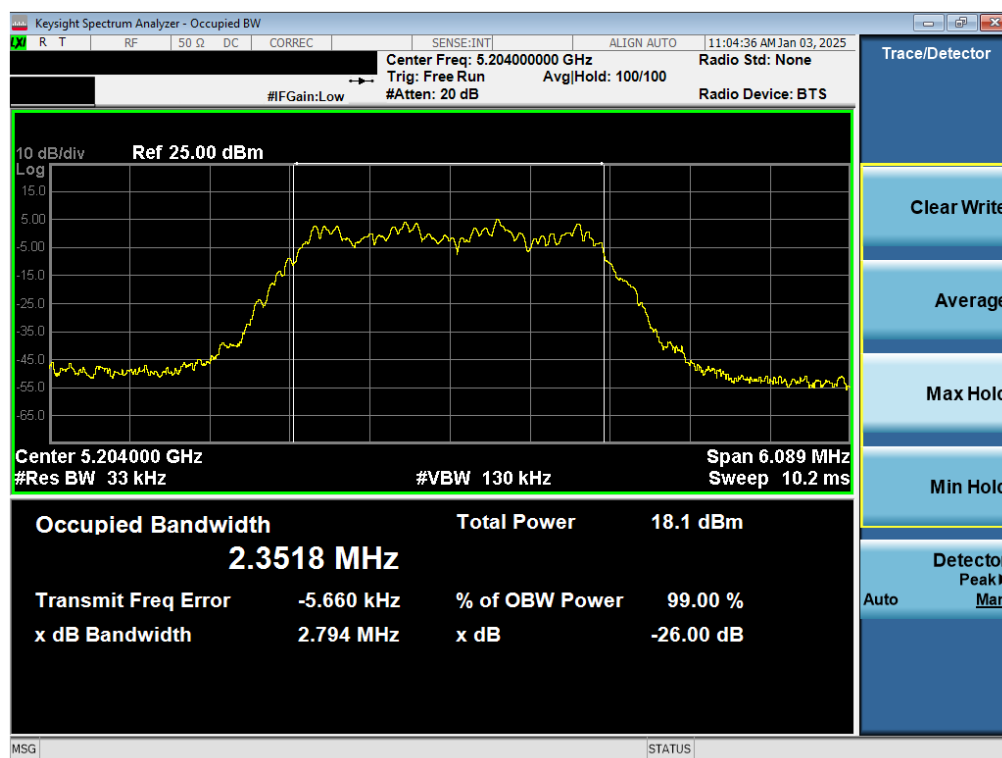
Plot 7-2. 26dB BW & 99% OBW Antenna WF8 (NB UNII HDR4, ePA- 5204MHz)
