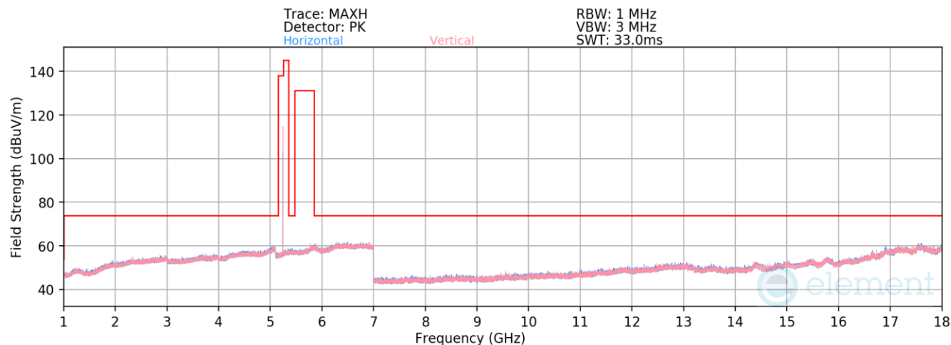
Plot 7-64. Radiated Spurious Emissions 1-18GHz TxBF (NB UNII BDR, ePA – 5245MHz)
