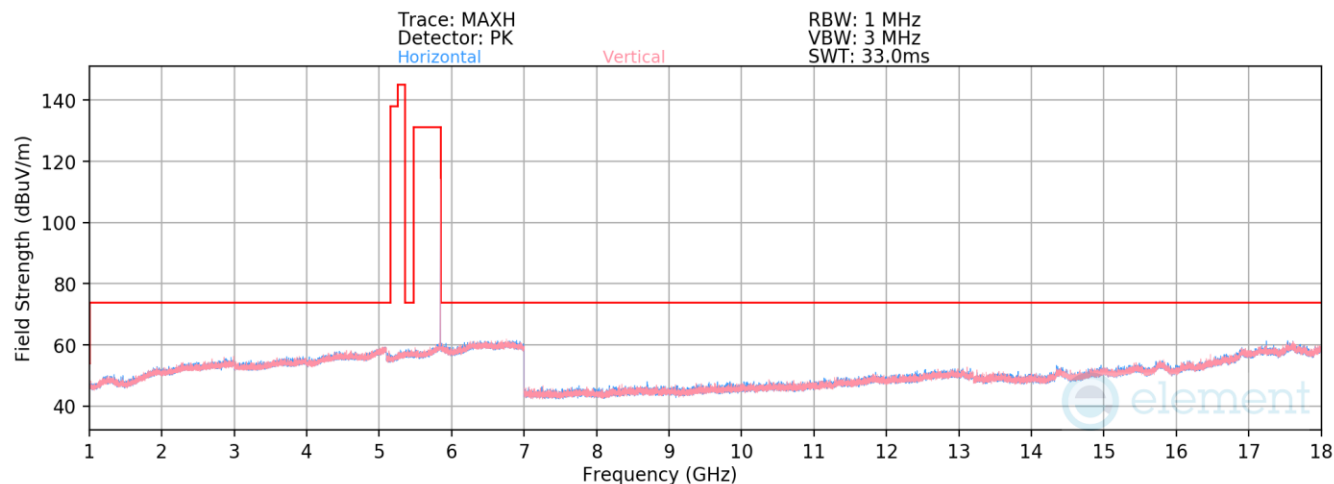
Plot 7-76. Radiated Spurious Emissions 1-18GHz TxBF (NB UNII HDR4, ePA – 5844MHz)
