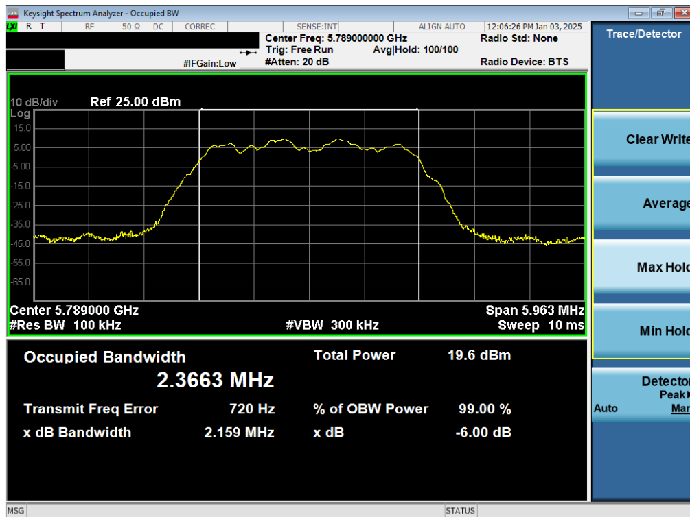
Plot 7-11. 6dB BW & 99% OBW Antenna WF7a (NB UNII HDR4, 5789MHz)
