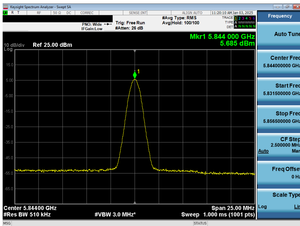
Plot 7-20. PSD Antenna WF8 (NB UNII BDR, iPA – 5844MHz)
