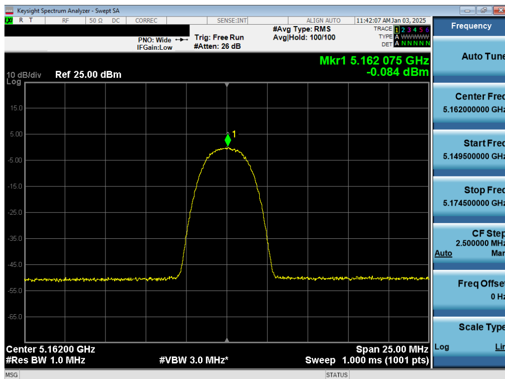
Plot 7-43. PSD TxBF Antenna WF8 (NB UNII HDR4, iPA – 5162MHz)
