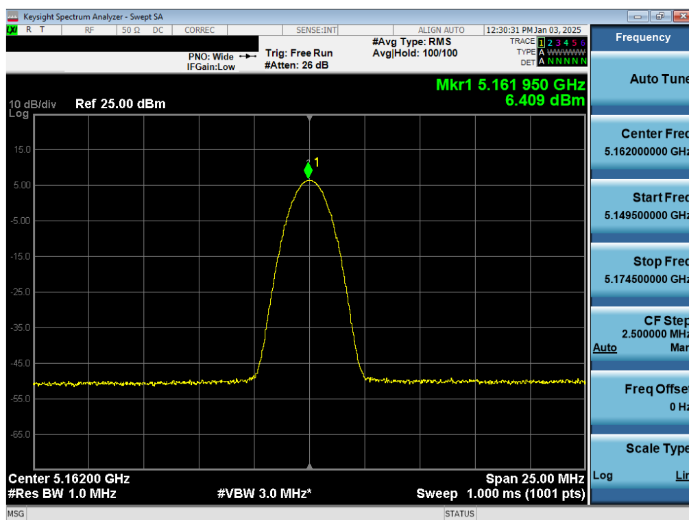
Plot 7-38. PSD TxBF Antenna WF7a (NB UNII BDR, ePA – 5162MHz)
