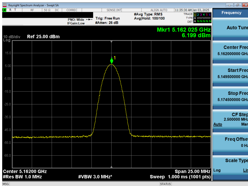
Plot 7-39. PSD TxBF Antenna WF8 (NB UNII BDR, iPA – 5162MHz)
