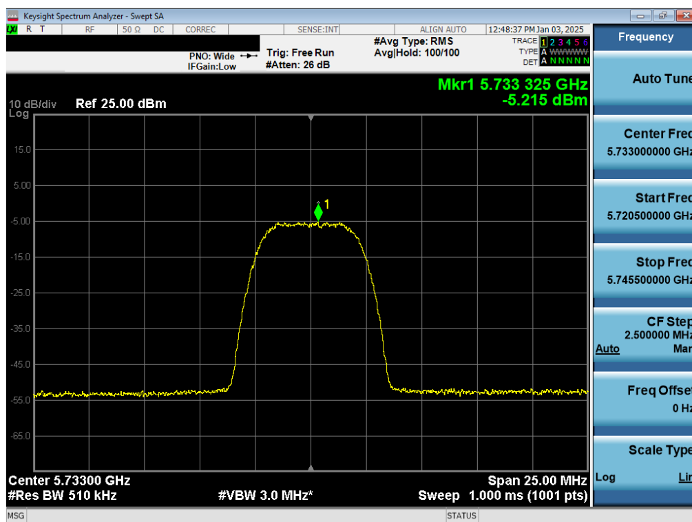
Plot 7-60. PSD TxBF Antenna WF7a (NB UNII HDR8, iPA – 5733MHz)
