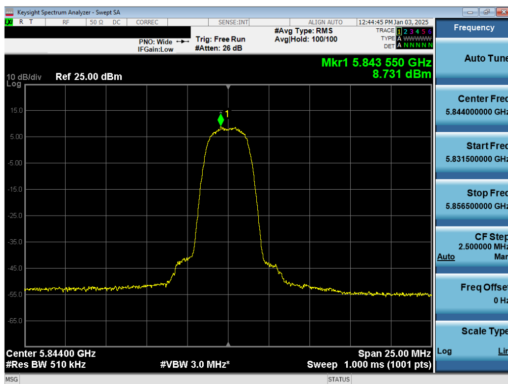
Plot 7-54. PSD TxBF Antenna WF7a (NB UNII HDR4, ePA – 5844MHz)
