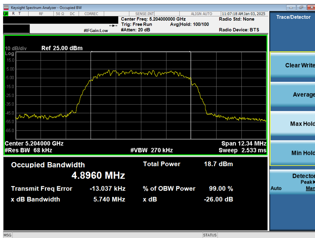
Plot 7-3. 26dB BW & 99% OBW Antenna WF8 (NB UNII HDR8, ePA- 5204MHz)
