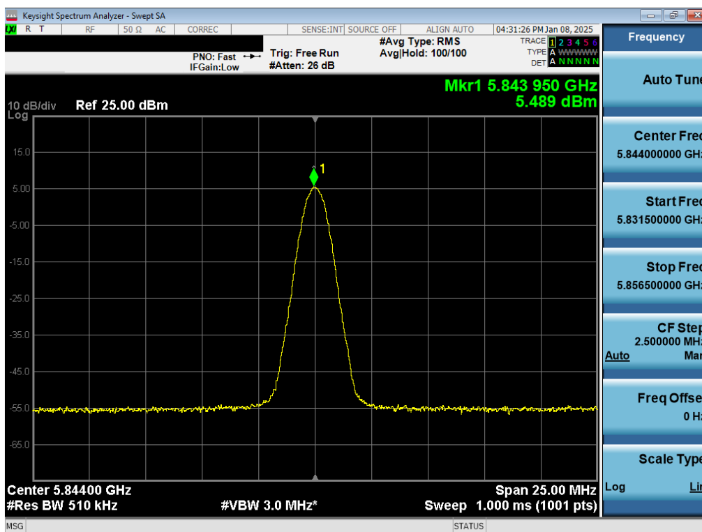
Plot 7-51. PSD TxBF Antenna WF8 (NB UNII BDR, iPA – 5844MHz)
