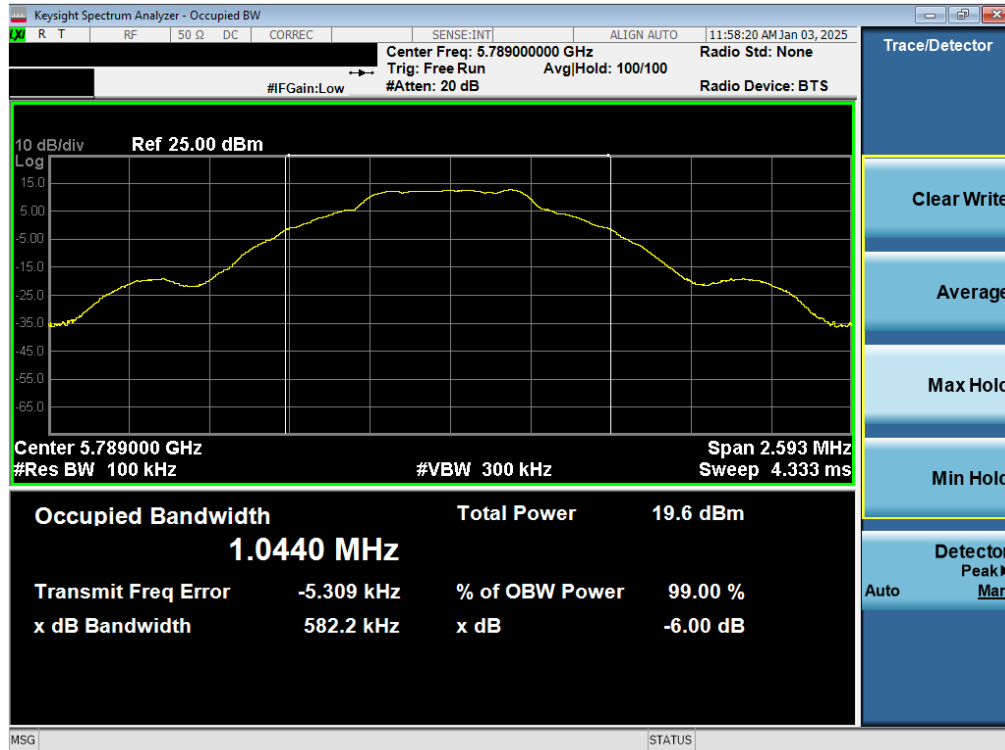
Plot 7-10. 6dB BW & 99% OBW Antenna WF7a (NB UNII BDR, 5789MHz)
