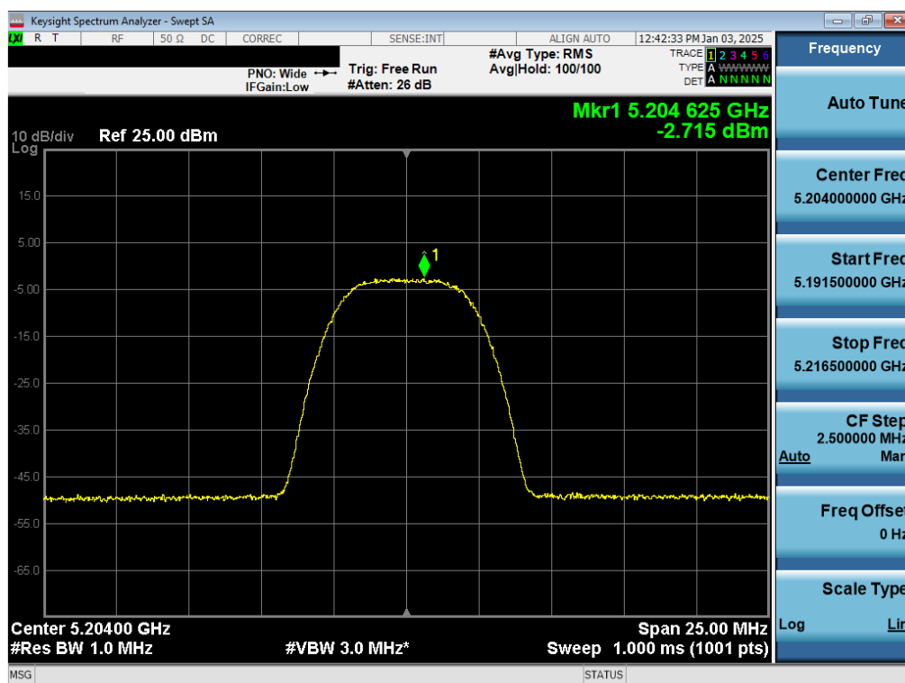
Plot 7-48. PSD TxBF Antenna WF7a (NB UNII HDR8, iPA – 5204MHz)
