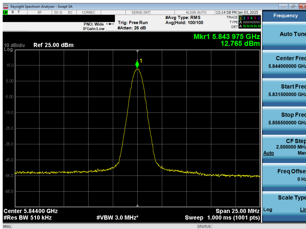
Plot 7-31. PSD Antenna WF7a (NB UNII BDR, ePA – 5844MHz)
