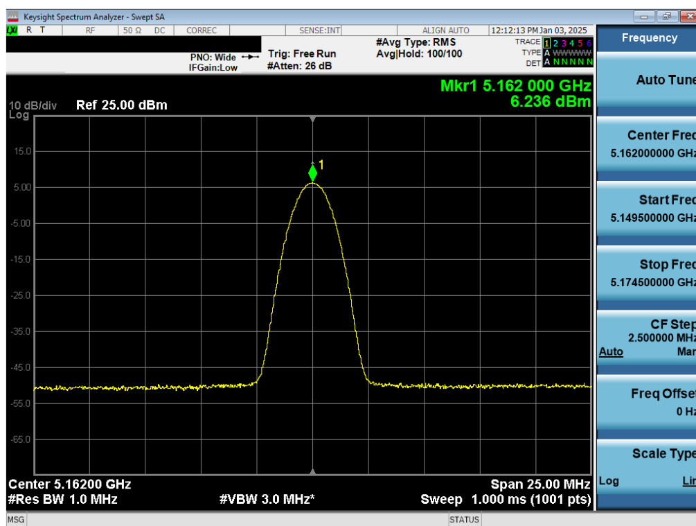
Plot 7-26. PSD Antenna WF7a (NB UNII BDR, iPA – 5162MHz)
