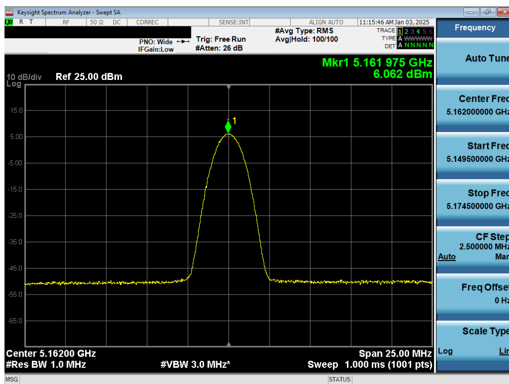
Plot 7-14. PSD Antenna WF8 (NB UNII BDR, iPA – 5162MHz)
