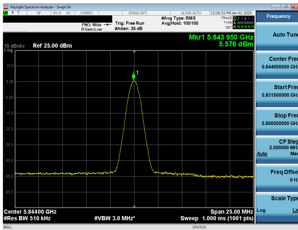
Plot 7-52. PSD TxBF Antenna WF7a (NB UNII BDR, iPA – 5844MHz)
