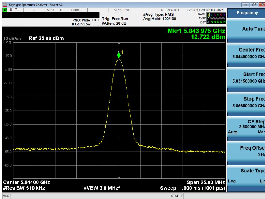
Plot 7-50. PSD TxBF Antenna WF7a (NB UNII BDR, ePA – 5844MHz)
