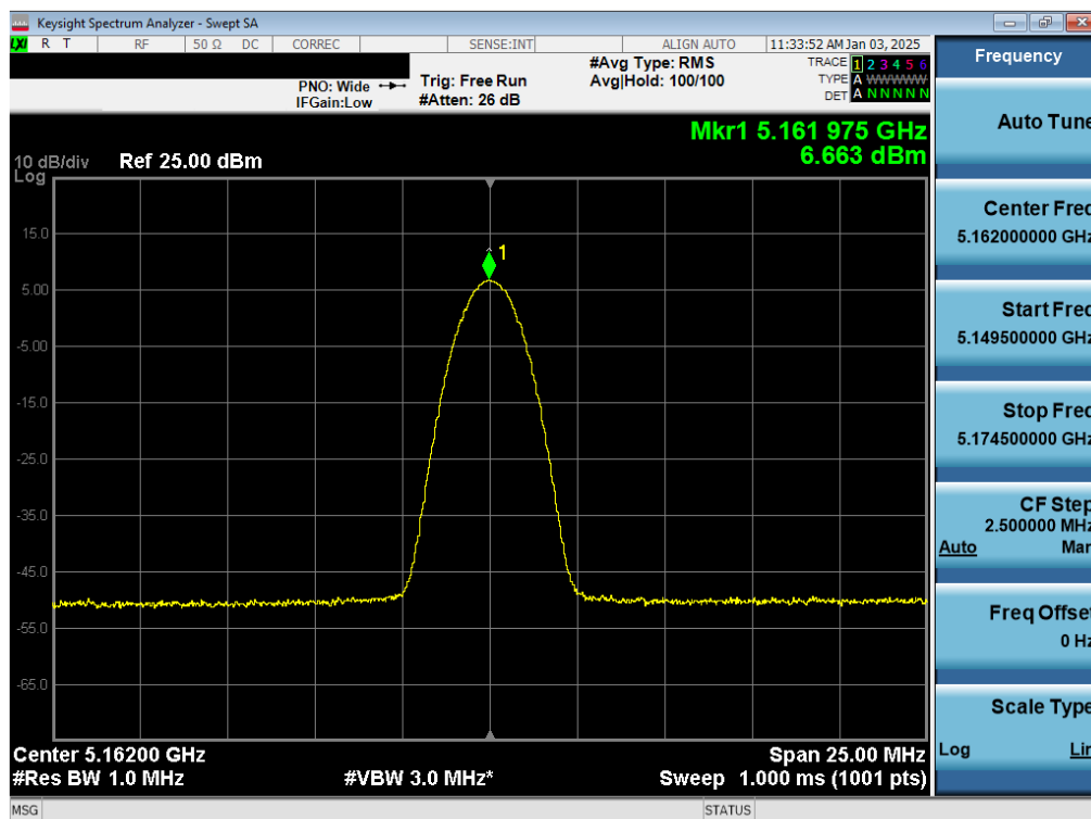
Plot 7-37. PSD TxBF Antenna WF8 (NB UNII BDR, ePA – 5162MHz)
