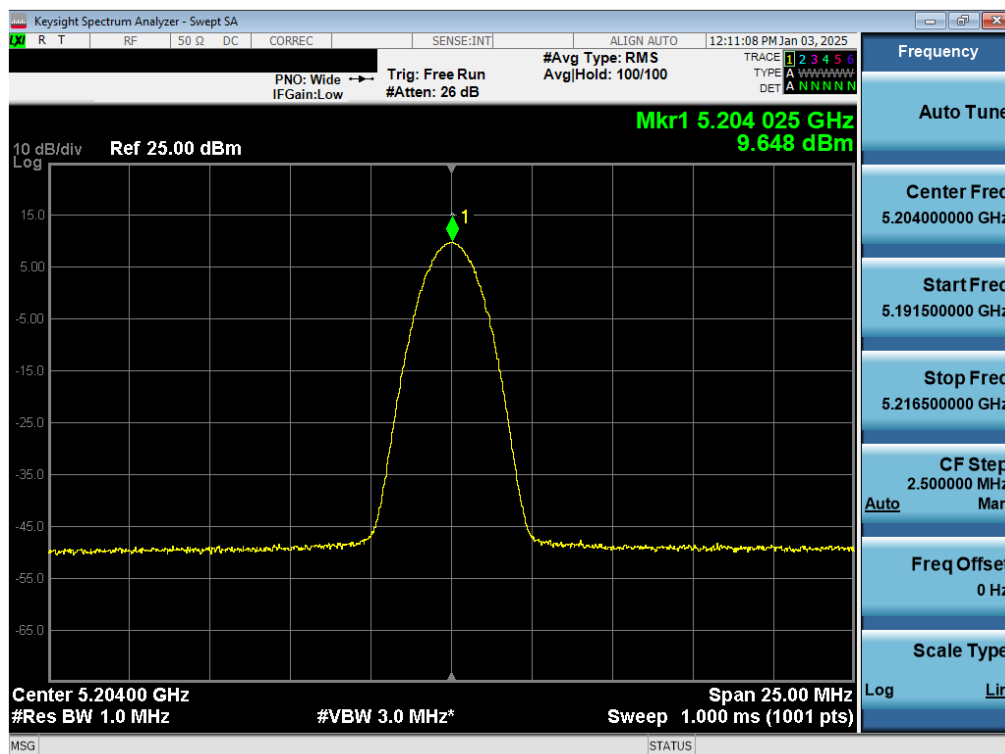
Plot 7-25. PSD Antenna WF7a (NB UNII BDR, ePA – 5204MHz)
