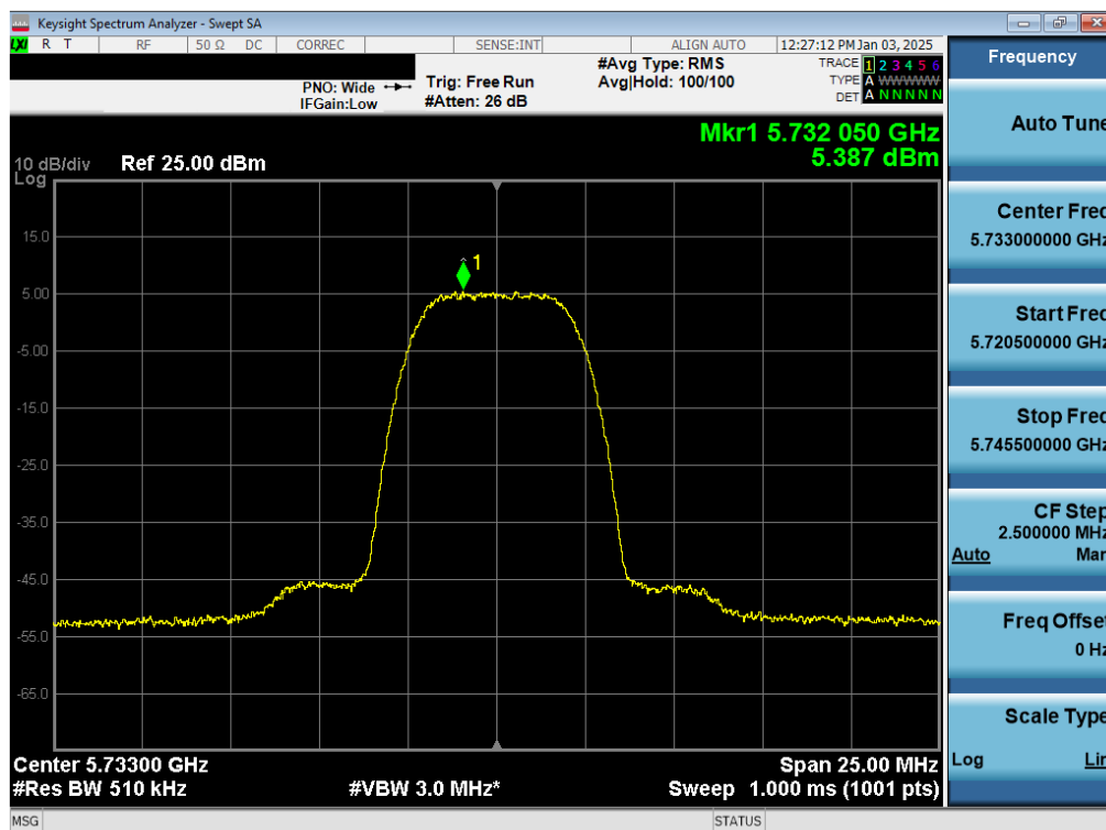
Plot 7-35. PSD Antenna WF7a (NB UNII HDR8, ePA – 5733MHz)
