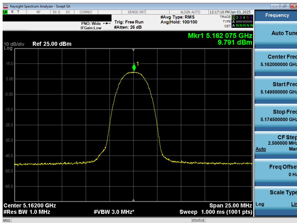
Plot 7-27. PSD Antenna WF7a (NB UNII HDR4, ePA – 5162MHz)
