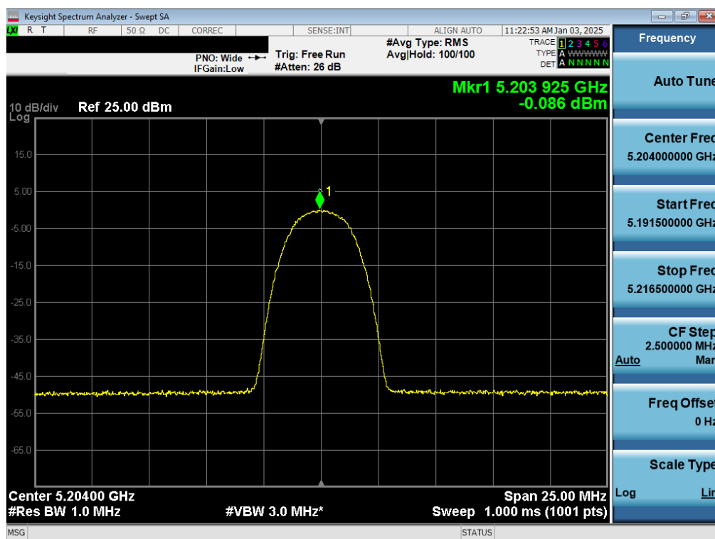
Plot 7-16. PSD Antenna WF8 (NB UNII HDR4, iPA – 5204MHz)
