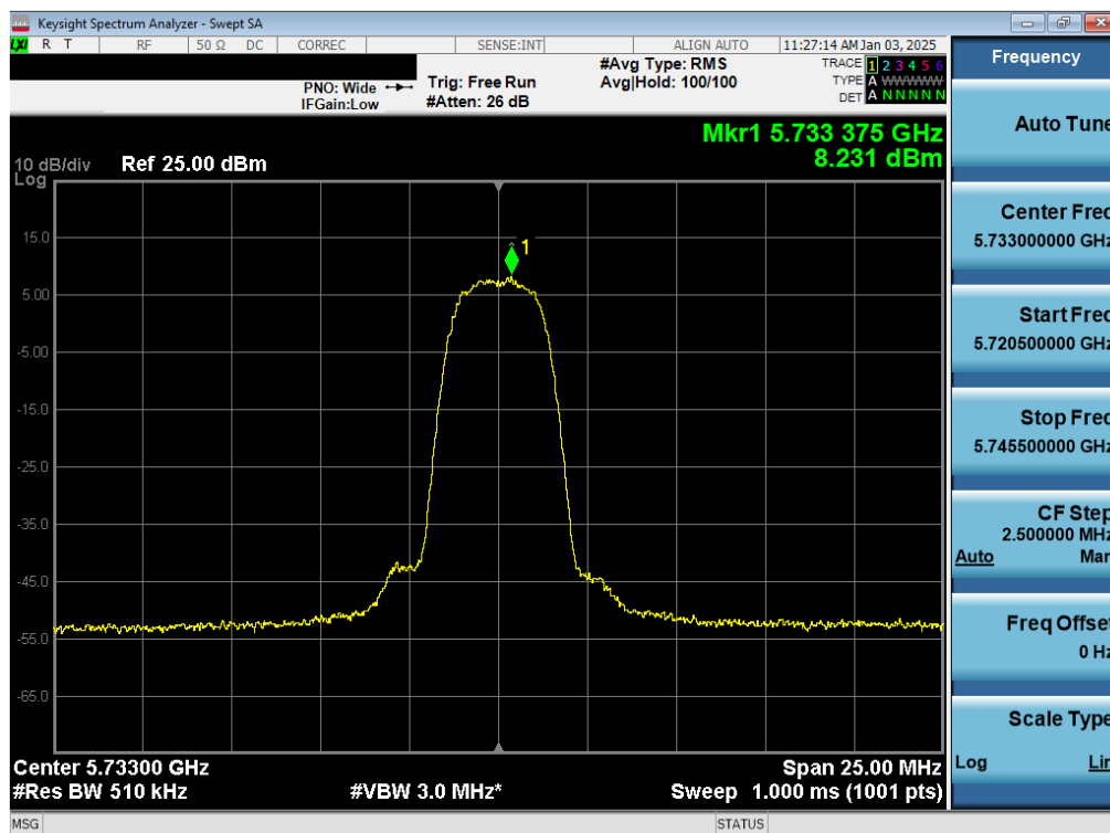
Plot 7-21. PSD Antenna WF8 (NB UNII HDR4, ePA – 5733MHz)
