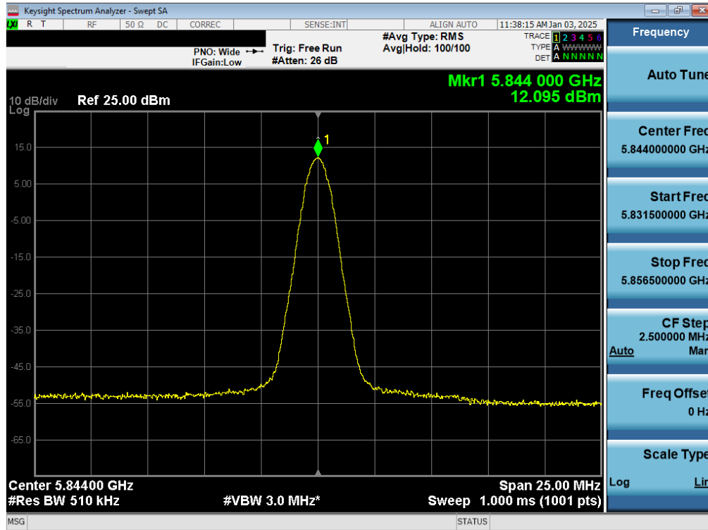
Plot 7-49. PSD TxBF Antenna WF8 (NB UNII BDR, ePA – 5844MHz)
