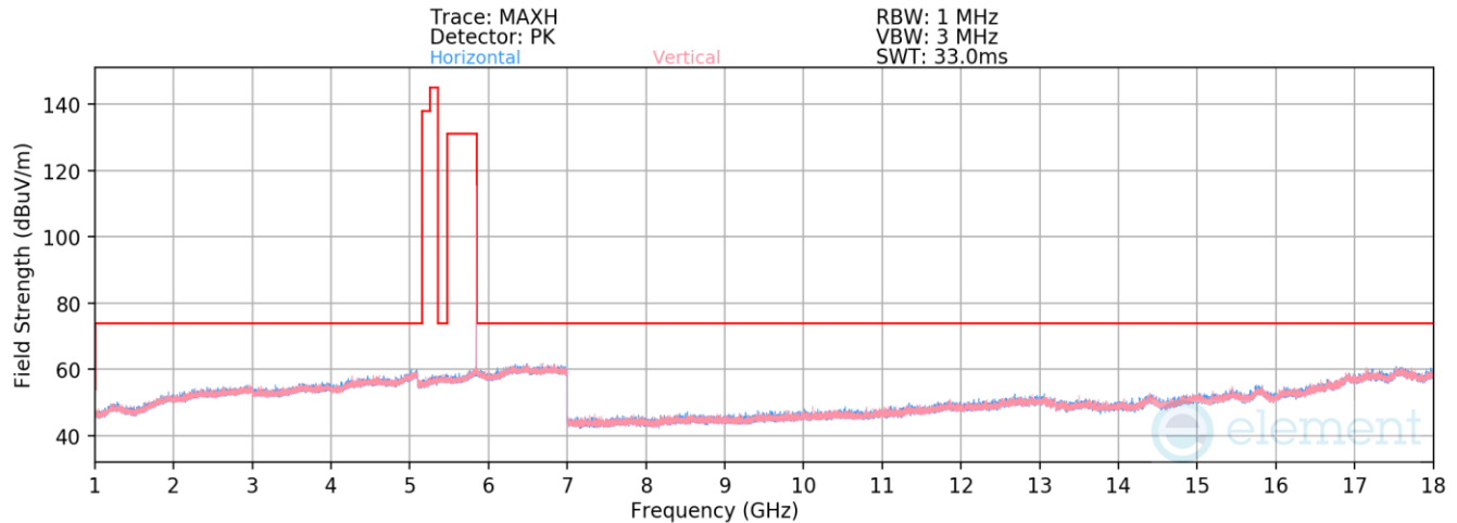
Plot 7-68. Radiated Spurious Emissions 1-18GHz TxBF (NB UNII BDR, ePA – 5844MHz)
