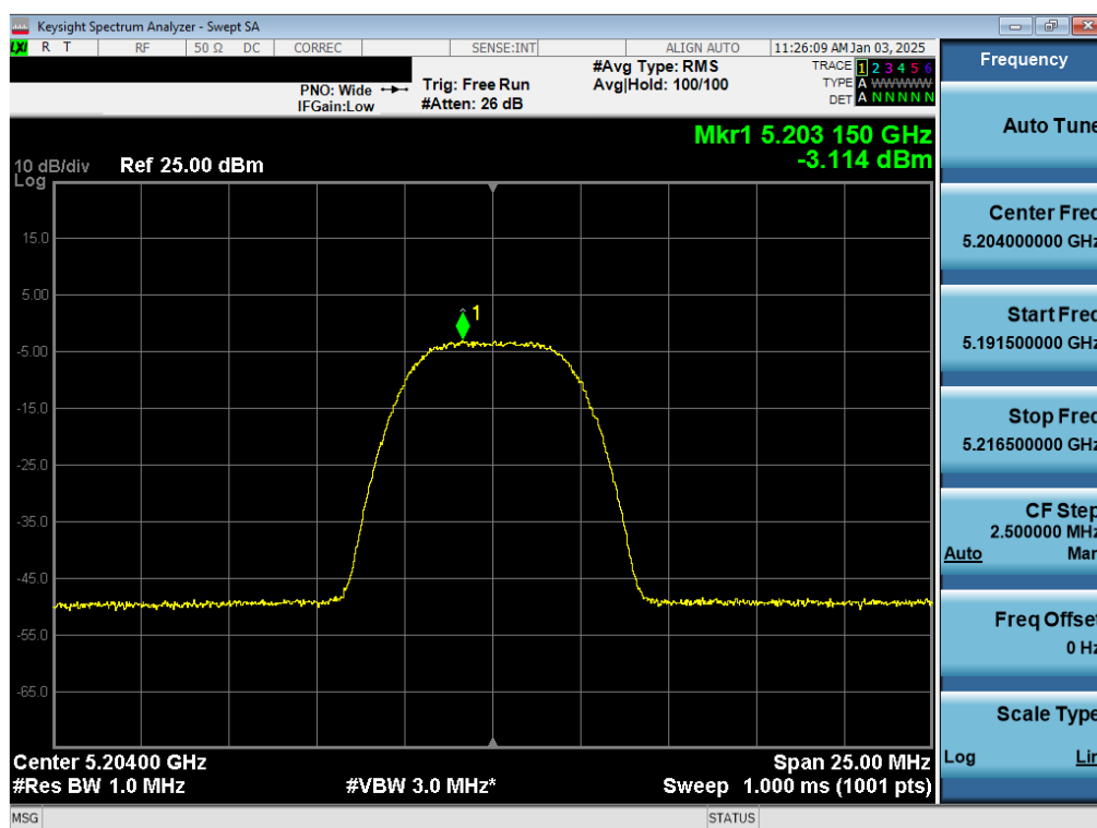
Plot 7-18. PSD Antenna WF8 (NB UNII HDR8, iPA – 5204MHz)
