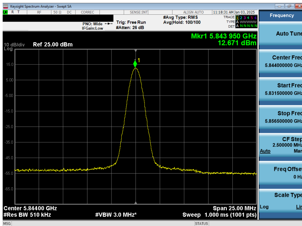
Plot 7-19. PSD Antenna WF8 (NB UNII BDR, ePA – 5844MHz)
