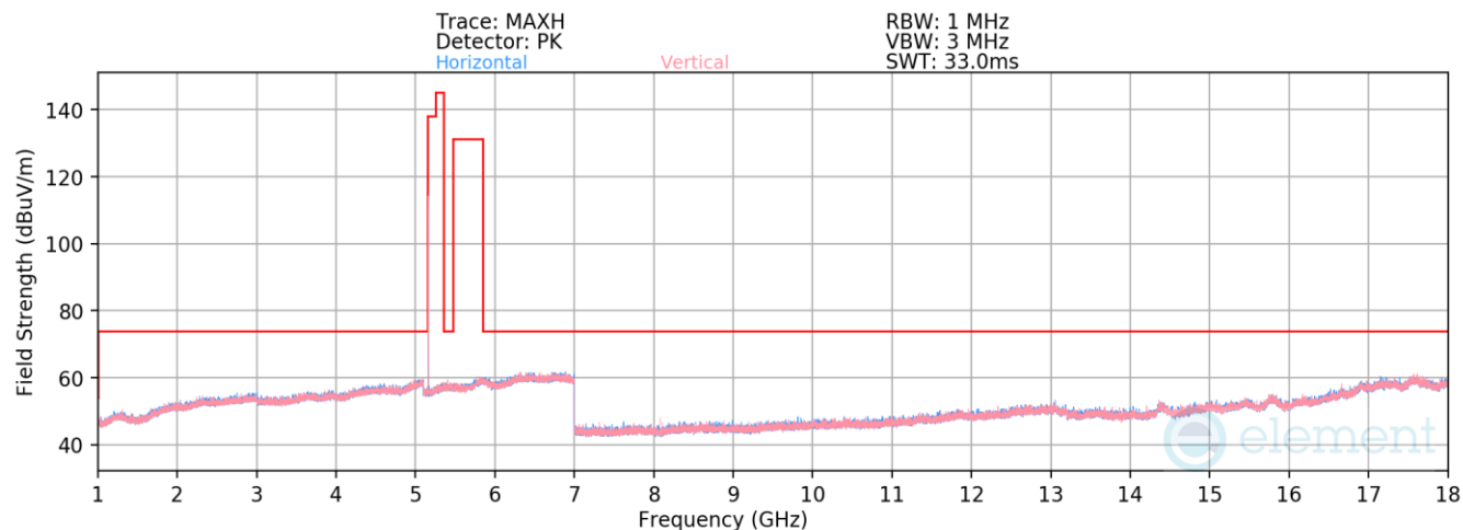
Plot 7-69. Radiated Spurious Emissions 1-18GHz TxBF (NB UNII HDR4, ePA - 5162MHz)
