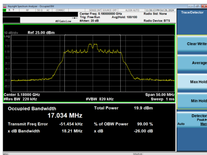
Plot 7-1. 26dB BW & 99% OBW Antenna WF8 (20MHz BW 11ax Index 4 – RU26 – Ch.36)
