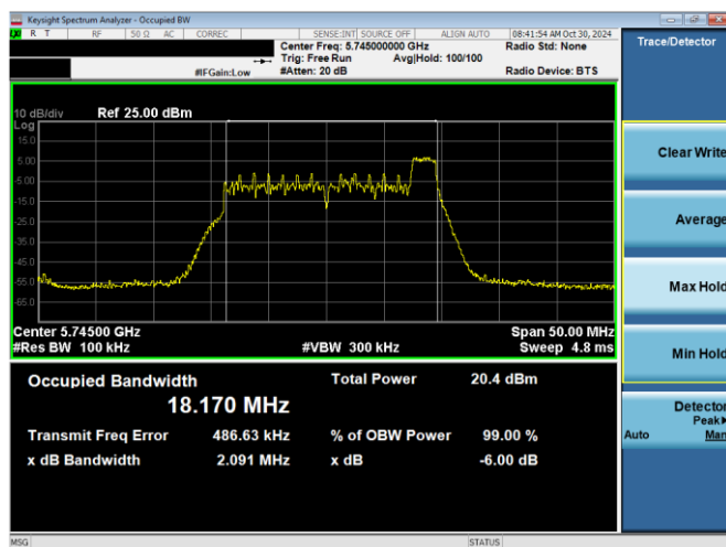
Plot 7-7. 6dB BW & 99% OBW Antenna WF7a (20MHz BW 11ax Index 8 – RU26 – Ch.149)
