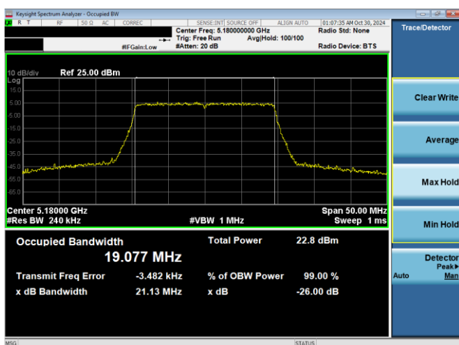
Plot 7-2. 26dB BW & 99% OBW Antenna WF8 (20MHz BW 11ax– RU242 – Ch.36)
