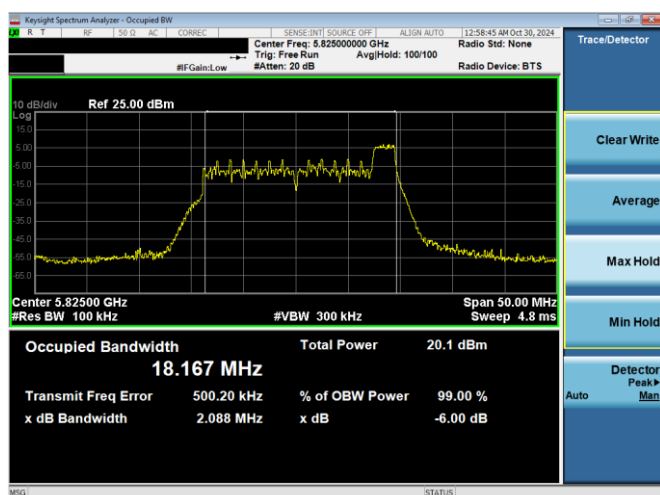
Plot 7-5. 6dB BW & 99% OBW Antenna WF8 (20MHz BW 11ax Index 8 – RU26 – Ch.165)
