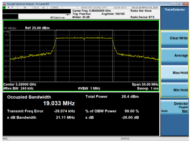
Plot 7-4. 26dB BW & 99% OBW Antenna WF7a (20MHz BW 11ax– RU242 – Ch.116)
