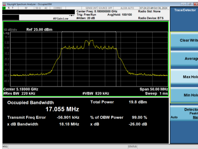
Plot 7-3. 26dB BW & 99% OBW Antenna WF7a (20MHz BW 11ax Index 4 – RU26 – Ch.36)
