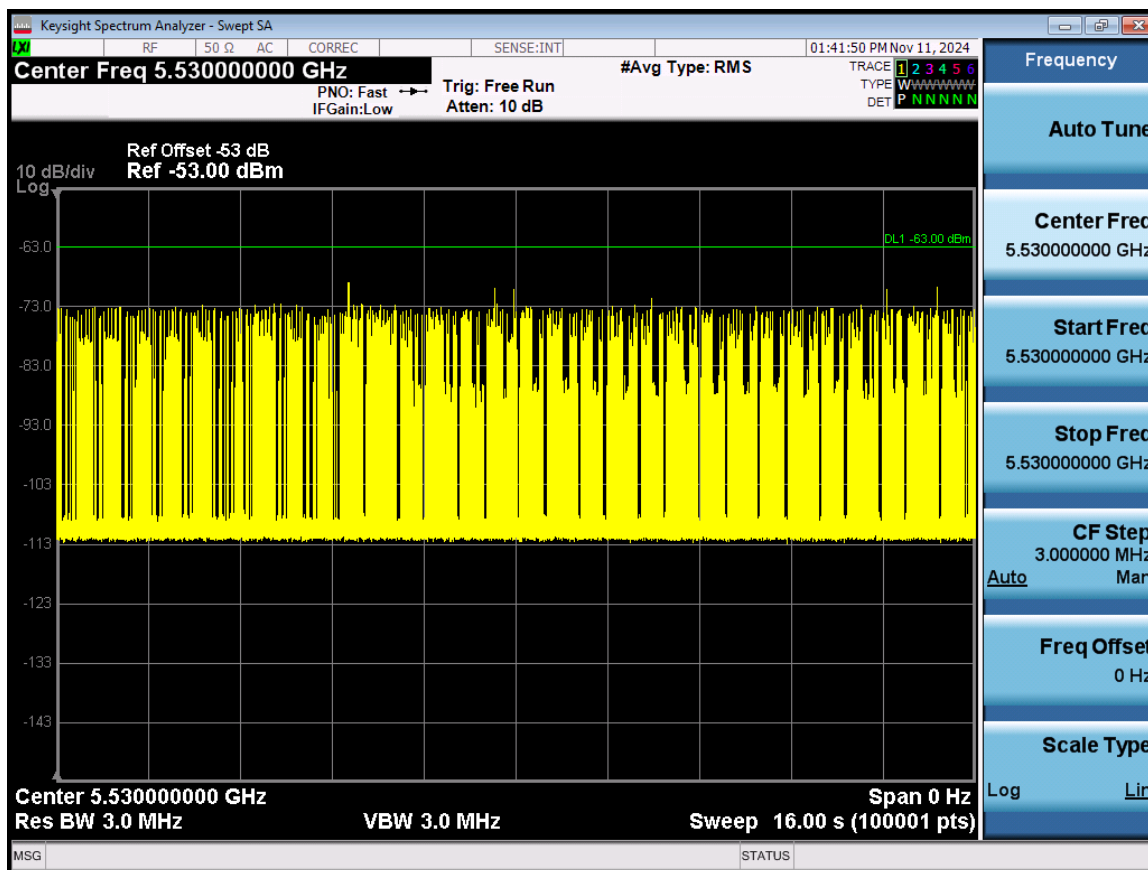
Figure 9-9. 5530 MHz - Channel Loading - Mode 4 (80MHz)
