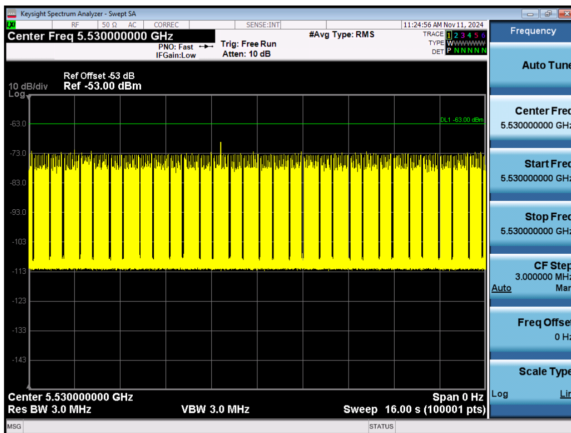
Figure 9-7. 5530MHz - Channel Loading - Mode 3 (80MHz)
