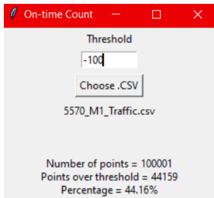
Figure 9-4. 5570MHz - Channel Loading Calculation - Mode 1 (160MHz)
