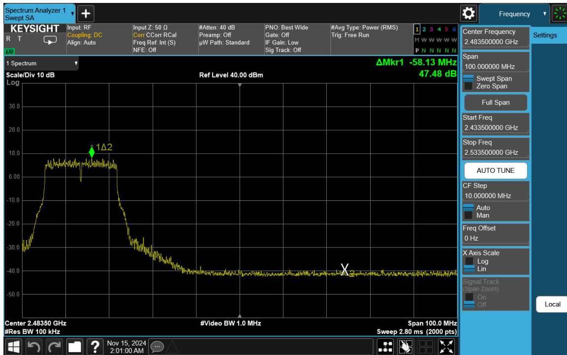
Plot 7-80. Band Edge Plot Antenna WF7b (802.11g – Ch. 8)
