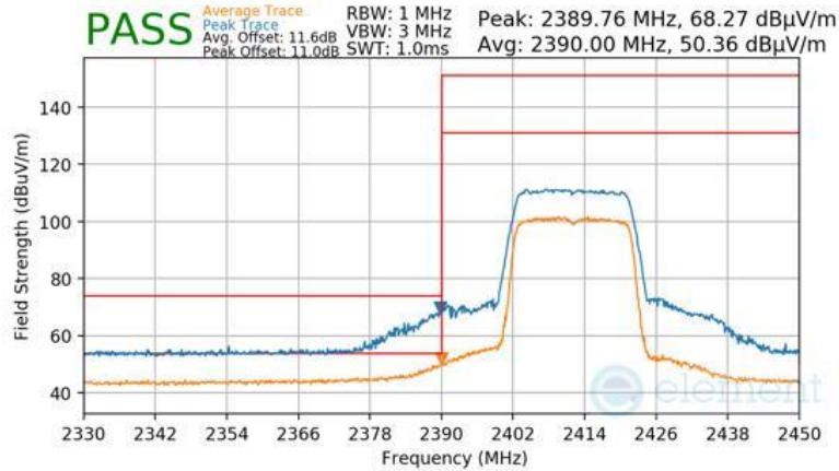
Plot 7-157 Radiated Restricted Lower Band Edge Measurement Antenna WF8
