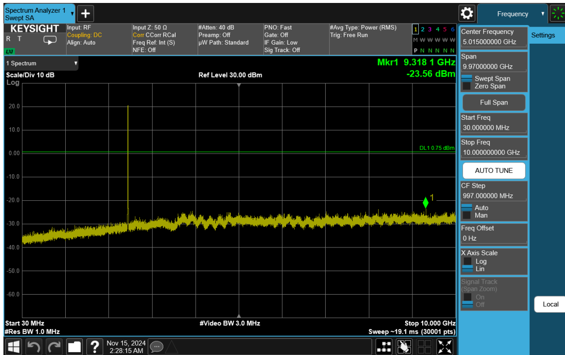
Plot 7-123. Conducted Spurious Plot Antenna WF7b (802.11b – Ch. 11)
