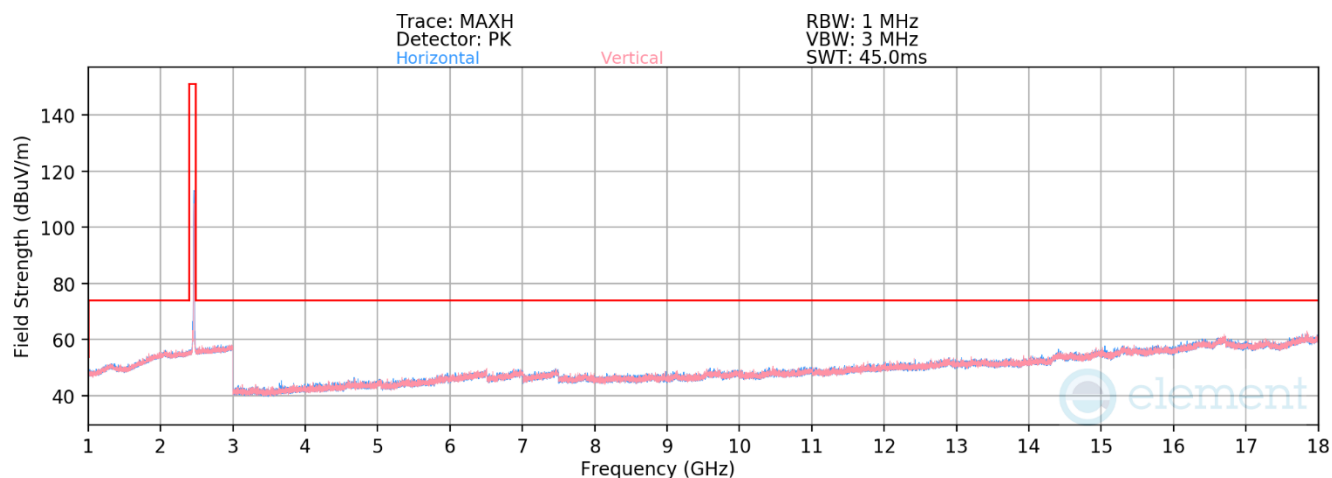
Plot 7-130. Radiated Spurious Emissions above 1GHz Antenna WF7b (802.11b – Ch. 11)
