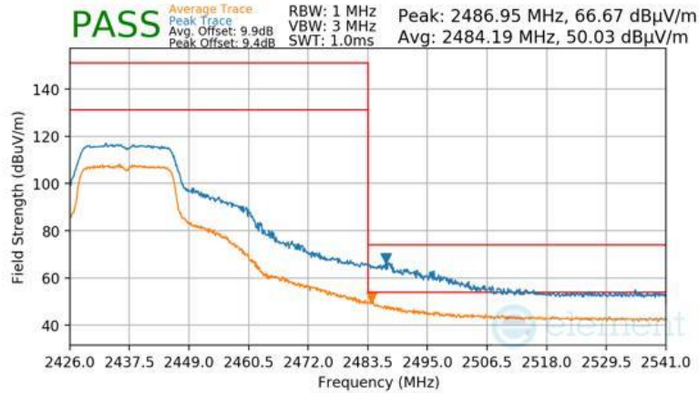
Plot 7-149 Radiated Restricted Upper Band Edge Measurement Antenna WF8
