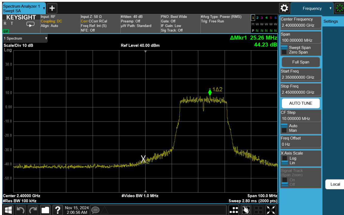
Plot 7-88. Band Edge Plot Antenna WF7b (802.11n (2.4GHz) – Ch. 3)
