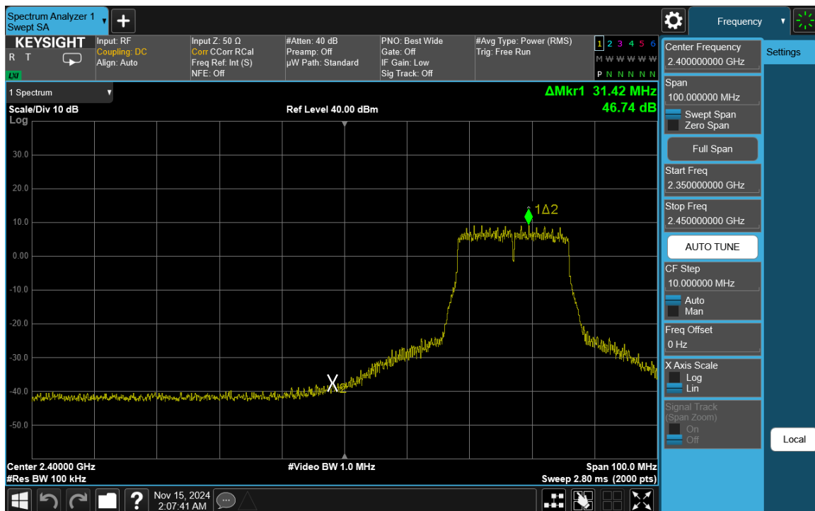
Plot 7-89. Band Edge Plot Antenna WF7b (802.11n (2.4GHz) – Ch. 4)
