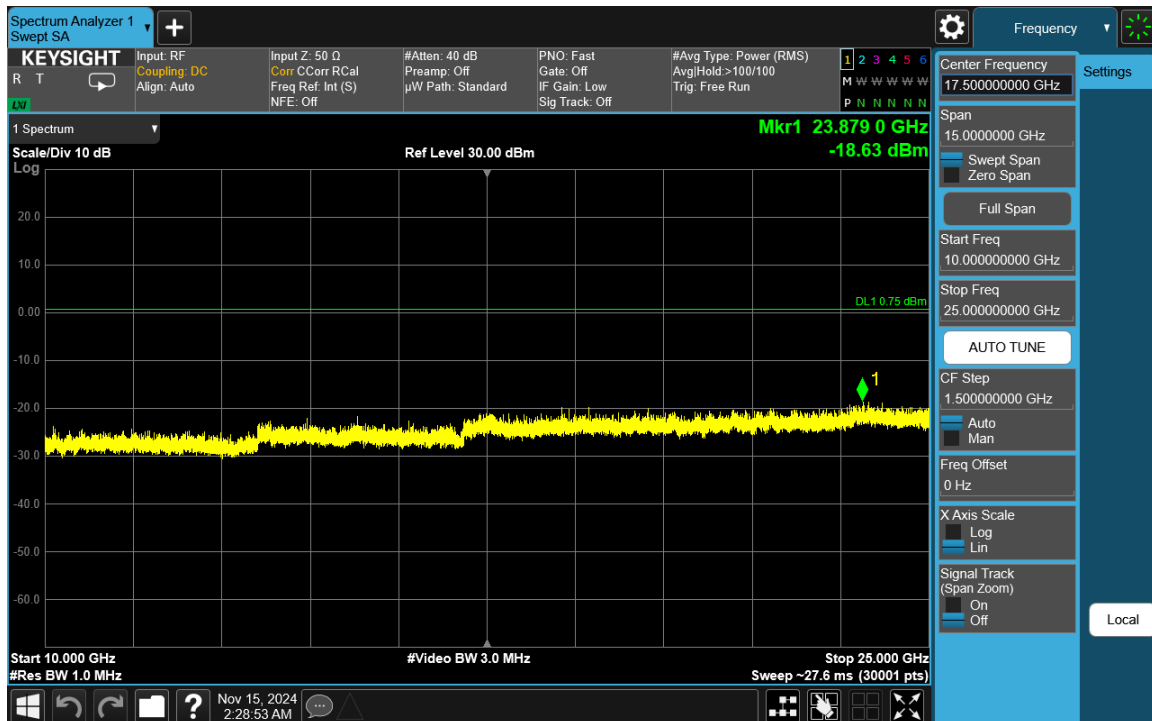
Plot 7-124. Conducted Spurious Plot Antenna WF7b (802.11b – Ch. 11)
