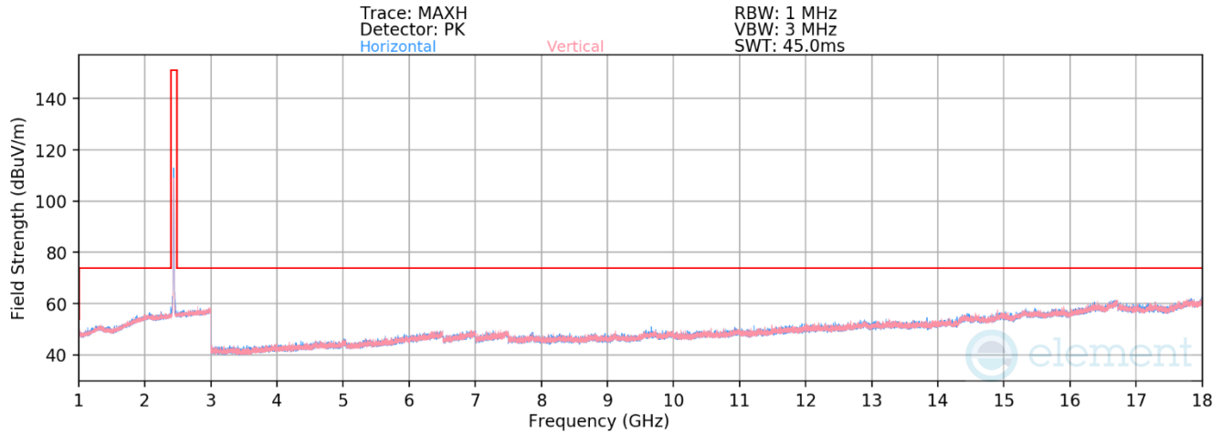
Plot 7-129. Radiated Spurious Emissions above 1GHz Antenna WF7b (802.11b – Ch. 6)
