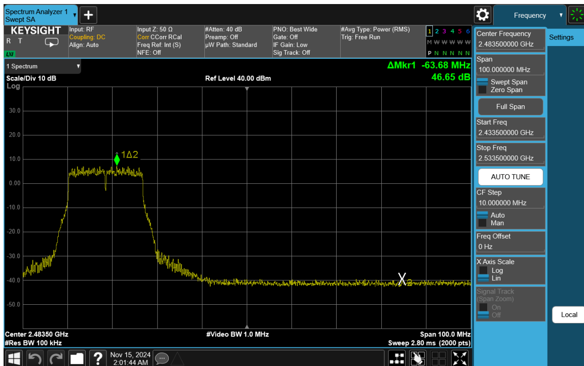
Plot 7-81. Band Edge Plot Antenna WF7b (802.11g – Ch. 9)
