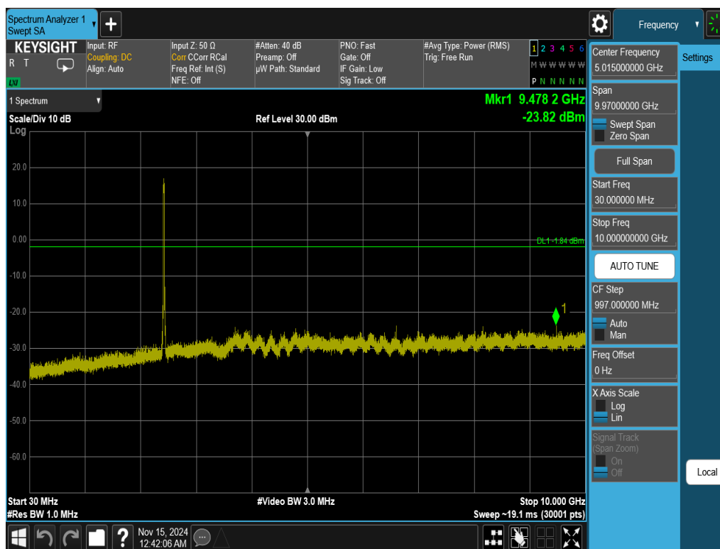
Plot 7-63. Conducted Spurious Plot Antenna WF7b (802.11ax OFDMA – RU242 – Ch. 6)
