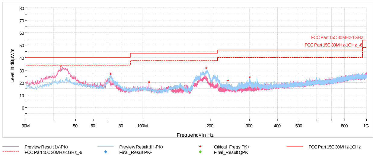
Plot 7-128. Radiated Spurious Emissions below 1GHz CDD Ch.6 (RU26), with AC/DC adaptor via USB-C cable with wire charger
