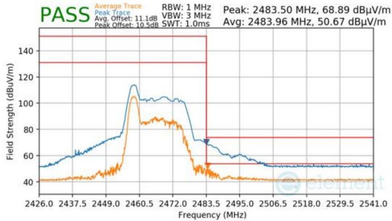
Plot 7-94 Radiated Restricted Upper Band Edge Measurement Antenna WF7b (Peak & Average – RU26)
