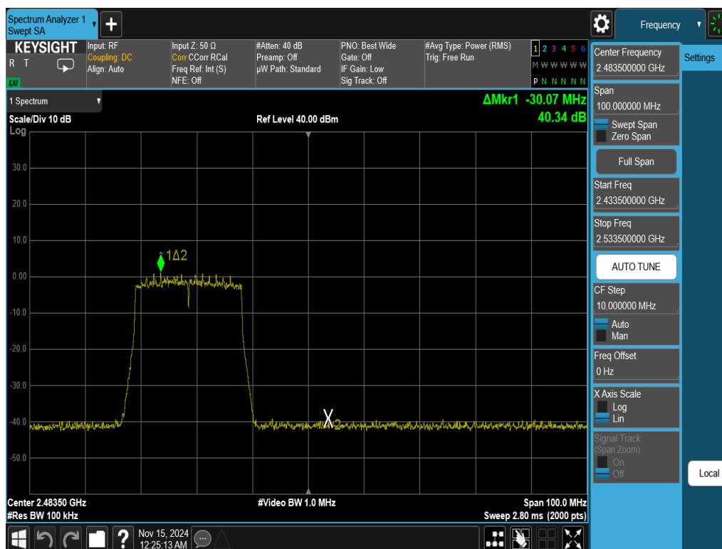
Plot 7-41. Band Edge Antenna WF7b (802.11ax OFDMA – RU242 – Ch. 11)
