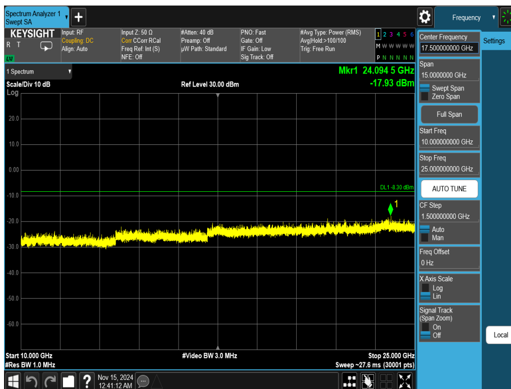
Plot 7-62. Conducted Spurious Plot Antenna WF7b (802.11ax OFDMA – RU242 – Ch. 1)
