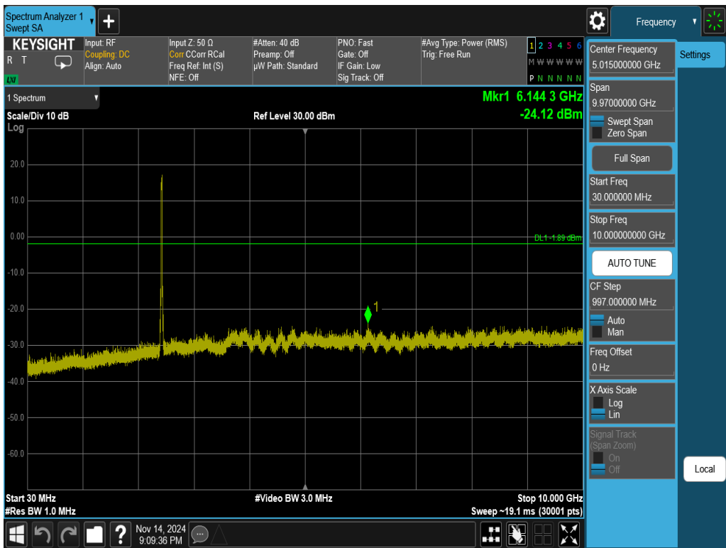
Plot 7-51. Conducted Spurious Plot Antenna WF8 (802.11ax OFDMA – RU242 – Ch. 6)
