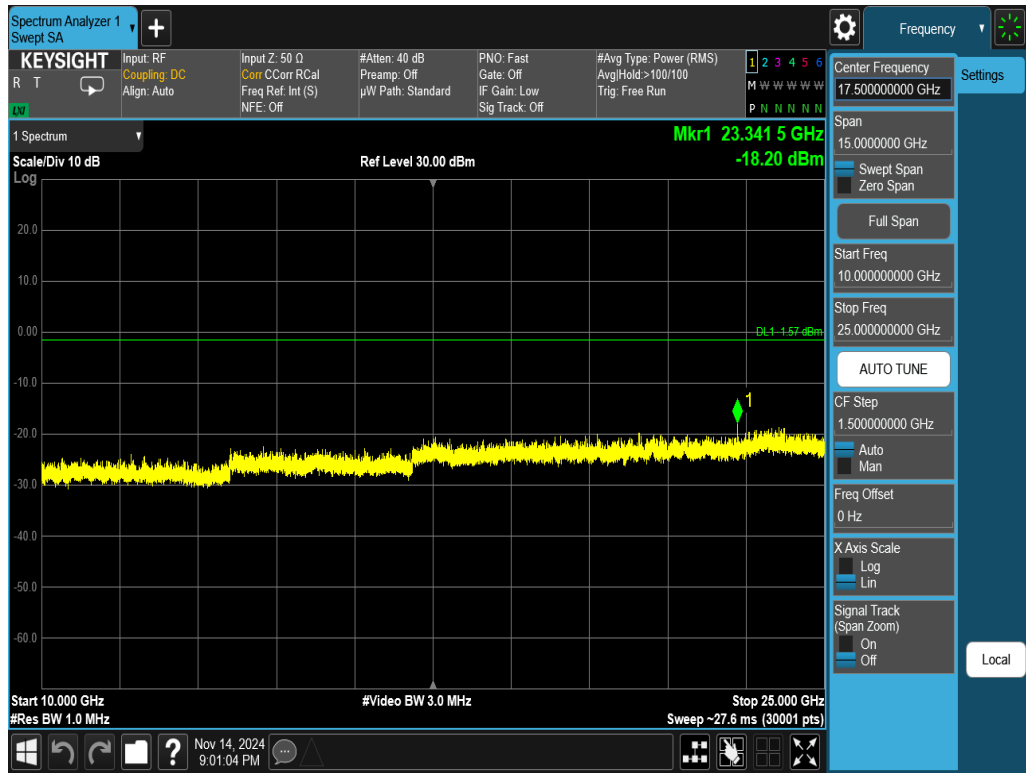
Plot 7-46. Conducted Spurious Plot Antenna WF8 (802.11ax OFDMA – RU26 – Ch. 6)
