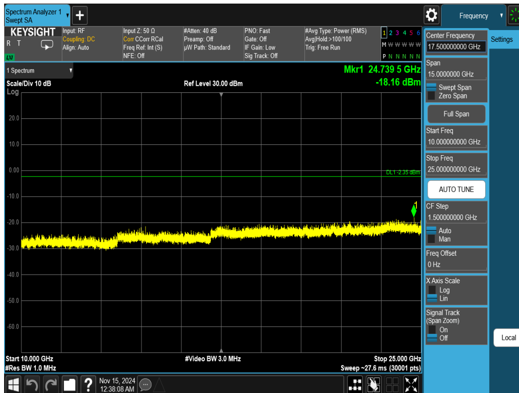
Plot 7-60. Conducted Spurious Plot Antenna WF7b (802.11ax OFDMA – RU26 – Ch. 11)
