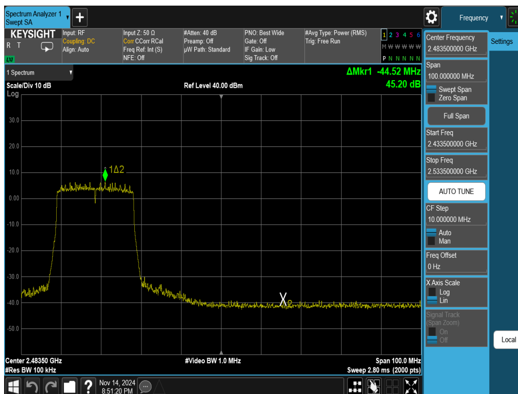
Plot 7-24. Band Edge Antenna WF8 (802.11ax OFDMA – RU242 – Ch. 9)
