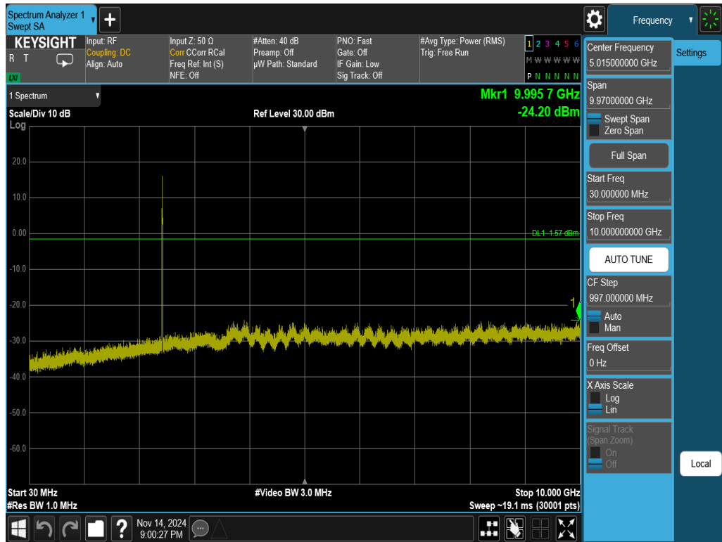
Plot 7-45. Conducted Spurious Plot Antenna WF8 (802.11ax OFDMA – RU26 – Ch. 6)
