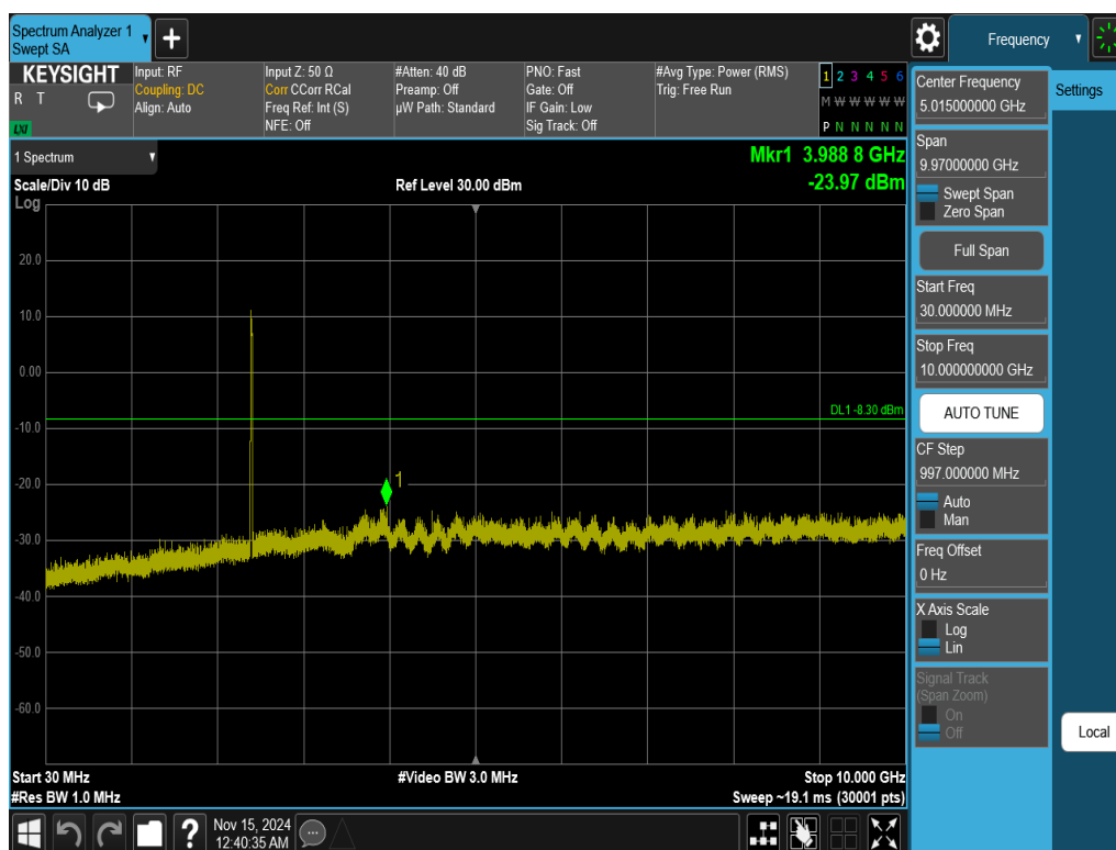
Plot 7-61. Conducted Spurious Plot Antenna WF7b (802.11ax OFDMA – RU242 – Ch. 1)
