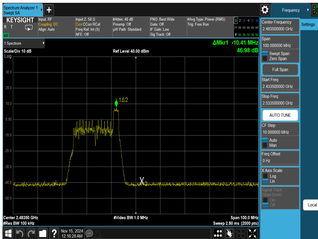
Plot 7-29. Band Edge Antenna WF7b (802.11ax OFDMA – RU26 Index 8 – Ch. 12)
