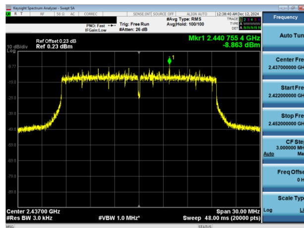
Plot 7-12. Power Spectral Density Plot Antenna WF7b (802.11ax OFDMA – RU242 – Ch. 6)
