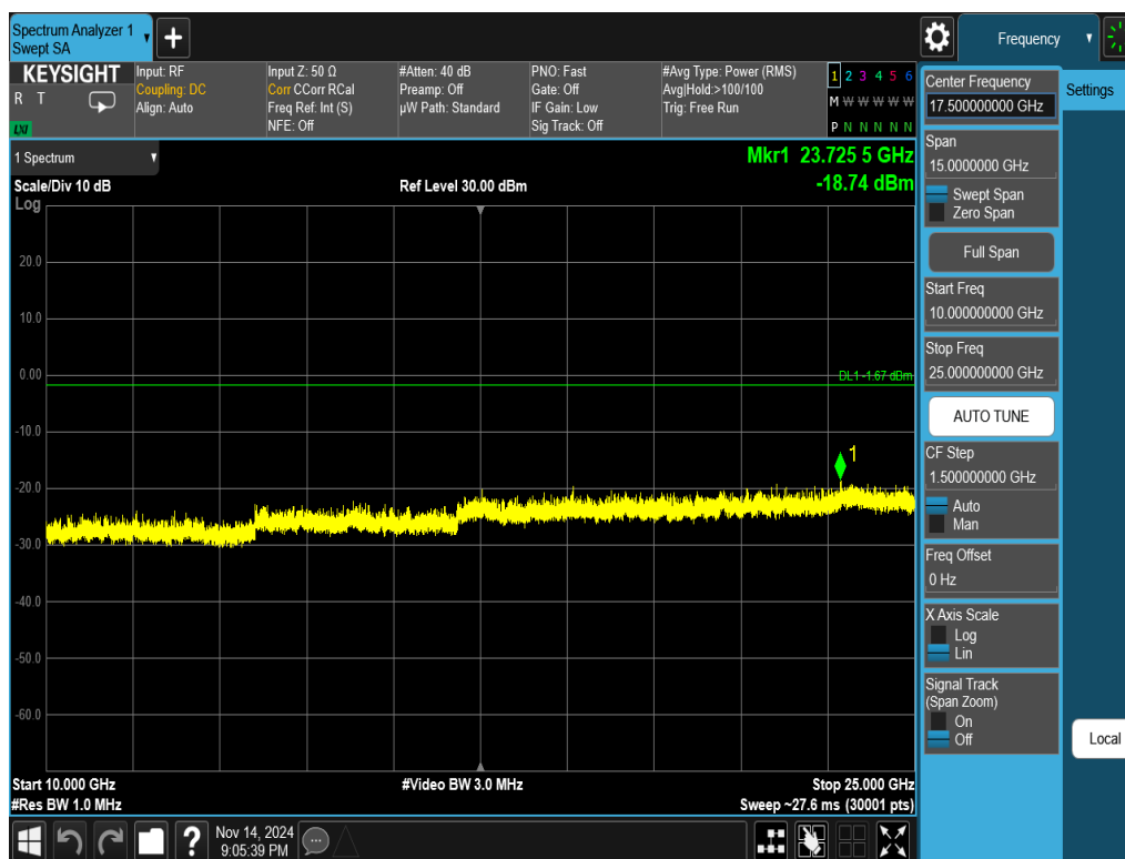
Plot 7-48. Conducted Spurious Plot Antenna WF8 (802.11ax OFDMA – RU26 – Ch. 11)
