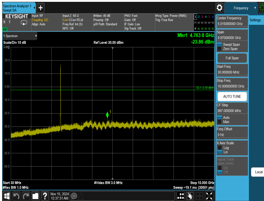
Plot 7-59. Conducted Spurious Plot Antenna WF7b (802.11ax OFDMA – RU26 – Ch. 11)
