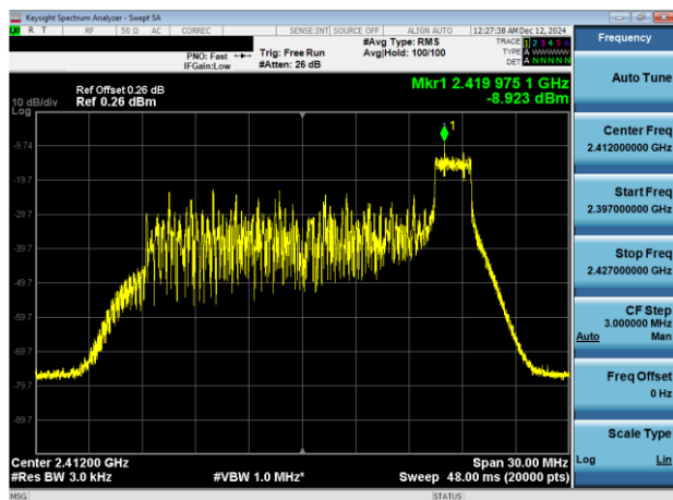
Plot 7-7. Power Spectral Density Plot Antenna WF7b (802.11ax OFDMA – RU26 Index 8 – Ch. 1)
