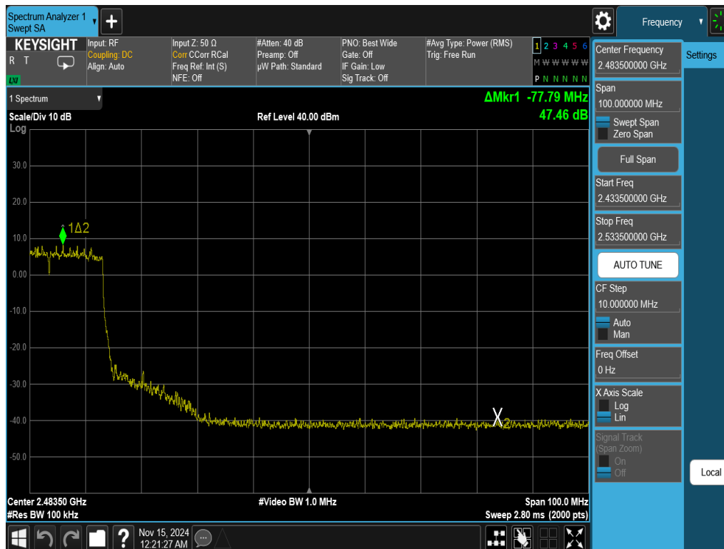
Plot 7-36. Band Edge Antenna WF7b (802.11ax OFDMA – RU242 – Ch. 6(High Channel))
