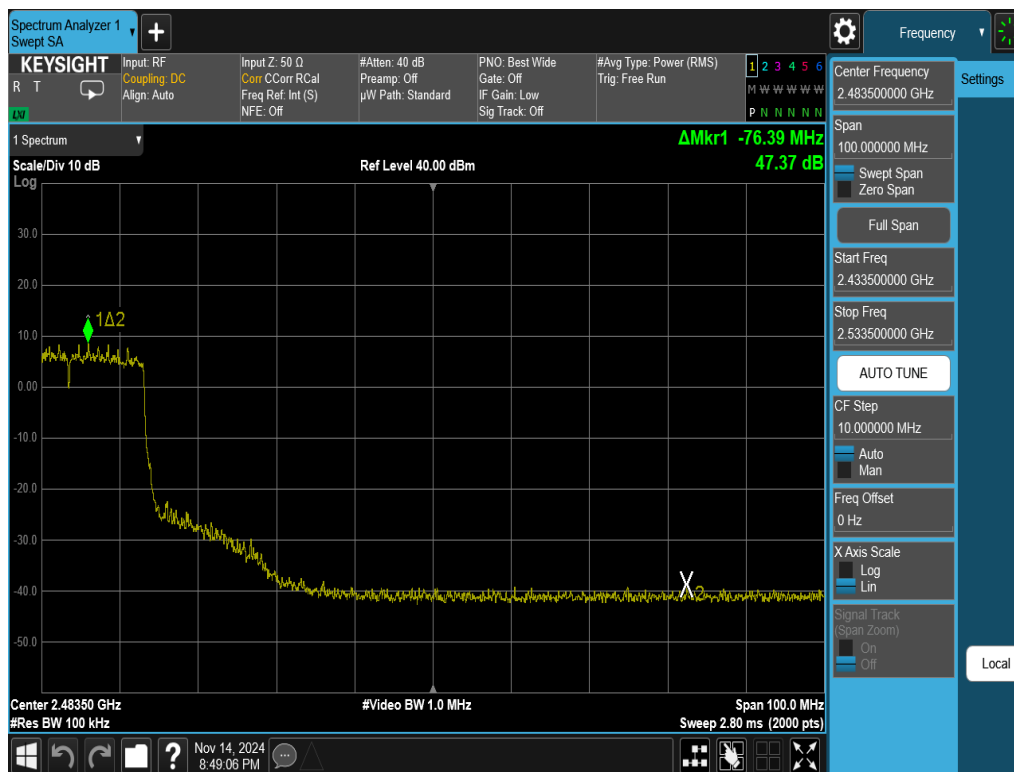
Plot 7-21. Band Edge Antenna WF8 (802.11ax OFDMA – RU242 – Ch. 6(High Channel))
