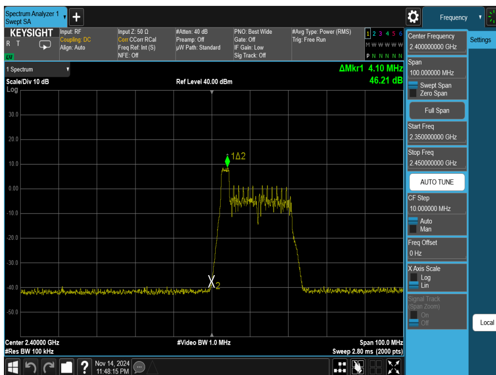
Plot 7-28. Band Edge Antenna WF7b (802.11ax OFDMA – RU26 Index 0 – Ch. 1)
