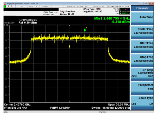
Plot 7-6. Power Spectral Density Plot Antenna WF8 (802.11ax OFDMA – RU242 – Ch. 6)
