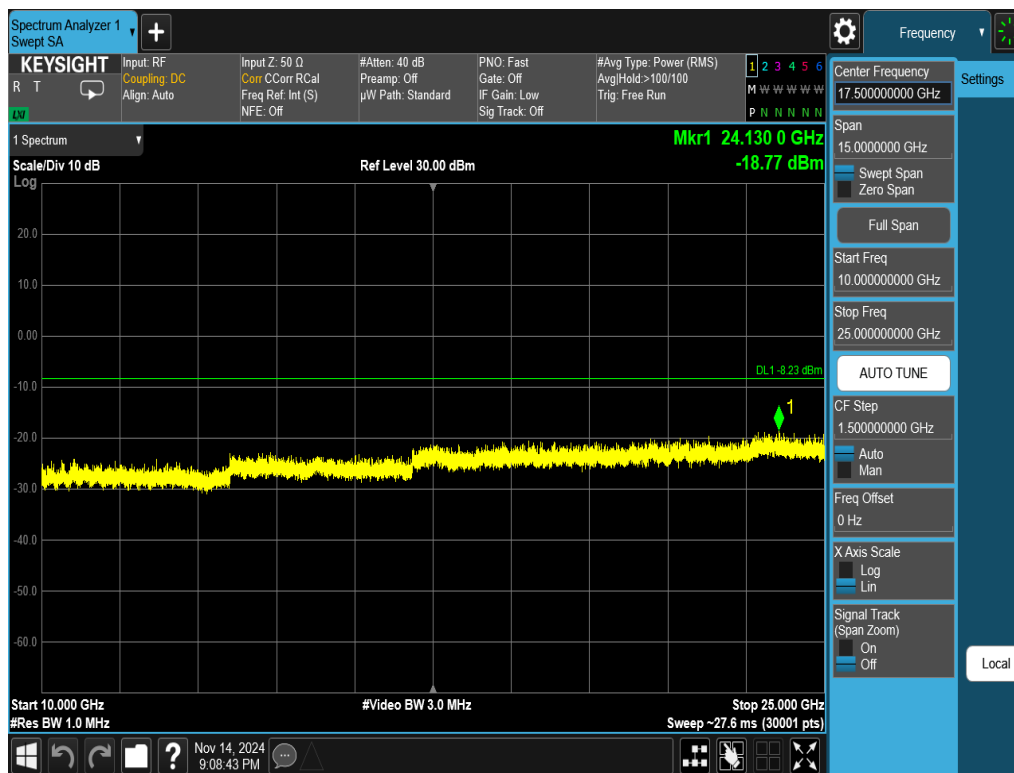
Plot 7-50. Conducted Spurious Plot Antenna WF8 (802.11ax OFDMA – RU242 – Ch. 1)
