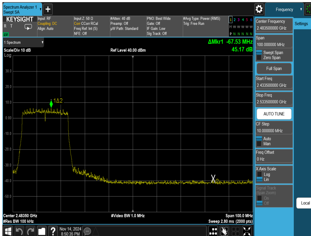
Plot 7-23. Band Edge Antenna WF8 (802.11ax OFDMA – RU242 – Ch. 8)
