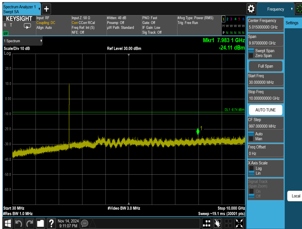
Plot 7-53. Conducted Spurious Plot Antenna WF8 (802.11ax OFDMA – RU242 – Ch. 11)
