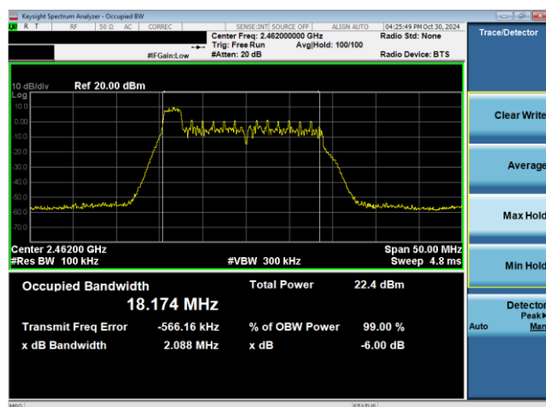
Plot 7-1. 6dB BW & 99% OBW Plot Antenna WF8 (802.11ax OFDMA – RU26 Index 0 – Ch. 11)
