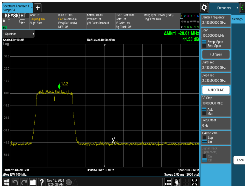
Plot 7-40. Band Edge Antenna WF7b (802.11ax OFDMA – RU242 – Ch. 10)
