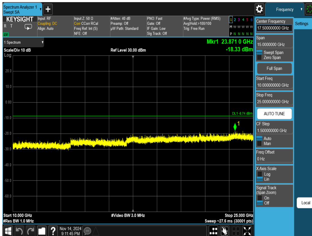
Plot 7-54. Conducted Spurious Plot Antenna WF8 (802.11ax OFDMA – RU242 – Ch. 11)
