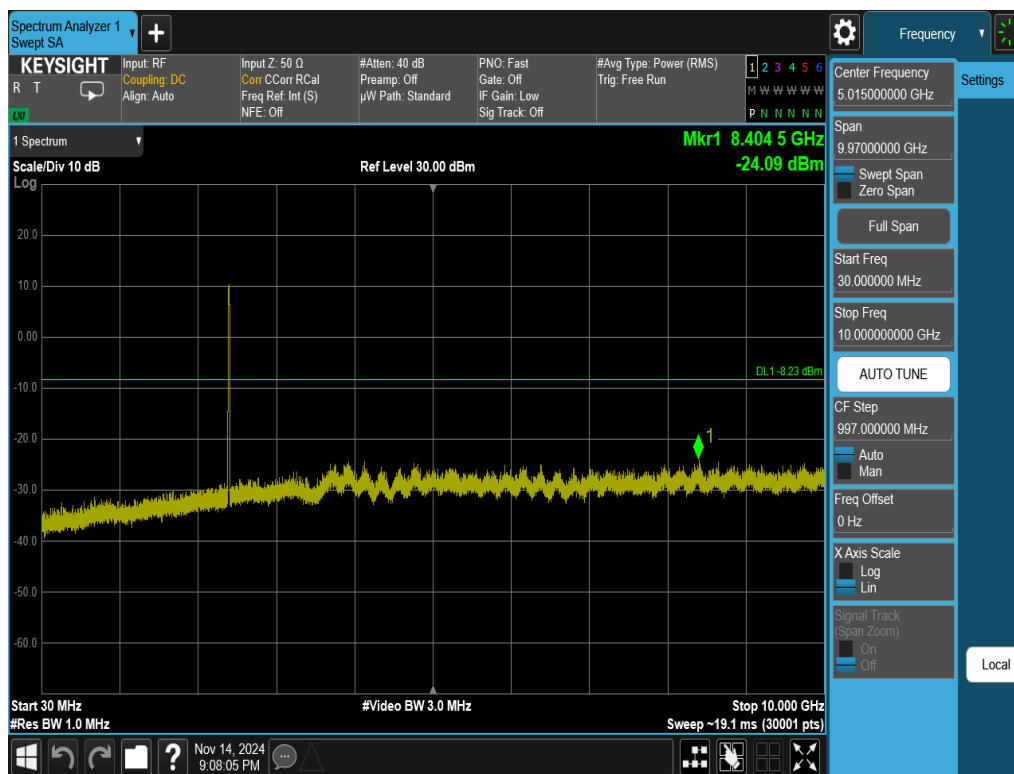
Plot 7-49. Conducted Spurious Plot Antenna WF8 (802.11ax OFDMA – RU242 – Ch. 1)
