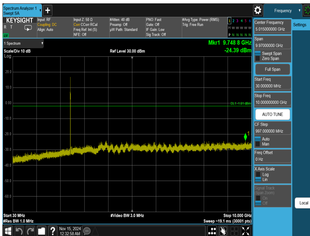
Plot 7-57. Conducted Spurious Plot Antenna WF7b (802.11ax OFDMA – RU26 – Ch. 6)
