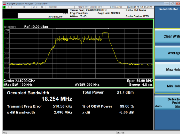
Plot 7-3. 6dB BW & 99% OBW Antenna WF7b (802.11ax OFDMA – RU26 Index 8 – Ch. 11)
