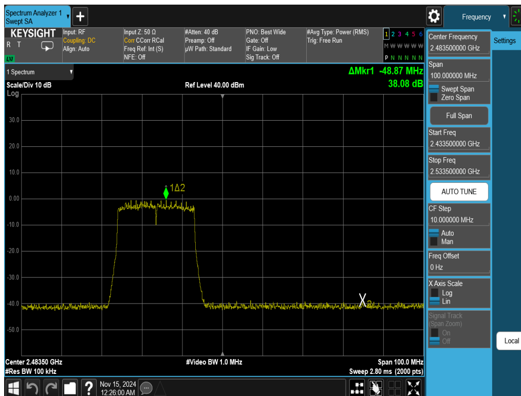
Plot 7-42. Band Edge Antenna WF7b (802.11ax OFDMA – RU242 – Ch. 12)
