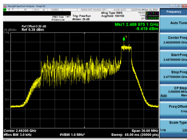
Plot 7-10. Power Spectral Density Plot Antenna WF7b (802.11ax OFDMA – RU26 Index 8 – Ch. 11)
