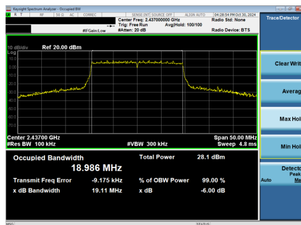
Plot 7-2. 6dB BW & 99% OBW Plot Antenna WF8 (802.11ax OFDMA – RU242 – Ch. 6)
