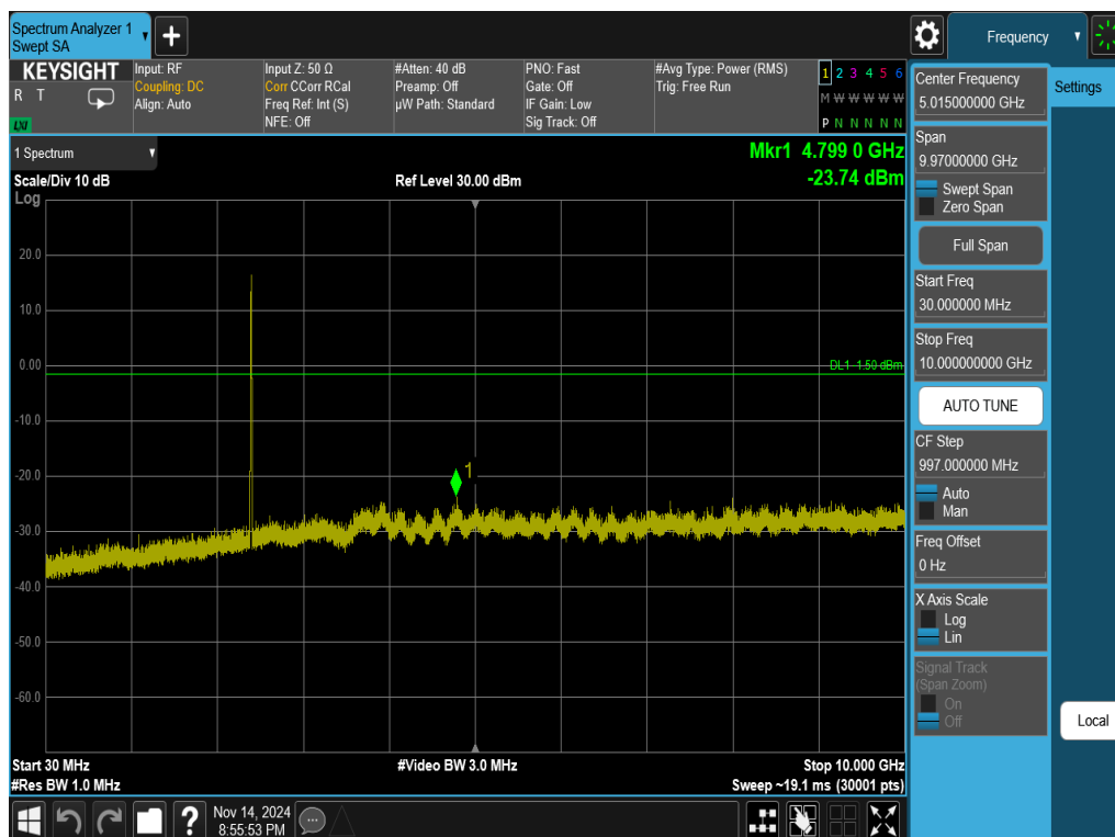
Plot 7-43. Conducted Spurious Plot Antenna WF8 (802.11ax OFDMA – RU26 – Ch. 1)
