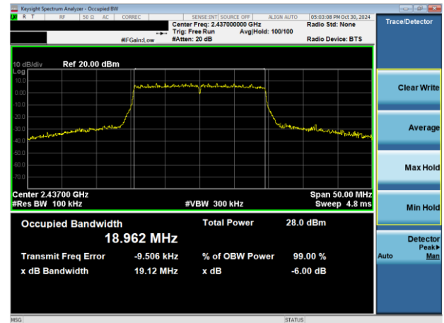
Plot 7-4. 6dB BW & 99% OBW Plot Antenna WF7b (802.11ax OFDMA – RU242 – Ch. 6)
