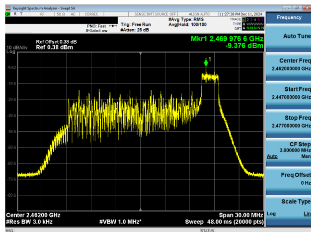
Plot 7-9. Power Spectral Density Plot Antenna WF8 (802.11ax OFDMA – RU26 Index 8 – Ch. 11)
