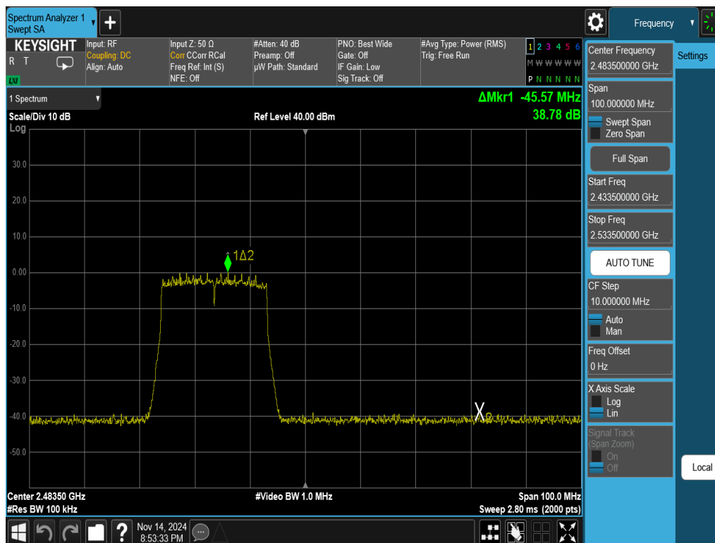
Plot 7-27. Band Edge Antenna WF8 (802.11ax OFDMA – RU242 – Ch. 12)
