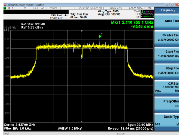
Plot 7-11. Power Spectral Density Plot Antenna WF8 (802.11ax OFDMA – RU242 – Ch. 6)
