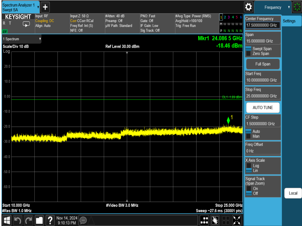
Plot 7-52. Conducted Spurious Plot Antenna WF8 (802.11ax OFDMA – RU242 – Ch. 6)
