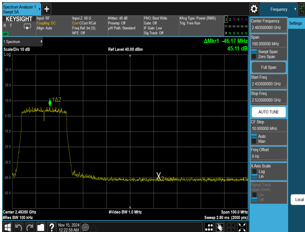
Plot 7-38. Band Edge Antenna WF7b (802.11ax OFDMA – RU242 – Ch. 8)
