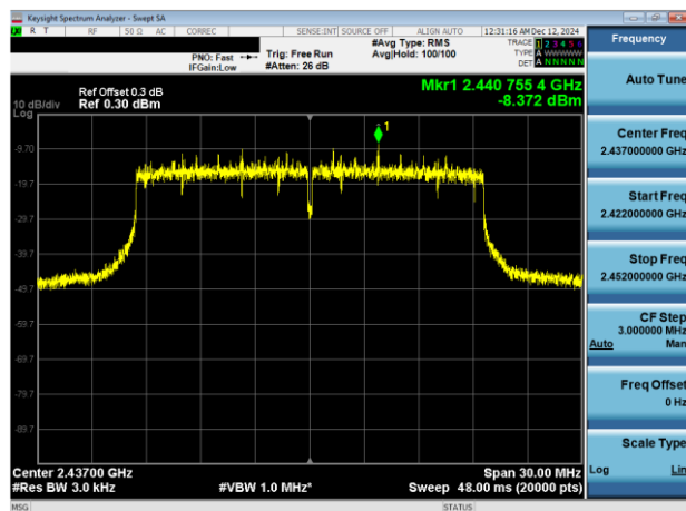
Plot 7-8. Power Spectral Density Plot Antenna WF7b (802.11ax OFDMA – RU242 – Ch. 6)
