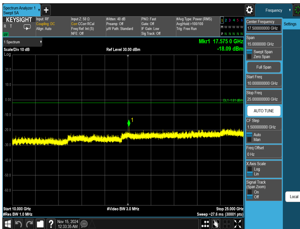
Plot 7-58. Conducted Spurious Plot Antenna WF7b (802.11ax OFDMA – RU26 – Ch. 6)
