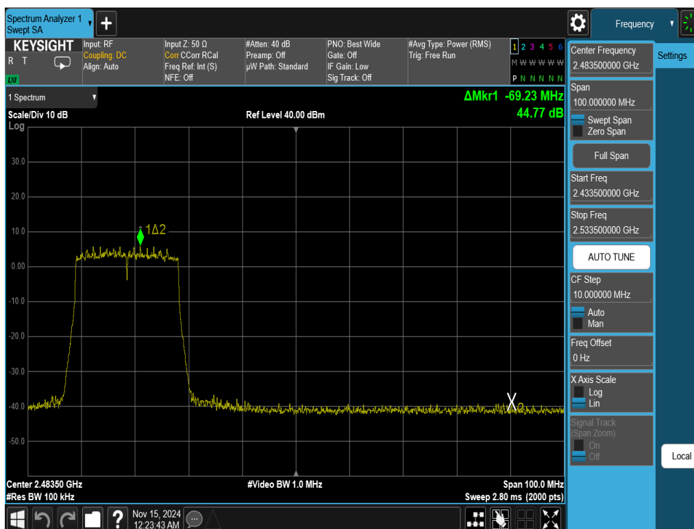
Plot 7-39. Band Edge Antenna WF7b (802.11ax OFDMA – RU242 – Ch. 9)
