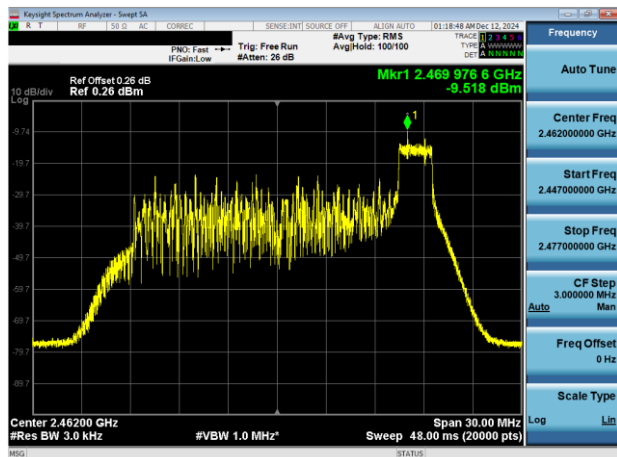
Plot 7-5. Power Spectral Density Plot Antenna WF8 (802.11ax OFDMA – RU26 Index 8 – Ch. 11)
