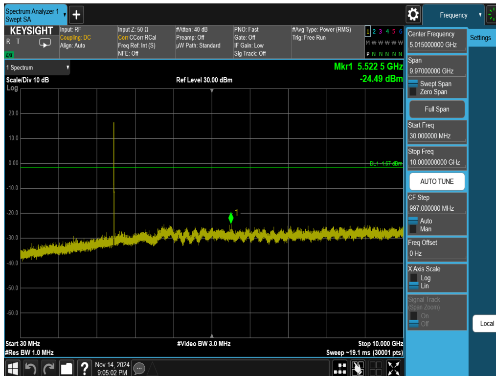
Plot 7-47. Conducted Spurious Plot Antenna WF8 (802.11ax OFDMA – RU26 – Ch. 11)
