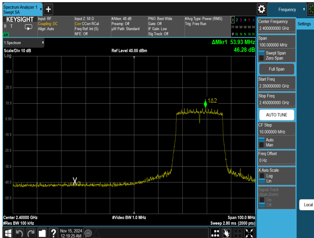
Plot 7-33. Band Edge Antenna WF7b (802.11ax OFDMA – RU242 – Ch. 4)
