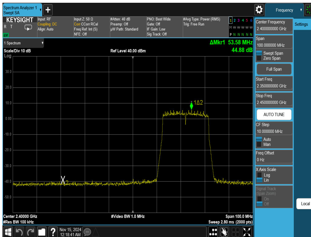
Plot 7-32. Band Edge Antenna WF7b (802.11ax OFDMA – RU242 – Ch. 3)
