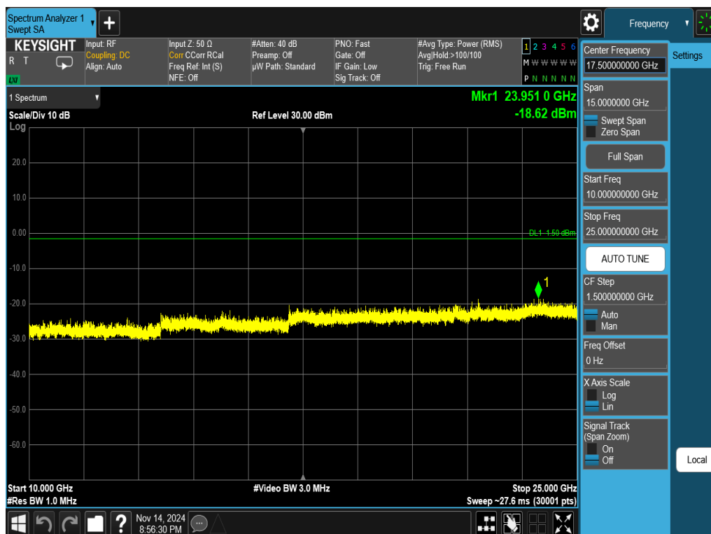
Plot 7-44. Conducted Spurious Plot Antenna WF8 (802.11ax OFDMA – RU26 – Ch. 1)
