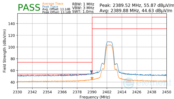
Plot 7-86. Radiated Restricted Lower Band Edge Measurement Antenna WF8
