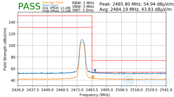
Plot 7-87. Radiated Restricted Upper Band Edge Measurement Antenna WF8
