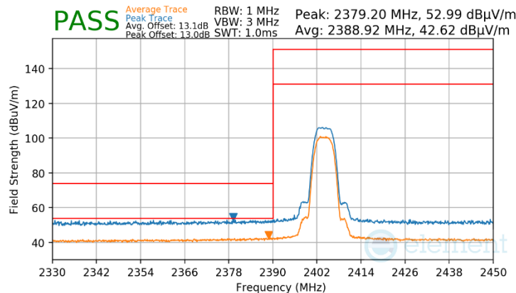
Plot 7-90. Radiated Restricted Lower Band Edge Measurement Antenna WF7b
