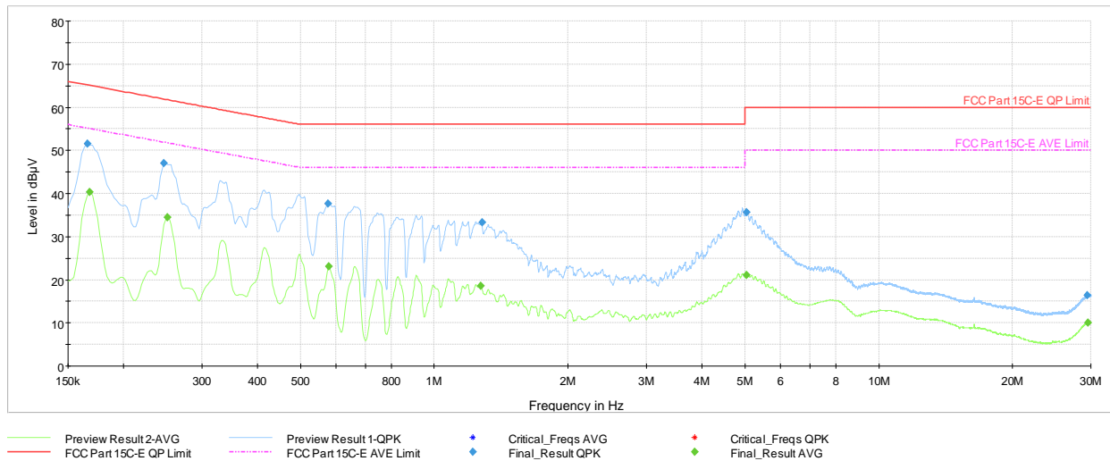
Plot 7-99. AC Line Conducted Plot with Bluetooth HDR TxBF (N, 4Mbps ePA - Ch.38 with AC/DC Adapter via USB-C cable with wire charger)
