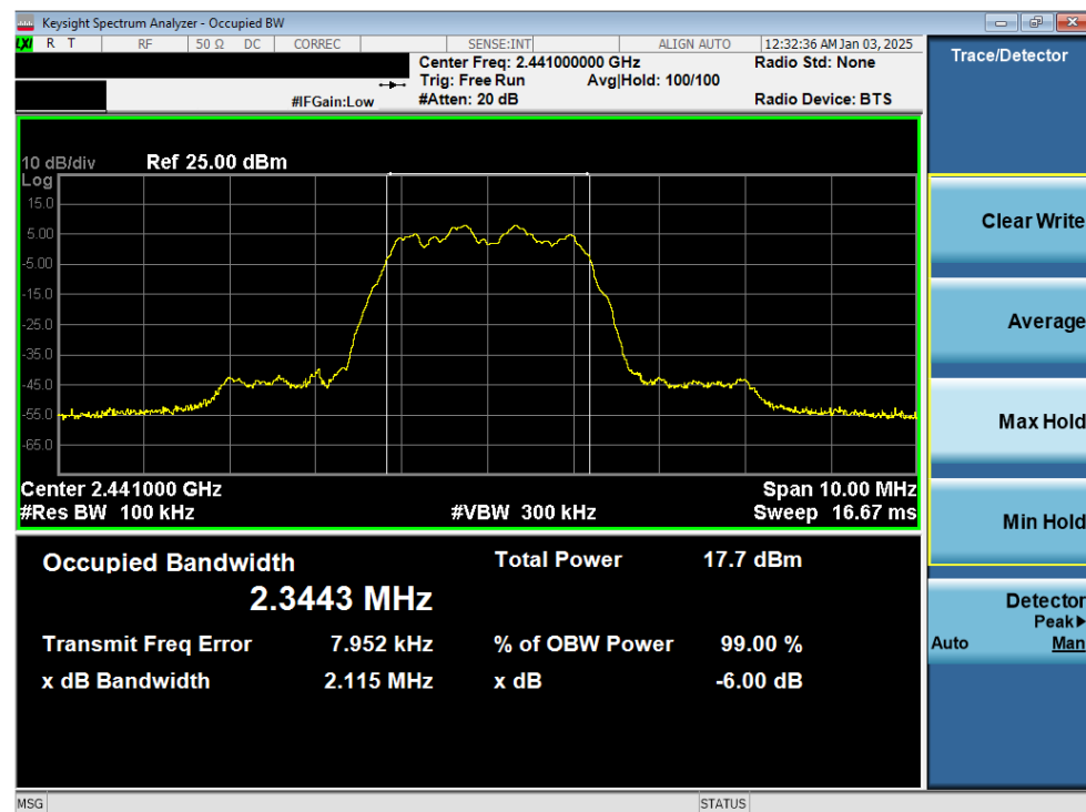
Plot 7-8. 6dB BW & 99% OBW Plot Antenna WF7b (Bluetooth (HDR4), 4Mbps, ePA – Ch. 38)
