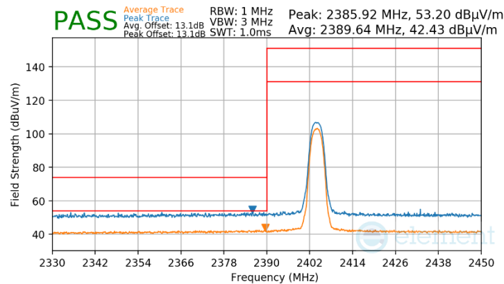
Plot 7-89. Radiated Restricted Lower Band Edge Measurement Antenna WF7b
