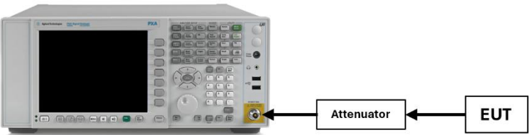
Figure 7-1. Test Instrument & Measurement Setup
