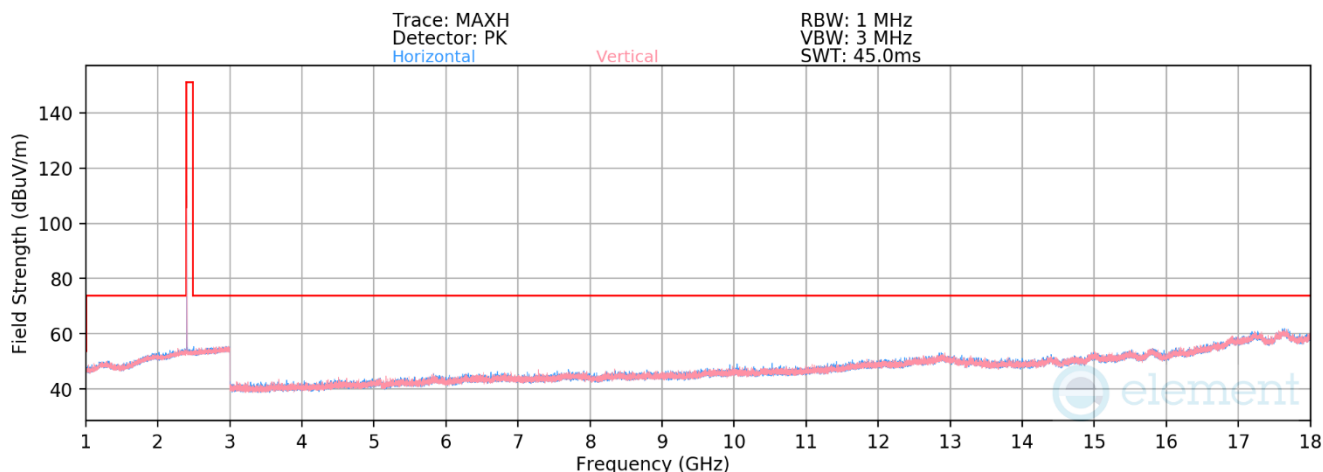
Plot 7-81. Radiated Spurious Emissions 1-18GHz TxBF (4Mbps, HDR4, ePA – Ch. 1)
