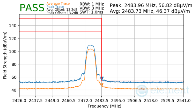
Plot 7-88. Radiated Restricted Upper Band Edge Measurement Antenna WF8
