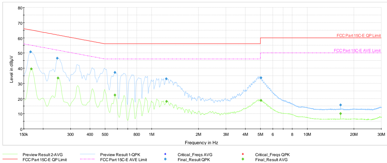
Plot 7-98. AC Line Conducted Plot with Bluetooth HDR Tx BF (L1, 4Mbps ePA - Ch.38 with AC/DC Adapter via USB-C cable with wire charger)
