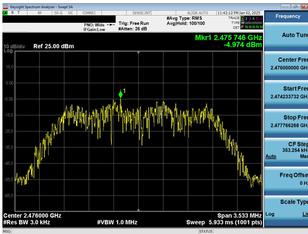
Plot 7-41. Power Spectral Density Plot TxBF Antenna WF8 (Bluetooth (HDR4), 4Mbps, ePA – Ch. 73)
