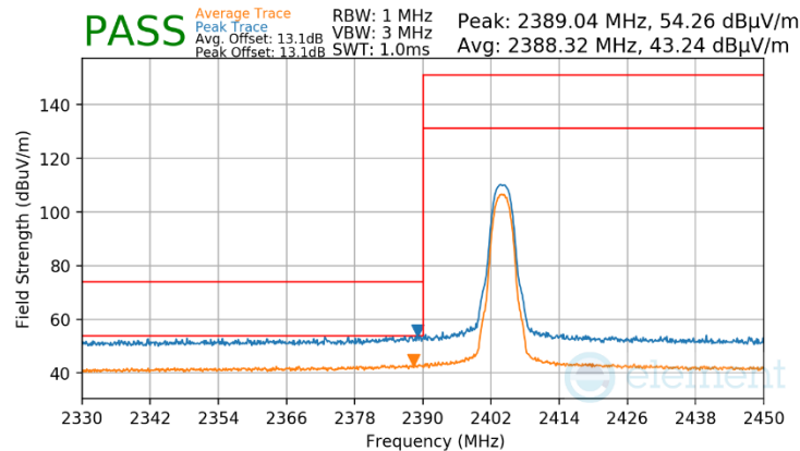
Plot 7-85. Radiated Restricted Lower Band Edge Measurement Antenna WF8
