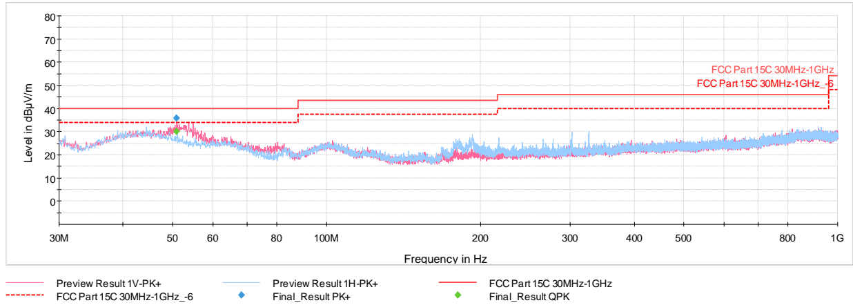
Plot 7-97. Radiated Spurious Emissions Below 1GHz TxBF (4Mbps, ePA – Ch.38 with AC/DC Adapter via USB-C cable with wire charger)
