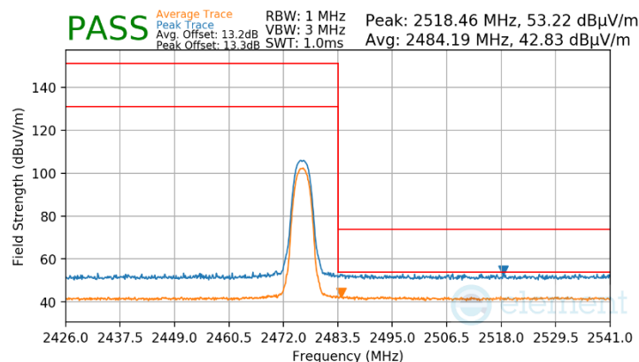
Plot 7-91. Radiated Restricted Upper Band Edge Measurement Antenna WF7b
