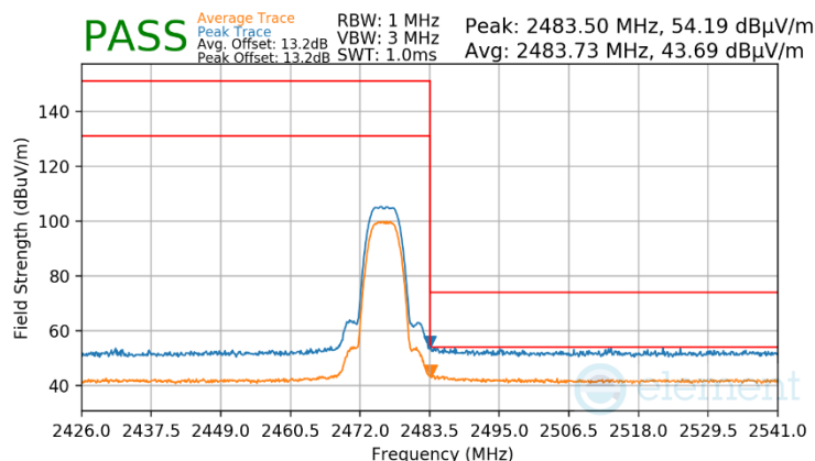
Plot 7-92. Radiated Restricted Upper Band Edge Measurement Antenna WF7b
