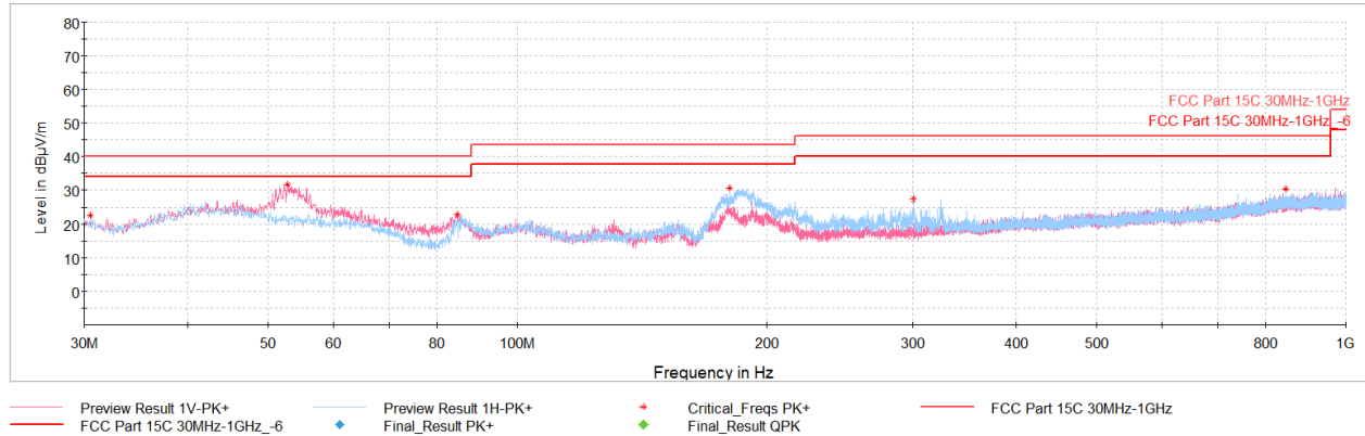
Plot 7-78. Radiated Spurious Emissions – Simultaneous Transmission Below 1GHz (with AC/DC Adapter)
