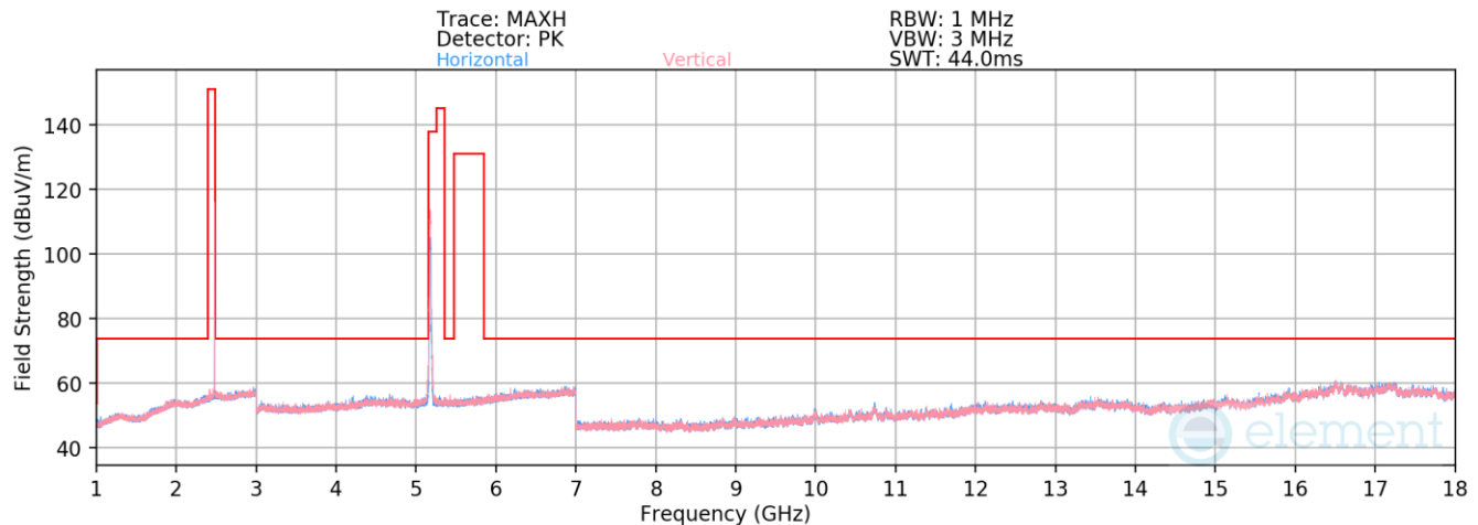
Plot 7-63. Radiated Spurious Emissions – Simultaneous Transmission Above 1GHz (with AC/DC Adapter)
