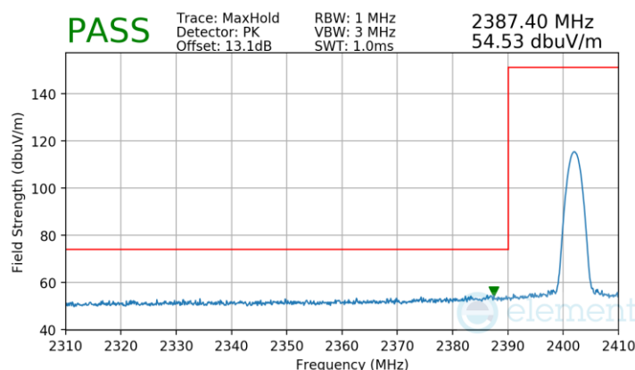
Plot 7-66. Radiated Restricted Lower Band Edge Measurement Antenna WF8
