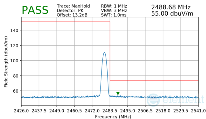
Plot 7-72. Radiated Restricted Upper Band Edge Measurement Antenna WF7b
