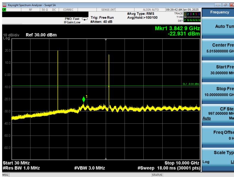
Plot 7-57. Conducted Simultaneous Tx Spurious Plots AntennaWF8 (Bluetooth + UNII)
