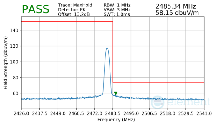
Plot 7-67. Radiated Restricted Upper Band Edge Measurement Antenna WF8
