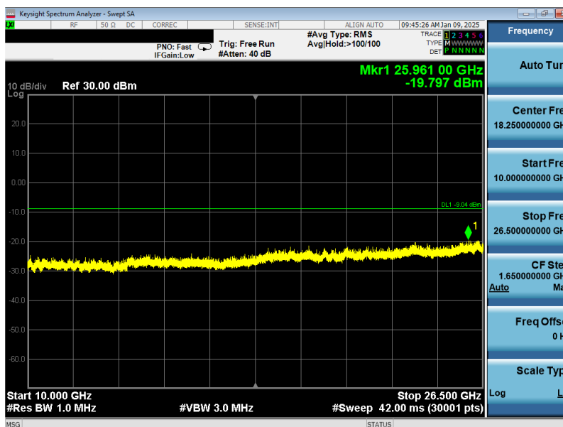
Plot 7-58. Conducted Simultaneous Tx Spurious Plots AntennaWF8 (Bluetooth + UNII)
