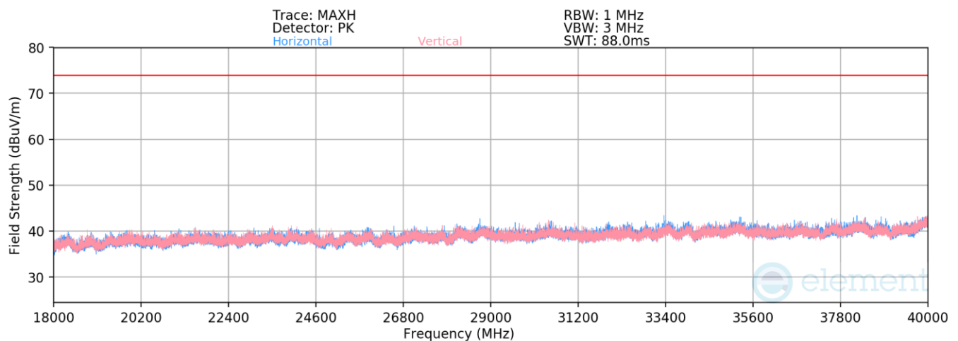
Plot 7-64. Radiated Spurious Emissions – Simultaneous Transmission Above 18GHz (with AC/DC Adapter)
