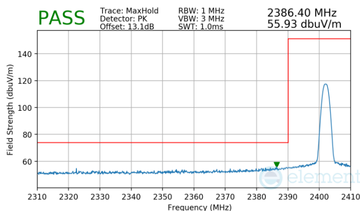
Plot 7-65. Radiated Restricted Lower Band Edge Measurement Antenna WF8
