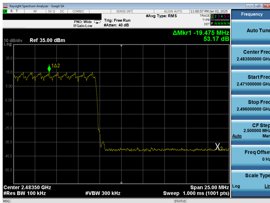
Plot 7-28. Band Edge Plot Antenna WF7b (Bluetooth with Hopping Enabled, 8DPSK, ePA – Ch 78)
