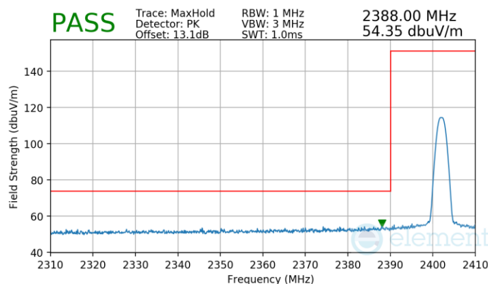
Plot 7-69. Radiated Restricted Lower Band Edge Measurement Antenna WF7b
