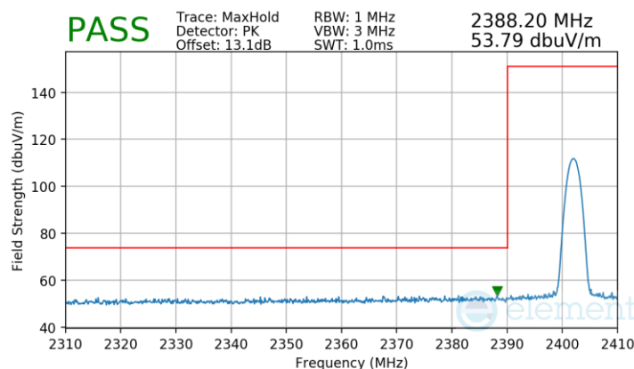
Plot 7-70. Radiated Restricted Lower Band Edge Measurement Antenna WF7b
