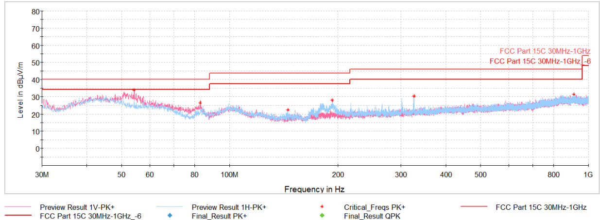
Plot 7-77. Radiated Spurious Emissions Below 1GHz TxBF (GFSK ePA – Ch.39, with AC/DC Adapter)
