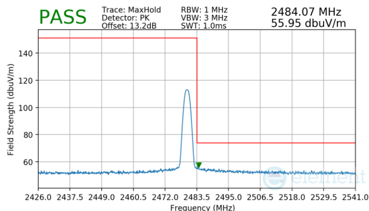
Plot 7-71. Radiated Restricted Upper Band Edge Measurement Antenna WF7b
