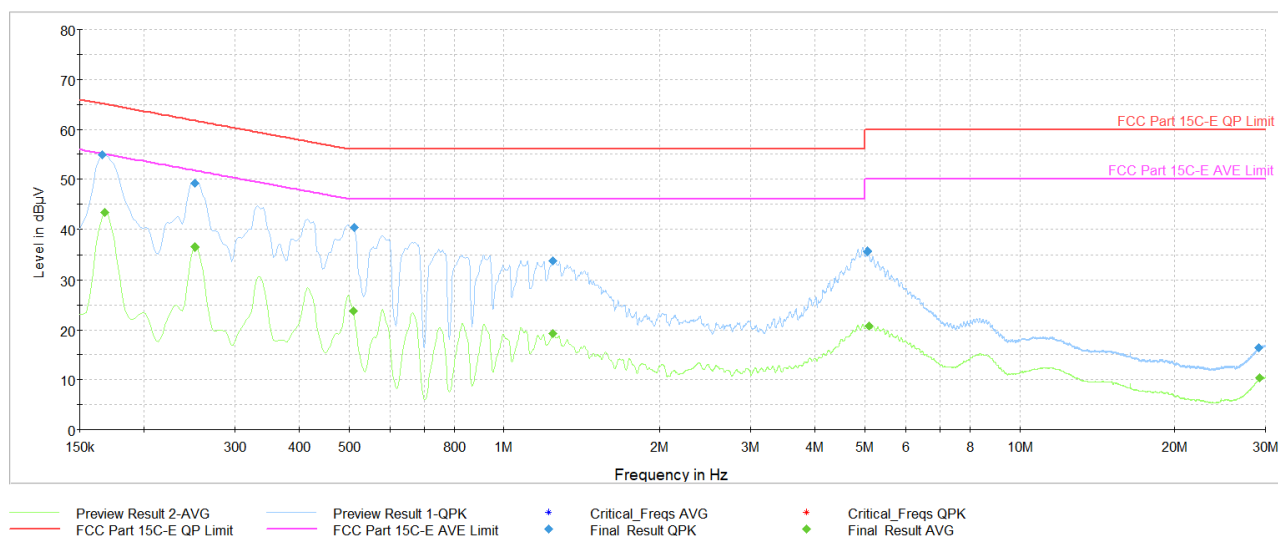
Plot 7-80. AC Line-Conducted Test Plot TxBF (N, GFSK ePA – Ch.39, with AC/DC Adapter)
