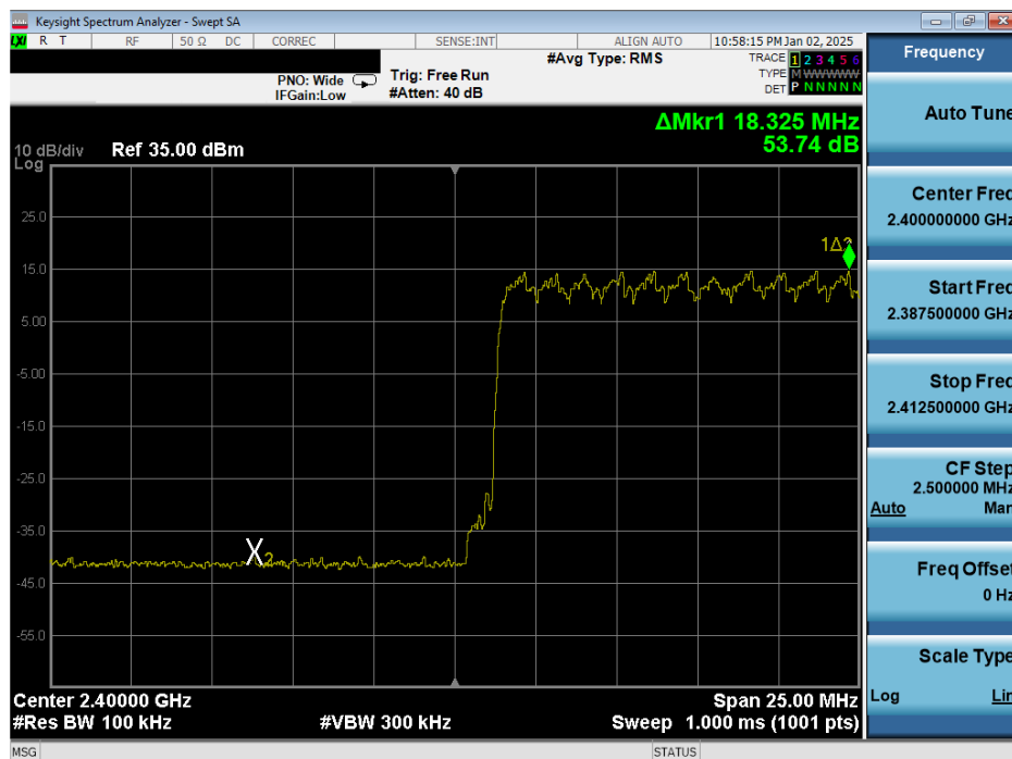
Plot 7-27. Band Edge Plot Antenna WF7b (Bluetooth with Hopping Enabled, 8DPSK, ePA – Ch. 0)
