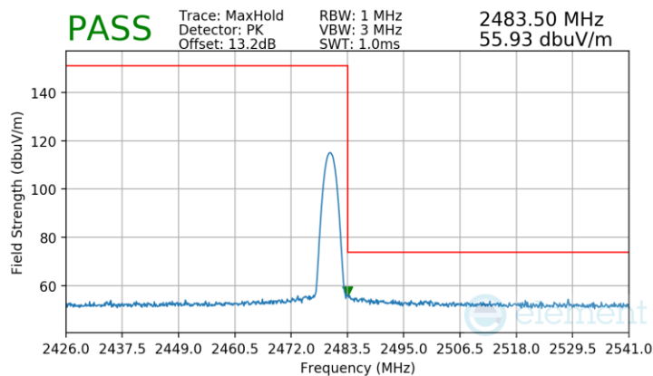
Plot 7-68. Radiated Restricted Upper Band Edge Measurement Antenna WF8
