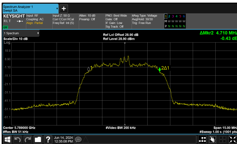
Figure 72 - Core 0 (A) 5789 MHz (CH64) 99% Bandwidth
