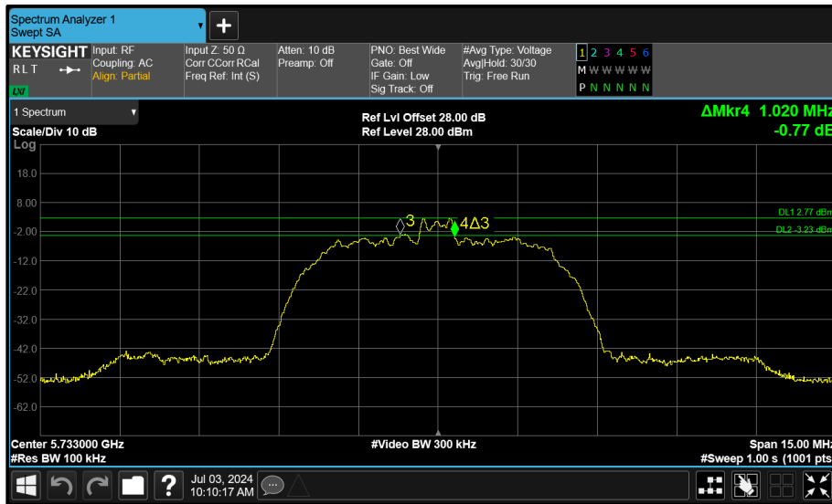
Figure 121 - Core 1 (B) 5733 MHz (CH8) 6 dB Bandwidth
