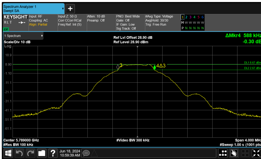
Figure 99 - Core 0 (A) 5789 MHz (CH64) 6 dB Bandwidth
