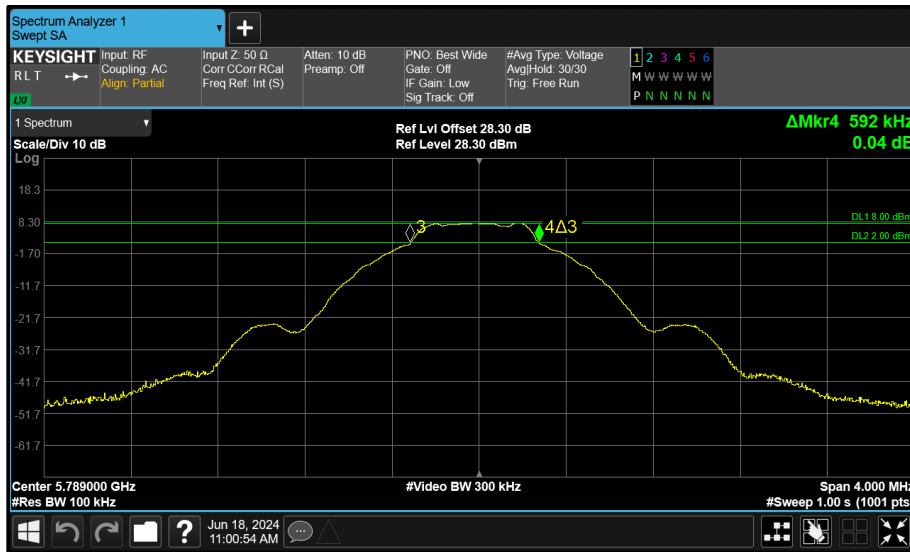
Figure 101 - Core 1 (B) 5789 MHz (CH64) 6 dB Bandwidth
