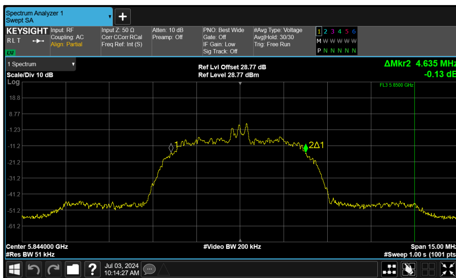
Figure 126 - Core 0 (A) 5844 MHz (CH119) 99% Bandwidth
