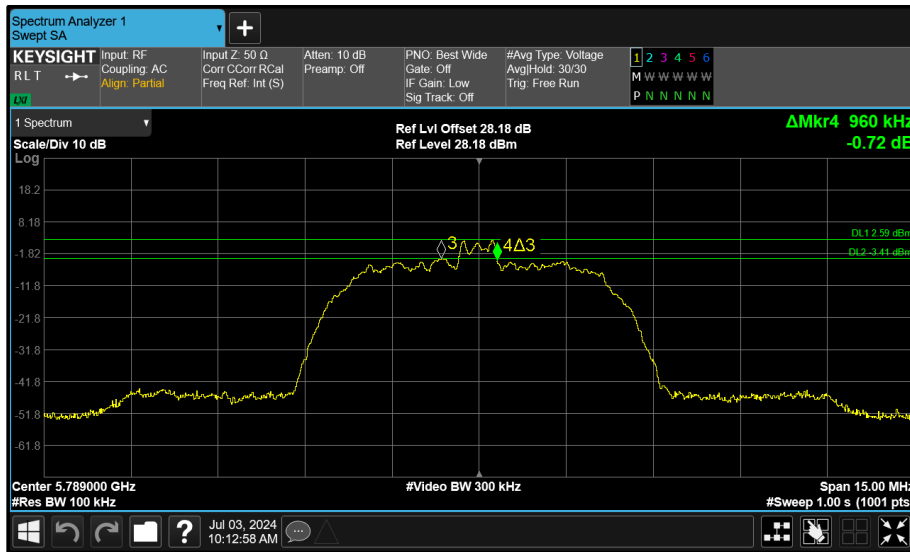
Figure 125 - Core 1 (B) 5789 MHz (CH64) 6 dB Bandwidth
