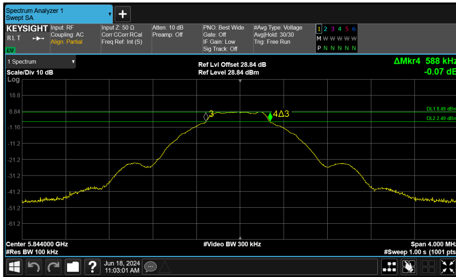
Figure 103 - Core 0 (A) 5844 MHz (CH119) 6 dB Bandwidth
