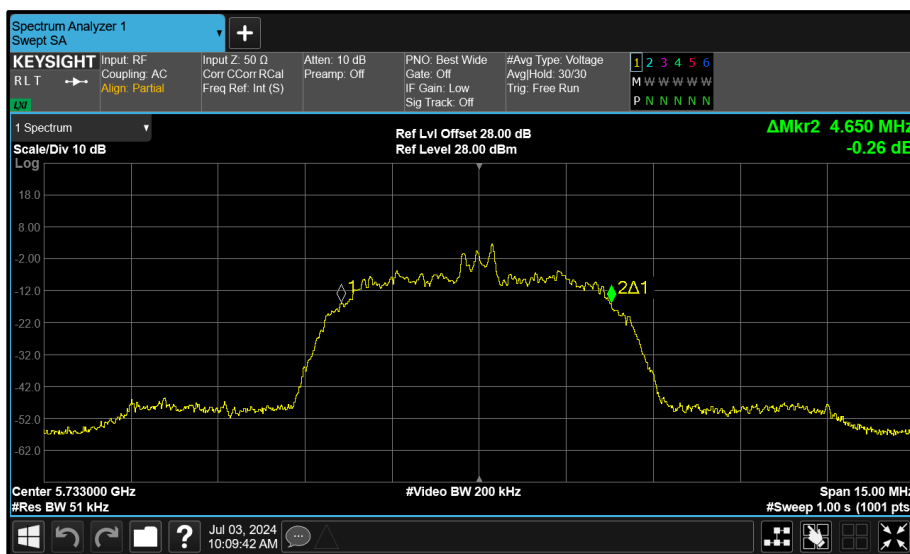
Figure 120 - Core 1 (B) 5733 MHz (CH8) 99% Bandwidth
