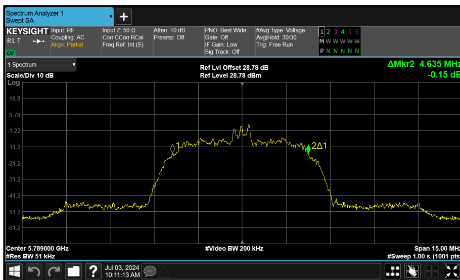
Figure 122 - Core 0 (A) 5789 MHz (CH64) 99% Bandwidth
