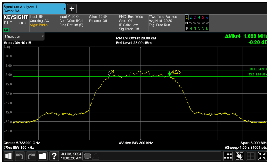
Figure 109 - Core 1 (B) 5733 MHz (CH8) 6 dB Bandwidth
