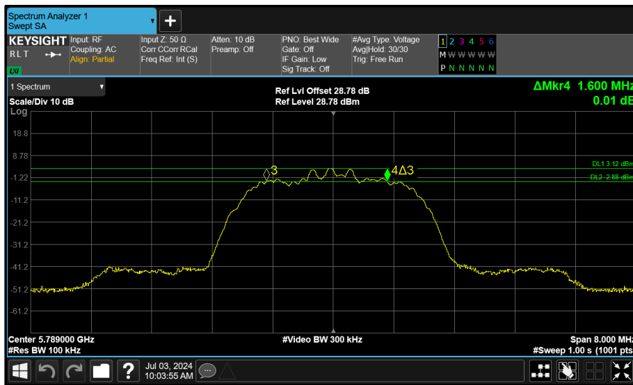
Figure 111 - Core 0 (A) 5789 MHz (CH64) 6 dB Bandwidth
