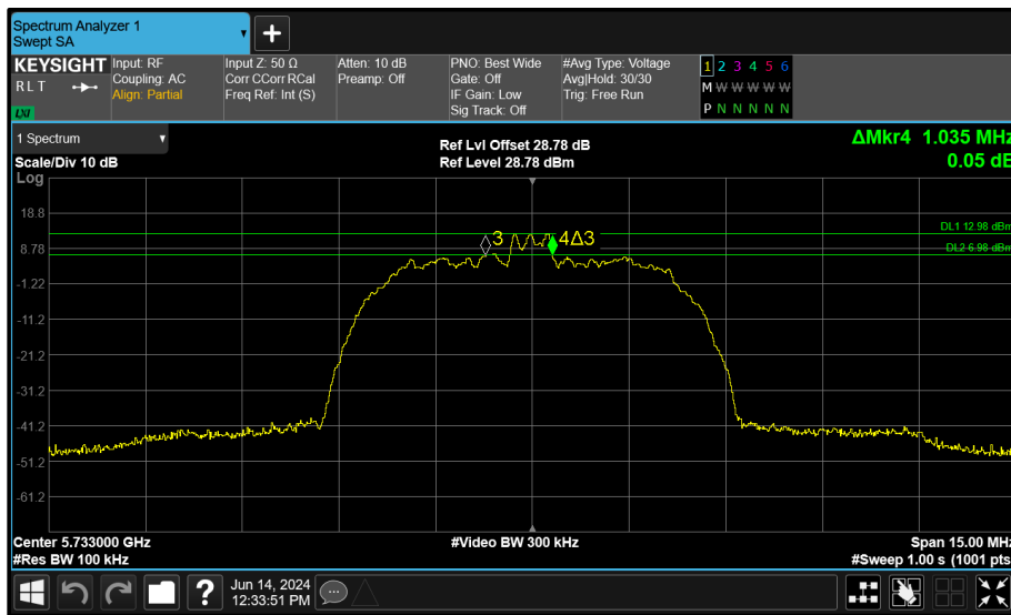
Figure 71 - Core 0 (A) 5733 MHz (CH8) 6 dB Bandwidth
