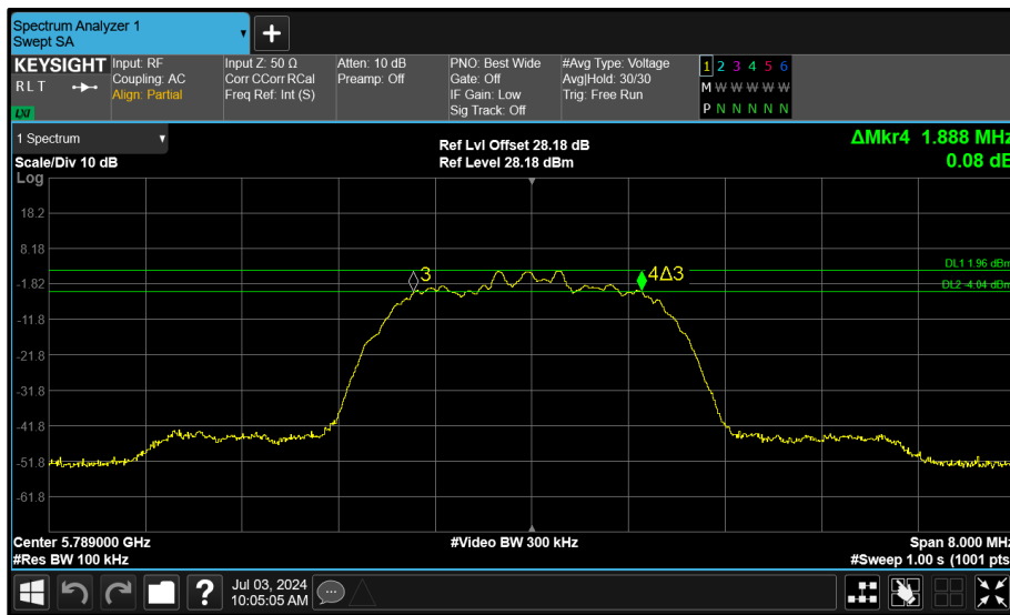
Figure 113 - Core 1 (B) 5789 MHz (CH64) 6 dB Bandwidth
