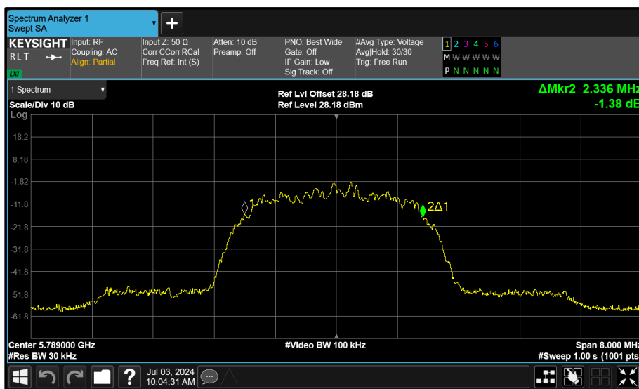
Figure 112 - Core 1 (B) 5789 MHz (CH64) 99% Bandwidth
