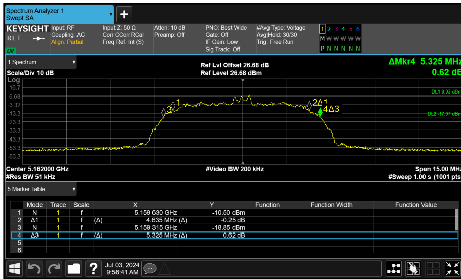
Figure 137 - Core 1 (B) 5162 MHz (CH12) 26 dB and 99% Bandwidth
