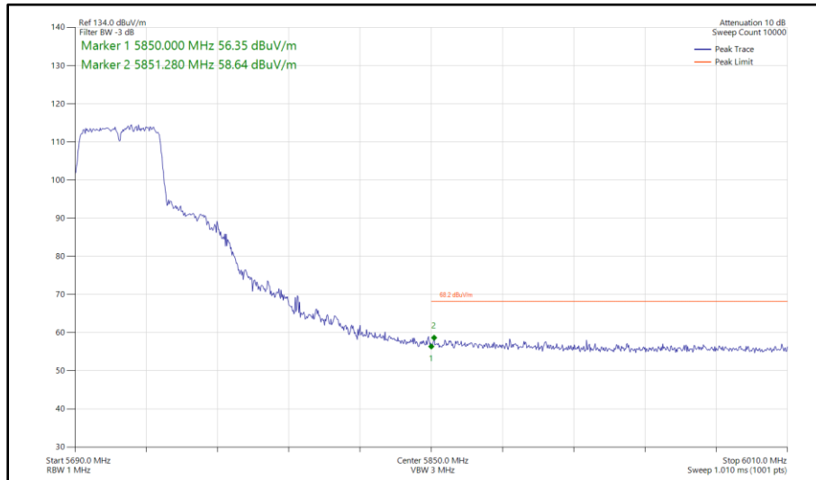
Figure 443 - 802.11n HT40, SISO, Core 0 - 5710 MHz Band Edge Frequency 5850 MHz
