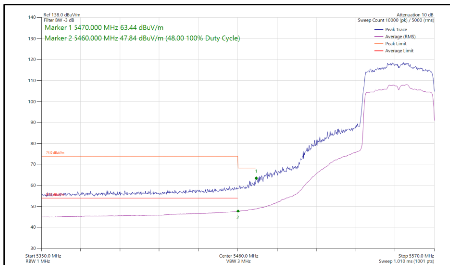
Figure 476 - 802.11ax HE40, SU, CDD, Core 0 - Core 1 - 5550 MHz Band Edge Frequency 5470 MHz
