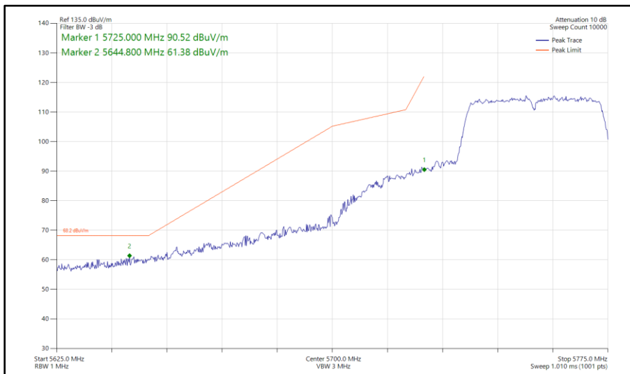
Figure 435 - 802.11n HT40, SISO, Core 0 - 5755 MHz Band Edge Frequency 5725 MHz
