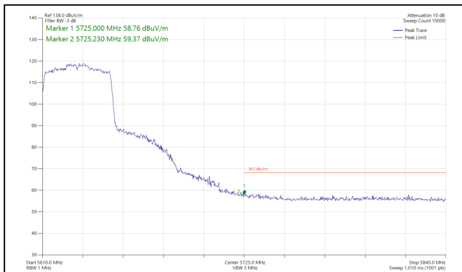
Figure 462 - 802.11ax HE40, SU, SISO, Core 1 - 5630 MHz Band Edge Frequency 5725 MHz
