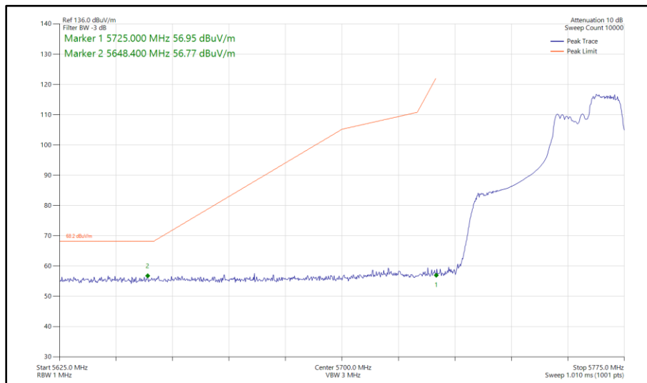
Figure 437 - 802.11ax HE40, RU 106-56, SISO, Core 0 - 5755 MHz Band Edge Frequency 5725 MHz
