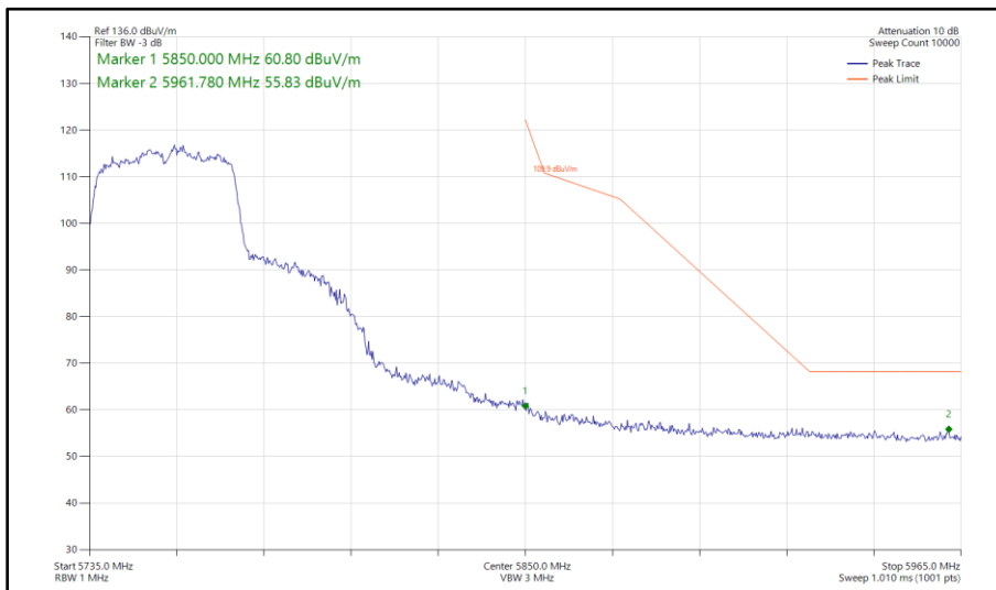
Figure 487 - 802.11n HT40, CDD, Core 0 - Core 1 - 5755 MHz Band Edge Frequency 5850 MHz
