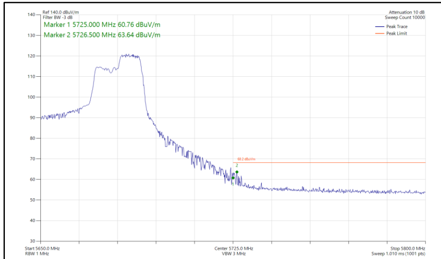
Figure 485 - 802.11ax HE40, RU 106-56, CDD, Core 0 - Core 1 - 5670 MHz Band Edge Frequency 5725 MHz
