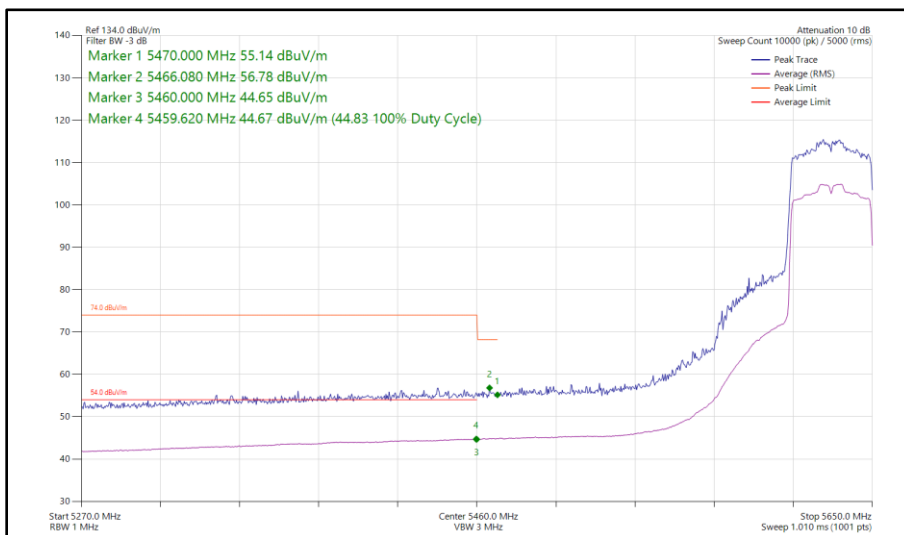
Figure 434 - 802.11ax HE40, SU, SISO, Core 0 - 5630 MHz Band Edge Frequency 5470 MHz
