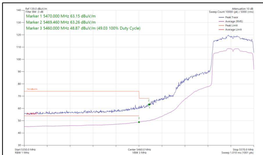
Figure 454 - 802.11ax HE40, SU, SISO, Core 1 - 5550 MHz Band Edge Frequency 5470 MHz
