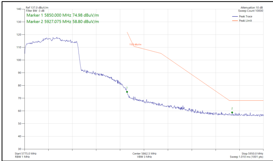
Figure 469 - 802.11ax HE40, SU, SISO, Core 1 - 5795 MHz Band Edge Frequency 5850 MHz
