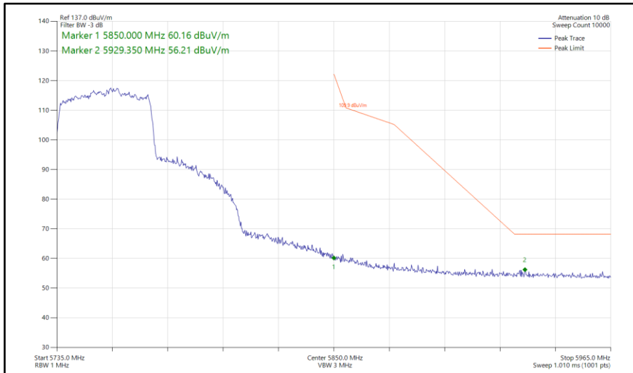
Figure 491 - 802.11ax HE40, SU, CDD, Core 0 - Core 1 - 5755 MHz Band Edge Frequency 5850 MHz
