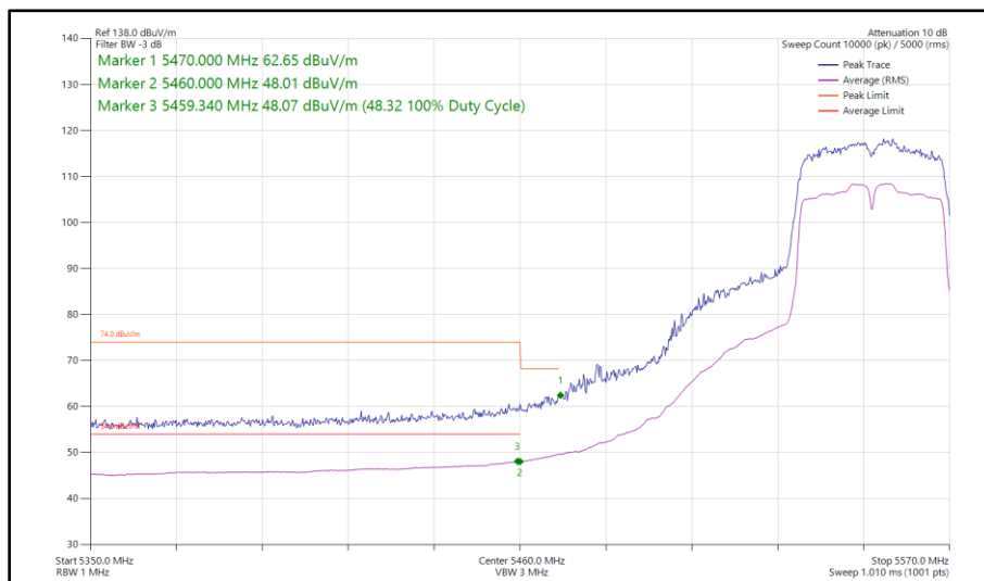
Figure 450 - 802.11n HT40, SISO, Core 1 - 5550 MHz Band Edge Frequency 5470 MHz
