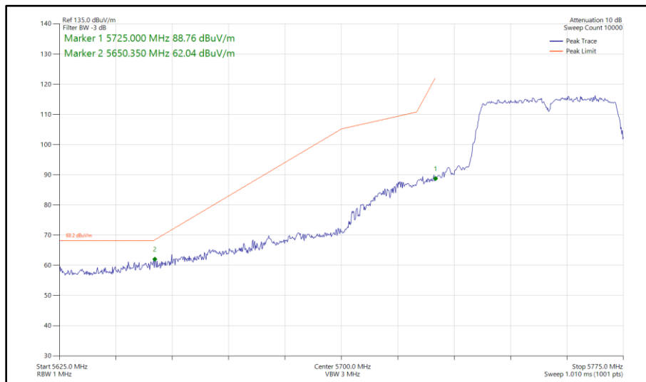
Figure 457 - 802.11n HT40, SISO, Core 1 - 5755 MHz Band Edge Frequency 5725 MHz
