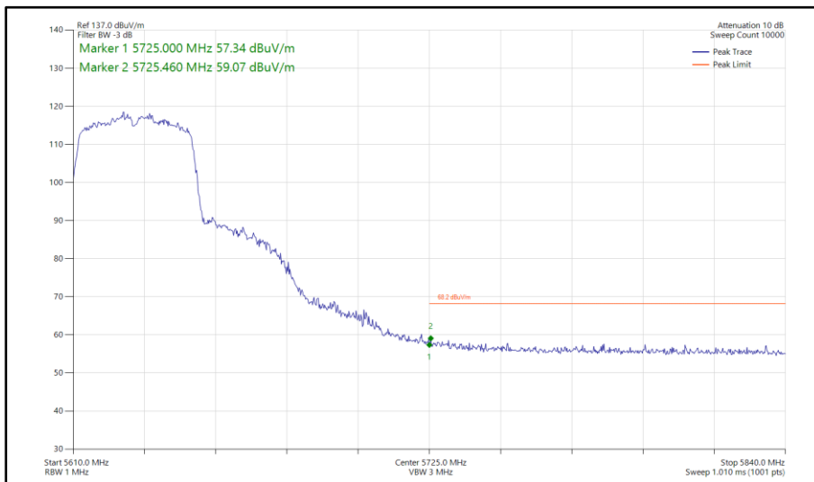
Figure 481 - 802.11n HT40, CDD, Core 0 - Core 1 - 5630 MHz Band Edge Frequency 5725 MHz
