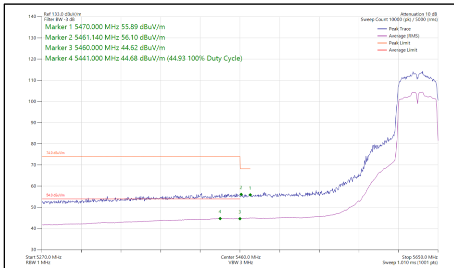
Figure 429 - 802.11n HT40, SISO, Core 0 - 5630 MHz Band Edge Frequency 5470 MHz
