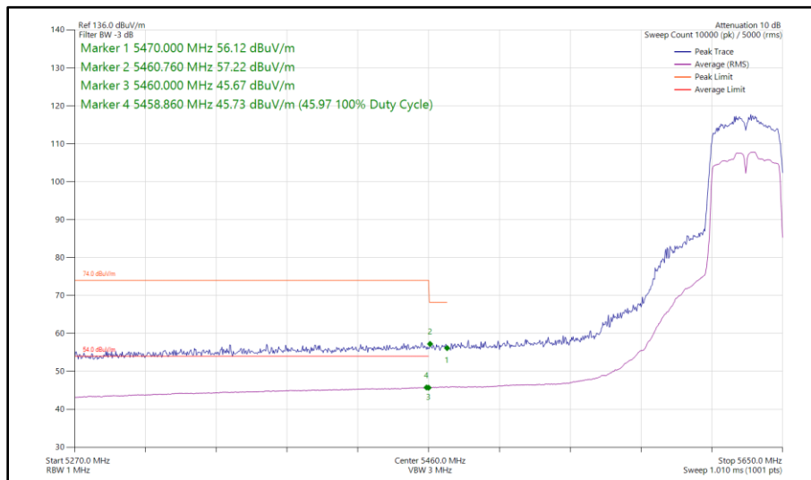
Figure 451 - 802.11n HT40, SISO, Core 1 - 5630 MHz Band Edge Frequency 5470 MHz
