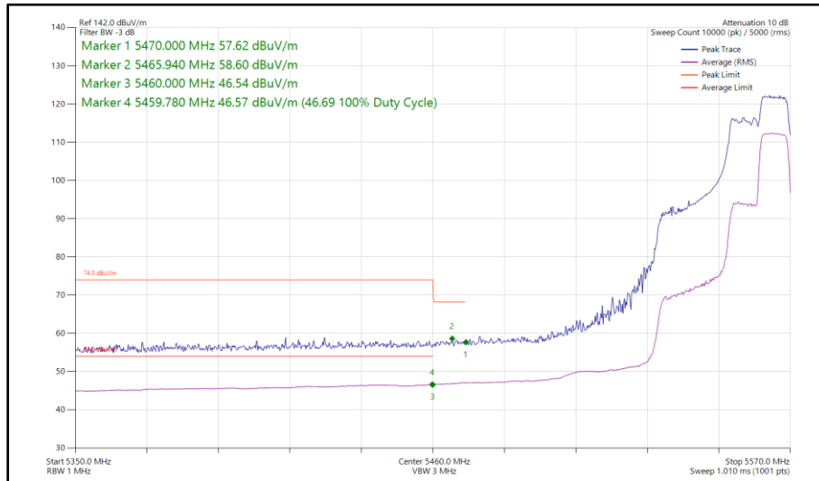
Figure 455 - 802.11ax HE40, RU 106-56, SISO, Core 1 - 5550 MHz Band Edge Frequency 5470 MHz
