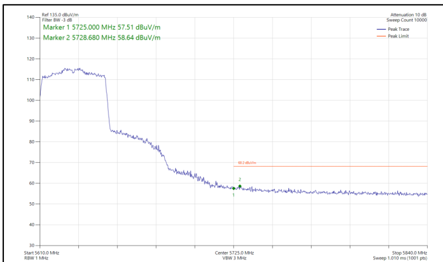
Figure 440 - 802.11ax HE40, SU, SISO, Core 0 - 5630 MHz Band Edge Frequency 5725 MHz
