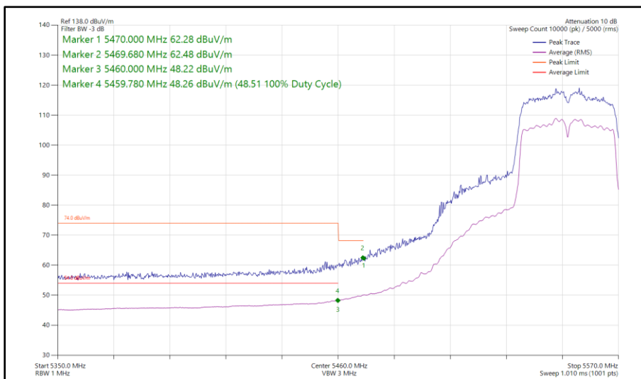
Figure 472 - 802.11n HT40, CDD, Core 0 - Core 1 - 5550 MHz Band Edge Frequency 5470 MHz
