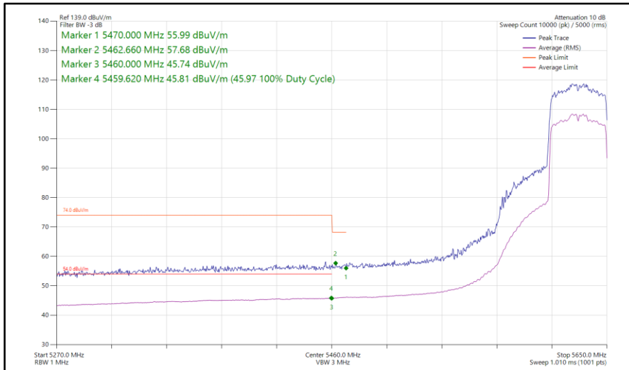
Figure 477 - 802.11ax HE40, SU, CDD, Core 0 - Core 1 - 5630 MHz Band Edge Frequency 5470 MHz
