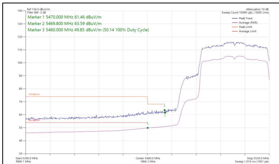
Figure 452 - 802.11ax HE40, SU, SISO, Core 1 - 5510 MHz Band Edge Frequency 5470 MHz
