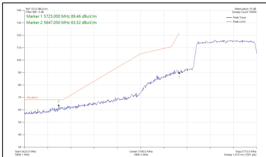
Figure 458 - 802.11ax HE40, SU, SISO, Core 1 - 5755 MHz Band Edge Frequency 5725 MHz
