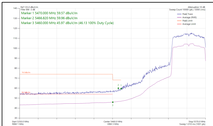
Figure 432 - 802.11ax HE40, SU, SISO, Core 0 - 5550 MHz Band Edge Frequency 5470 MHz
