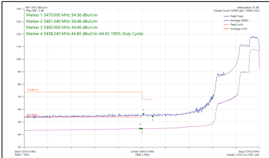
Figure 433 - 802.11ax HE40, RU 106-56, SISO, Core 0 - 5550 MHz Band Edge Frequency 5470 MHz
