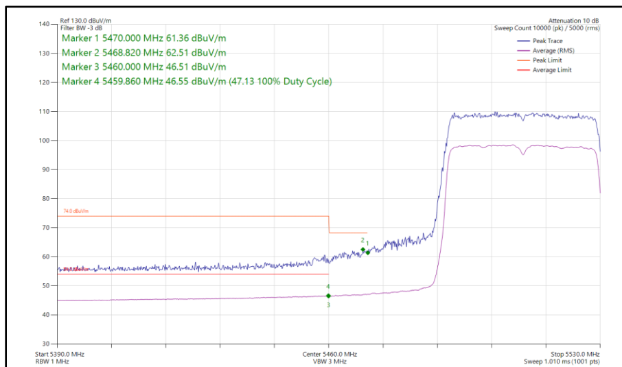
Figure 430 - 802.11ax HE40, SU, SISO, Core 0 - 5510 MHz Band Edge Frequency 5470 MHz
