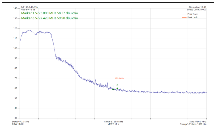
Figure 422 - 802.11ac VHT20, TxBF, Core 0 - Core 1 - 5680 MHz Band Edge Frequency 5725 MHz
