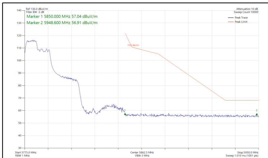
Figure 448 - 802.11ax HE40, RU 106-53, SISO, Core 0 - 5795 MHz Band Edge Frequency 5850 MHz
