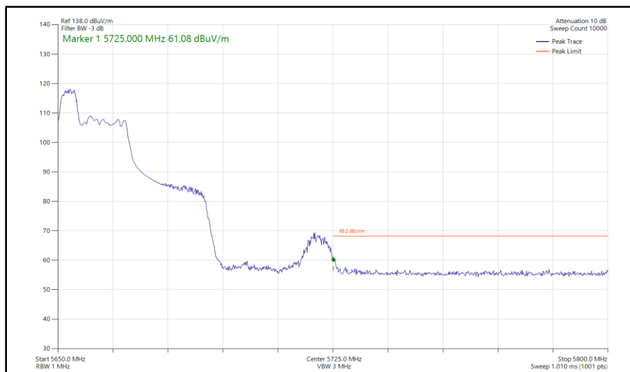
Figure 464 - 802.11ax HE40, RU 52-37, SISO, Core 1 - 5670 MHz Band Edge Frequency 5725 MHz
