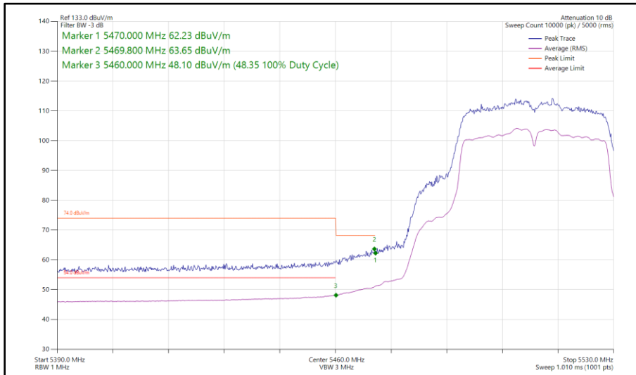
Figure 471 - 802.11n HT40, CDD, Core 0 - Core 1 - 5510 MHz Band Edge Frequency 5470 MHz
