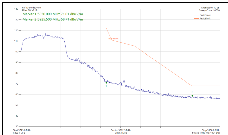
Figure 466 - 802.11n HT40, SISO, Core 1 - 5795 MHz Band Edge Frequency 5850 MHz
