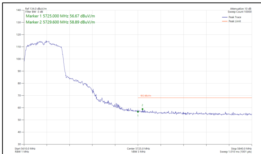
Figure 438 - 802.11n HT40, SISO, Core 0 - 5630 MHz Band Edge Frequency 5725 MHz
