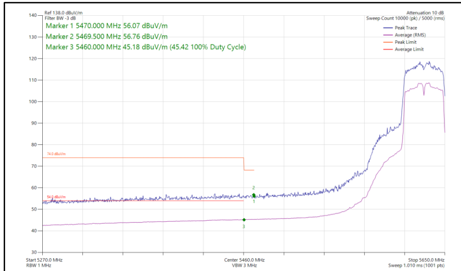
Figure 473 - 802.11n HT40, CDD, Core 0 - Core 1 - 5630 MHz Band Edge Frequency 5470 MHz
