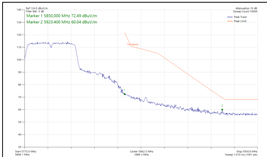
Figure 444 - 802.11n HT40, SISO, Core 0 - 5795 MHz Band Edge Frequency 5850 MHz
