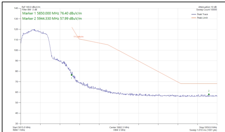
Figure 426 - 802.11ac VHT20, TxBF, Core 0 - Core 1 - 5825 MHz Band Edge Frequency 5850 MHz
