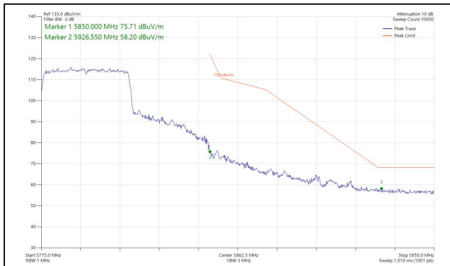
Figure 447 - 802.11ax HE40, SU, SISO, Core 0 - 5795 MHz Band Edge Frequency 5850 MHz
