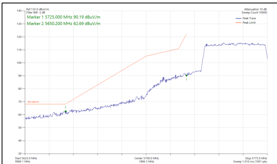
Figure 436 - 802.11ax HE40, SU, SISO, Core 0 - 5755 MHz Band Edge Frequency 5725 MHz
