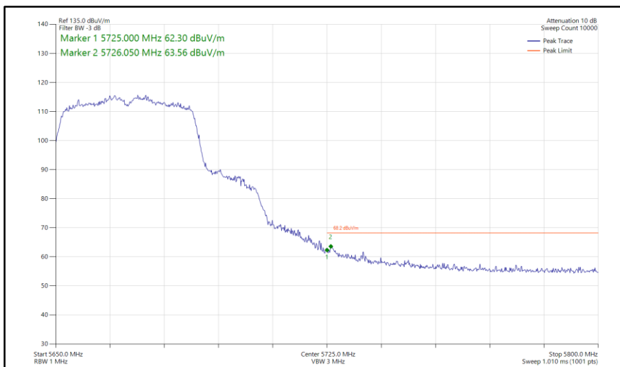
Figure 482 - 802.11n HT40, CDD, Core 0 - Core 1 - 5670 MHz Band Edge Frequency 5725 MHz
