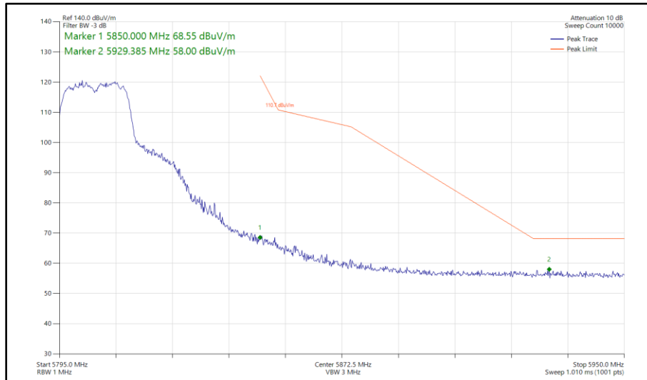
Figure 425 - 802.11ac VHT20, TxBF, Core 0 - Core 1 - 5805 MHz Band Edge Frequency 5850 MHz
