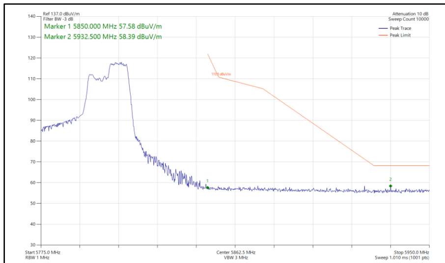
Figure 493 - 802.11ax HE40, RU 106-56, CDD, Core 0 - Core 1 - 5795 MHz Band Edge Frequency 5850 MHz
