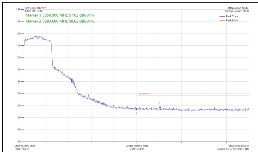
Figure 467 - 802.11ax HE40, SU, SISO, Core 1 - 5710 MHz Band Edge Frequency 5850 MHz
