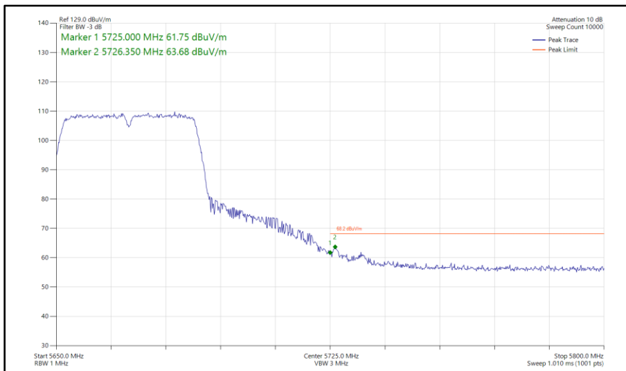
Figure 439 - 802.11n HT40, SISO, Core 0 - 5670 MHz Band Edge Frequency 5725 MHz
