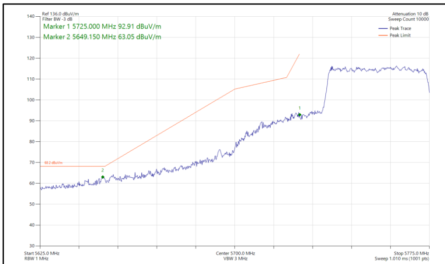
Figure 479 - 802.11ax HE40, SU, CDD, Core 0 - Core 1 - 5755 MHz Band Edge Frequency 5725 MHz
