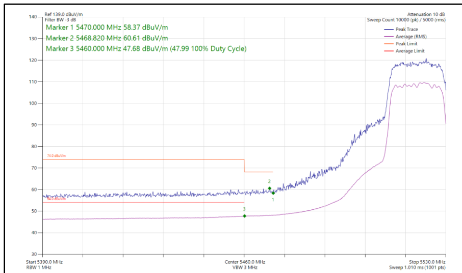
Figure 419 - 802.11ac VHT20, TxBF, Core 0 - Core 1 - 5520 MHz Band Edge Frequency 5470 MHz
