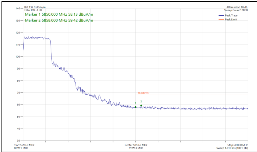
Figure 489 - 802.11ax HE40, SU, CDD, Core 0 - Core 1 - 5710 MHz Band Edge Frequency 5850 MHz
