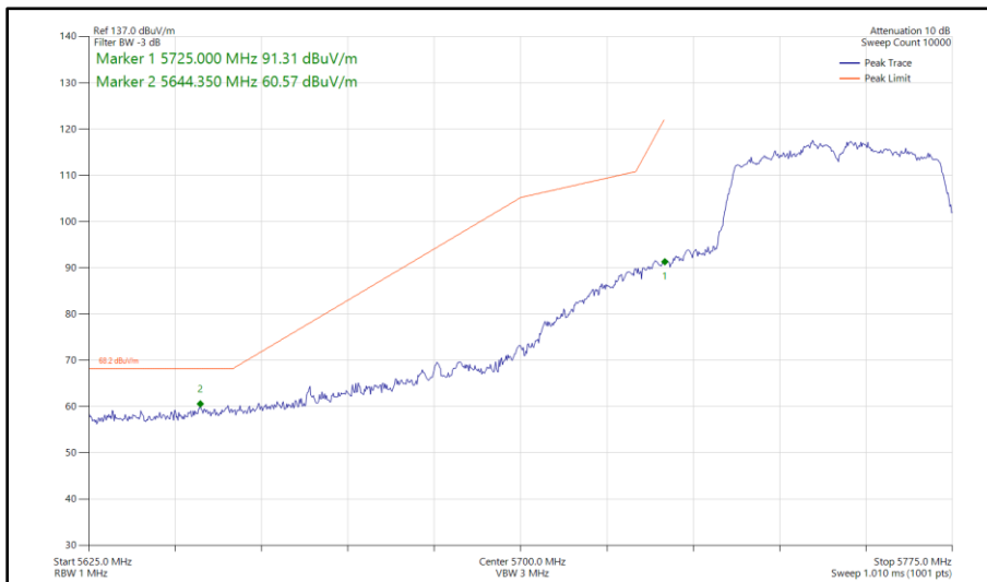
Figure 478 - 802.11n HT40, CDD, Core 0 - Core 1 - 5755 MHz Band Edge Frequency 5725 MHz
