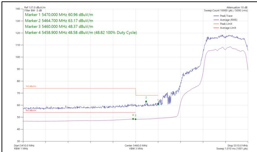
Figure 418 - 802.11ac VHT20, TxBF, Core 0 - Core 1 - 5500 MHz Band Edge Frequency 5470 MHz
