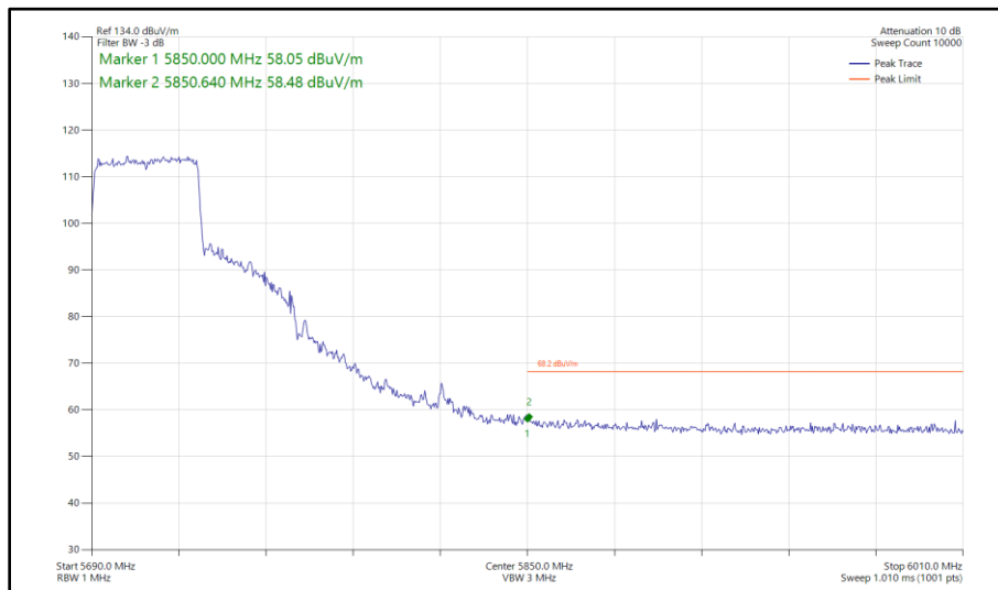
Figure 445 - 802.11ax HE40, SU, SISO, Core 0 - 5710 MHz Band Edge Frequency 5850 MHz
