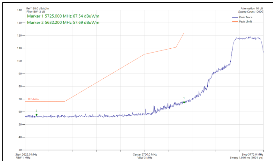
Figure 421 - 802.11ac VHT20, TxBF, Core 0 - Core 1 - 5765 MHz Band Edge Frequency 5725 MHz
