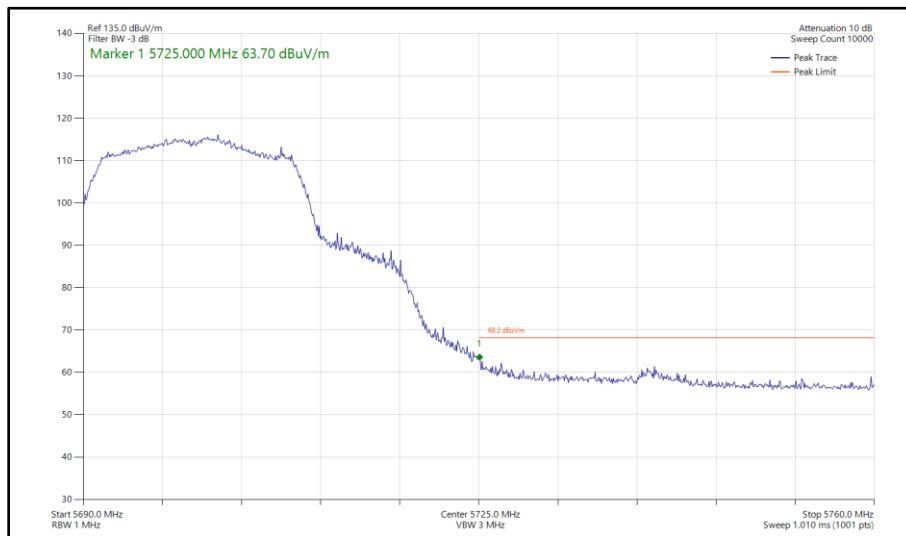
Figure 423 - 802.11ac VHT20, TxBF, Core 0 - Core 1 - 5700 MHz Band Edge Frequency 5725 MHz
