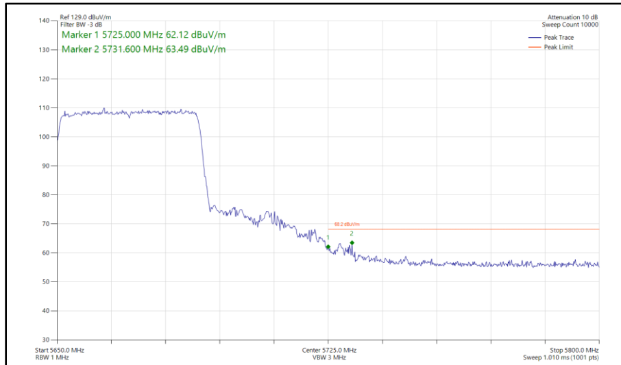
Figure 441 - 802.11ax HE40, SU, SISO, Core 0 - 5670 MHz Band Edge Frequency 5725 MHz
