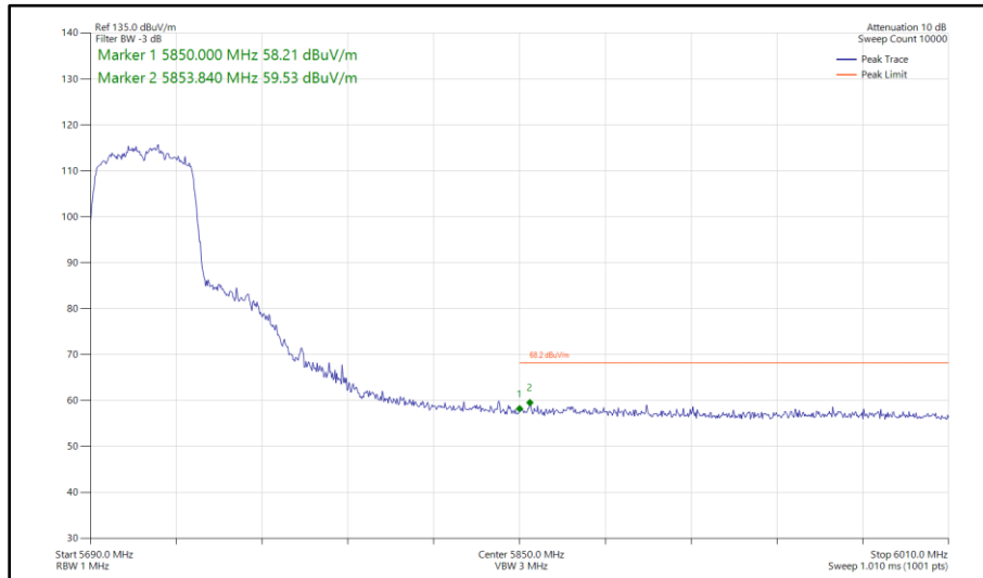
Figure 465 - 802.11n HT40, SISO, Core 1 - 5710 MHz Band Edge Frequency 5850 MHz
