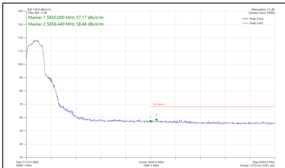
Figure 424 - 802.11ac VHT20, TxBF, Core 0 - Core 1 - 5720 MHz Band Edge Frequency 5850 MHz
