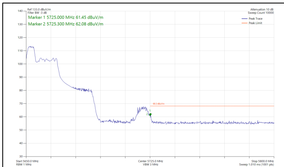
Figure 442 - 802.11ax HE40, RU 52-37, SISO, Core 0 - 5670 MHz Band Edge Frequency 5725 MHz
