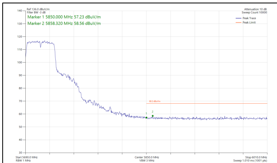
Figure 486 - 802.11n HT40, CDD, Core 0 - Core 1 - 5710 MHz Band Edge Frequency 5850 MHz
