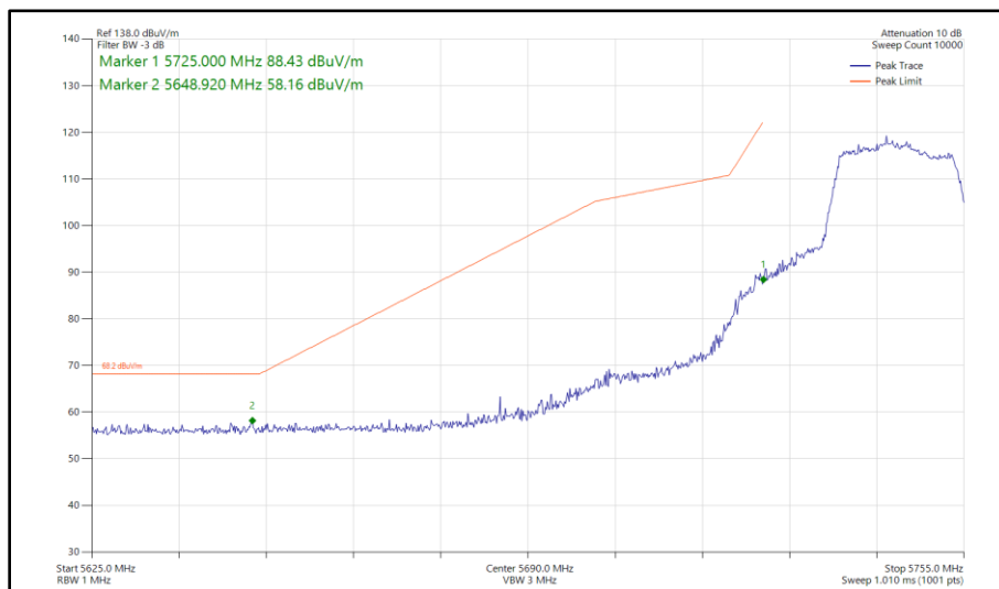
Figure 420 - 802.11ac VHT20, TxBF, Core 0 - Core 1 - 5745 MHz Band Edge Frequency 5725 MHz
