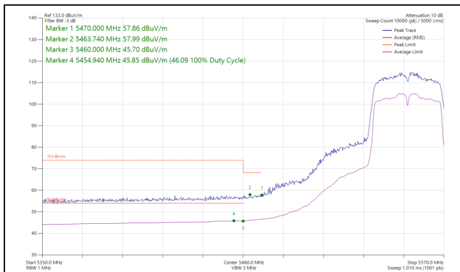
Figure 428 - 802.11n HT40, SISO, Core 0 - 5550 MHz Band Edge Frequency 5470 MHz
