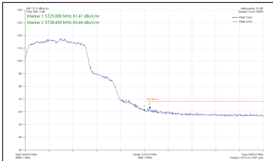
Figure 461 - 802.11n HT40, SISO, Core 1 - 5670 MHz Band Edge Frequency 5725 MHz
