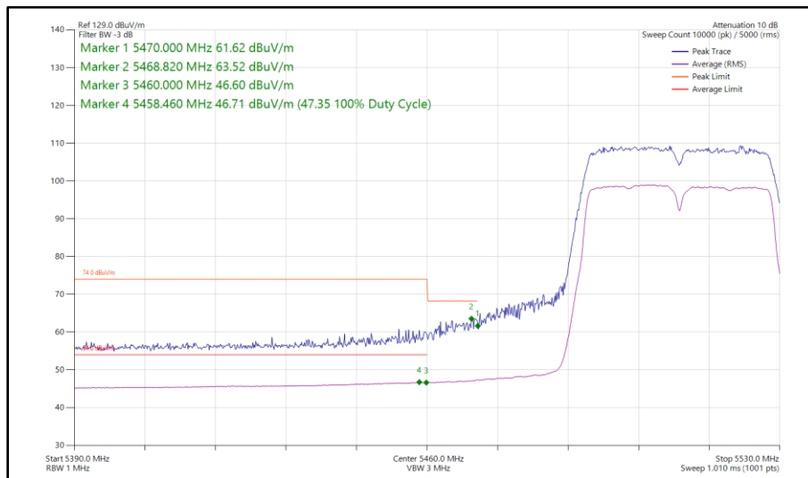
Figure 427 - 802.11n HT40, SISO, Core 0 - 5510 MHz Band Edge Frequency 5470 MHz
