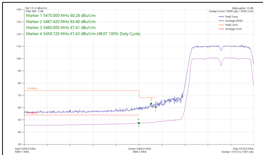
Figure 449 - 802.11n HT40, SISO, Core 1 - 5510 MHz Band Edge Frequency 5470 MHz
