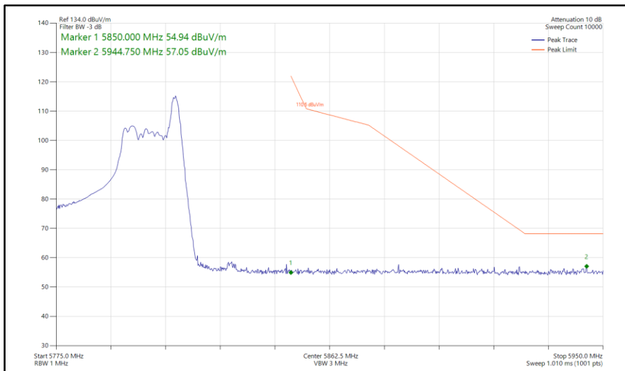
Figure 470 - 802.11ax HE40, RU 26-17, SISO, Core 1 - 5795 MHz Band Edge Frequency 5850 MHz
