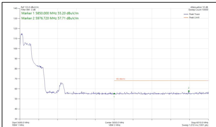
Figure 446 - 802.11ax HE40, RU 52-37, SISO, Core 0 - 5710 MHz Band Edge Frequency 5850 MHz
