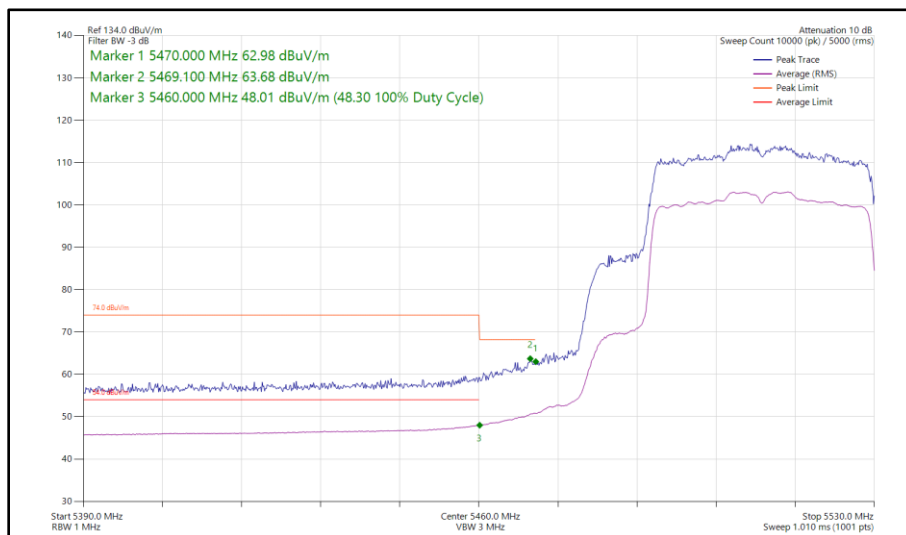
Figure 474 - 802.11ax HE40, SU, CDD, Core 0 - Core 1 - 5510 MHz Band Edge Frequency 5470 MHz
