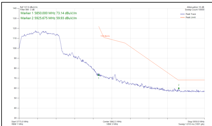
Figure 488 - 802.11n HT40, CDD, Core 0 - Core 1 - 5795 MHz Band Edge Frequency 5850 MHz
