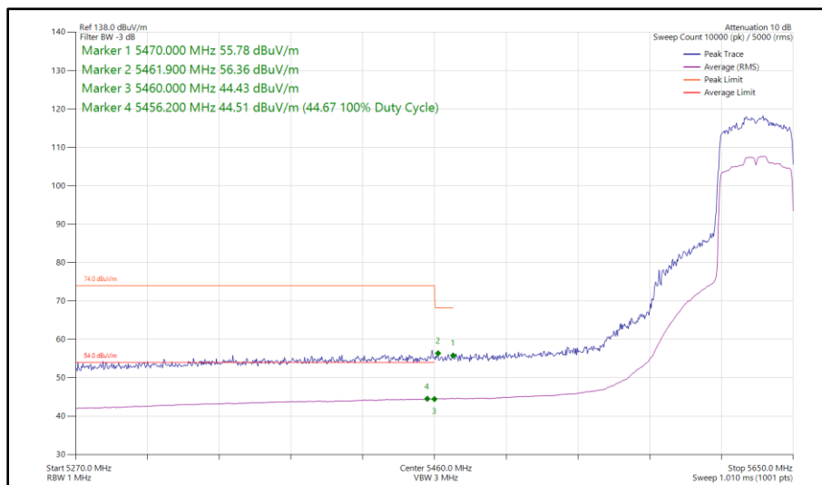
Figure 456 - 802.11ax HE40, SU, SISO, Core 1 - 5630 MHz Band Edge Frequency 5470 MHz
