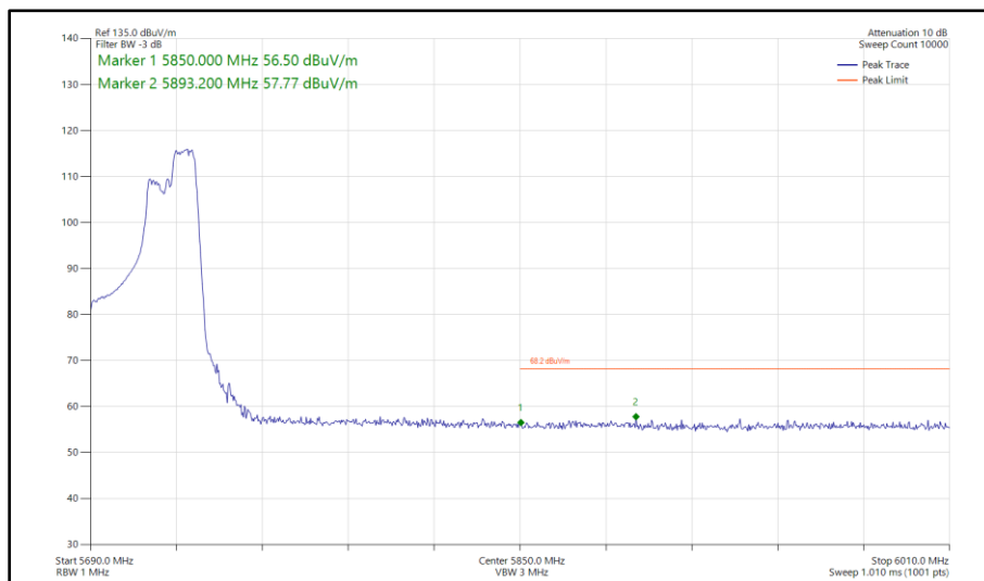
Figure 468 - 802.11ax HE40, RU 106-56, SISO, Core 1 - 5710 MHz Band Edge Frequency 5850 MHz
