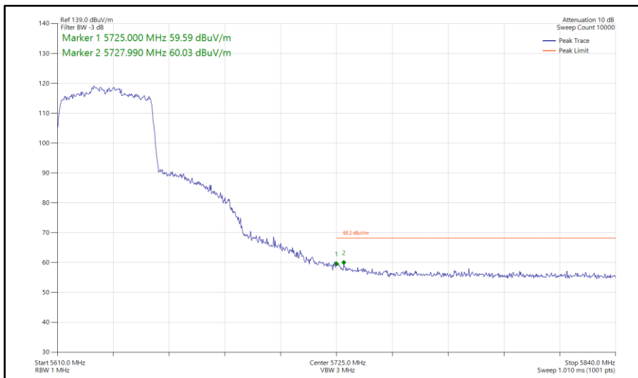
Figure 483 - 802.11ax HE40, SU, CDD, Core 0 - Core 1 - 5630 MHz Band Edge Frequency 5725 MHz
