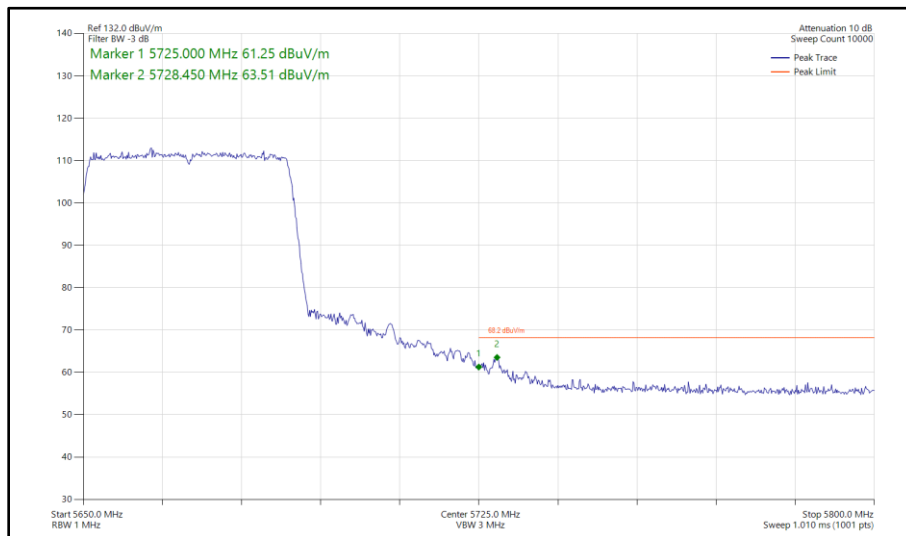
Figure 463 - 802.11ax HE40, SU, SISO, Core 1 - 5670 MHz Band Edge Frequency 5725 MHz
