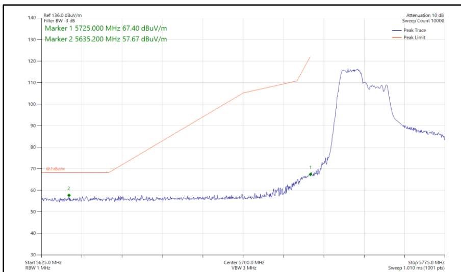
Figure 480 - 802.11ax HE40, RU 106-53, CDD, Core 0 - Core 1 - 5755 MHz Band Edge Frequency 5725 MHz
