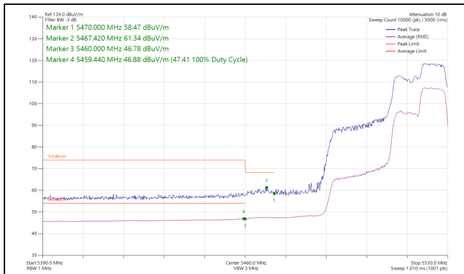
Figure 475 - 802.11ax HE40, RU 106-56, CDD, Core 0 - Core 1 - 5510 MHz Band Edge Frequency 5470 MHz
