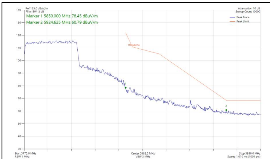
Figure 492 - 802.11ax HE40, SU, CDD, Core 0 - Core 1 - 5795 MHz Band Edge Frequency 5850 MHz
