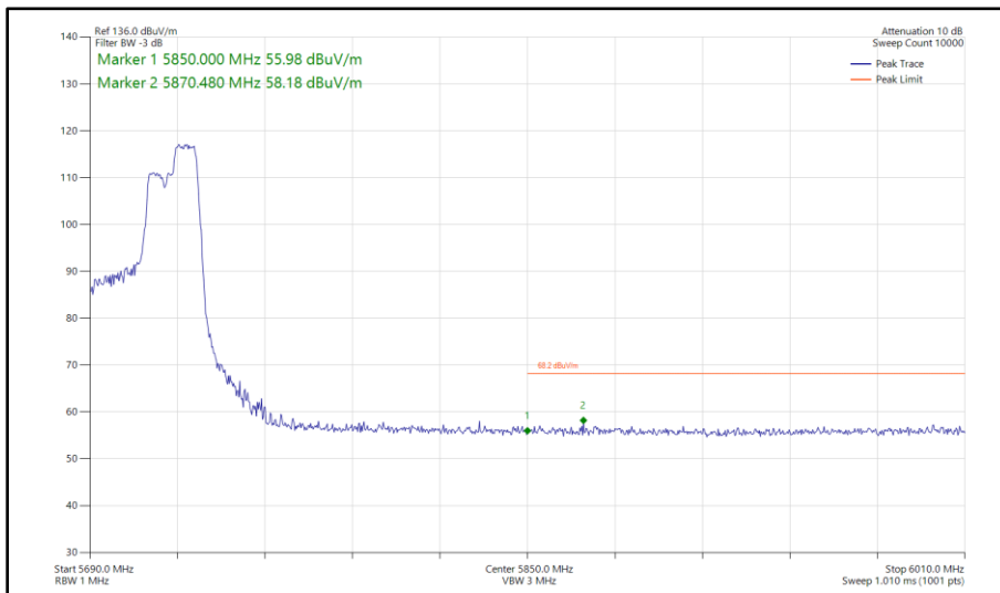
Figure 490 - 802.11ax HE40, RU 106-56, CDD, Core 0 - Core 1 - 5710 MHz Band Edge Frequency 5850 MHz
