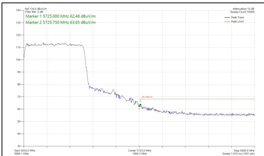
Figure 484 - 802.11ax HE40, SU, CDD, Core 0 - Core 1 - 5670 MHz Band Edge Frequency 5725 MHz
