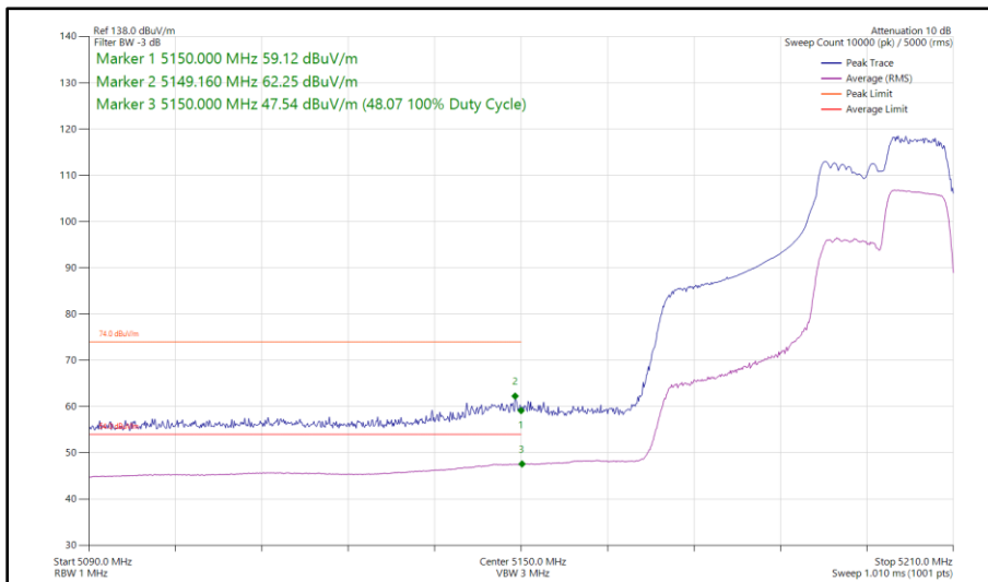
Figure 96 - 802.11ax HE40, RU 106-56, SISO, Core 1 - 5190 MHz Band Edge Frequency 5150 MHz
