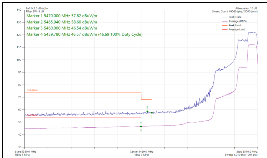
Figure 109 - 802.11ax HE40, RU 106-56, SISO, Core 1 - 5550 MHz Band Edge Frequency 5460 MHz
