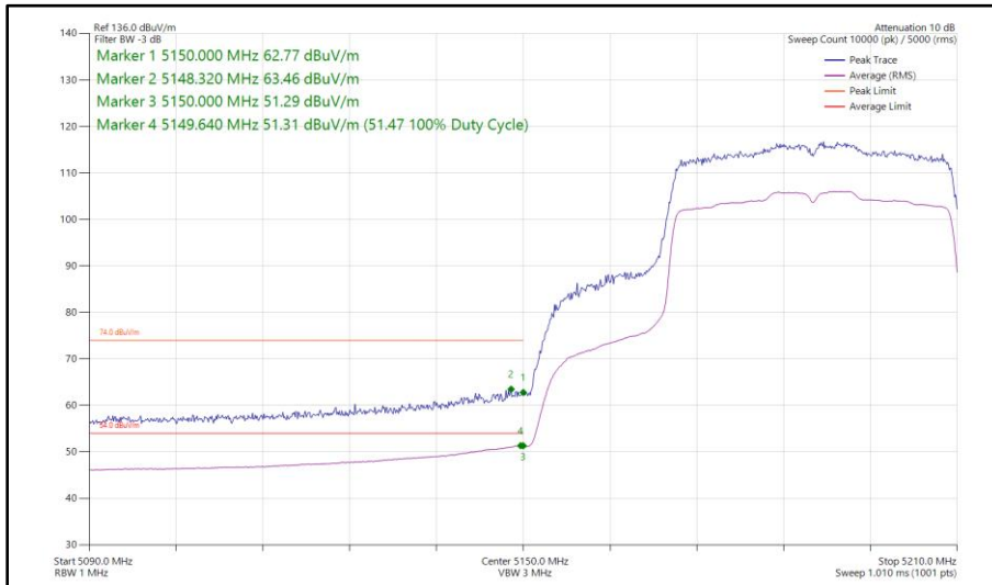
Figure 95 - 802.11ax HE40, SU, SISO, Core 1 - 5190 MHz Band Edge Frequency 5150 MHz
