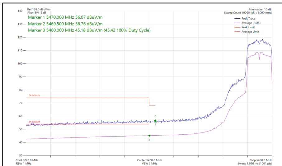
Figure 123 - 802.11n HT40, CDD, Core 0 - Core 1 - 5630 MHz Band Edge Frequency 5460 MHz
