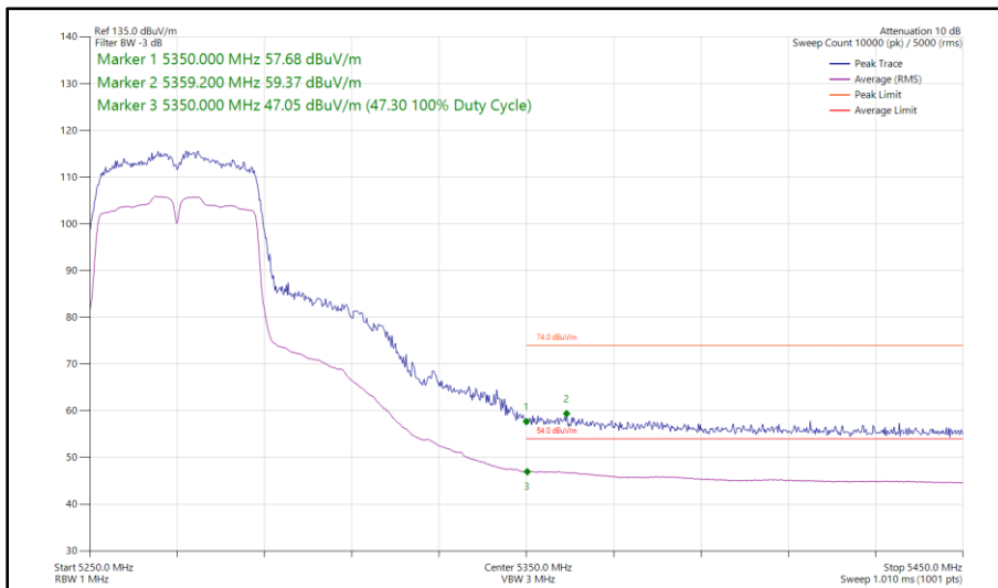
Figure 79 - 802.11n HT40, SISO, Core 0 - 5270 MHz Band Edge Frequency 5350 MHz
