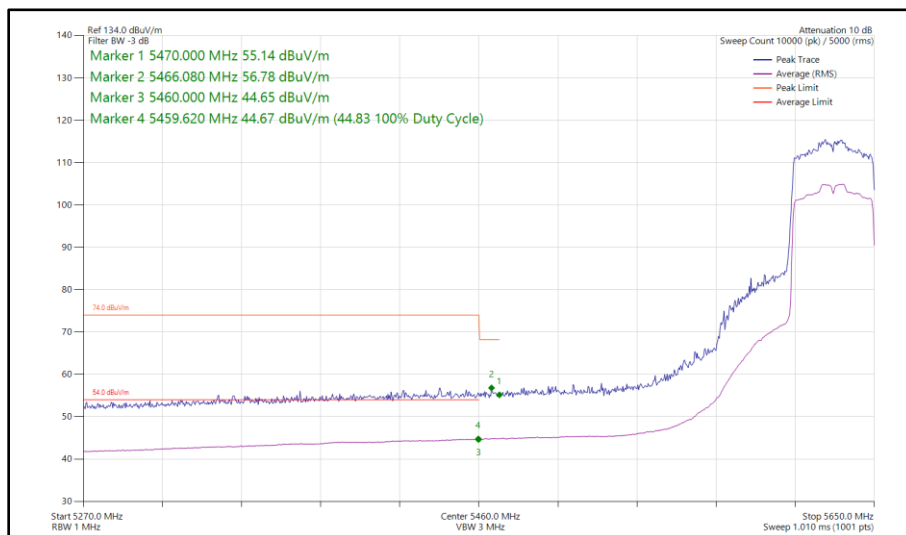
Figure 91 - 802.11ax HE40, SU, SISO, Core 0 - 5630 MHz Band Edge Frequency 5460 MHz
