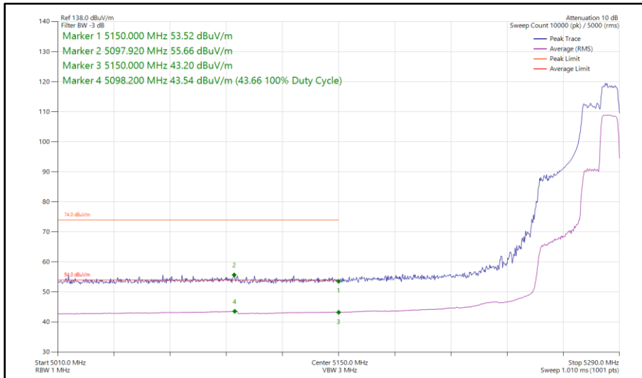
Figure 78 - 802.11ax HE40, RU 106-56, SISO, Core 0 - 5270 MHz Band Edge Frequency 5150 MHz
