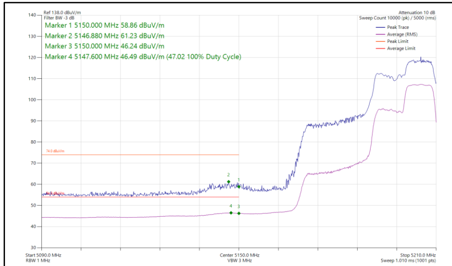
Figure 114 - 802.11ax HE40, RU 106-56, CDD, Core 0 - Core 1 - 5190 MHz Band Edge Frequency 5150 MHz
