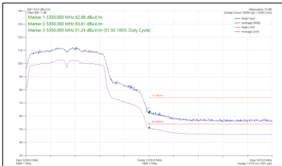
Figure 117 - 802.11n HT40, CDD, Core 0 - Core 1 - 5310 MHz Band Edge Frequency 5350 MHz
