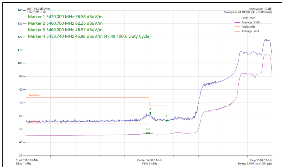
Figure 107 - 802.11ax HE40, RU 52-44, SISO, Core 1 - 5510 MHz Band Edge Frequency 5460 MHz
