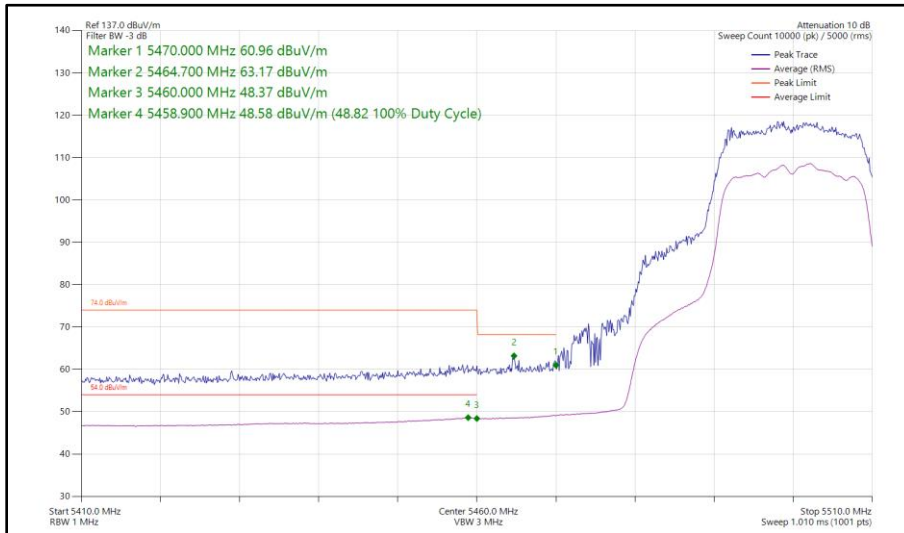
Figure 71 - 802.11ac VHT20, TxBF, Core 0 - Core 1 - 5500 MHz Band Edge Frequency 5460 MHz
