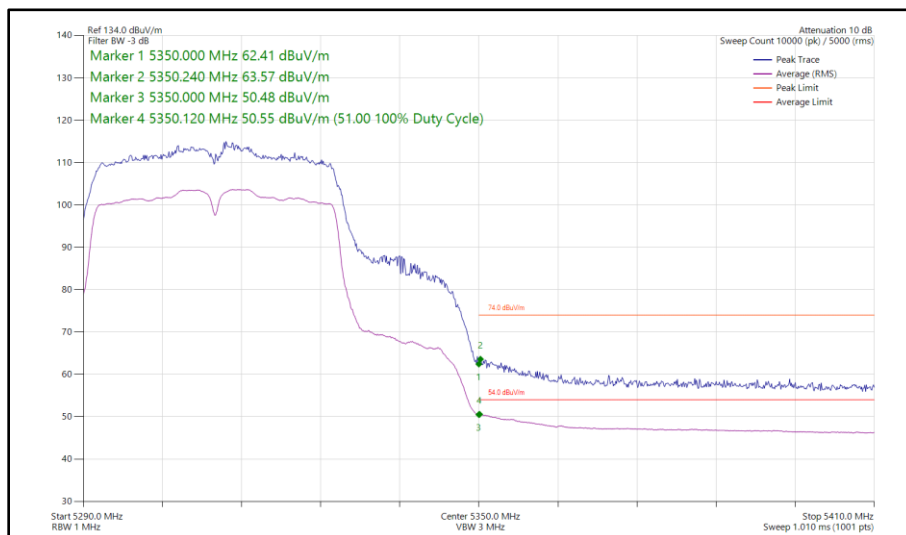
Figure 100 - 802.11n HT40, SISO, Core 1 - 5310 MHz Band Edge Frequency 5350 MHz
