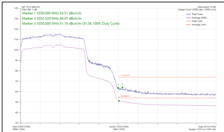
Figure 101 - 802.11ax HE40, SU, SISO, Core 1 - 5310 MHz Band Edge Frequency 5350 MHz
