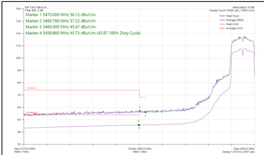
Figure 105 - 802.11n HT40, SISO, Core 1 - 5630 MHz Band Edge Frequency 5460 MHz
