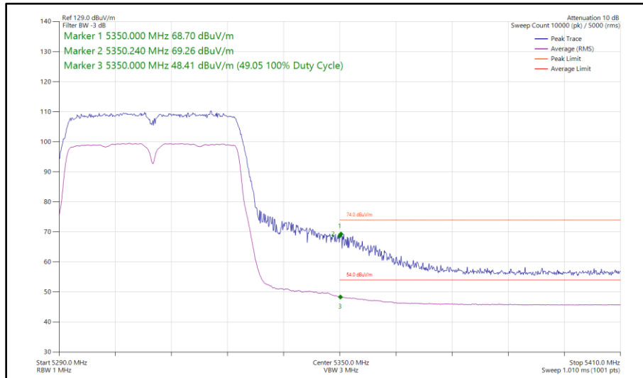
Figure 80 - 802.11n HT40, SISO, Core 0 - 5310 MHz Band Edge Frequency 5350 MHz
