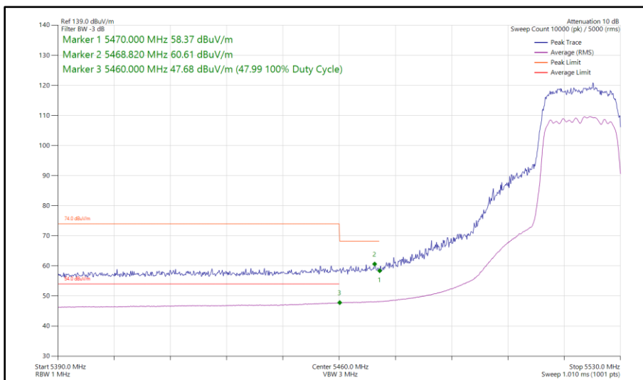
Figure 72 - 802.11ac VHT20, TxBF, Core 0 - Core 1 - 5520 MHz Band Edge Frequency 5460 MHz
