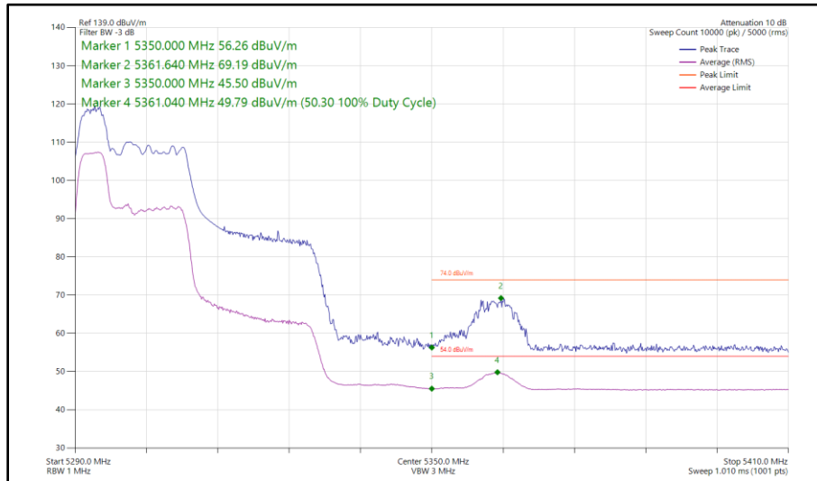
Figure 120 - 802.11ax HE40, RU 52-37, CDD, Core 0 - Core 1 - 5310 MHz Band Edge Frequency 5350 MHz
