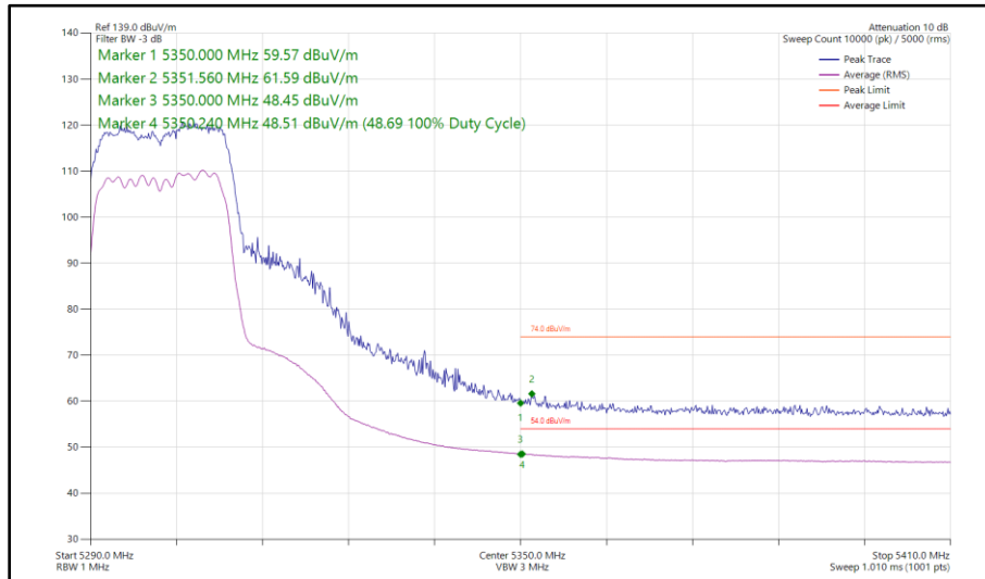
Figure 69 - 802.11ac VHT20, TxBF, Core 0 - Core 1 - 5300 MHz Band Edge Frequency 5350 MHz
