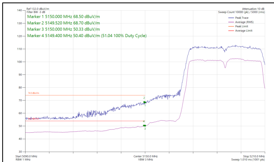
Figure 92 - 802.11n HT40, SISO, Core 1 - 5190 MHz Band Edge Frequency 5150 MHz
