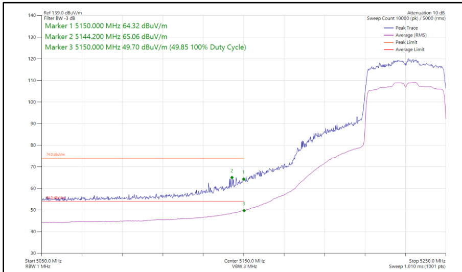
Figure 97 - 802.11ax HE40, SU, SISO, Core 1 - 5230 MHz Band Edge Frequency 5150 MHz
