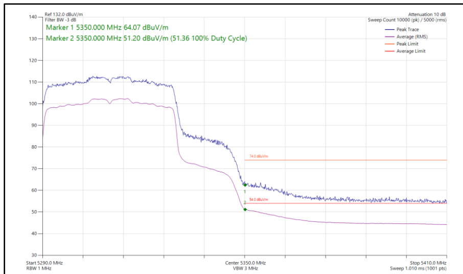
Figure 119 - 802.11ax HE40, SU, CDD, Core 0 - Core 1 - 5310 MHz Band Edge Frequency 5350 MHz
