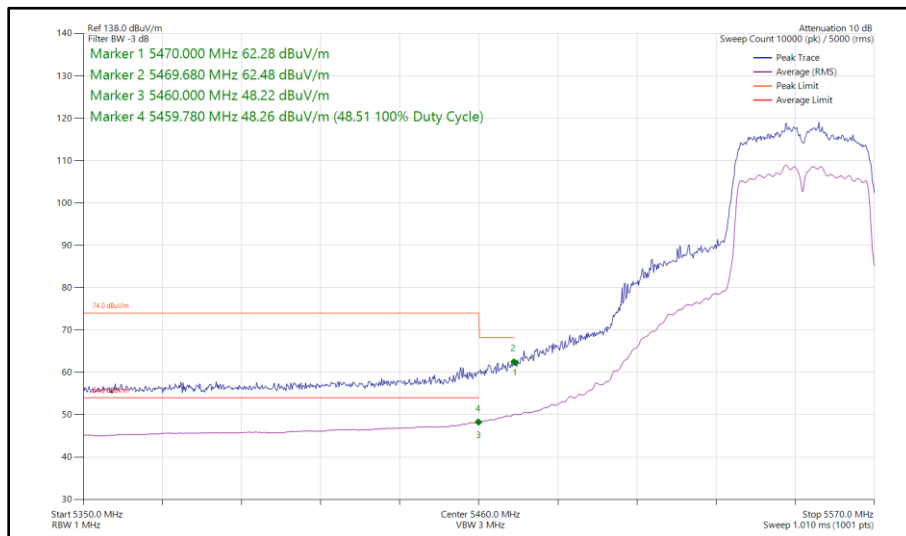
Figure 122 - 802.11n HT40, CDD, Core 0 - Core 1 - 5550 MHz Band Edge Frequency 5460 MHz
