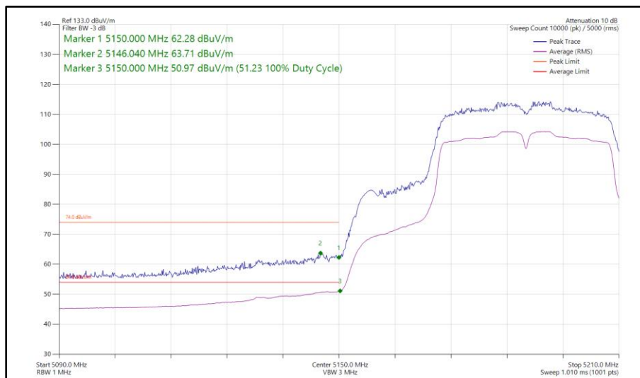
Figure 73 - 802.11n HT40, SISO, Core 0 - 5190 MHz Band Edge Frequency 5150 MHz
