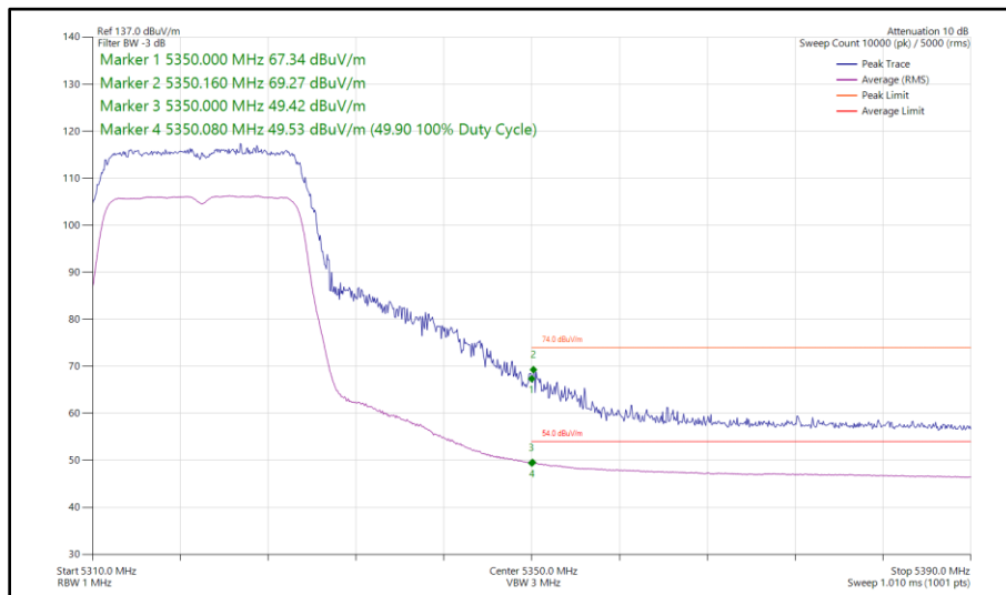
Figure 61 - 802.11n HT20, SDM, Core 0 - Core 1 - 5320 MHz Band Edge Frequency 5350 MHz
