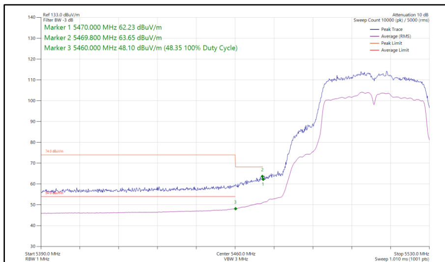
Figure 121 - 802.11n HT40, CDD, Core 0 - Core 1 - 5510 MHz Band Edge Frequency 5460 MHz
