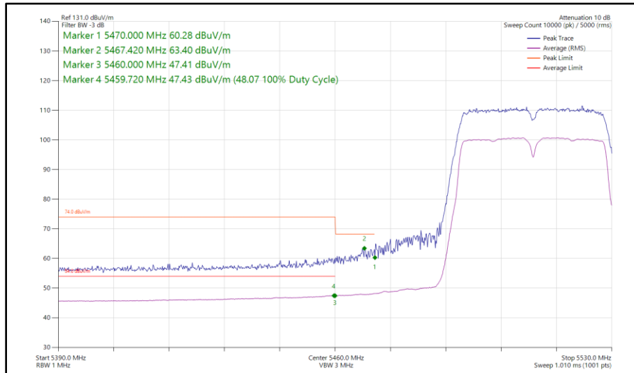
Figure 103 - 802.11n HT40, SISO, Core 1 - 5510 MHz Band Edge Frequency 5460 MHz
