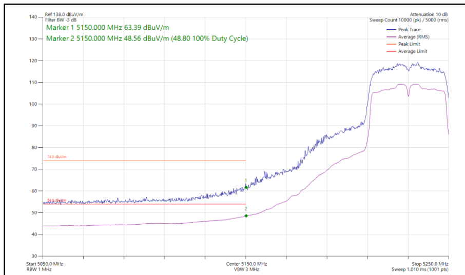
Figure 93 - 802.11n HT40, SISO, Core 1 - 5230 MHz Band Edge Frequency 5150 MHz
