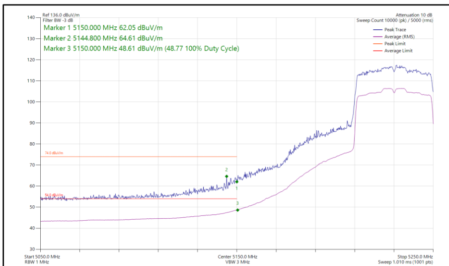
Figure 77 - 802.11ax HE40, SU, SISO, Core 0 - 5230 MHz Band Edge Frequency 5150 MHz
