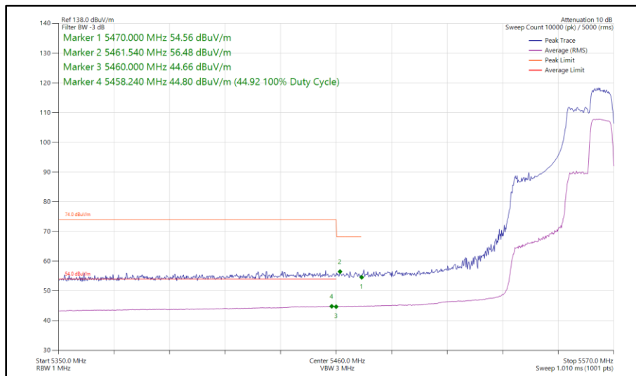
Figure 90 - 802.11ax HE40, RU 106-56, SISO, Core 0 - 5550 MHz Band Edge Frequency 5460 MHz
