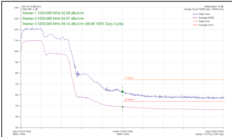
Figure 63 - 802.11ax HE20, RU 106-53, SDM, Core 0 - Core 1 - 5320 MHz Band Edge Frequency 5350 MHz
