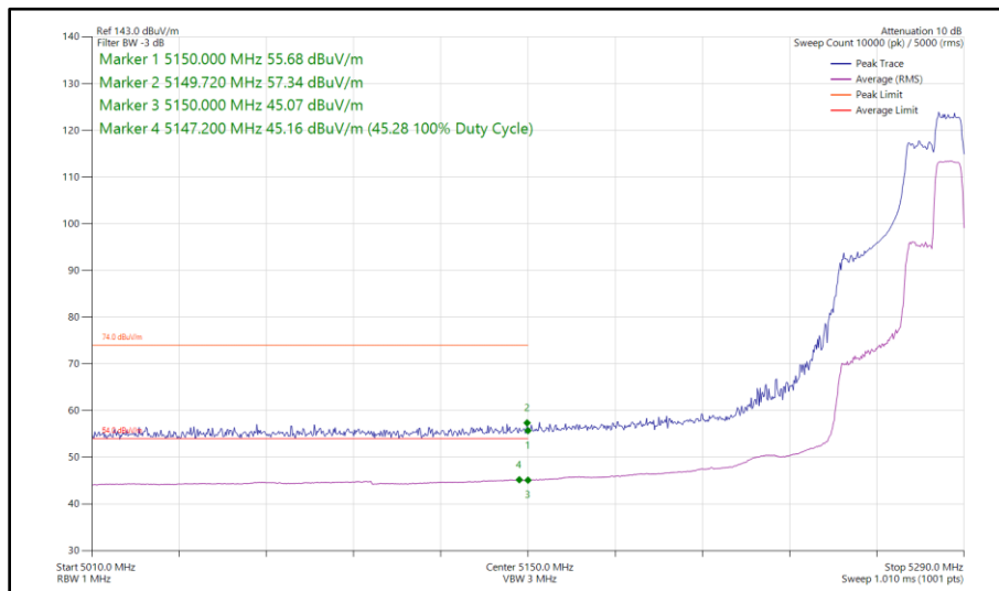
Figure 99 - 802.11ax HE40, RU 106-56, SISO, Core 1 - 5270 MHz Band Edge Frequency 5150 MHz
