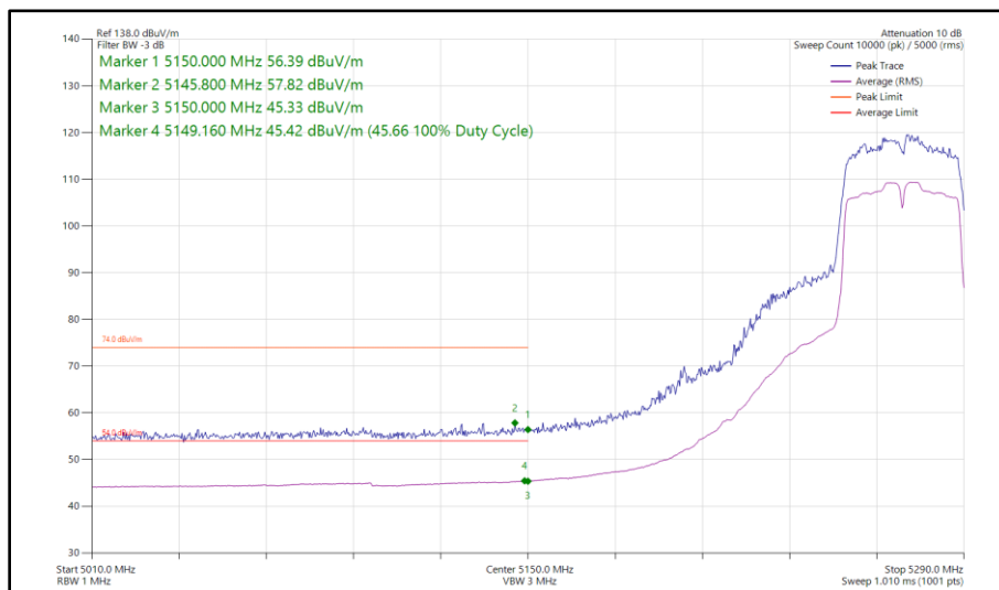
Figure 94 - 802.11n HT40, SISO, Core 1 - 5270 MHz Band Edge Frequency 5150 MHz
