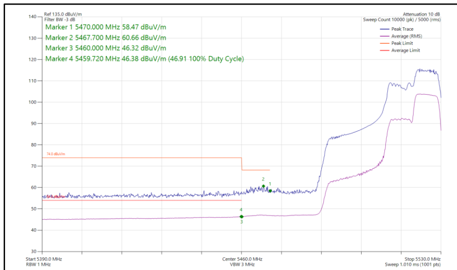
Figure 88 - 802.11ax HE40, RU 106-56, SISO, Core 0 - 5510 MHz Band Edge Frequency 5460 MHz
