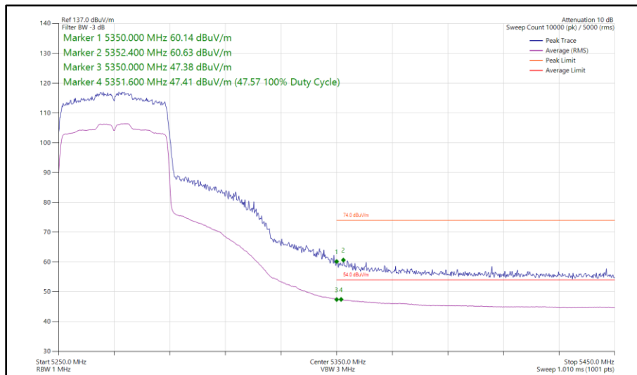
Figure 81 - 802.11ax HE40, SU, SISO, Core 0 - 5270 MHz Band Edge Frequency 5350 MHz
