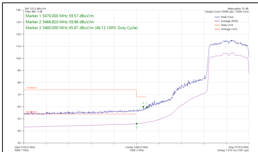
Figure 89 - 802.11ax HE40, SU, SISO, Core 0 - 5550 MHz Band Edge Frequency 5460 MHz
