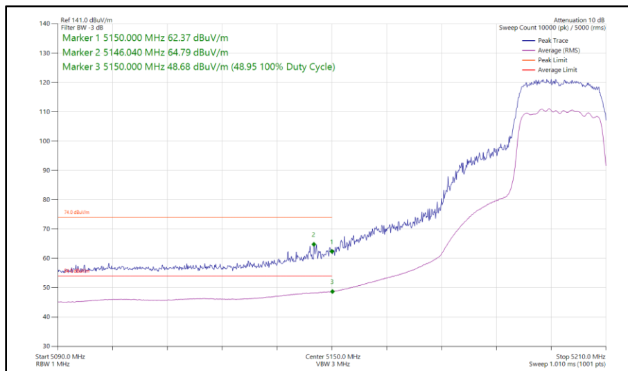
Figure 68 - 802.11ac VHT20, TxBF, Core 0 - Core 1 - 5200 MHz Band Edge Frequency 5150 MHz
