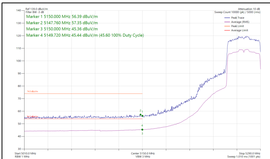
Figure 98 - 802.11ax HE40, SU, SISO, Core 1 - 5270 MHz Band Edge Frequency 5150 MHz
