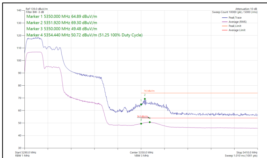
Figure 102 - 802.11ax HE40, RU 106-53, SISO, Core 1 - 5310 MHz Band Edge Frequency 5350 MHz
