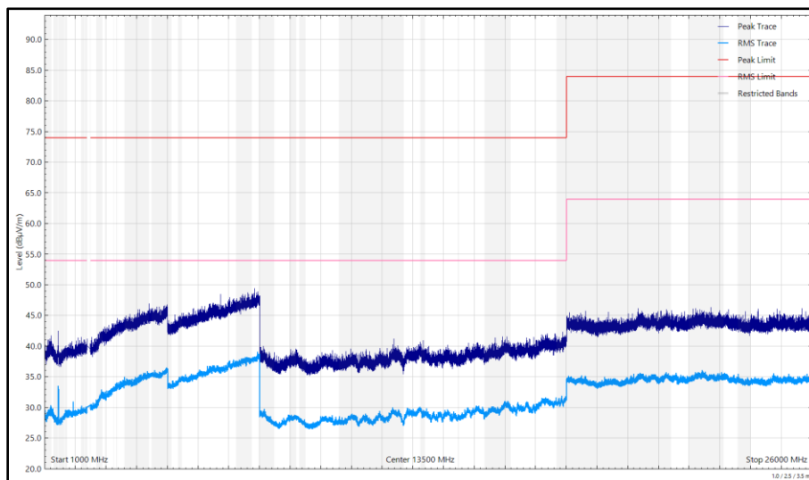
Figure 274 - 2402 MHz (CH0), DH5, iPA, Core 2, 1 GHz to 26 GHz, Vertical
