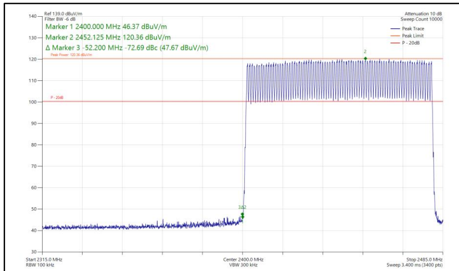
Figure 253 - Bluetooth DH5, MIMO, Core 0 - Core 1 - Hopping Band Edge Frequency 2400 MHz
