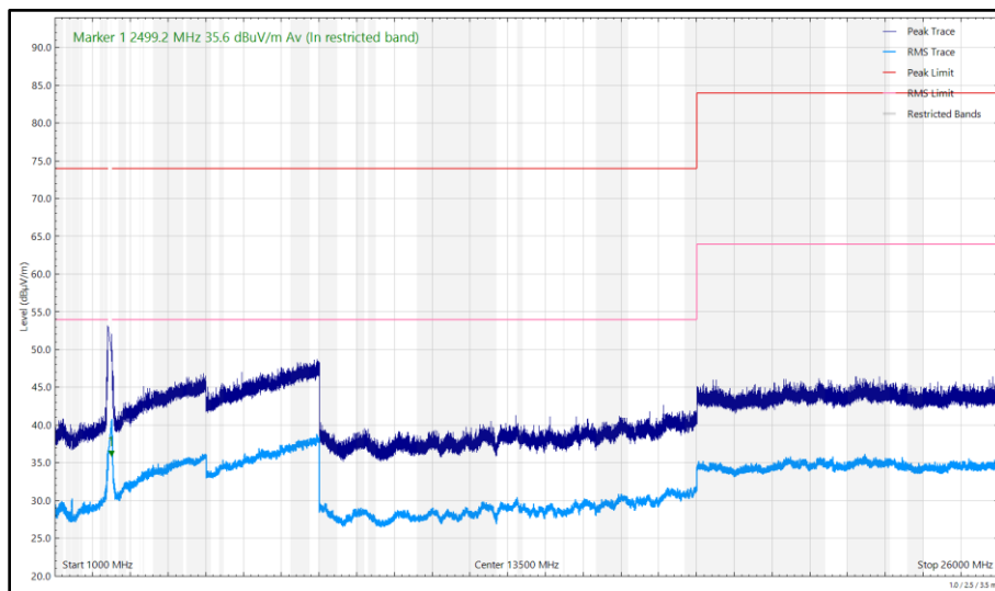
Figure 263 - 2480 MHz (CH78), DH5, ePA, Core 0 + Core 1, 1 GHz to 26 GHz, Horizontal
