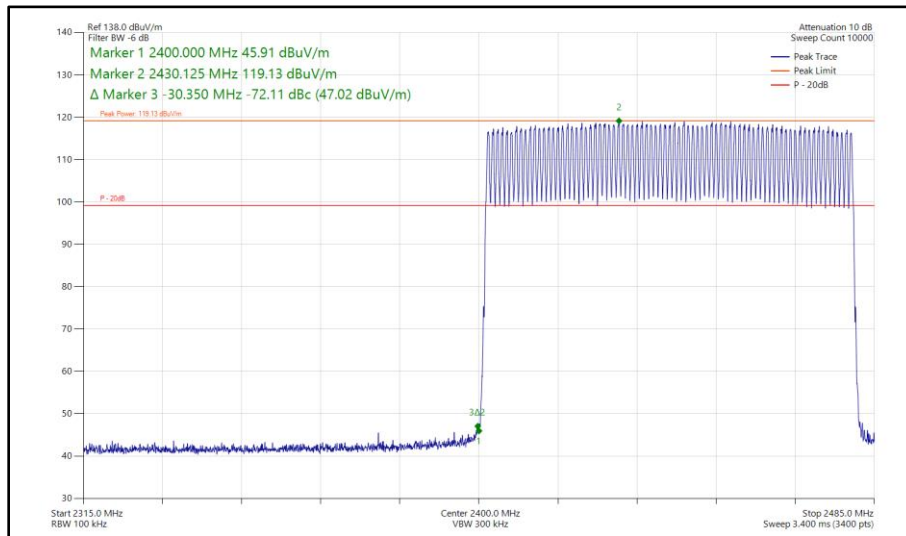
Figure 247 - Bluetooth DH5, SISO, Core 1 - Hopping Band Edge Frequency 2400 MHz
