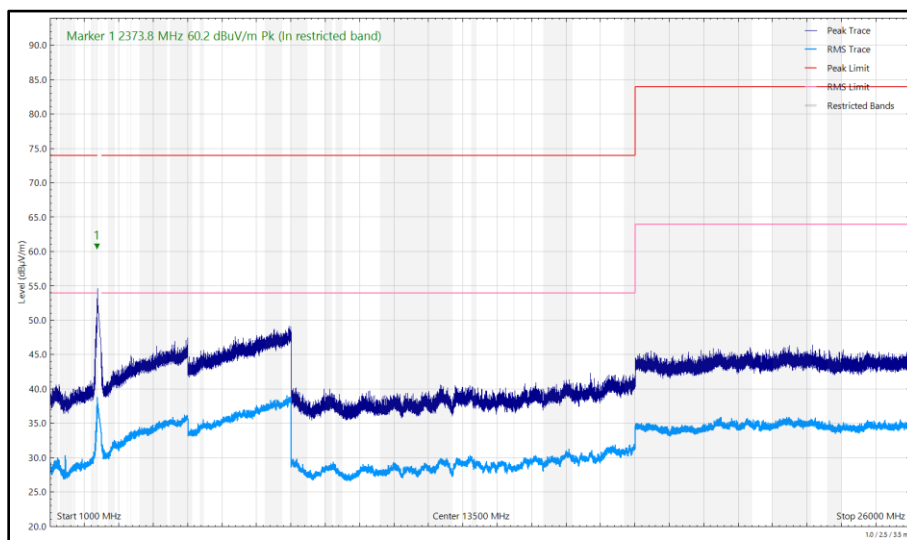
Figure 257 - 2402 MHz (CH0), DH5, ePA, Core 0 + Core 1, 1 GHz to 26 GHz, Horizontal
