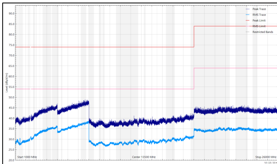
Figure 268 - 2441 MHz (CH39), DH5, iPA, Core 0 + Core 1, 1 GHz to 26 GHz, Horizontal
