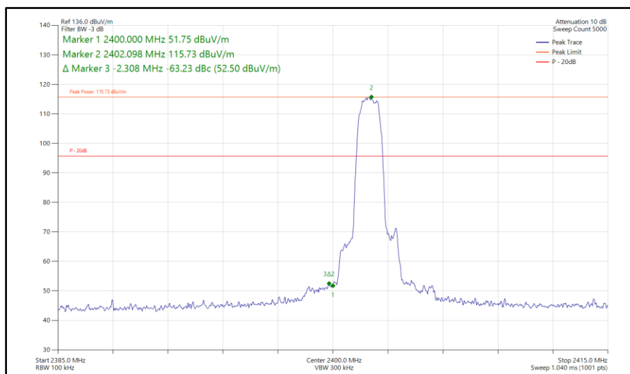
Figure 246 - Bluetooth 3-DH5, SISO, Core 1 - 2402 MHz Band Edge Frequency 2400 MHz
