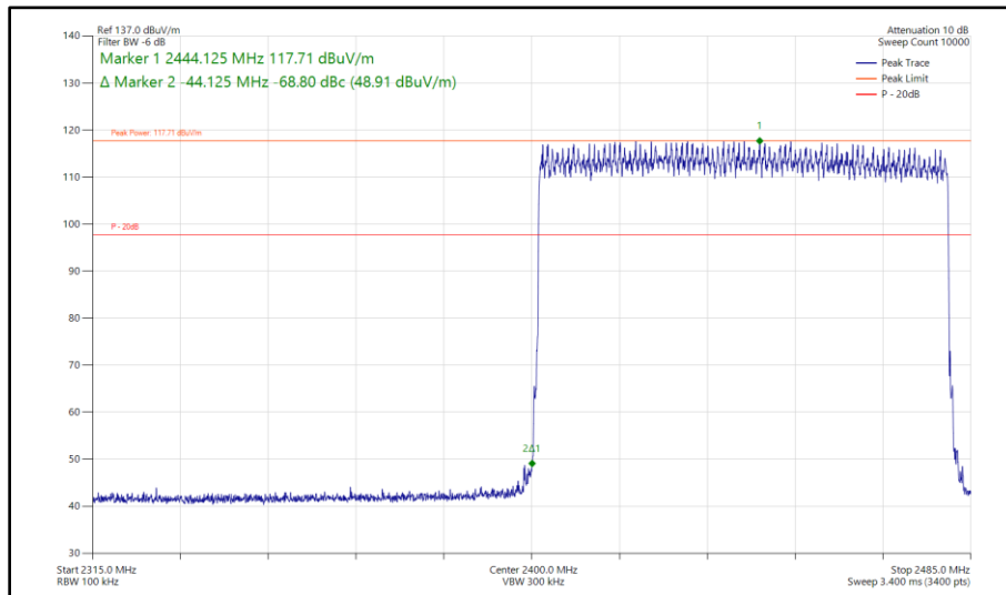
Figure 249 - Bluetooth 3-DH5, SISO, Core 1 - Hopping Band Edge Frequency 2400 MHz
