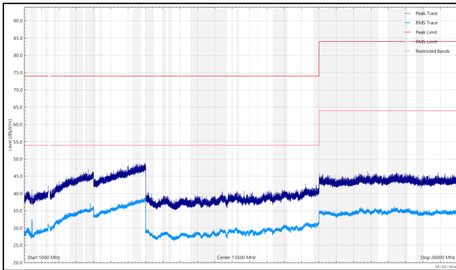
Figure 266 - 2402 MHz (CH0), DH5, iPA, Core 0 + Core 1, 1 GHz to 26 GHz, Vertical
