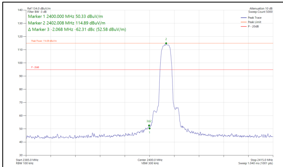
Figure 251 - Bluetooth 2-DH5, MIMO, Core 0 - Core 1 - 2402 MHz Band Edge Frequency 2400 MHz
