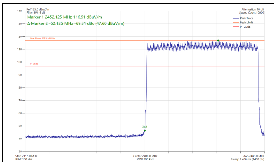
Figure 248 - Bluetooth 2-DH5, SISO, Core 1 - Hopping Band Edge Frequency 2400 MHz
