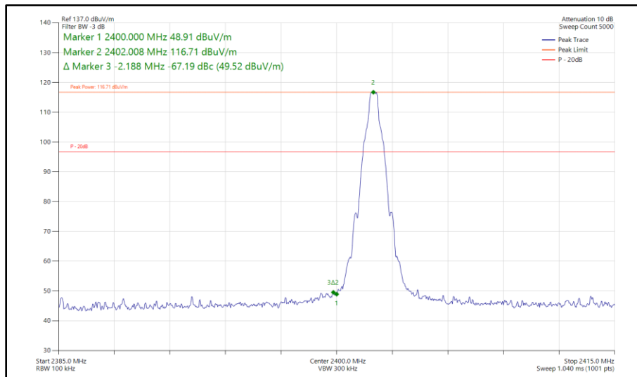
Figure 244 - Bluetooth DH5, SISO, Core 1 - 2402 MHz Band Edge Frequency 2400 MHz
