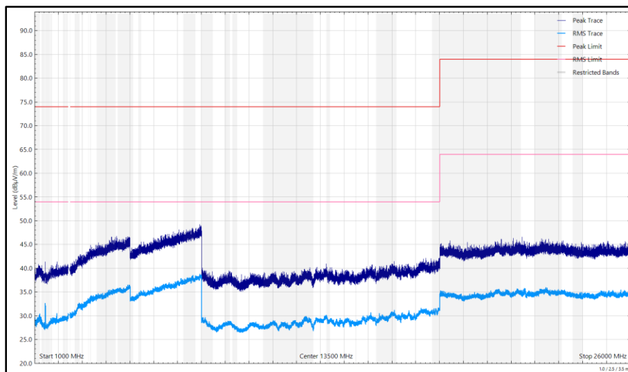
Figure 278 - 2441 MHz (CH39), DH5, iPA, Core 2, 1 GHz to 26 GHz, Vertical
