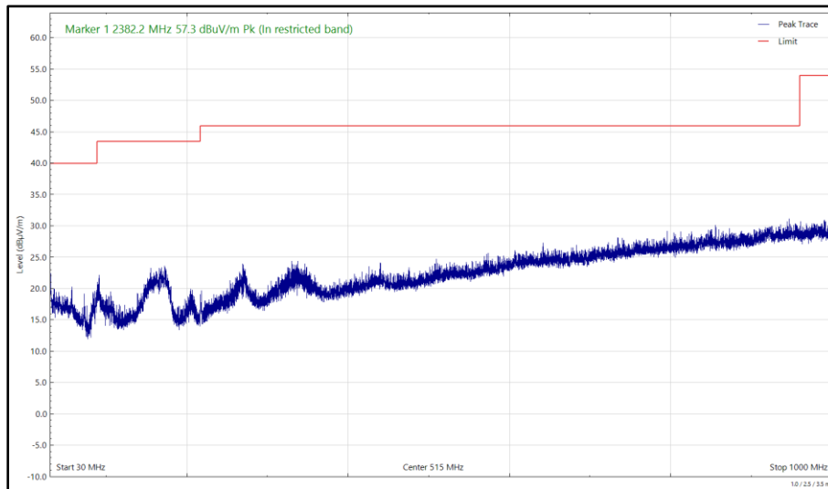
Figure 261 - 2441 MHz (CH39), DH5, ePA, Core 0 + Core 1, 30 MHz to 1 GHz, Vertical (Peak)
