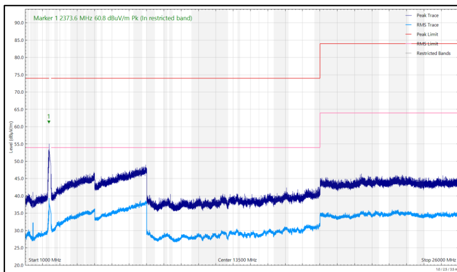
Figure 258 - 2402 MHz (CH0), DH5, ePA, Core 0 + Core 1, 1 GHz to 26 GHz, Vertical
