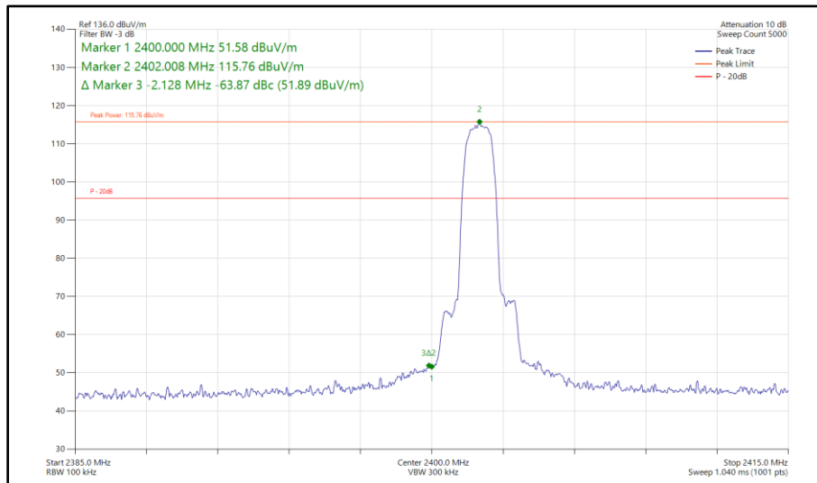
Figure 245 - Bluetooth 2-DH5, SISO, Core 1 - 2402 MHz Band Edge Frequency 2400 MHz
