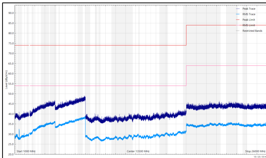
Figure 280 - 2480 MHz (CH78), DH5, iPA, Core 2, 1 GHz to 26 GHz, Vertical
