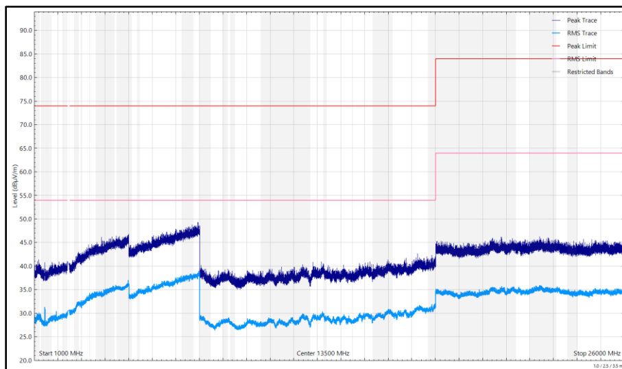
Figure 276 - 2441 MHz (CH39), DH5, iPA, Core 2, 1 GHz to 26 GHz, Horizontal
