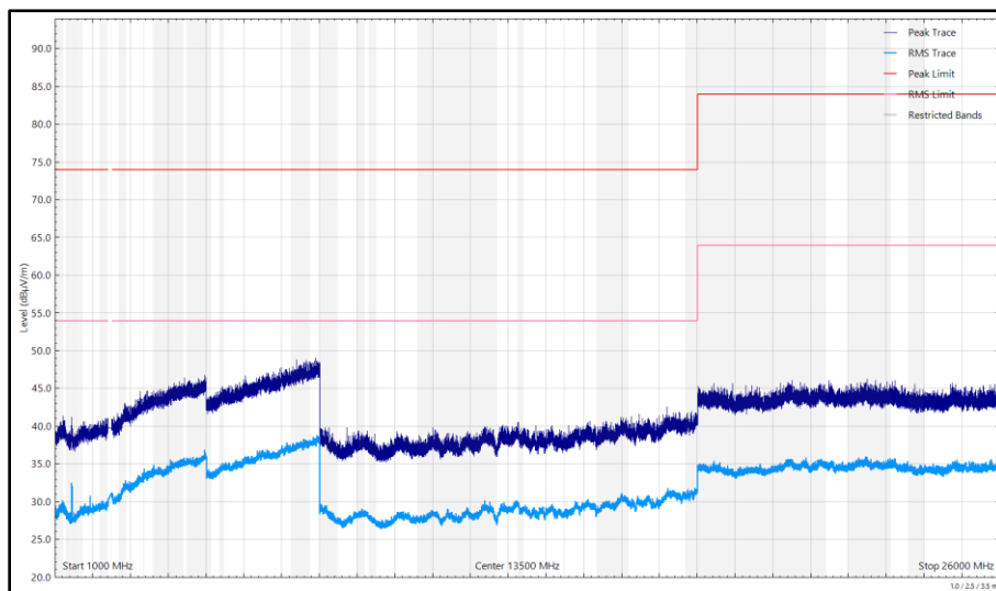
Figure 272 - 2480 MHz (CH78), DH5, iPA, Core 0 + Core 1, 1 GHz to 26 GHz, Vertical
