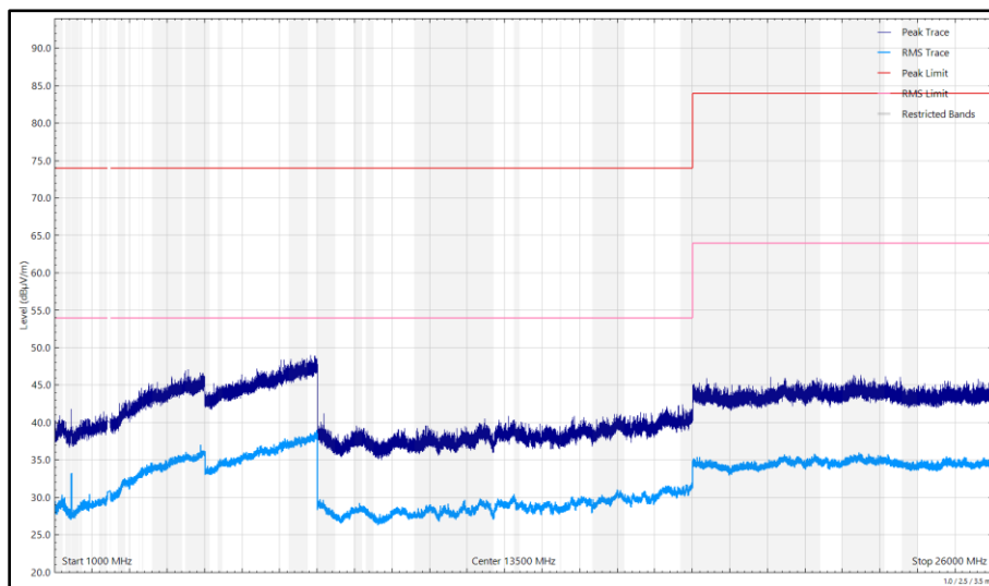
Figure 270 - 2441 MHz (CH39), DH5, iPA, Core 0 + Core 1, 1 GHz to 26 GHz, Vertical
