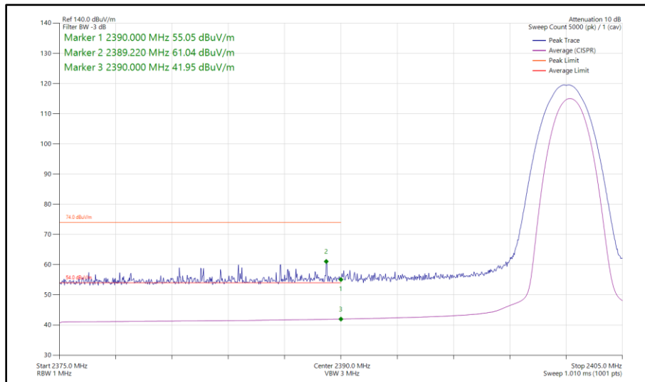
Figure 32 - Bluetooth 2-DH5, SISO, Core 1 - 2402 MHz Band Edge Frequency 2390 MHz
