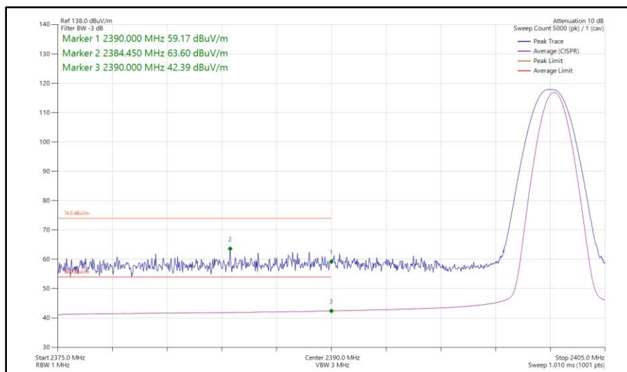
Figure 31 - Bluetooth DH5, SISO, Core 1 - 2402 MHz Band Edge Frequency 2390 MHz
