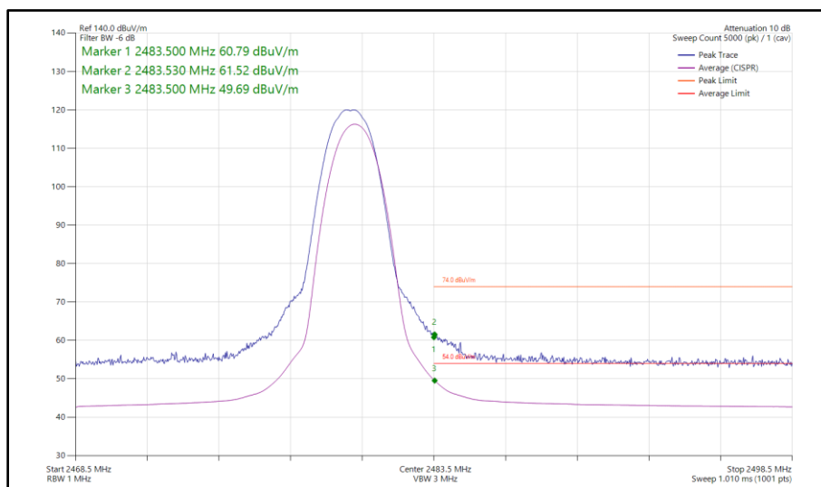
Figure 29 - Bluetooth 2-DH5, SISO, Core 0 - 2480 MHz Band Edge Frequency 2483.5 MHz
