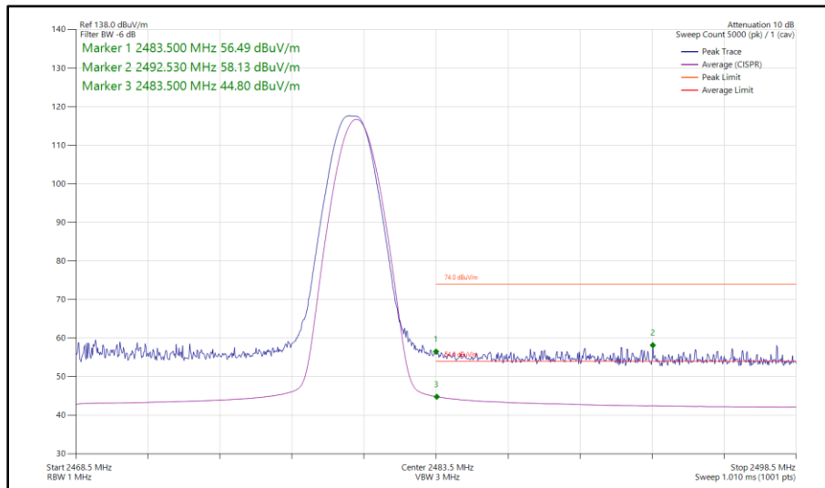
Figure 34 - Bluetooth DH5, SISO, Core 1 - 2480 MHz Band Edge Frequency 2483.5 MHz
