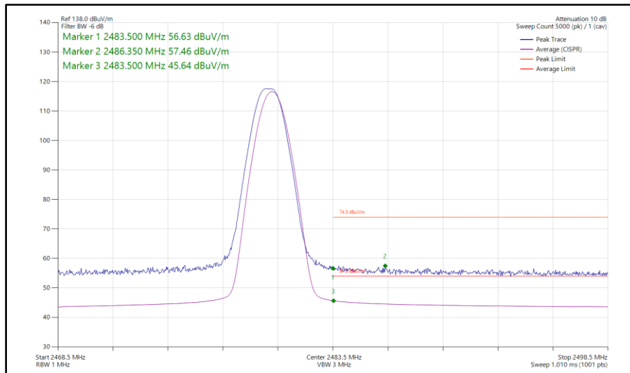
Figure 40 - Bluetooth DH5, MIMO, Core 0 - Core 1 - 2480 MHz Band Edge Frequency 2483.5 MHz
