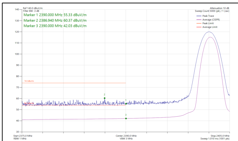
Figure 33 - Bluetooth 3-DH5, SISO, Core 1 - 2402 MHz Band Edge Frequency 2390 MHz
