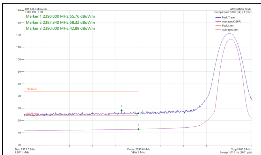
Figure 27 - Bluetooth 3-DH5, SISO, Core 0 - 2402 MHz Band Edge Frequency 2390 MHz
