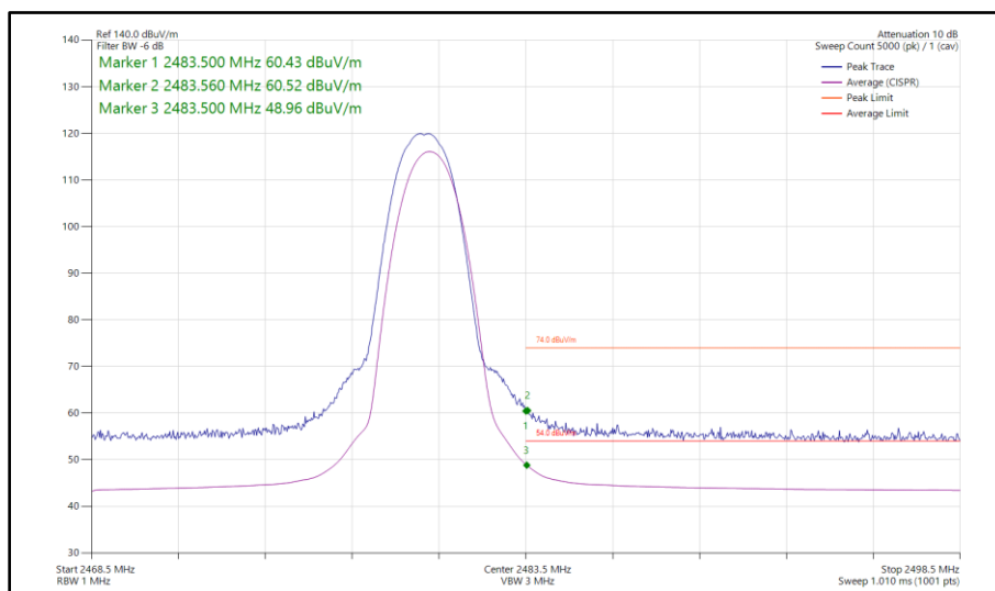
Figure 41 - Bluetooth 2-DH5, MIMO, Core 0 - Core 1 - 2480 MHz Band Edge Frequency 2483.5 MHz
