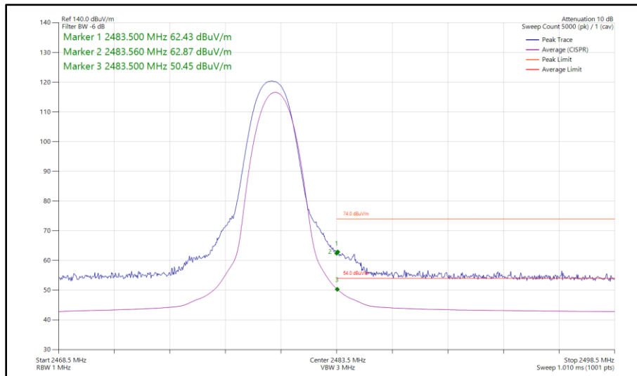
Figure 30 - Bluetooth 3-DH5, SISO, Core 0 - 2480 MHz Band Edge Frequency 2483.5 MHz
