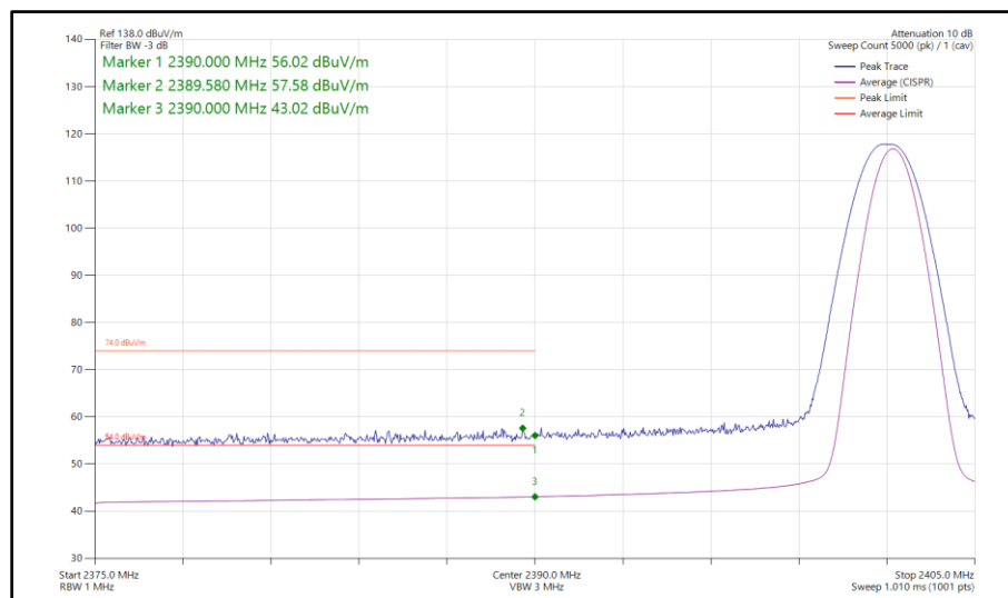
Figure 25 - Bluetooth DH5, SISO, Core 0 - 2402 MHz Band Edge Frequency 2390 MHz
