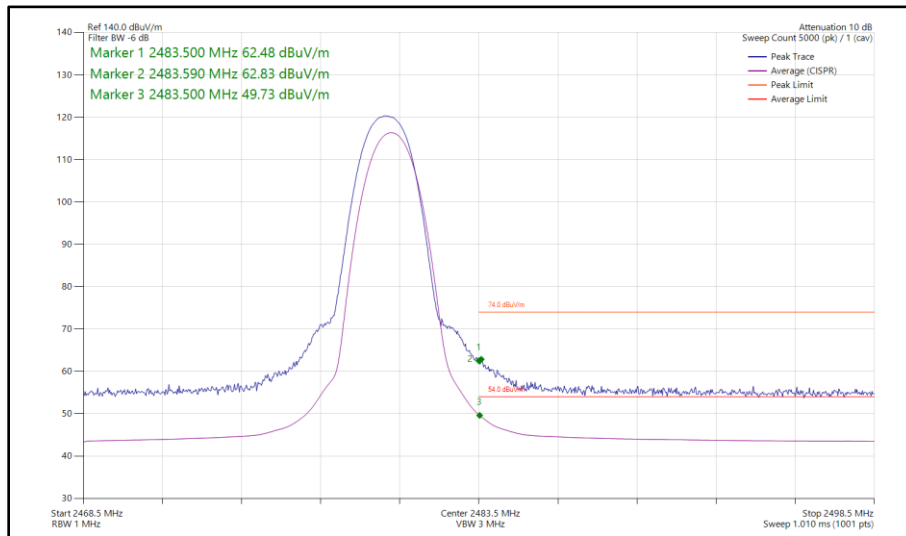
Figure 42 - Bluetooth 3-DH5, MIMO, Core 0 - Core 1 - 2480 MHz Band Edge Frequency 2483.5 MHz
