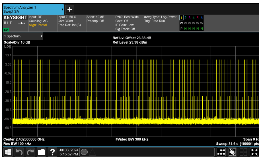
Figure 54 - 8-DPSK - 2402 MHz Accumulated Transmit Time
