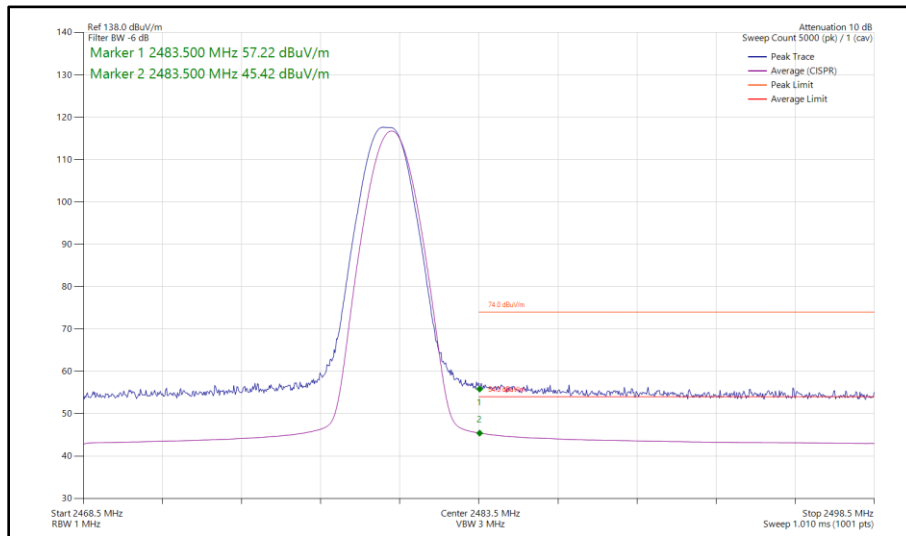
Figure 28 - Bluetooth DH5, SISO, Core 0 - 2480 MHz Band Edge Frequency 2483.5 MHz
