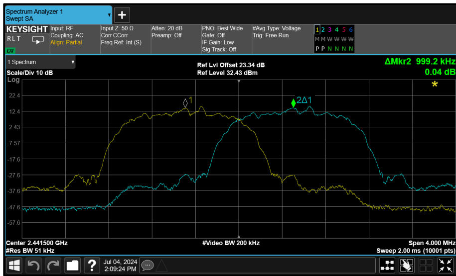
Figure 66 - 8-DPSK - 2441 MHz (CH39)
