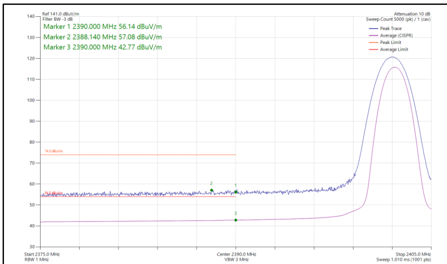
Figure 39 - Bluetooth 3-DH5, MIMO, Core 0 - Core 1 - 2402 MHz Band Edge Frequency 2390 MHz
