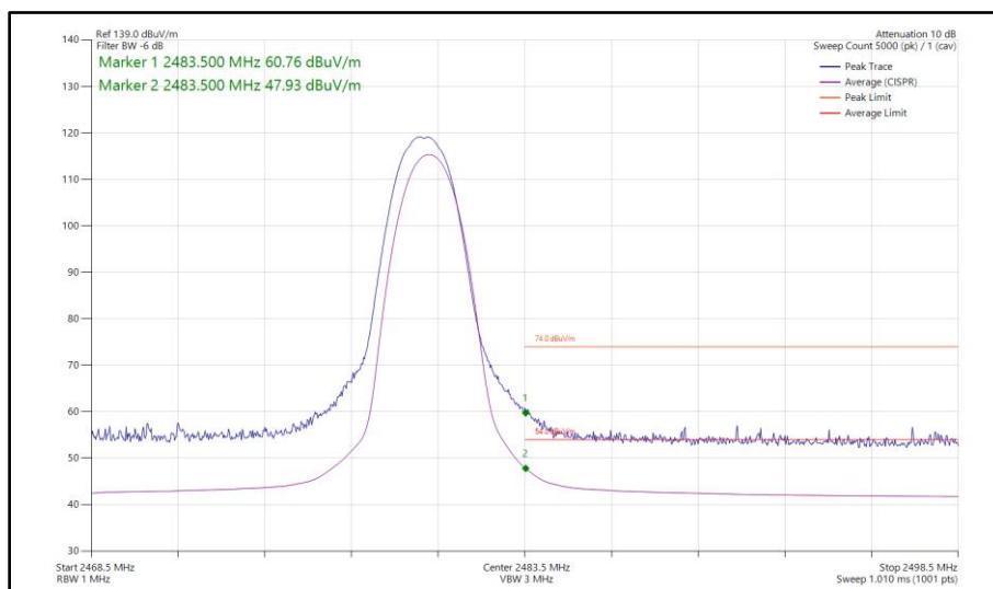
Figure 35 - Bluetooth 2-DH5, SISO, Core 1 - 2480 MHz Band Edge Frequency 2483.5 MHz
