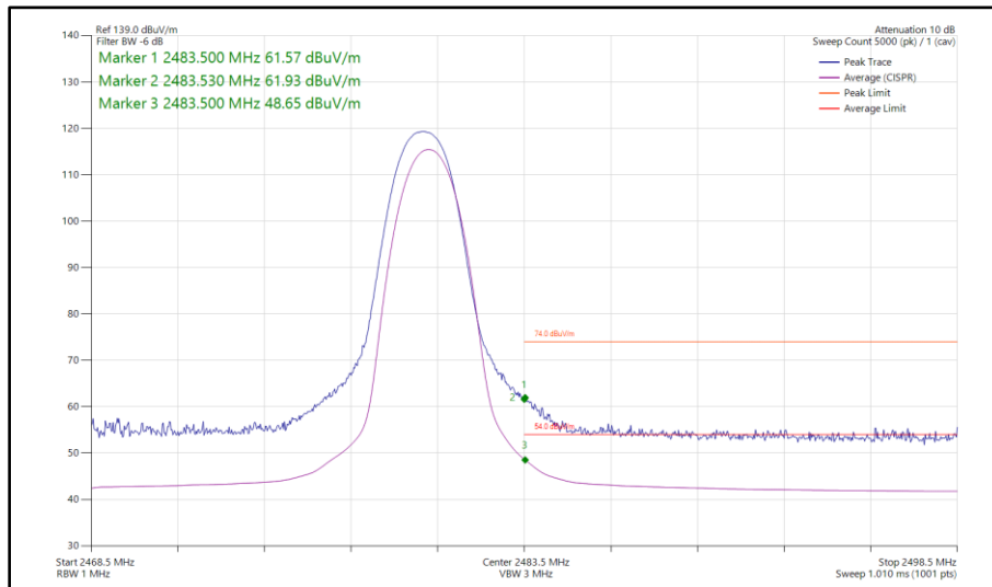
Figure 36 - Bluetooth 3-DH5, SISO, Core 1 - 2480 MHz Band Edge Frequency 2483.5 MHz
