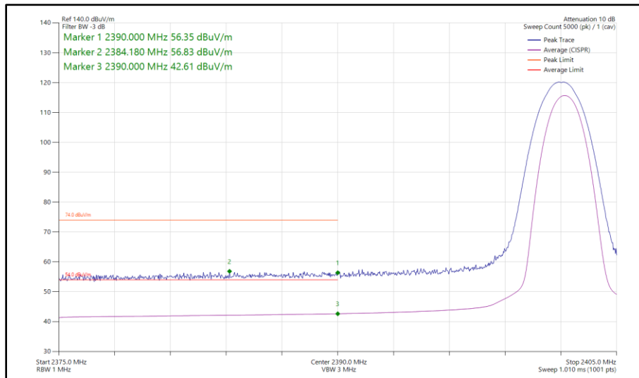
Figure 26 - Bluetooth 2-DH5, SISO, Core 0 - 2402 MHz Band Edge Frequency 2390 MHz
