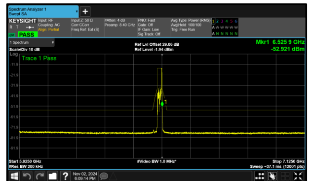
Figure 277 - A (Core 0) 802.11ax HE20 RU26 LPI 6515 MHz (CH113)
