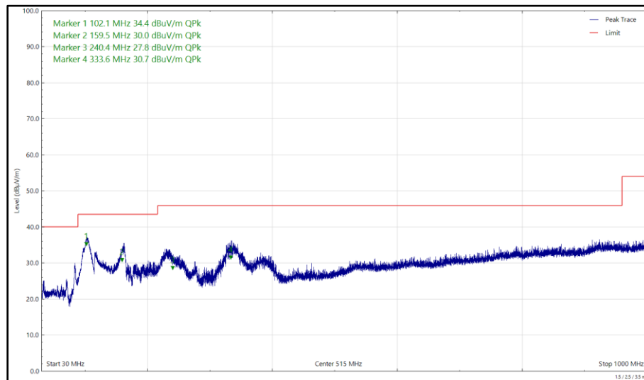
Figure 265 - 6995 MHz (CH209), HE20, SU, CDD, Core 0 + Core 1, 30 MHz to 1 GHz, Horizontal (Peak)
