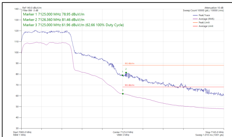
Figure 182 - 802.11ax HE20, SU, SDM, Core 0 - Core 1 - 7095 MHz Band Edge Frequency 7125 MHz
