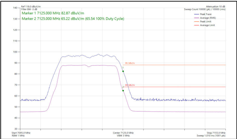
Figure 173 - 802.11a, SISO, Core 1 - 7115 MHz Band Edge Frequency 7125 MHz
