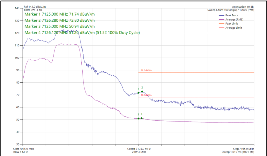
Figure 179 - 802.11ax HE20, RU 106-54, CDD, Core 0 - Core 1 - 7095 MHz Band Edge Frequency 7125 MHz
