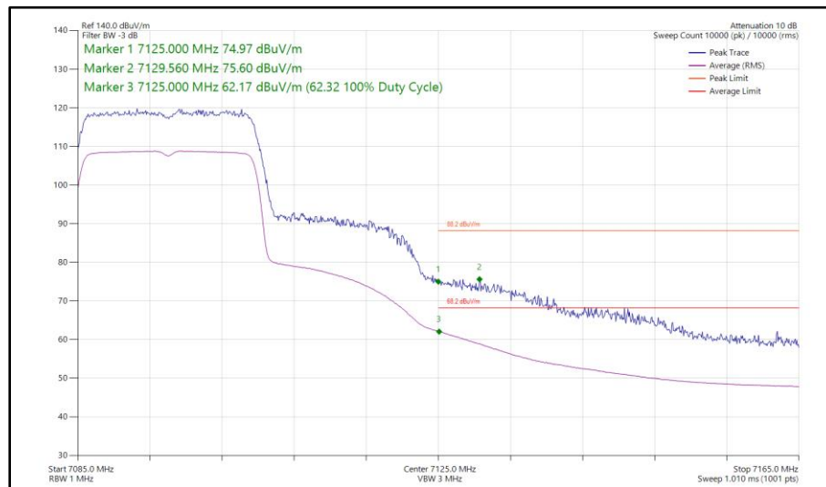
Figure 174 - 802.11ax HE20, SU, SISO, Core 1 - 7095 MHz Band Edge Frequency 7125 MHz
