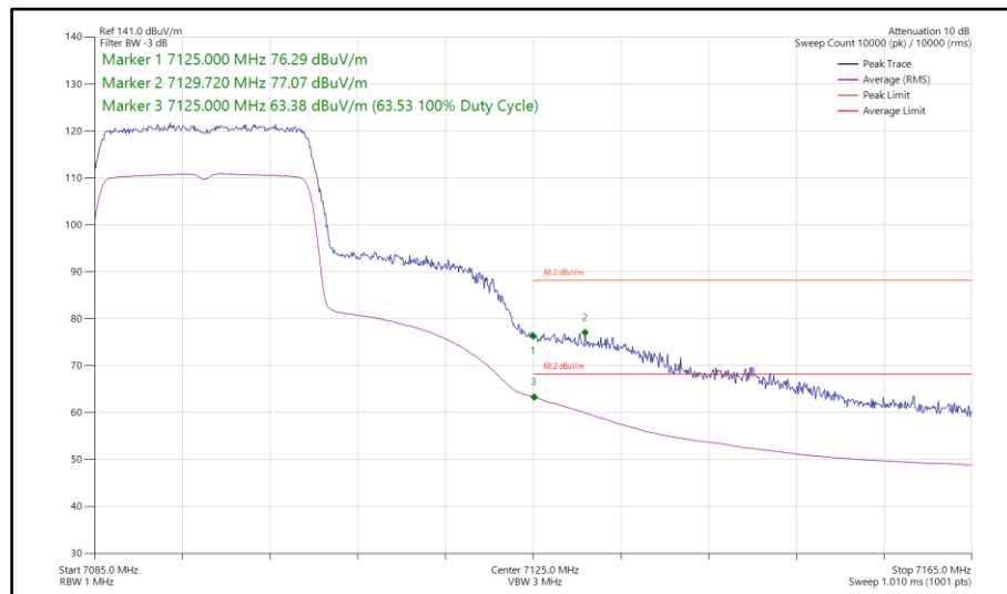
Figure 167 - 802.11ax HE20, SU, SISO, Core 0 - 7095 MHz Band Edge Frequency 7125 MHz
