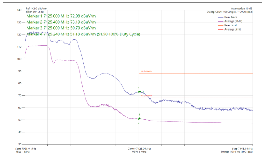
Figure 168 - 802.11ax HE20, RU 106-53, SISO, Core 0 - 7095 MHz Band Edge Frequency 7125 MHz
