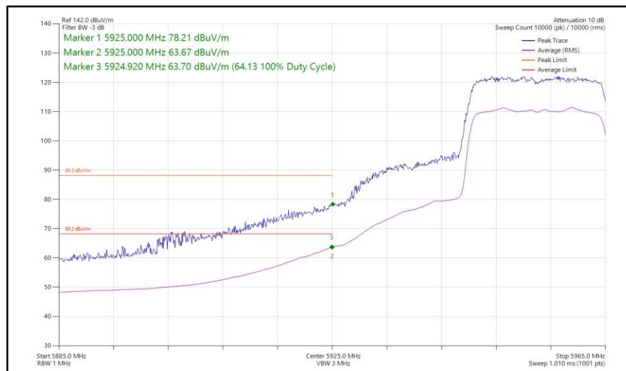
Figure 180 - 802.11ax HE20, SU, SDM, Core 0 - Core 1 - 5955 MHz Band Edge Frequency 5925 MHz
