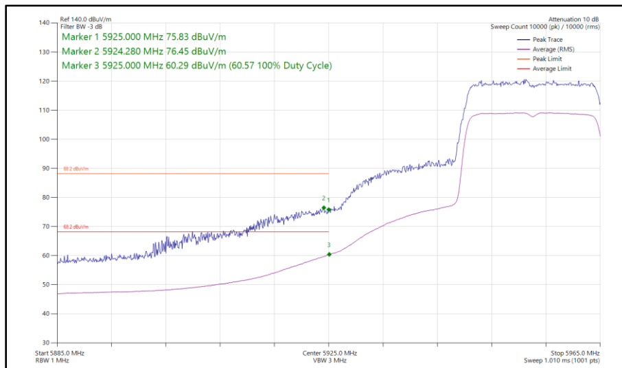
Figure 170 - 802.11ax HE20, SU, SISO, Core 1 - 5955 MHz Band Edge Frequency 5925 MHz
