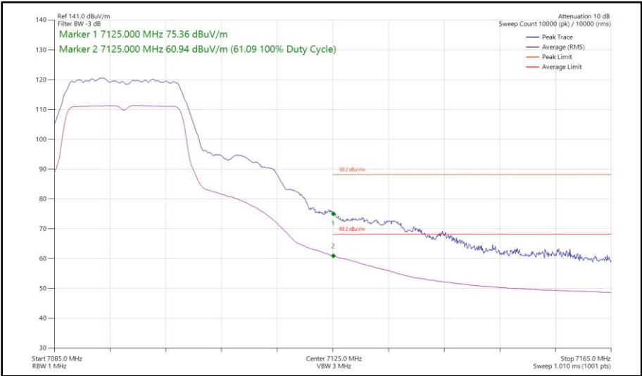
Figure 165 - 802.11a, SISO, Core 0 - 7095 MHz Band Edge Frequency 7125 MHz
