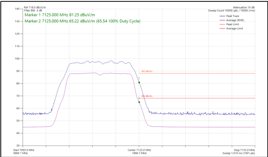
Figure 166 - 802.11a, SISO, Core 0 - 7115 MHz Band Edge Frequency 7125 MHz
