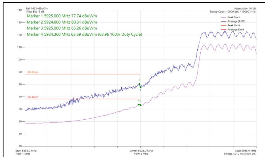
Figure 176 - 802.11ax HE20, SU, CDD, Core 0 - Core 1 - 5955 MHz Band Edge Frequency 5925 MHz
