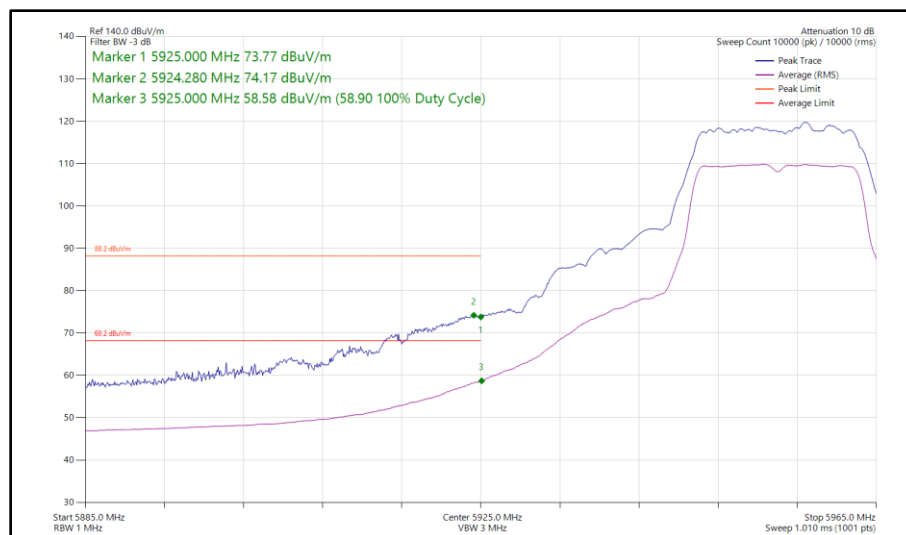
Figure 162 - 802.11a, SISO, Core 0 - 5955 MHz Band Edge Frequency 5925 MHz
