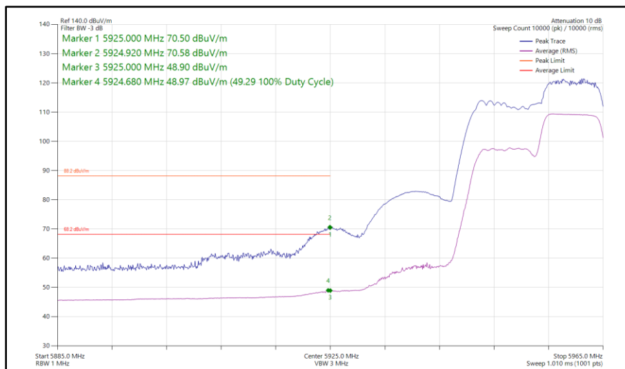
Figure 164 - 802.11ax HE20, RU 106-54, SISO, Core 0 - 5955 MHz Band Edge Frequency 5925 MHz
