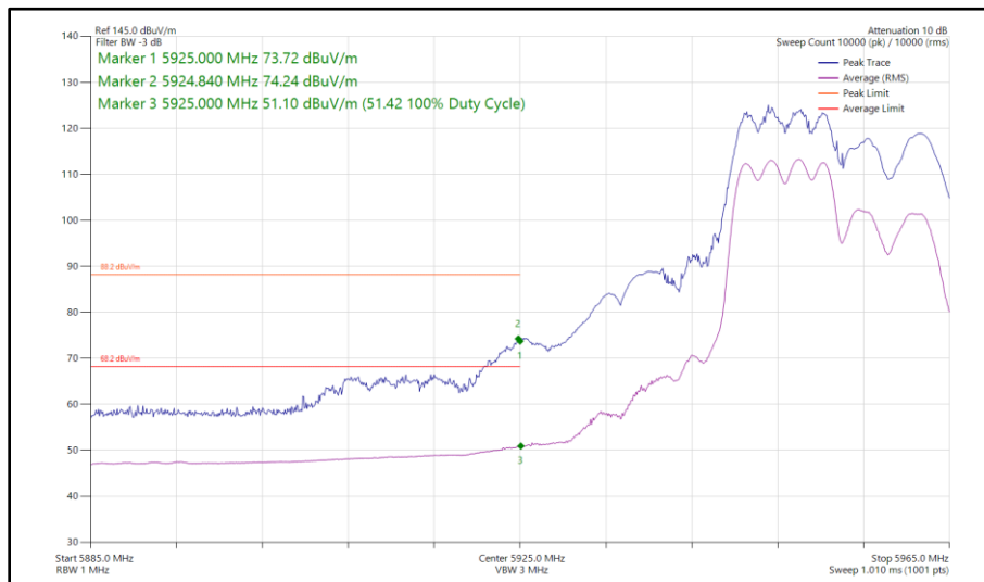
Figure 181 - 802.11ax HE20, RU 106-53, SDM, Core 0 - Core 1 - 5955 MHz Band Edge Frequency 5925 MHz
