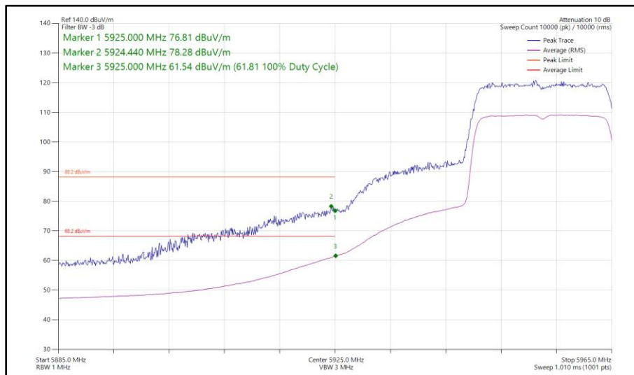
Figure 163 - 802.11ax HE20, SU, SISO, Core 0 - 5955 MHz Band Edge Frequency 5925 MHz
