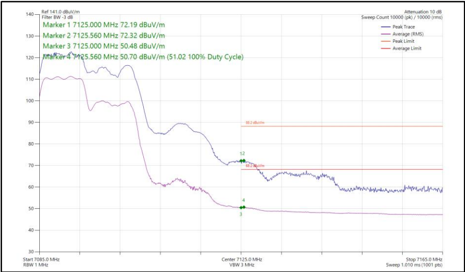
Figure 183 - 802.11ax HE20, RU 106-53, SDM, Core 0 - Core 1 - 7095 MHz Band Edge Frequency 7125 MHz
