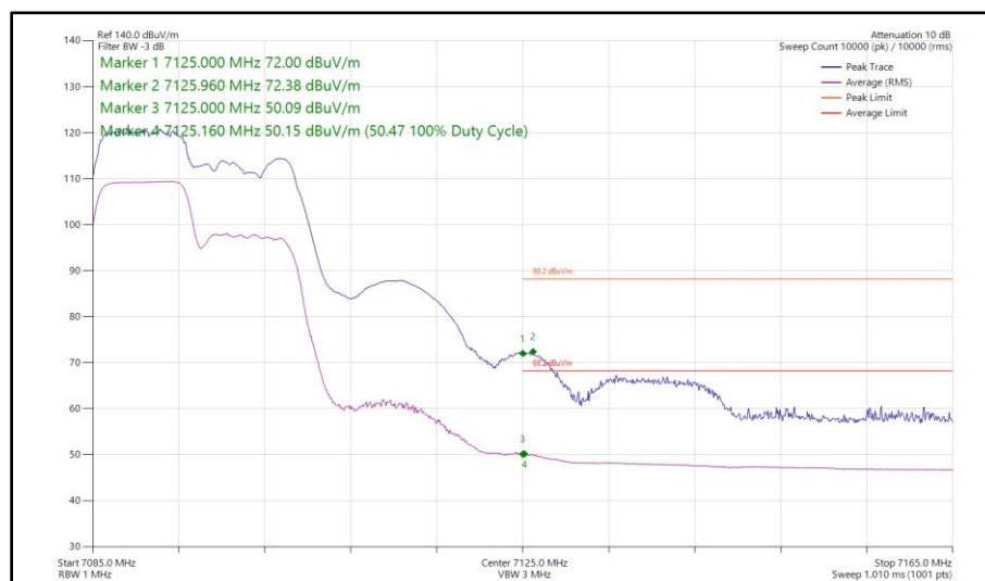
Figure 175 - 802.11ax HE20, RU 106-53, SISO, Core 1 - 7095 MHz Band Edge Frequency 7125 MHz
