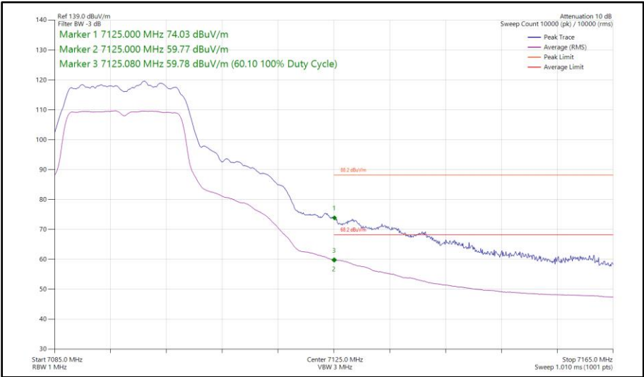
Figure 172 - 802.11a, SISO, Core 1 - 7095 MHz Band Edge Frequency 7125 MHz
