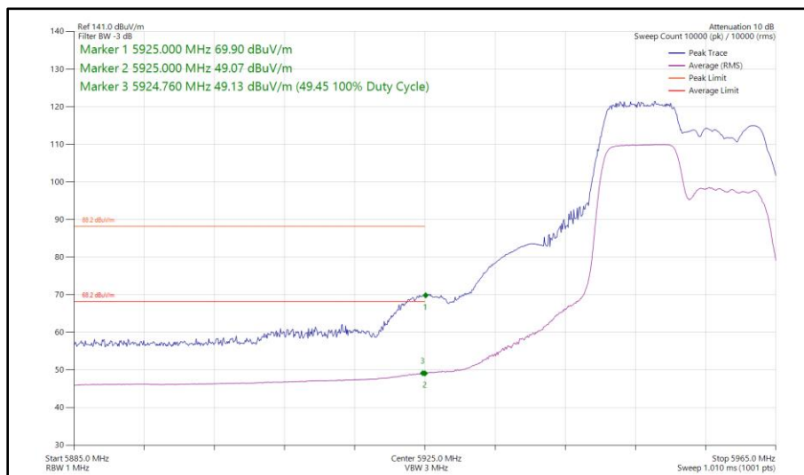
Figure 171 - 802.11ax HE20, RU 106-53, SISO, Core 1 - 5955 MHz Band Edge Frequency 5925 MHz
