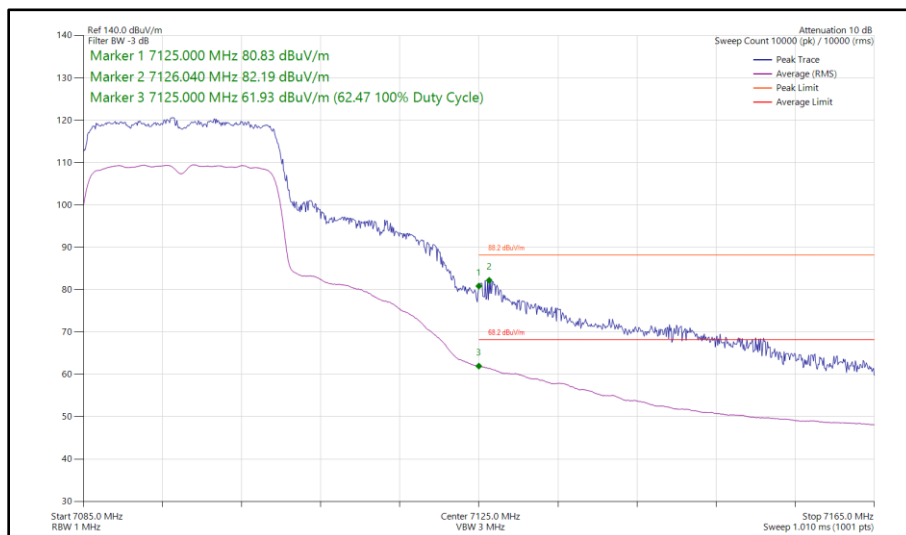
Figure 178 - 802.11ax HE20, SU, CDD, Core 0 - Core 1 - 7095 MHz Band Edge Frequency 7125 MHz
