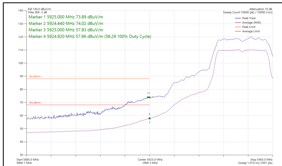
Figure 169 - 802.11a, SISO, Core 1 - 5955 MHz Band Edge Frequency 5925 MHz
