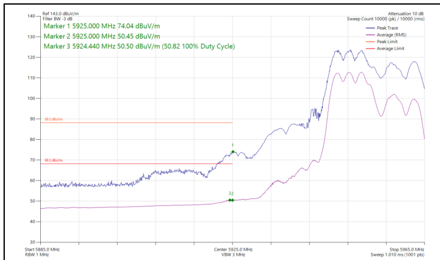
Figure 177 - 802.11ax HE20, RU 106-53, CDD, Core 0 - Core 1 - 5955 MHz Band Edge Frequency 5925 MHz
