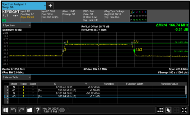
Figure 79 - 802.11ax HE160 SU VLP Minimum 26 dB EBW
