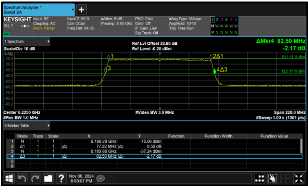
Figure 77 - 802.11ax HE80 SU VLP Minimum 26 dB EBW
