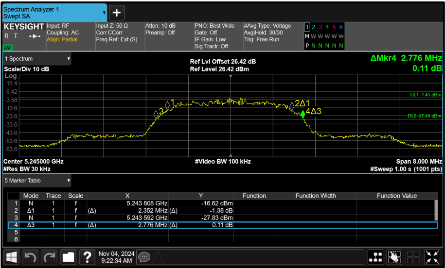
Figure 96 - Core 1 (B) 5245 MHz (CH95) 26 dB and 99% Bandwidth
