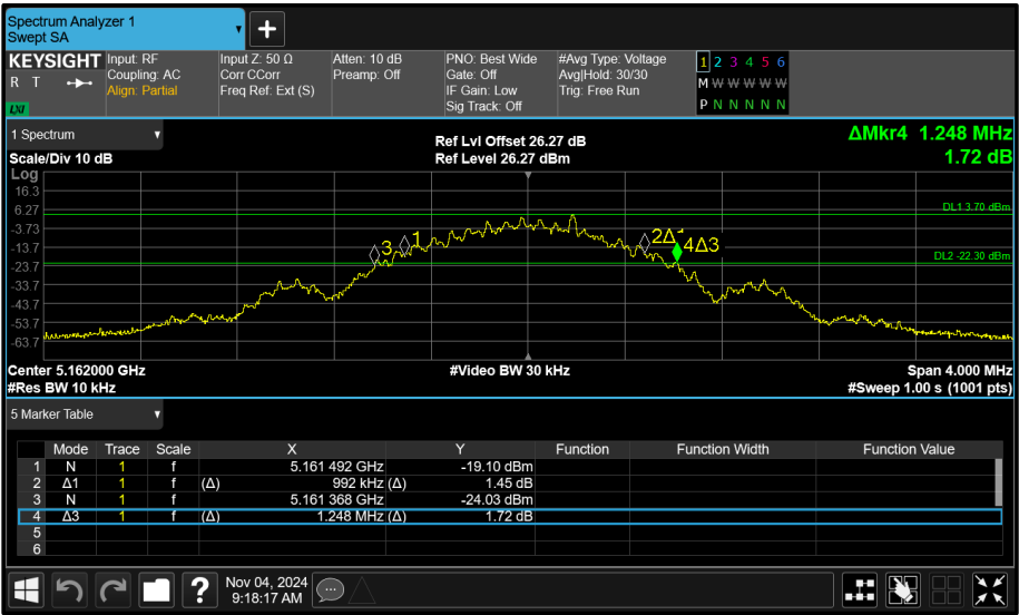
Figure 85 - Core 1 (B) 5162 MHz (CH12) 26 dB and 99% Bandwidth
