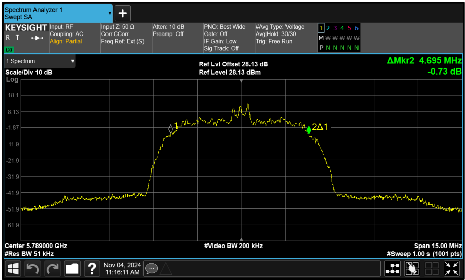
Figure 77 - Core 0 (A) 5789 MHz (CH64) 99% Bandwidth
