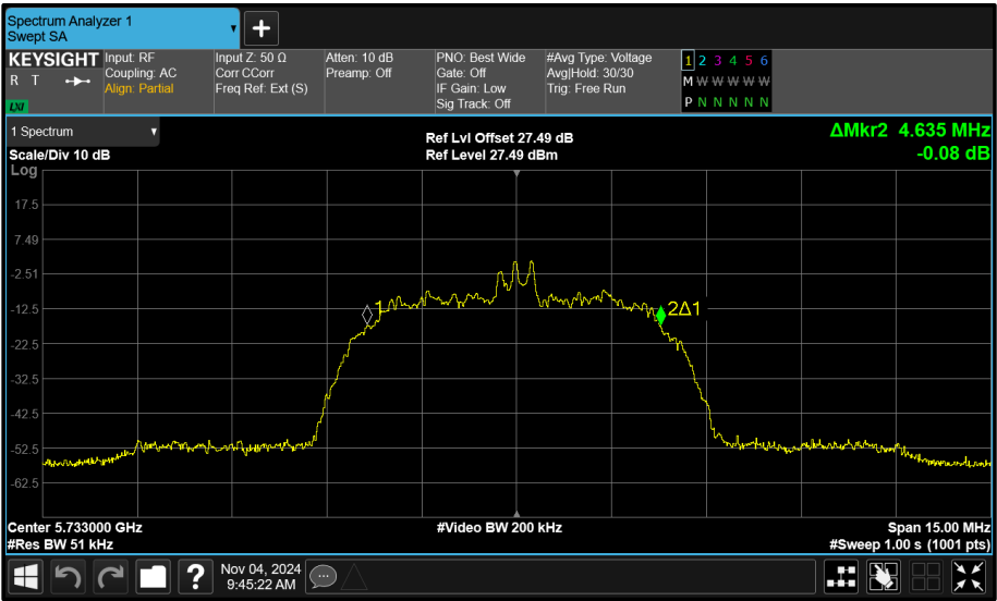
Figure 136 - Core 1 (B) 5733 MHz (CH8) 99% Bandwidth
