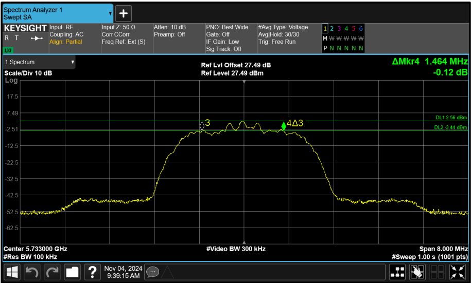
Figure 131 - Core 1 (B) 5733 MHz (CH8) 6 dB Bandwidth
