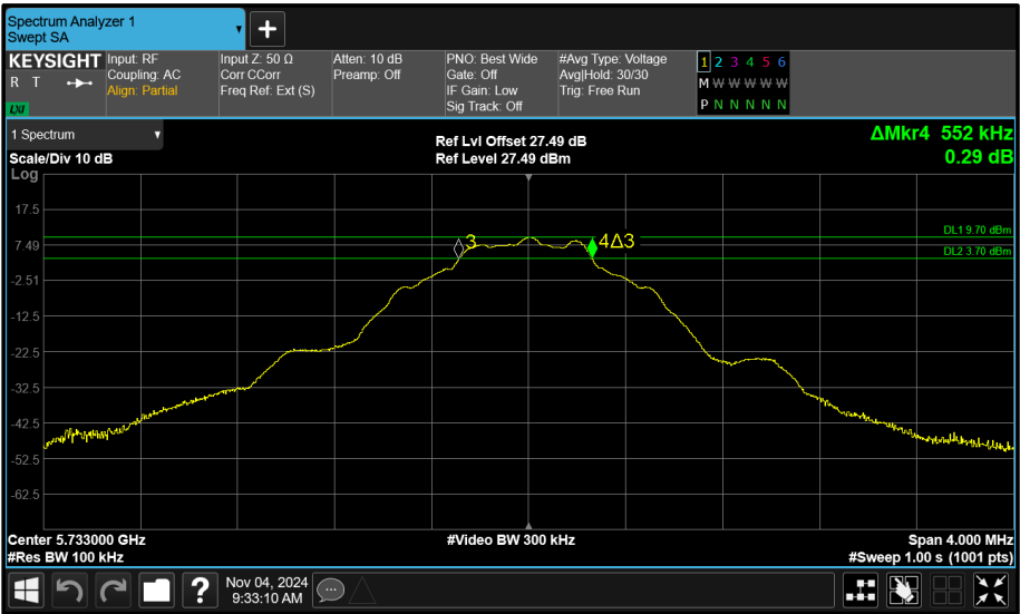
Figure 113 - Core 1 (B) 5733 MHz (CH8) 6 dB Bandwidth
