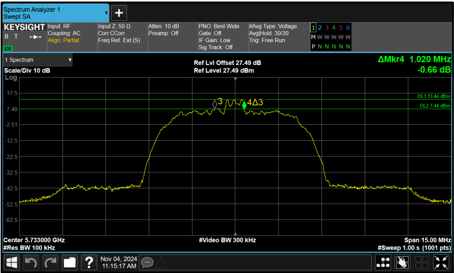
Figure 76 - Core 1 (B) 5733 MHz (CH8) 6 dB Bandwidth
