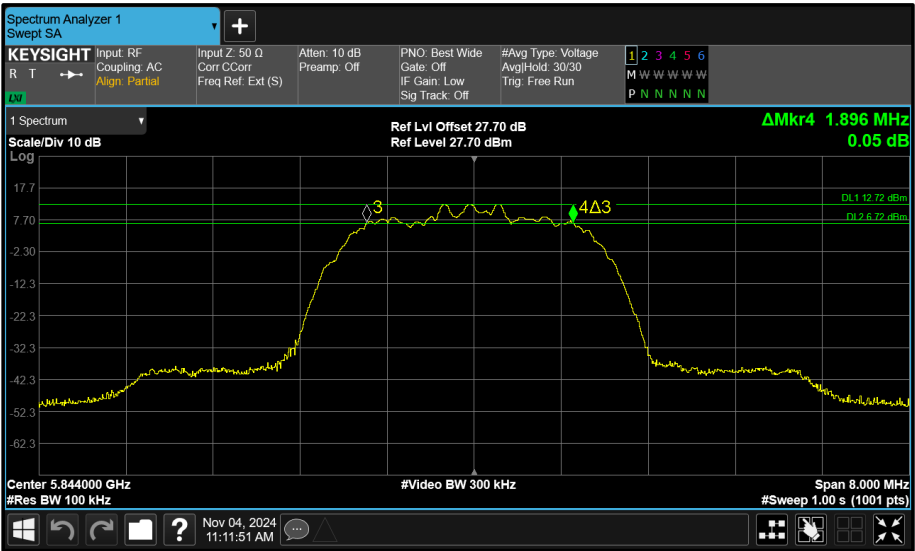
Figure 72 - Core 1 (B) 5844 MHz (CH119) 6 dB Bandwidth
