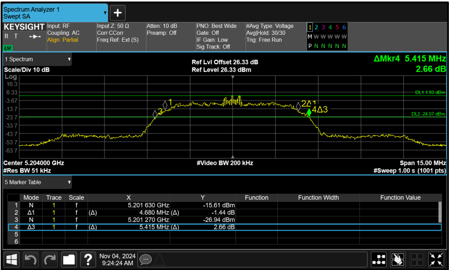
Figure 98 - Core 1 (B) 5204 MHz (CH54) 26 dB and 99% Bandwidth
