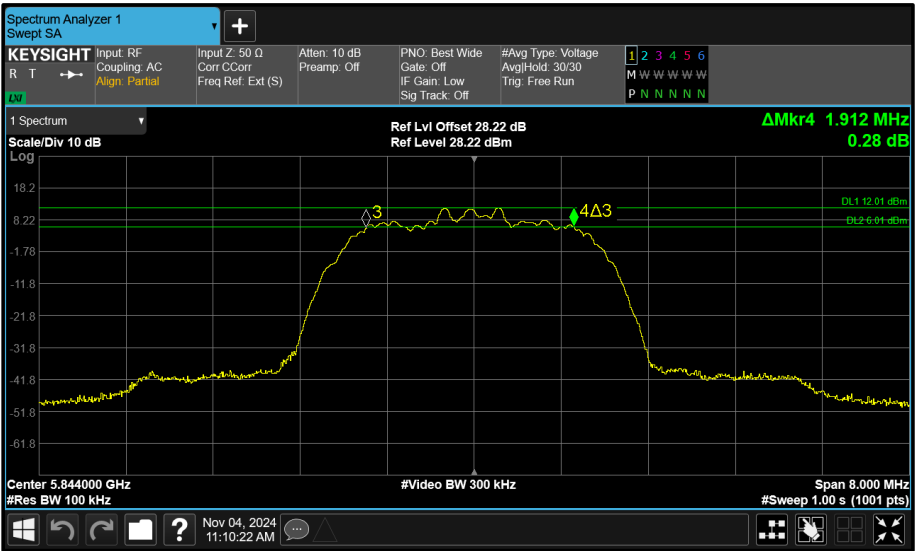
Figure 70 - Core 0 (A) 5844 MHz (CH119) 6 dB Bandwidth
