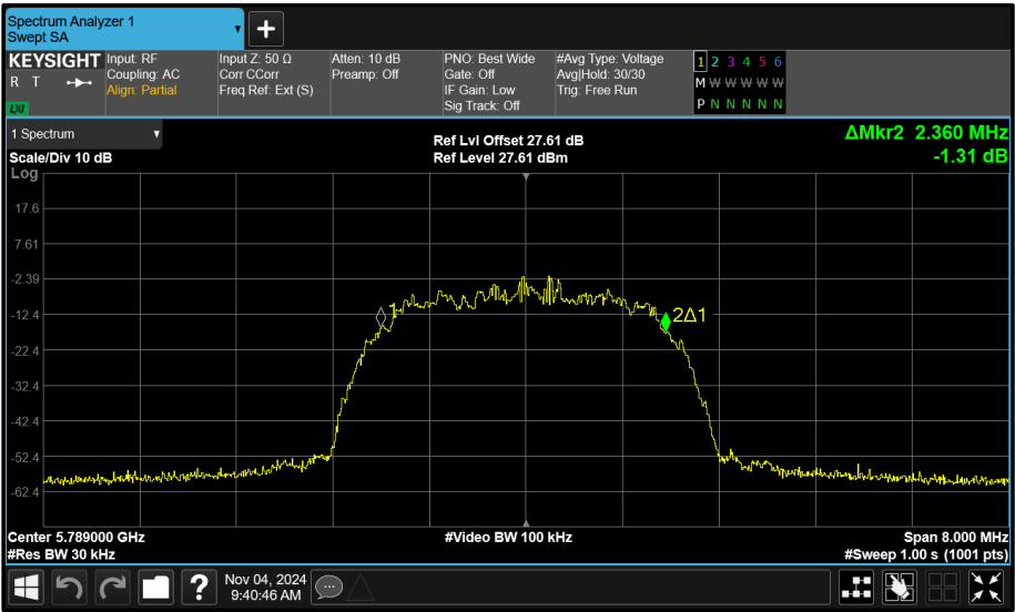
Figure 132 - Core 1 (B) 5789 MHz (CH64) 99% Bandwidth
