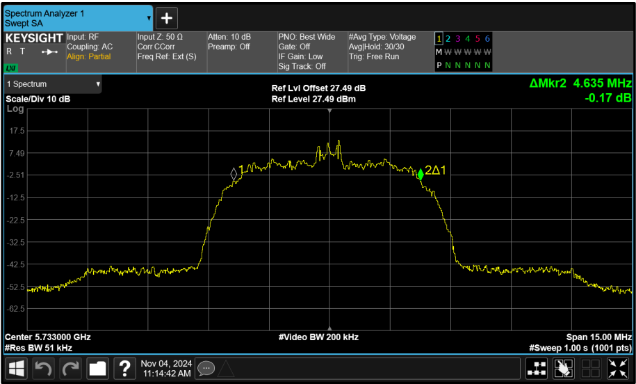
Figure 75 - Core 1 (B) 5733 MHz (CH8) 99% Bandwidth
