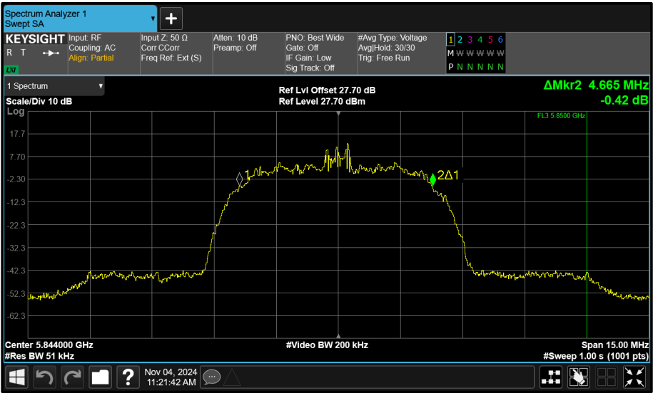
Figure 83 - Core 1 (B) 5844 MHz (CH119) 99% Bandwidth
