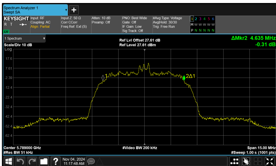
Figure 79 - Core 1 (B) 5789 MHz (CH64) 99% Bandwidth
