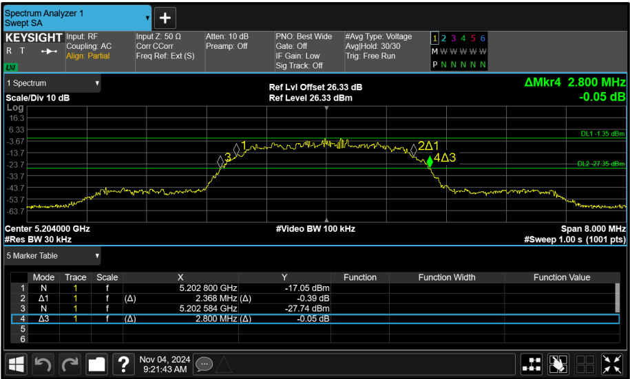
Figure 95 - Core 1 (B) 5204 MHz (CH54) 26 dB and 99% Bandwidth
