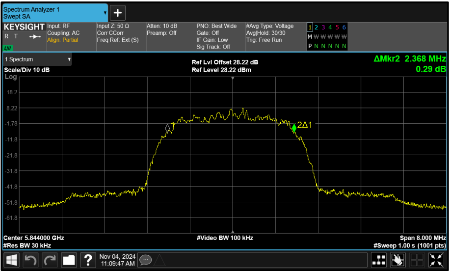
Figure 69 - Core 0 (A) 5844 MHz (CH119) 99% Bandwidth
