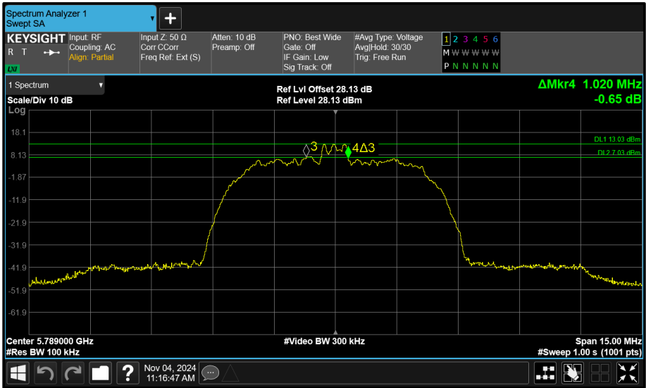
Figure 78 - Core 0 (A) 5789 MHz (CH64) 6 dB Bandwidth
