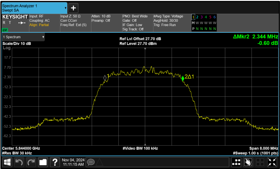
Figure 71 - Core 1 (B) 5844 MHz (CH119) 99% Bandwidth
