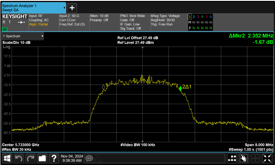
Figure 130 - Core 1 (B) 5733 MHz (CH8) 99% Bandwidth
