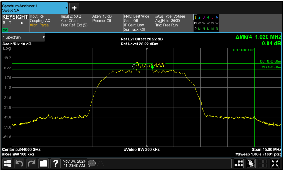
Figure 82 - Core 0 (A) 5844 MHz (CH119) 6 dB Bandwidth
