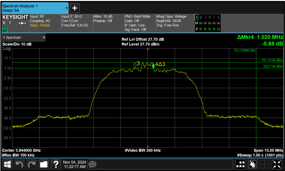
Figure 84 - Core 1 (B) 5844 MHz (CH119) 6 dB Bandwidth
