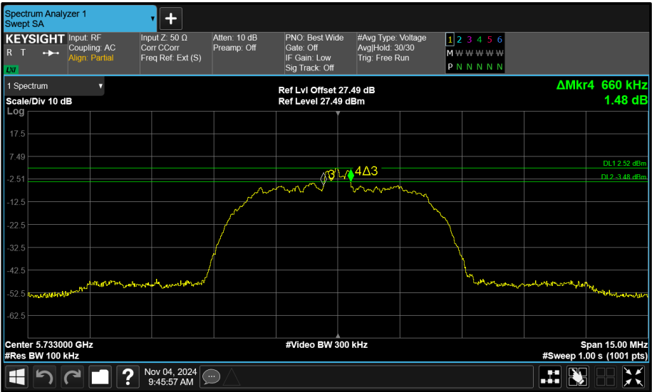
Figure 137 - Core 1 (B) 5733 MHz (CH8) 6 dB Bandwidth
