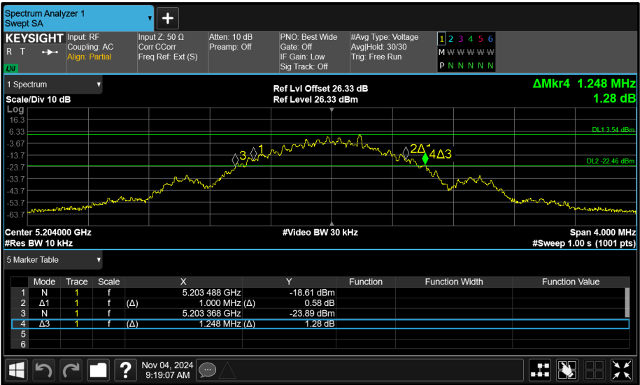
Figure 86 - Core 1 (B) 5204 MHz (CH54) 26 dB and 99% Bandwidth
