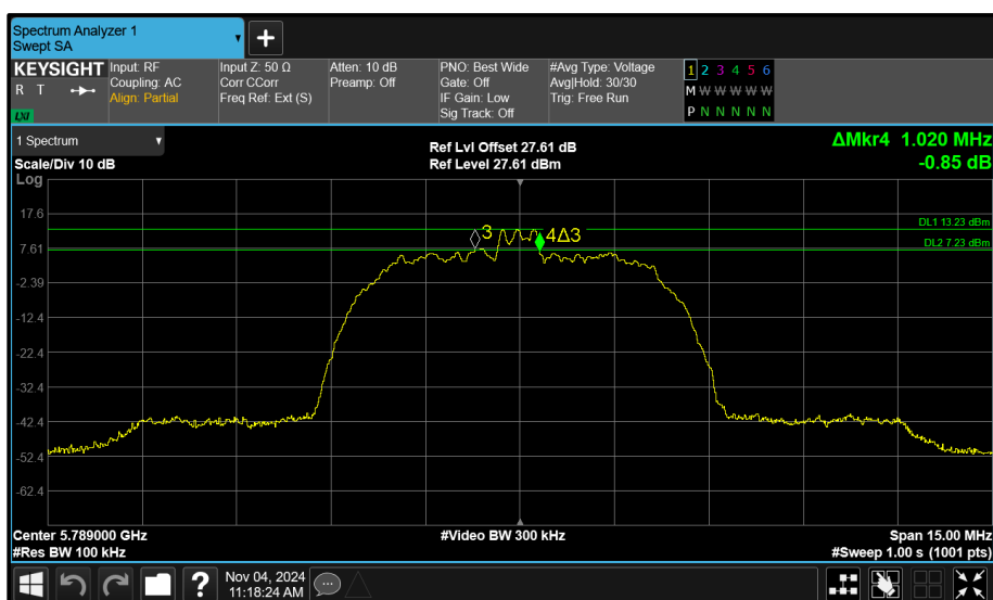
Figure 80 - Core 1 (B) 5789 MHz (CH64) 6 dB Bandwidth
