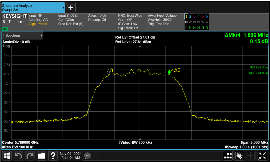
Figure 133 - Core 1 (B) 5789 MHz (CH64) 6 dB Bandwidth
