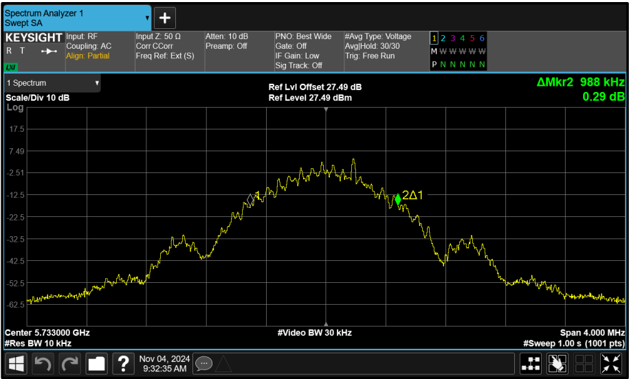
Figure 112 - Core 1 (B) 5733 MHz (CH8) 99% Bandwidth
