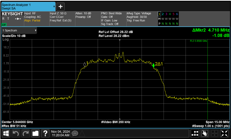
Figure 81 - Core 0 (A) 5844 MHz (CH119) 99% Bandwidth
