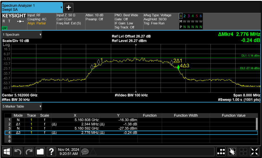
Figure 94 - Core 1 (B) 5162 MHz (CH12) 26 dB and 99% Bandwidth
