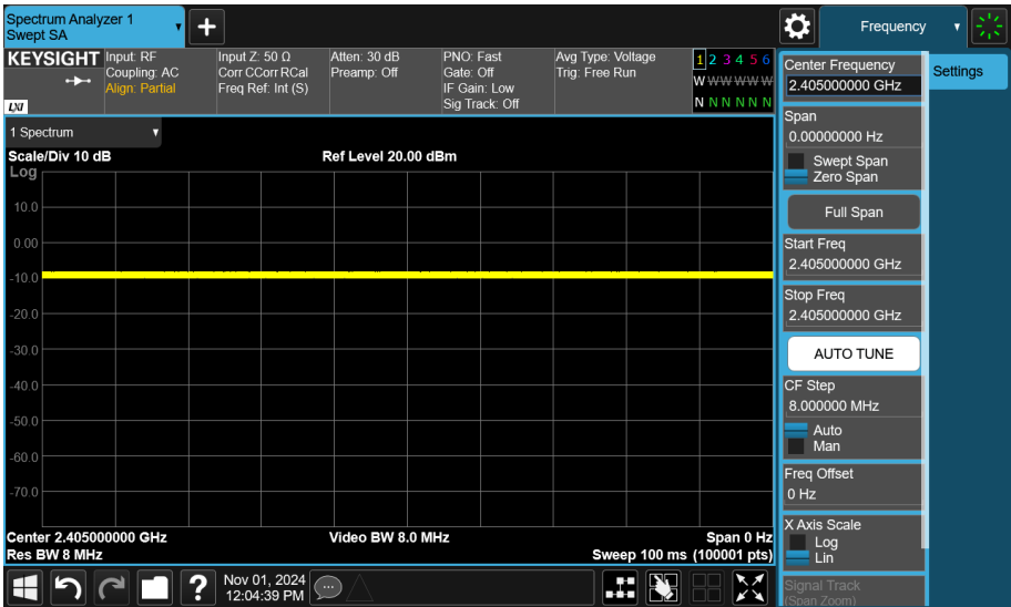
Figure 8 - Thread ePA - Frequency of 2405 MHz (100% Duty Cycle)
