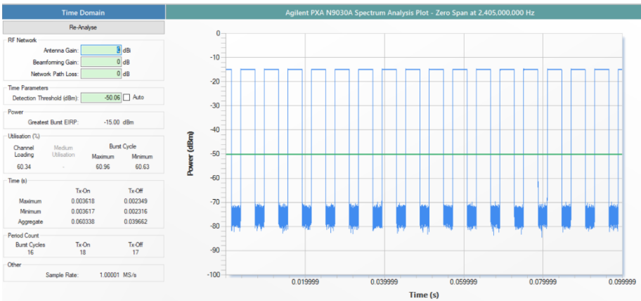
Figure 9 - Thread ePA - Frequency of 2405 MHz (60.96% Duty Cycle)
