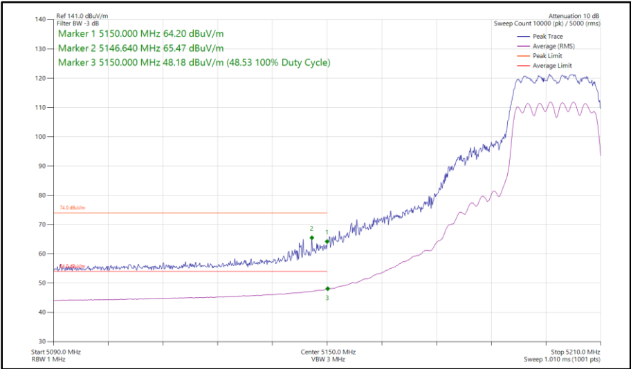
Figure 46 - 802.11n HT20, CDD, Core 0 - Core 1 - 5200 MHz Band Edge Frequency 5150 MHz
