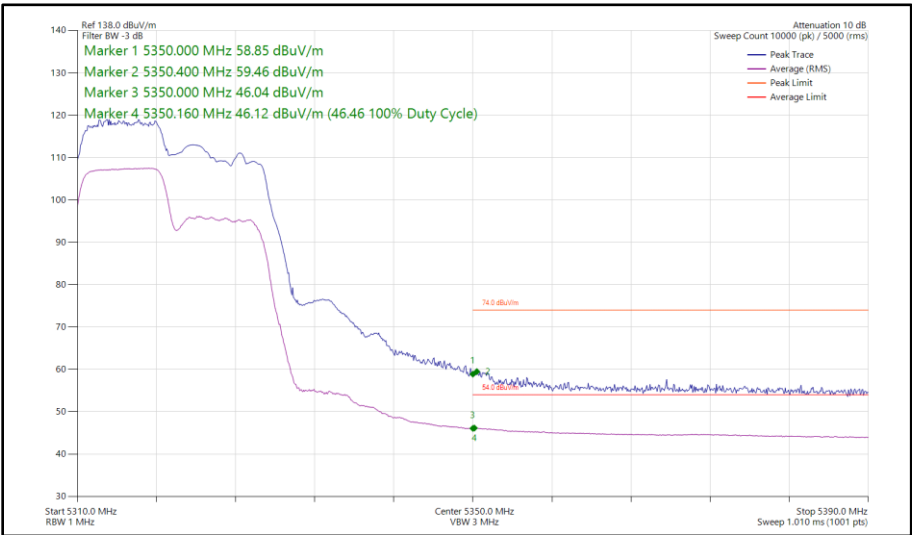
Figure 36 - 802.11ax HE20, RU 106-53, SISO, Core 1 - 5320 MHz Band Edge Frequency 5350 MHz
