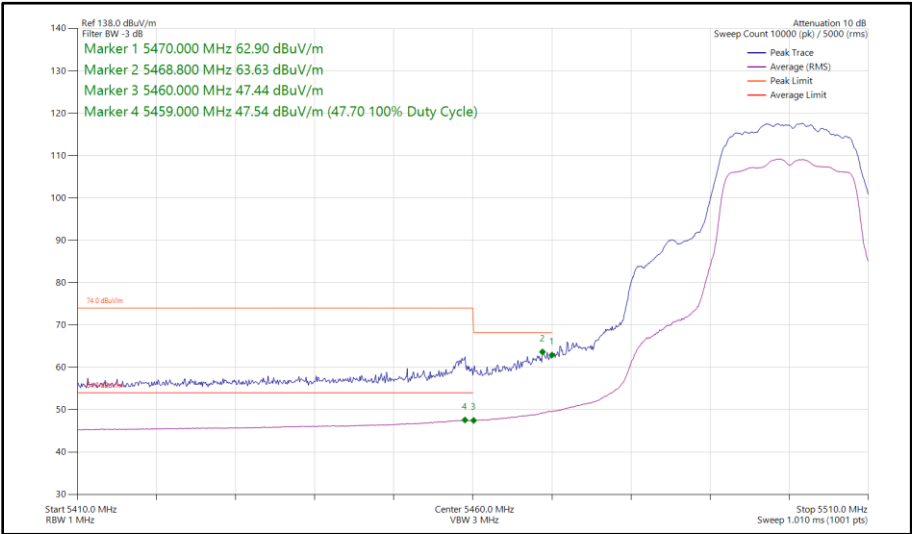
Figure 37 - 802.11a, SISO, Core 1 - 5500 MHz Band Edge Frequency 5460 MHz
