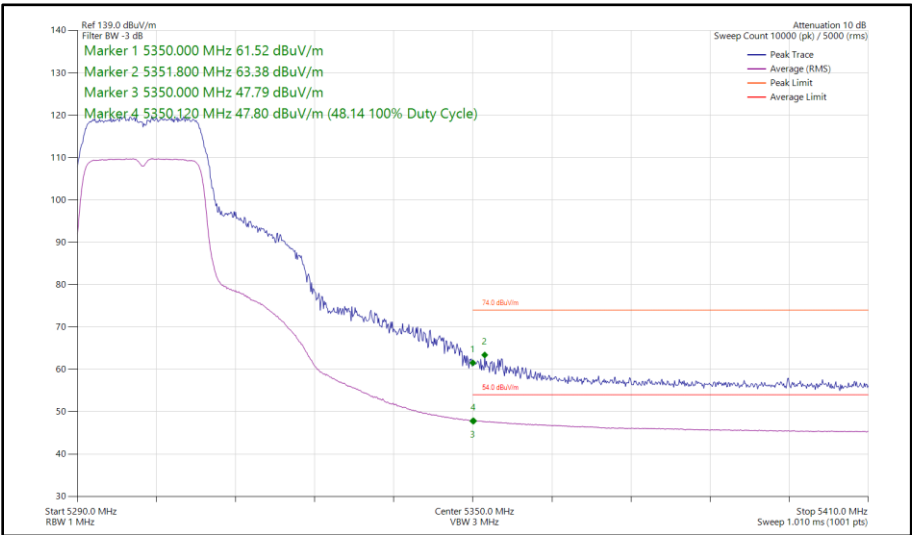
Figure 32 - 802.11n HT20, SISO, Core 1 - 5300 MHz Band Edge Frequency 5350 MHz
