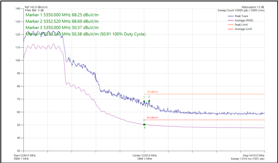
Figure 52 - 802.11ax HE20, SU, CDD, Core 0 - Core 1 - 5300 MHz Band Edge Frequency 5350 MHz
