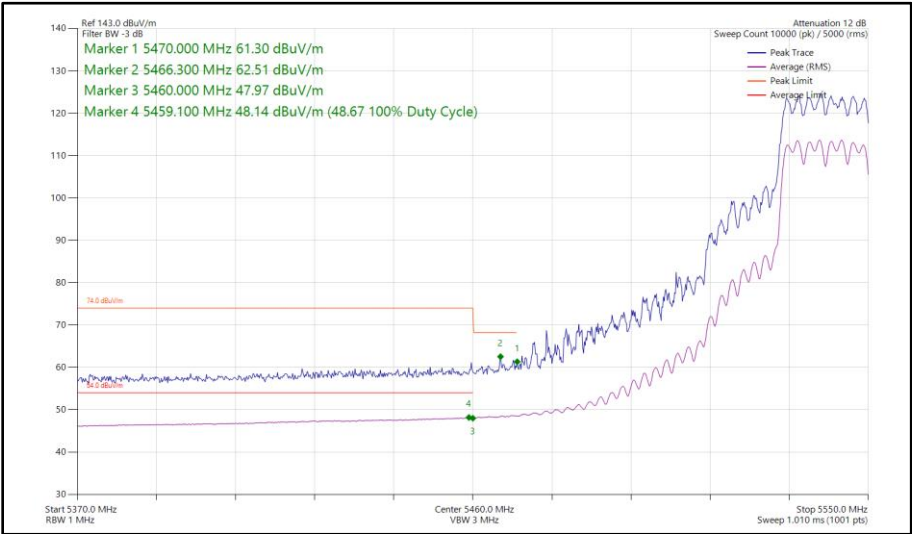
Figure 60 - 802.11ax HE20, SU, CDD, Core 0 - Core 1 - 5540 MHz Band Edge Frequency 5460 MHz
