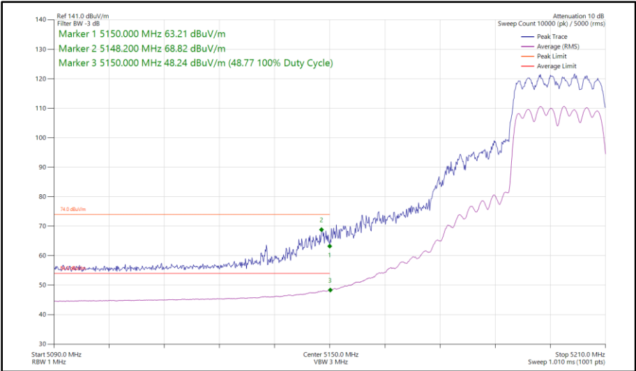
Figure 49 - 802.11ax HE20, SU, CDD, Core 0 - Core 1 - 5200 MHz Band Edge Frequency 5150 MHz
