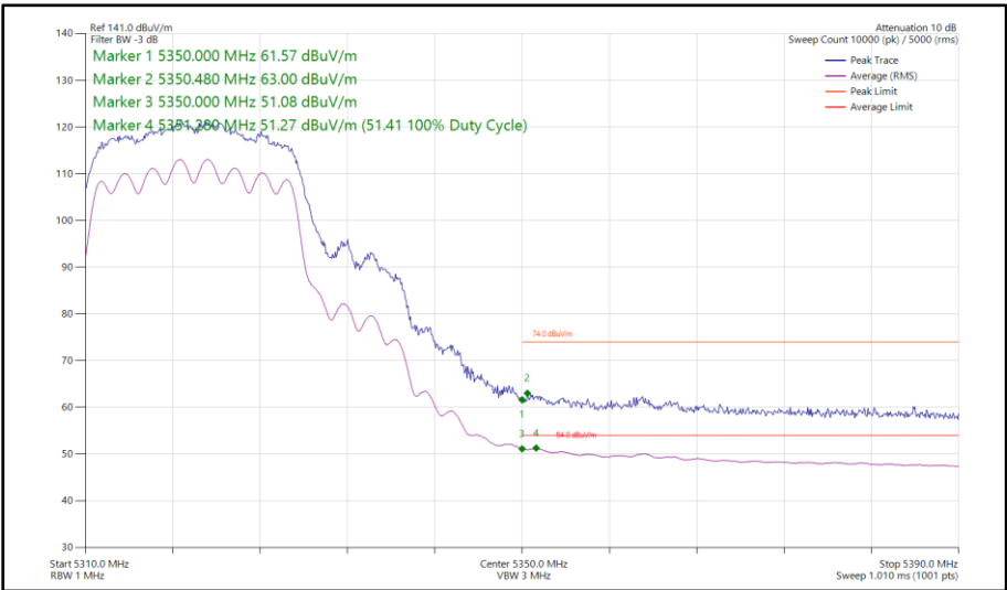
Figure 51 - 802.11n HT20, CDD, Core 0 - Core 1 - 5320 MHz Band Edge Frequency 5350 MHz
