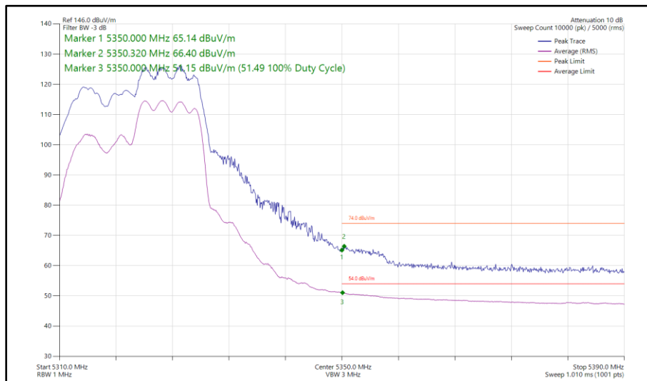
Figure 54 - 802.11ax HE20, RU 106-54, CDD, Core 0 - Core 1 - 5320 MHz Band Edge Frequency 5350 MHz
