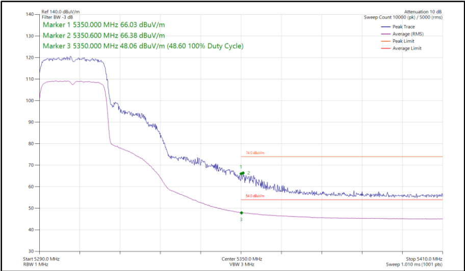
Figure 34 - 802.11ax HE20, SU, SISO, Core 1 - 5300 MHz Band Edge Frequency 5350 MHz
