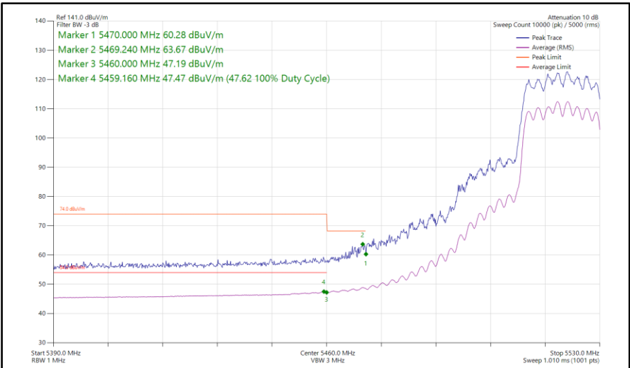
Figure 59 - 802.11ax HE20, SU, CDD, Core 0 - Core 1 - 5520 MHz Band Edge Frequency 5460 MHz
