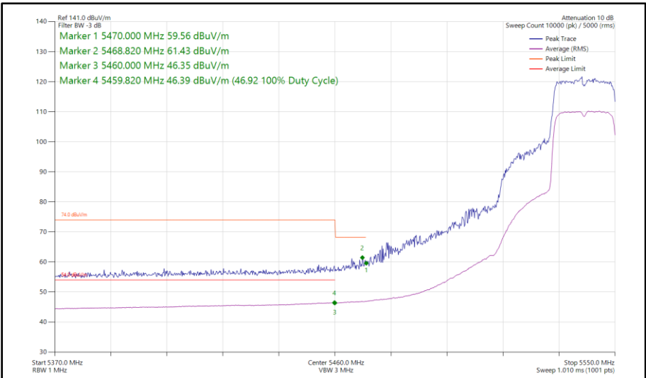
Figure 22 - 802.11ax HE20, SU, SISO, Core 0 - 5540 MHz Band Edge Frequency 5460 MHz
