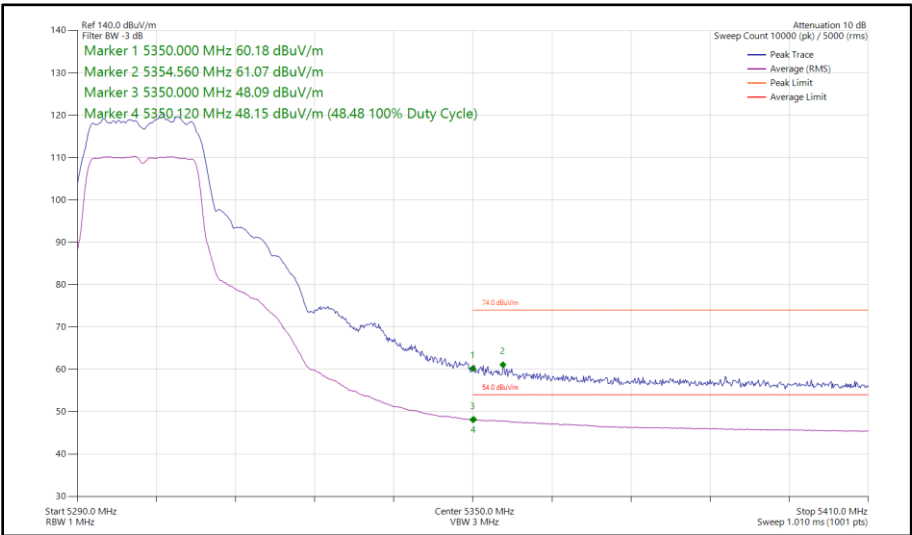
Figure 30 - 802.11a, SISO, Core 1 - 5300 MHz Band Edge Frequency 5350 MHz
