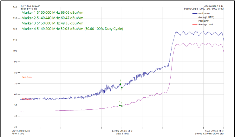
Figure 47 - 802.11ax HE20, SU, CDD, Core 0 - Core 1 - 5180 MHz Band Edge Frequency 5150 MHz
