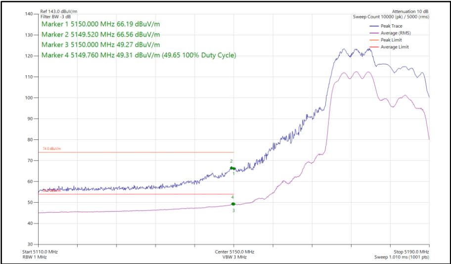
Figure 48 - 802.11ax HE20, RU 106-53, CDD, Core 0 - Core 1 - 5180 MHz Band Edge Frequency 5150 MHz
