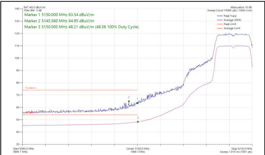
Figure 26 - 802.11n HT20, SISO, Core 1 - 5200 MHz Band Edge Frequency 5150 MHz
