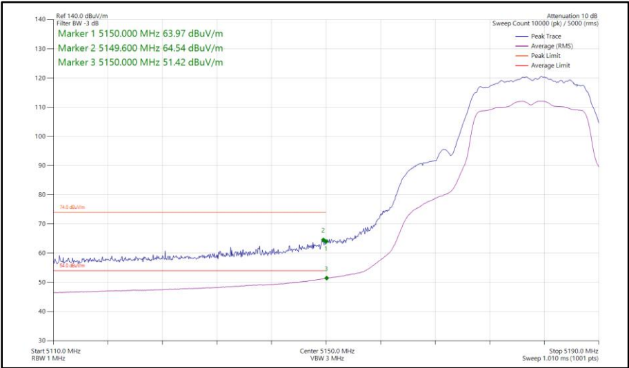
Figure 23 - 802.11a, SISO, Core 1 - 5180 MHz Band Edge Frequency 5150 MHz
