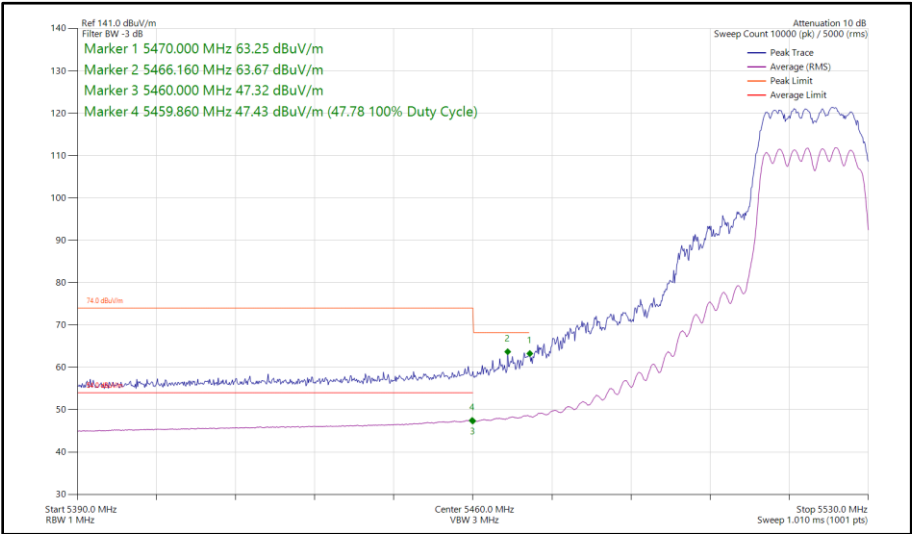
Figure 56 - 802.11n HT20, CDD, Core 0 - Core 1 - 5520 MHz Band Edge Frequency 5460 MHz
