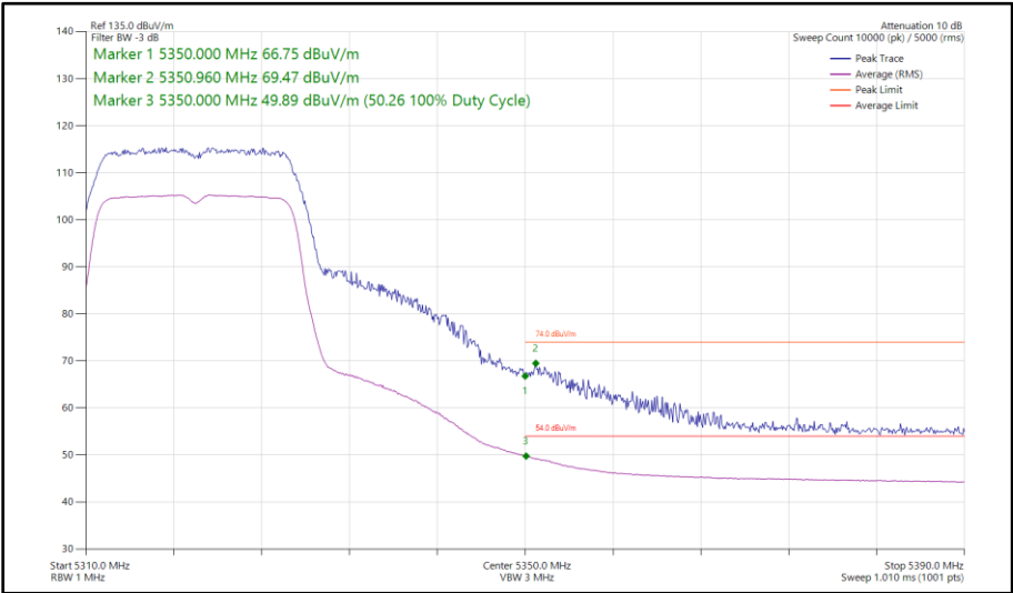
Figure 33 - 802.11n HT20, SISO, Core 1 - 5320 MHz Band Edge Frequency 5350 MHz
