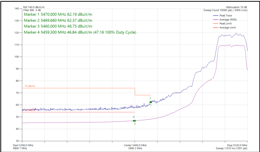
Figure 38 - 802.11a, SISO, Core 1 - 5520 MHz Band Edge Frequency 5460 MHz
