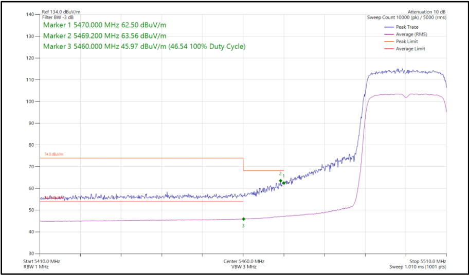
Figure 41 - 802.11ax HE20, SU, SISO, Core 1 - 5500 MHz Band Edge Frequency 5460 MHz
