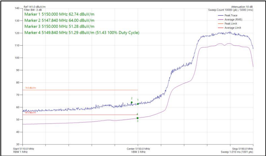
Figure 25 - 802.11n HT20, SISO, Core 1 - 5180 MHz Band Edge Frequency 5150 MHz
