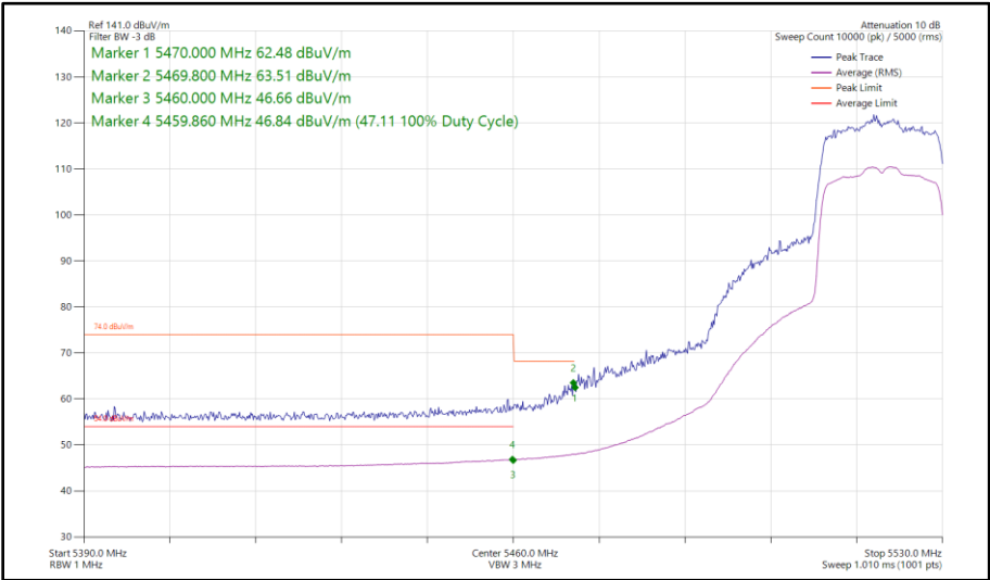
Figure 43 - 802.11ax HE20, SU, SISO, Core 1 - 5520 MHz Band Edge Frequency 5460 MHz
