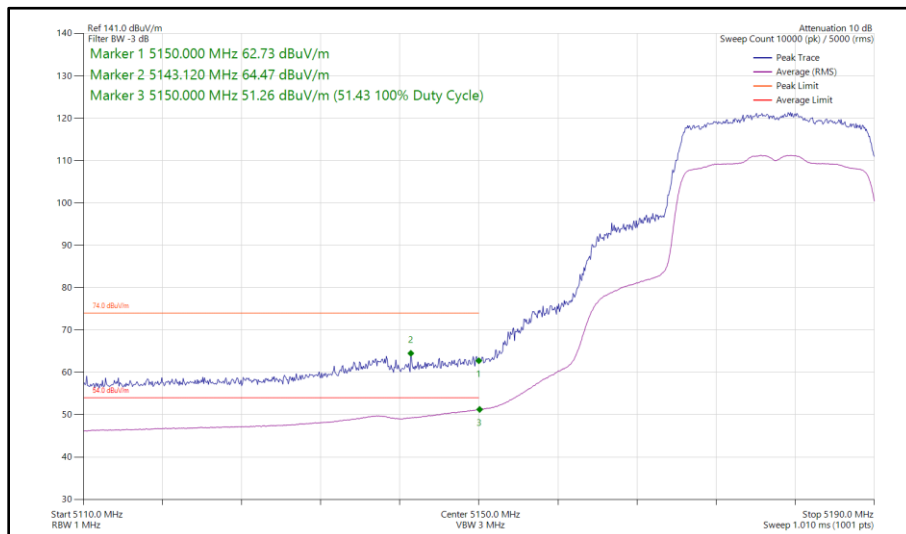
Figure 27 - 802.11ax HE20, SU, SISO, Core 1 - 5180 MHz Band Edge Frequency 5150 MHz
