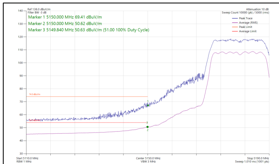
Figure 45 - 802.11n HT20, CDD, Core 0 - Core 1 - 5180 MHz Band Edge Frequency 5150 MHz
