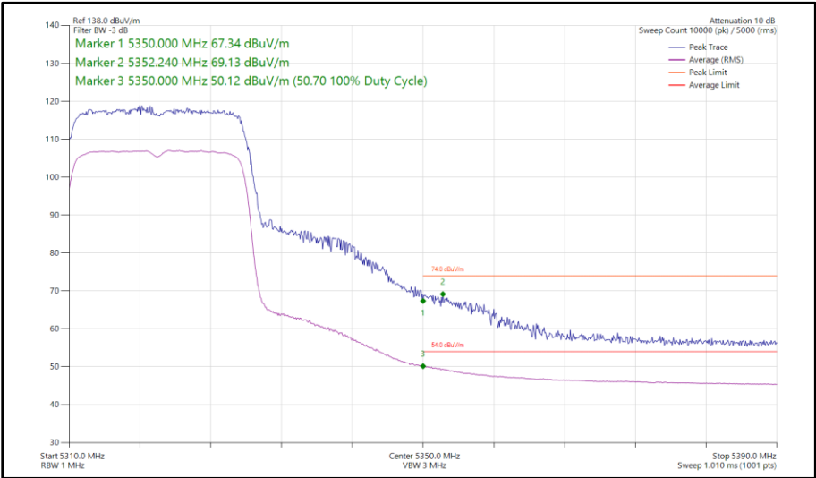
Figure 35 - 802.11ax HE20, SU, SISO, Core 1 - 5320 MHz Band Edge Frequency 5350 MHz
