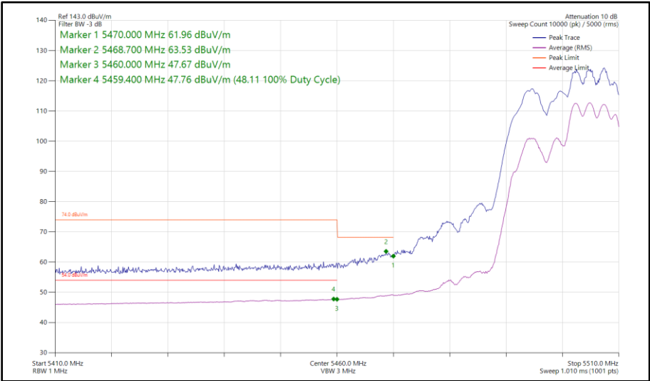
Figure 58 - 802.11ax HE20, RU 106-54, CDD, Core 0 - Core 1 - 5500 MHz Band Edge Frequency 5460 MHz
