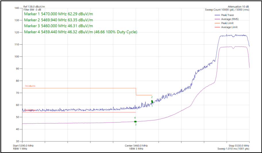
Figure 40 - 802.11n HT20, SISO, Core 1 - 5520 MHz Band Edge Frequency 5460 MHz
