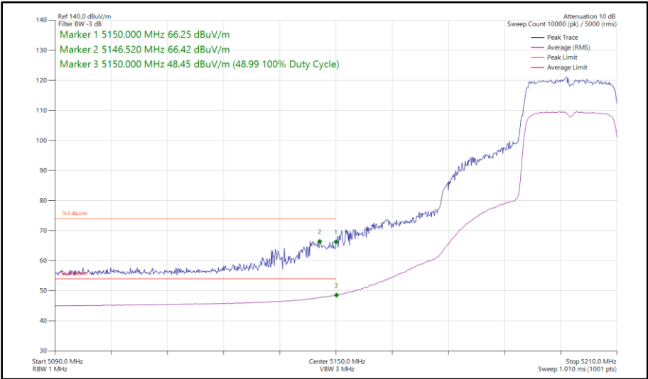
Figure 29 - 802.11ax HE20, SU, SISO, Core 1 - 5200 MHz Band Edge Frequency 5150 MHz
