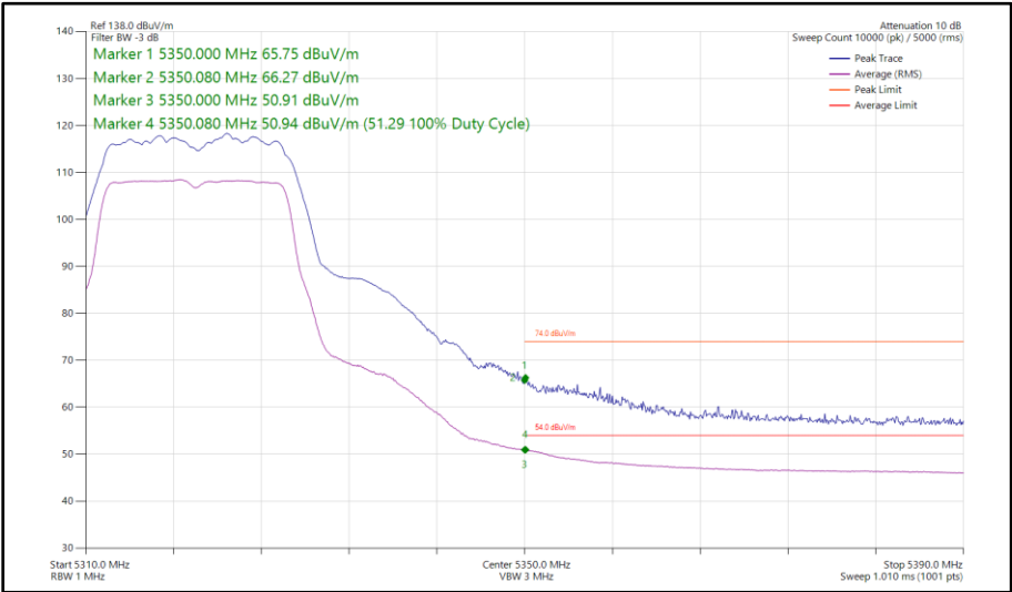
Figure 31 - 802.11a, SISO, Core 1 - 5320 MHz Band Edge Frequency 5350 MHz
