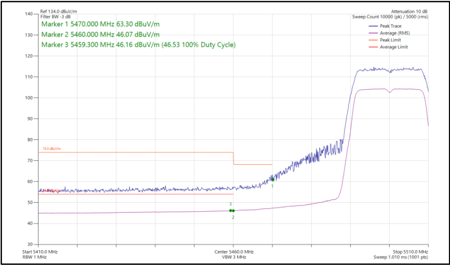
Figure 39 - 802.11n HT20, SISO, Core 1 - 5500 MHz Band Edge Frequency 5460 MHz
