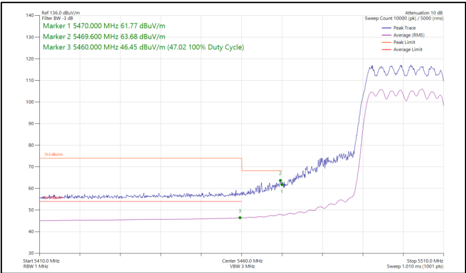
Figure 57 - 802.11ax HE20, SU, CDD, Core 0 - Core 1 - 5500 MHz Band Edge Frequency 5460 MHz
