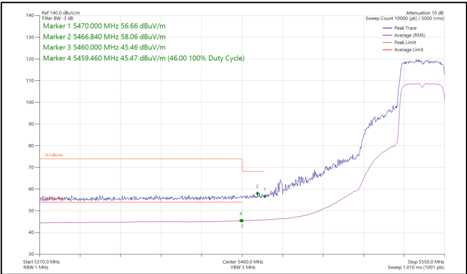
Figure 44 - 802.11ax HE20, SU, SISO, Core 1 - 5540 MHz Band Edge Frequency 5460 MHz
