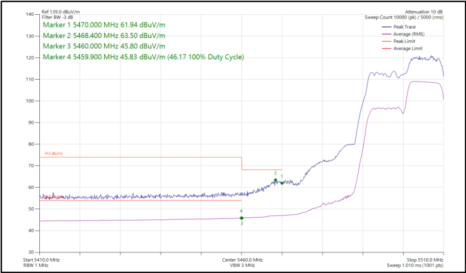
Figure 42 - 802.11ax HE20, RU 106-54, SISO, Core 1 - 5500 MHz Band Edge Frequency 5460 MHz
