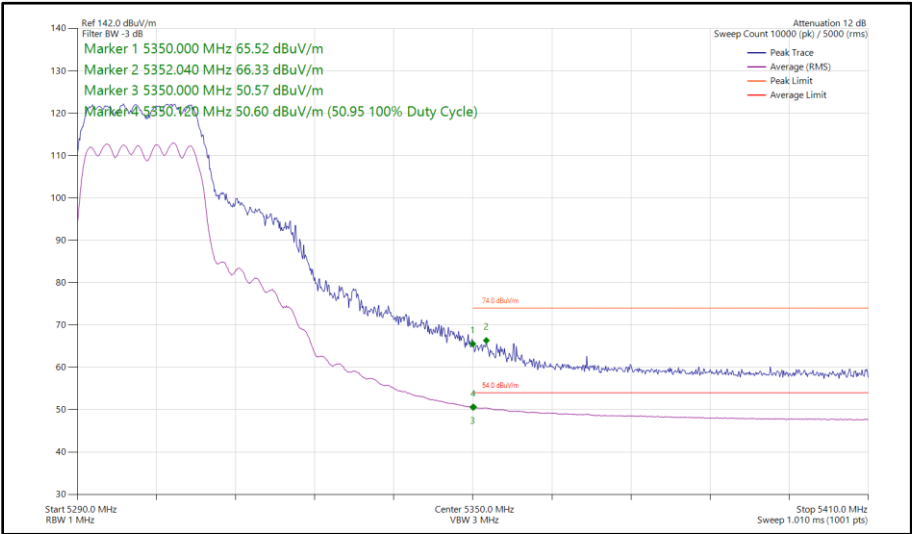
Figure 50 - 802.11n HT20, CDD, Core 0 - Core 1 - 5300 MHz Band Edge Frequency 5350 MHz
