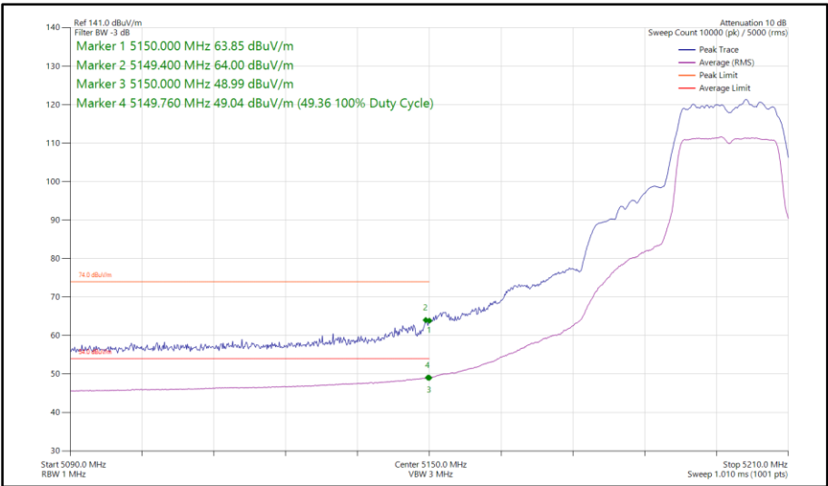
Figure 24 - 802.11a, SISO, Core 1 - 5200 MHz Band Edge Frequency 5150 MHz
