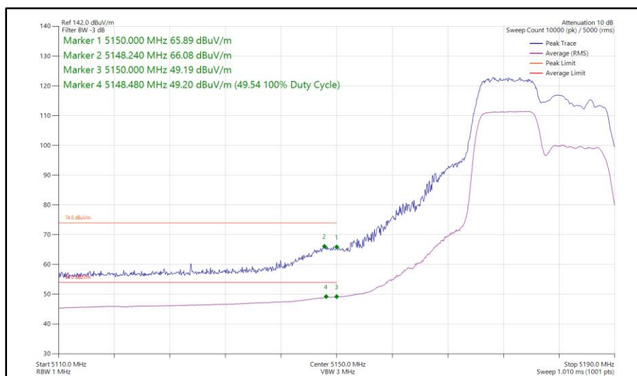
Figure 28 - 802.11ax HE20, RU 106-53, SISO, Core 1 - 5180 MHz Band Edge Frequency 5150 MHz
