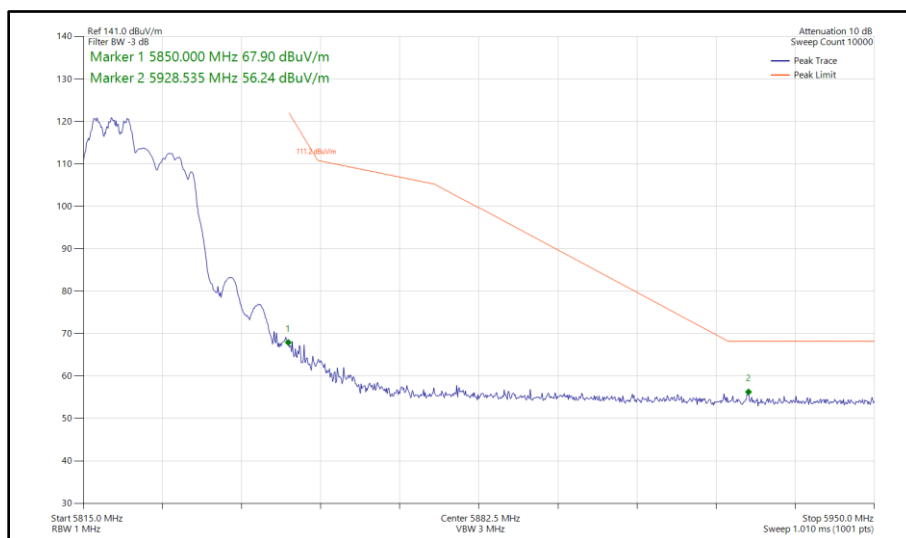
Figure 324 - 802.11ax HE20, RU 106-53, CDD, Core 0-1 - 5825 MHz Band Edge Frequency 5850 MHz
