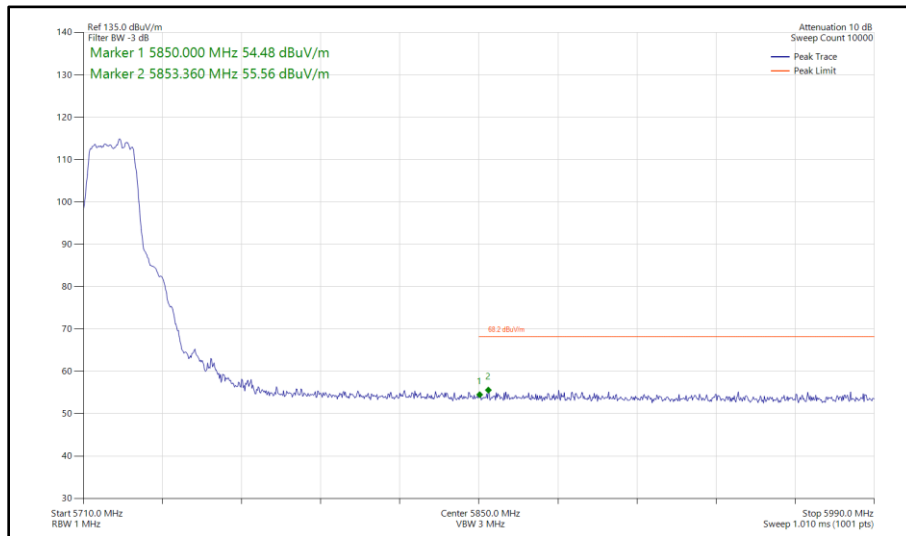
Figure 282 - 802.11a, SISO, Core 0 - 5720 MHz Band Edge Frequency 5850 MHz
