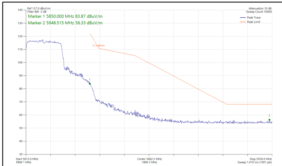
Figure 288 - 802.11ax HE20, SU, SISO, Core 0 - 5825 MHz Band Edge Frequency 5850 MHz
