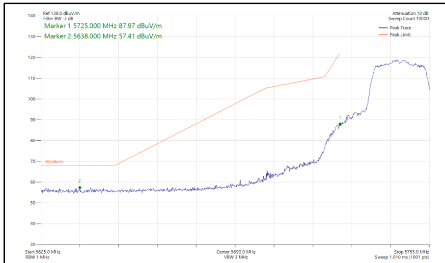
Figure 328 - 802.11n HT20, SDM, Core 0-1 - 5745 MHz Band Edge Frequency 5725 MHz
