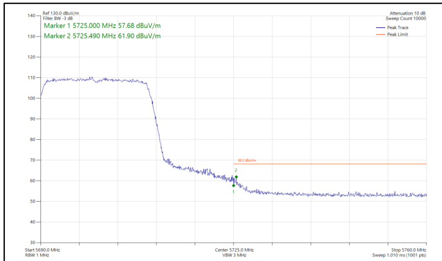
Figure 280 - 802.11ax HE20, SU, SISO, Core 0 - 5700 MHz Band Edge Frequency 5725 MHz
