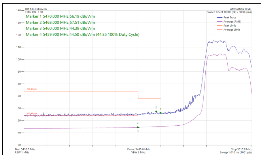
Figure 312 - 802.11ax HE20, RU 106-53, CDD, Core 0-1 - 5500 MHz Band Edge Frequency 5470 MHz
