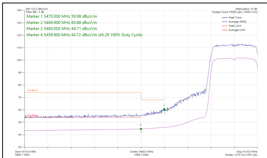
Figure 292 - 802.11ax HE20, SU, SISO, Core 1 - 5500 MHz Band Edge Frequency 5470 MHz
