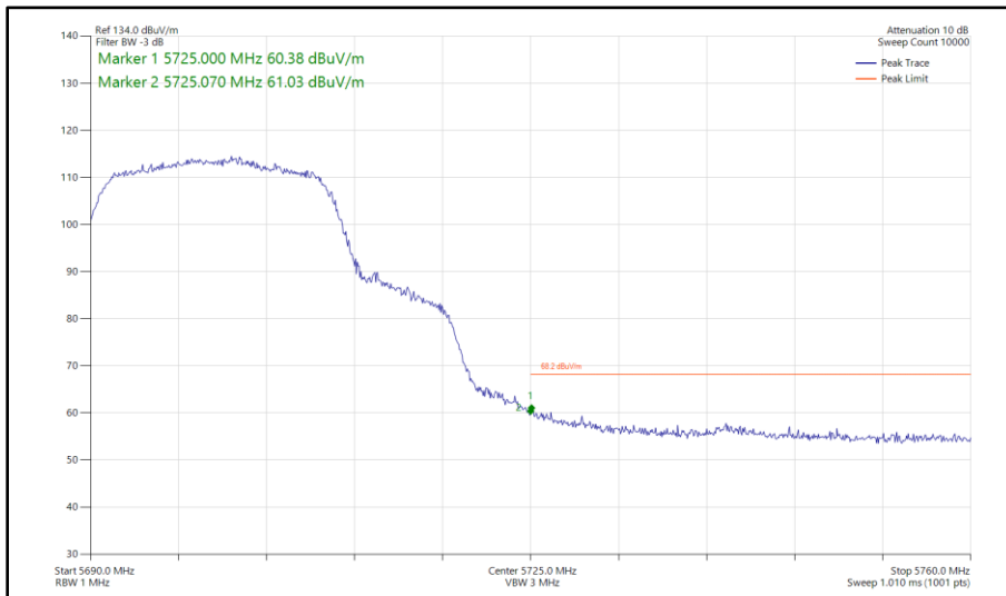
Figure 299 - 802.11n HT20, SISO, Core 1 - 5700 MHz Band Edge Frequency 5725 MHz
