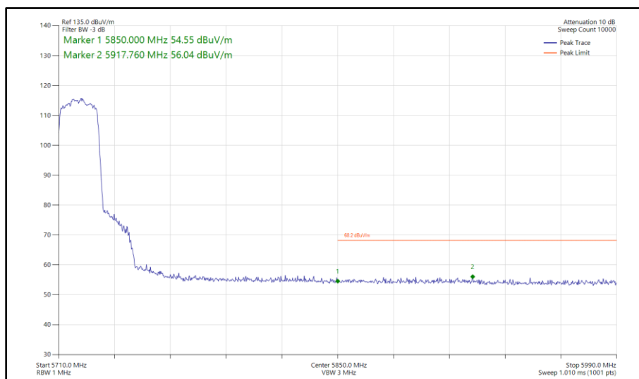
Figure 306 - 802.11ax HE20, SU, SISO, Core 1 - 5720 MHz Band Edge Frequency 5850 MHz
