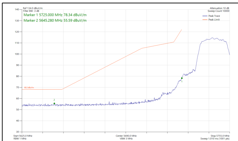
Figure 294 - 802.11a, SISO, Core 1 - 5745 MHz Band Edge Frequency 5725 MHz
