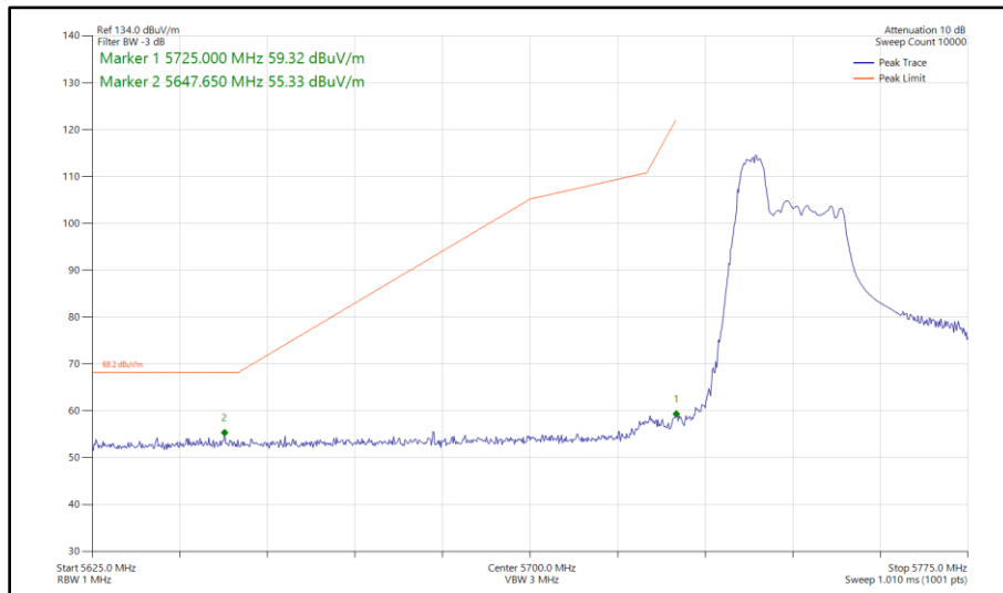
Figure 351 - 802.11ax HE40, RU 52-37, SISO, Core 0 - 5755 MHz Band Edge Frequency 5725 MHz
