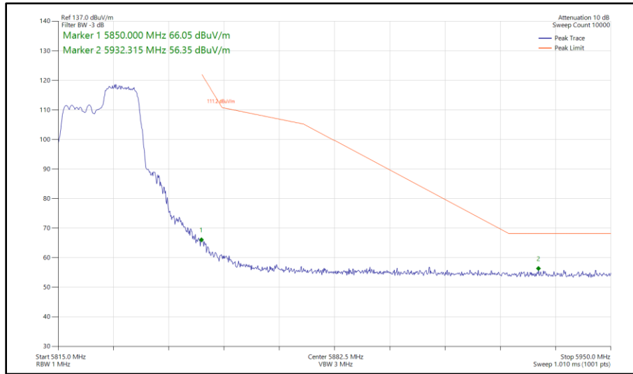
Figure 309 - 802.11ax HE20, RU 106-54, SISO, Core 1 - 5825 MHz Band Edge Frequency 5850 MHz
