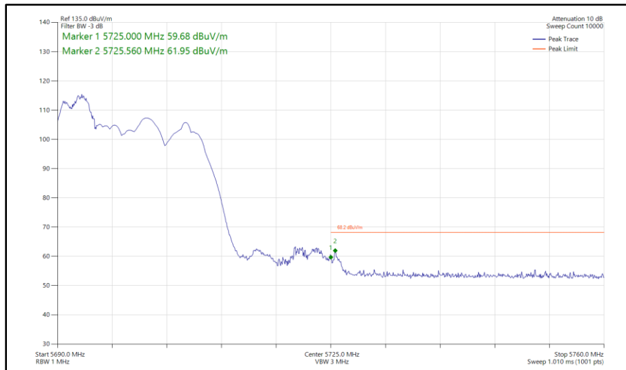
Figure 334 - 802.11ax HE20, RU 52-37, SDM, Core 0-1 - 5700 MHz Band Edge Frequency 5725 MHz
