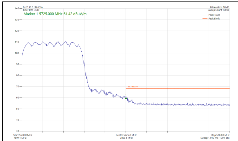
Figure 317 - 802.11ax HE20, SU, CDD, Core 0-1 - 5700 MHz Band Edge Frequency 5725 MHz
