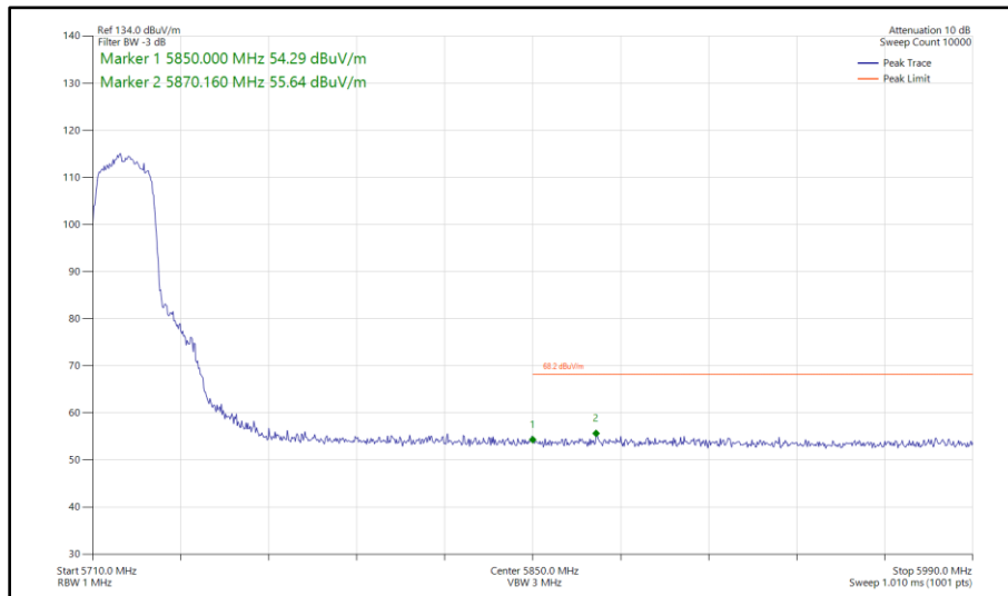
Figure 284 - 802.11n HT20, SISO, Core 0 - 5720 MHz Band Edge Frequency 5850 MHz
