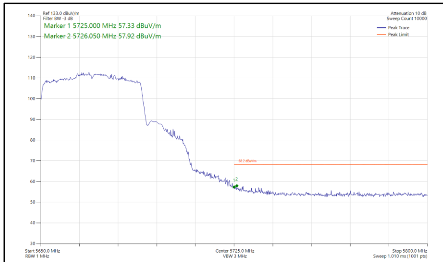
Figure 353 - 802.11ax HE40, SU, SISO, Core 0 - 5670 MHz Band Edge Frequency 5725 MHz
