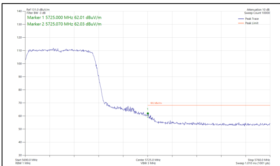
Figure 300 - 802.11ax HE20, SU, SISO, Core 1 - 5700 MHz Band Edge Frequency 5725 MHz
