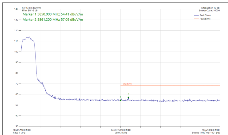
Figure 335 - 802.11n HT20, SDM, Core 0-1 - 5720 MHz Band Edge Frequency 5850 MHz
