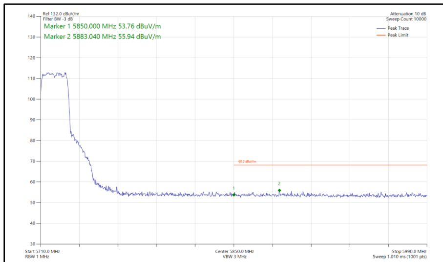
Figure 337 - 802.11ax HE20, SU, SDM, Core 0-1 - 5720 MHz Band Edge Frequency 5850 MHz
