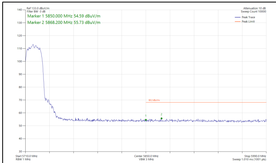
Figure 319 - 802.11n HT20, CDD, Core 0-1 - 5720 MHz Band Edge Frequency 5850 MHz
