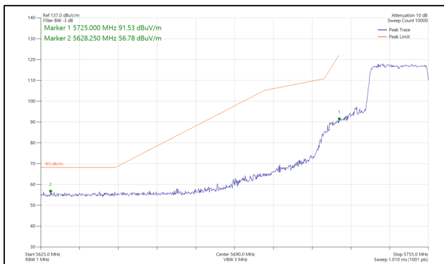
Figure 329 - 802.11ax HE20, SU, SDM, Core 0-1 - 5745 MHz Band Edge Frequency 5725 MHz
