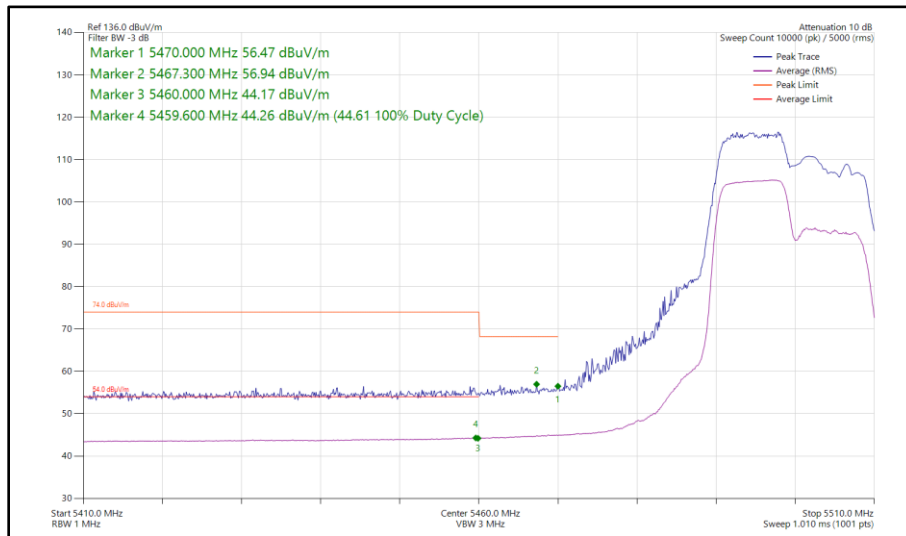
Figure 293 - 802.11ax HE20, RU 106-53, SISO, Core 1 - 5500 MHz Band Edge Frequency 5470 MHz
