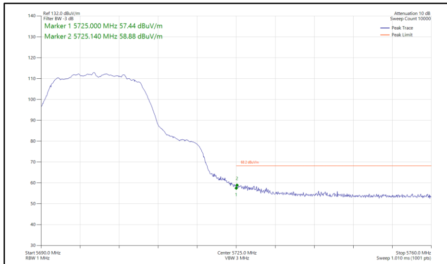
Figure 278 - 802.11a, SISO, Core 0 - 5700 MHz Band Edge Frequency 5725 MHz
