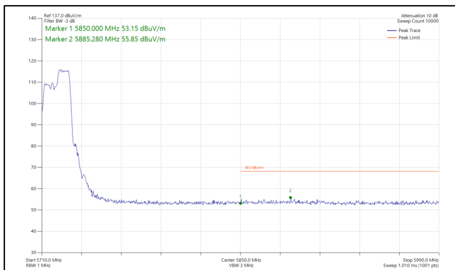
Figure 287 - 802.11ax HE20, RU 106-54, SISO, Core 0 - 5720 MHz Band Edge Frequency 5850 MHz
