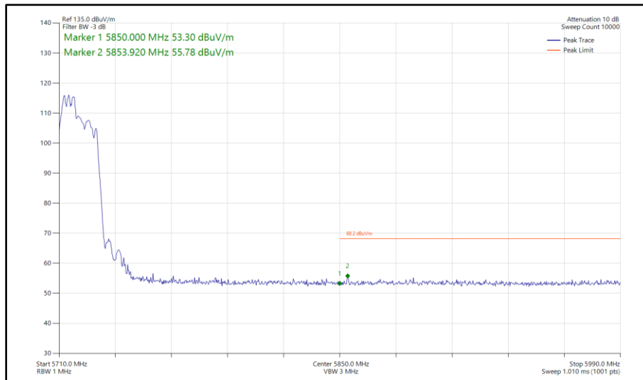
Figure 338 - 802.11ax HE20, RU 106-53, SDM, Core 0-1 - 5720 MHz Band Edge Frequency 5850 MHz
