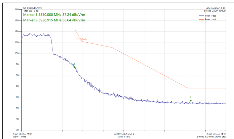
Figure 339 - 802.11ax HE20, SU, SDM, Core 0-1 - 5825 MHz Band Edge Frequency 5850 MHz
