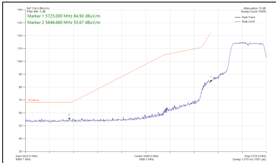
Figure 295 - 802.11n HT20, SISO, Core 1 - 5745 MHz Band Edge Frequency 5725 MHz
