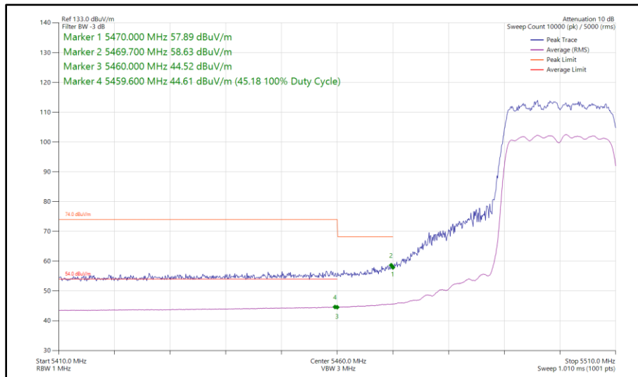
Figure 311 - 802.11ax HE20, SU, CDD, Core 0-1 - 5500 MHz Band Edge Frequency 5470 MHz
