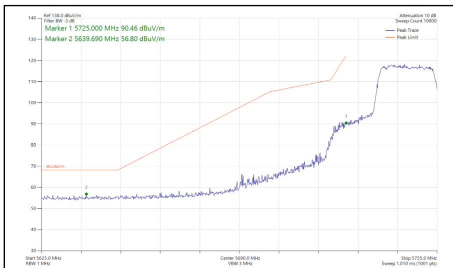
Figure 342 - 802.11ac VHT20, TxBF, Core 0-1 - 5745 MHz Band Edge Frequency 5725 MHz
