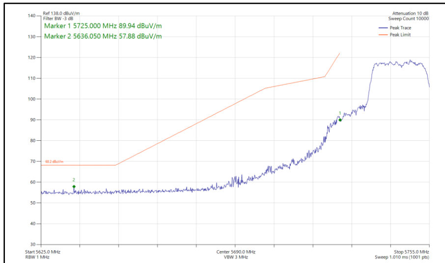
Figure 313 - 802.11n HT20, CDD, Core 0-1 - 5745 MHz Band Edge Frequency 5725 MHz
