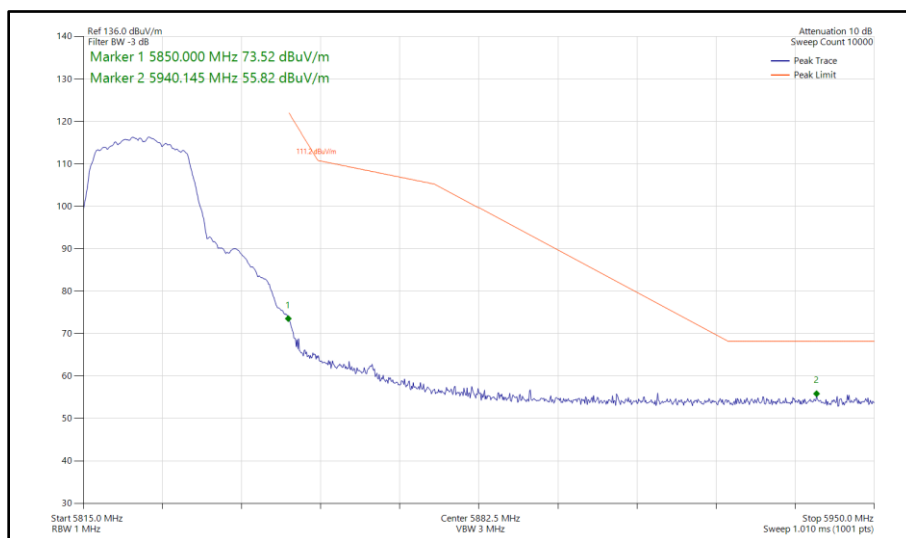
Figure 283 - 802.11a, SISO, Core 0 - 5825 MHz Band Edge Frequency 5850 MHz
