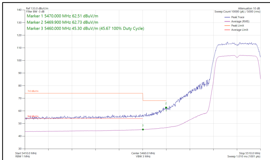
Figure 291 - 802.11n HT20, SISO, Core 1 - 5500 MHz Band Edge Frequency 5470 MHz
