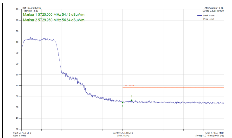
Figure 331 - 802.11n HT20, SDM, Core 0-1 - 5680 MHz Band Edge Frequency 5725 MHz
