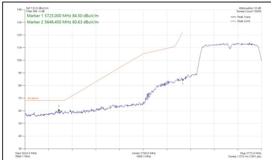
Figure 349 - 802.11n HT40, SISO, Core 0 - 5755 MHz Band Edge Frequency 5725 MHz
