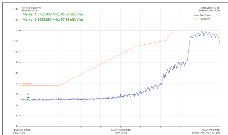
Figure 314 - 802.11ax HE20, SU, CDD, Core 0-1 - 5745 MHz Band Edge Frequency 5725 MHz
