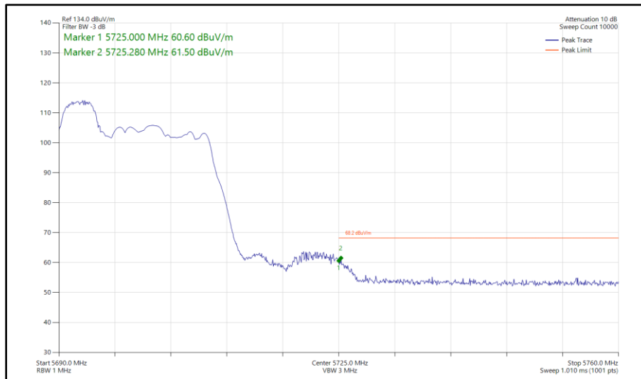
Figure 301 - 802.11ax HE20, RU 52-37, SISO, Core 1 - 5700 MHz Band Edge Frequency 5725 MHz
