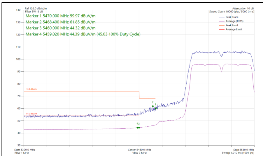
Figure 346 - 802.11n HT40, SISO, Core 0 - 5510 MHz Band Edge Frequency 5470 MHz
