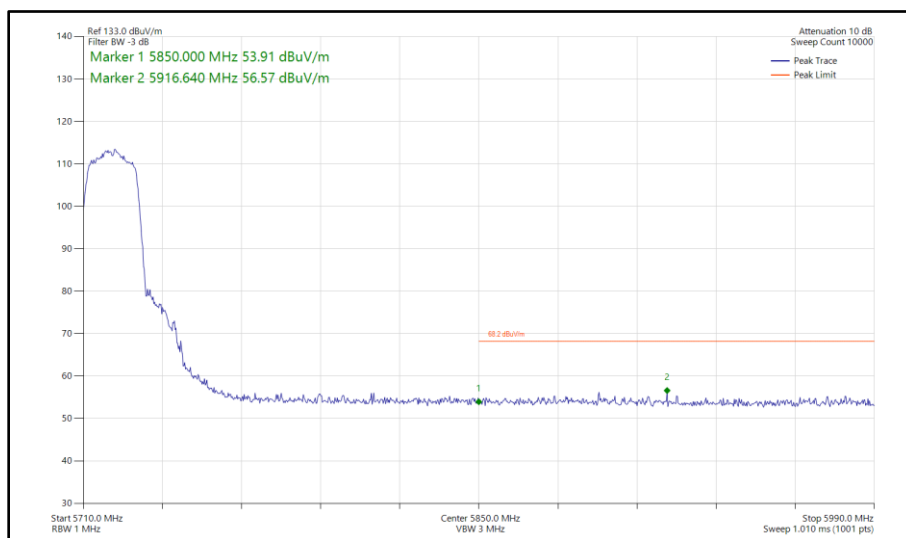
Figure 304 - 802.11n HT20, SISO, Core 1 - 5720 MHz Band Edge Frequency 5850 MHz
