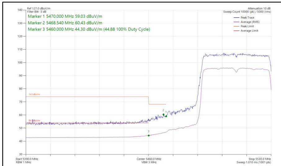
Figure 347 - 802.11ax HE40, SU, SISO, Core 0 - 5510 MHz Band Edge Frequency 5470 MHz
