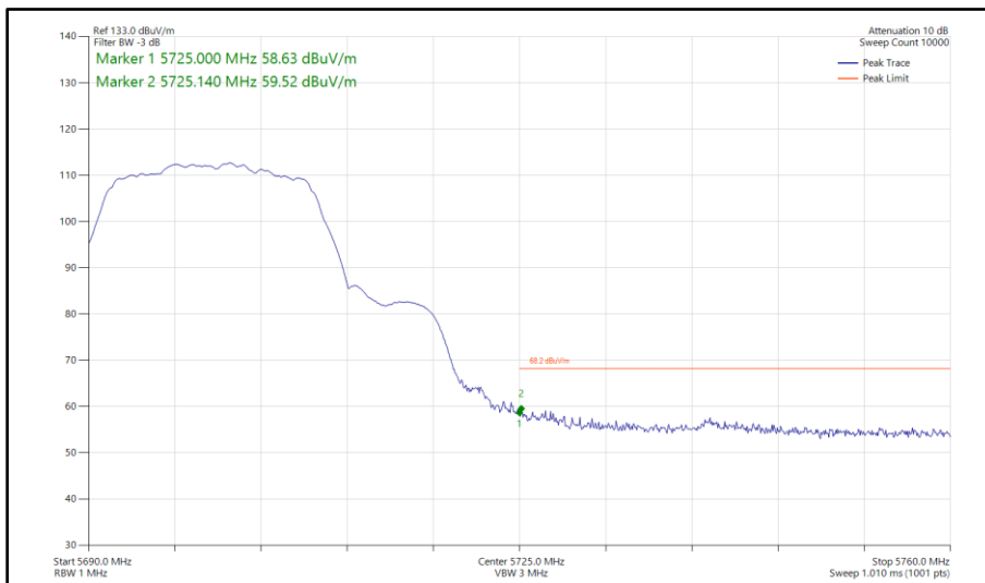
Figure 298 - 802.11a, SISO, Core 1 - 5700 MHz Band Edge Frequency 5725 MHz
