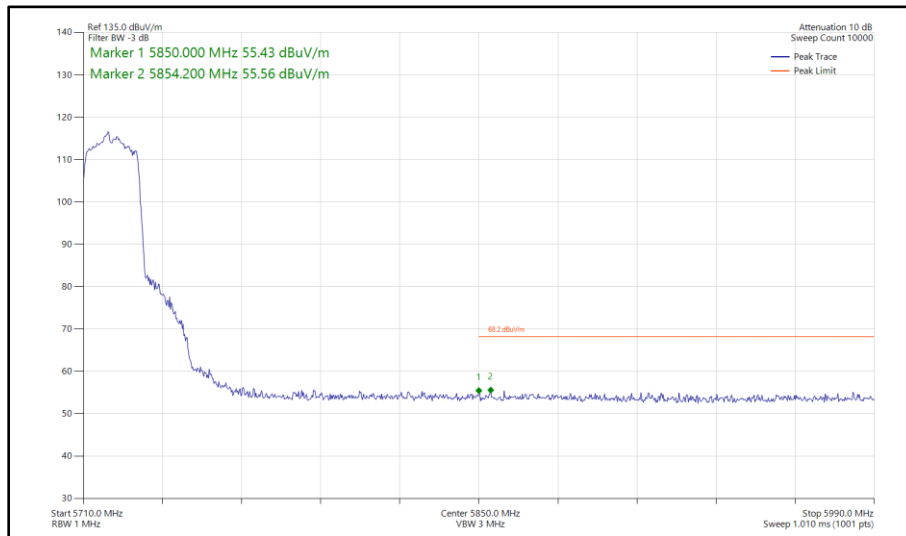
Figure 286 - 802.11ax HE20, SU, SISO, Core 0 - 5720 MHz Band Edge Frequency 5850 MHz
