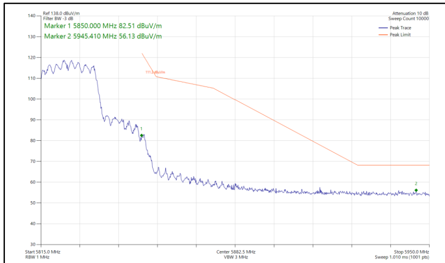
Figure 323 - 802.11ax HE20, SU, CDD, Core 0-1 - 5825 MHz Band Edge Frequency 5850 MHz
