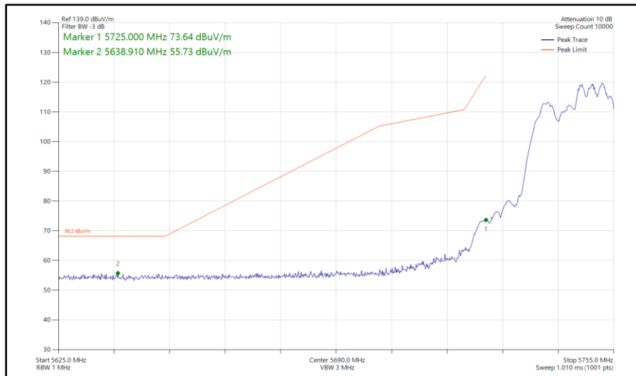
Figure 330 - 802.11ax HE20, RU 106-54, SDM, Core 0-1 - 5745 MHz Band Edge Frequency 5725 MHz
