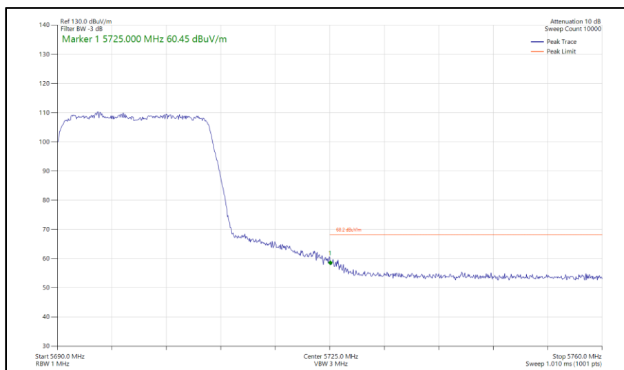
Figure 333 - 802.11ax HE20, SU, SDM, Core 0-1 - 5700 MHz Band Edge Frequency 5725 MHz
