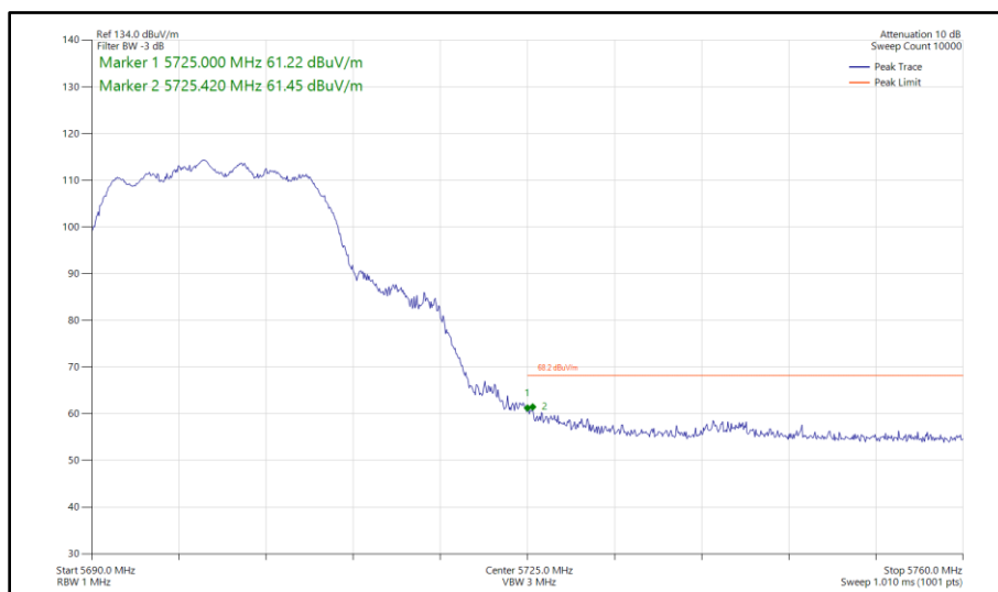
Figure 316 - 802.11n HT20, CDD, Core 0-1 - 5700 MHz Band Edge Frequency 5725 MHz
