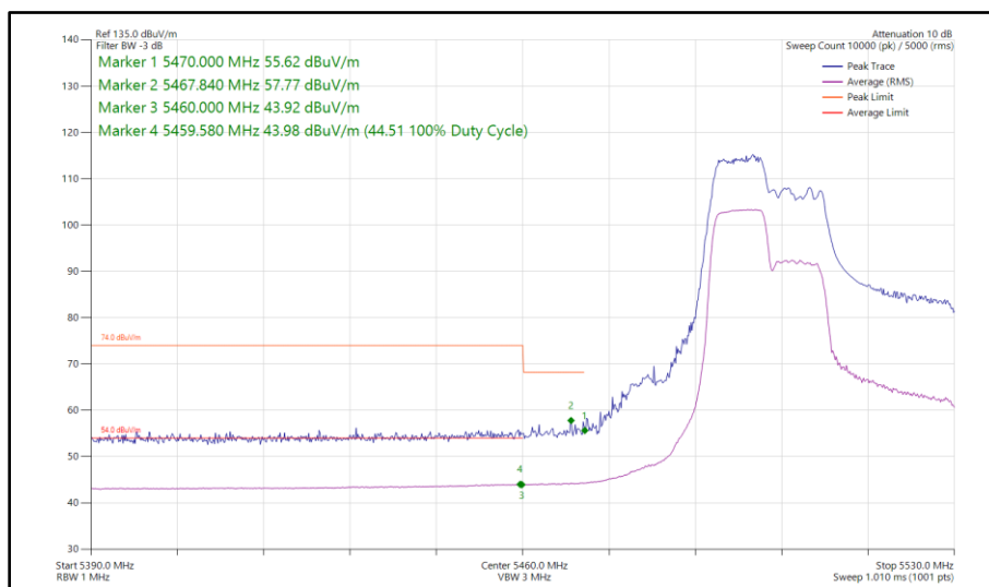
Figure 348 - 802.11ax HE40, RU 106-53, SISO, Core 0 - 5510 MHz Band Edge Frequency 5470 MHz
