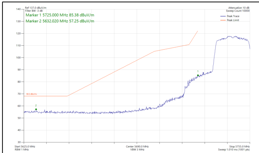
Figure 276 - 802.11ax HE20, SU, SISO, Core 0 - 5745 MHz Band Edge Frequency 5725 MHz
