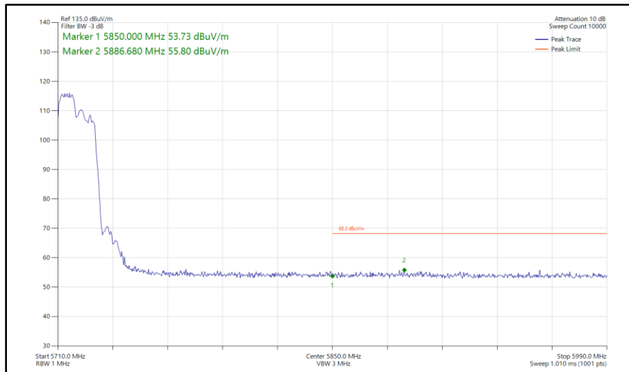
Figure 307 - 802.11ax HE20, RU 106-53, SISO, Core 1 - 5720 MHz Band Edge Frequency 5850 MHz
