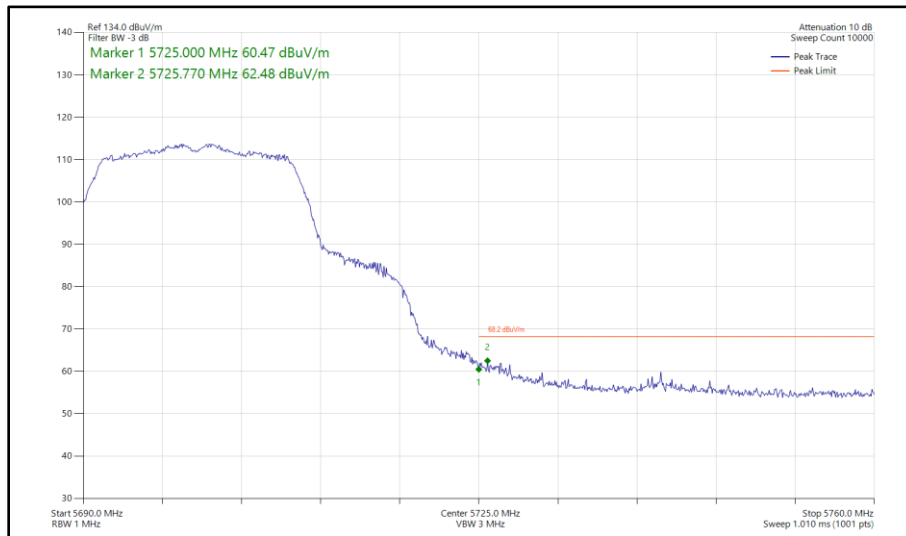
Figure 332 - 802.11n HT20, SDM, Core 0-1 - 5700 MHz Band Edge Frequency 5725 MHz
