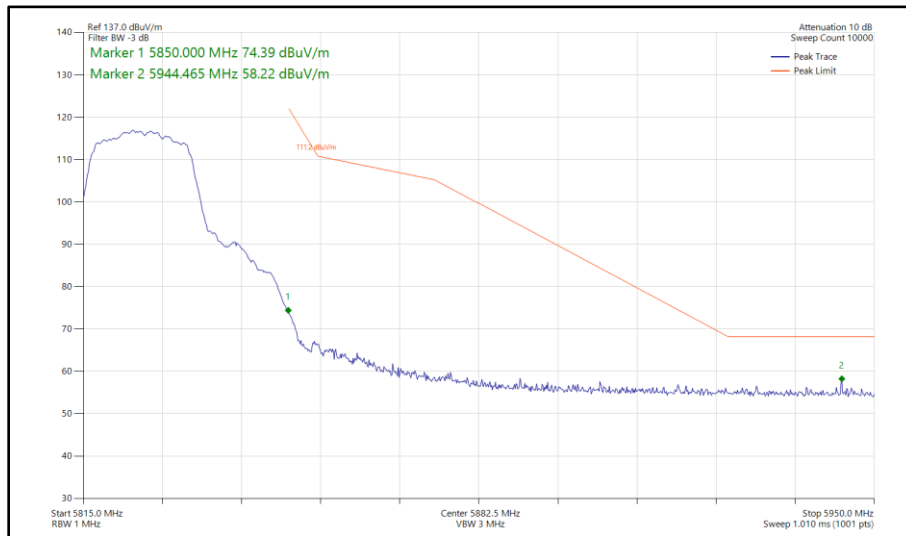
Figure 303 - 802.11a, SISO, Core 1 - 5825 MHz Band Edge Frequency 5850 MHz
