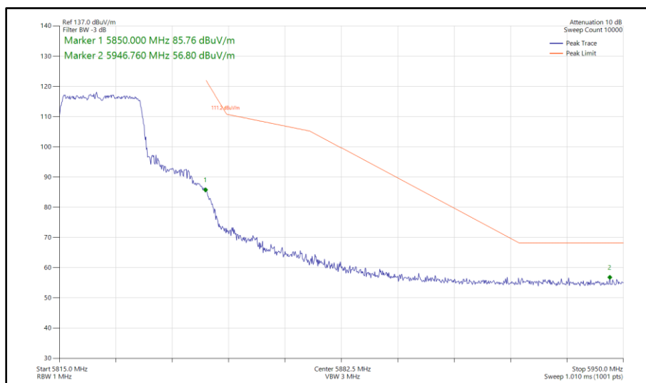
Figure 308 - 802.11ax HE20, SU, SISO, Core 1 - 5825 MHz Band Edge Frequency 5850 MHz
