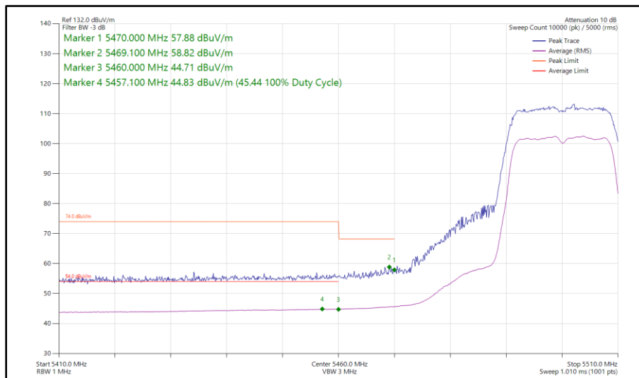
Figure 325 - 802.11n HT20, SDM, Core 0-1 - 5500 MHz Band Edge Frequency 5470 MHz
