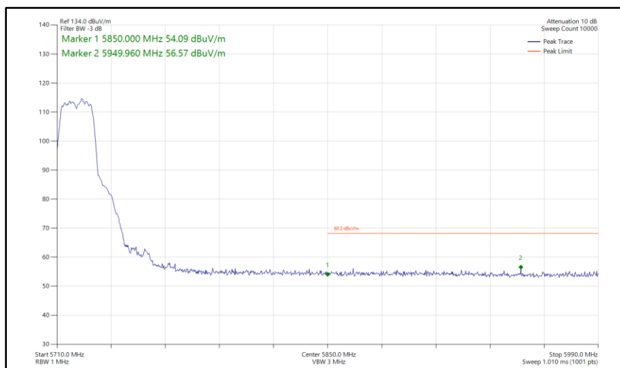
Figure 302 - 802.11a, SISO, Core 1 - 5720 MHz Band Edge Frequency 5850 MHz
