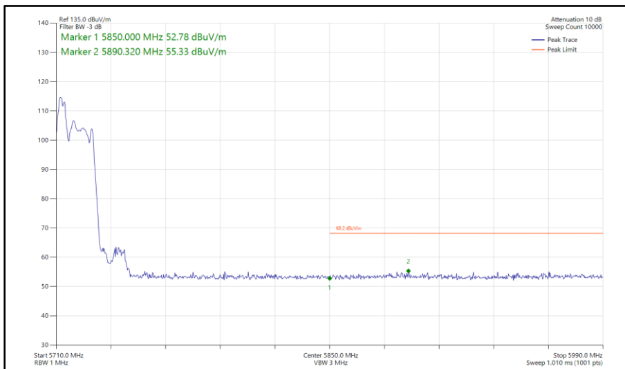
Figure 322 - 802.11ax HE20, RU 52-37, CDD, Core 0-1 - 5720 MHz Band Edge Frequency 5850 MHz
