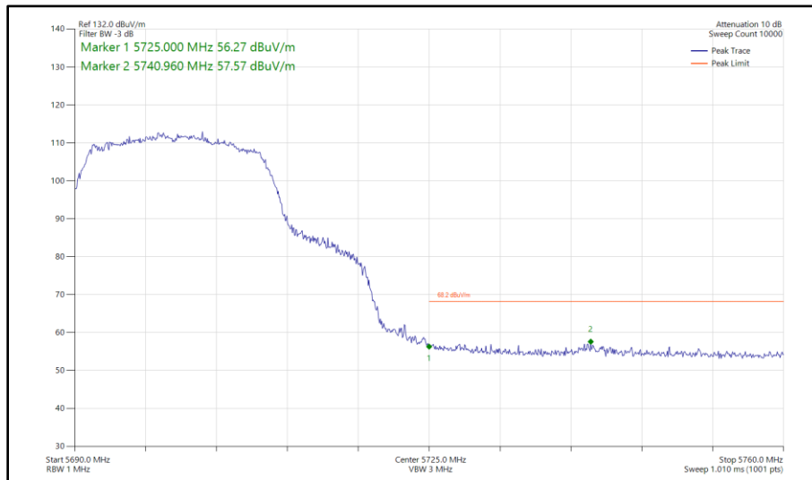
Figure 343 - 802.11ac VHT20, TxBF, Core 0-1 - 5700 MHz Band Edge Frequency 5725 MHz
