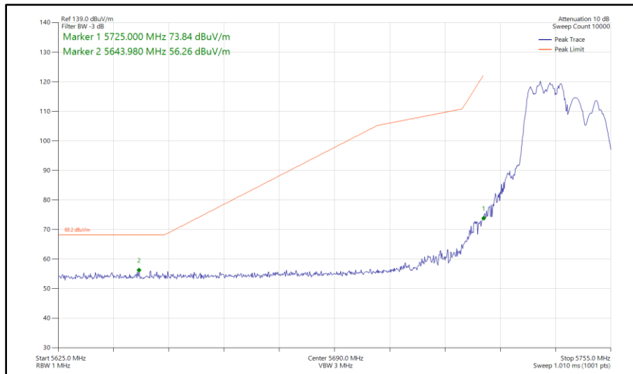
Figure 315 - 802.11ax HE20, RU 106-53, CDD, Core 0-1 - 5745 MHz Band Edge Frequency 5725 MHz
