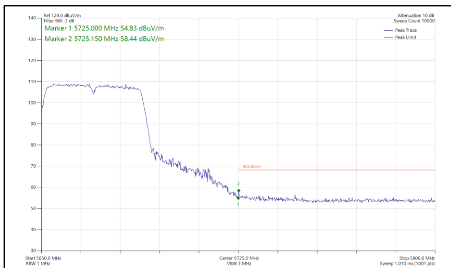
Figure 352 - 802.11n HT40, SISO, Core 0 - 5670 MHz Band Edge Frequency 5725 MHz
