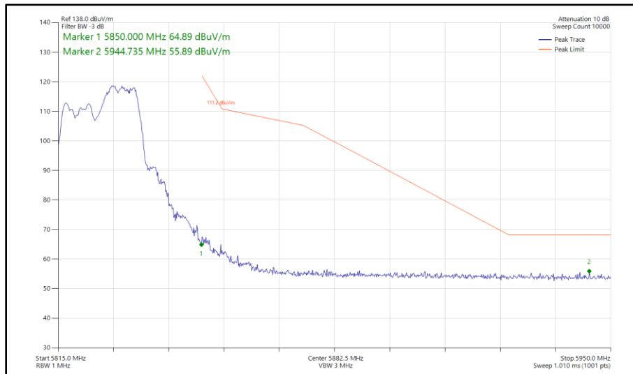
Figure 340 - 802.11ax HE20, RU 106-54, SDM, Core 0-1 - 5825 MHz Band Edge Frequency 5850 MHz
