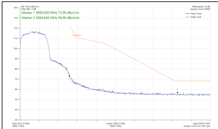
Figure 305 - 802.11n HT20, SISO, Core 1 - 5825 MHz Band Edge Frequency 5850 MHz
