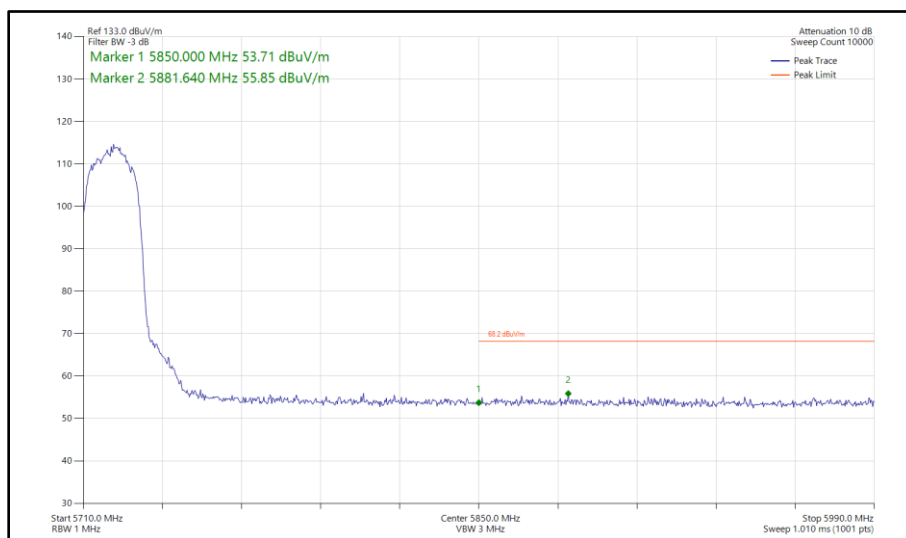
Figure 344 - 802.11ac VHT20, TxBF, Core 0-1 - 5720 MHz Band Edge Frequency 5850 MHz
