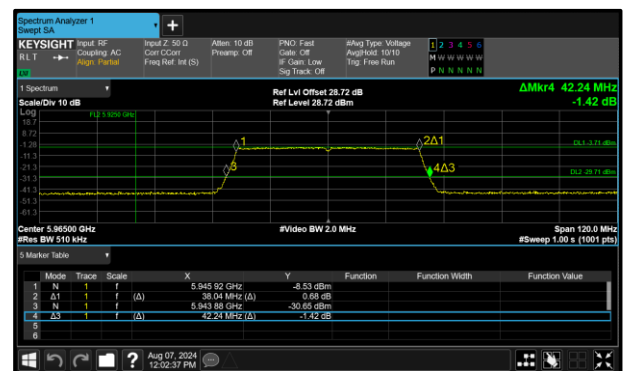
Figure 112 - 802.11ax HE40 SU LPI Maximum 26 dB OBW
