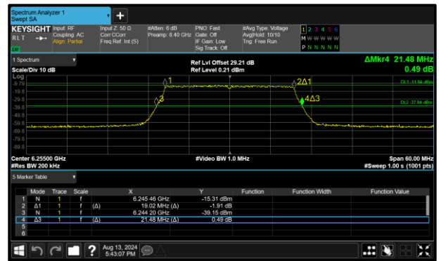
Figure 141 - 802.11ax HE20 SU VLP Maximum 26 dB OBW
