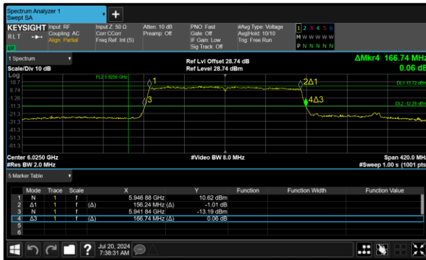
Figure 138 - 802.11ax HE160 SU SP Minimum 99% OBW
