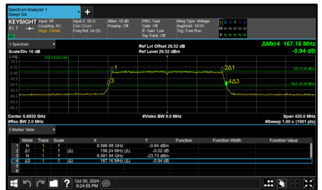
Figure 147 - 802.11ax HE160 SU VLP Maximum 26 dB OBW
