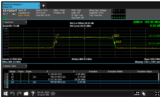
Figure 99 - 802.11ax HE160 SU VLP Minimum 26 dB OBW
