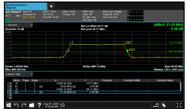
Figure 110 - 802.11ax HE20 SU LPI Maximum 26 dB OBW
