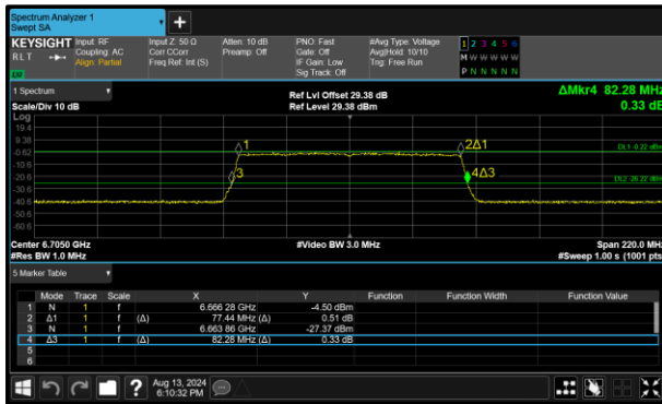
Figure 144 - 802.11ax HE80 SU VLP Minimum 26 dB OBW
