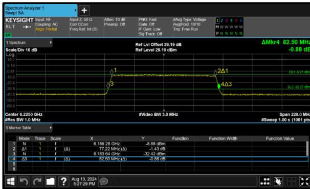
Figure 97 - 802.11ax HE80 SU VLP Minimum 26 dB OBW
