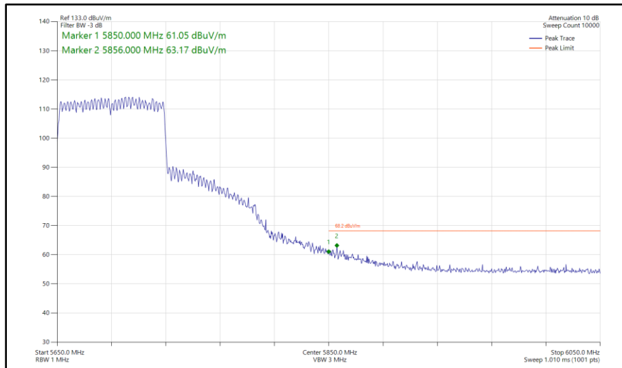
Figure 611 - 802.11ax HE80, SU, CDD, Core 0 - Core 1 - 5690 MHz Band Edge Frequency 5850 MHz
