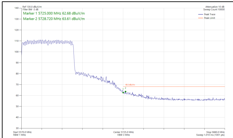
Figure 607 - 802.11ax HE80, SU, CDD, Core 0 - Core 1 - 5610 MHz Band Edge Frequency 5725 MHz
