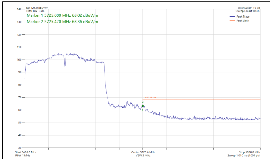
Figure 644 - 802.11ac VHT160, SISO, Core 1 - 5570 MHz Band Edge Frequency 5725 MHz
