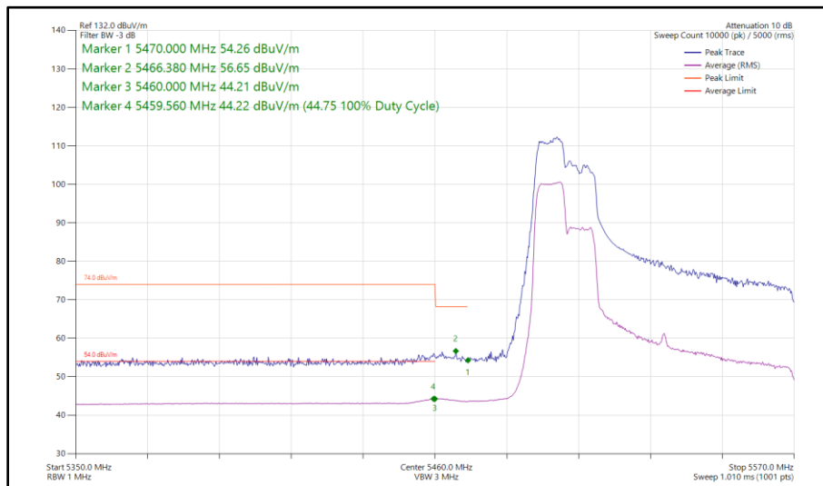
Figure 572 - 802.11ax HE80, RU 106-53, SISO, Core 0 - 5530 MHz Band Edge Frequency 5470 MHz
