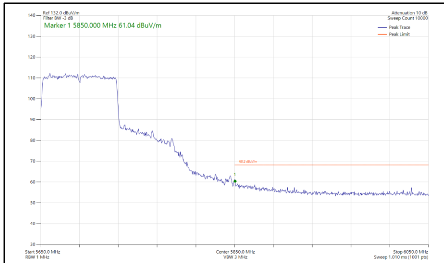
Figure 624 - 802.11ac VHT80, SDM, Core 0 - Core 1 - 5690 MHz Band Edge Frequency 5850 MHz
