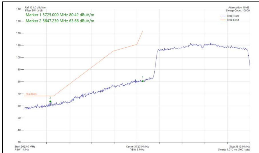
Figure 588 - 802.11ac VHT80, SISO, Core 1 - 5775 MHz Band Edge Frequency 5725 MHz
