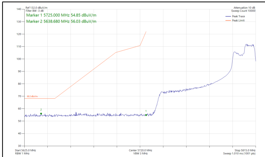
Figure 590 - 802.11ax HE80, RU 106-60, SISO, Core 1 - 5775 MHz Band Edge Frequency 5725 MHz
