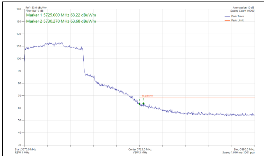
Figure 577 - 802.11ax HE80, SU, SISO, Core 0 - 5610 MHz Band Edge Frequency 5725 MHz
