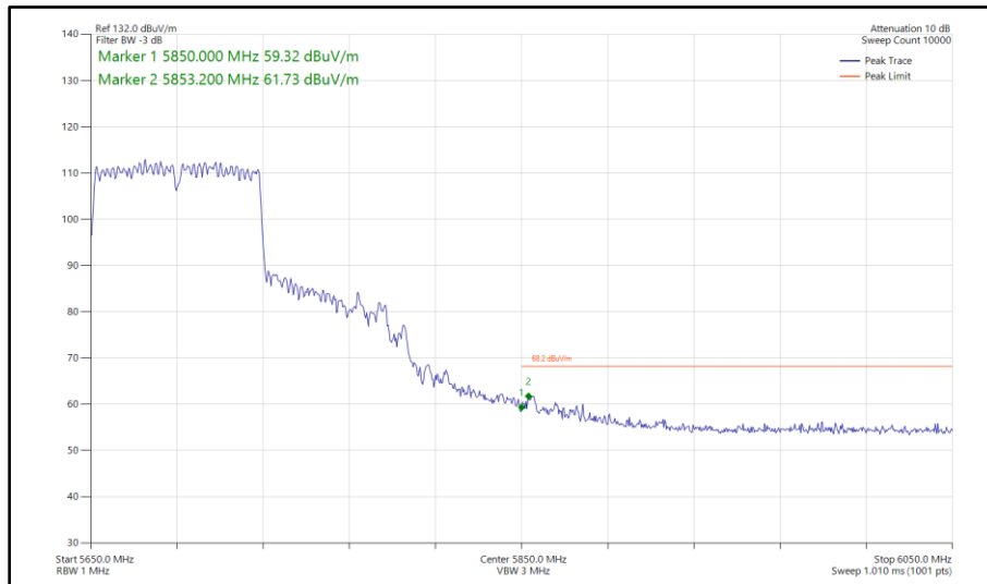
Figure 609 - 802.11ac VHT80, CDD, Core 0 - Core 1 - 5690 MHz Band Edge Frequency 5850 MHz
