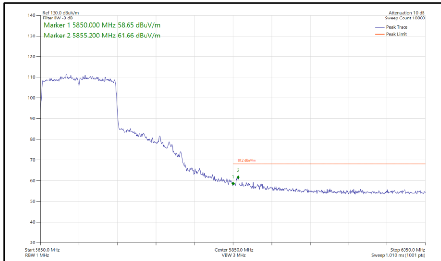
Figure 579 - 802.11ac VHT80, SISO, Core 0 - 5690 MHz Band Edge Frequency 5850 MHz
