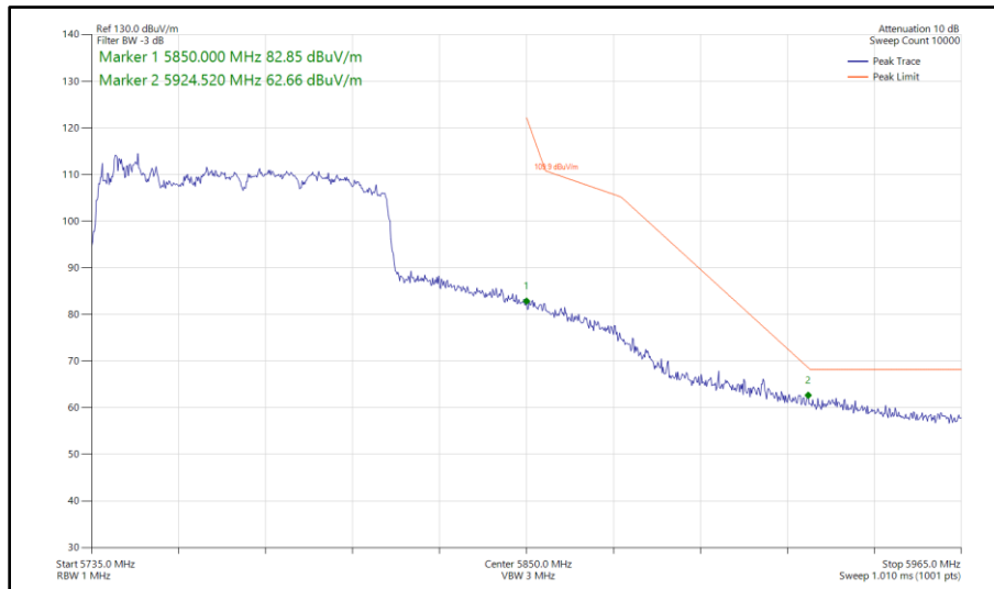
Figure 634 - 802.11ac VHT80, TxBF, Core 0 - Core 1 - 5775 MHz Band Edge Frequency 5850 MHz
