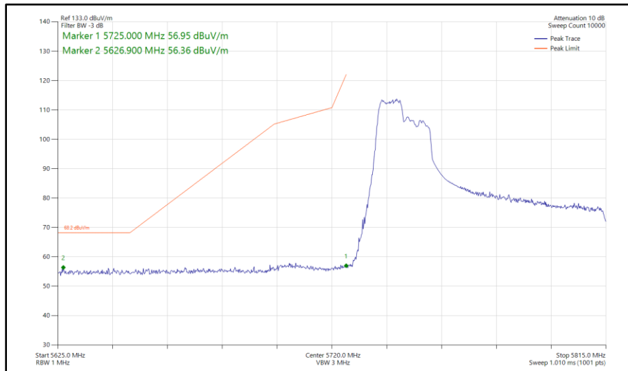
Figure 575 - 802.11ax HE80, RU 106-53, SISO, Core 0 - 5775 MHz Band Edge Frequency 5725 MHz
