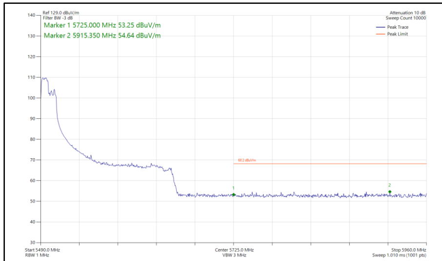
Figure 640 - 802.11ax HE160, RU 106-53P, SISO, Core 0 - 5570 MHz Band Edge Frequency 5725 MHz
