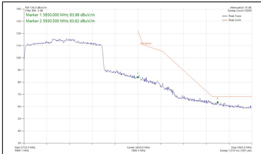
Figure 628 - 802.11ax HE80, SU, SDM, Core 0 - Core 1 - 5775 MHz Band Edge Frequency 5850 MHz
