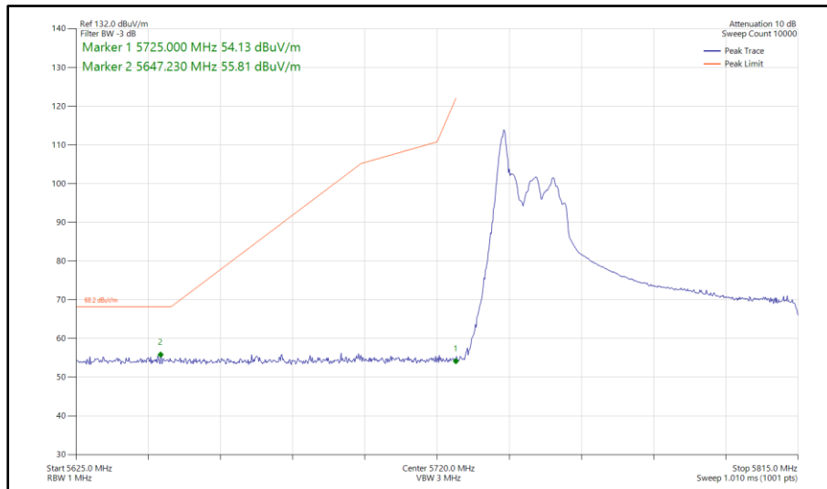
Figure 620 - 802.11ax HE80, RU 26-0, SDM, Core 0 - Core 1 - 5775 MHz Band Edge Frequency 5725 MHz
