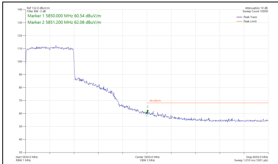
Figure 581 - 802.11ax HE80, SU, SISO, Core 0 - 5690 MHz Band Edge Frequency 5850 MHz
