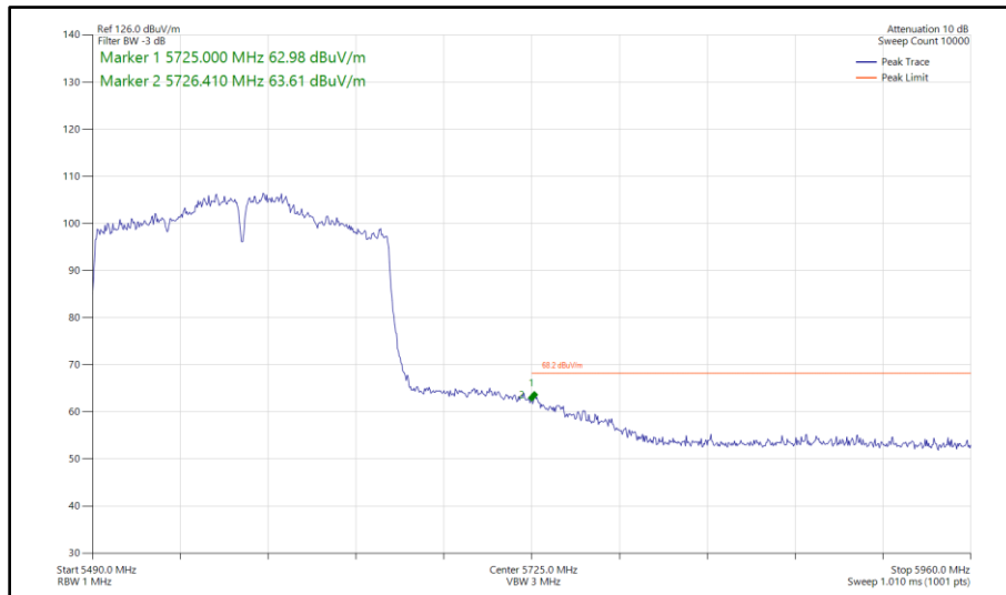
Figure 638 - 802.11ac VHT160, SISO, Core 0 - 5570 MHz Band Edge Frequency 5725 MHz
