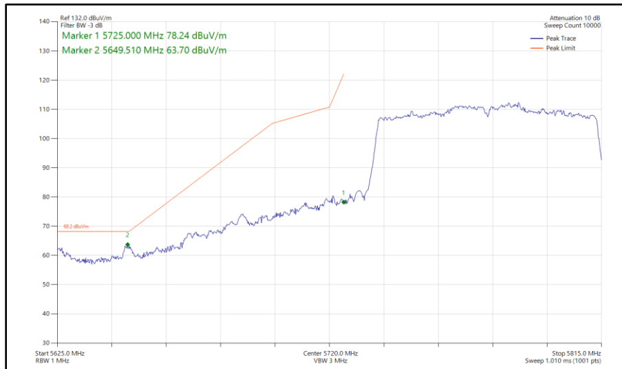
Figure 618 - 802.11ac VHT80, SDM, Core 0 - Core 1 - 5775 MHz Band Edge Frequency 5725 MHz
