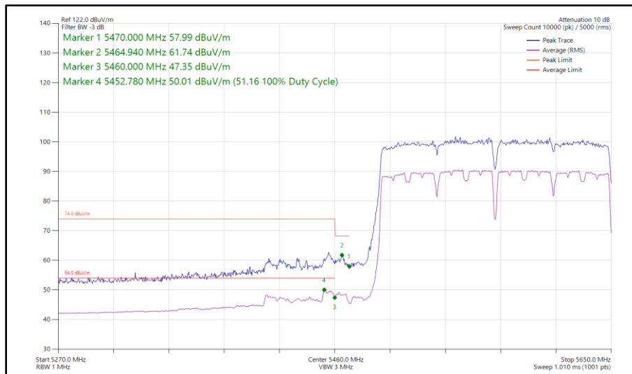
Figure 635 - 802.11ac VHT160, SISO, Core 0 - 5570 MHz Band Edge Frequency 5470 MHz
