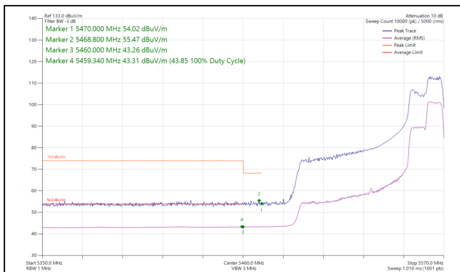
Figure 587 - 802.11ax HE80, RU 106-60, SISO, Core 1 - 5530 MHz Band Edge Frequency 5470 MHz
