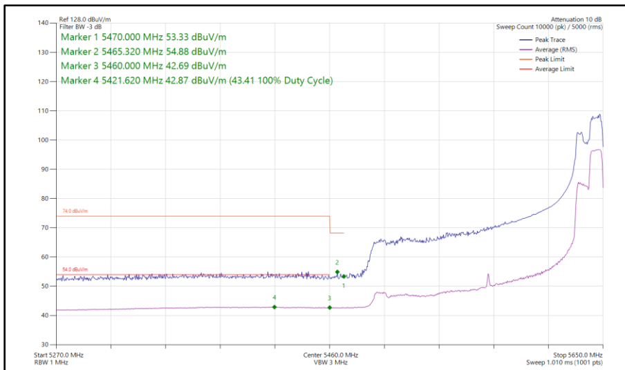
Figure 643 - 802.11ax HE160, RU 106-60S, SISO, Core 1 - 5570 MHz Band Edge Frequency 5470 MHz
