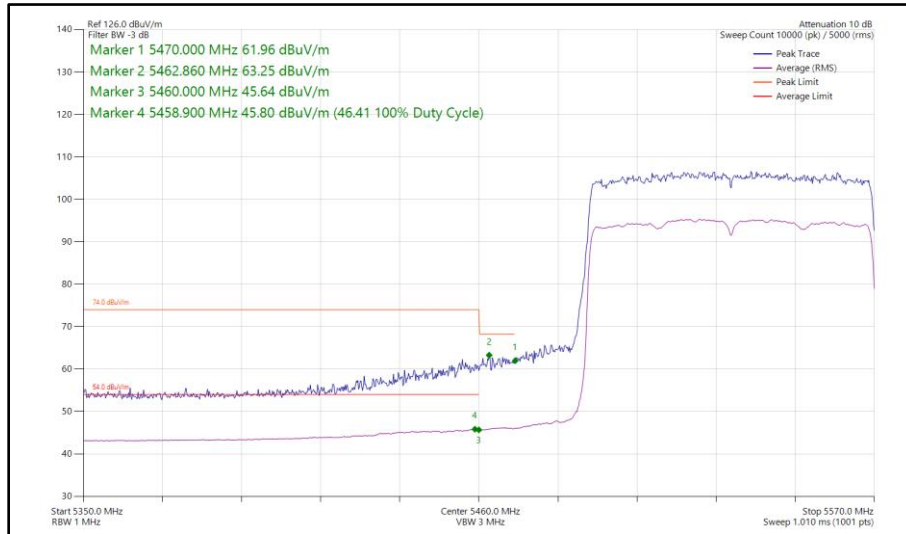
Figure 571 - 802.11ax HE80, SU, SISO, Core 0 - 5530 MHz Band Edge Frequency 5470 MHz
