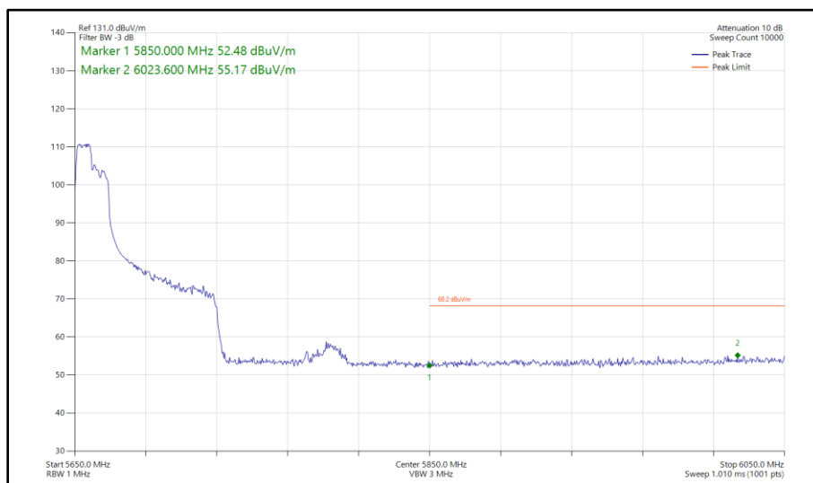
Figure 597 - 802.11ax HE80, RU 106-53, SISO, Core 1 - 5690 MHz Band Edge Frequency 5850 MHz
