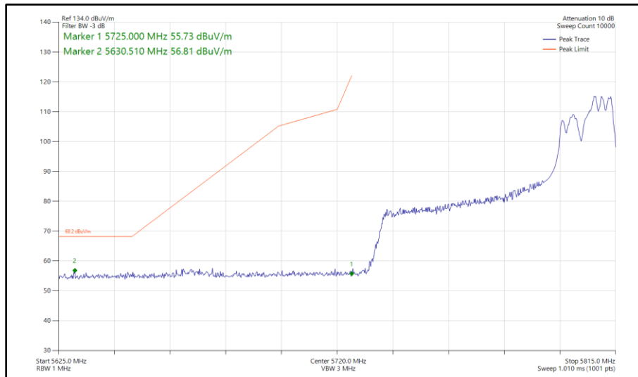
Figure 605 - 802.11ax HE80, RU 106-60, CDD, Core 0 - Core 1 - 5775 MHz Band Edge Frequency 5725 MHz
