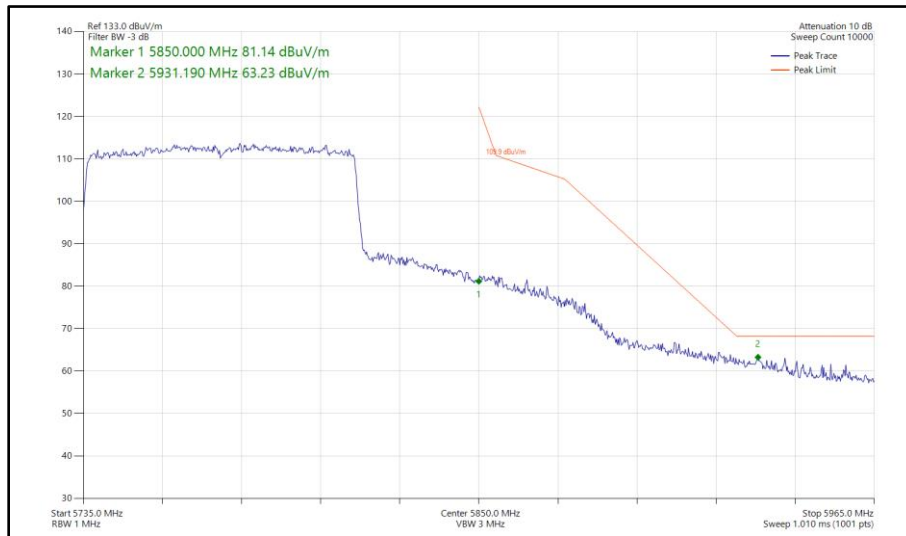
Figure 583 - 802.11ax HE80, SU, SISO, Core 0 - 5775 MHz Band Edge Frequency 5850 MHz
