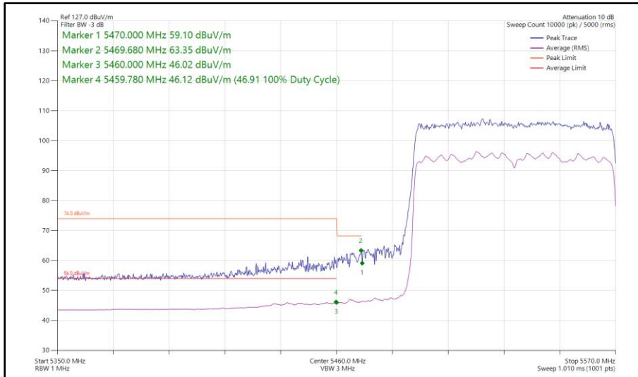
Figure 616 - 802.11ax HE80, SU, SDM, Core 0 - Core 1 - 5530 MHz Band Edge Frequency 5470 MHz
