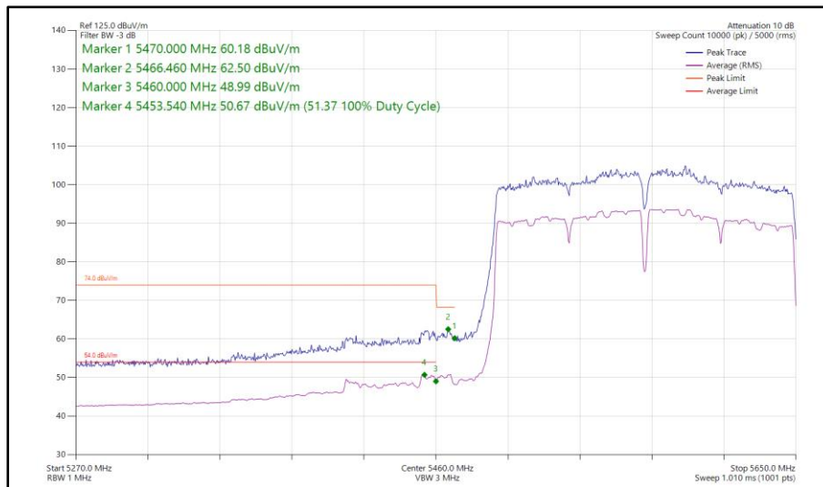
Figure 641 - 802.11ac VHT160, SISO, Core 1 - 5570 MHz Band Edge Frequency 5470 MHz
