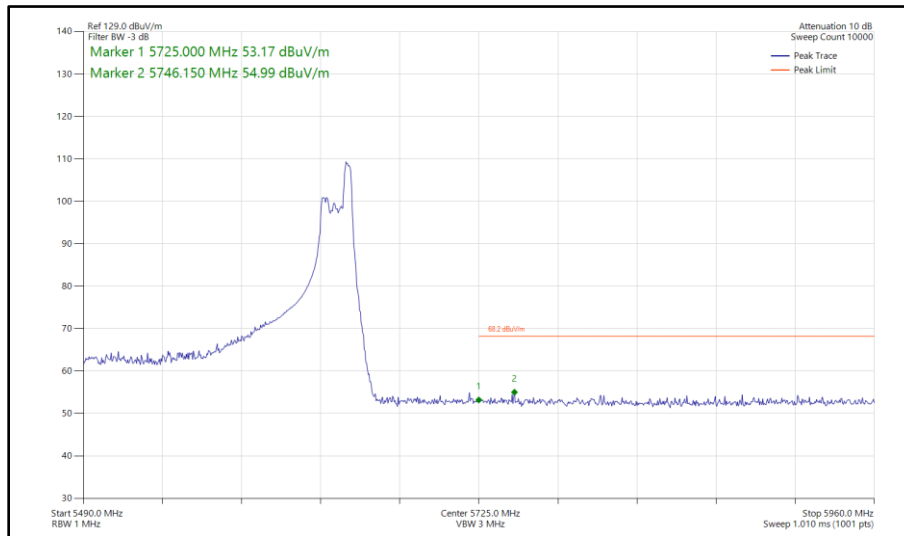
Figure 646 - 802.11ax HE160, RU 52-52S, SISO, Core 1 - 5570 MHz Band Edge Frequency 5725 MHz
