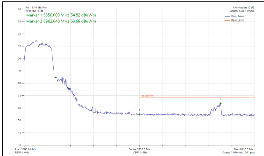
Figure 568 - 802.11ac VHT40, TxBF, Core 0 - Core 1 - 5710 MHz Band Edge Frequency 5850 MHz
