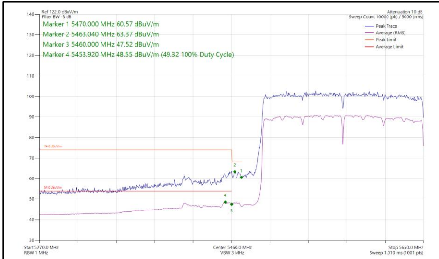
Figure 642 - 802.11ax HE160, SU, SISO, Core 1 - 5570 MHz Band Edge Frequency 5470 MHz
