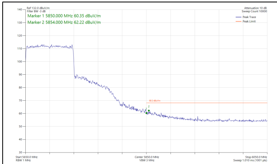
Figure 626 - 802.11ax HE80, SU, SDM, Core 0 - Core 1 - 5690 MHz Band Edge Frequency 5850 MHz
