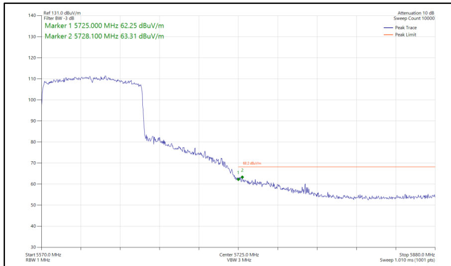
Figure 592 - 802.11ax HE80, SU, SISO, Core 1 - 5610 MHz Band Edge Frequency 5725 MHz
