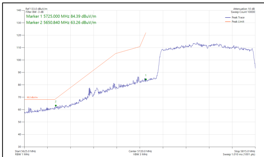
Figure 631 - 802.11ac VHT80, TxBF, Core 0 - Core 1 - 5775 MHz Band Edge Frequency 5725 MHz
