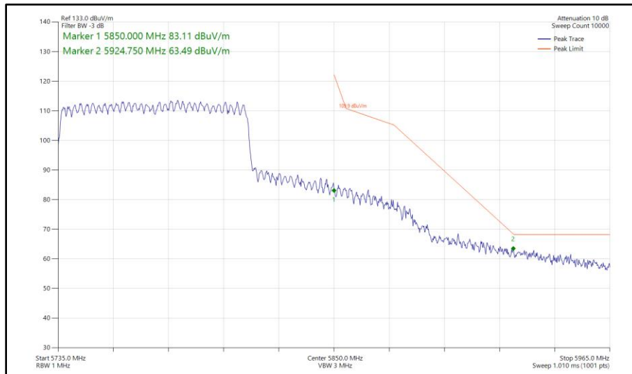
Figure 613 - 802.11ax HE80, SU, CDD, Core 0 - Core 1 - 5775 MHz Band Edge Frequency 5850 MHz
