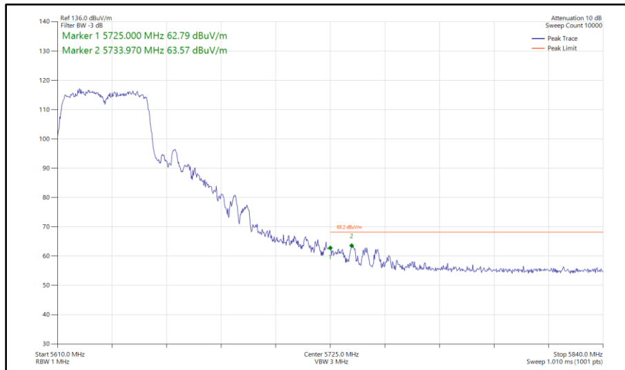
Figure 566 - 802.11ac VHT40, TxBF, Core 0 - Core 1 - 5630 MHz Band Edge Frequency 5725 MHz
