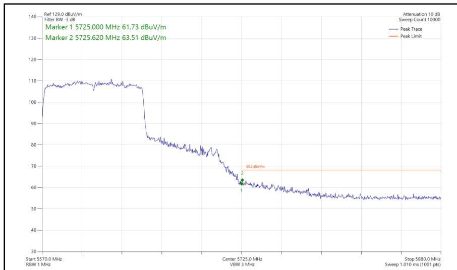
Figure 632 - 802.11ac VHT80, TxBF, Core 0 - Core 1 - 5610 MHz Band Edge Frequency 5725 MHz
