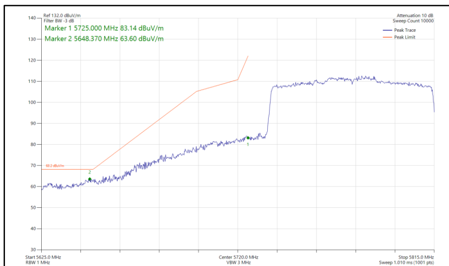
Figure 619 - 802.11ax HE80, SU, SDM, Core 0 - Core 1 - 5775 MHz Band Edge Frequency 5725 MHz
