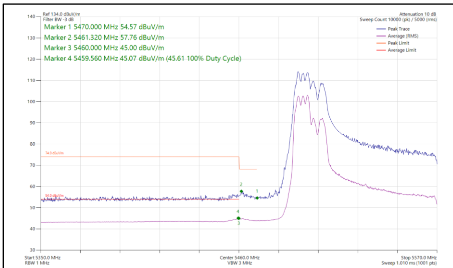
Figure 617 - 802.11ax HE80, RU 106-53, SDM, Core 0 - Core 1 - 5530 MHz Band Edge Frequency 5470 MHz
