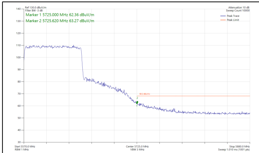
Figure 622 - 802.11ax HE80, SU, SDM, Core 0 - Core 1 - 5610 MHz Band Edge Frequency 5725 MHz
