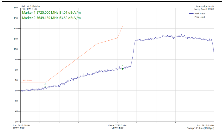
Figure 573 - 802.11ac VHT80, SISO, Core 0 - 5775 MHz Band Edge Frequency 5725 MHz
