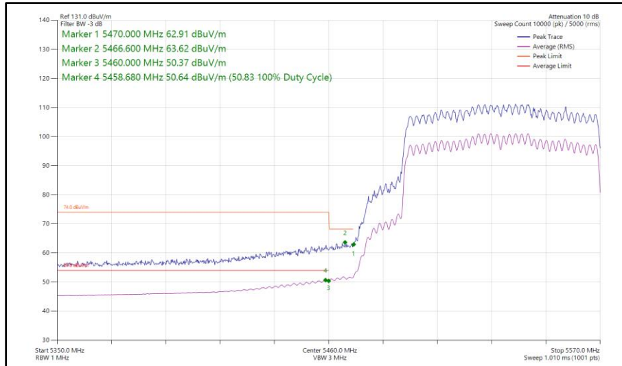
Figure 601 - 802.11ax HE80, SU, CDD, Core 0 - Core 1 - 5530 MHz Band Edge Frequency 5470 MHz
