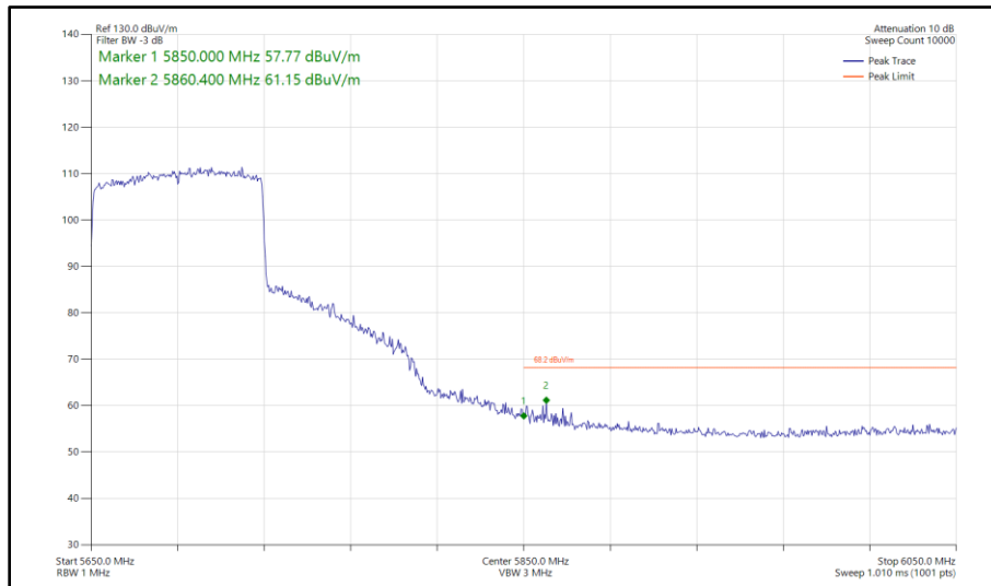
Figure 596 - 802.11ax HE80, SU, SISO, Core 1 - 5690 MHz Band Edge Frequency 5850 MHz
