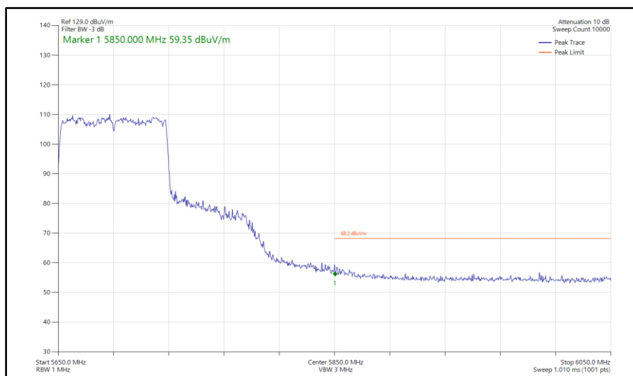
Figure 633 - 802.11ac VHT80, TxBF, Core 0 - Core 1 - 5690 MHz Band Edge Frequency 5850 MHz
