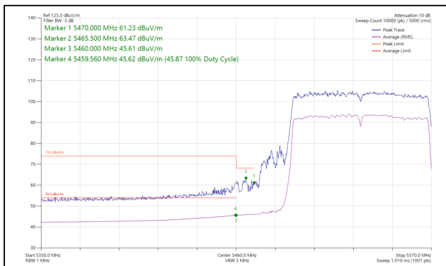
Figure 630 - 802.11ac VHT80, TxBF, Core 0 - Core 1 - 5530 MHz Band Edge Frequency 5470 MHz
