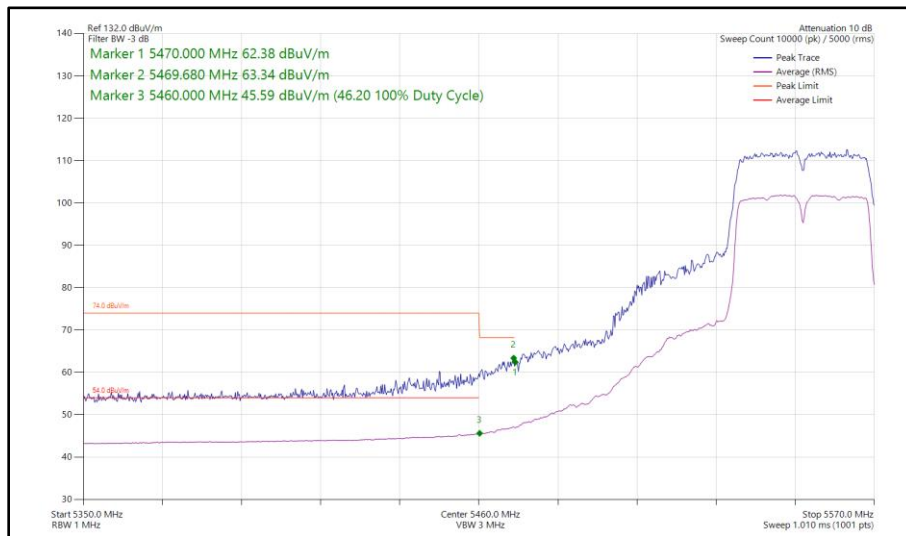
Figure 502 - 802.11n HT40, SISO, Core 1 - 5550 MHz Band Edge Frequency 5470 MHz
