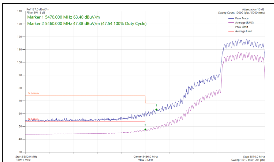
Figure 526 - 802.11ax HE40, SU, CDD, Core 0 - Core 1 - 5550 MHz Band Edge Frequency 5470 MHz
