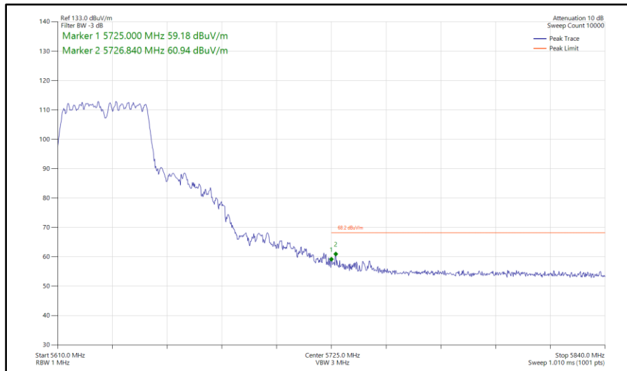
Figure 531 - 802.11n HT40, CDD, Core 0 - Core 1 - 5630 MHz Band Edge Frequency 5725 MHz
