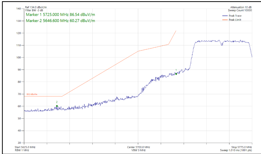
Figure 486 - 802.11n HT40, SISO, Core 0 - 5755 MHz Band Edge Frequency 5725 MHz
