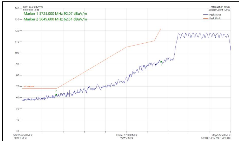
Figure 529 - 802.11ax HE40, SU, CDD, Core 0 - Core 1 - 5755 MHz Band Edge Frequency 5725 MHz
