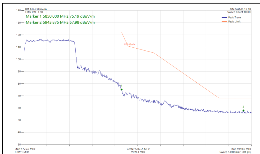
Figure 499 - 802.11ax HE40, SU, SISO, Core 0 - 5795 MHz Band Edge Frequency 5850 MHz
