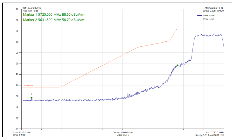
Figure 547 - 802.11n HT20, SDM, Core 0 - Core 1 - 5745 MHz Band Edge Frequency 5725 MHz
