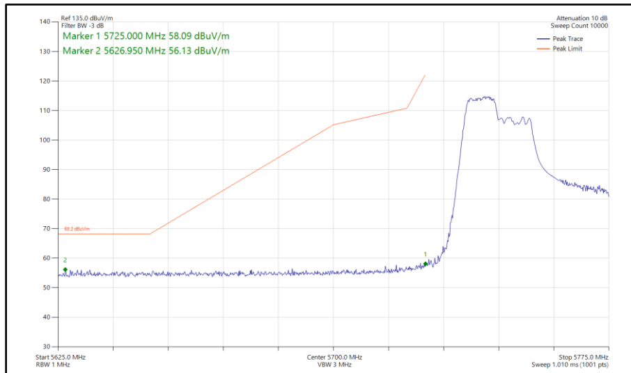
Figure 509 - 802.11ax HE40, RU 106-53, SISO, Core 1 - 5755 MHz Band Edge Frequency 5725 MHz
