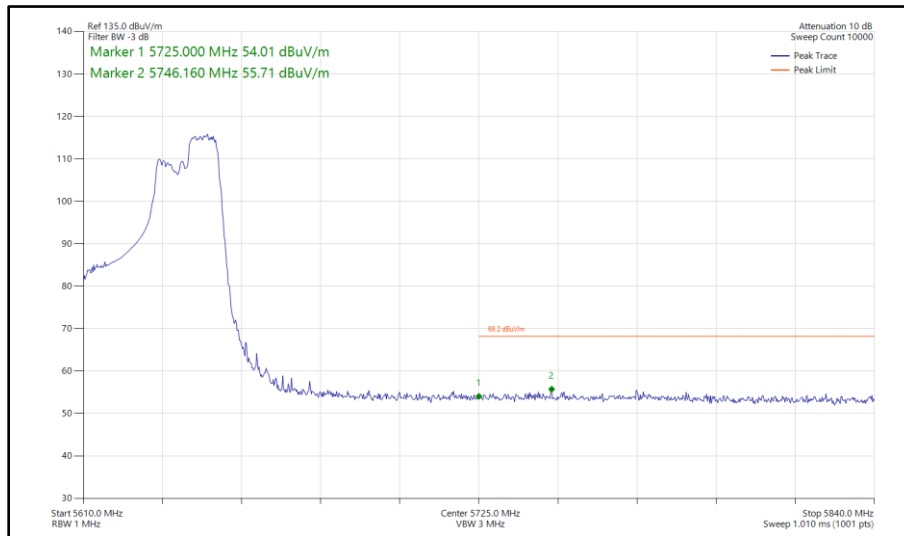
Figure 513 - 802.11ax HE40, RU 106-56, SISO, Core 1 - 5630 MHz Band Edge Frequency 5725 MHz
