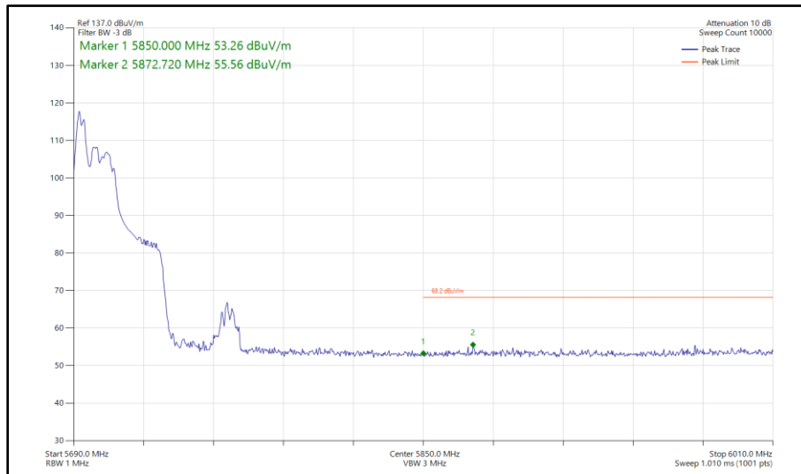
Figure 539 - 802.11ax HE40, RU 52-37, CDD, Core 0 - Core 1 - 5710 MHz Band Edge Frequency 5850 MHz
