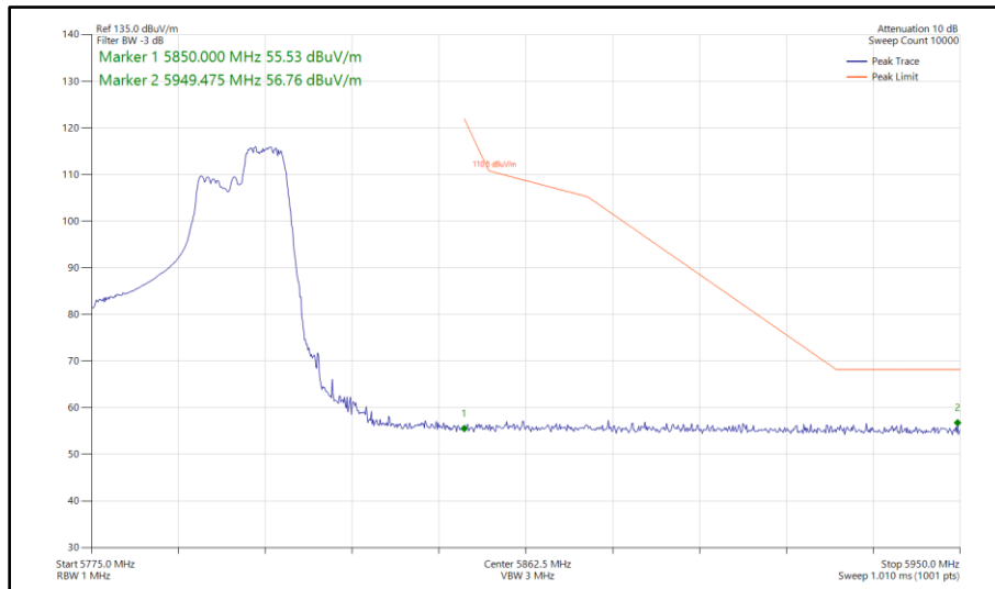
Figure 521 - 802.11ax HE40, RU 106-56, SISO, Core 1 - 5795 MHz Band Edge Frequency 5850 MHz
