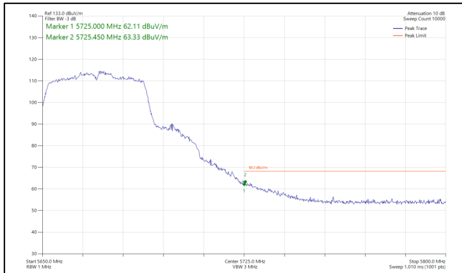
Figure 511 - 802.11n HT40, SISO, Core 1 - 5670 MHz Band Edge Frequency 5725 MHz
