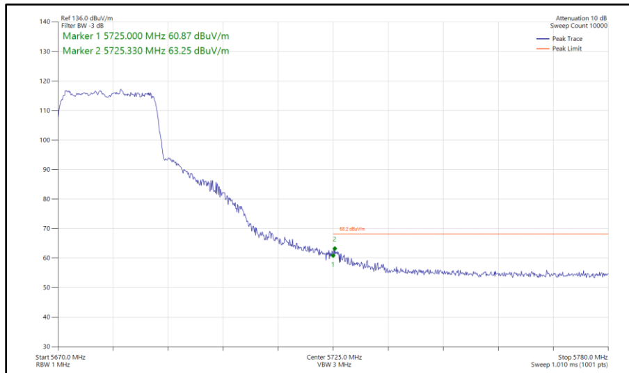
Figure 552 - 802.11ax HE20, SU, SDM, Core 0 - Core 1 - 5680 MHz Band Edge Frequency 5725 MHz
