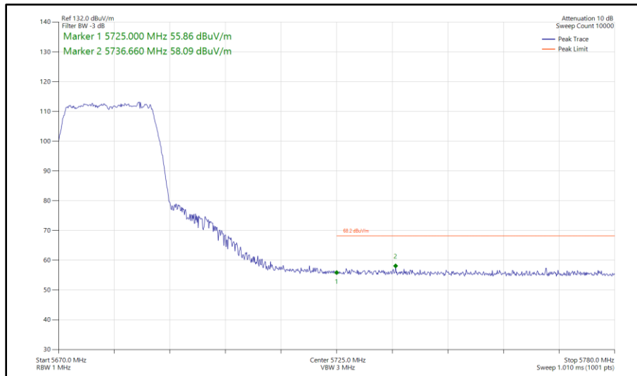
Figure 550 - 802.11n HT20, SDM, Core 0 - Core 1 - 5680 MHz Band Edge Frequency 5725 MHz
