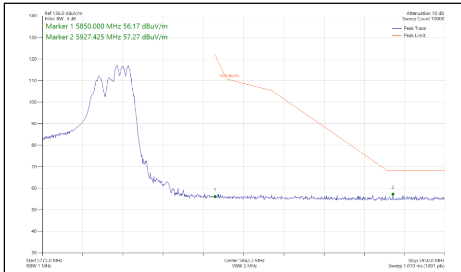
Figure 541 - 802.11ax HE40, RU 106-56, CDD, Core 0 - Core 1 - 5795 MHz Band Edge Frequency 5850 MHz
