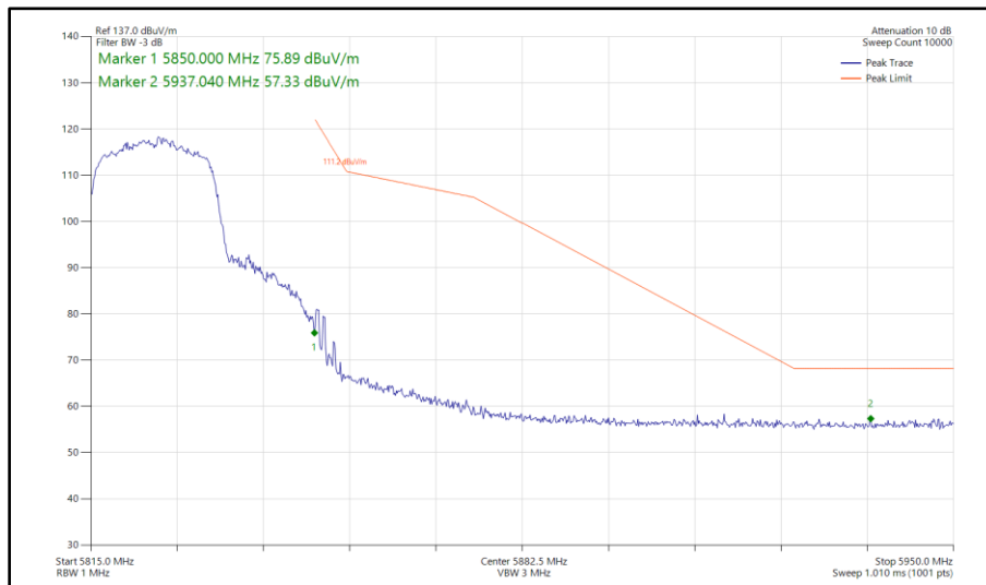
Figure 557 - 802.11n HT20, SDM, Core 0 - Core 1 - 5825 MHz Band Edge Frequency 5850 MHz
