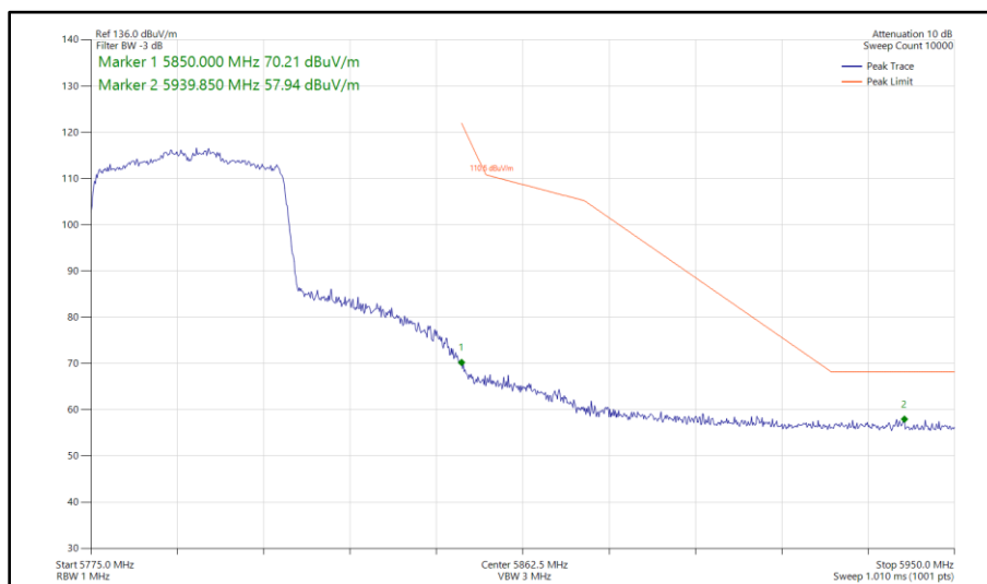
Figure 520 - 802.11ax HE40, SU, SISO, Core 1 - 5795 MHz Band Edge Frequency 5850 MHz
