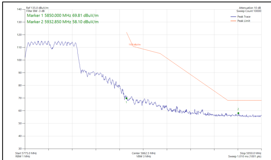
Figure 537 - 802.11n HT40, CDD, Core 0 - Core 1 - 5795 MHz Band Edge Frequency 5850 MHz
