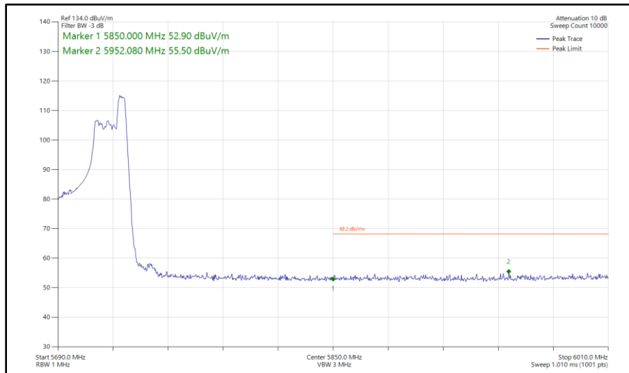
Figure 498 - 802.11ax HE40, RU 52-44, SISO, Core 0 - 5710 MHz Band Edge Frequency 5850 MHz
