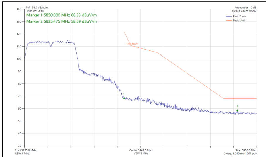
Figure 517 - 802.11n HT40, SISO, Core 1 - 5795 MHz Band Edge Frequency 5850 MHz
