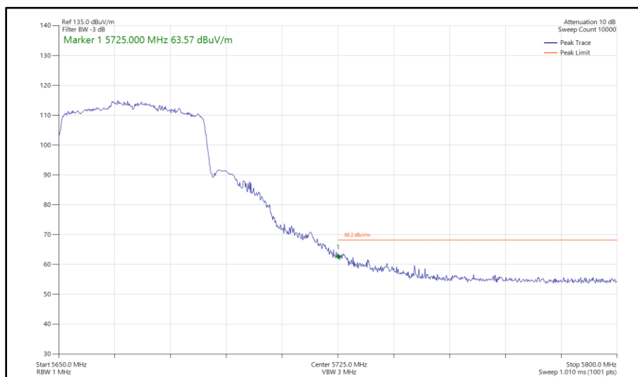
Figure 514 - 802.11ax HE40, SU, SISO, Core 1 - 5670 MHz Band Edge Frequency 5725 MHz
