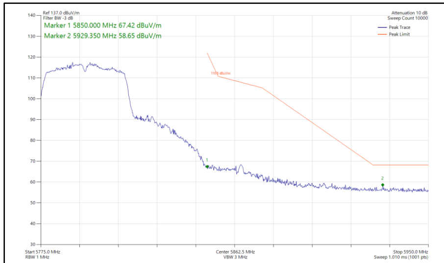
Figure 496 - 802.11n HT40, SISO, Core 0 - 5795 MHz Band Edge Frequency 5850 MHz
