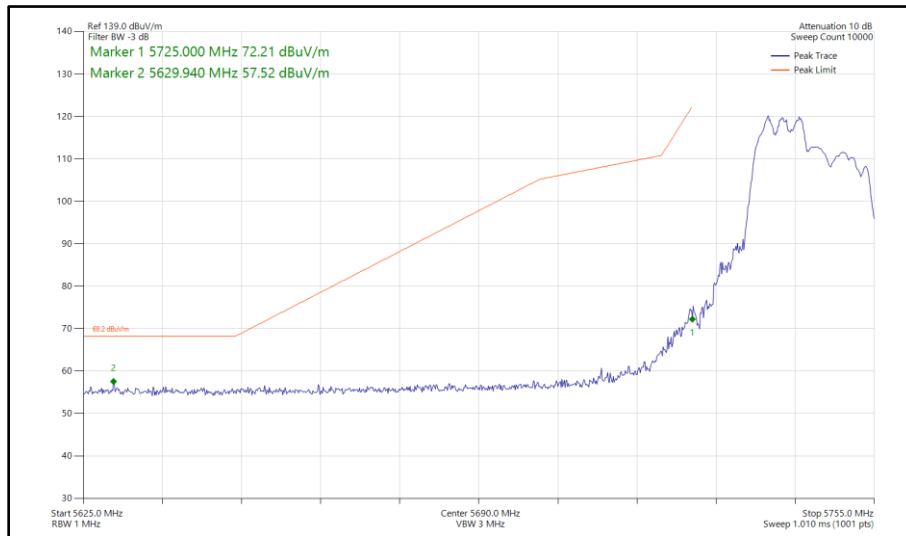
Figure 548 - 802.11ax HE20, RU 106-53, SDM, Core 0 - Core 1 - 5745 MHz Band Edge Frequency 5725 MHz
