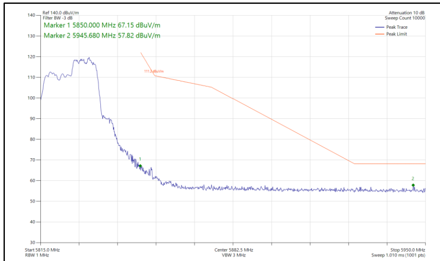
Figure 562 - 802.11ax HE20, RU 106-54, SDM, Core 0 - Core 1 - 5825 MHz Band Edge Frequency 5850 MHz
