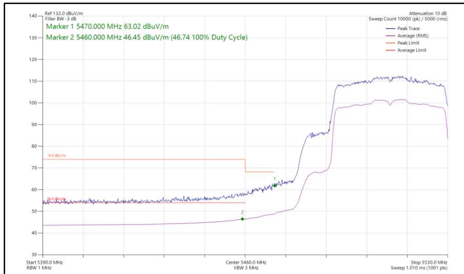
Figure 503 - 802.11ax HE40, SU, SISO, Core 1 - 5510 MHz Band Edge Frequency 5470 MHz
