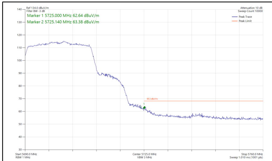
Figure 554 - 802.11ax HE20, SU, SDM, Core 0 - Core 1 - 5700 MHz Band Edge Frequency 5725 MHz
