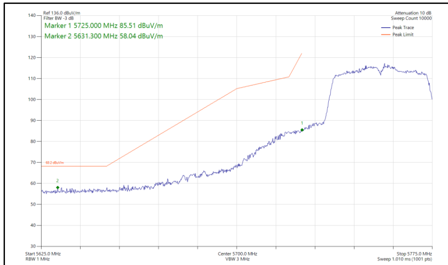
Figure 507 - 802.11n HT40, SISO, Core 1 - 5755 MHz Band Edge Frequency 5725 MHz
