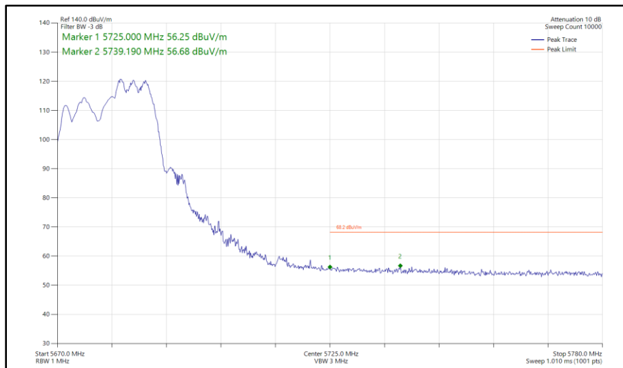
Figure 553 - 802.11ax HE20, RU 106-54, SDM, Core 0 - Core 1 - 5680 MHz Band Edge Frequency 5725 MHz
