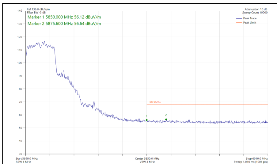
Figure 536 - 802.11n HT40, CDD, Core 0 - Core 1 - 5710 MHz Band Edge Frequency 5850 MHz
