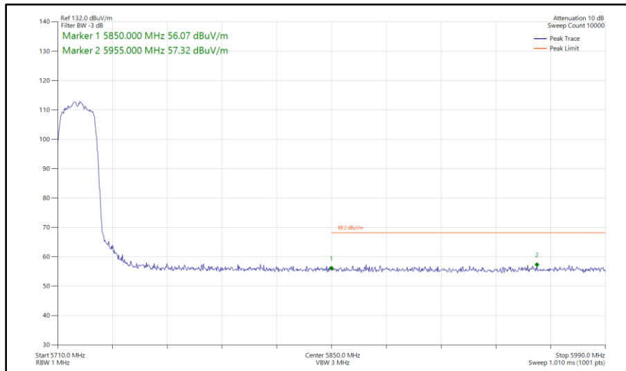
Figure 556 - 802.11n HT20, SDM, Core 0 - Core 1 - 5720 MHz Band Edge Frequency 5850 MHz
