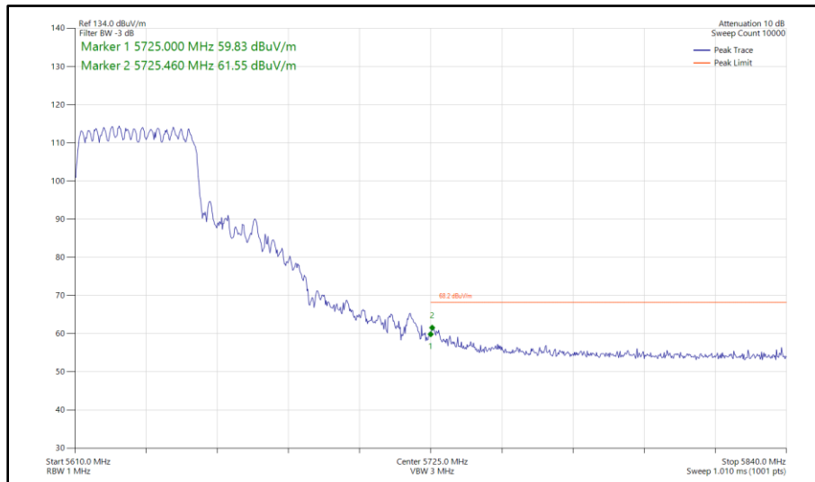
Figure 533 - 802.11ax HE40, SU, CDD, Core 0 - Core 1 - 5630 MHz Band Edge Frequency 5725 MHz
