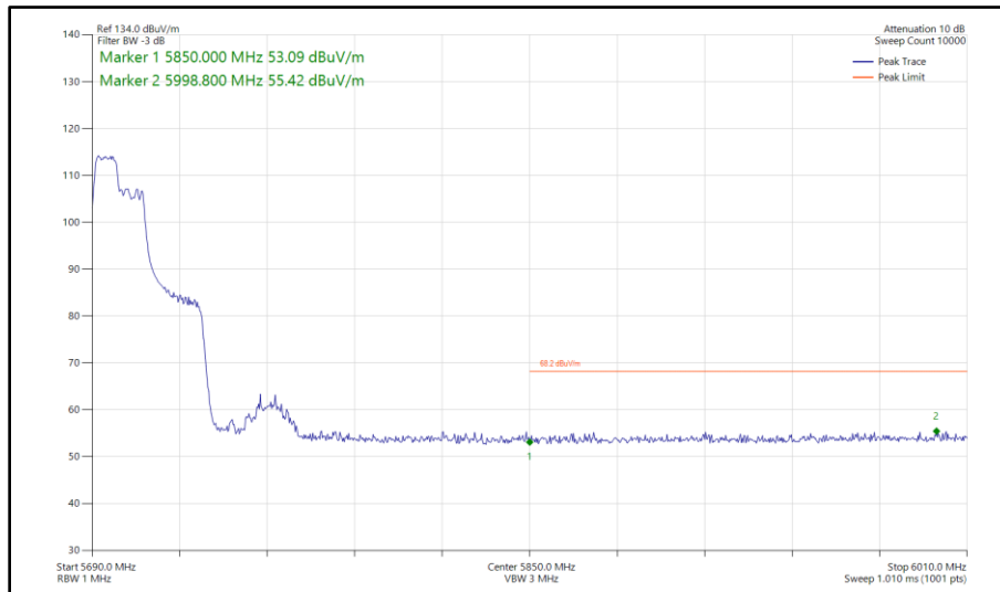
Figure 519 - 802.11ax HE40, RU 106-53, SISO, Core 1 - 5710 MHz Band Edge Frequency 5850 MHz
