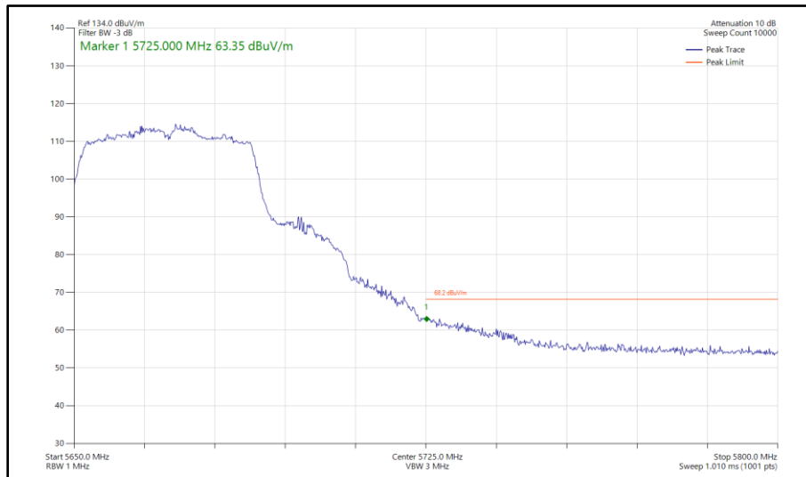
Figure 490 - 802.11n HT40, SISO, Core 0 - 5670 MHz Band Edge Frequency 5725 MHz
