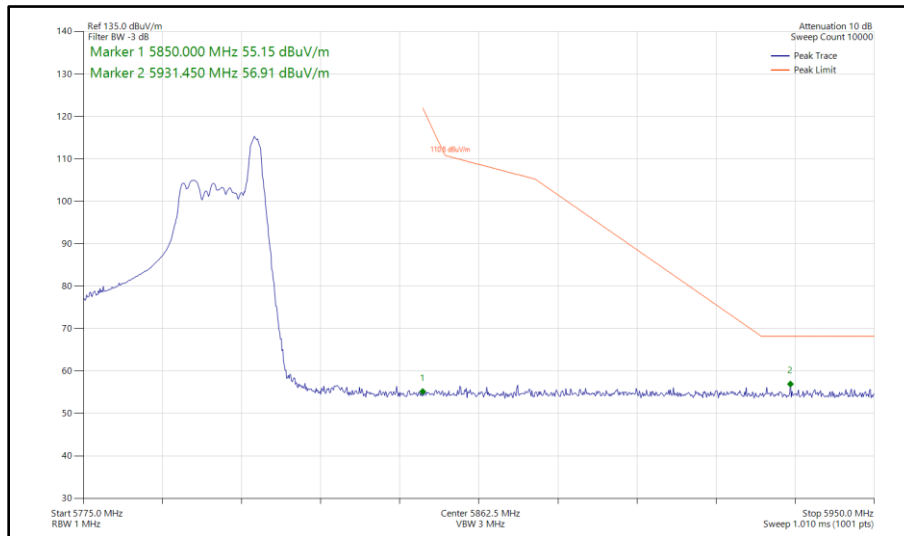
Figure 500 - 802.11ax HE40, RU 26-17, SISO, Core 0 - 5795 MHz Band Edge Frequency 5850 MHz
