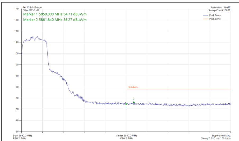
Figure 516 - 802.11n HT40, SISO, Core 1 - 5710 MHz Band Edge Frequency 5850 MHz
