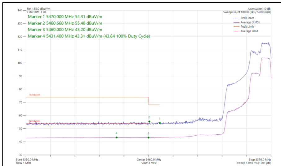
Figure 485 - 802.11ax HE40, RU 106-56, SISO, Core 0 - 5550 MHz Band Edge Frequency 5470 MHz
