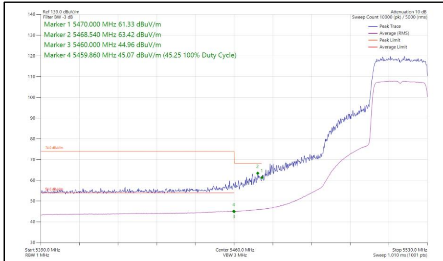
Figure 465 - 802.11ax HE20, SU, TxBF, Core 0 - Core 1 - 5520 MHz Band Edge Frequency 5470 MHz
