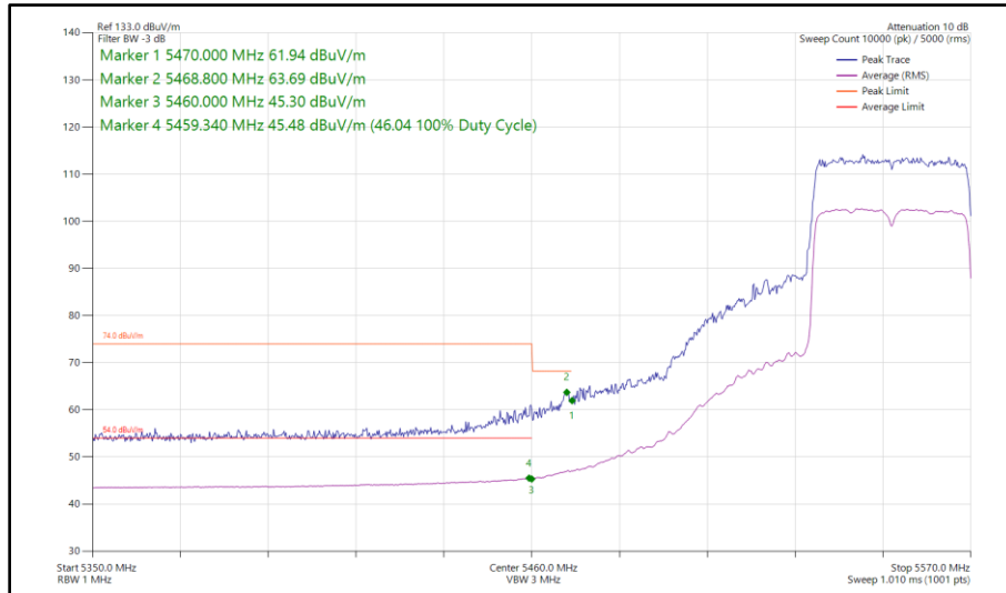
Figure 484 - 802.11ax HE40, SU, SISO, Core 0 - 5550 MHz Band Edge Frequency 5470 MHz
