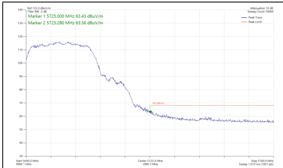
Figure 428 - 802.11n HT20, CDD, Core 0 - Core 1 - 5700 MHz Band Edge Frequency 5725 MHz
