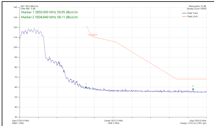
Figure 438 - 802.11ax HE20, SU, CDD, Core 0 - Core 1 - 5805 MHz Band Edge Frequency 5850 MHz
