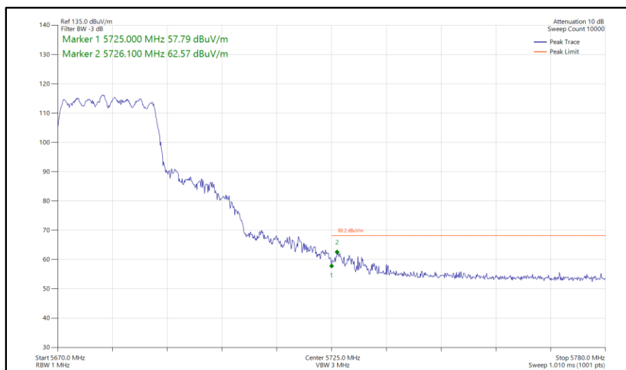
Figure 429 - 802.11ax HE20, SU, CDD, Core 0 - Core 1 - 5680 MHz Band Edge Frequency 5725 MHz
