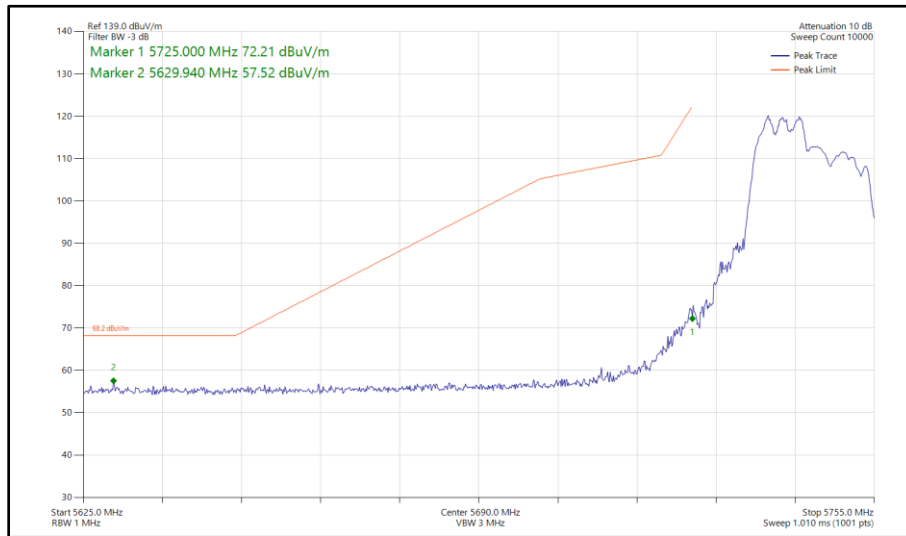
Figure 447 - 802.11ax HE20, RU 106-53, SDM, Core 0 - Core 1 - 5745 MHz Band Edge Frequency 5725 MHz
