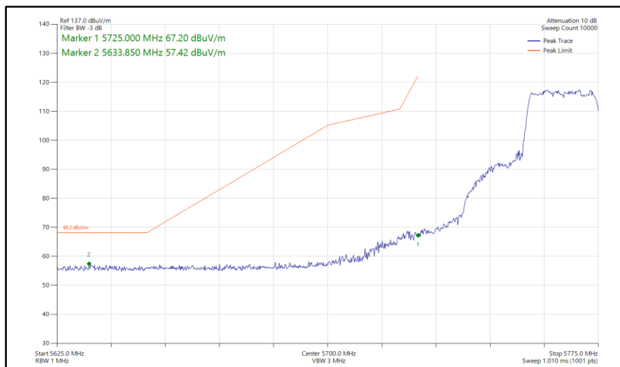
Figure 448 - 802.11ax HE20, SU, SDM, Core 0 - Core 1 - 5765 MHz Band Edge Frequency 5725 MHz
