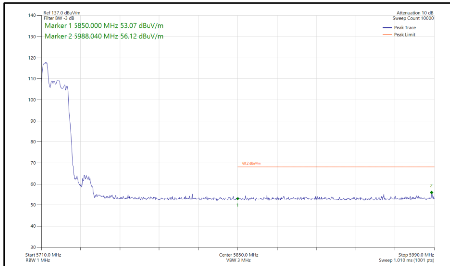
Figure 412 - 802.11ax HE20, RU 52-37, SISO, Core 1 - 5720 MHz Band Edge Frequency 5850 MHz
