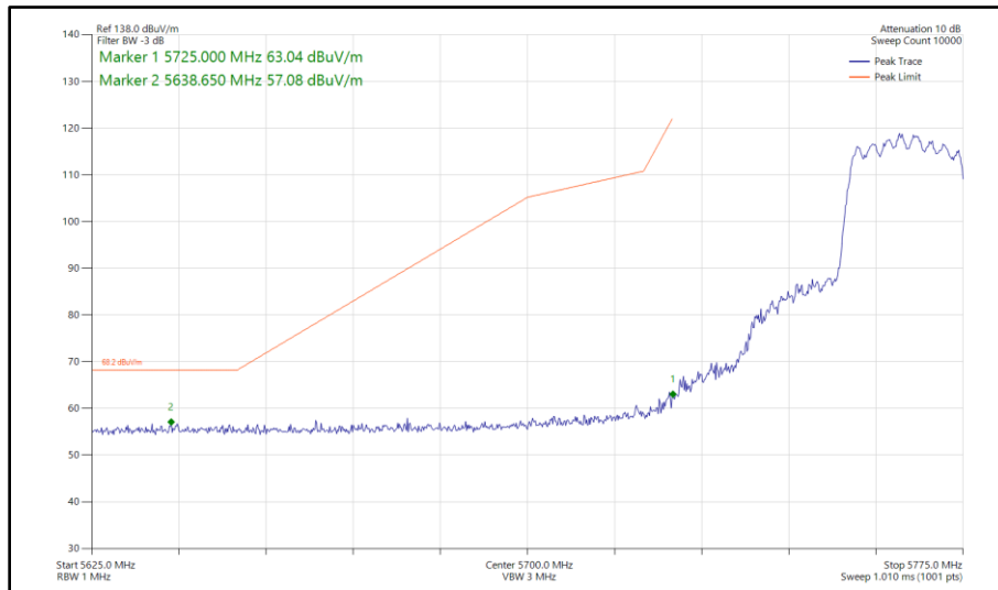
Figure 426 - 802.11ax HE20, SU, CDD, Core 0 - Core 1 - 5765 MHz Band Edge Frequency 5725 MHz
