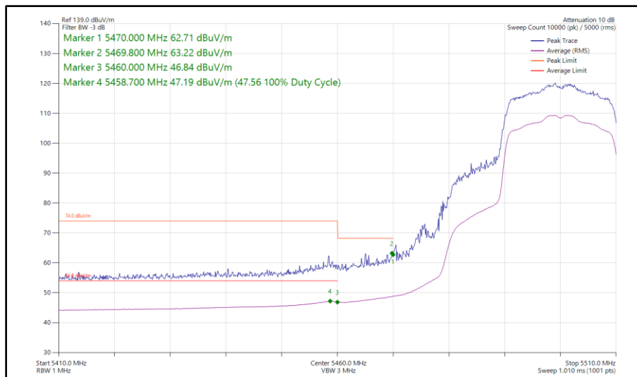
Figure 464 - 802.11ax HE20, SU, TxBF, Core 0 - Core 1 - 5500 MHz Band Edge Frequency 5470 MHz
