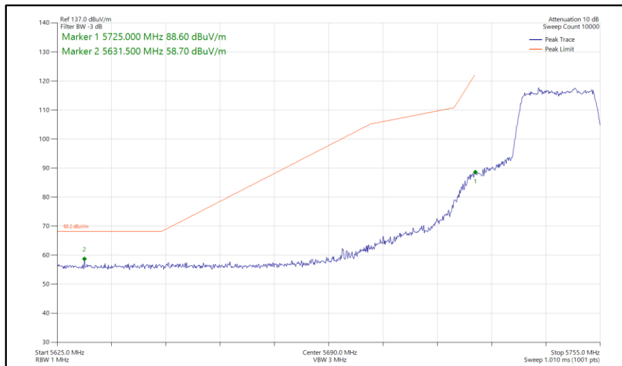
Figure 446 - 802.11n HT20, SDM, Core 0 - Core 1 - 5745 MHz Band Edge Frequency 5725 MHz
