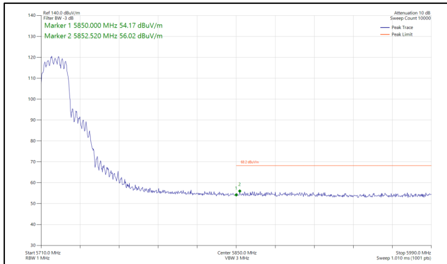
Figure 436 - 802.11ax HE20, SU, CDD, Core 0 - Core 1 - 5720 MHz Band Edge Frequency 5850 MHz
