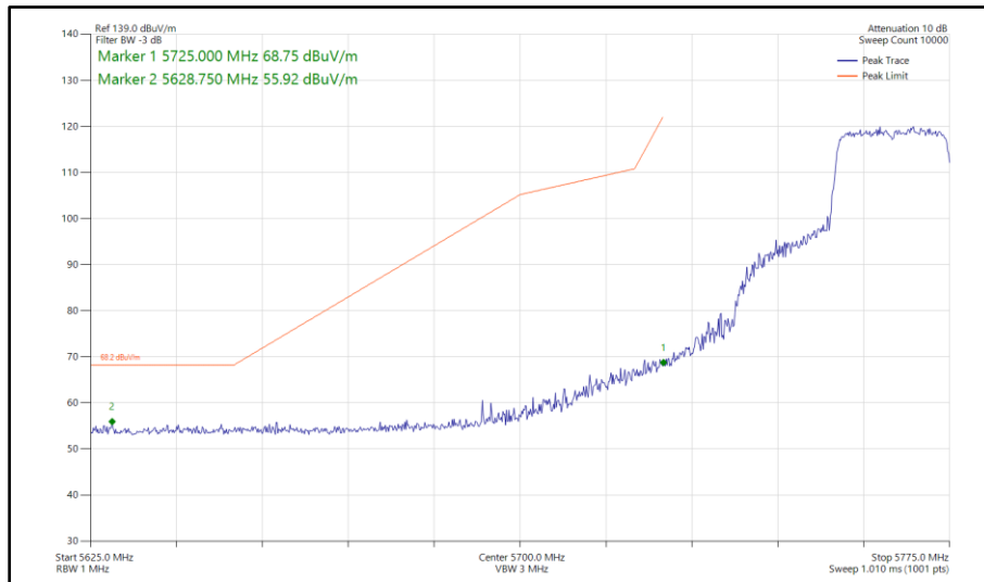
Figure 469 - 802.11ax HE20, SU, TxBF, Core 0 - Core 1 - 5765 MHz Band Edge Frequency 5725 MHz
