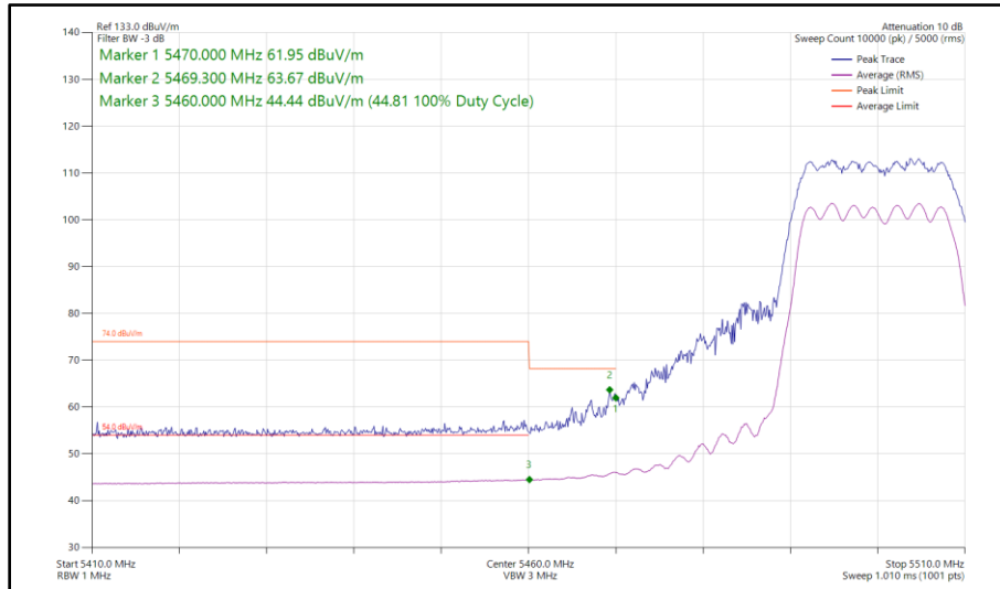
Figure 416 - 802.11n HT20, CDD, Core 0 - Core 1 - 5500 MHz Band Edge Frequency 5470 MHz
