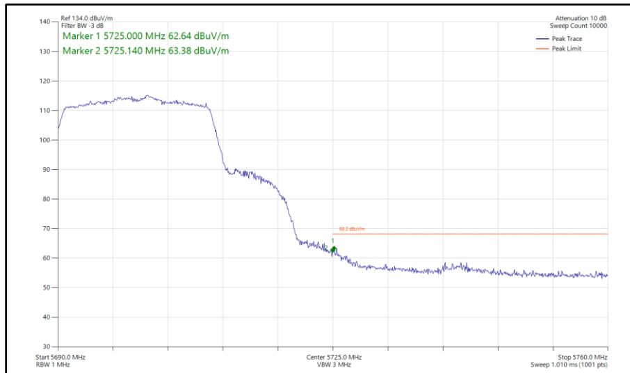
Figure 453 - 802.11ax HE20, SU, SDM, Core 0 - Core 1 - 5700 MHz Band Edge Frequency 5725 MHz
