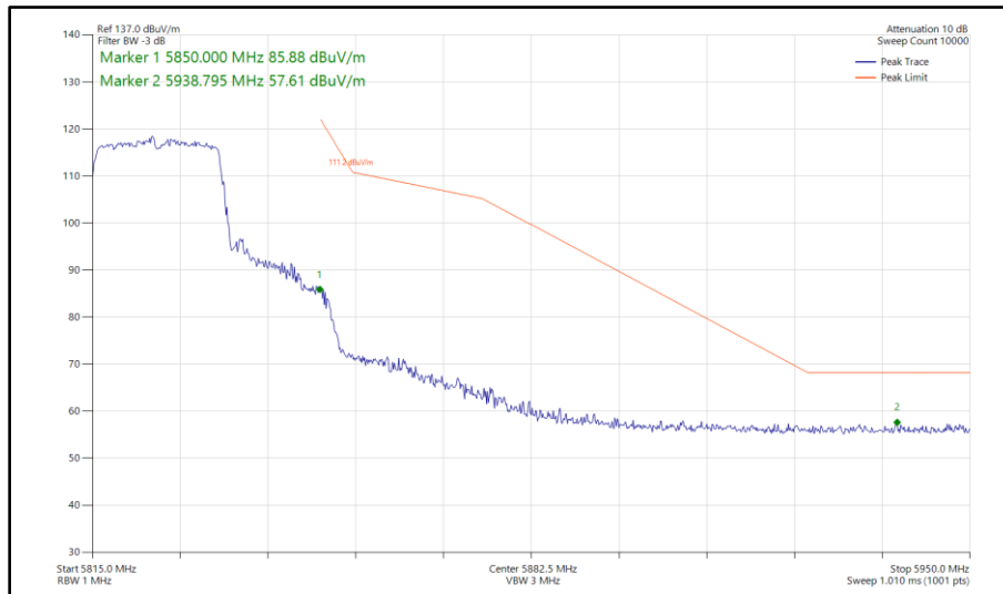
Figure 414 - 802.11ax HE20, SU, SISO, Core 1 - 5825 MHz Band Edge Frequency 5850 MHz
