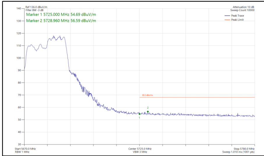
Figure 430 - 802.11ax HE20, RU 106-54, CDD, Core 0 - Core 1 - 5680 MHz Band Edge Frequency 5725 MHz
