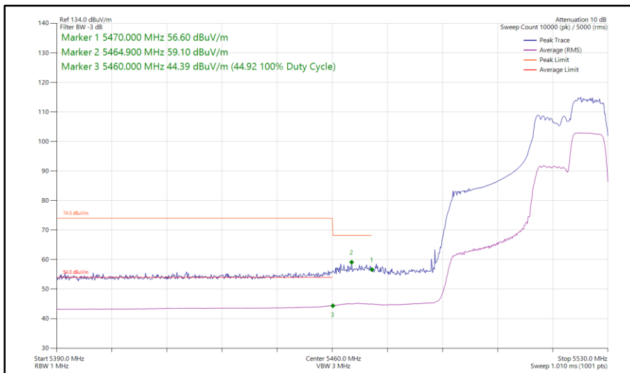
Figure 483 - 802.11ax HE40, RU 106-56, SISO, Core 0 - 5510 MHz Band Edge Frequency 5470 MHz
