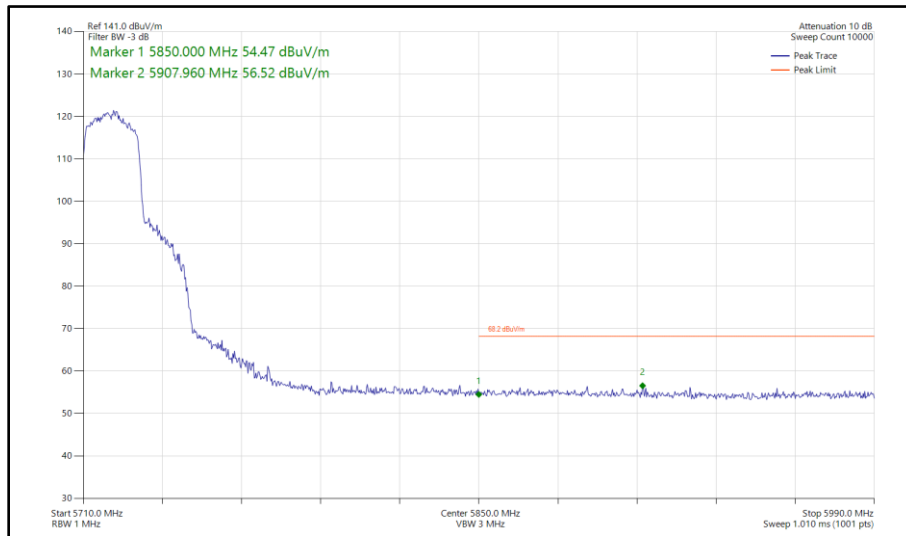
Figure 477 - 802.11ax HE20, SU, TxBF, Core 0 - Core 1 - 5720 MHz Band Edge Frequency 5850 MHz
