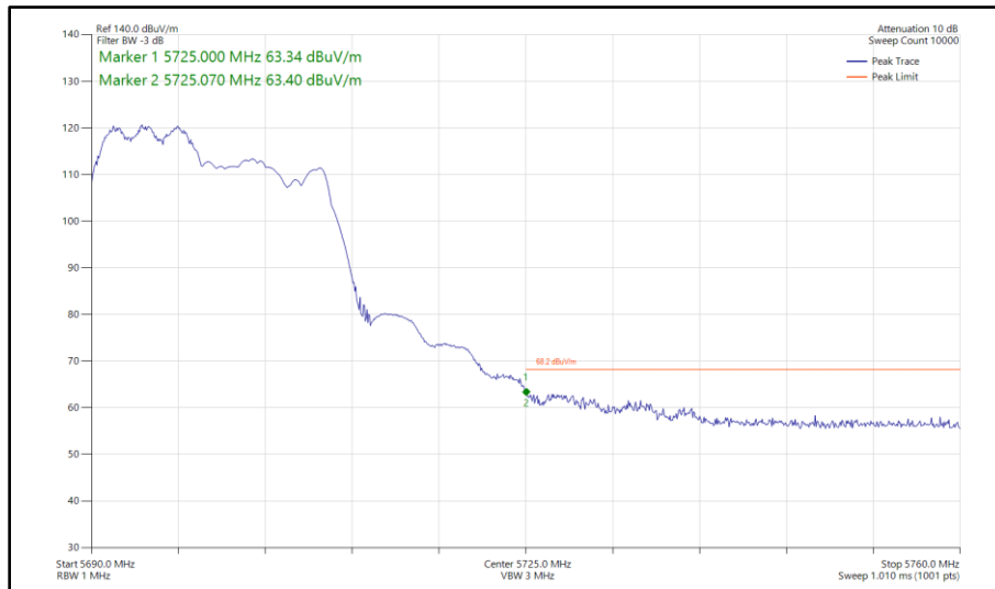
Figure 432 - 802.11ax HE20, RU 106-53, CDD, Core 0 - Core 1 - 5700 MHz Band Edge Frequency 5725 MHz
