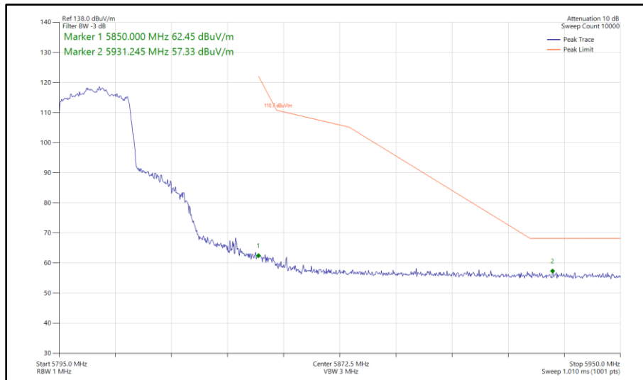
Figure 459 - 802.11ax HE20, SU, SDM, Core 0 - Core 1 - 5805 MHz Band Edge Frequency 5850 MHz
