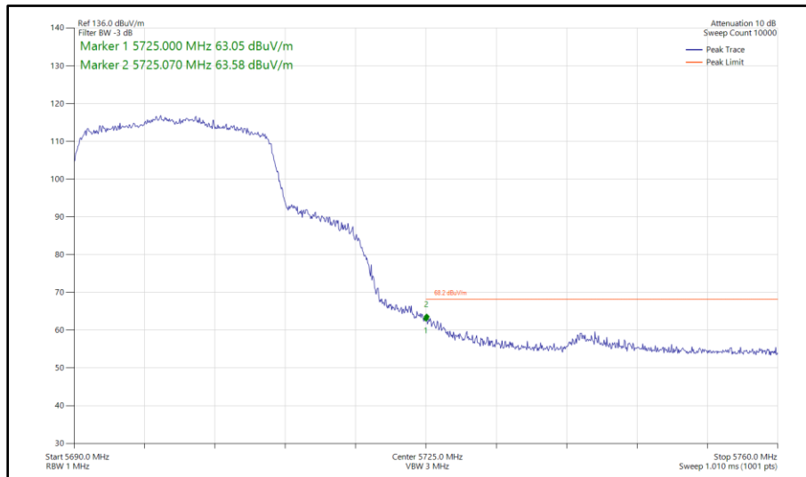
Figure 473 - 802.11ax HE20, SU, TxBF, Core 0 - Core 1 - 5700 MHz Band Edge Frequency 5725 MHz
