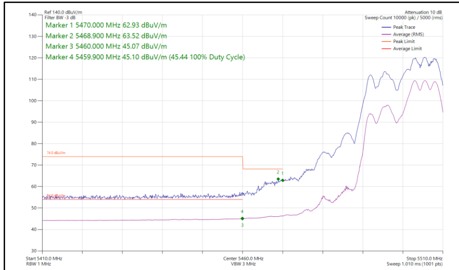
Figure 443 - 802.11ax HE20, RU 106-54, SDM, Core 0 - Core 1 - 5500 MHz Band Edge Frequency 5470 MHz
