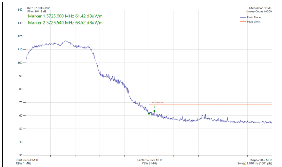
Figure 471 - 802.11ac VHT20, TxBF, Core 0 - Core 1 - 5700 MHz Band Edge Frequency 5725 MHz
