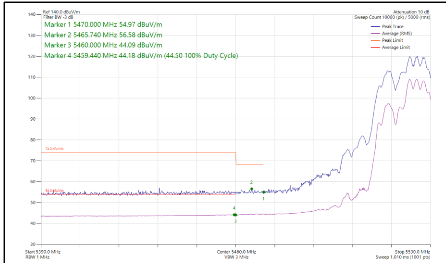
Figure 445 - 802.11ax HE20, RU 106-54, SDM, Core 0 - Core 1 - 5520 MHz Band Edge Frequency 5470 MHz
