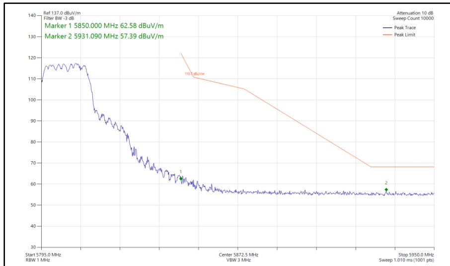
Figure 434 - 802.11n HT20, CDD, Core 0 - Core 1 - 5805 MHz Band Edge Frequency 5850 MHz
