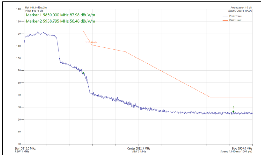
Figure 479 - 802.11ax HE20, SU, TxBF, Core 0 - Core 1 - 5825 MHz Band Edge Frequency 5850 MHz
