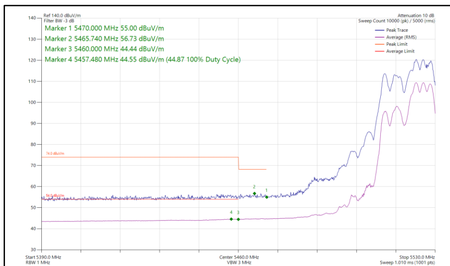
Figure 421 - 802.11ax HE20, RU 106-54, CDD, Core 0 - Core 1 - 5520 MHz Band Edge Frequency 5470 MHz
