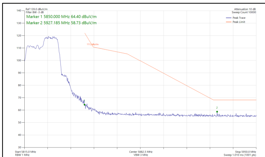
Figure 415 - 802.11ax HE20, RU 106-54, SISO, Core 1 - 5825 MHz Band Edge Frequency 5850 MHz
