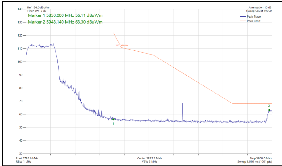
Figure 475 - 802.11ac VHT20, TxBF, Core 0 - Core 1 - 5805 MHz Band Edge Frequency 5850 MHz
