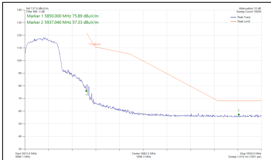
Figure 456 - 802.11n HT20, SDM, Core 0 - Core 1 - 5825 MHz Band Edge Frequency 5850 MHz
