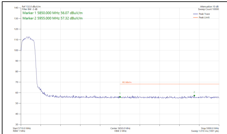
Figure 455 - 802.11n HT20, SDM, Core 0 - Core 1 - 5720 MHz Band Edge Frequency 5850 MHz
