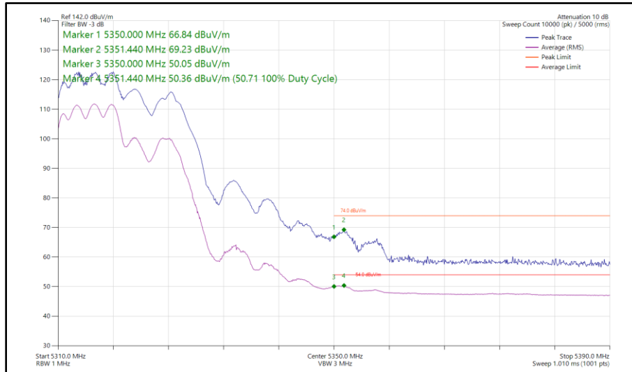
Figure 60 - 802.11ax HE20, RU 106-53, CDD, Core 0 - Core 1 - 5320 MHz Band Edge Frequency 5350 MHz
