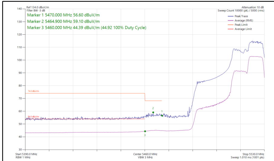
Figure 104 - 802.11ax HE40, RU 106-56, SISO, Core 0 - 5510 MHz Band Edge Frequency 5460 MHz
