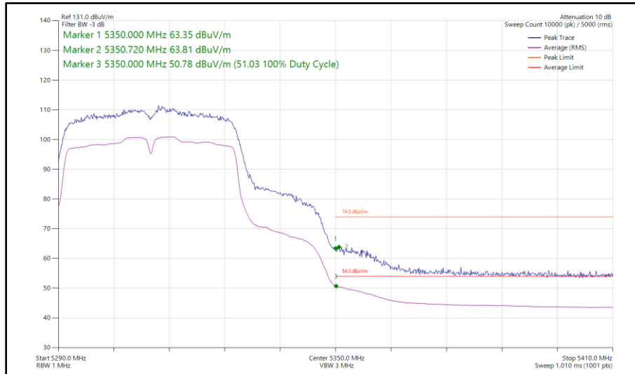
Figure 96 - 802.11n HT40, SISO, Core 0 - 5310 MHz Band Edge Frequency 5350 MHz
