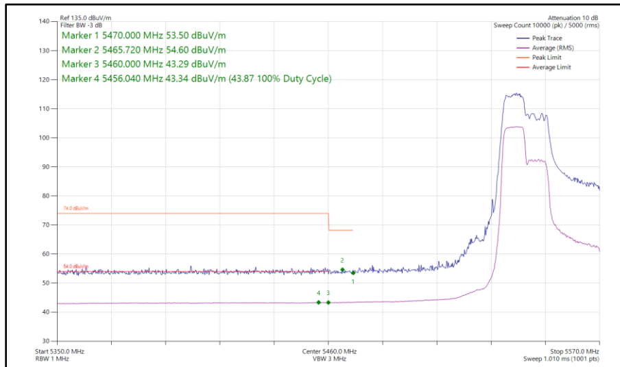
Figure 106 - 802.11ax HE40, RU 106-53, SISO, Core 0 - 5550 MHz Band Edge Frequency 5460 MHz
