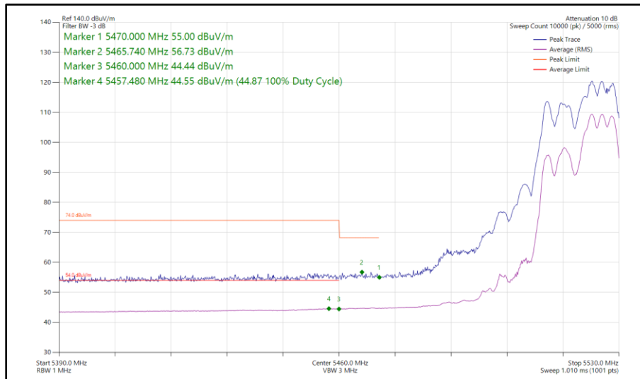
Figure 66 - 802.11ax HE20, RU 106-54, CDD, Core 0 - Core 1 - 5520 MHz Band Edge Frequency 5460 MHz
