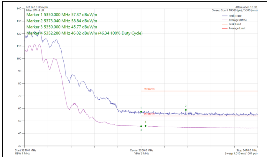
Figure 58 - 802.11ax HE20, RU 106-53, CDD, Core 0 - Core 1 - 5300 MHz Band Edge Frequency 5350 MHz
