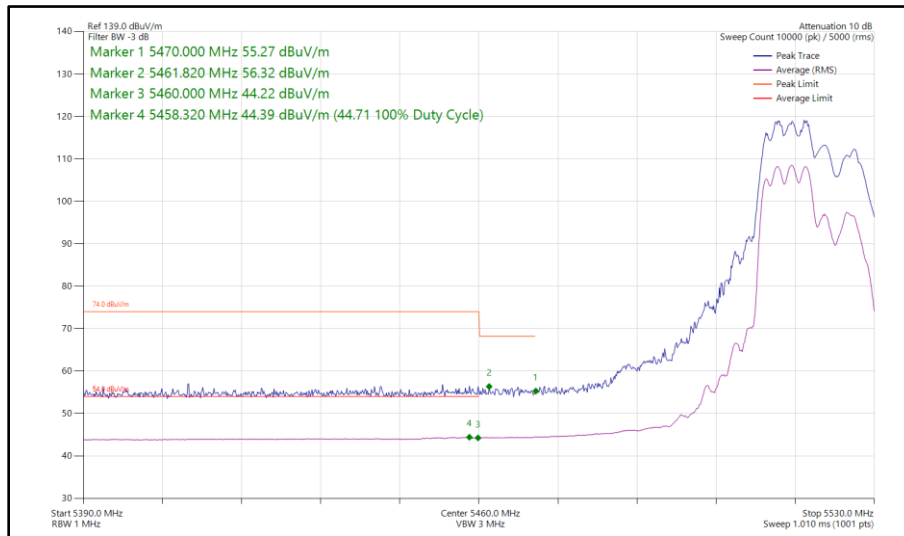
Figure 82 - 802.11ax HE20, RU 106-53, SDM, Core 0 - Core 1 - 5520 MHz Band Edge Frequency 5460 MHz
