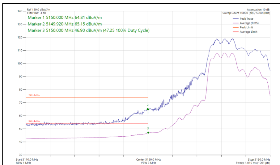
Figure 69 - 802.11ax HE20, RU 106-53, SDM, Core 0 - Core 1 - 5180 MHz Band Edge Frequency 5150 MHz
