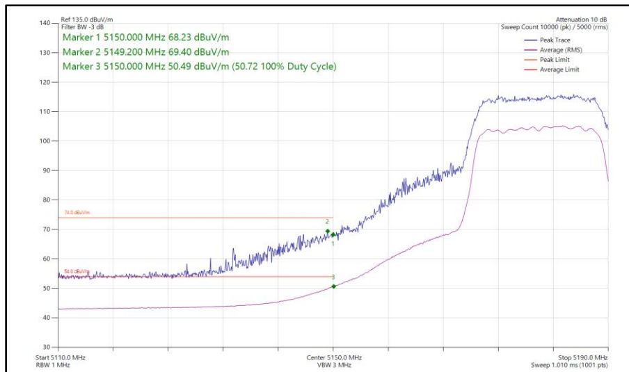
Figure 83 - 802.11ac VHT20, TxBF, Core 0 - Core 1 - 5180 MHz Band Edge Frequency 5150 MHz
