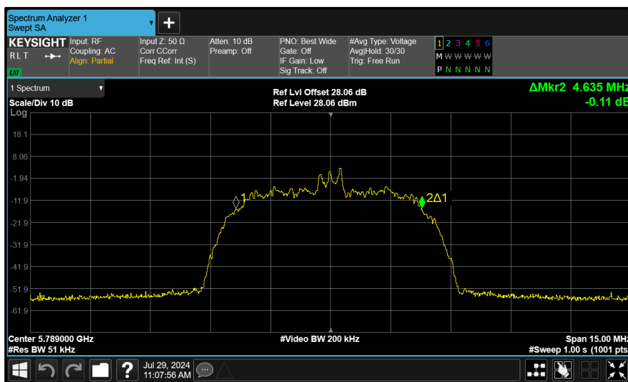
Figure 60 - Core 1 (B) 5789 MHz (CH64) 99% Bandwidth
