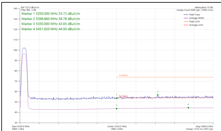
Figure 12 - Narrowband HDR8, SISO, Core 1 - 5245 MHz Band Edge Frequency 5350 MHz
