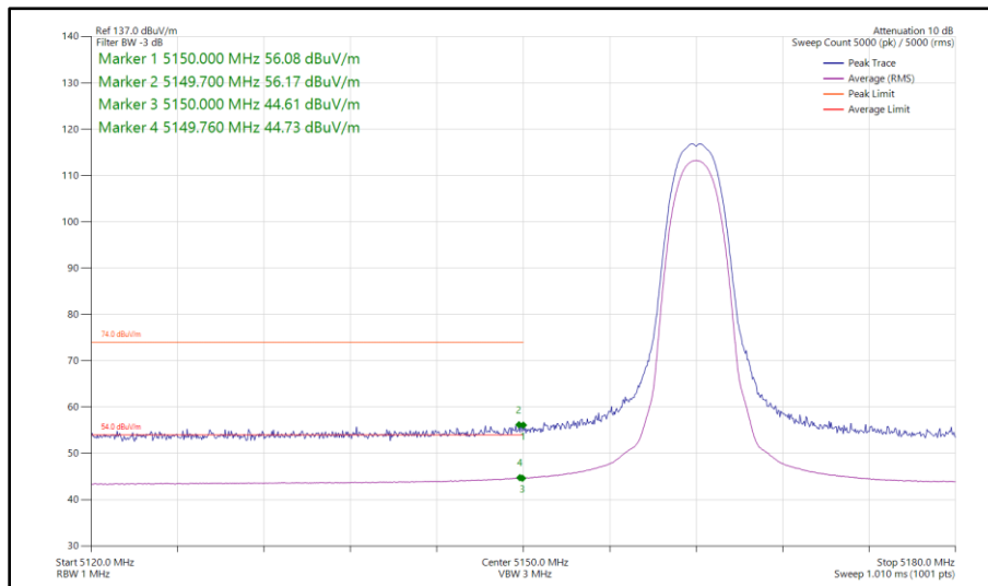
Figure 19 - Narrowband HDR4, SISO, Core 0 - 5162 MHz Band Edge Frequency 5150 MHz
