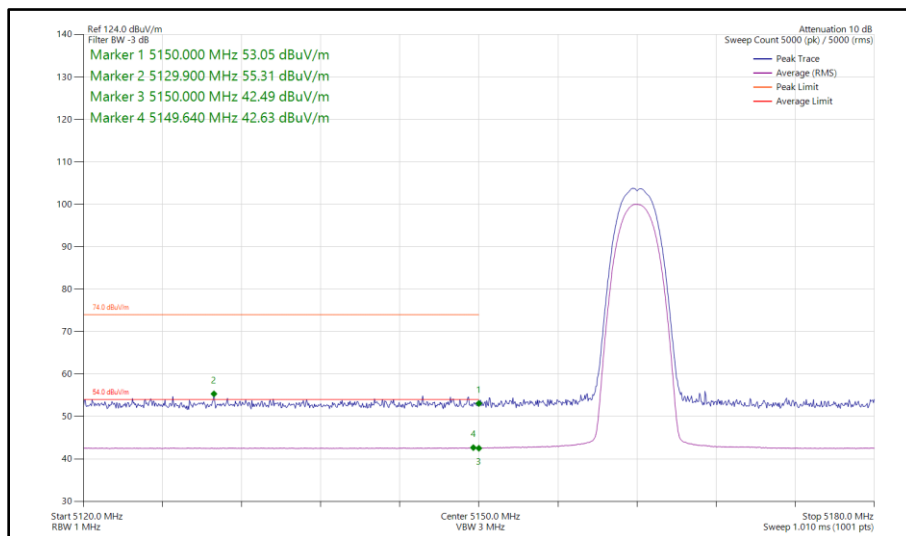
Figure 8 - Narrowband HDR4, SISO, Core 1 - 5162 MHz Band Edge Frequency 5150 MHz
