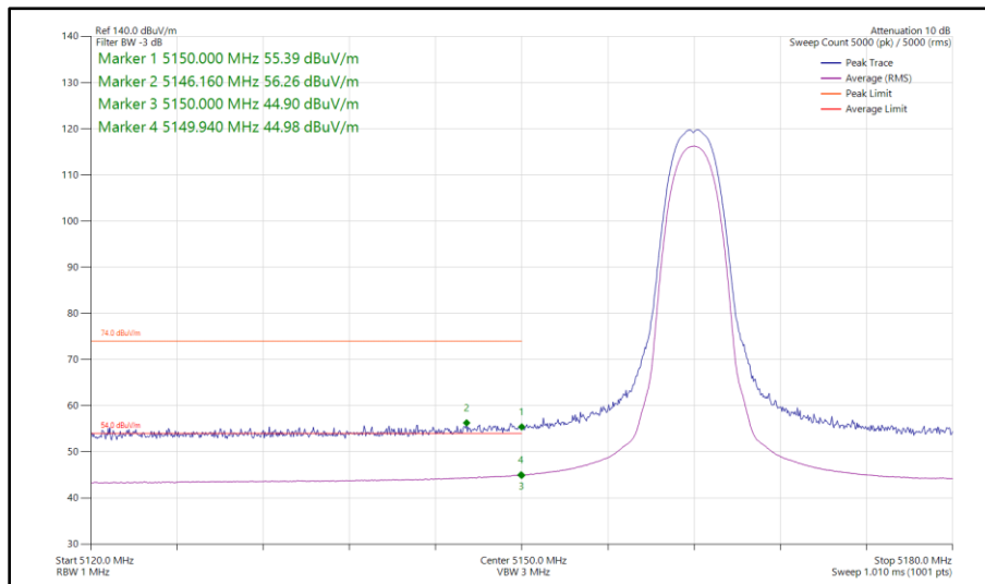
Figure 27 - Narrowband HDR4, MIMO, Core 0 - Core 1 - 5162 MHz Band Edge Frequency 5150 MHz
