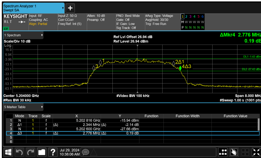
Figure 35 - Core 1 (B) 5204 MHz (CH54) 26 dB and 99% Bandwidth
