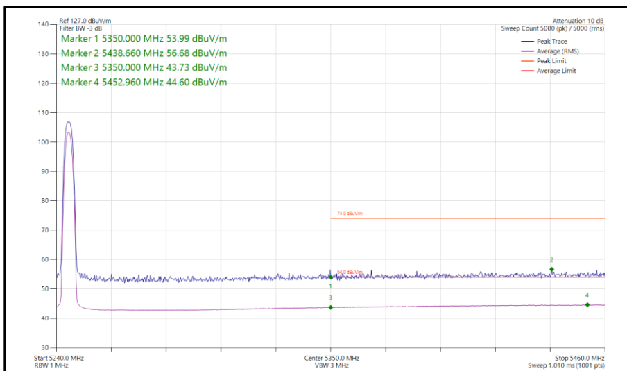
Figure 5 - Narrowband HDR4, SISO, Core 0 - 5245 MHz Band Edge Frequency 5350 MHz
