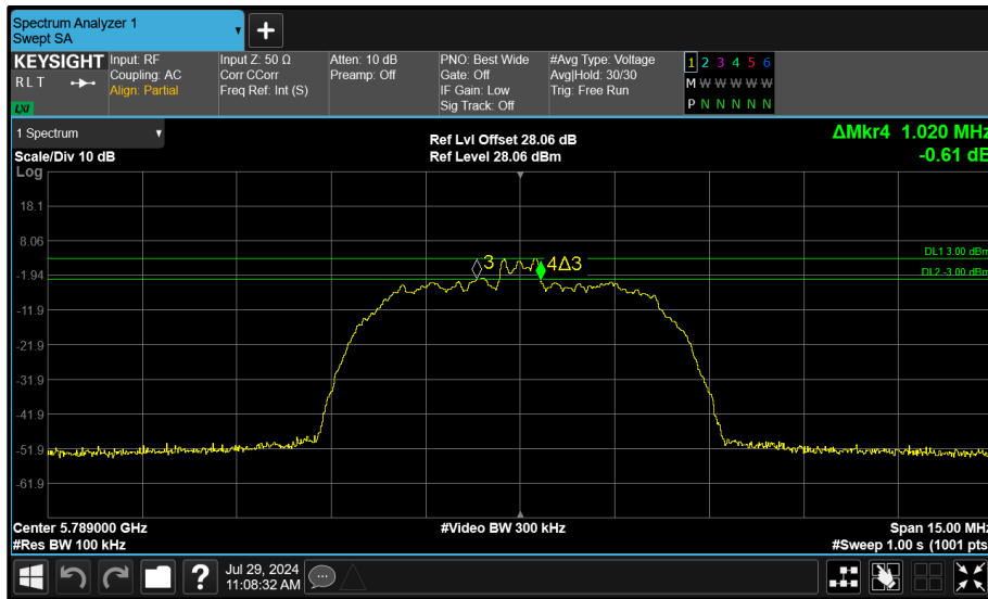
Figure 61 - Core 1 (B) 5789 MHz (CH64) 6 dB Bandwidth
