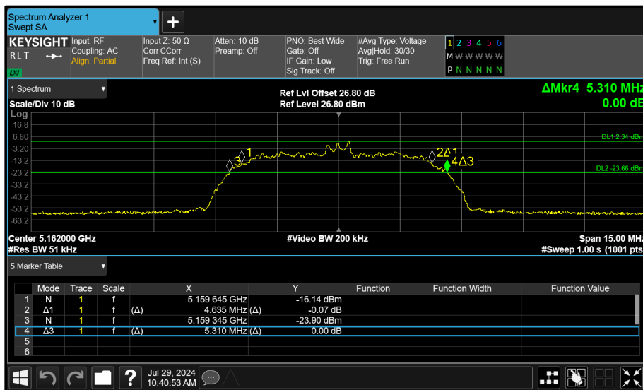
Figure 37 - Core 1 (B) 5162 MHz (CH12) 26 dB and 99% Bandwidth
