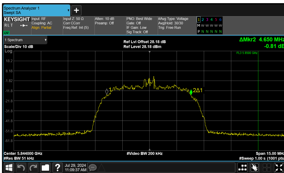
Figure 62 - Core 1 (B) 5844 MHz (CH119) 99% Bandwidth
