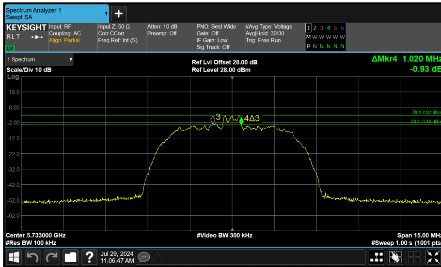
Figure 59 - Core 1 (B) 5733 MHz (CH8) 6 dB Bandwidth
