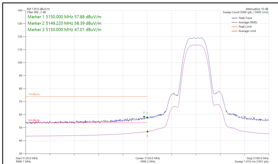
Figure 28 - Narrowband HDR8, MIMO, Core 0 - Core 1 - 5162 MHz Band Edge Frequency 5150 MHz
