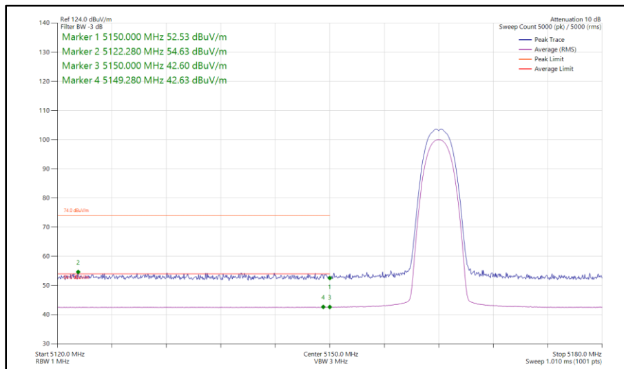
Figure 2 - Narrowband HDR4, SISO, Core 0 - 5162 MHz Band Edge Frequency 5150 MHz
