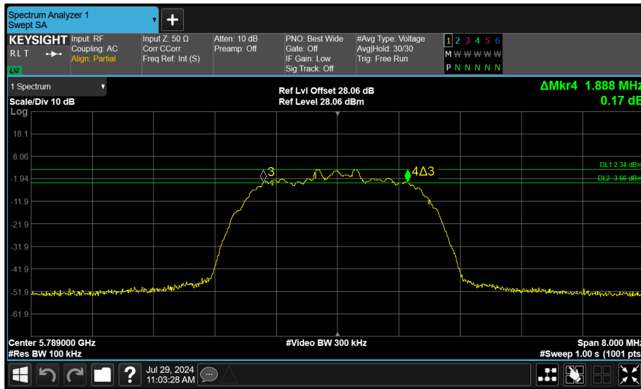
Figure 55 - Core 1 (B) 5789 MHz (CH64) 6 dB Bandwidth
