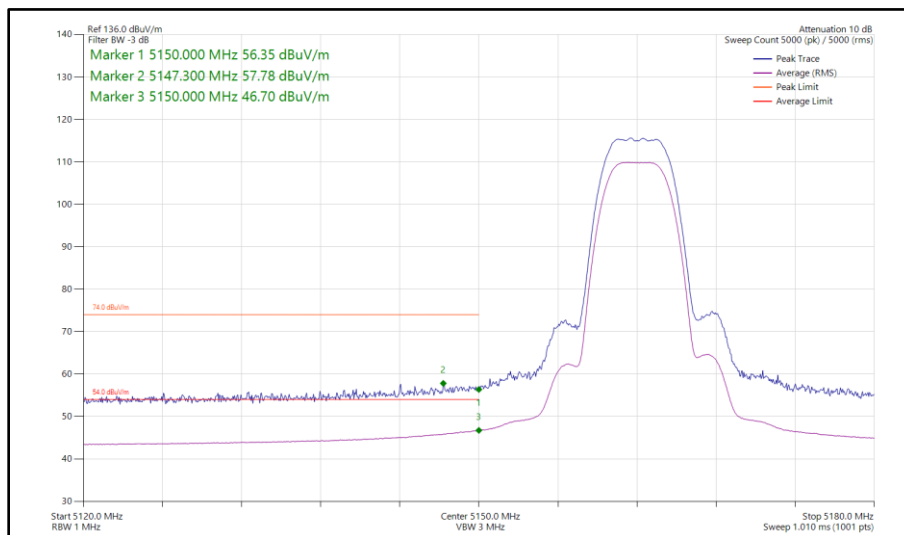
Figure 20 - Narrowband HDR8, SISO, Core 0 - 5162 MHz Band Edge Frequency 5150 MHz
