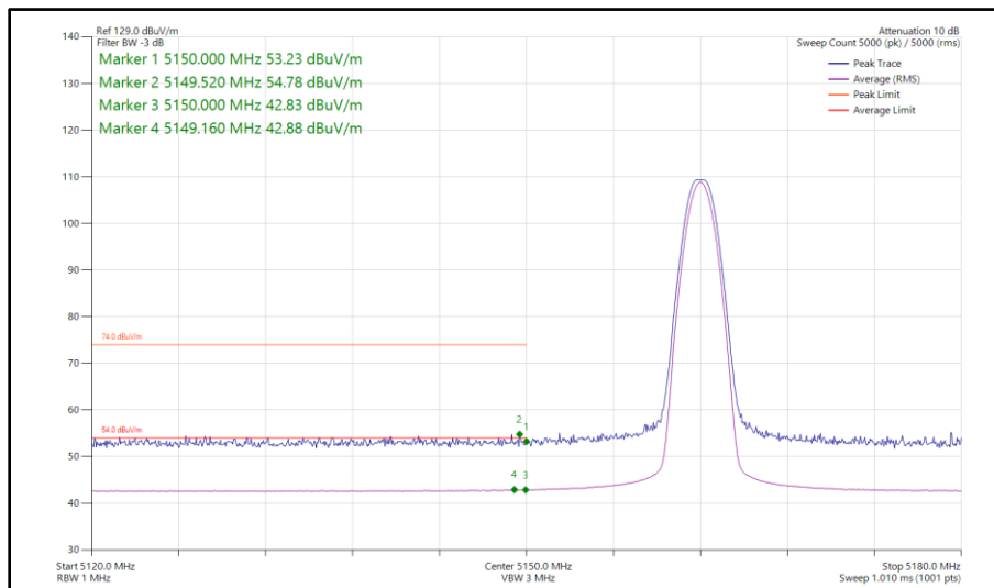
Figure 1 - Narrowband DH5, SISO, Core 0 - 5162 MHz Band Edge Frequency 5150 MHz
