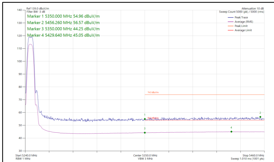
Figure 22 - Narrowband HDR8, SISO, Core 0 - 5245 MHz Band Edge Frequency 5350 MHz
