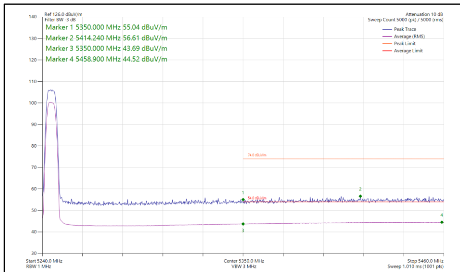
Figure 6 - Narrowband HDR8, SISO, Core 0 - 5245 MHz Band Edge Frequency 5350 MHz
