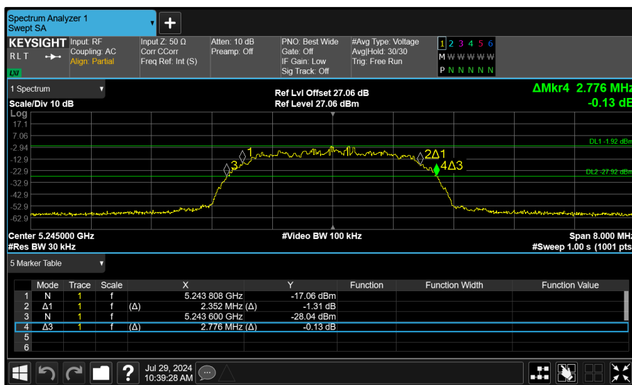
Figure 36 - Core 1 (B) 5245 MHz (CH95) 26 dB and 99% Bandwidth
