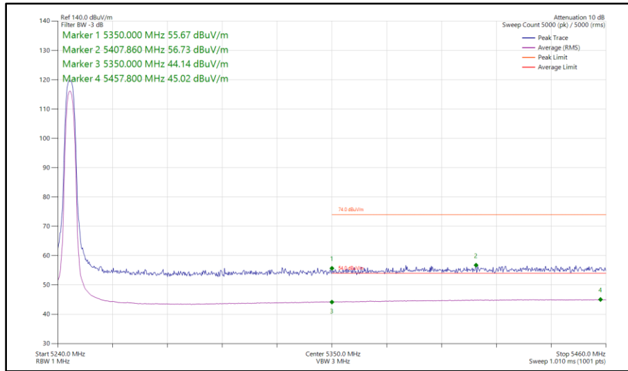
Figure 21 - Narrowband HDR4, SISO, Core 0 - 5245 MHz Band Edge Frequency 5350 MHz
