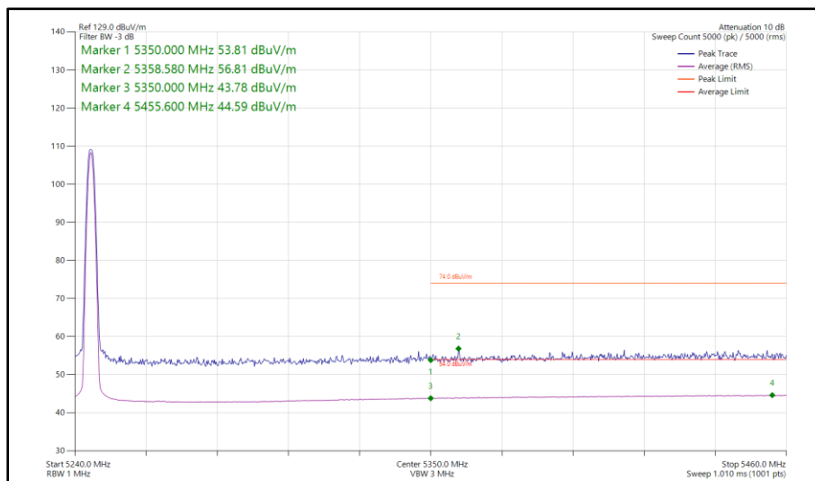
Figure 10 - Narrowband DH5, SISO, Core 1 - 5245 MHz Band Edge Frequency 5350 MHz
