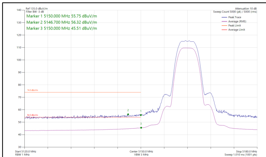
Figure 24 - Narrowband HDR8, SISO, Core 1 - 5162 MHz Band Edge Frequency 5150 MHz
