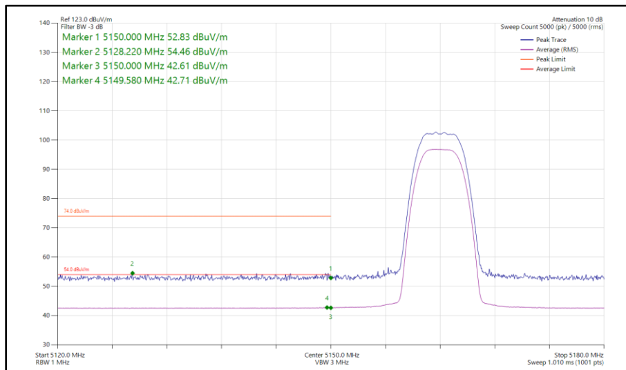
Figure 9 - Narrowband HDR8, SISO, Core 1 - 5162 MHz Band Edge Frequency 5150 MHz
