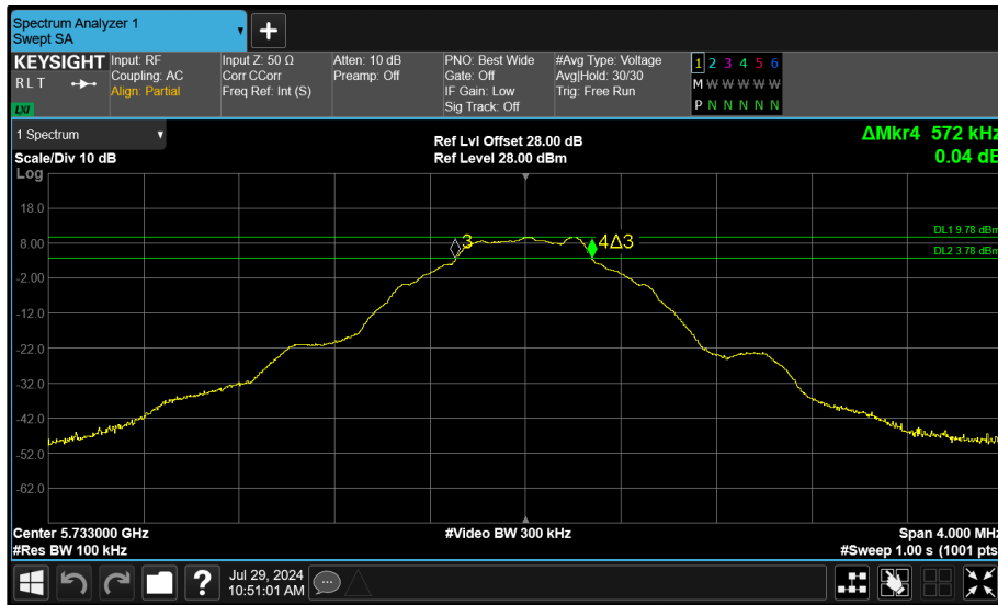
Figure 47 - Core 1 (B) 5733 MHz (CH8) 6 dB Bandwidth
