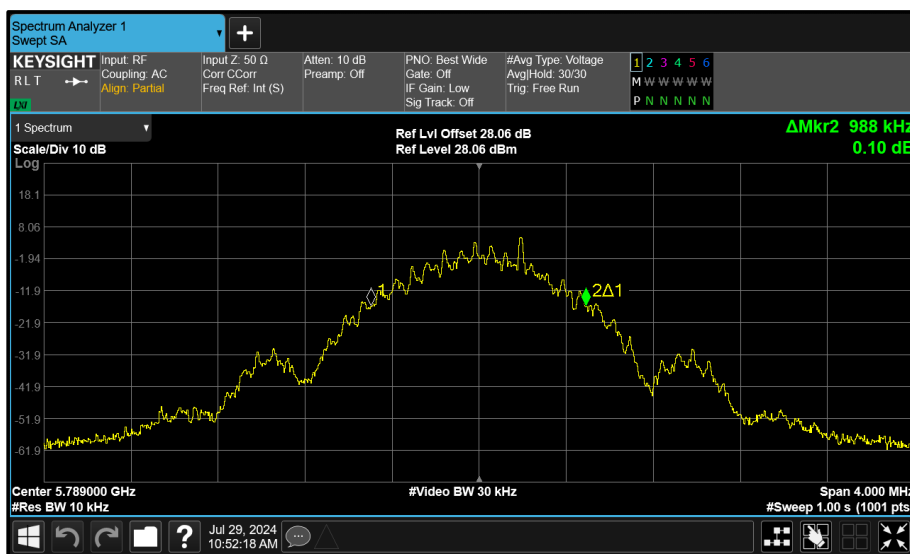
Figure 48 - Core 1 (B) 5789 MHz (CH64) 99% Bandwidth
