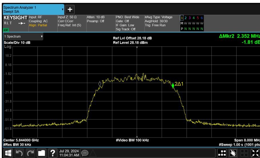
Figure 56 - Core 1 (B) 5844 MHz (CH119) 99% Bandwidth
