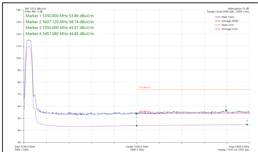
Figure 26 - Narrowband HDR8, SISO, Core 1 - 5245 MHz Band Edge Frequency 5350 MHz
