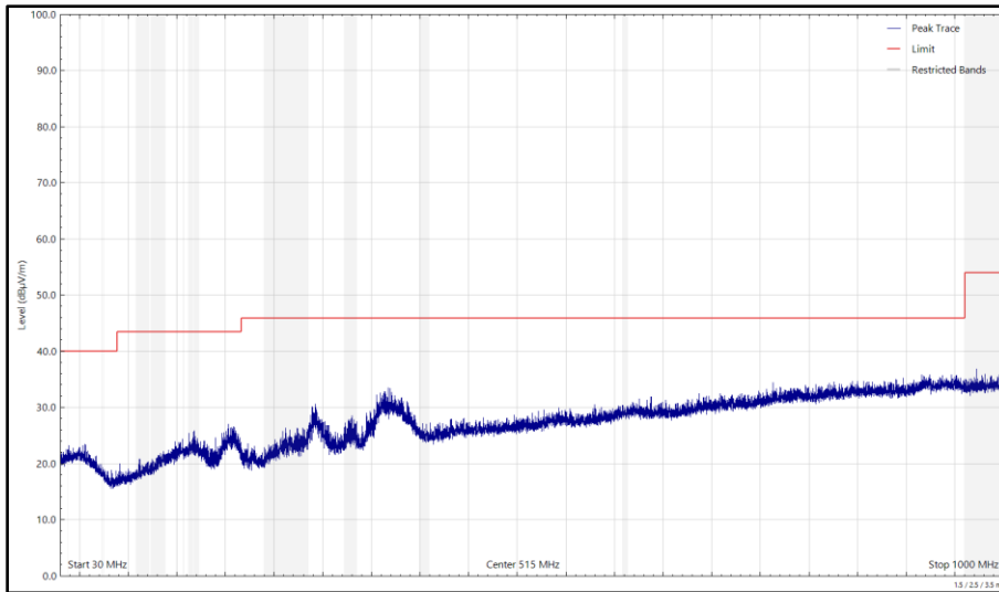
Figure 205 - 2442 MHz (CH7), 802.11g, Core 0, 30 MHz to 1 GHz, Horizontal (Peak)
