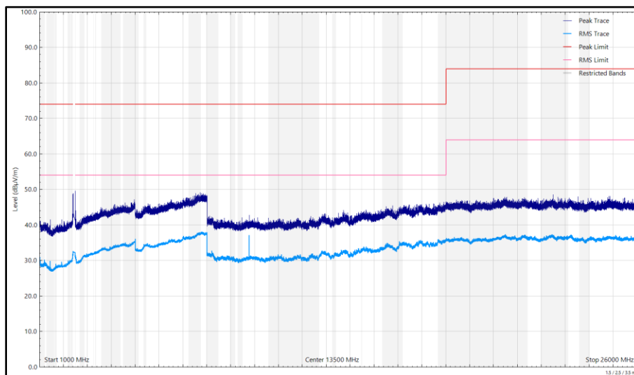
Figure 192 - 2442 MHz (CH7), 802.11b, Core 0, 1 GHz to 26 GHz, Vertical
