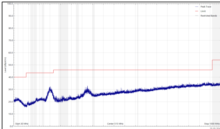
Figure 198 - 2442 MHz (CH7), 802.11b, Core 1, 30 MHz to 1 GHz, Vertical (Peak)
