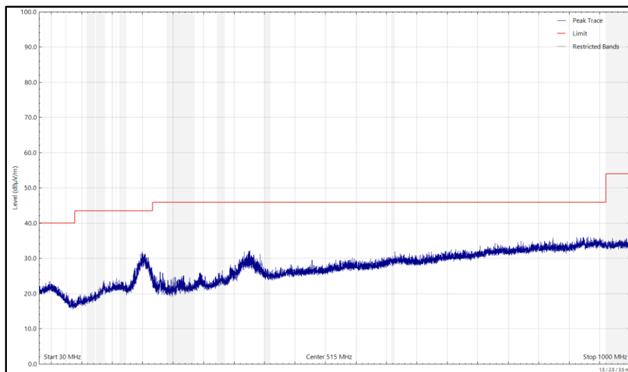
Figure 214 - 2442 MHz (CH7), 802.11g, Core 1, 30 MHz to 1 GHz, Vertical (Peak)
