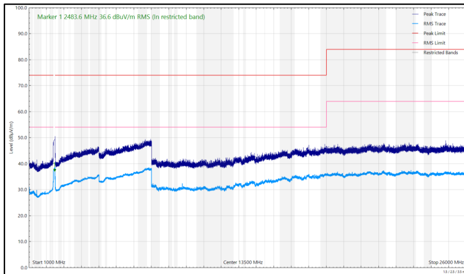
Figure 223 - 2442 MHz (CH7), HT20, CDD, Core 0 + Core 1, 1 GHz to 26 GHz, Horizontal
