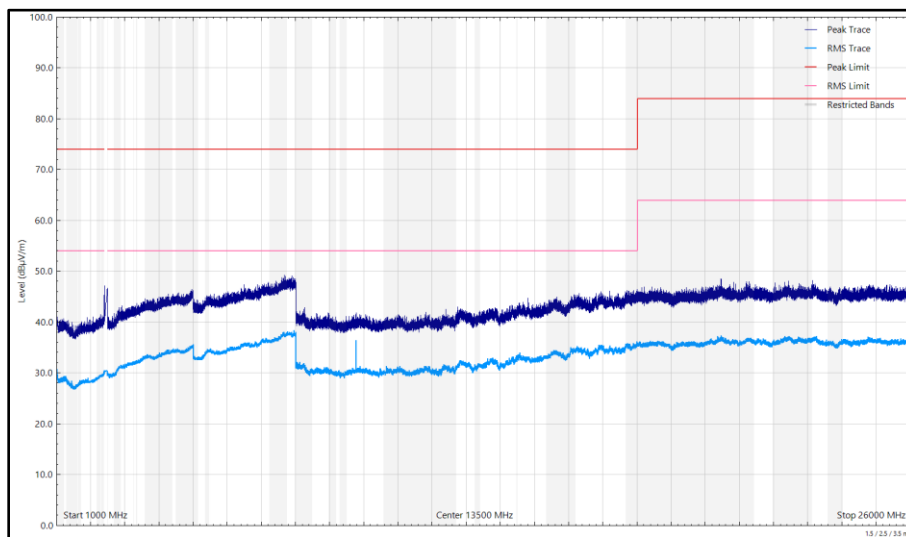
Figure 200 - 2442 MHz (CH7), 802.11b, Core 1, 1 GHz to 26 GHz, Vertical
