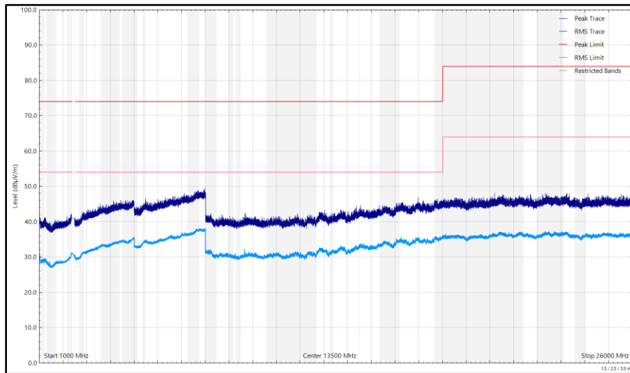
Figure 203 - 2412 MHz (CH1), 802.11g, Core 0, 1 GHz to 26 GHz, Horizontal
