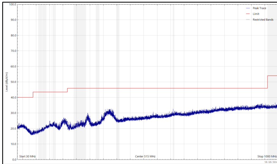
Figure 189 - 2442 MHz (CH7), 802.11b, Core 0, 30 MHz to 1 GHz, Horizontal (Peak)
