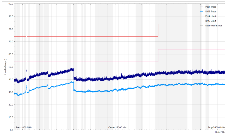
Figure 231 - 2442 MHz (CH7), HE20, RU26-0, CDD, Core 0 + Core 1, 1 GHz to 26 GHz, Horizontal
