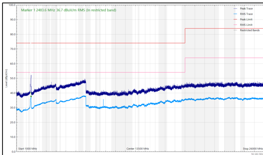
Figure 208 - 2442 MHz (CH7), 802.11g, Core 0, 1 GHz to 26 GHz, Vertical
