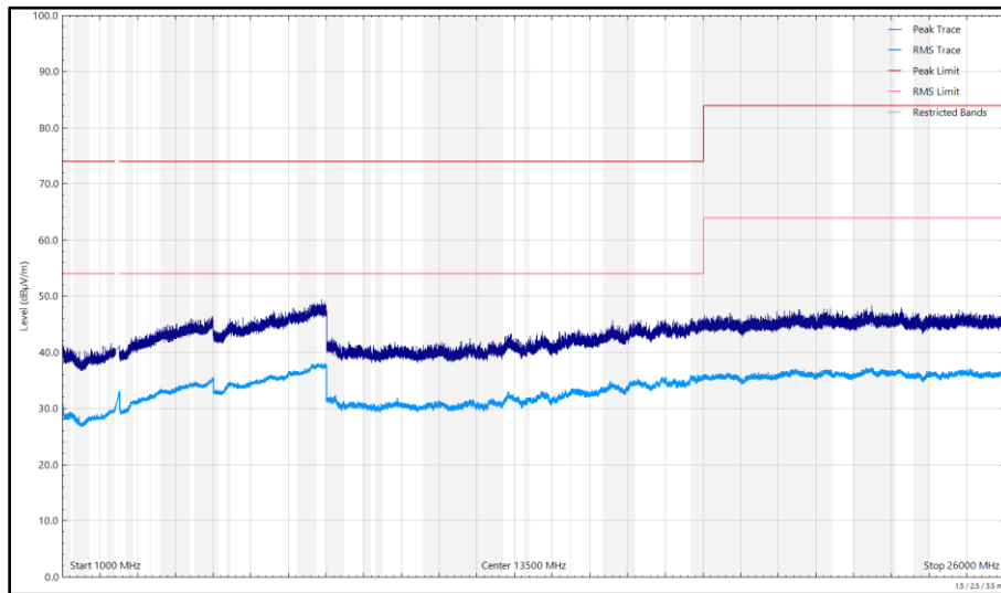
Figure 193 - 2472 MHz (CH13), 802.11b, Core 0, 1 GHz to 26 GHz, Horizontal
