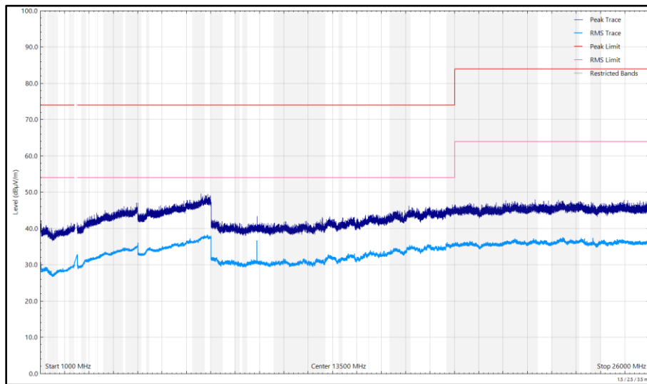
Figure 194 - 2472 MHz (CH13), 802.11b, Core 0, 1 GHz to 26 GHz, Vertical
