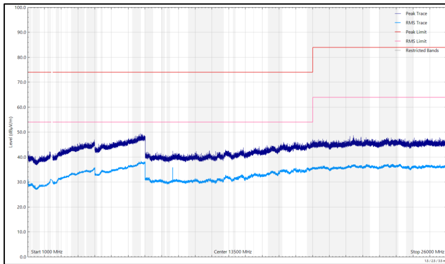
Figure 204 - 2412 MHz (CH1), 802.11g, Core 0, 1 GHz to 26 GHz, Vertical
