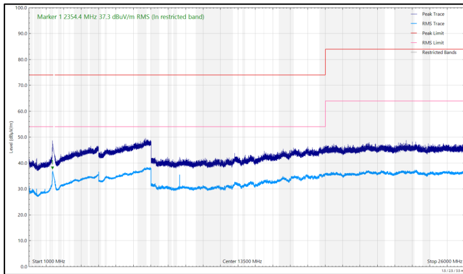
Figure 220 - 2412 MHz (CH1), HT20, CDD, Core 0 + Core 1, 1 GHz to 26 GHz, Vertical
