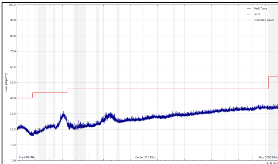
Figure 206 - 2442 MHz (CH7), 802.11g, Core 0, 30 MHz to 1 GHz, Vertical (Peak)
