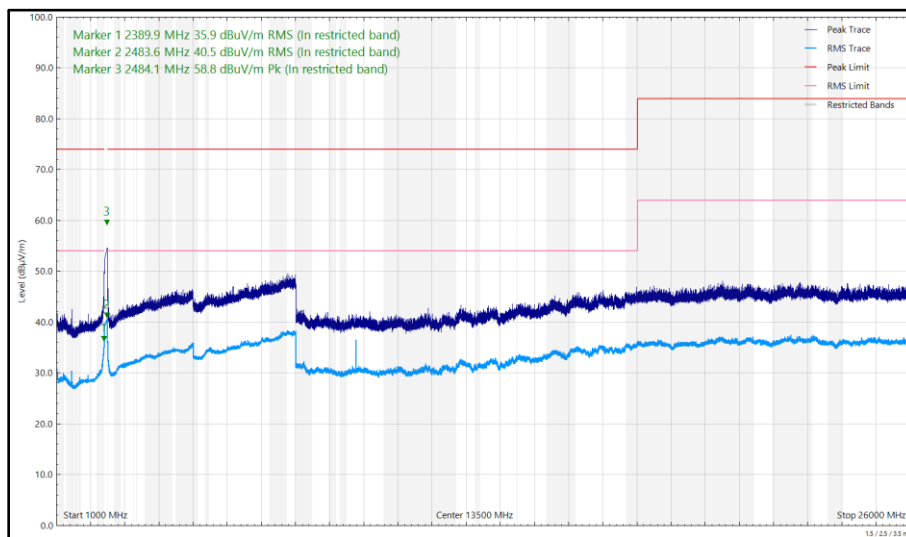
Figure 216 - 2442 MHz (CH7), 802.11g, Core 1, 1 GHz to 26 GHz, Vertical
