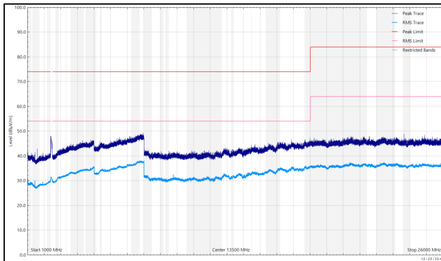
Figure 191 - 2442 MHz (CH7), 802.11b, Core 0, 1 GHz to 26 GHz, Horizontal
