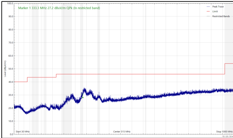
Figure 229 - 2442 MHz (CH7), HE20, RU26-0, CDD, Core 0 + Core 1, 30 MHz to 1 GHz, Horizontal (Peak)
