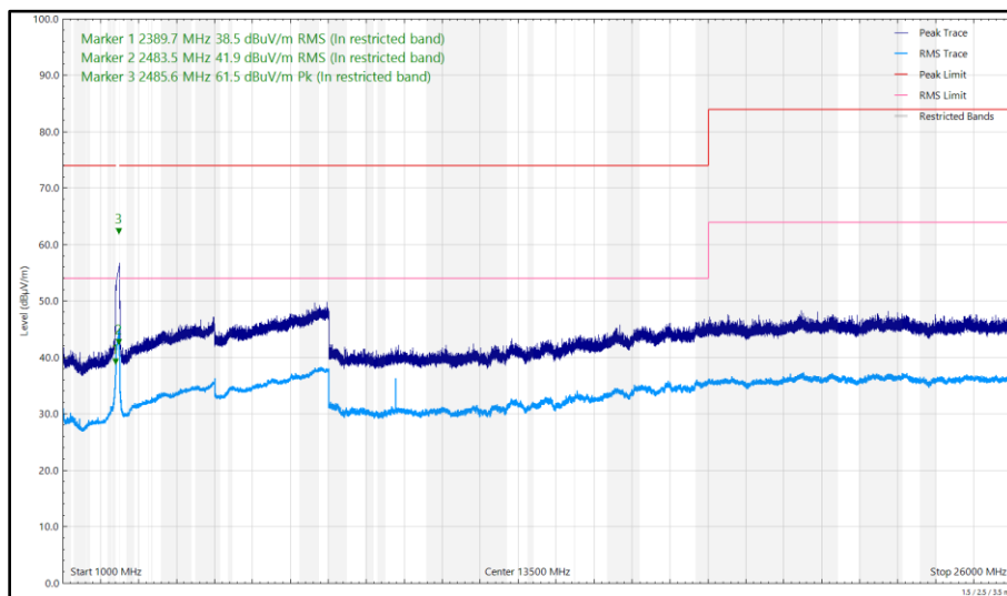
Figure 224 - 2442 MHz (CH7), HT20, CDD, Core 0 + Core 1, 1 GHz to 26 GHz, Vertical
