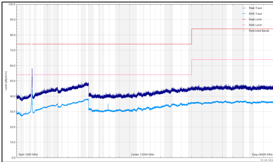
Figure 234 - 2472 MHz (CH13), HE20, RU26-0, CDD, Core 0 + Core 1, 1 GHz to 26 GHz, Vertical
