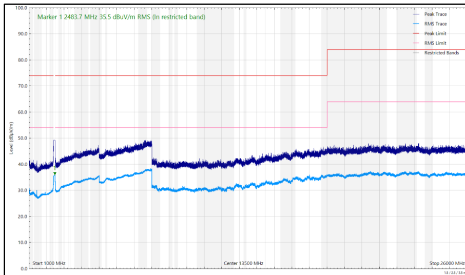
Figure 215 - 2442 MHz (CH7), 802.11g, Core 1, 1 GHz to 26 GHz, Horizontal
