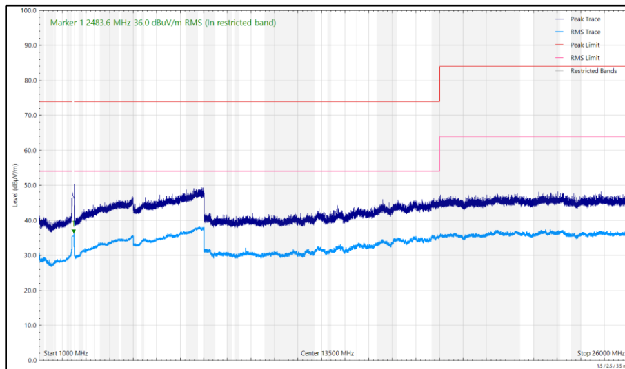
Figure 207 - 2442 MHz (CH7), 802.11g, Core 0, 1 GHz to 26 GHz, Horizontal
