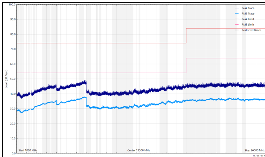
Figure 187 - 2412 MHz (CH1), 802.11b, Core 0, 1 GHz to 26 GHz, Horizontal
