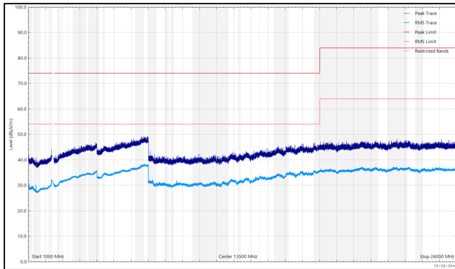
Figure 219 - 2412 MHz (CH1), HT20, CDD, Core 0 + Core 1, 1 GHz to 26 GHz, Horizontal
