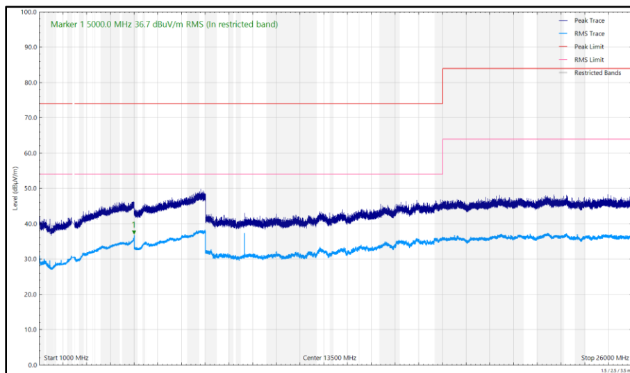
Figure 188 - 2412 MHz (CH1), 802.11b, Core 0, 1 GHz to 26 GHz, Vertical
