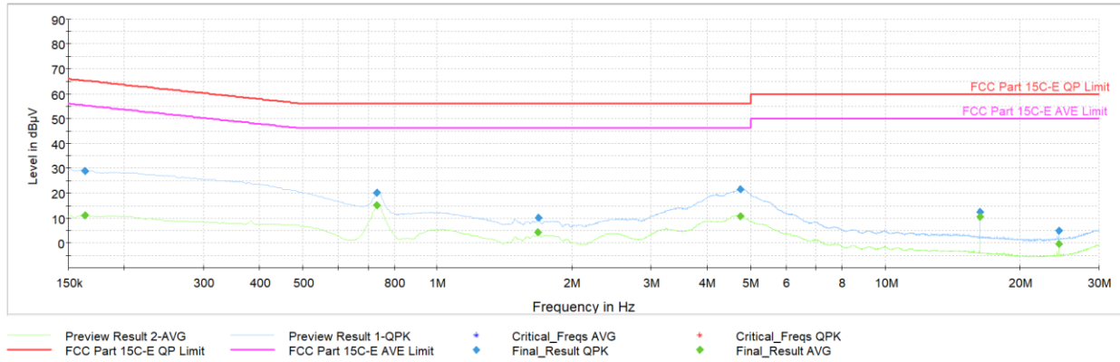
Plot 7-38. AC Line-Conducted Test Plot (L1, GFSK – Ch.39, with AC/DC Adapter)
