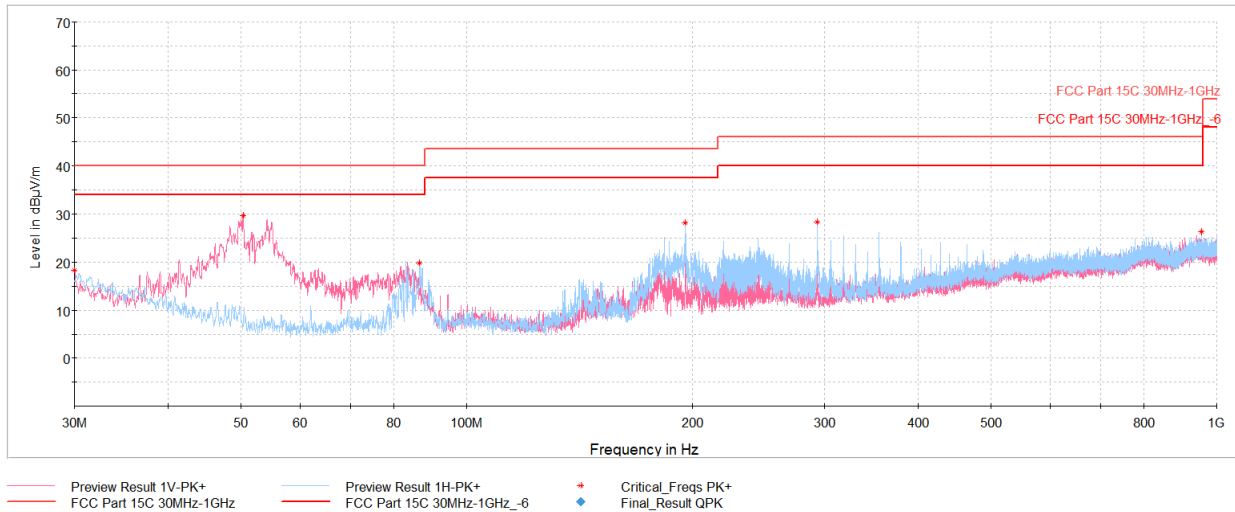
Plot 7-37. Radiated Spurious Emissions Below 1GHz (GFSK – Ch.39, with AC/DC Adapter)
