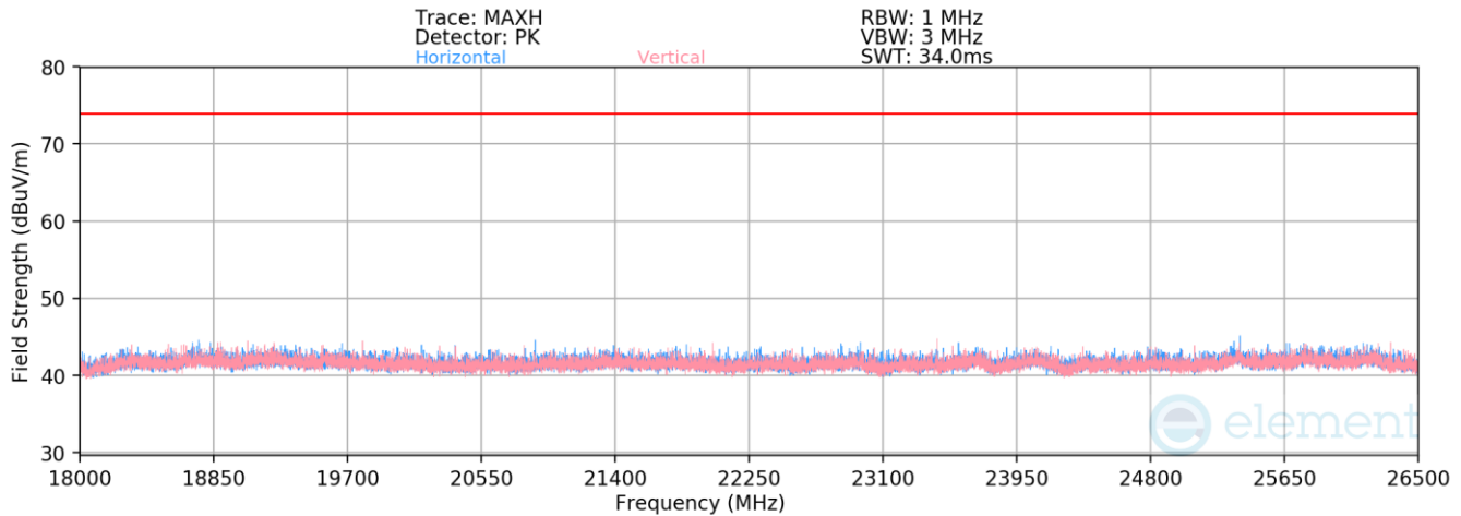
Plot 7-31. Radiated Spurious Emissions Above 18GHz (BT GFSK – Ch. 39)
