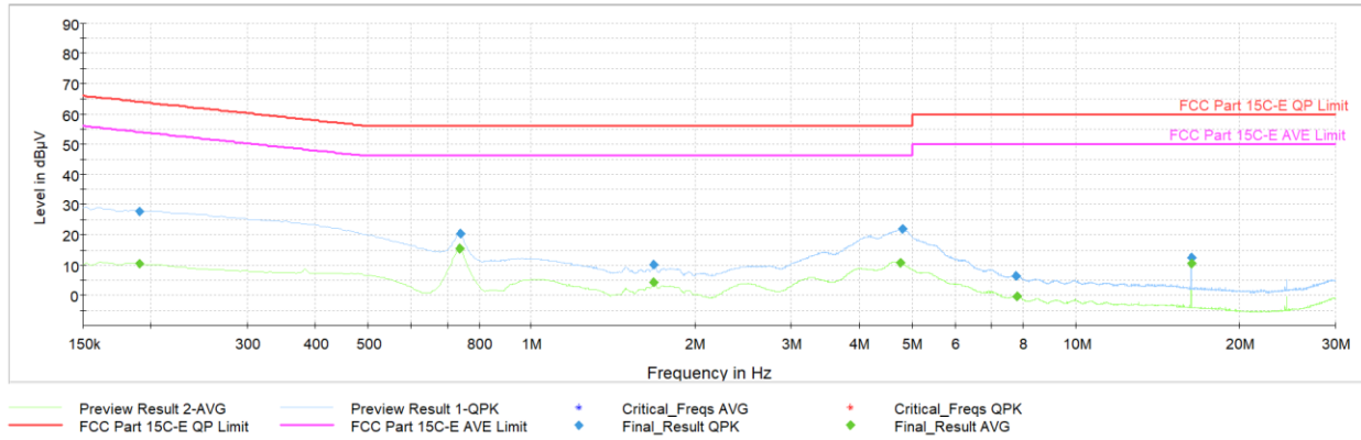
Plot 7-39. AC Line-Conducted Test Plot (N, GFSK – Ch.39, with AC/DC Adapter)
