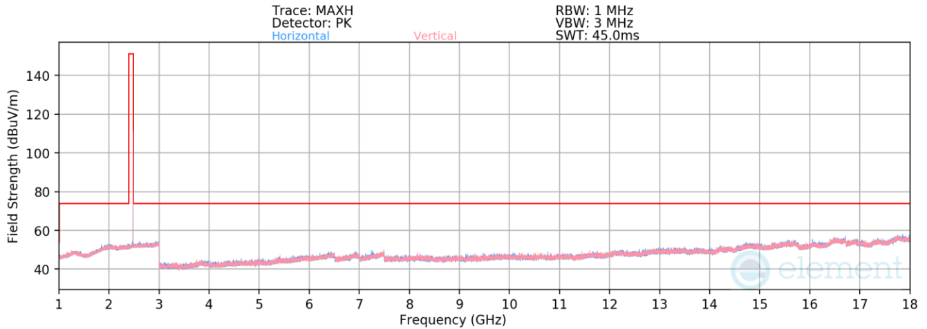
Plot 7-32. Radiated Spurious Emissions above 1GHz (BT GFSK – Ch. 78)
