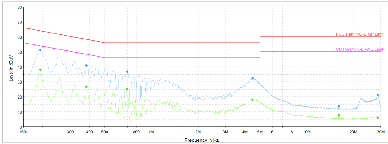
Plot 7-33. AC Line Conducted Plot with Bluetooth LE (N, 1Mbps – Ch.39, with AC/DC Adapter)
