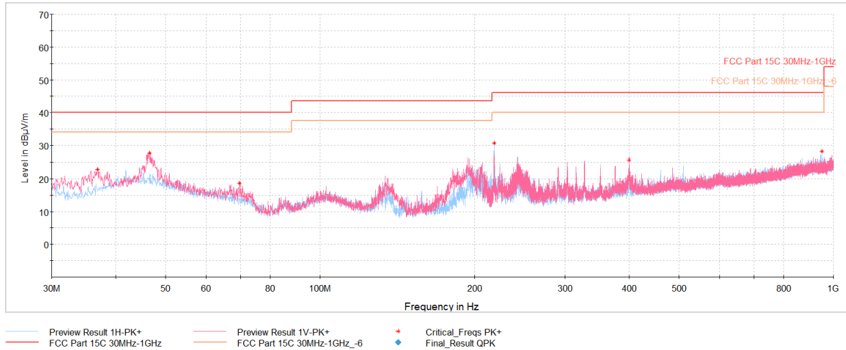
Plot 7-31. Radiated Spurious Emissions Below 1GHz (1Mbps – Ch.39, Pol. H & V, with AC/DC Adapter)
