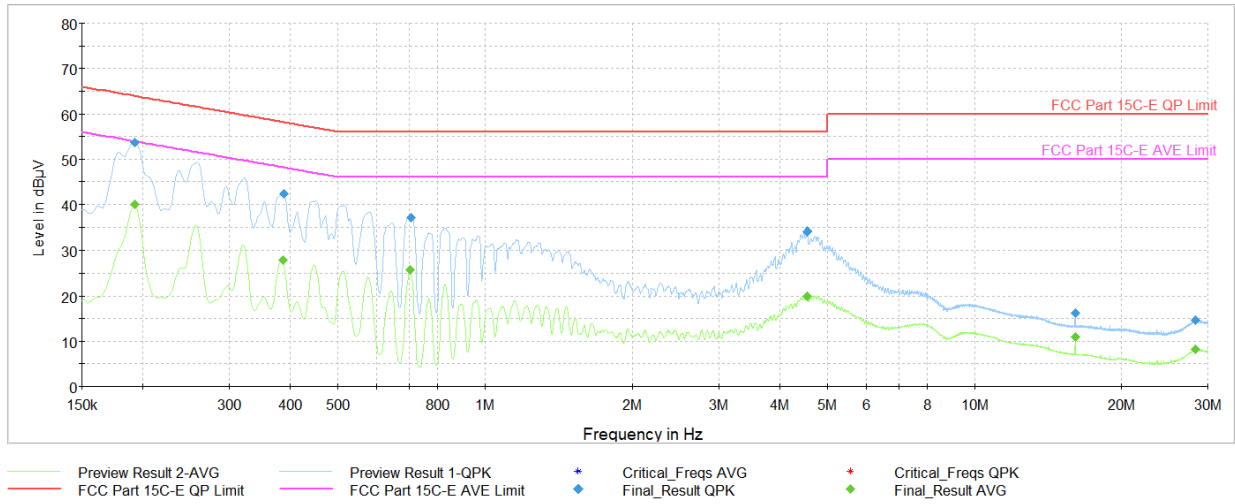
Plot 7-32. AC Line Conducted Plot with Bluetooth LE (L1, 1Mbps – Ch.39, with AC/DC Adapter)
