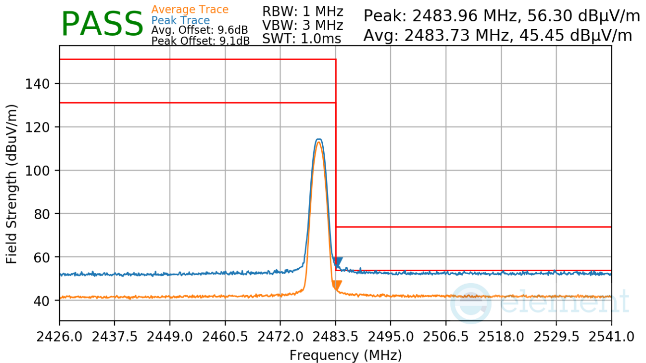
Plot 7-28. Radiated Restricted Upper Band Edge Measurement (Average & Peak)
