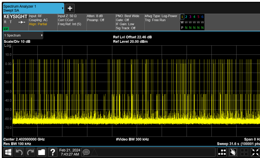
Figure 8 - \pi/4 DQPSK - 2402 MHz Accumulated Transmit Time
