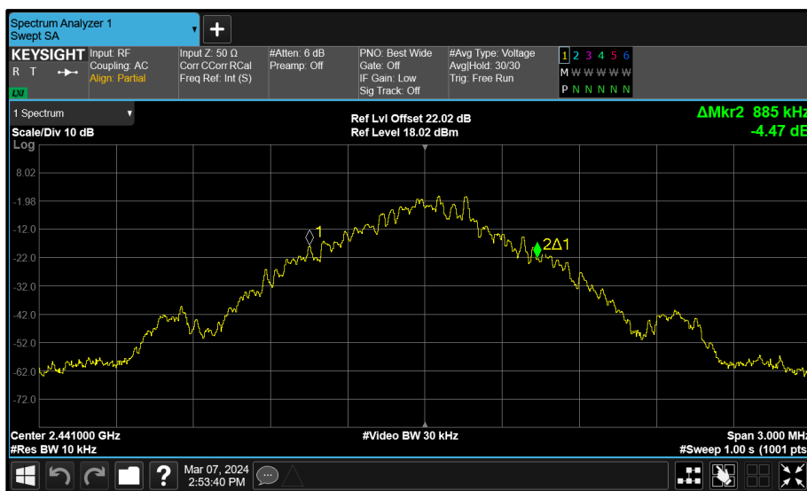
Figure 20 - Core 0 (A) 2441 MHz (CH39) 99% Bandwidth
