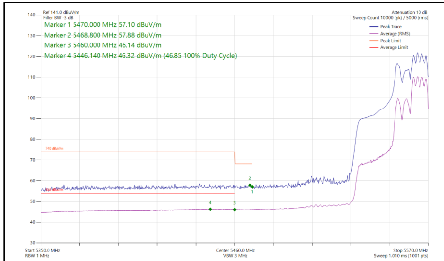
Figure 531 - 802.11ax HE40, RU 106-56, SDM, Core 0 - Core 1 - 5550 MHz Band Edge Frequency 5470 MHz
