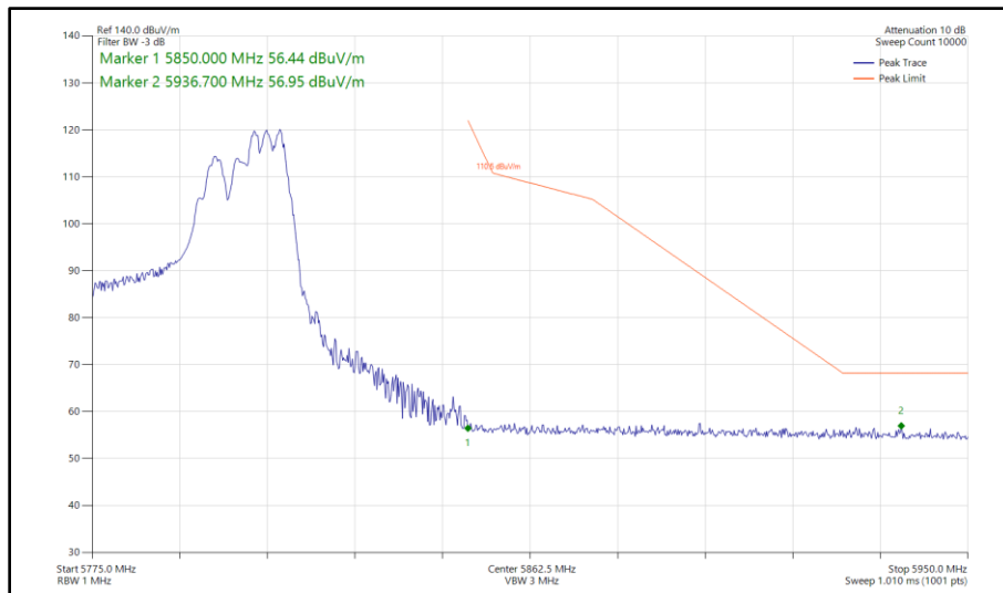
Figure 525 - 802.11ax HE40, RU 106-56, CDD, Core 0 - Core 1 - 5795 MHz Band Edge Frequency 5850 MHz
