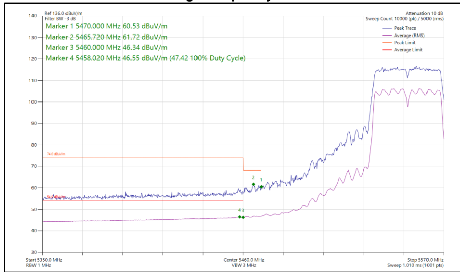
Figure 527 - 802.11n HT40, SDM, Core 0 - Core 1 - 5550 MHz Band Edge Frequency 5470 MHz
