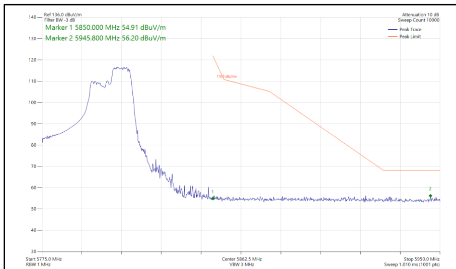
Figure 505 - 802.11ax HE40, RU 106-56, SISO, Core 1 - 5795 MHz Band Edge Frequency 5850 MHz
