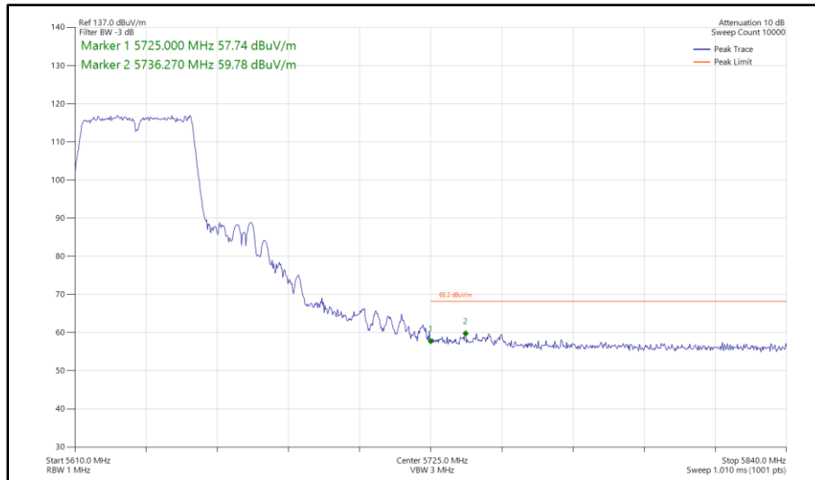
Figure 535 - 802.11n HT40, SDM, Core 0 - Core 1 - 5630 MHz Band Edge Frequency 5725 MHz
