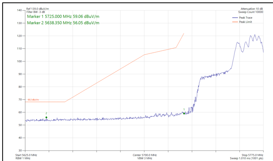
Figure 514 - 802.11ax HE40, RU 106-56, CDD, Core 0 - Core 1 - 5755 MHz Band Edge Frequency 5725 MHz
