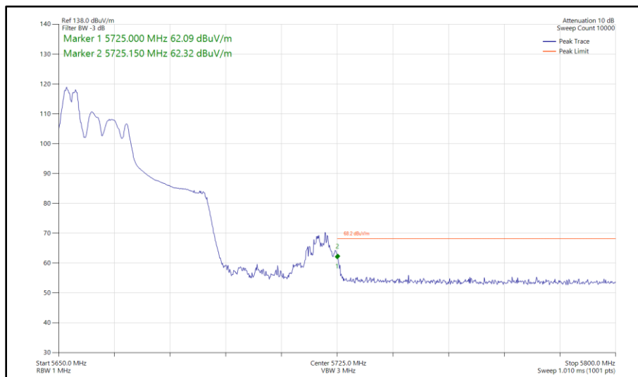
Figure 540 - 802.11ax HE40, RU 52-37, SDM, Core 0 - Core 1 - 5670 MHz Band Edge Frequency 5725 MHz
