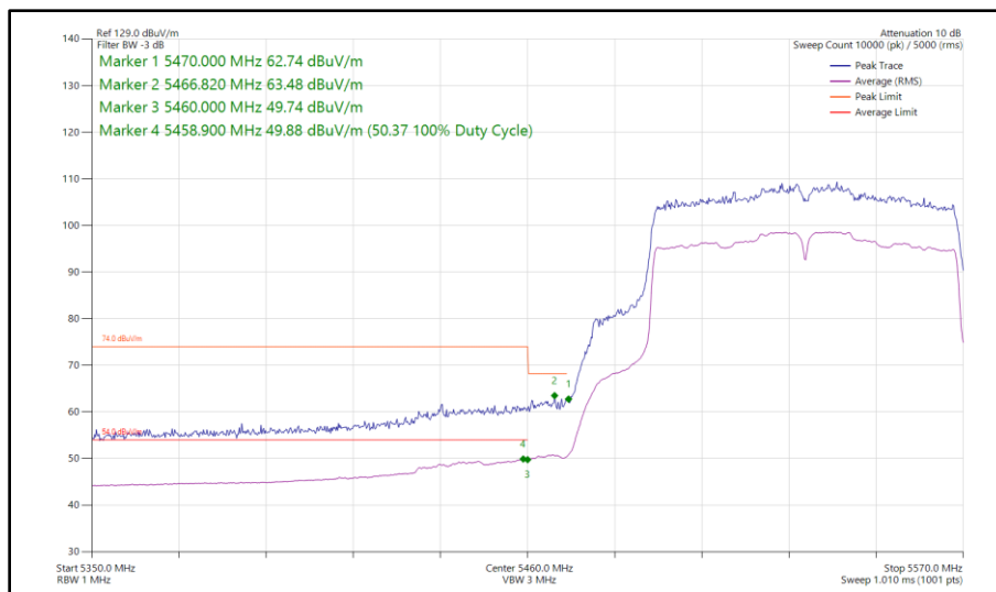
Figure 554 - 802.11ac VHT80, SISO, Core 0 - 5530 MHz Band Edge Frequency 5470 MHz
