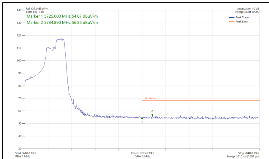
Figure 497 - 802.11ax HE40, RU 106-56, SISO, Core 1 - 5630 MHz Band Edge Frequency 5725 MHz
