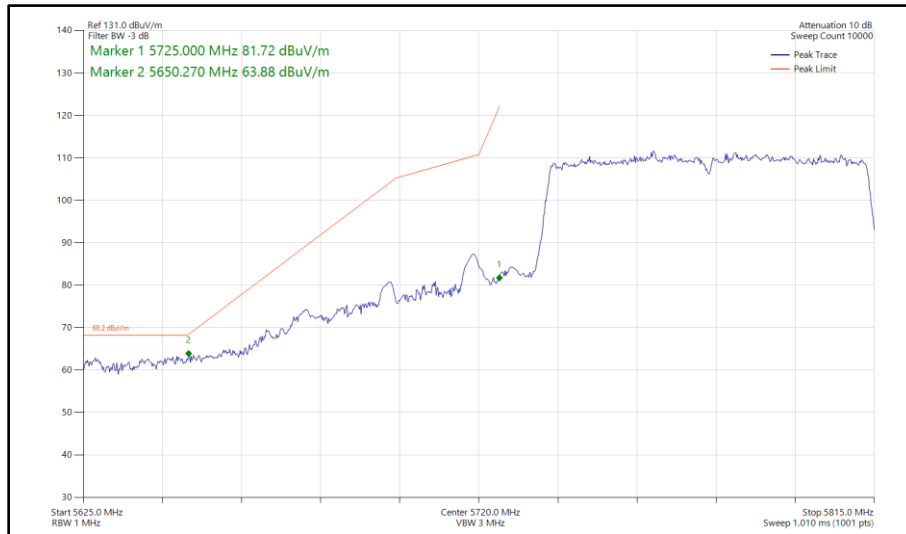
Figure 572 - 802.11ac VHT80, SISO, Core 1 - 5775 MHz Band Edge Frequency 5725 MHz
