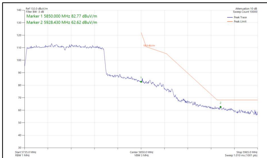
Figure 564 - 802.11ac VHT80, SISO, Core 0 - 5775 MHz Band Edge Frequency 5850 MHz
