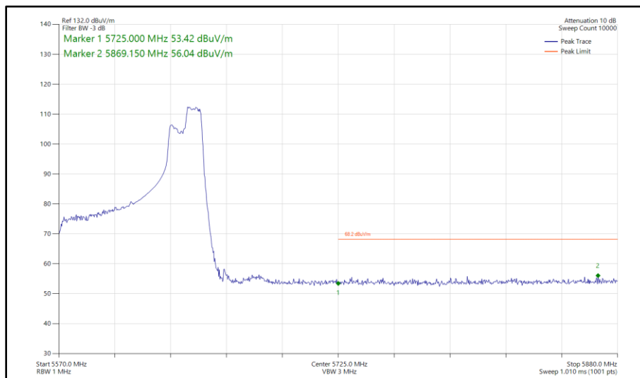
Figure 577 - 802.11ax HE80, RU 106-60, SISO, Core 1 - 5610 MHz Band Edge Frequency 5725 MHz
