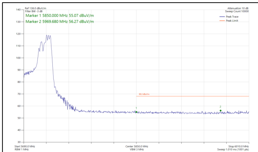
Figure 544 - 802.11ax HE40, RU 106-56, SDM, Core 0 - Core 1 - 5710 MHz Band Edge Frequency 5850 MHz
