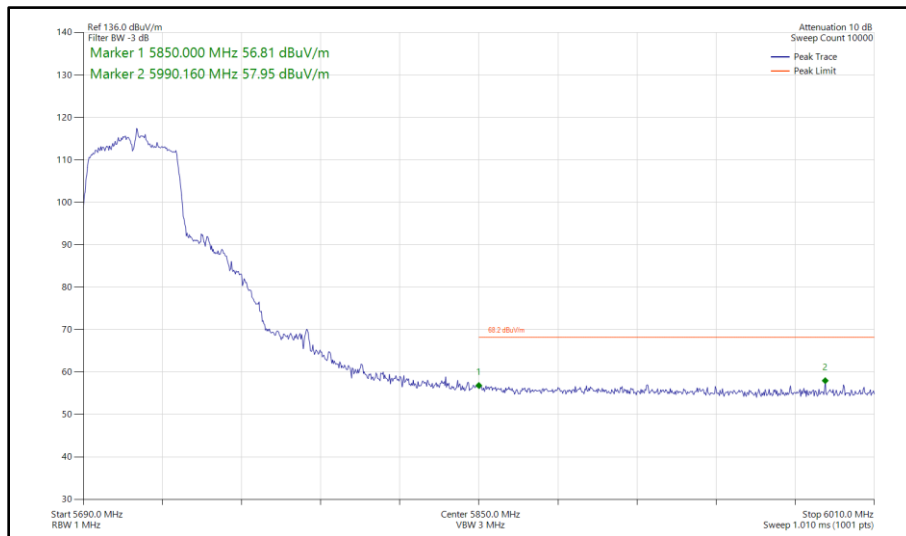
Figure 500 - 802.11n HT40, SISO, Core 1 - 5710 MHz Band Edge Frequency 5850 MHz
