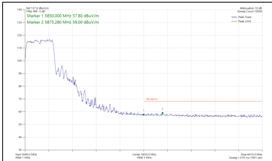
Figure 552 - 802.11ac VHT40, TxBF, Core 0 - Core 1 - 5710 MHz Band Edge Frequency 5850 MHz
