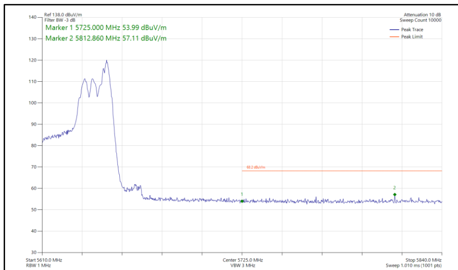
Figure 538 - 802.11ax HE40, RU 52-44, SDM, Core 0 - Core 1 - 5630 MHz Band Edge Frequency 5725 MHz
