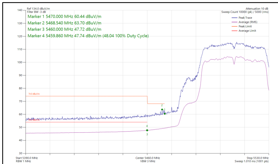
Figure 547 - 802.11ac VHT40, TxBF, Core 0 - Core 1 - 5510 MHz Band Edge Frequency 5470 MHz
