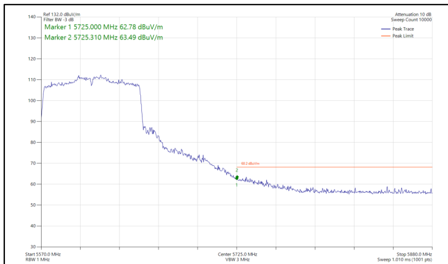
Figure 575 - 802.11ac VHT80, SISO, Core 1 - 5610 MHz Band Edge Frequency 5725 MHz
