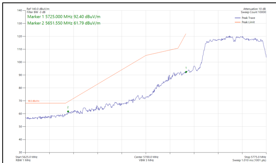
Figure 532 - 802.11n HT40, SDM, Core 0 - Core 1 - 5755 MHz Band Edge Frequency 5725 MHz
