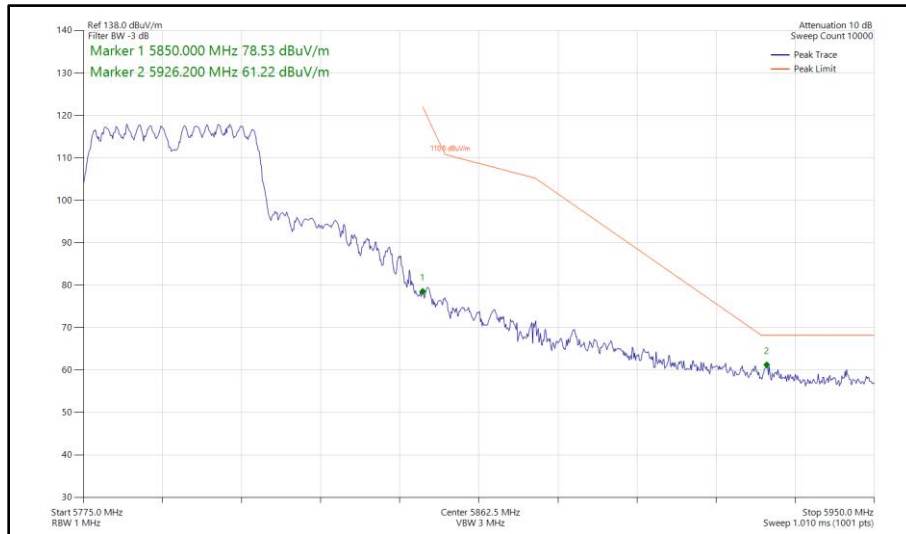
Figure 521 - 802.11n HT40, CDD, Core 0 - Core 1 - 5795 MHz Band Edge Frequency 5850 MHz
