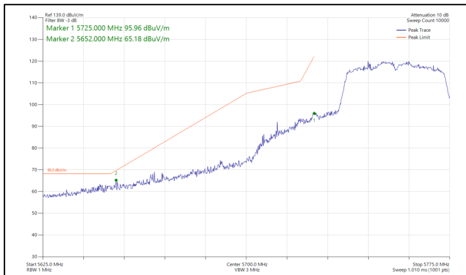
Figure 549 - 802.11ac VHT40, TxBF, Core 0 - Core 1 - 5755 MHz Band Edge Frequency 5725 MHz
