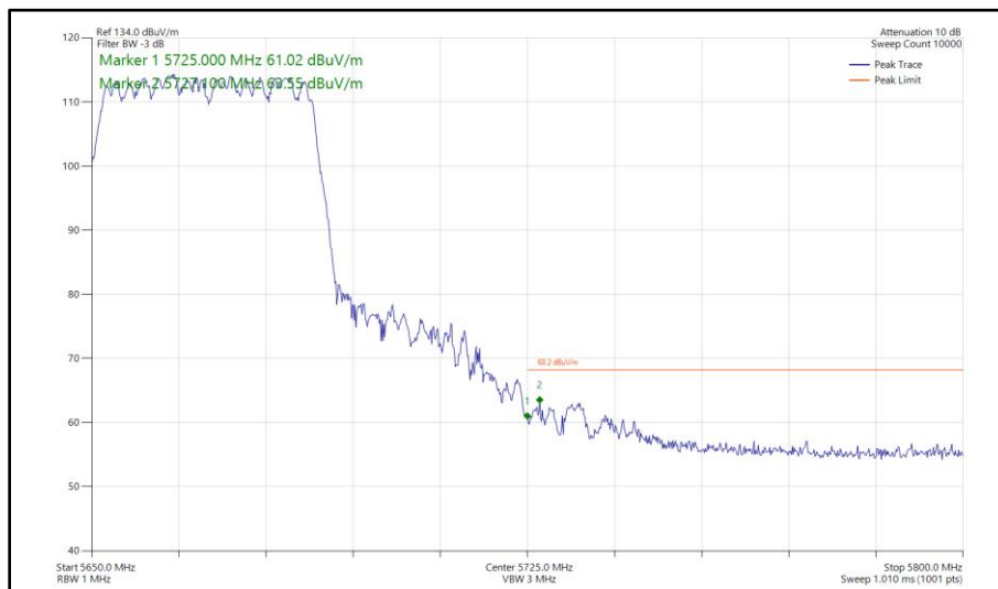
Figure 516 - 802.11n HT40, CDD, Core 0 - Core 1 - 5670 MHz Band Edge Frequency 5725 MHz
