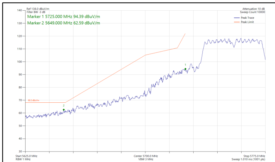
Figure 512 - 802.11n HT40, CDD, Core 0 - Core 1 - 5755 MHz Band Edge Frequency 5725 MHz
