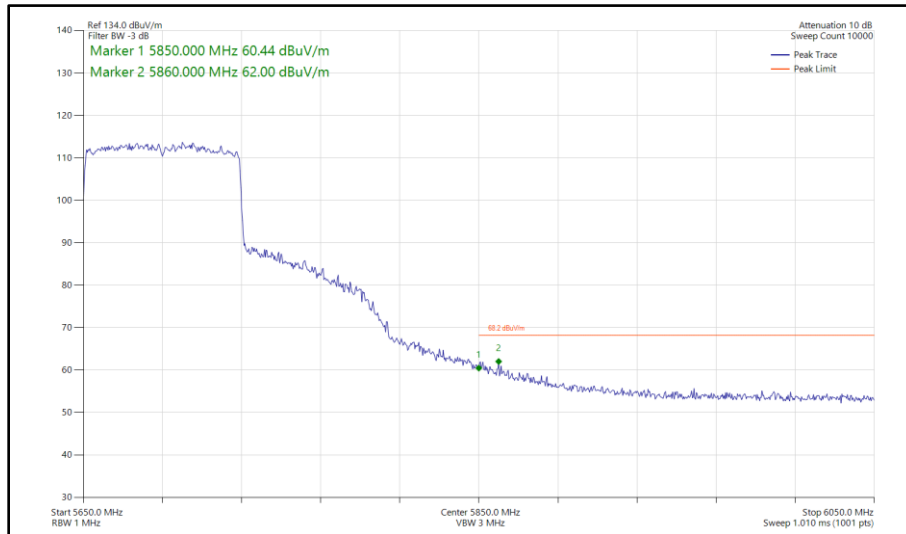
Figure 565 - 802.11ax HE80, SU, SISO, Core 0 - 5690 MHz Band Edge Frequency 5850 MHz
