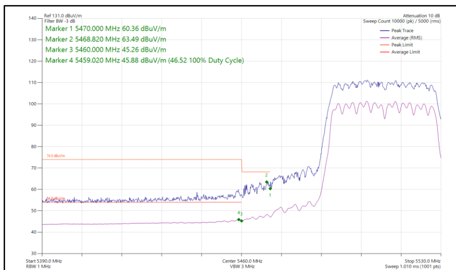
Figure 506 - 802.11n HT40, CDD, Core 0 - Core 1 - 5510 MHz Band Edge Frequency 5470 MHz
