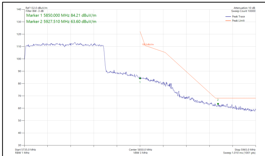
Figure 567 - 802.11ax HE80, SU, SISO, Core 0 - 5775 MHz Band Edge Frequency 5850 MHz
