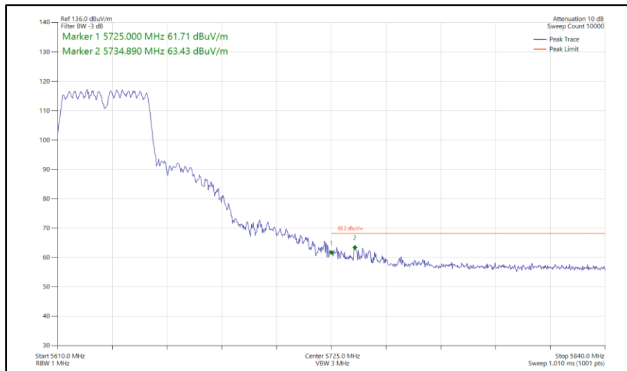
Figure 515 - 802.11n HT40, CDD, Core 0 - Core 1 - 5630 MHz Band Edge Frequency 5725 MHz
