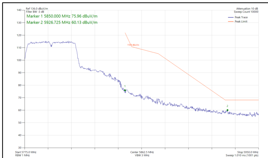
Figure 501 - 802.11n HT40, SISO, Core 1 - 5795 MHz Band Edge Frequency 5850 MHz
