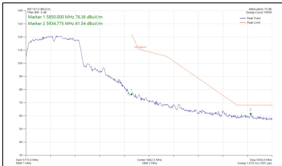
Figure 542 - 802.11n HT40, SDM, Core 0 - Core 1 - 5795 MHz Band Edge Frequency 5850 MHz
