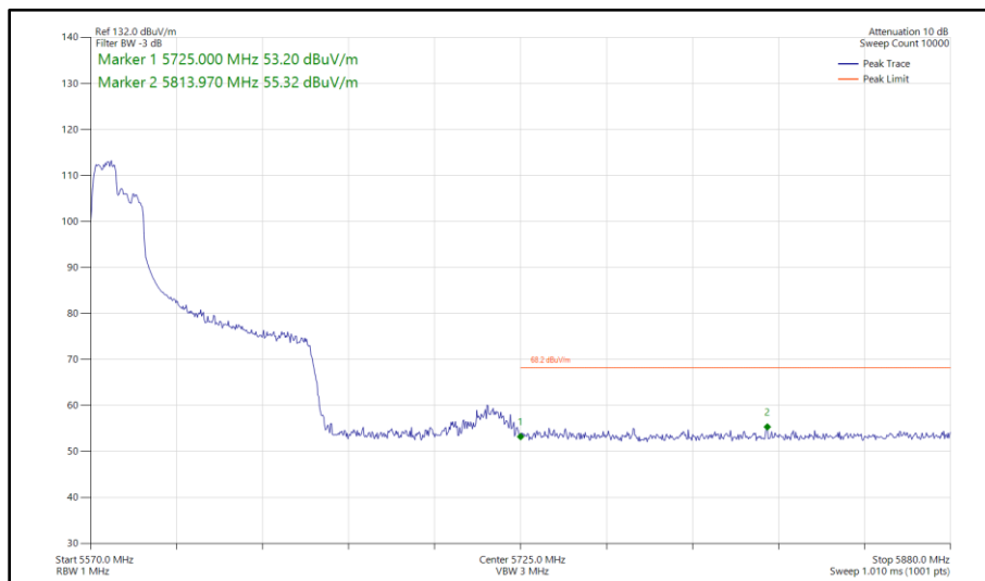
Figure 562 - 802.11ax HE80, RU 106-53, SISO, Core 0 - 5610 MHz Band Edge Frequency 5725 MHz
