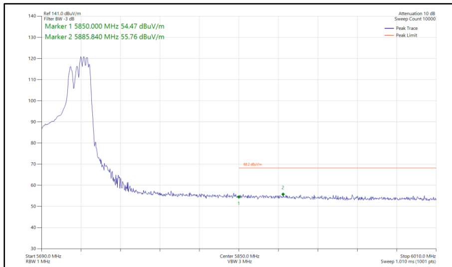
Figure 523 - 802.11ax HE40, RU 106-56, CDD, Core 0 - Core 1 - 5710 MHz Band Edge Frequency 5850 MHz
