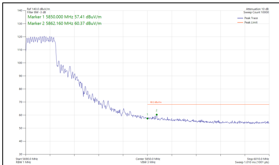
Figure 522 - 802.11ax HE40, SU, CDD, Core 0 - Core 1 - 5710 MHz Band Edge Frequency 5850 MHz
