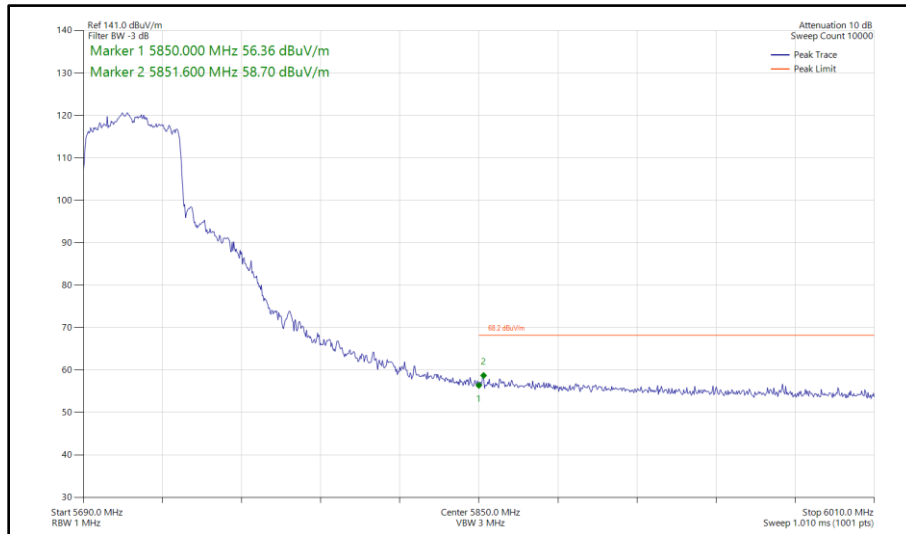
Figure 543 - 802.11ax HE40, SU, SDM, Core 0 - Core 1 - 5710 MHz Band Edge Frequency 5850 MHz
