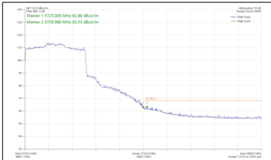
Figure 561 - 802.11ax HE80, SU, SISO, Core 0 - 5610 MHz Band Edge Frequency 5725 MHz
