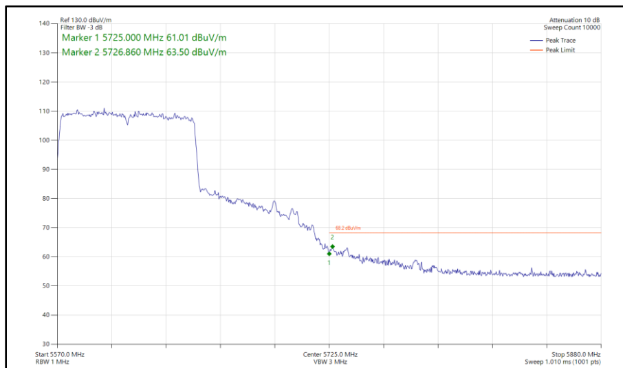
Figure 560 - 802.11ac VHT80, SISO, Core 0 - 5610 MHz Band Edge Frequency 5725 MHz
