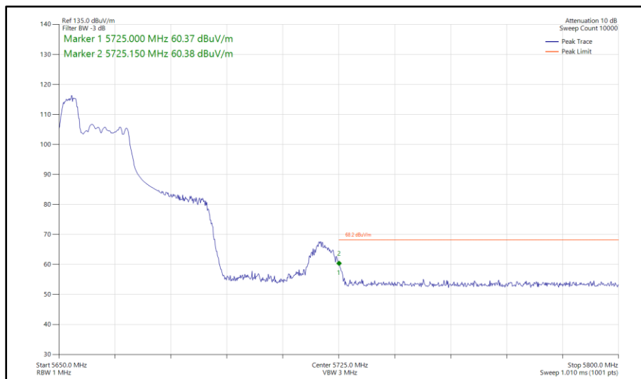
Figure 499 - 802.11ax HE40, RU 52-37, SISO, Core 1 - 5670 MHz Band Edge Frequency 5725 MHz
