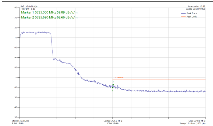
Figure 537 - 802.11ax HE40, SU, SDM, Core 0 - Core 1 - 5630 MHz Band Edge Frequency 5725 MHz
