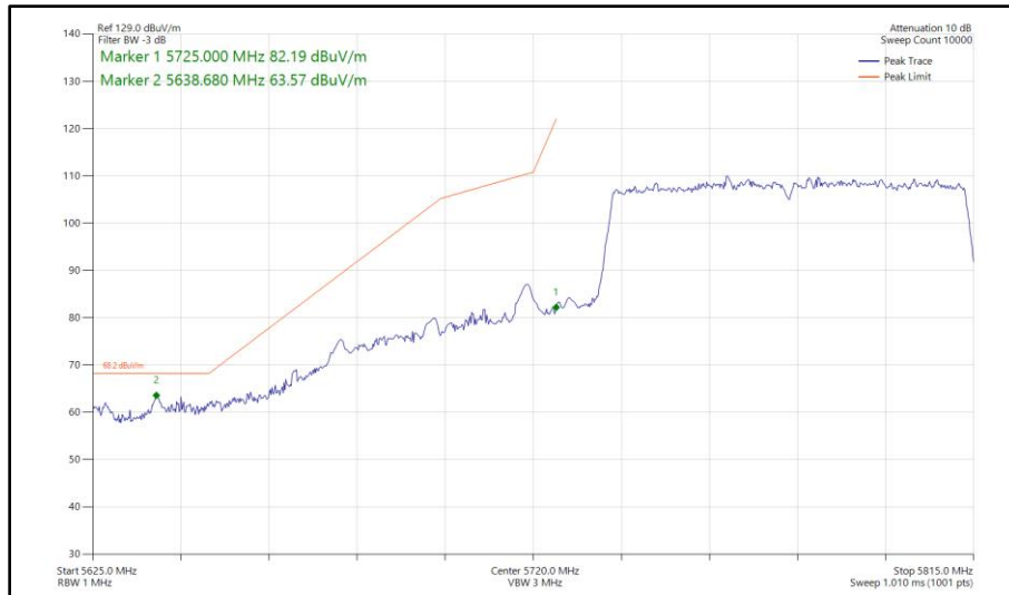
Figure 557 - 802.11ac VHT80, SISO, Core 0 - 5775 MHz Band Edge Frequency 5725 MHz
