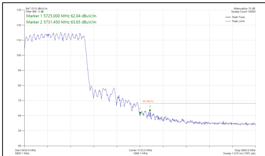
Figure 518 - 802.11ax HE40, SU, CDD, Core 0 - Core 1 - 5670 MHz Band Edge Frequency 5725 MHz
