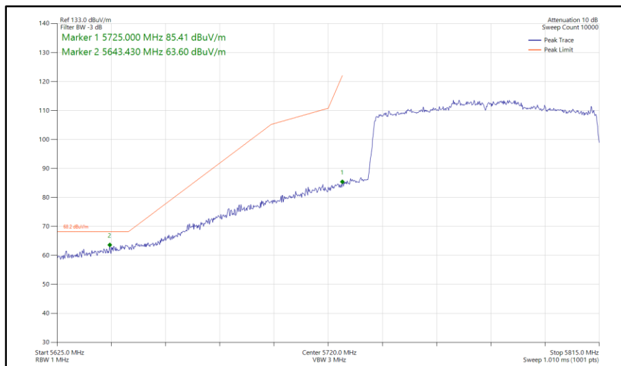
Figure 573 - 802.11ax HE80, SU, SISO, Core 1 - 5775 MHz Band Edge Frequency 5725 MHz
