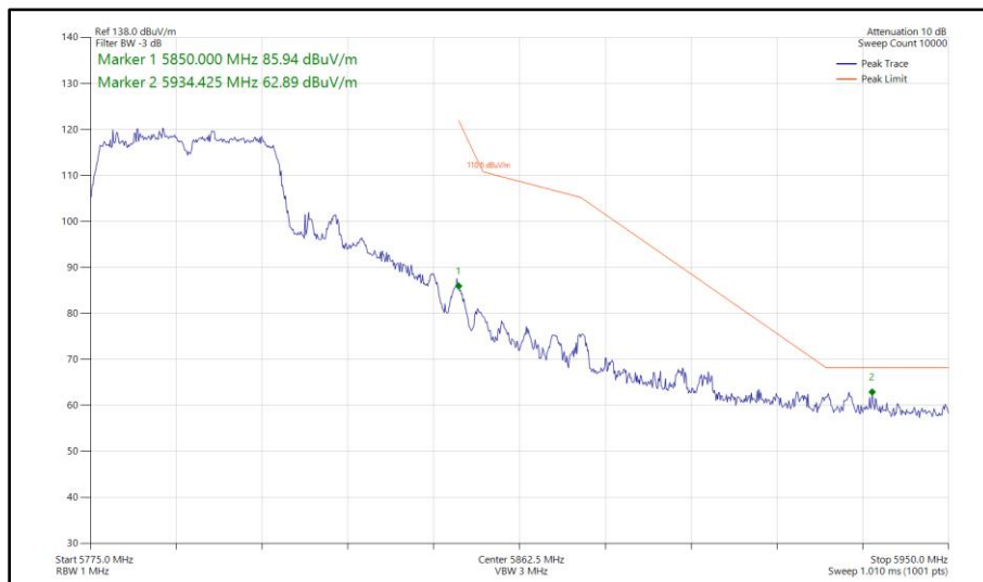
Figure 553 - 802.11ac VHT40, TxBF, Core 0 - Core 1 - 5795 MHz Band Edge Frequency 5850 MHz
