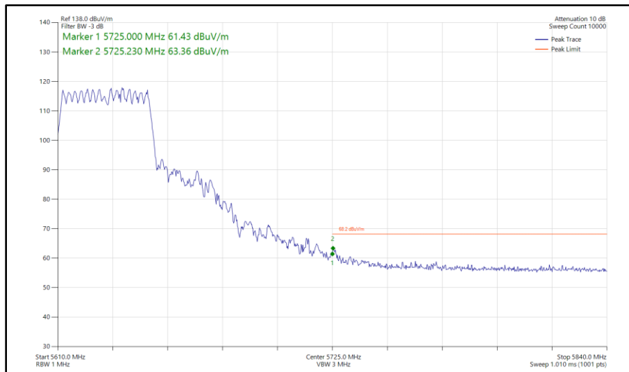
Figure 517 - 802.11ax HE40, SU, CDD, Core 0 - Core 1 - 5630 MHz Band Edge Frequency 5725 MHz
