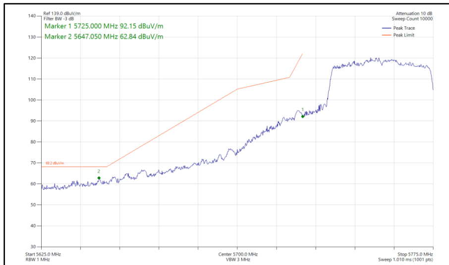
Figure 533 - 802.11ax HE40, SU, SDM, Core 0 - Core 1 - 5755 MHz Band Edge Frequency 5725 MHz
