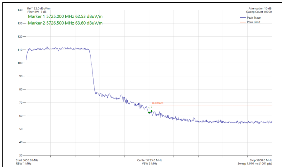
Figure 498 - 802.11ax HE40, SU, SISO, Core 1 - 5670 MHz Band Edge Frequency 5725 MHz
