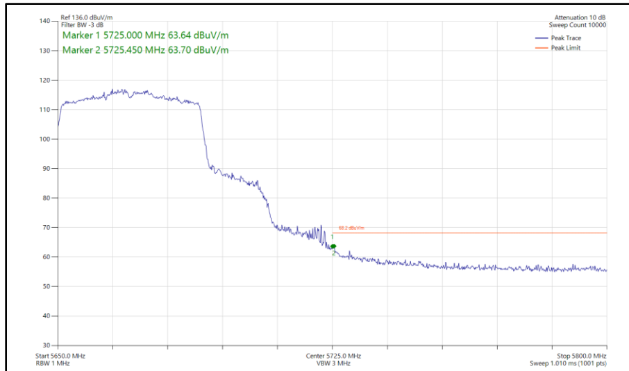
Figure 539 - 802.11ax HE40, SU, SDM, Core 0 - Core 1 - 5670 MHz Band Edge Frequency 5725 MHz
