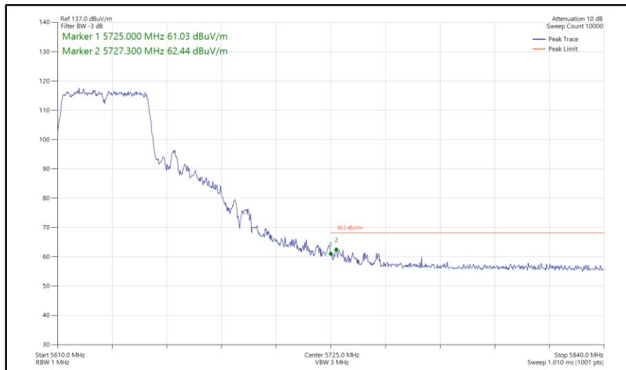
Figure 550 - 802.11ac VHT40, TxBF, Core 0 - Core 1 - 5630 MHz Band Edge Frequency 5725 MHz
