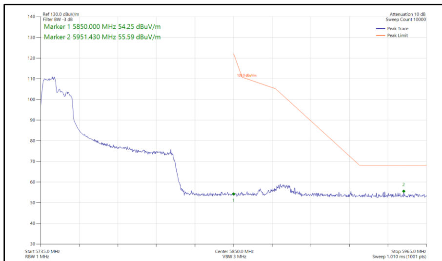
Figure 568 - 802.11ax HE80, RU 106-53, SISO, Core 0 - 5775 MHz Band Edge Frequency 5850 MHz
