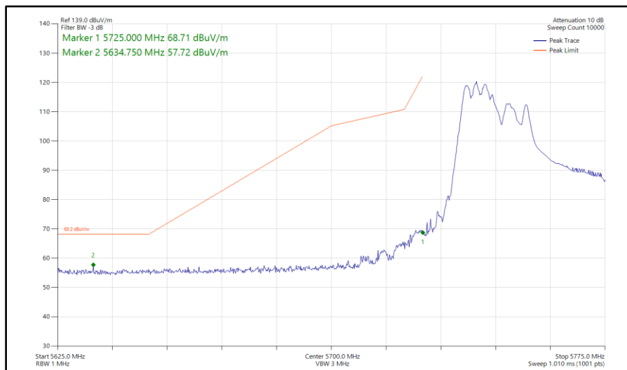
Figure 534 - 802.11ax HE40, RU 106-53, SDM, Core 0 - Core 1 - 5755 MHz Band Edge Frequency 5725 MHz
