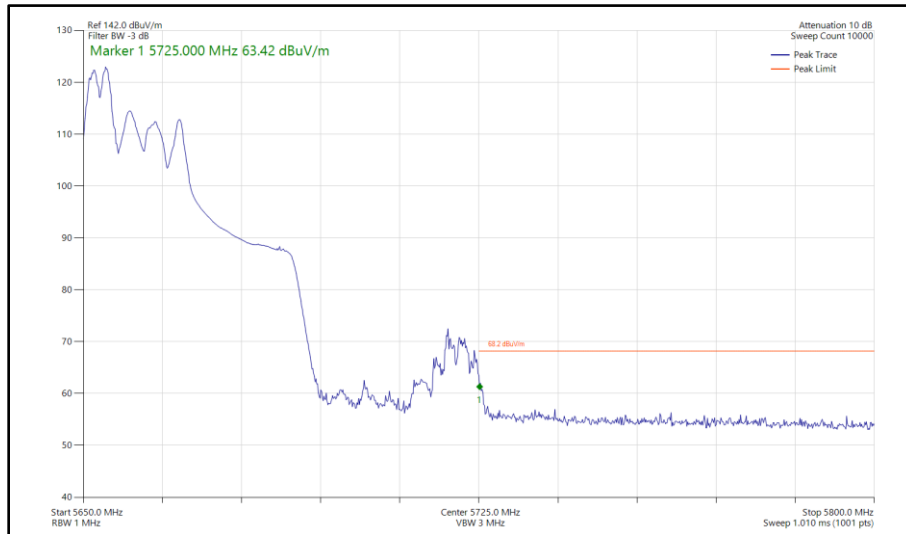
Figure 519 - 802.11ax HE40, RU 52-37, CDD, Core 0 - Core 1 - 5670 MHz Band Edge Frequency 5725 MHz
