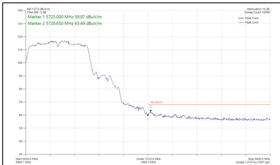
Figure 536 - 802.11n HT40, SDM, Core 0 - Core 1 - 5670 MHz Band Edge Frequency 5725 MHz
