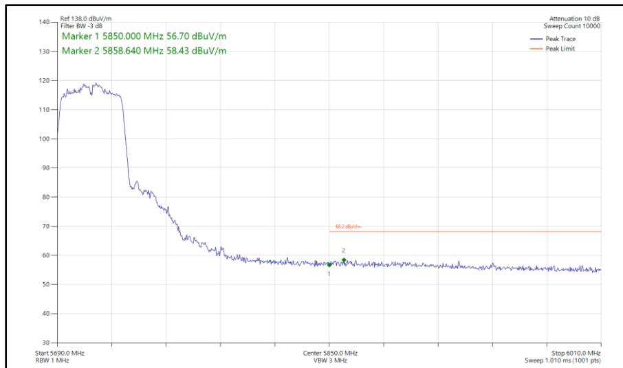
Figure 541 - 802.11n HT40, SDM, Core 0 - Core 1 - 5710 MHz Band Edge Frequency 5850 MHz
