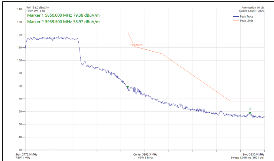
Figure 545 - 802.11ax HE40, SU, SDM, Core 0 - Core 1 - 5795 MHz Band Edge Frequency 5850 MHz
