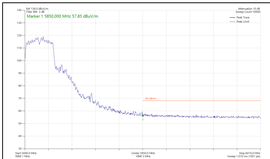
Figure 520 - 802.11n HT40, CDD, Core 0 - Core 1 - 5710 MHz Band Edge Frequency 5850 MHz
