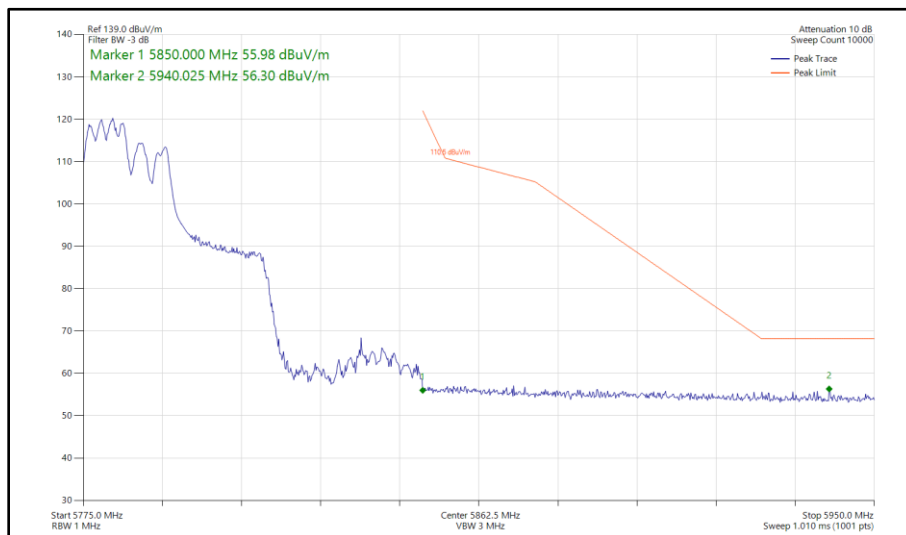
Figure 546 - 802.11ax HE40, RU 106-53, SDM, Core 0 - Core 1 - 5795 MHz Band Edge Frequency 5850 MHz
