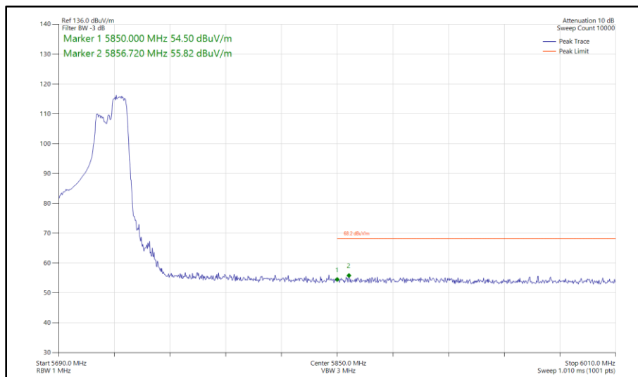
Figure 503 - 802.11ax HE40, RU 106-56, SISO, Core 1 - 5710 MHz Band Edge Frequency 5850 MHz
