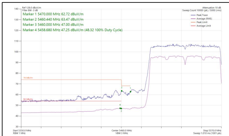
Figure 569 - 802.11ac VHT80, SISO, Core 1 - 5530 MHz Band Edge Frequency 5470 MHz
