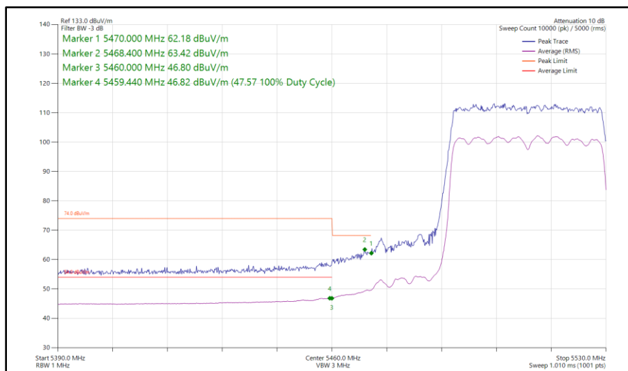
Figure 528 - 802.11ax HE40, SU, SDM, Core 0 - Core 1 - 5510 MHz Band Edge Frequency 5470 MHz
