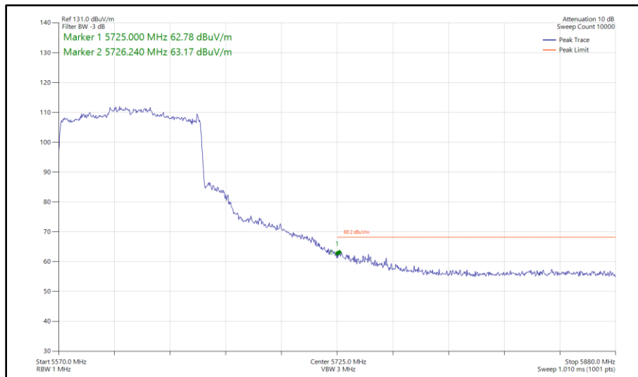
Figure 576 - 802.11ax HE80, SU, SISO, Core 1 - 5610 MHz Band Edge Frequency 5725 MHz
