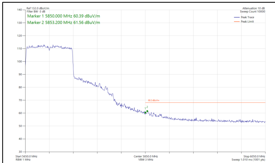
Figure 563 - 802.11ac VHT80, SISO, Core 0 - 5690 MHz Band Edge Frequency 5850 MHz
