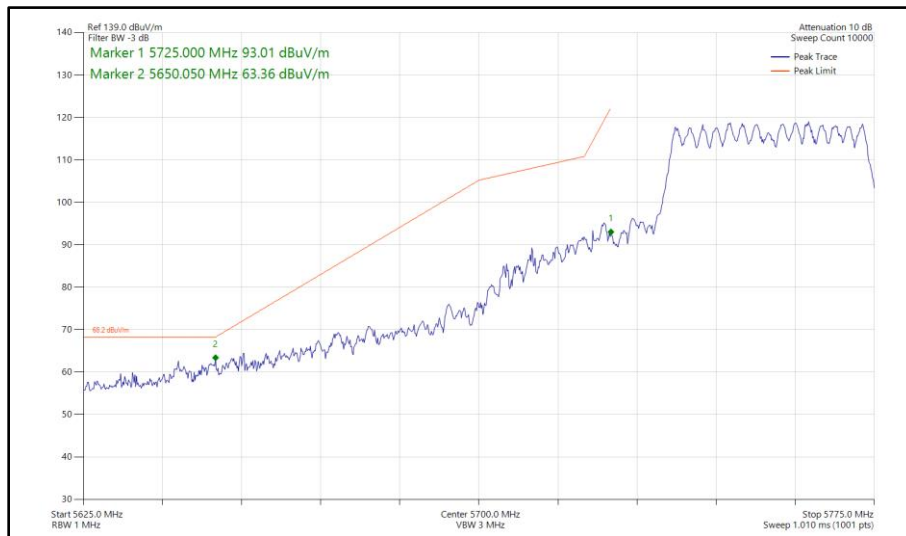
Figure 513 - 802.11ax HE40, SU, CDD, Core 0 - Core 1 - 5755 MHz Band Edge Frequency 5725 MHz
