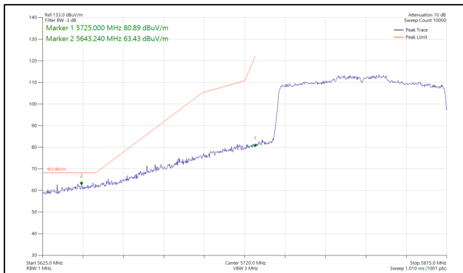
Figure 558 - 802.11ax HE80, SU, SISO, Core 0 - 5775 MHz Band Edge Frequency 5725 MHz
