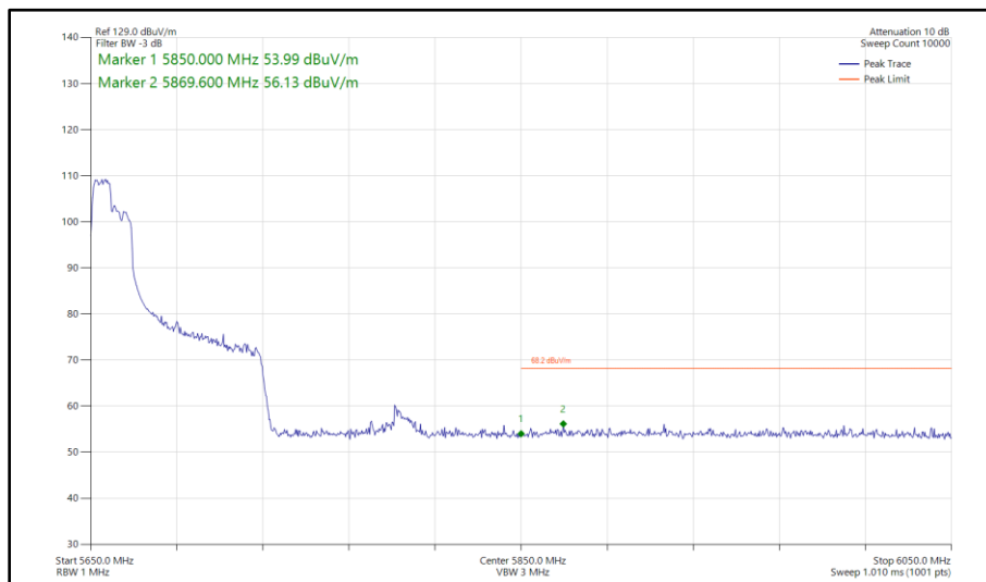
Figure 566 - 802.11ax HE80, RU 106-53, SISO, Core 0 - 5690 MHz Band Edge Frequency 5850 MHz
