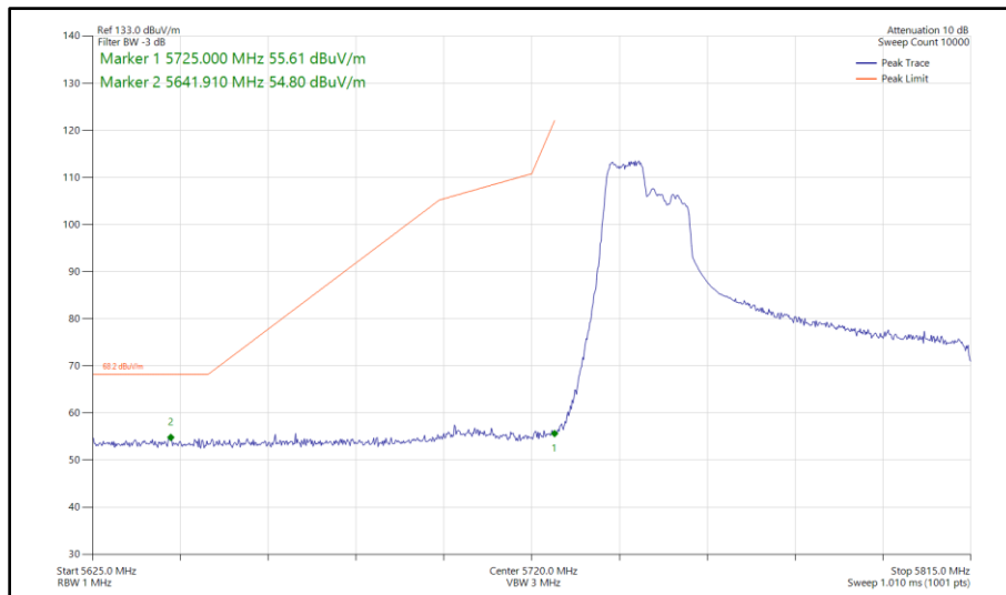
Figure 574 - 802.11ax HE80, RU 106-53, SISO, Core 1 - 5775 MHz Band Edge Frequency 5725 MHz
