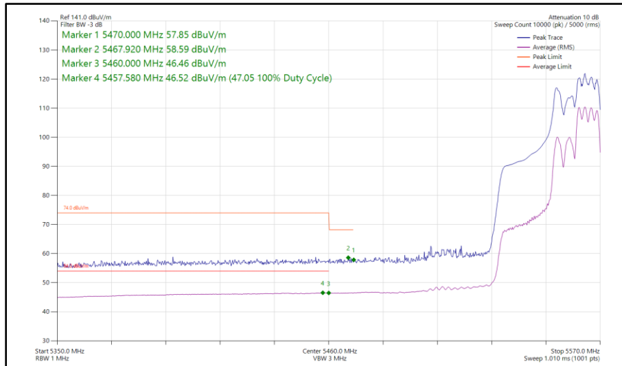
Figure 511 - 802.11ax HE40, RU 106-56, CDD, Core 0 - Core 1 - 5550 MHz Band Edge Frequency 5470 MHz
