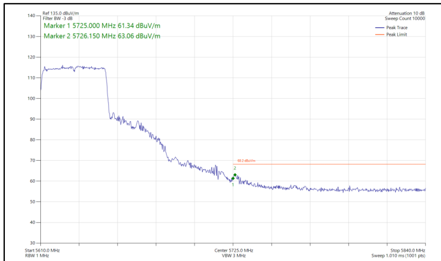
Figure 496 - 802.11ax HE40, SU, SISO, Core 1 - 5630 MHz Band Edge Frequency 5725 MHz
