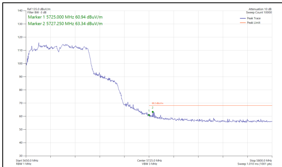
Figure 551 - 802.11ac VHT40, TxBF, Core 0 - Core 1 - 5670 MHz Band Edge Frequency 5725 MHz
