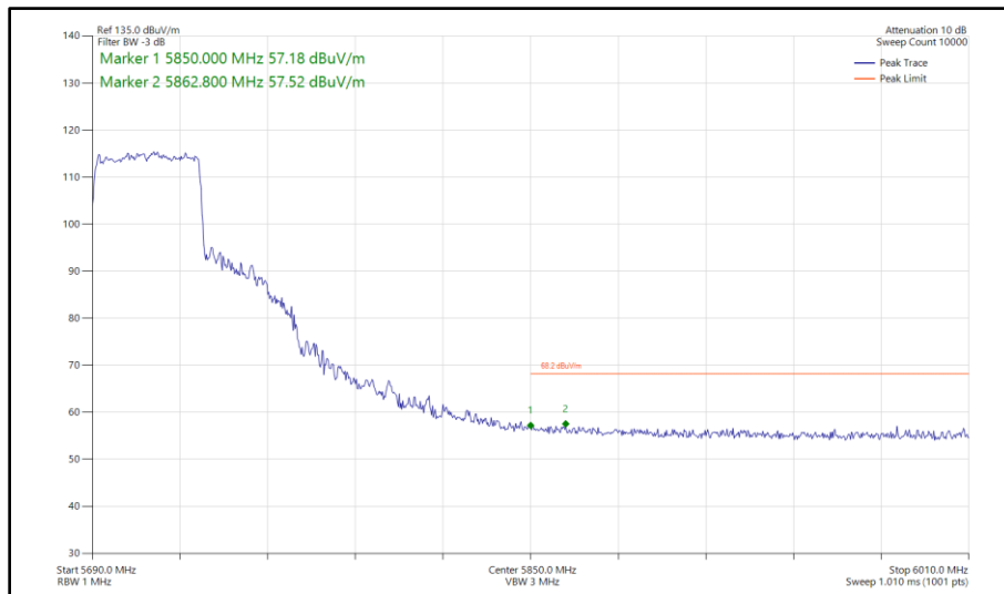
Figure 502 - 802.11ax HE40, SU, SISO, Core 1 - 5710 MHz Band Edge Frequency 5850 MHz
