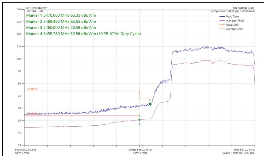
Figure 555 - 802.11ax HE80, SU, SISO, Core 0 - 5530 MHz Band Edge Frequency 5470 MHz
