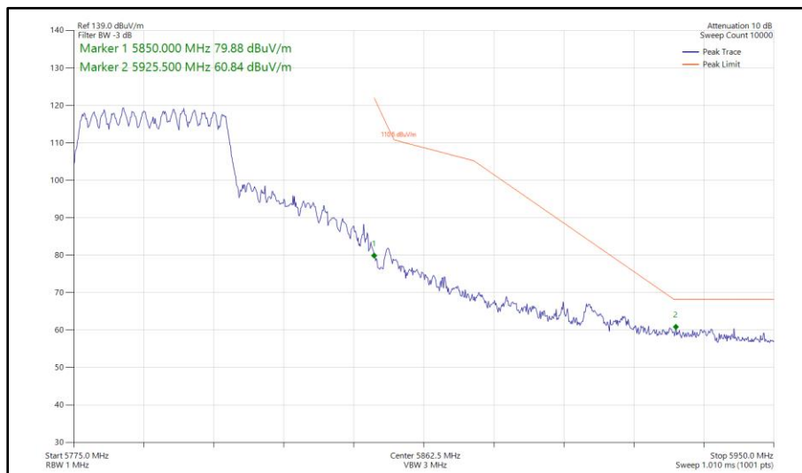
Figure 524 - 802.11ax HE40, SU, CDD, Core 0 - Core 1 - 5795 MHz Band Edge Frequency 5850 MHz
