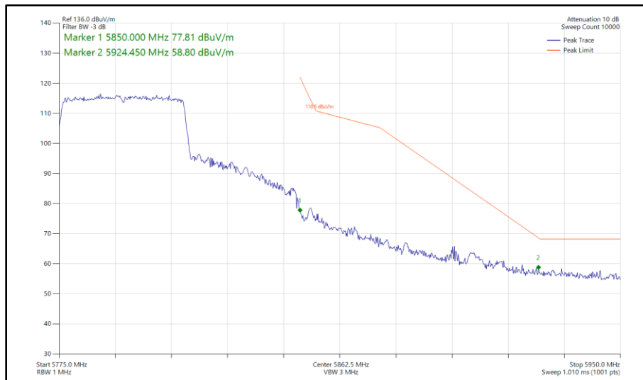
Figure 504 - 802.11ax HE40, SU, SISO, Core 1 - 5795 MHz Band Edge Frequency 5850 MHz
