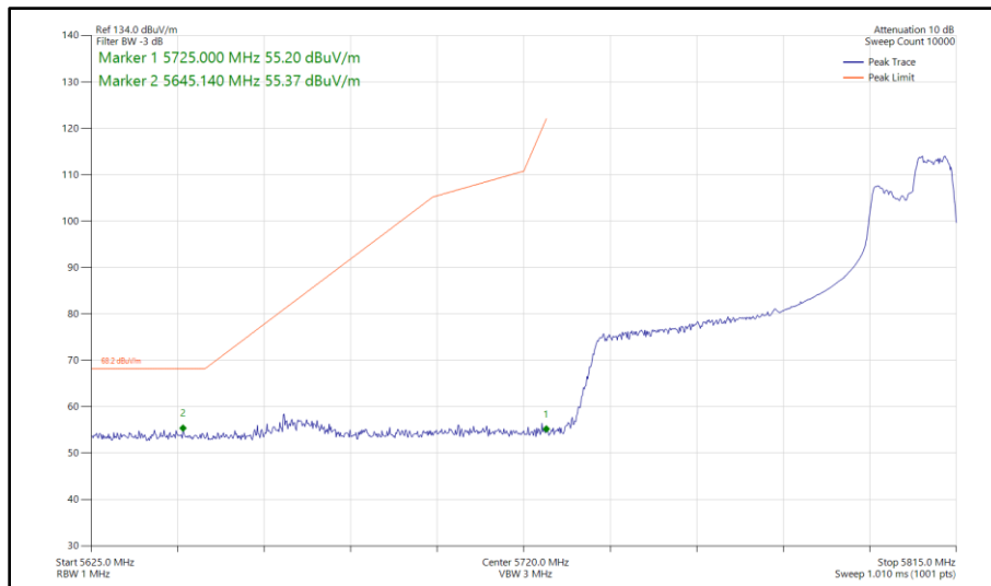
Figure 559 - 802.11ax HE80, RU 106-60, SISO, Core 0 - 5775 MHz Band Edge Frequency 5725 MHz
