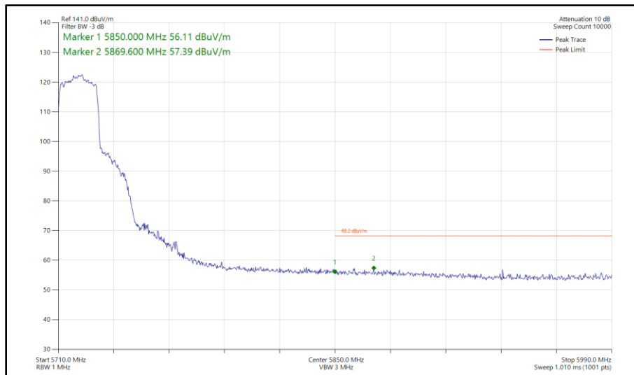
Figure 451 - 802.11ax HE20, SU, SDM, Core 0 - Core 1 - 5720 MHz Band Edge Frequency 5850 MHz
