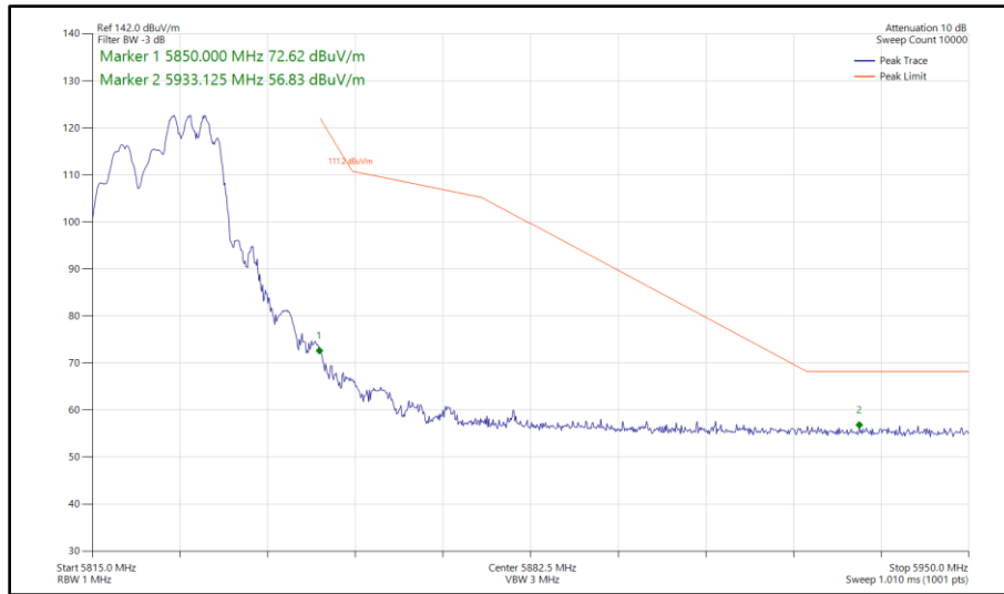
Figure 432 - 802.11ax HE20, RU 106-54, CDD, Core 0 - Core 1 - 5825 MHz Band Edge Frequency 5850 MHz
