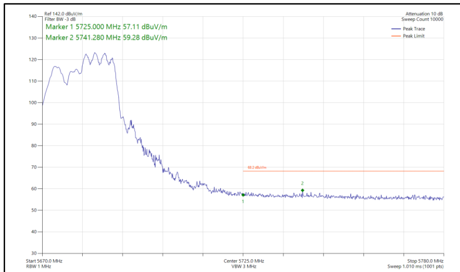
Figure 422 - 802.11ax HE20, RU 106-54, CDD, Core 0 - Core 1 - 5680 MHz Band Edge Frequency 5725 MHz
