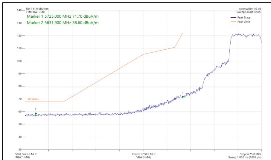
Figure 442 - 802.11ax HE20, SU, SDM, Core 0 - Core 1 - 5765 MHz Band Edge Frequency 5725 MHz
