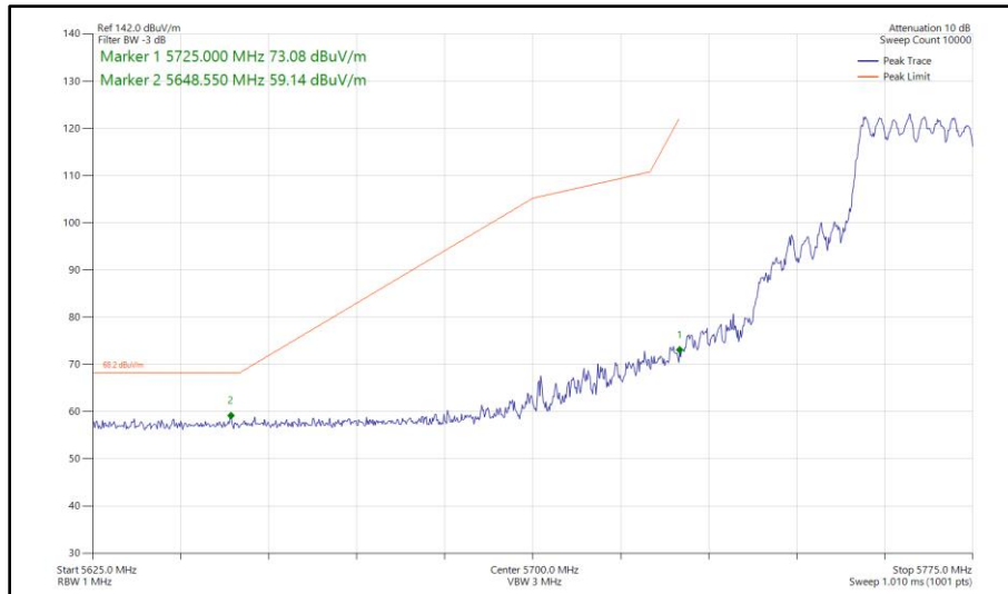
Figure 418 - 802.11ax HE20, SU, CDD, Core 0 - Core 1 - 5765 MHz Band Edge Frequency 5725 MHz
