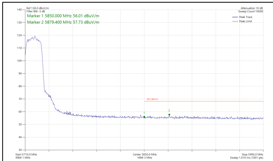
Figure 449 - 802.11n HT20, SDM, Core 0 - Core 1 - 5720 MHz Band Edge Frequency 5850 MHz
