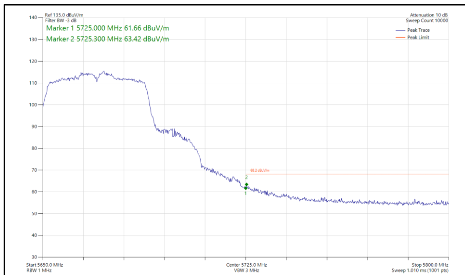
Figure 474 - 802.11n HT40, SISO, Core 0 - 5670 MHz Band Edge Frequency 5725 MHz
