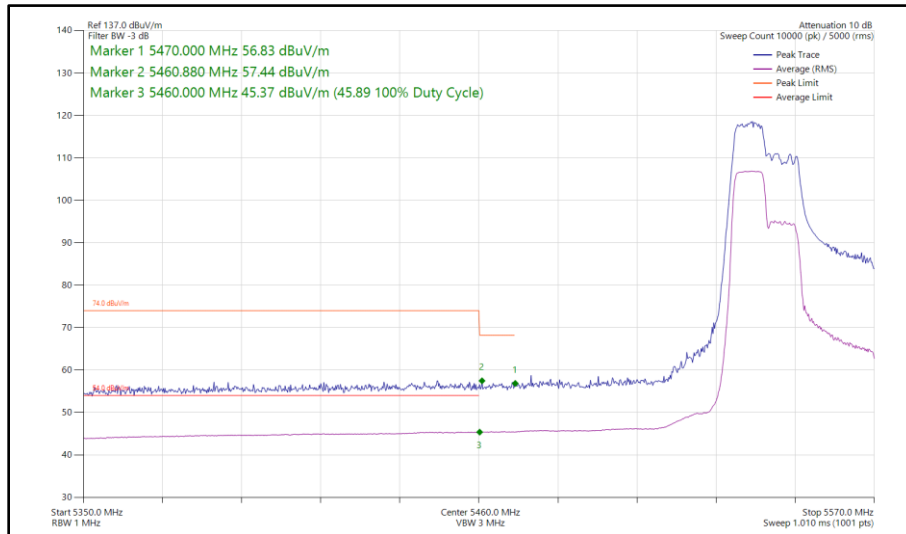
Figure 469 - 802.11ax HE40, RU 106-53, SISO, Core 0 - 5550 MHz Band Edge Frequency 5470 MHz
