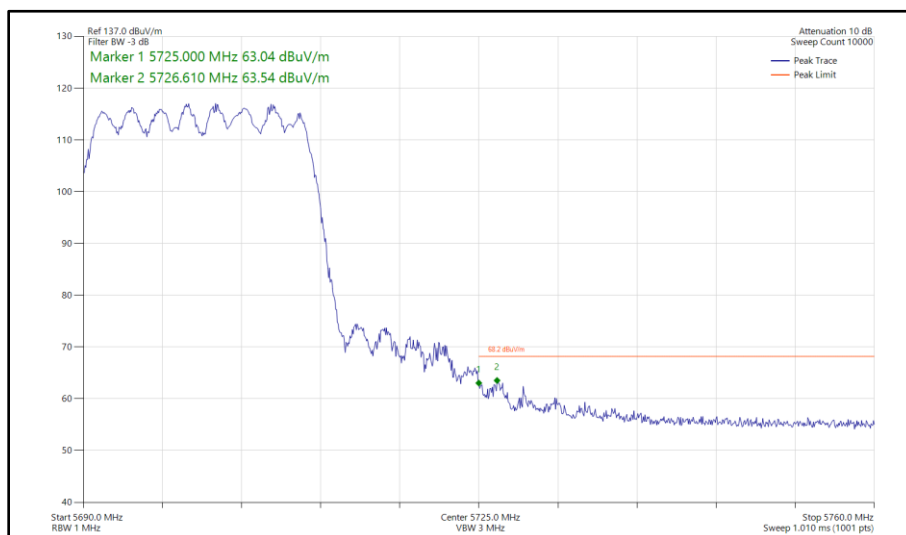
Figure 423 - 802.11ax HE20, SU, CDD, Core 0 - Core 1 - 5700 MHz Band Edge Frequency 5725 MHz
