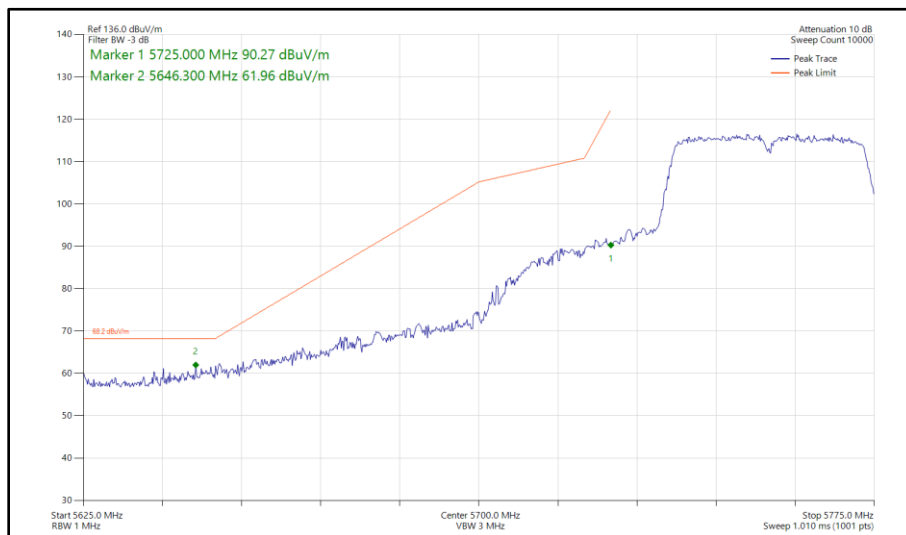
Figure 470 - 802.11n HT40, SISO, Core 0 - 5755 MHz Band Edge Frequency 5725 MHz
