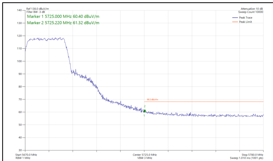
Figure 460 - 802.11ac VHT20, TxBF, Core 0 - Core 1 - 5680 MHz Band Edge Frequency 5725 MHz
