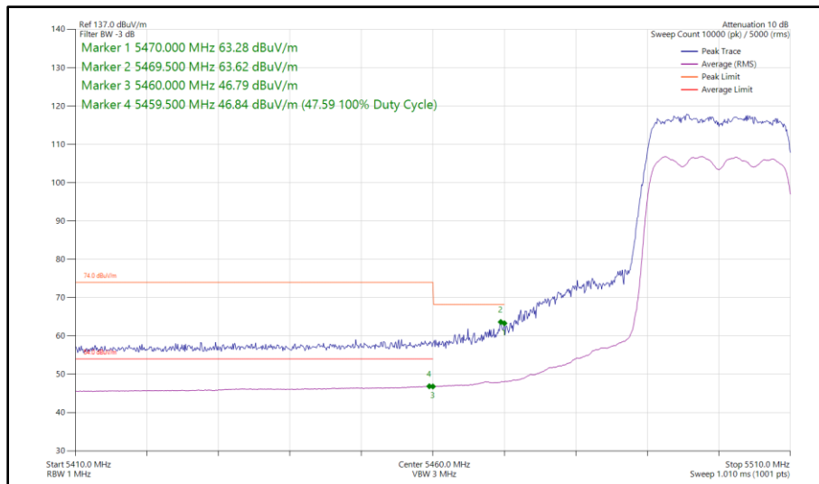
Figure 435 - 802.11ax HE20, SU, SDM, Core 0 - Core 1 - 5500 MHz Band Edge Frequency 5470 MHz
