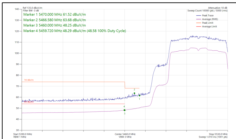
Figure 466 - 802.11ax HE40, SU, SISO, Core 0 - 5510 MHz Band Edge Frequency 5470 MHz
