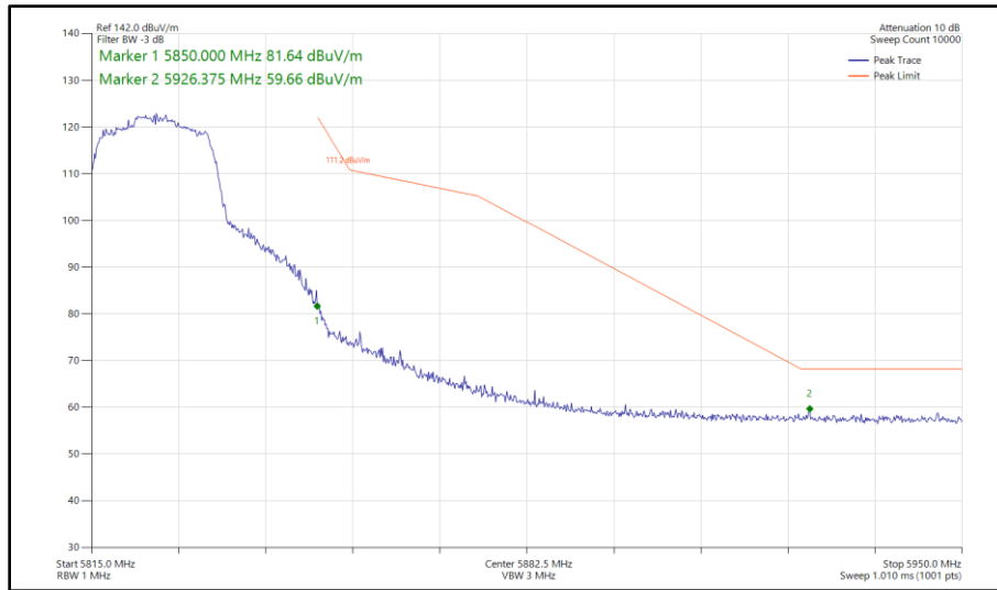
Figure 463 - 802.11ac VHT20, TxBF, Core 0 - Core 1 - 5825 MHz Band Edge Frequency 5850 MHz
