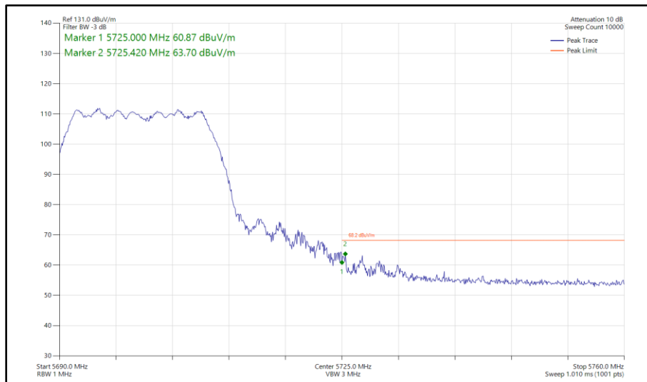
Figure 420 - 802.11n HT20, CDD, Core 0 - Core 1 - 5700 MHz Band Edge Frequency 5725 MHz
