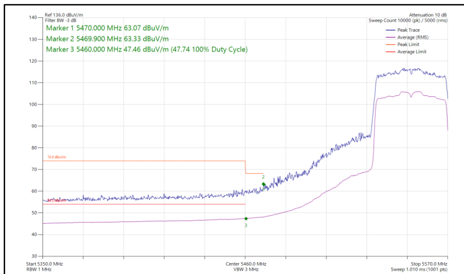
Figure 468 - 802.11ax HE40, SU, SISO, Core 0 - 5550 MHz Band Edge Frequency 5470 MHz
