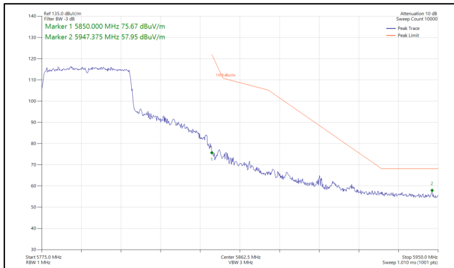
Figure 483 - 802.11ax HE40, SU, SISO, Core 0 - 5795 MHz Band Edge Frequency 5850 MHz
