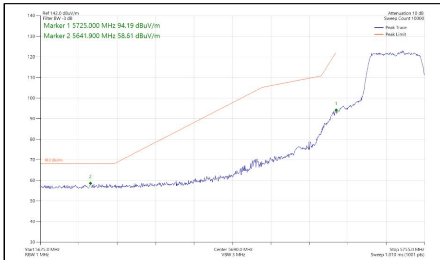
Figure 439 - 802.11n HT20, SDM, Core 0 - Core 1 - 5745 MHz Band Edge Frequency 5725 MHz
