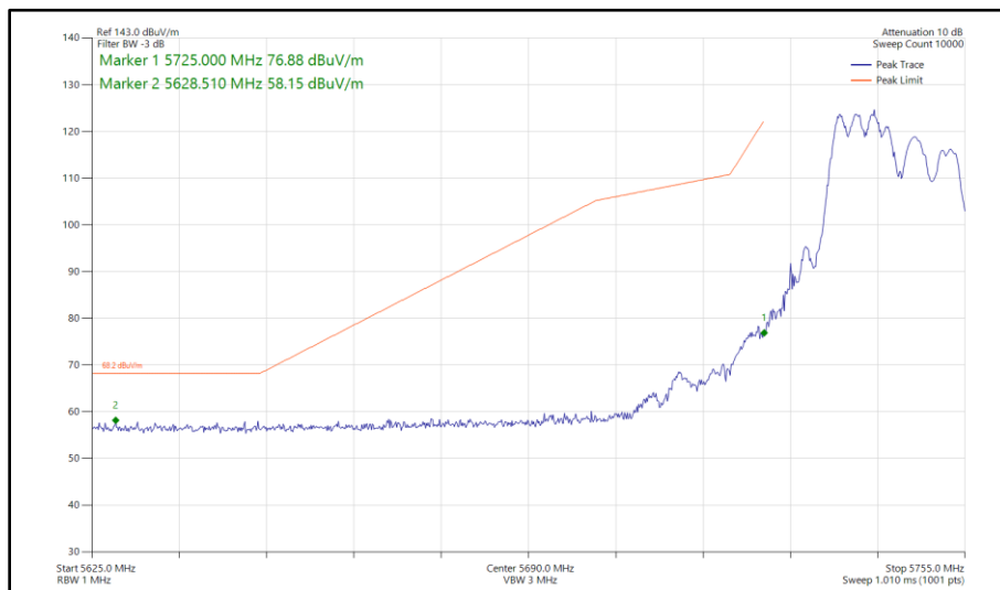
Figure 417 - 802.11ax HE20, RU 106-53, CDD, Core 0 - Core 1 - 5745 MHz Band Edge Frequency 5725 MHz
