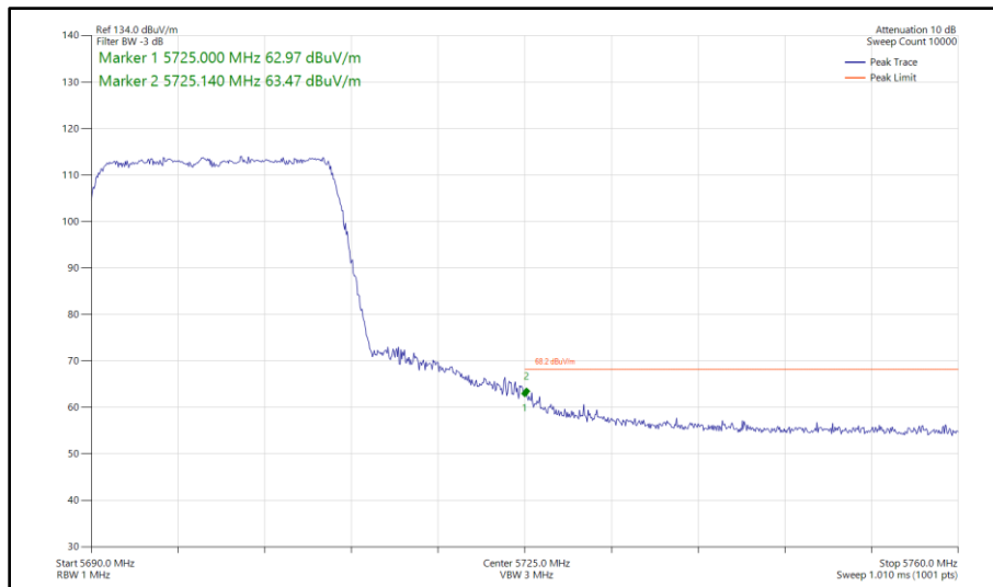
Figure 447 - 802.11ax HE20, SU, SDM, Core 0 - Core 1 - 5700 MHz Band Edge Frequency 5725 MHz
