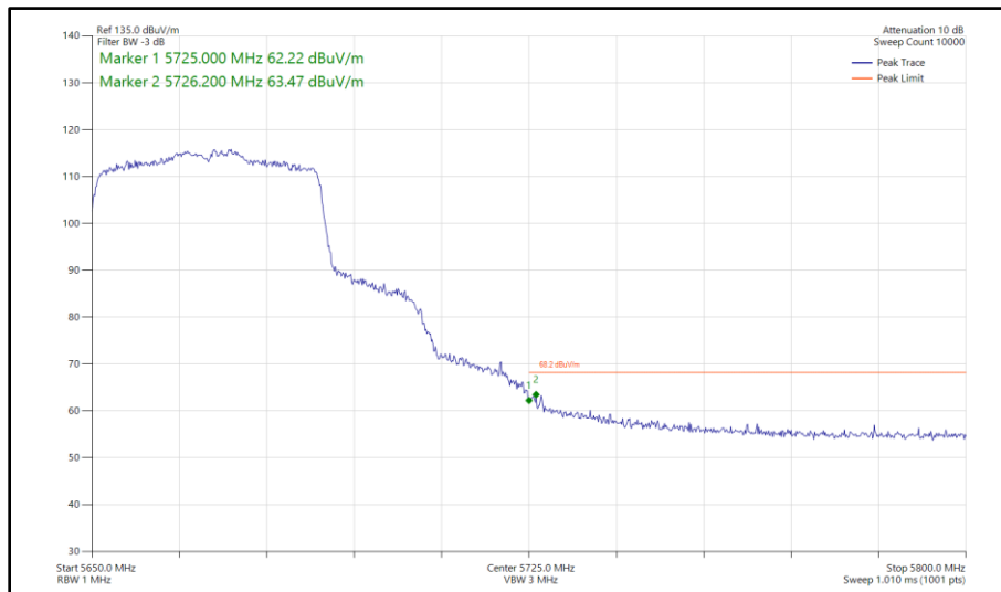
Figure 477 - 802.11ax HE40, SU, SISO, Core 0 - 5670 MHz Band Edge Frequency 5725 MHz
