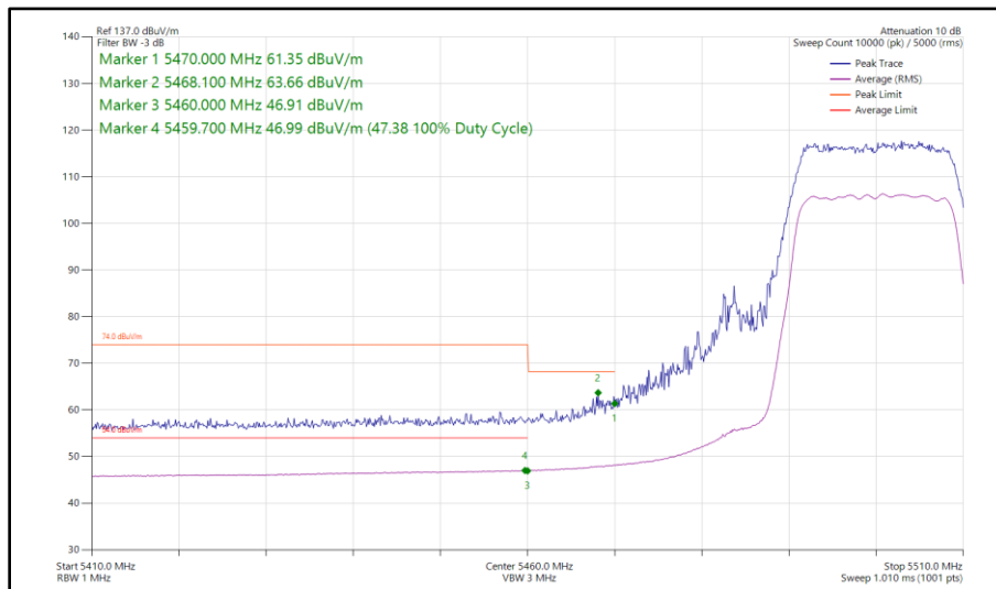
Figure 456 - 802.11ac VHT20, TxBF, Core 0 - Core 1 - 5500 MHz Band Edge Frequency 5470 MHz
