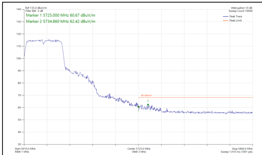
Figure 494 - 802.11n HT40, SISO, Core 1 - 5630 MHz Band Edge Frequency 5725 MHz
