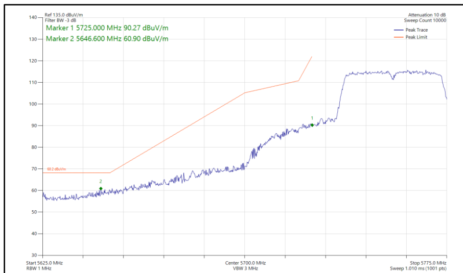
Figure 491 - 802.11n HT40, SISO, Core 1 - 5755 MHz Band Edge Frequency 5725 MHz
