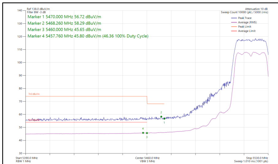
Figure 434 - 802.11n HT20, SDM, Core 0 - Core 1 - 5520 MHz Band Edge Frequency 5470 MHz
