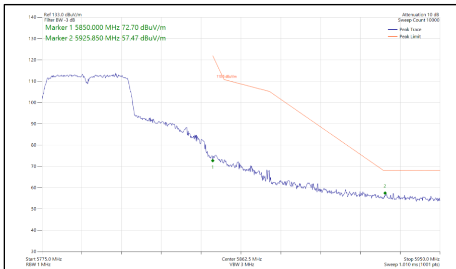
Figure 480 - 802.11n HT40, SISO, Core 0 - 5795 MHz Band Edge Frequency 5850 MHz
