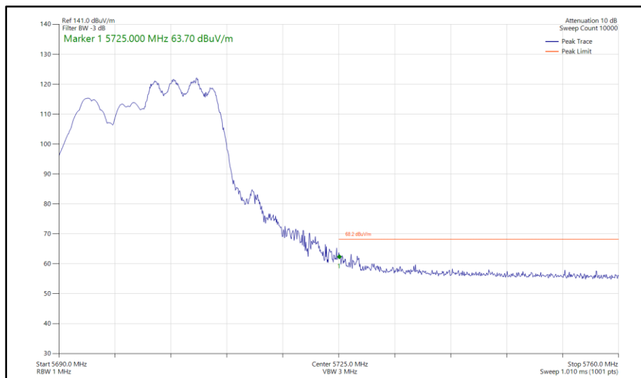
Figure 448 - 802.11ax HE20, RU 106-54, SDM, Core 0 - Core 1 - 5700 MHz Band Edge Frequency 5725 MHz
