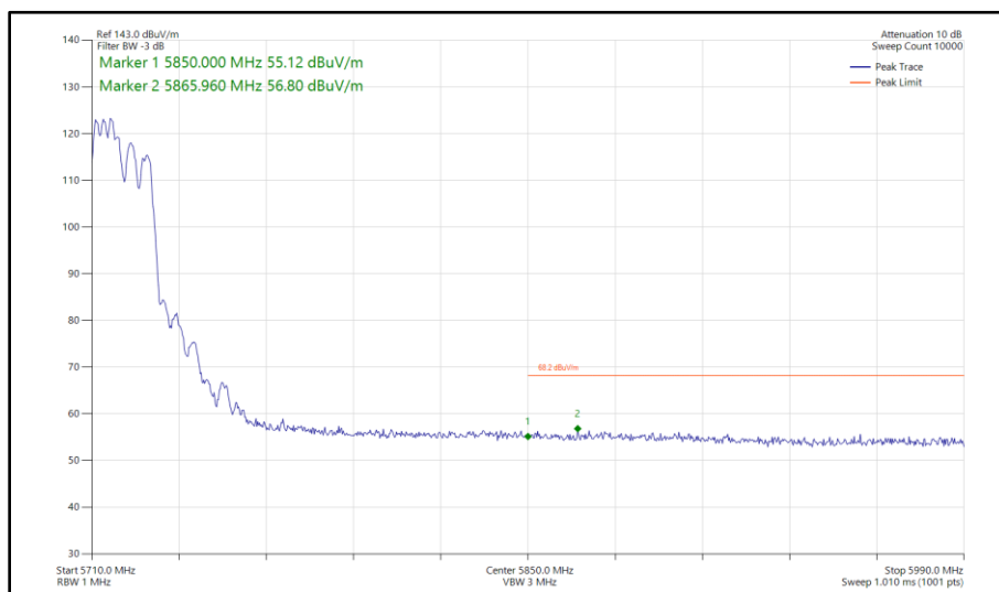
Figure 452 - 802.11ax HE20, RU 106-53, SDM, Core 0 - Core 1 - 5720 MHz Band Edge Frequency 5850 MHz
