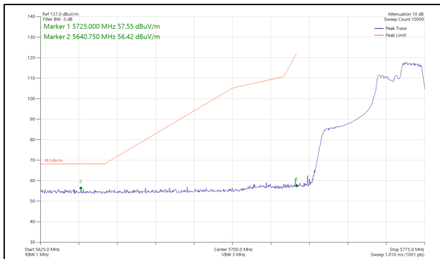
Figure 472 - 802.11ax HE40, RU 106-56, SISO, Core 0 - 5755 MHz Band Edge Frequency 5725 MHz
