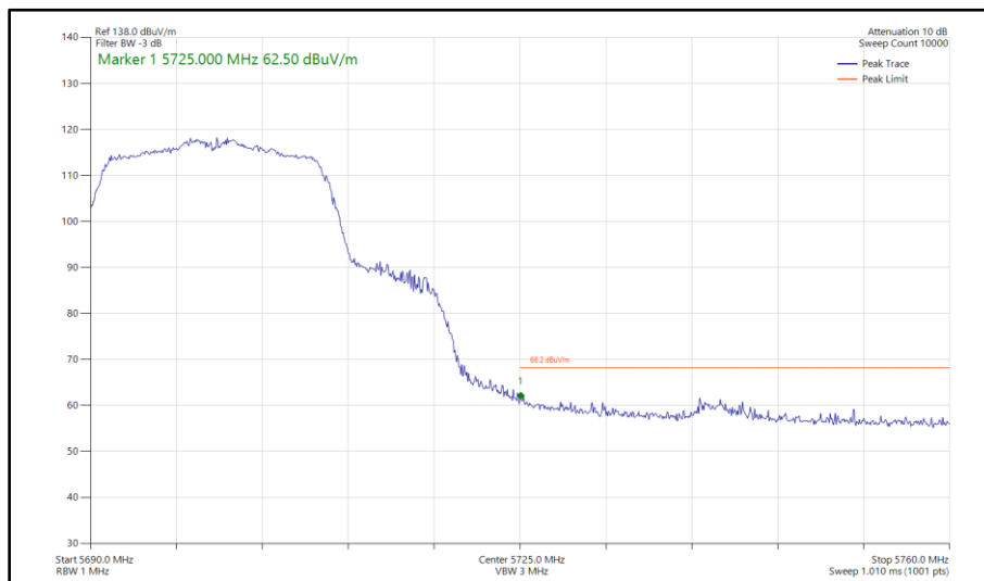
Figure 444 - 802.11n HT20, SDM, Core 0 - Core 1 - 5700 MHz Band Edge Frequency 5725 MHz
