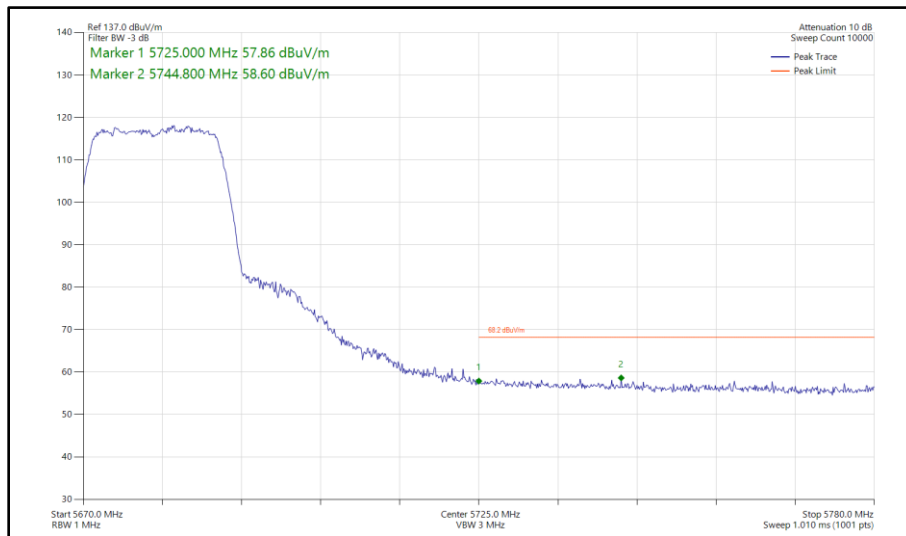
Figure 443 - 802.11n HT20, SDM, Core 0 - Core 1 - 5680 MHz Band Edge Frequency 5725 MHz
