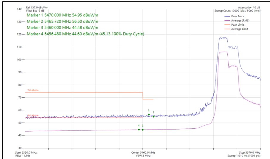
Figure 490 - 802.11ax HE40, RU 106-53, SISO, Core 1 - 5550 MHz Band Edge Frequency 5470 MHz
