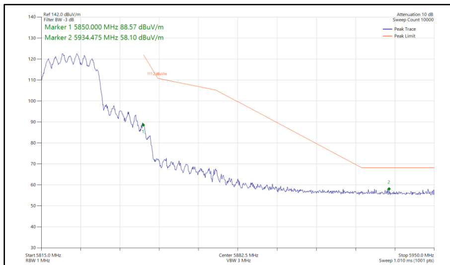
Figure 431 - 802.11ax HE20, SU, CDD, Core 0 - Core 1 - 5825 MHz Band Edge Frequency 5850 MHz
