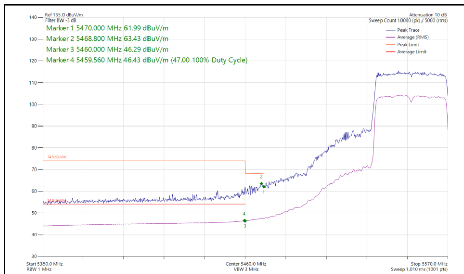
Figure 489 - 802.11ax HE40, SU, SISO, Core 1 - 5550 MHz Band Edge Frequency 5470 MHz
