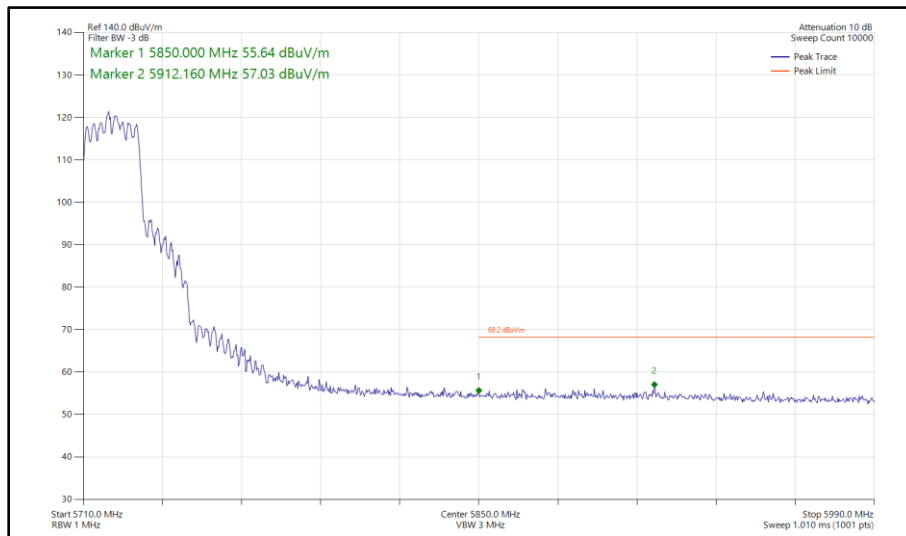
Figure 428 - 802.11ax HE20, SU, CDD, Core 0 - Core 1 - 5720 MHz Band Edge Frequency 5850 MHz
