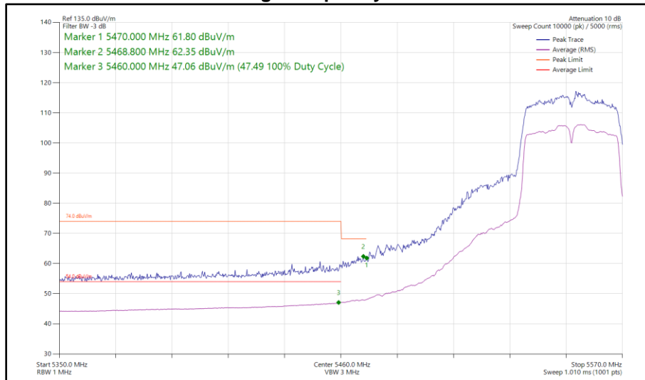
Figure 486 - 802.11n HT40, SISO, Core 1 - 5550 MHz Band Edge Frequency 5470 MHz
