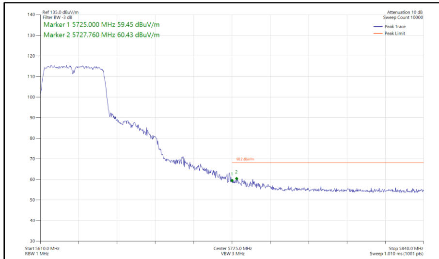
Figure 473 - 802.11n HT40, SISO, Core 0 - 5630 MHz Band Edge Frequency 5725 MHz
