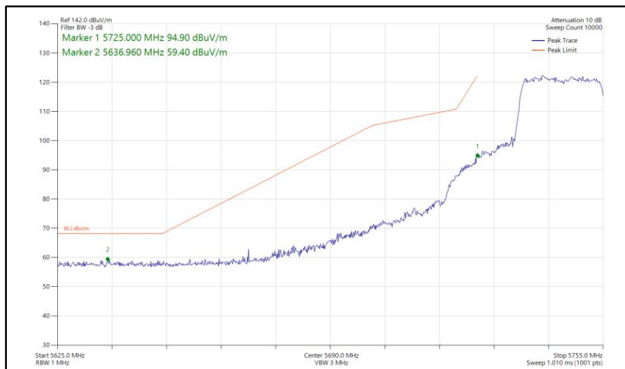
Figure 440 - 802.11ax HE20, SU, SDM, Core 0 - Core 1 - 5745 MHz Band Edge Frequency 5725 MHz
