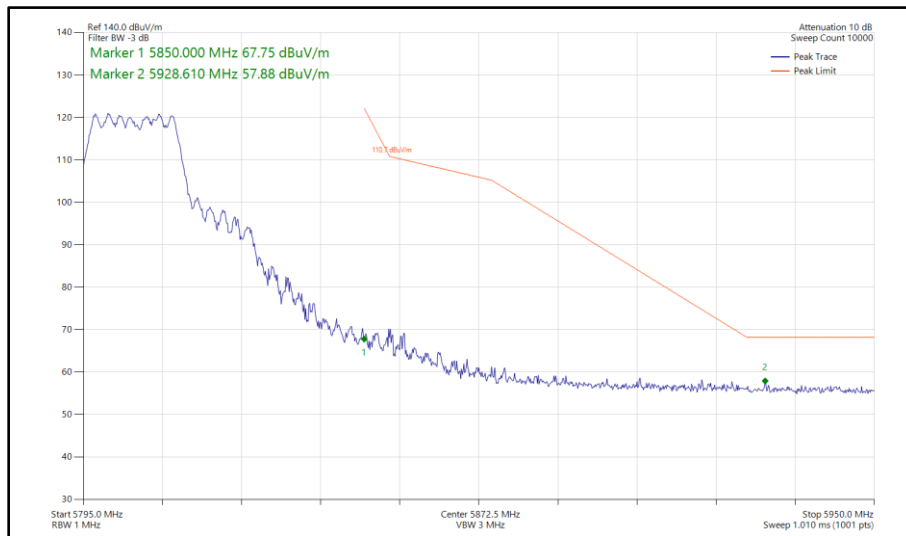
Figure 426 - 802.11n HT20, CDD, Core 0 - Core 1 - 5805 MHz Band Edge Frequency 5850 MHz
