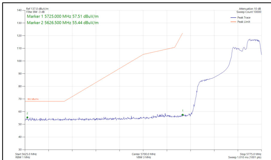
Figure 493 - 802.11ax HE40, RU 106-56, SISO, Core 1 - 5755 MHz Band Edge Frequency 5725 MHz
