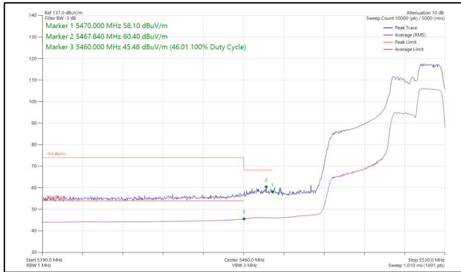
Figure 488 - 802.11ax HE40, RU 106-56, SISO, Core 1 - 5510 MHz Band Edge Frequency 5470 MHz
