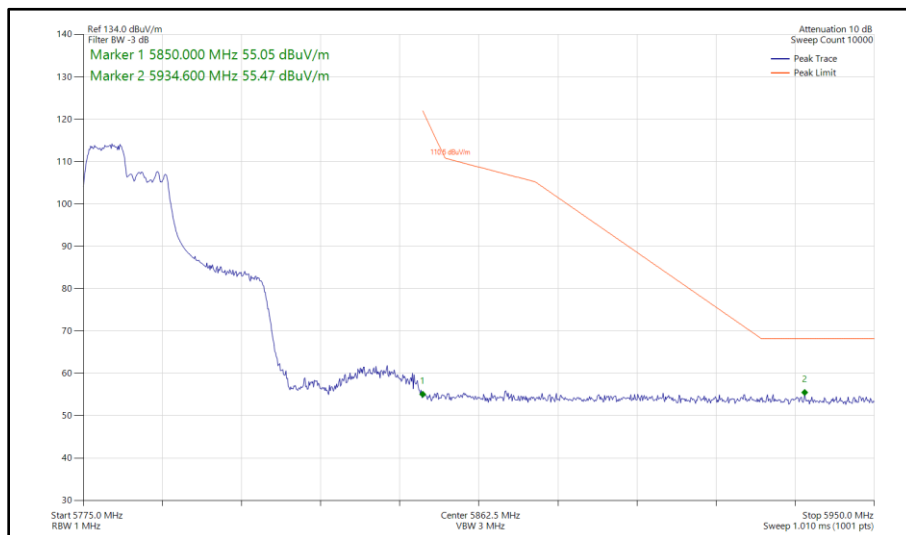
Figure 484 - 802.11ax HE40, RU 106-53, SISO, Core 0 - 5795 MHz Band Edge Frequency 5850 MHz
