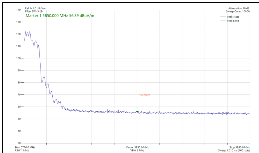
Figure 429 - 802.11ax HE20, RU 106-53, CDD, Core 0 - Core 1 - 5720 MHz Band Edge Frequency 5850 MHz
