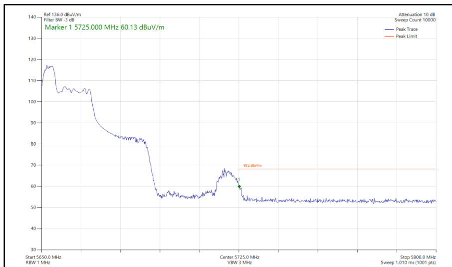
Figure 478 - 802.11ax HE40, RU 52-37, SISO, Core 0 - 5670 MHz Band Edge Frequency 5725 MHz
