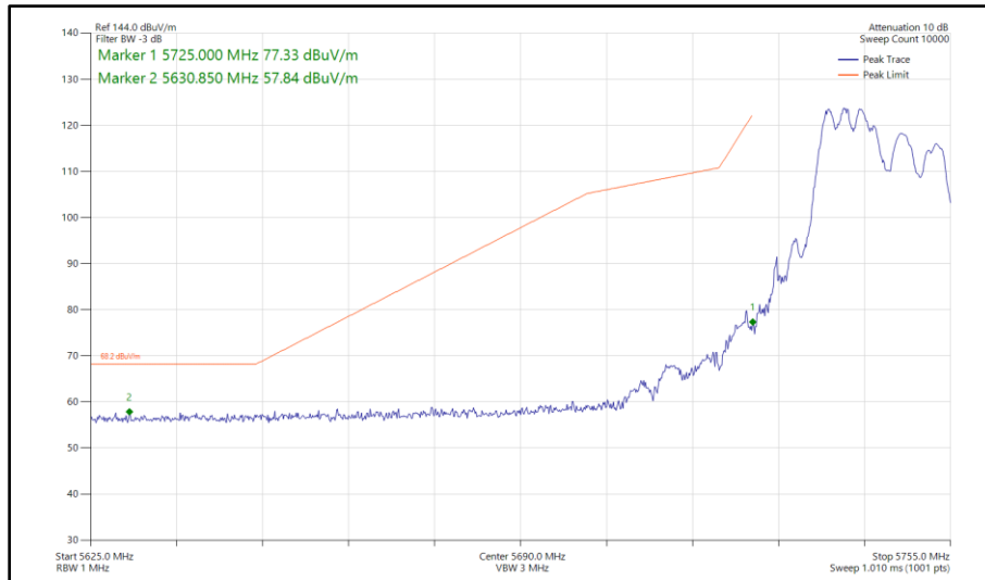
Figure 441 - 802.11ax HE20, RU 106-53, SDM, Core 0 - Core 1 - 5745 MHz Band Edge Frequency 5725 MHz
