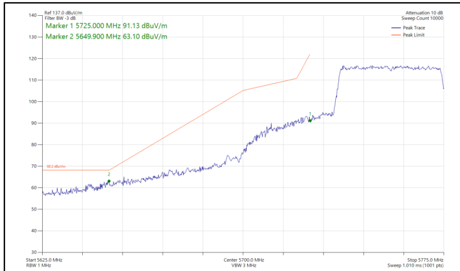
Figure 471 - 802.11ax HE40, SU, SISO, Core 0 - 5755 MHz Band Edge Frequency 5725 MHz
