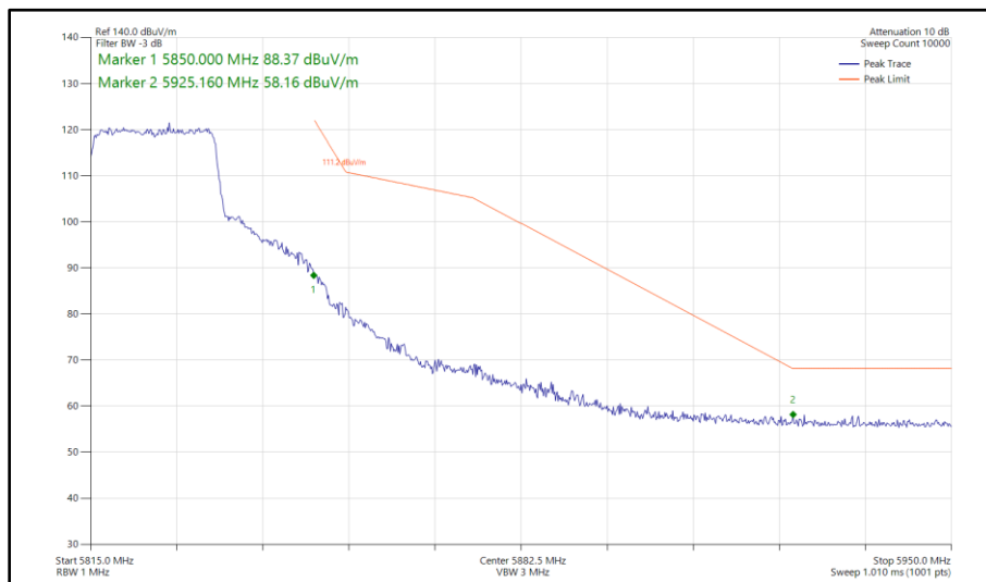
Figure 454 - 802.11ax HE20, SU, SDM, Core 0 - Core 1 - 5825 MHz Band Edge Frequency 5850 MHz
