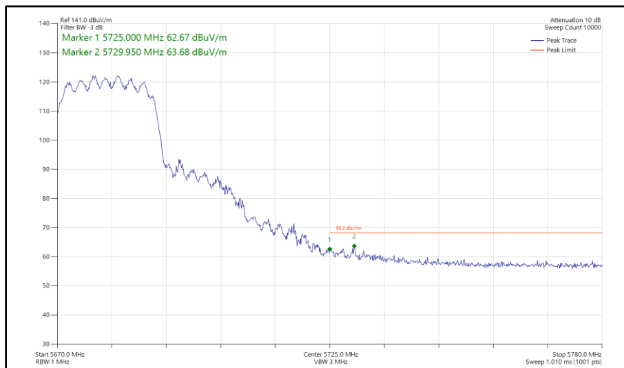
Figure 421 - 802.11ax HE20, SU, CDD, Core 0 - Core 1 - 5680 MHz Band Edge Frequency 5725 MHz
