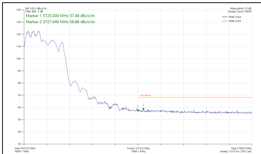
Figure 446 - 802.11ax HE20, RU 106-53, SDM, Core 0 - Core 1 - 5680 MHz Band Edge Frequency 5725 MHz
