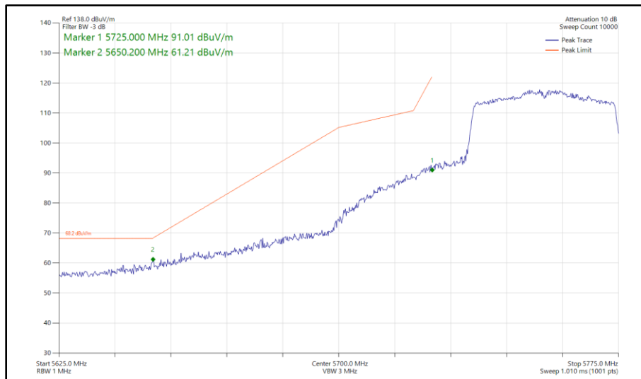
Figure 492 - 802.11ax HE40, SU, SISO, Core 1 - 5755 MHz Band Edge Frequency 5725 MHz
