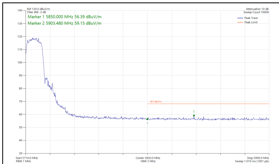
Figure 462 - 802.11ac VHT20, TxBF, Core 0 - Core 1 - 5720 MHz Band Edge Frequency 5850 MHz
