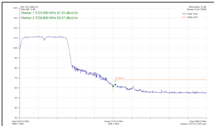
Figure 495 - 802.11n HT40, SISO, Core 1 - 5670 MHz Band Edge Frequency 5725 MHz
