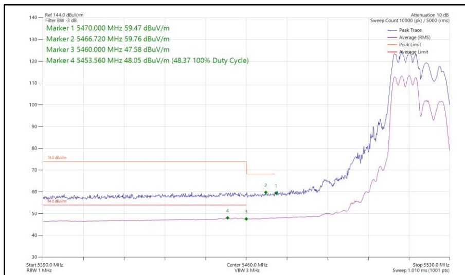
Figure 438 - 802.11ax HE20, RU 106-53, SDM, Core 0 - Core 1 - 5520 MHz Band Edge Frequency 5470 MHz
