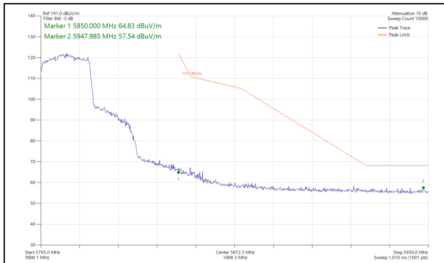
Figure 453 - 802.11ax HE20, SU, SDM, Core 0 - Core 1 - 5805 MHz Band Edge Frequency 5850 MHz
