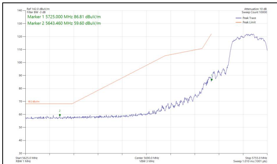
Figure 458 - 802.11ac VHT20, TxBF, Core 0 - Core 1 - 5745 MHz Band Edge Frequency 5725 MHz
