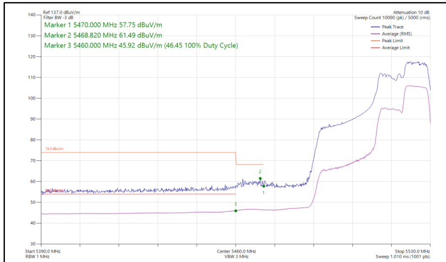
Figure 467 - 802.11ax HE40, RU 106-56, SISO, Core 0 - 5510 MHz Band Edge Frequency 5470 MHz
