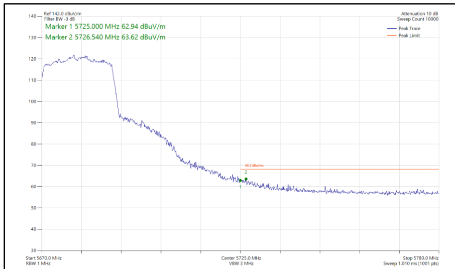
Figure 445 - 802.11ax HE20, SU, SDM, Core 0 - Core 1 - 5680 MHz Band Edge Frequency 5725 MHz
