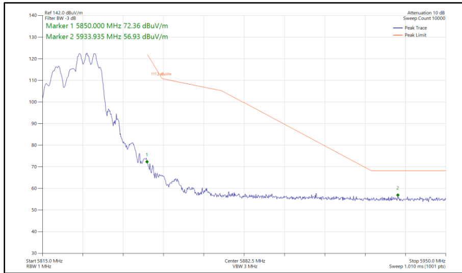
Figure 455 - 802.11ax HE20, RU 106-54, SDM, Core 0 - Core 1 - 5825 MHz Band Edge Frequency 5850 MHz
