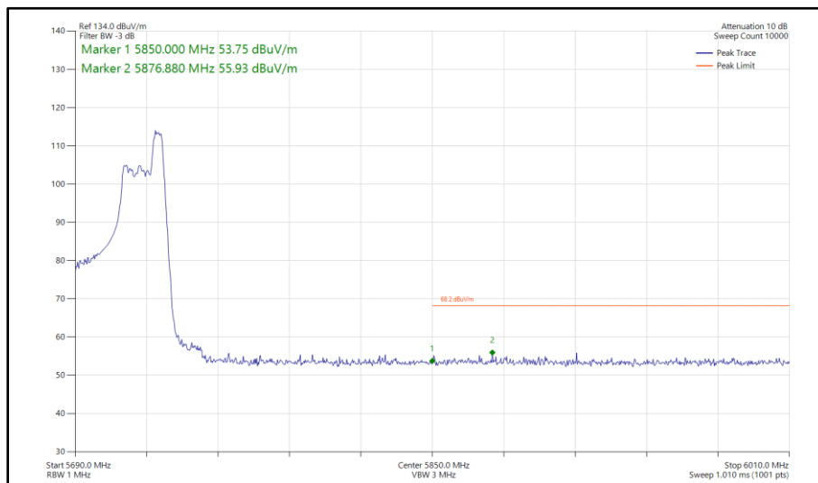
Figure 482 - 802.11ax HE40, RU 52-44, SISO, Core 0 - 5710 MHz Band Edge Frequency 5850 MHz
