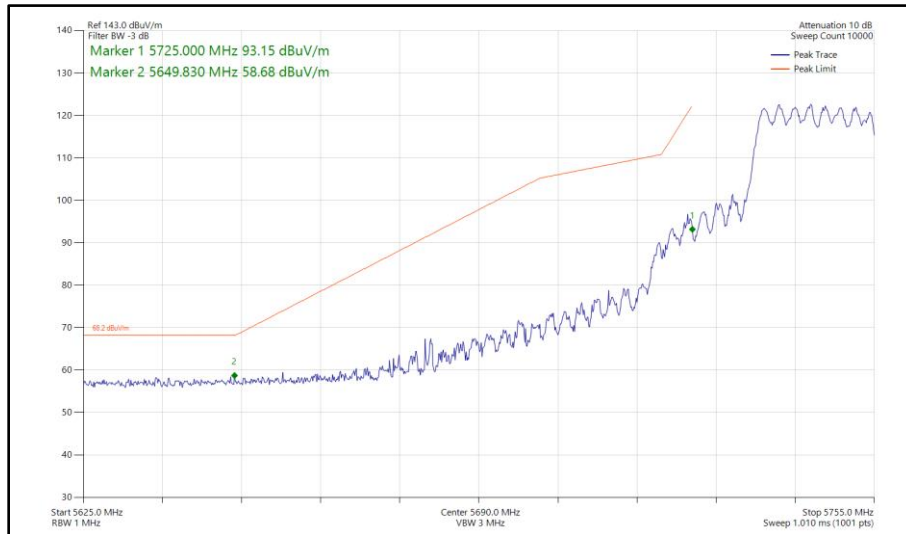
Figure 416 - 802.11ax HE20, SU, CDD, Core 0 - Core 1 - 5745 MHz Band Edge Frequency 5725 MHz
