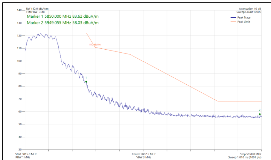
Figure 427 - 802.11n HT20, CDD, Core 0 - Core 1 - 5825 MHz Band Edge Frequency 5850 MHz
