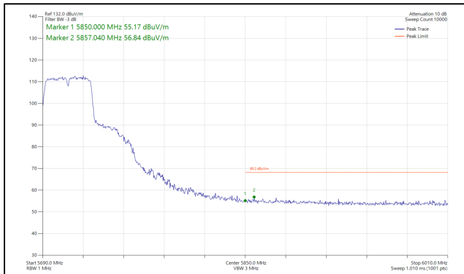
Figure 479 - 802.11n HT40, SISO, Core 0 - 5710 MHz Band Edge Frequency 5850 MHz
