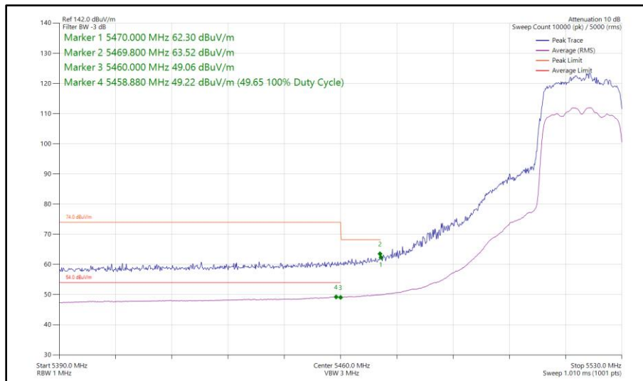
Figure 437 - 802.11ax HE20, SU, SDM, Core 0 - Core 1 - 5520 MHz Band Edge Frequency 5470 MHz
