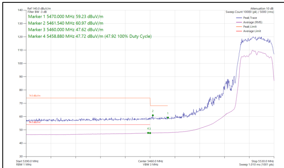
Figure 457 - 802.11ac VHT20, TxBF, Core 0 - Core 1 - 5520 MHz Band Edge Frequency 5470 MHz
