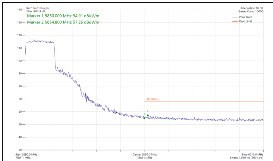
Figure 481 - 802.11ax HE40, SU, SISO, Core 0 - 5710 MHz Band Edge Frequency 5850 MHz
