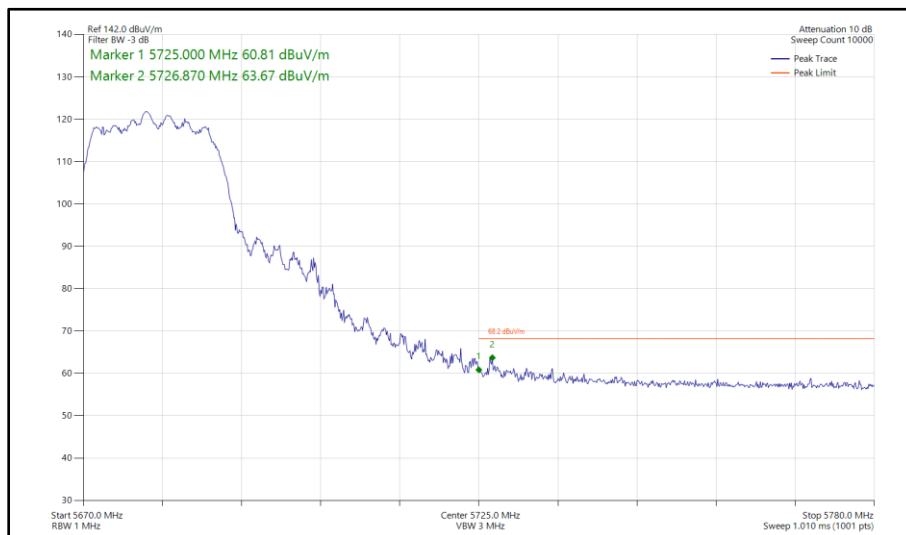
Figure 419 - 802.11n HT20, CDD, Core 0 - Core 1 - 5680 MHz Band Edge Frequency 5725 MHz
