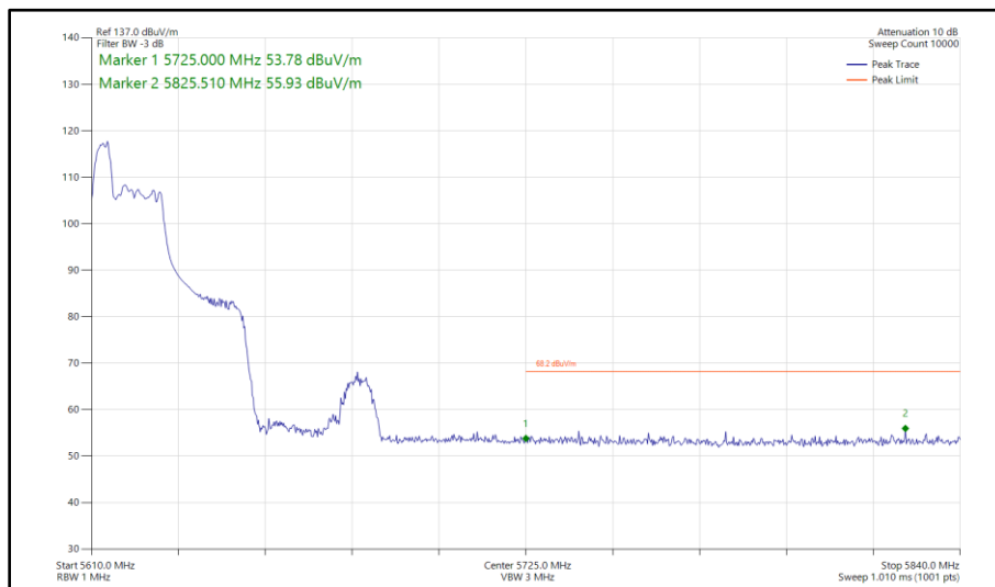
Figure 476 - 802.11ax HE40, RU 52-37, SISO, Core 0 - 5630 MHz Band Edge Frequency 5725 MHz
