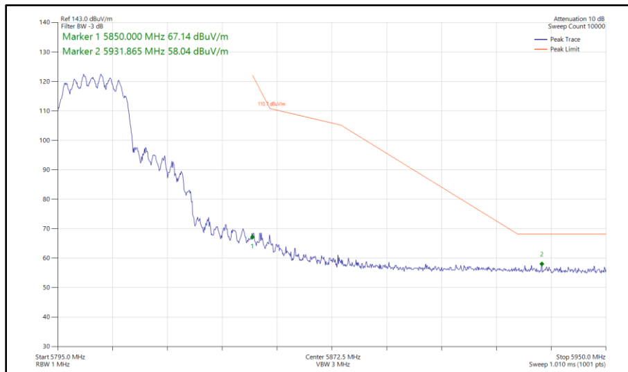
Figure 430 - 802.11ax HE20, SU, CDD, Core 0 - Core 1 - 5805 MHz Band Edge Frequency 5850 MHz
