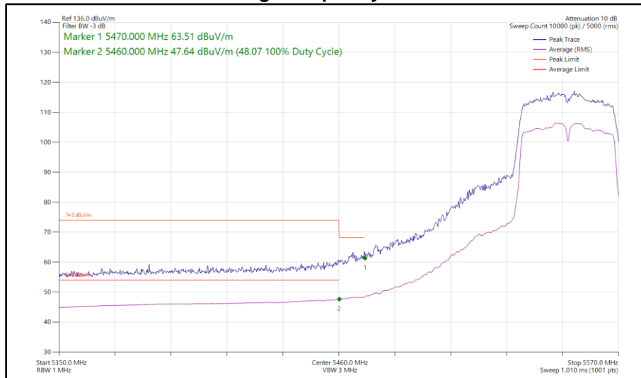
Figure 465 - 802.11n HT40, SISO, Core 0 - 5550 MHz Band Edge Frequency 5470 MHz
