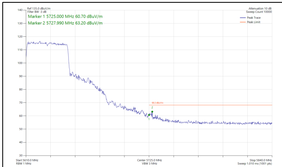
Figure 475 - 802.11ax HE40, SU, SISO, Core 0 - 5630 MHz Band Edge Frequency 5725 MHz
