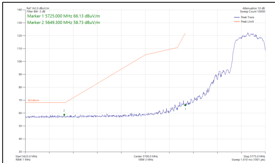
Figure 459 - 802.11ac VHT20, TxBF, Core 0 - Core 1 - 5765 MHz Band Edge Frequency 5725 MHz
