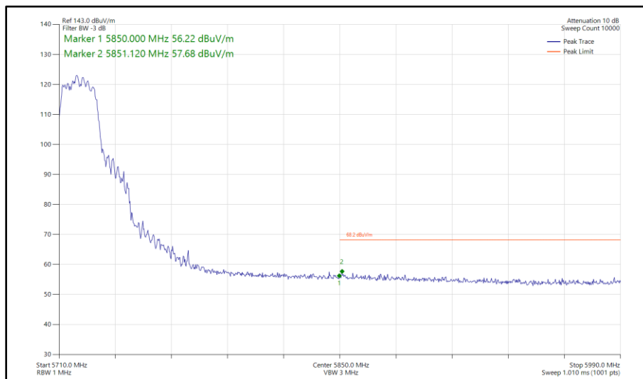
Figure 425 - 802.11n HT20, CDD, Core 0 - Core 1 - 5720 MHz Band Edge Frequency 5850 MHz
