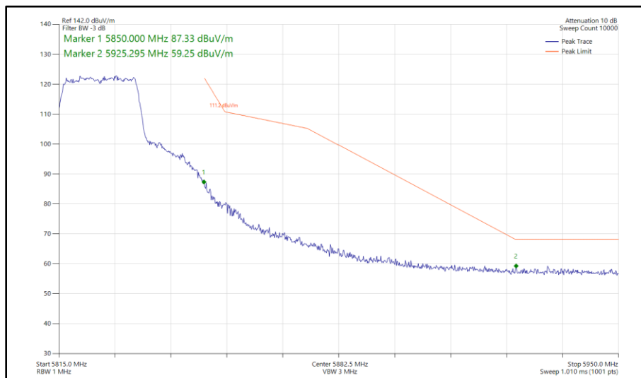
Figure 450 - 802.11n HT20, SDM, Core 0 - Core 1 - 5825 MHz Band Edge Frequency 5850 MHz
