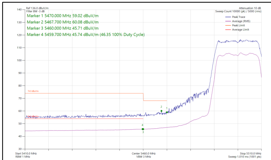
Figure 433 - 802.11n HT20, SDM, Core 0 - Core 1 - 5500 MHz Band Edge Frequency 5470 MHz
