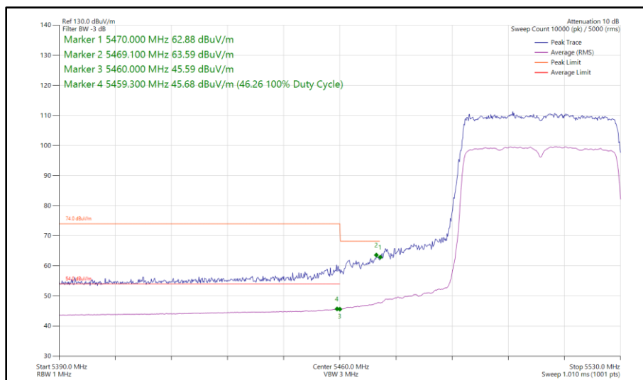
Figure 487 - 802.11ax HE40, SU, SISO, Core 1 - 5510 MHz Band Edge Frequency 5470 MHz
