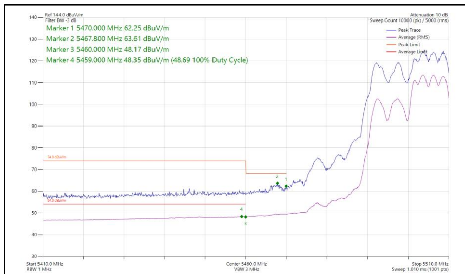
Figure 436 - 802.11ax HE20, RU 106-54, SDM, Core 0 - Core 1 - 5500 MHz Band Edge Frequency 5470 MHz
