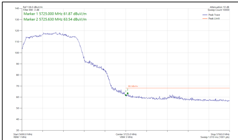
Figure 461 - 802.11ac VHT20, TxBF, Core 0 - Core 1 - 5700 MHz Band Edge Frequency 5725 MHz
