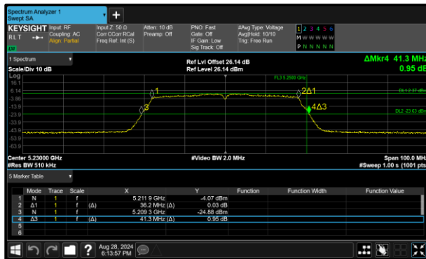
Figure 276 - 802.11n HT40 Minimum 99% OBW
