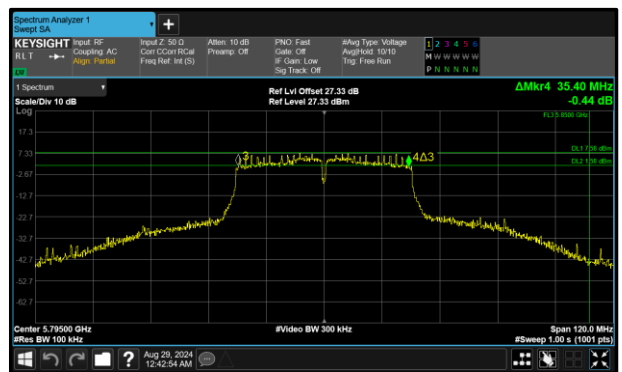
Figure 321 - 802.11n HT40 Maximum 6 dB EBW
