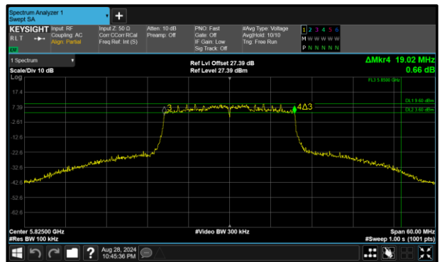
Figure 297 - 802.11ax HE20 SU Maximum 6 dB EBW
