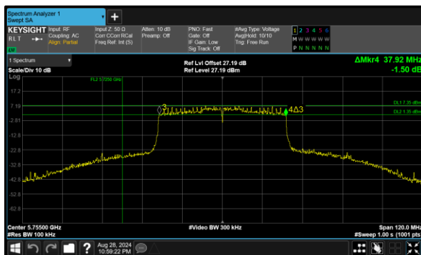
Figure 298 - 802.11ax HE40 SU Minimum 6 dB EBW
