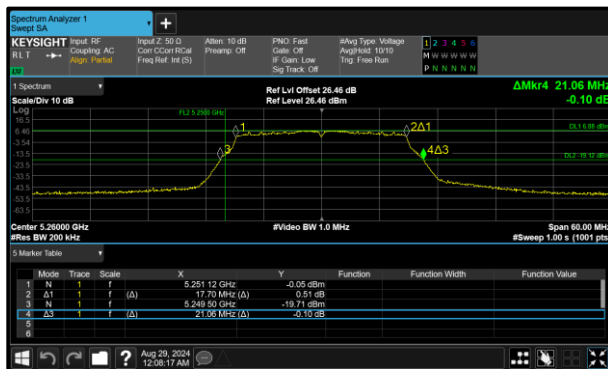
Figure 302 - 802.11n HT20 Minimum 99% OBW
