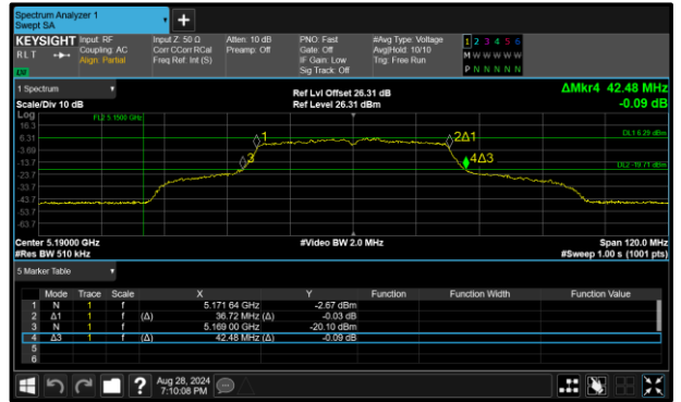
Figure 305 - 802.11n HT40 Maximum 99% OBW
