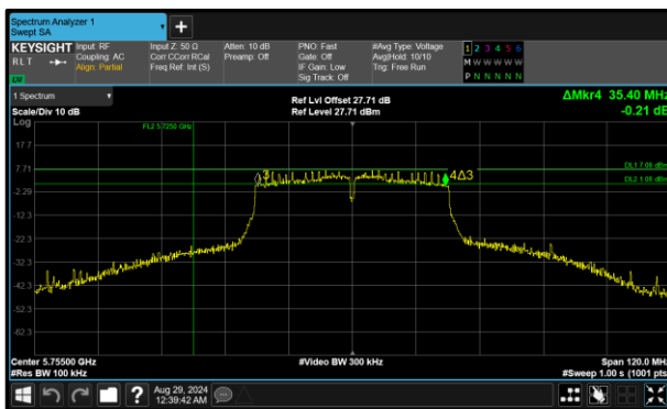
Figure 320 - 802.11n HT40 Minimum 6 dB EBW
