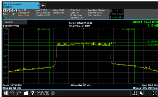
Figure 300 - 802.11ax HE80 SU Minimum 6 dB EBW
