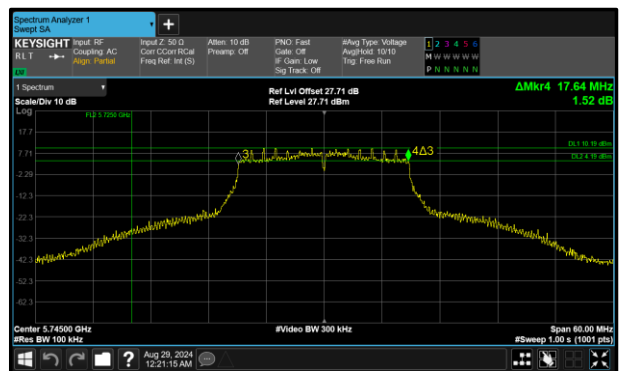
Figure 319 - 802.11n HT20 Maximum 6 dB EBW
