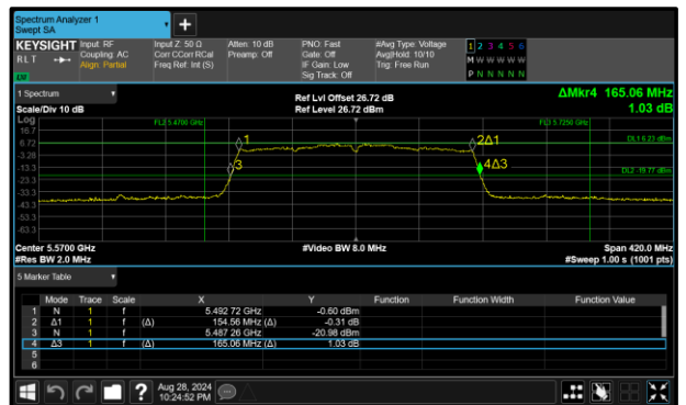
Figure 281 - 802.11ac VHT160 Maximum 99% OBW
