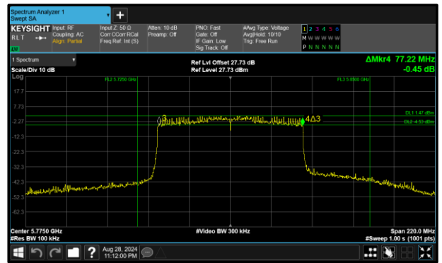
Figure 301 - 802.11ax HE80 SU Maximum 6 dB EBW
