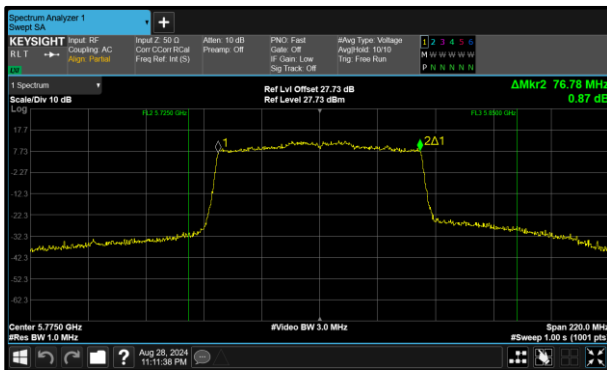
Figure 286 - 802.11ax HE80 SU Minimum 99% OBW
