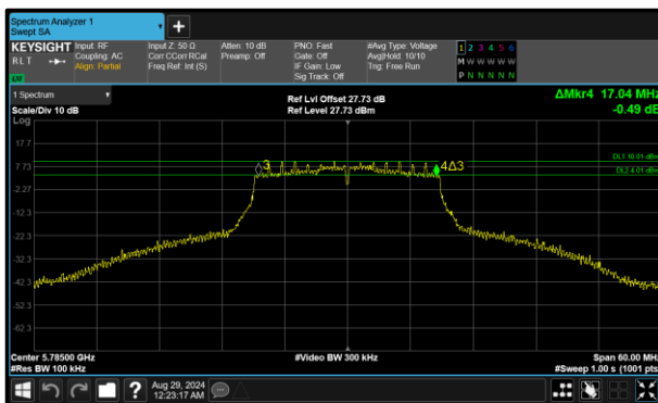
Figure 318 - 802.11n HT20 Minimum 6 dB EBW
