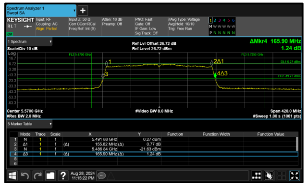
Figure 289 - 802.11ax HE160 SU Maximum 99% OBW
