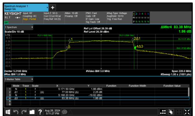
Figure 315 - 802.11ax HE80 SU Maximum 99% OBW
