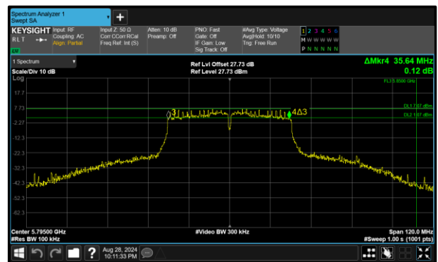
Figure 293 - 802.11n HT40 Maximum 6 dB EBW
