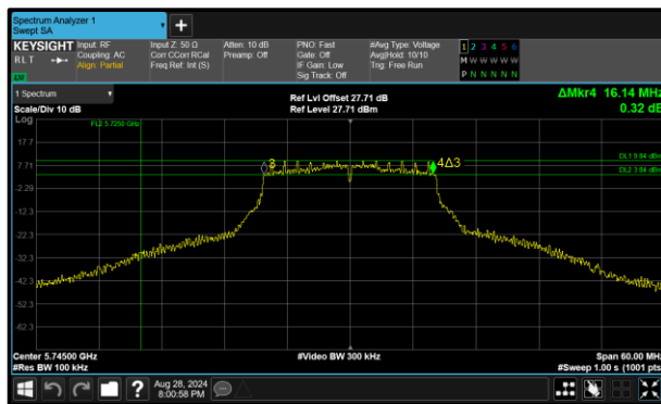
Figure 260 - 802.11a Minimum 6 dB EBW
