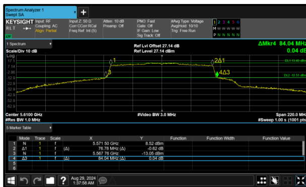
Figure 314 - 802.11ax HE80 SU Minimum 99% OBW
