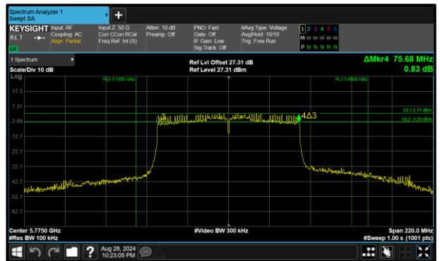
Figure 295 - 802.11ac VHT80 Maximum 6 dB EBW
