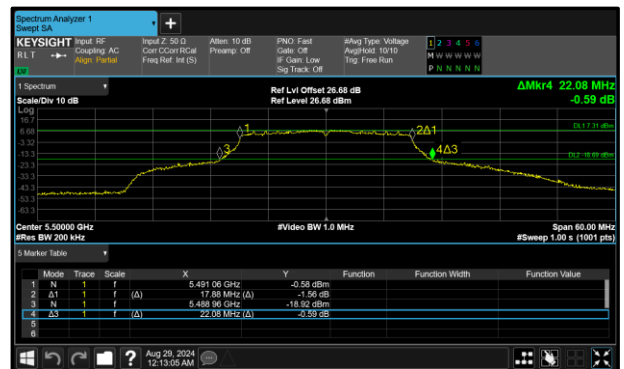
Figure 303 - 802.11n HT20 Maximum 99% OBW
