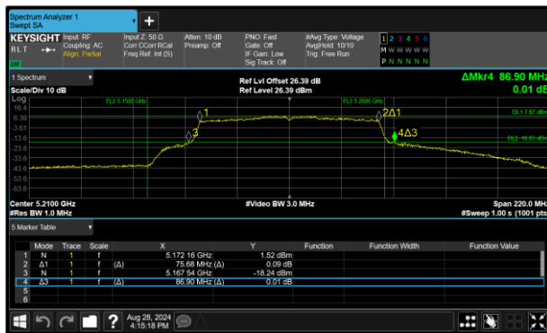
Figure 278 - 802.11ac VHT80 Minimum 99% OBW
