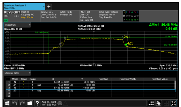
Figure 279 - 802.11ac VHT80 Maximum 99% OBW
