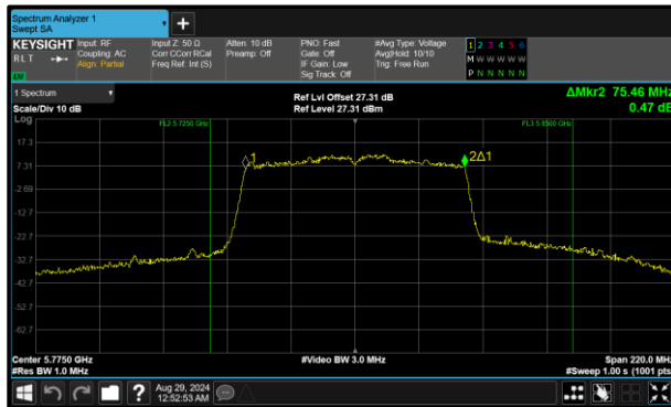
Figure 306 - 802.11ac VHT80 Minimum 99% OBW
