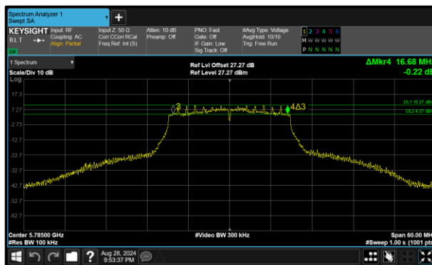
Figure 290 - 802.11n HT20 Minimum 6 dB EBW
