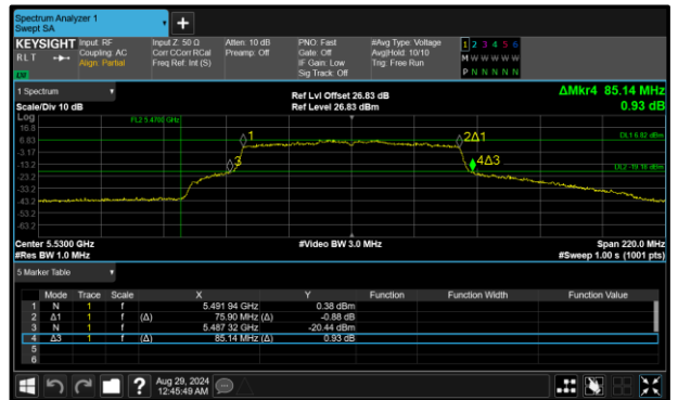
Figure 307 - 802.11ac VHT80 Maximum 99% OBW
