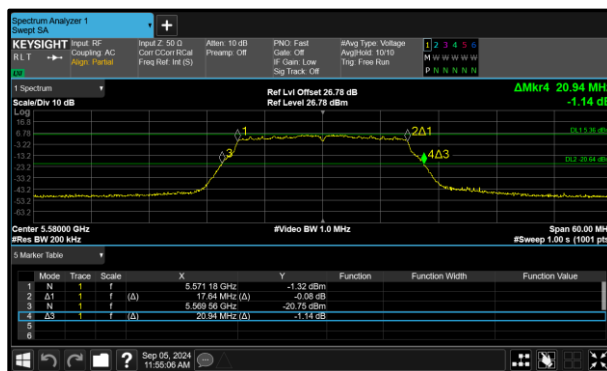
Figure 274 - 802.11n HT20 Minimum 99% OBW
