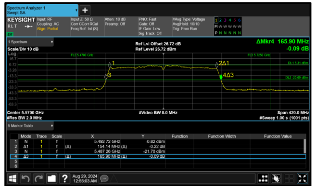
Figure 309 - 802.11ac VHT160 Maximum 99% OBW
