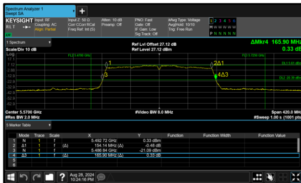
Figure 280 - 802.11ac VHT160 Minimum 99% OBW
