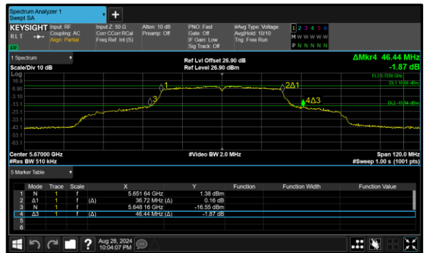
Figure 277 - 802.11n HT40 Maximum 99% OBW
