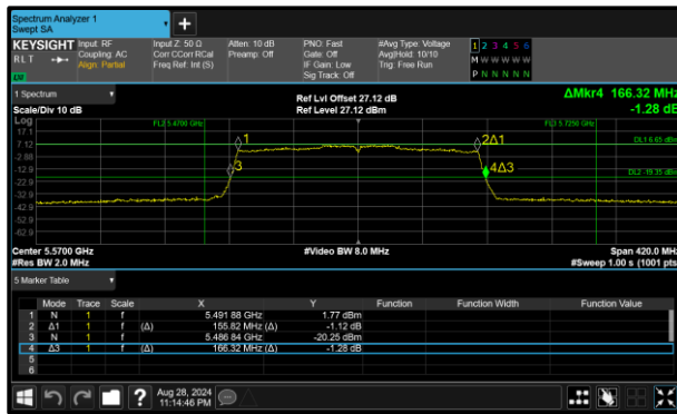
Figure 288 - 802.11ax HE160 SU Minimum 99% OBW
