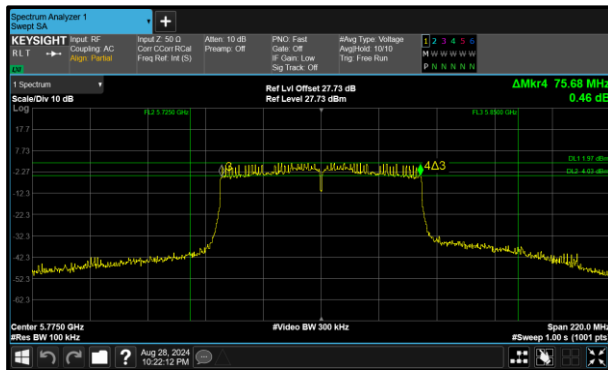
Figure 294 - 802.11ac VHT80 Minimum 6 dB EBW
