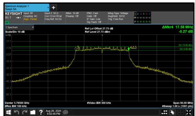
Figure 291 - 802.11n HT20 Maximum 6 dB EBW
