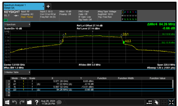
Figure 287 - 802.11ax HE80 SU Maximum 99% OBW
