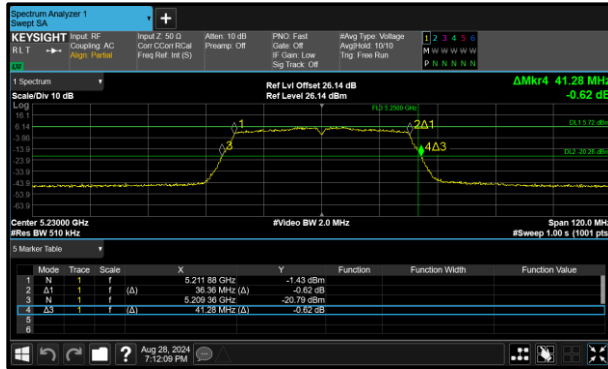
Figure 304 - 802.11n HT40 Minimum 99% OBW
