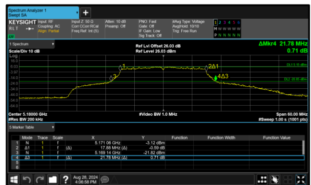
Figure 275 - 802.11n HT20 Maximum 99% OBW
