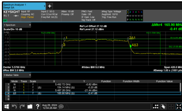
Figure 308 - 802.11ac VHT160 Minimum 99% OBW
