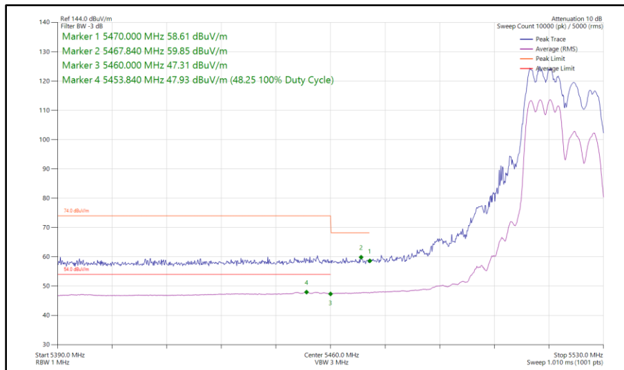
Figure 66 - 802.11ax HE20, RU 106-53, CDD, Core 0 - Core 1 - 5520 MHz Band Edge Frequency 5460 MHz
