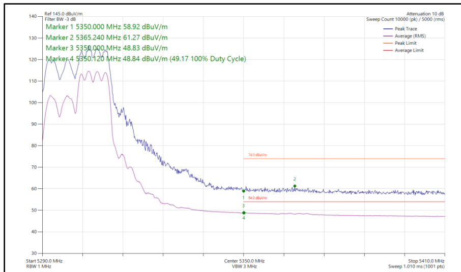
Figure 74 - 802.11ax HE20, RU 106-54, SDM, Core 0 - Core 1 - 5300 MHz Band Edge Frequency 5350 MHz
