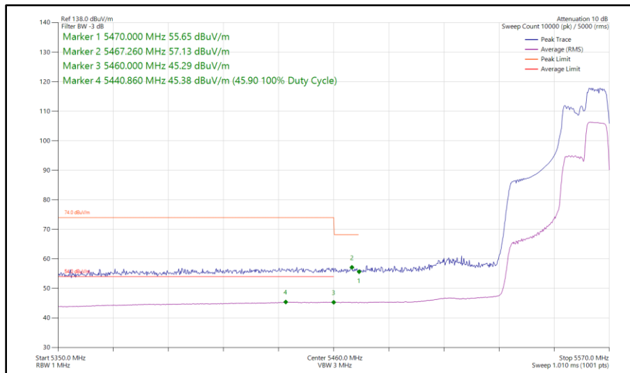
Figure 106 - 802.11ax HE40, RU 106-56, SISO, Core 0 - 5550 MHz Band Edge Frequency 5460 MHz
