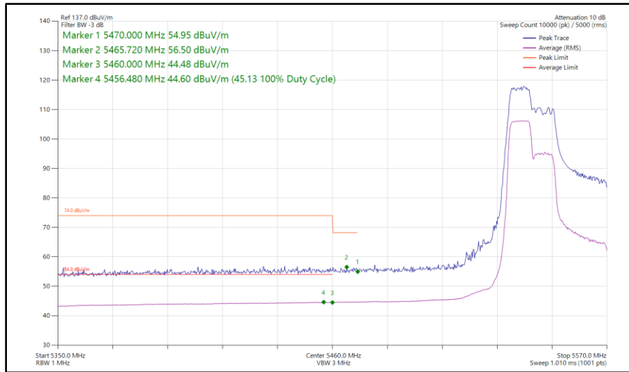
Figure 124 - 802.11ax HE40, RU 106-53, SISO, Core 1 - 5550 MHz Band Edge Frequency 5460 MHz
