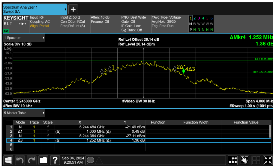
Figure 81 - Core 1 (B) 5245 MHz (CH95) 26 dB and 99% Bandwidth
