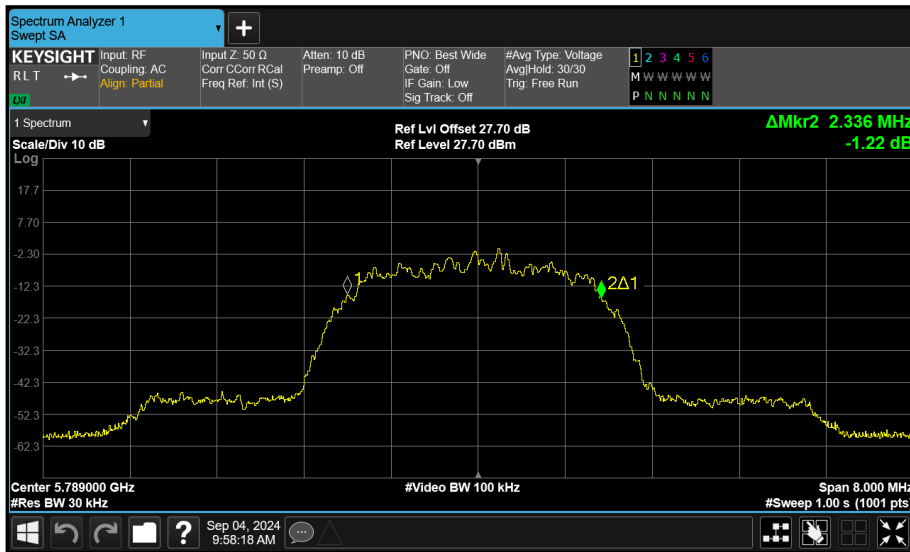
Figure 110 - Core 0 (A) 5789 MHz (CH64) 99% Bandwidth
