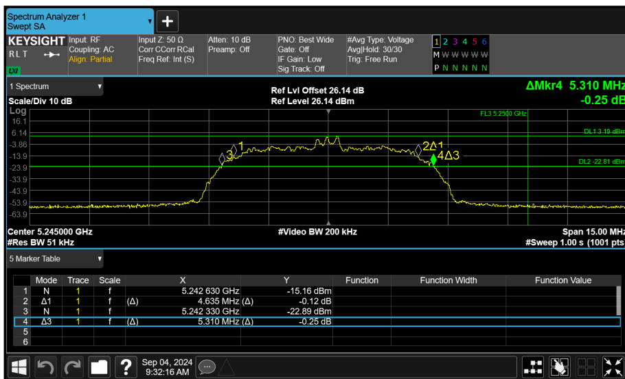
Figure 93 - Core 1 (B) 5245 MHz (CH95) 26 dB and 99% Bandwidth
