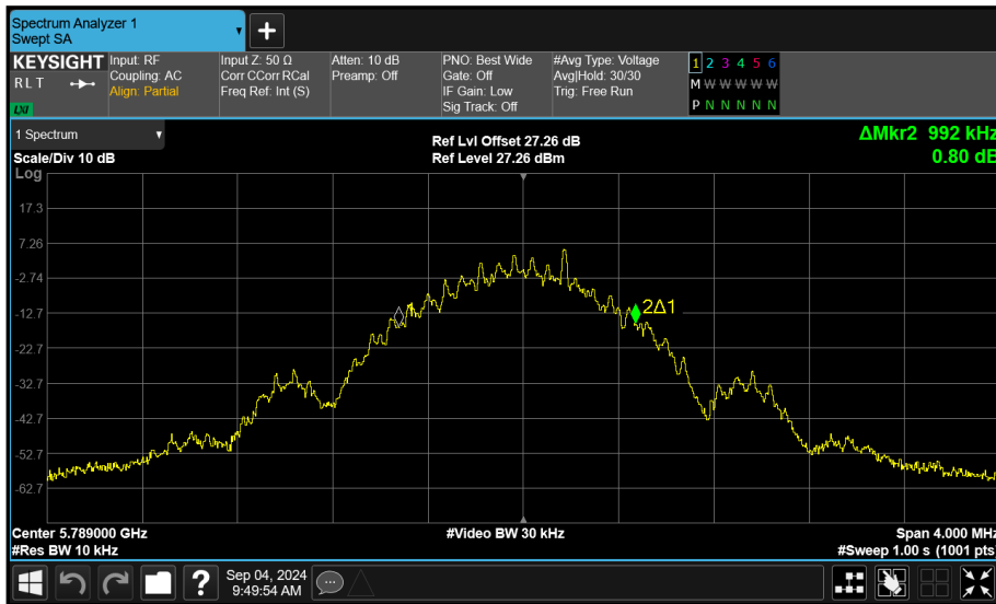
Figure 100 - Core 1 (B) 5789 MHz (CH64) 99% Bandwidth
