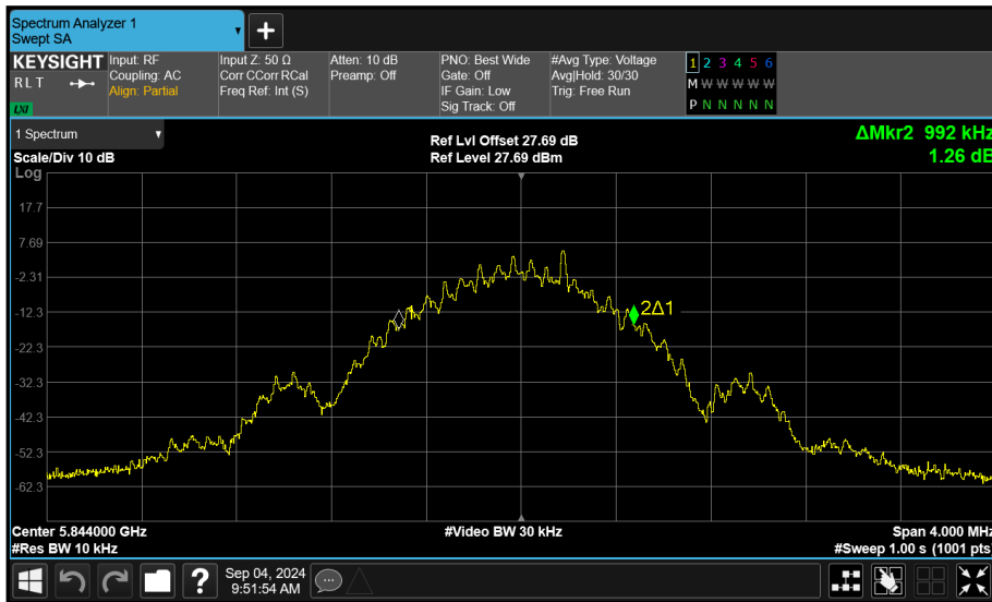
Figure 102 - Core 0 (A) 5844 MHz (CH119) 99% Bandwidth
