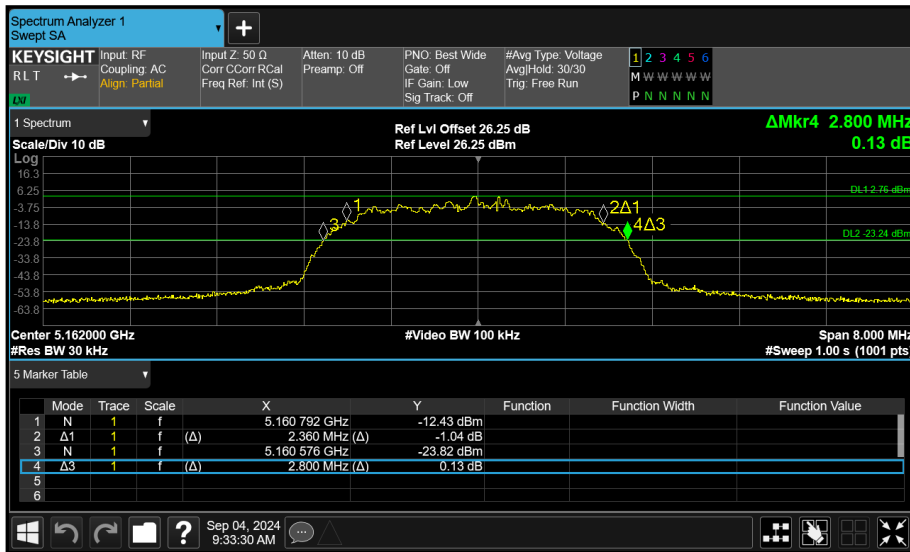
Figure 130 - Core 0 (A) 5162 MHz (CH12) 26 dB and 99% Bandwidth
