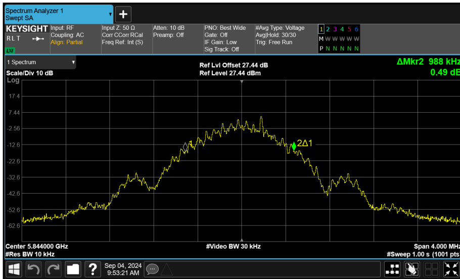
Figure 104 - Core 1 (B) 5844 MHz (CH119) 99% Bandwidth
