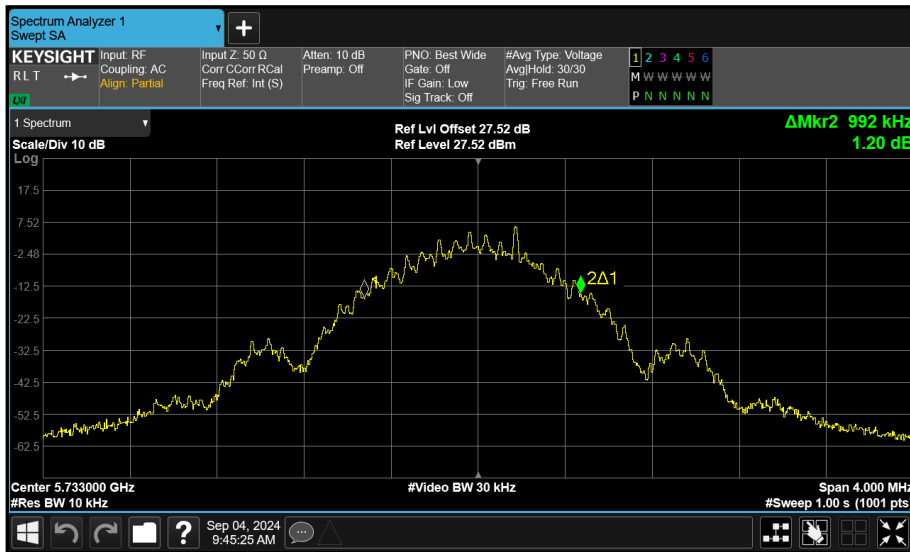
Figure 94 - Core 0 (A) 5733 MHz (CH8) 99% Bandwidth
