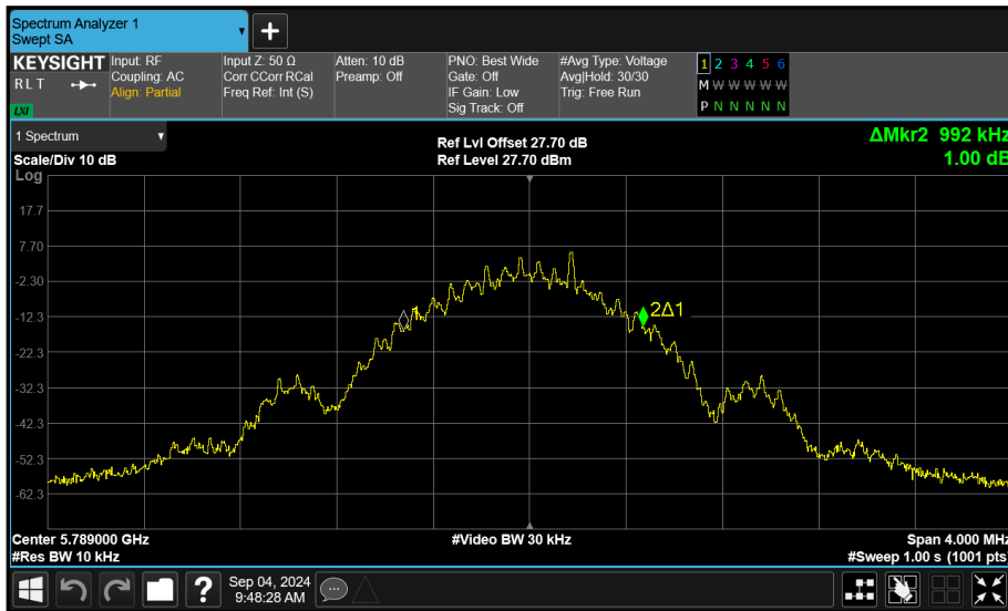
Figure 98 - Core 0 (A) 5789 MHz (CH64) 99% Bandwidth
