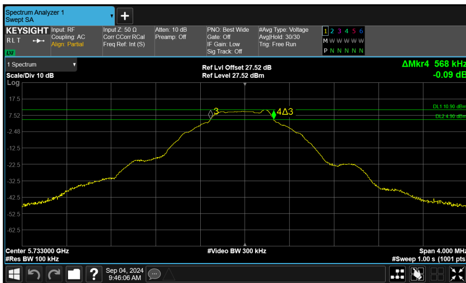
Figure 95 - Core 0 (A) 5733 MHz (CH8) 6 dB Bandwidth
