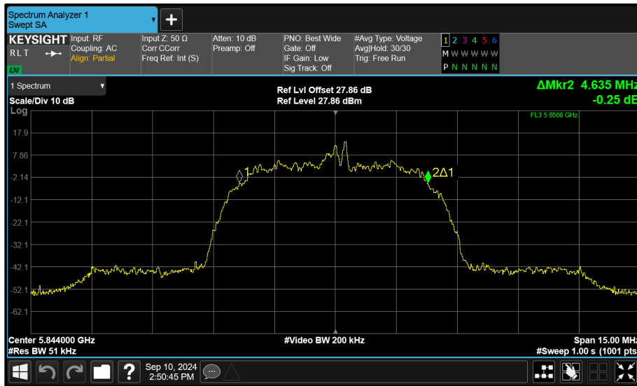
Figure 110 - Core 1 (B) 5844 MHz (CH119) 99% Bandwidth
