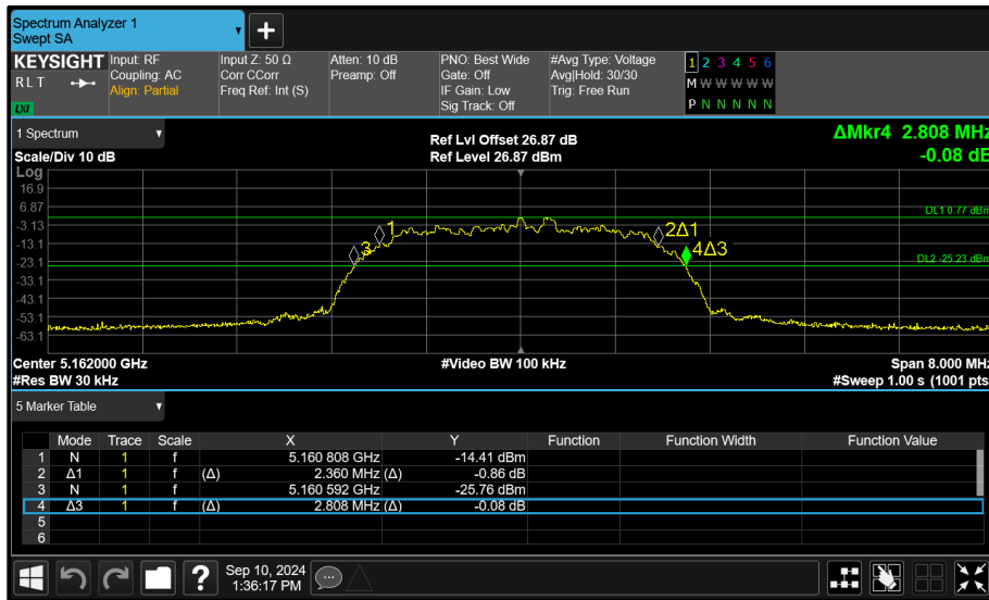
Figure 118 - Core 0 (A) 5162 MHz (CH12) 26 dB and 99% Bandwidth
