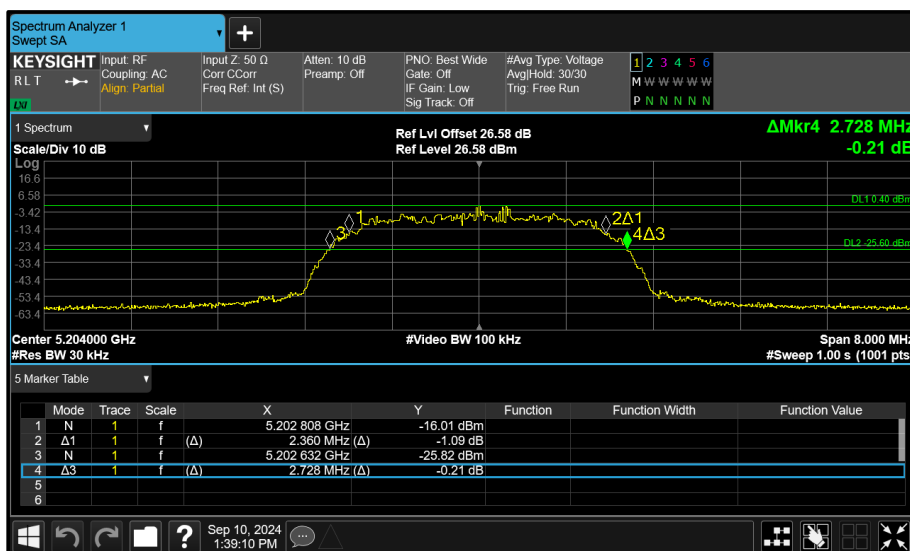
Figure 121 - Core 1 (B) 5204 MHz (CH54) 26 dB and 99% Bandwidth
