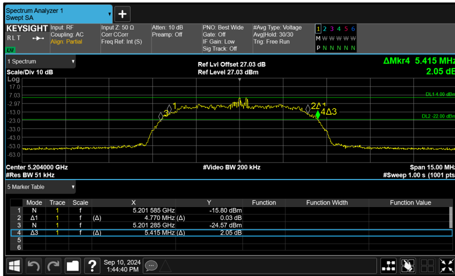
Figure 126 - Core 0 (A) 5204 MHz (CH54) 26 dB and 99% Bandwidth
