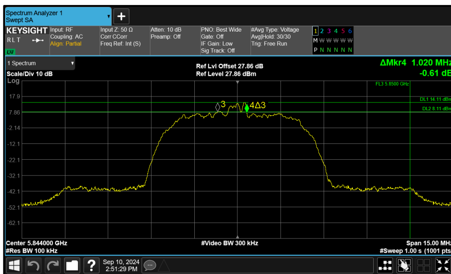
Figure 111 - Core 1 (B) 5844 MHz (CH119) 6 dB Bandwidth
