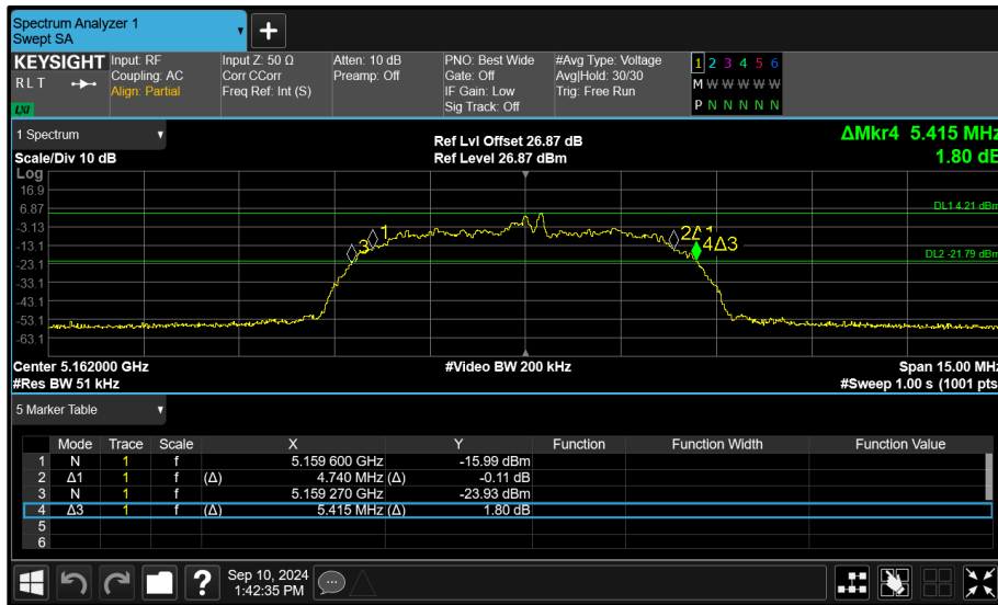
Figure 124 - Core 0 (A) 5162 MHz (CH12) 26 dB and 99% Bandwidth
