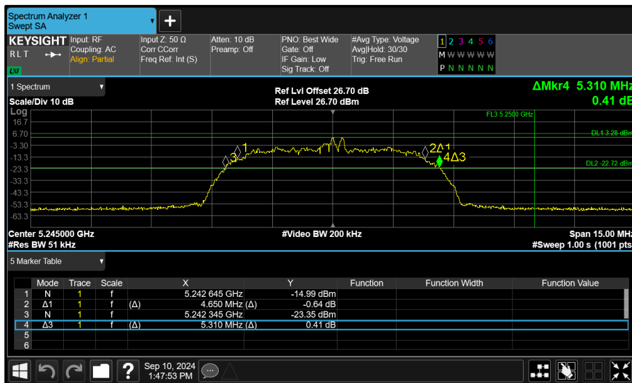
Figure 129 - Core 1 (B) 5245 MHz (CH95) 26 dB and 99% Bandwidth
