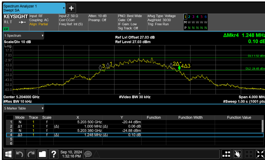
Figure 114 - Core 0 (A) 5204 MHz (CH54) 26 dB and 99% Bandwidth
