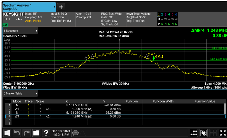
Figure 112 - Core 0 (A) 5162 MHz (CH12) 26 dB and 99% Bandwidth
