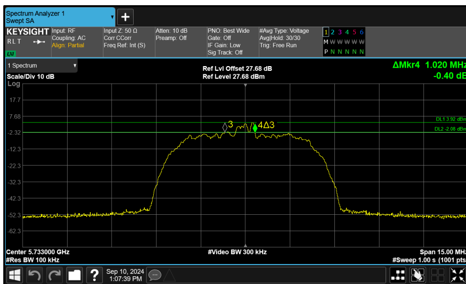
Figure 71 - Core 1 (B) 5733 MHz (CH8) 6 dB Bandwidth
