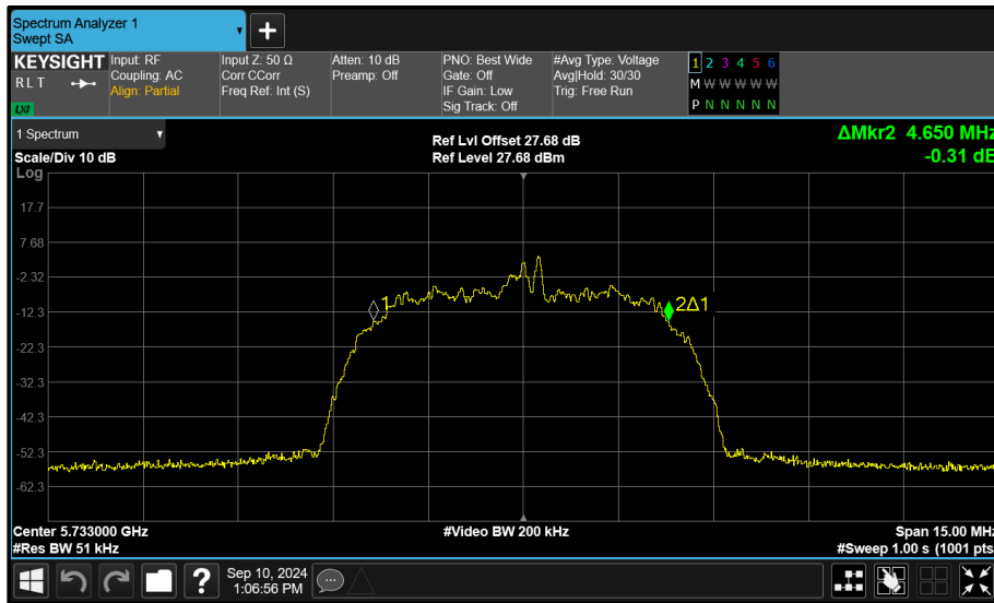
Figure 70 - Core 1 (B) 5733 MHz (CH8) 99% Bandwidth
