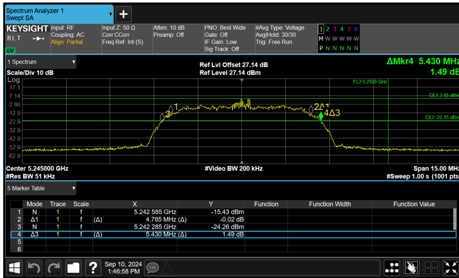
Figure 128 - Core 0 (A) 5245 MHz (CH95) 26 dB and 99% Bandwidth
