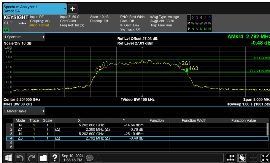
Figure 120 - Core 0 (A) 5204 MHz (CH54) 26 dB and 99% Bandwidth
