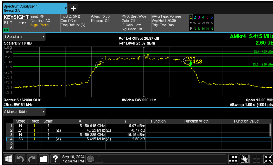
Figure 43 - Core 0 (A) 5162 MHz (CH12) 26 dB and 99% Bandwidth
