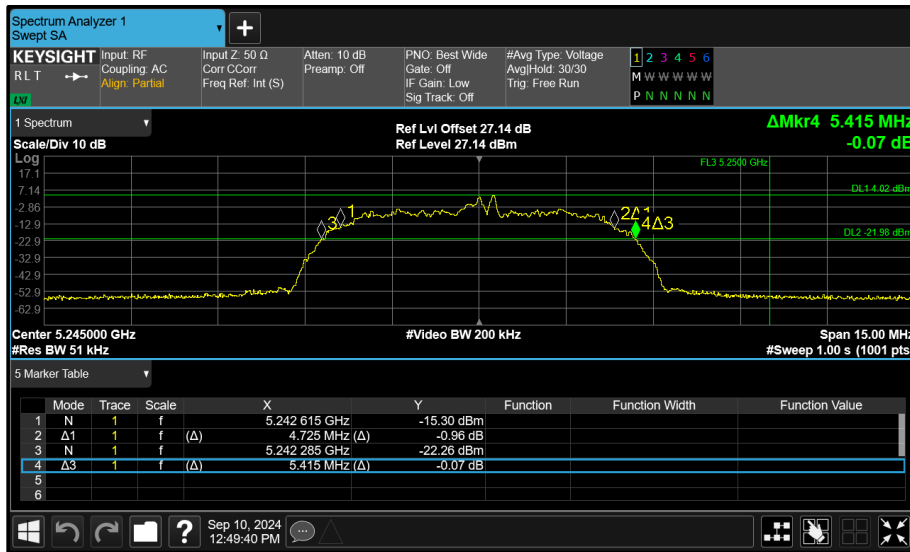
Figure 39 - Core 0 (A) 5245 MHz (CH95) 26 dB and 99% Bandwidth
