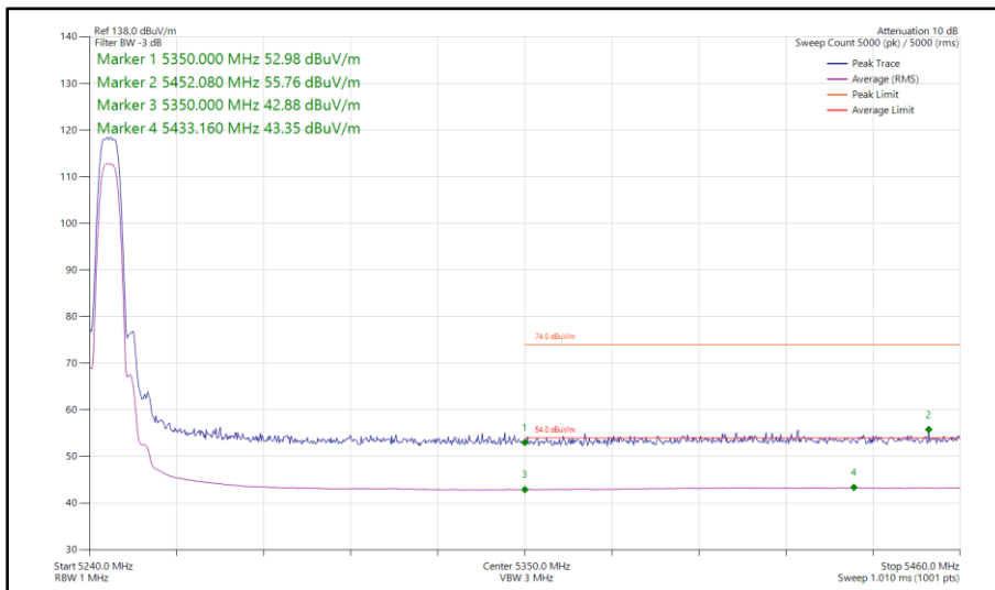
Figure 26 - Bluetooth HDR8, SISO, Core 1 - 5245 MHz Band Edge Frequency 5350 MHz
