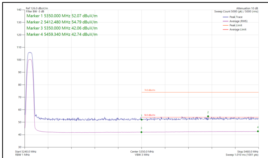
Figure 12 - Bluetooth HDR8, SISO, Core 1 - 5245 MHz Band Edge Frequency 5350 MHz
