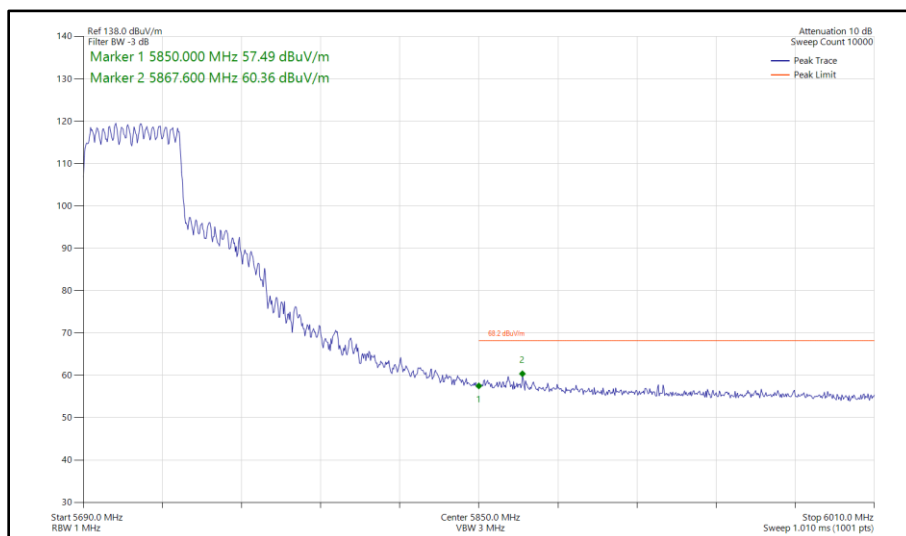
Figure 525 - 802.11ax HE40, SU, CDD, Core 0 - Core 1 - 5710 MHz Band Edge Frequency 5850 MHz
