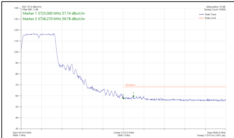
Figure 538 - 802.11n HT40, SDM, Core 0 - Core 1 - 5630 MHz Band Edge Frequency 5725 MHz
