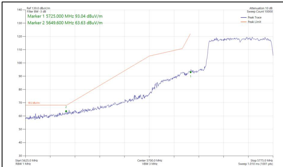
Figure 536 - 802.11ax HE40, SU, SDM, Core 0 - Core 1 - 5755 MHz Band Edge Frequency 5725 MHz
