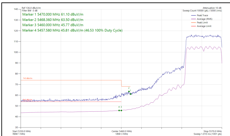
Figure 533 - 802.11ax HE40, SU, SDM, Core 0 - Core 1 - 5550 MHz Band Edge Frequency 5470 MHz
