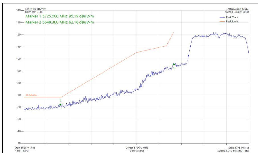
Figure 552 - 802.11ac VHT40, TxBF, Core 0 - Core 1 - 5755 MHz Band Edge Frequency 5725 MHz
