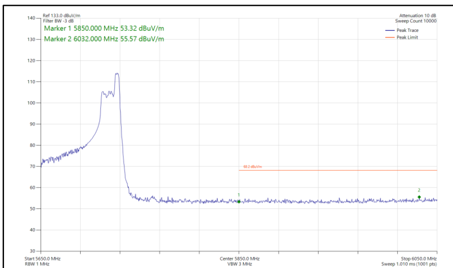
Figure 569 - 802.11ax HE80, RU 52-52, SISO, Core 0 - 5690 MHz Band Edge Frequency 5850 MHz
