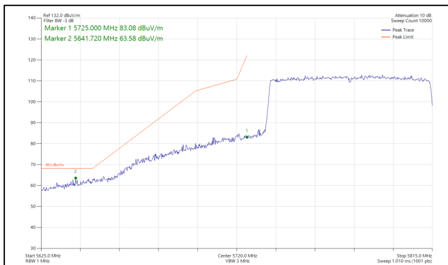
Figure 561 - 802.11ax HE80, SU, SISO, Core 0 - 5775 MHz Band Edge Frequency 5725 MHz
