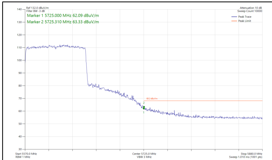
Figure 579 - 802.11ax HE80, SU, SISO, Core 1 - 5610 MHz Band Edge Frequency 5725 MHz
