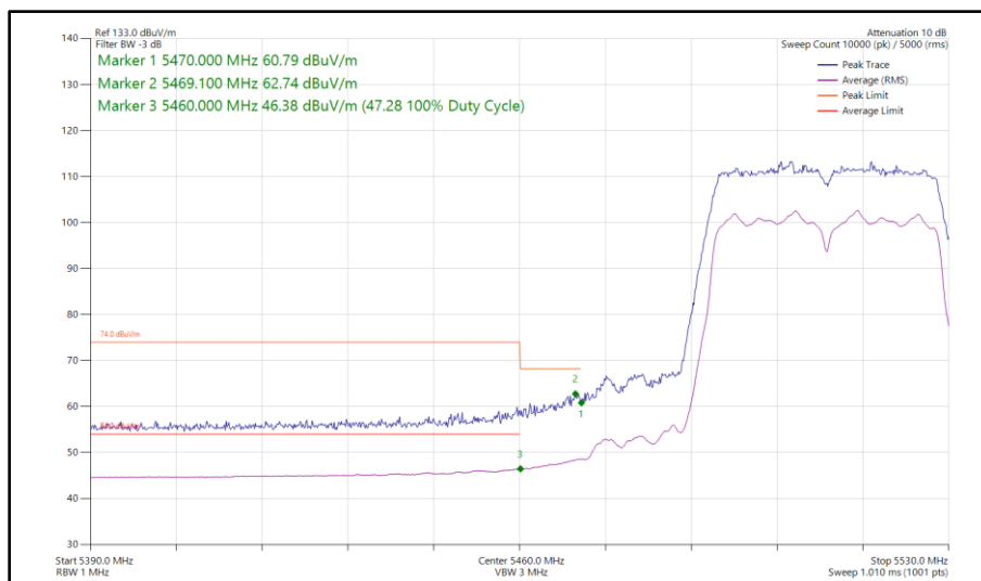
Figure 529 - 802.11n HT40, SDM, Core 0 - Core 1 - 5510 MHz Band Edge Frequency 5470 MHz
