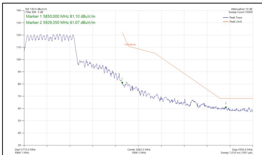
Figure 527 - 802.11ax HE40, SU, CDD, Core 0 - Core 1 - 5795 MHz Band Edge Frequency 5850 MHz
