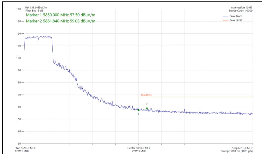
Figure 505 - 802.11ax HE40, SU, SISO, Core 1 - 5710 MHz Band Edge Frequency 5850 MHz
