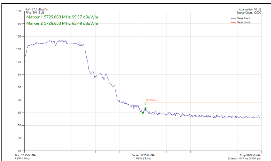
Figure 539 - 802.11n HT40, SDM, Core 0 - Core 1 - 5670 MHz Band Edge Frequency 5725 MHz
