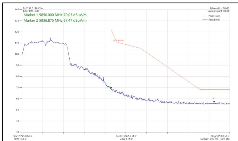
Figure 556 - 802.11ac VHT40, TxBF, Core 0 - Core 1 - 5795 MHz Band Edge Frequency 5850 MHz
