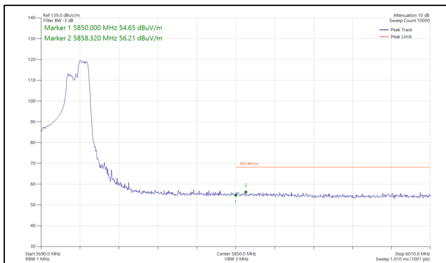
Figure 506 - 802.11ax HE40, RU 106-56, SISO, Core 1 - 5710 MHz Band Edge Frequency 5850 MHz
