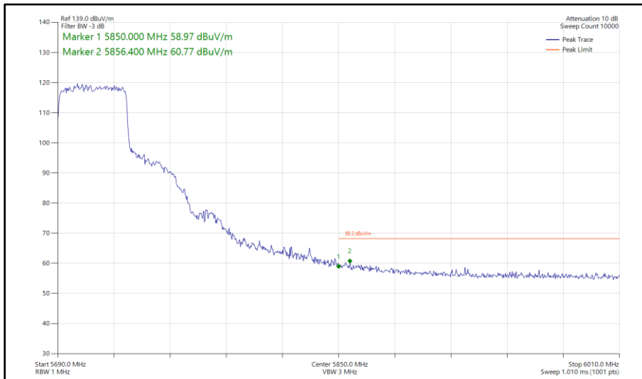
Figure 546 - 802.11ax HE40, SU, SDM, Core 0 - Core 1 - 5710 MHz Band Edge Frequency 5850 MHz
