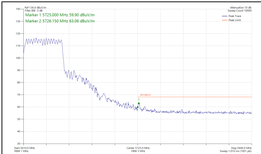
Figure 520 - 802.11ax HE40, SU, CDD, Core 0 - Core 1 - 5630 MHz Band Edge Frequency 5725 MHz
