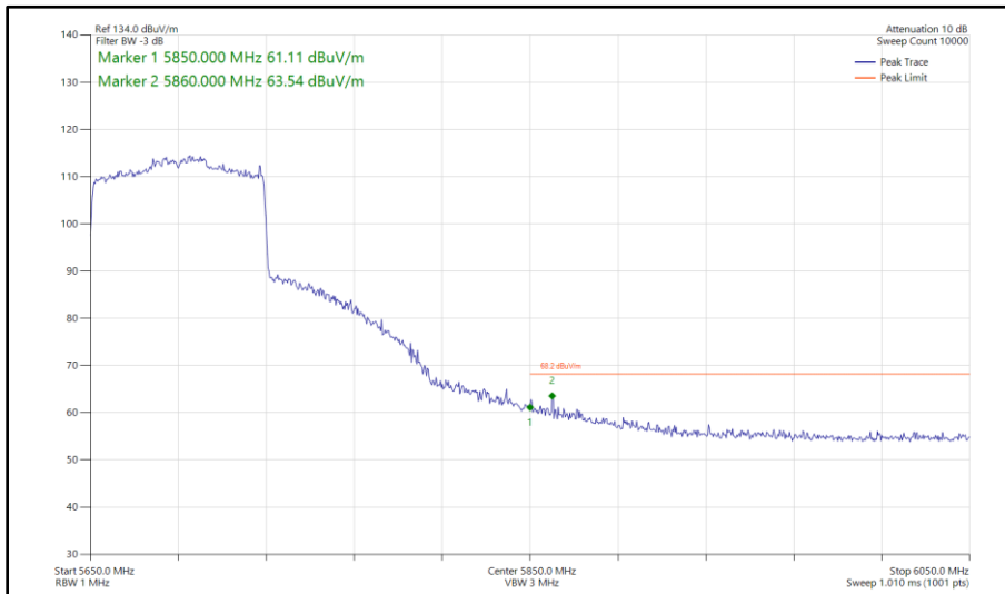
Figure 568 - 802.11ax HE80, SU, SISO, Core 0 - 5690 MHz Band Edge Frequency 5850 MHz
