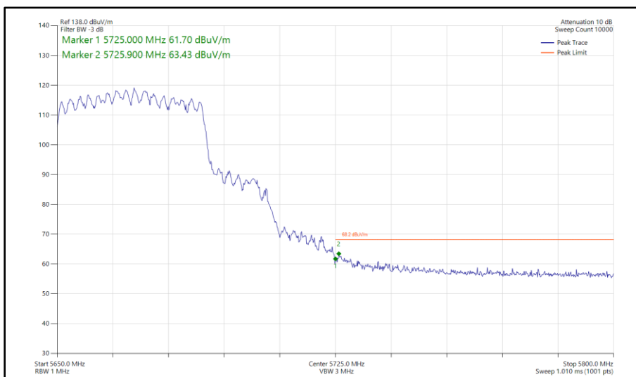
Figure 521 - 802.11ax HE40, SU, CDD, Core 0 - Core 1 - 5670 MHz Band Edge Frequency 5725 MHz
