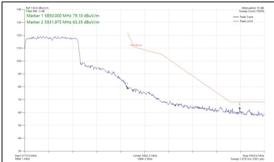
Figure 548 - 802.11ax HE40, SU, SDM, Core 0 - Core 1 - 5795 MHz Band Edge Frequency 5850 MHz
