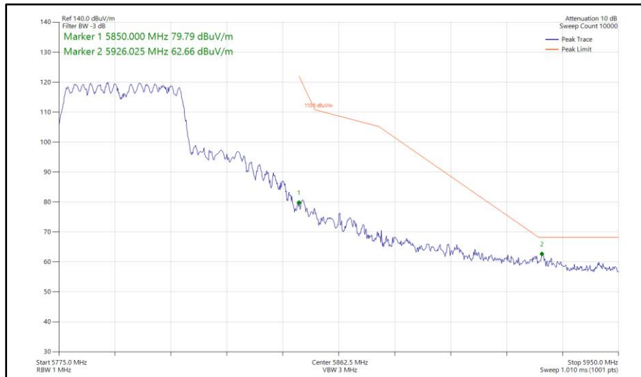
Figure 524 - 802.11n HT40, CDD, Core 0 - Core 1 - 5795 MHz Band Edge Frequency 5850 MHz
