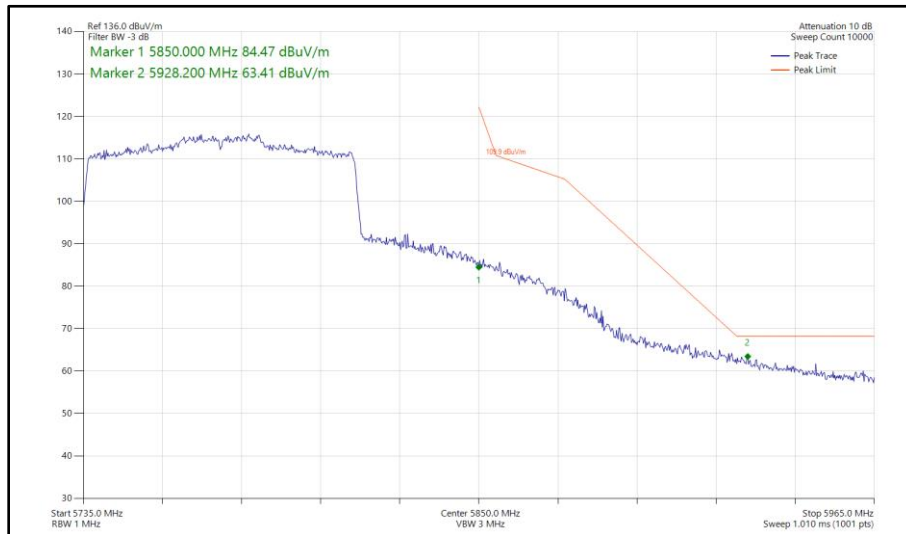
Figure 570 - 802.11ax HE80, SU, SISO, Core 0 - 5775 MHz Band Edge Frequency 5850 MHz
