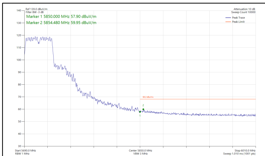
Figure 523 - 802.11n HT40, CDD, Core 0 - Core 1 - 5710 MHz Band Edge Frequency 5850 MHz
