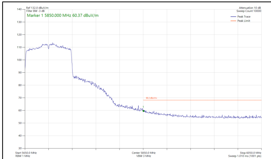
Figure 566 - 802.11ac VHT80, SISO, Core 0 - 5690 MHz Band Edge Frequency 5850 MHz
