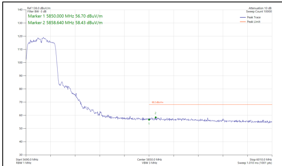
Figure 544 - 802.11n HT40, SDM, Core 0 - Core 1 - 5710 MHz Band Edge Frequency 5850 MHz
