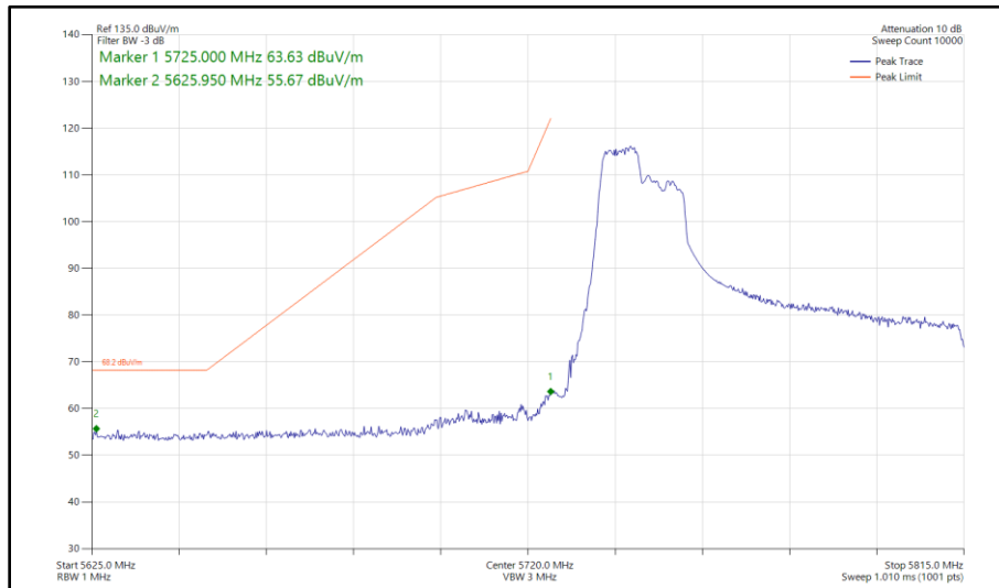
Figure 577 - 802.11ax HE80, RU 106-53, SISO, Core 1 - 5775 MHz Band Edge Frequency 5725 MHz
