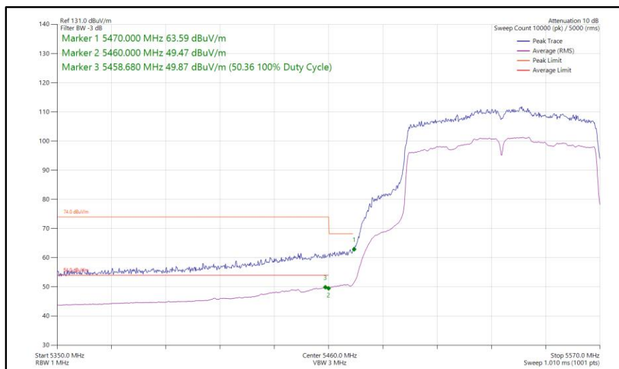
Figure 557 - 802.11ac VHT80, SISO, Core 0 - 5530 MHz Band Edge Frequency 5470 MHz
