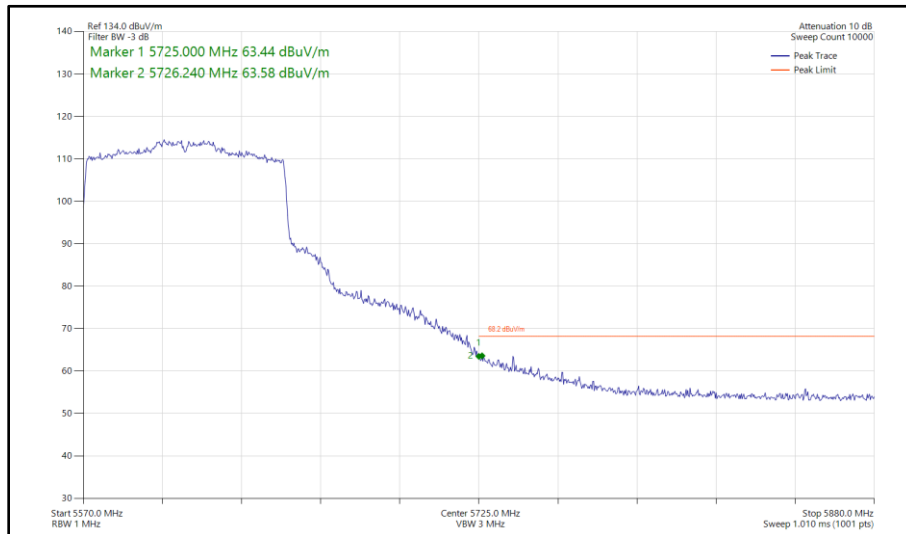
Figure 564 - 802.11ax HE80, SU, SISO, Core 0 - 5610 MHz Band Edge Frequency 5725 MHz
