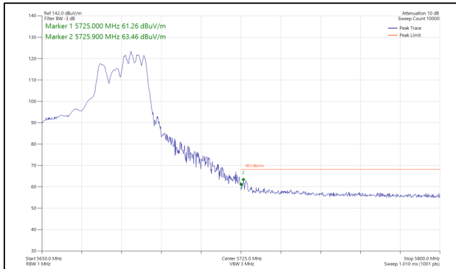
Figure 522 - 802.11ax HE40, RU 106-56, CDD, Core 0 - Core 1 - 5670 MHz Band Edge Frequency 5725 MHz
