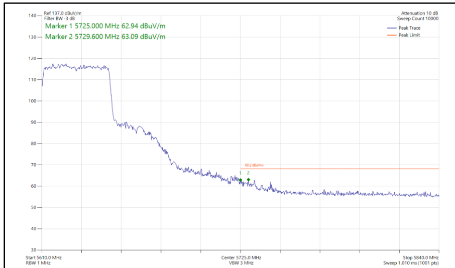
Figure 540 - 802.11ax HE40, SU, SDM, Core 0 - Core 1 - 5630 MHz Band Edge Frequency 5725 MHz
