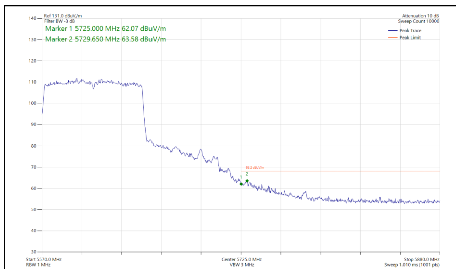
Figure 563 - 802.11ac VHT80, SISO, Core 0 - 5610 MHz Band Edge Frequency 5725 MHz
