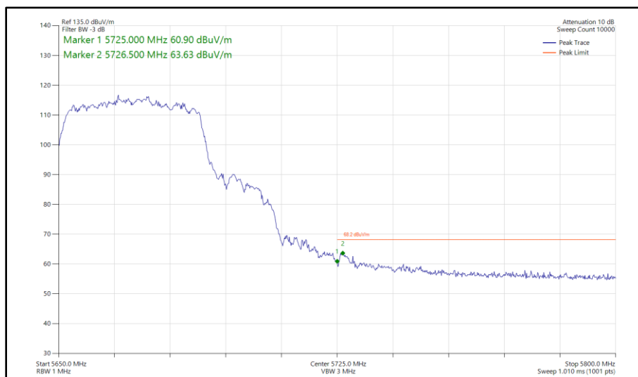
Figure 519 - 802.11n HT40, CDD, Core 0 - Core 1 - 5670 MHz Band Edge Frequency 5725 MHz
