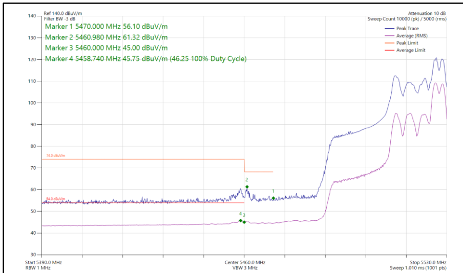
Figure 532 - 802.11ax HE40, RU 52-44, SDM, Core 0 - Core 1 - 5510 MHz Band Edge Frequency 5470 MHz
