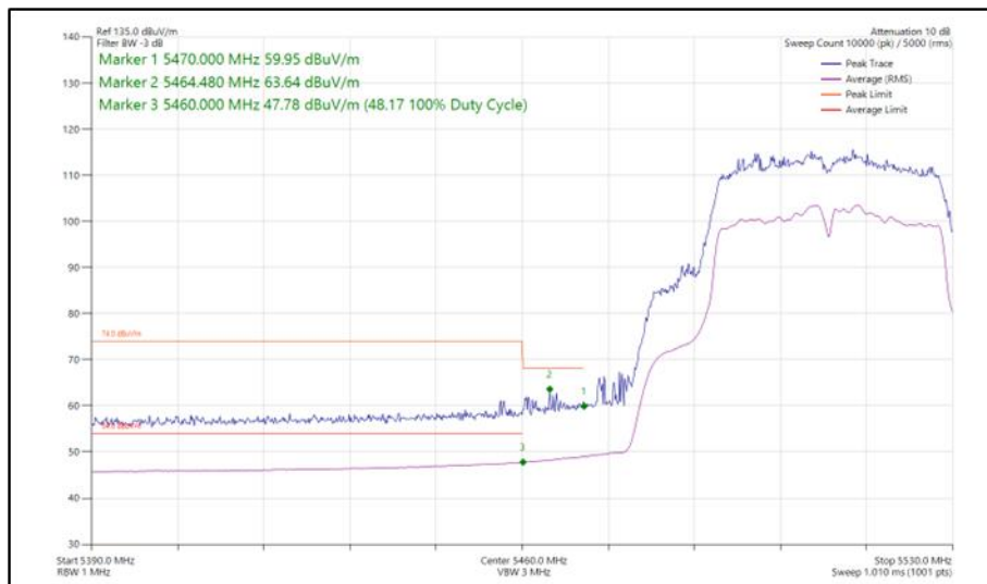
Figure 550 - 802.11ac VHT40, TxBF, Core 0 - Core 1 - 5510 MHz Band Edge Frequency 5470 MHz
