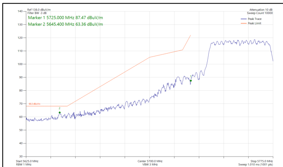
Figure 515 - 802.11n HT40, CDD, Core 0 - Core 1 - 5755 MHz Band Edge Frequency 5725 MHz
