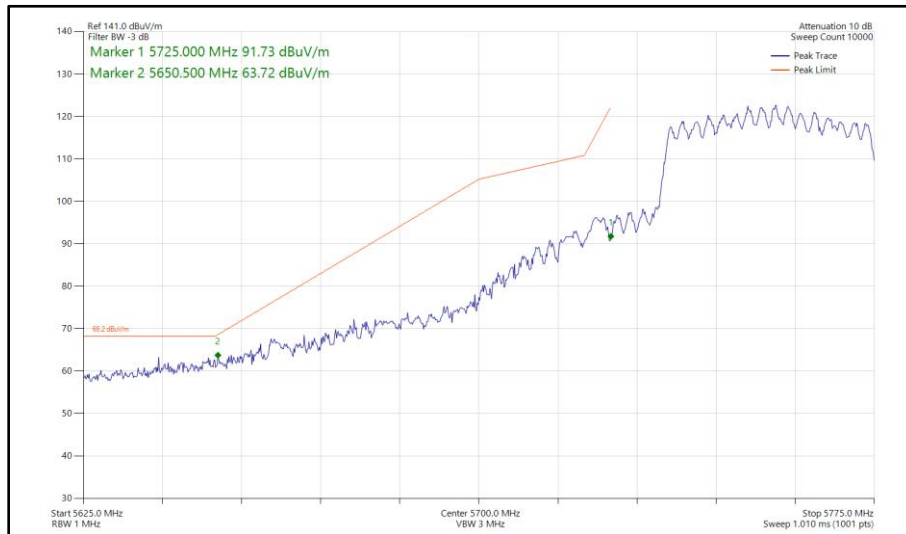
Figure 516 - 802.11ax HE40, SU, CDD, Core 0 - Core 1 - 5755 MHz Band Edge Frequency 5725 MHz
