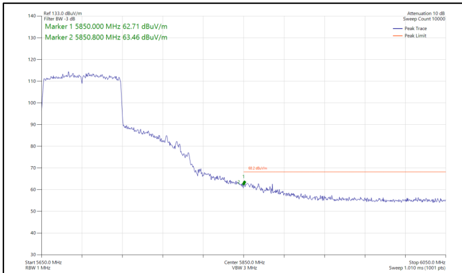
Figure 581 - 802.11ac VHT80, SISO, Core 1 - 5690 MHz Band Edge Frequency 5850 MHz
