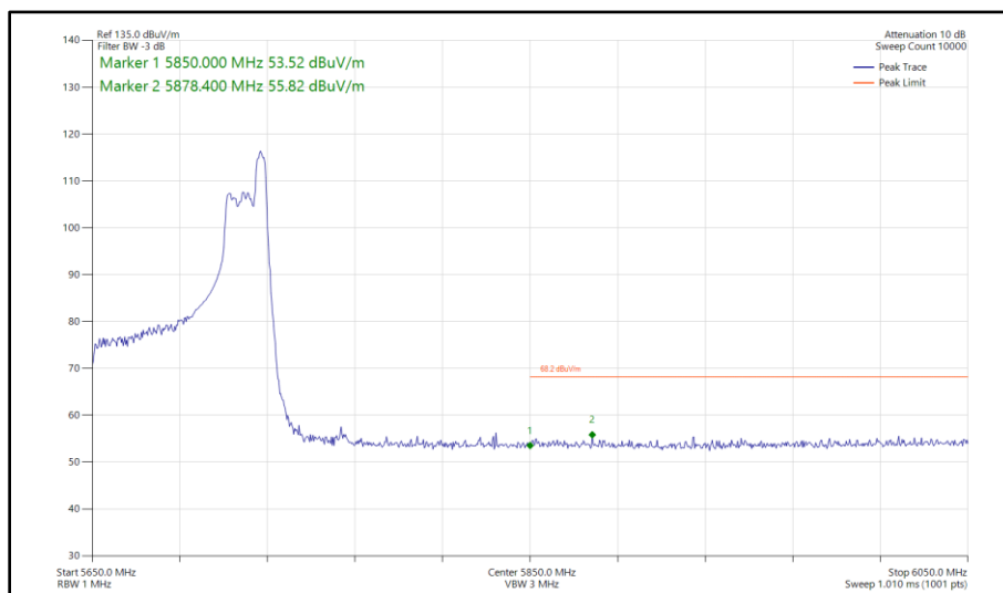
Figure 584 - 802.11ax HE80, RU 52-52, SISO, Core 1 - 5690 MHz Band Edge Frequency 5850 MHz
