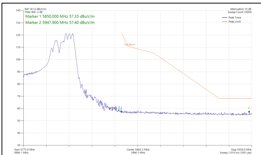
Figure 549 - 802.11ax HE40, RU 106-56, SDM, Core 0 - Core 1 - 5795 MHz Band Edge Frequency 5850 MHz
