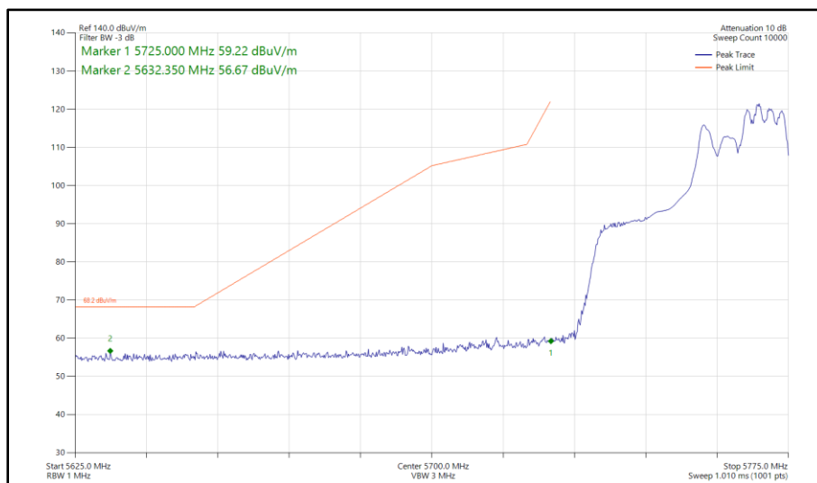
Figure 517 - 802.11ax HE40, RU 106-56, CDD, Core 0 - Core 1 - 5755 MHz Band Edge Frequency 5725 MHz
