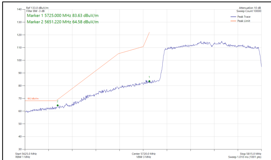
Figure 575 - 802.11ac VHT80, SISO, Core 1 - 5775 MHz Band Edge Frequency 5725 MHz
