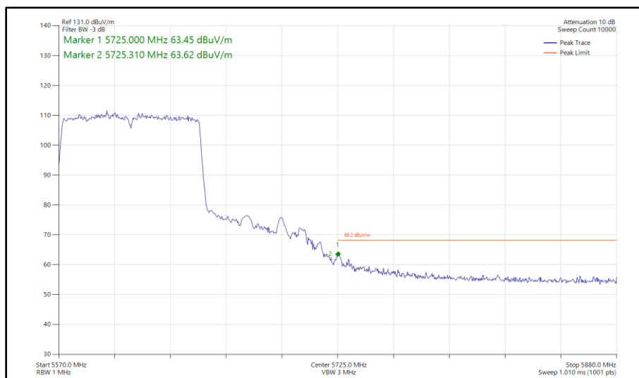
Figure 578 - 802.11ac VHT80, SISO, Core 1 - 5610 MHz Band Edge Frequency 5725 MHz
