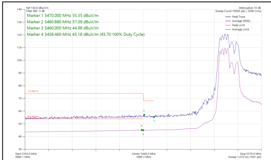
Figure 534 - 802.11ax HE40, RU 106-53, SDM, Core 0 - Core 1 - 5550 MHz Band Edge Frequency 5470 MHz
