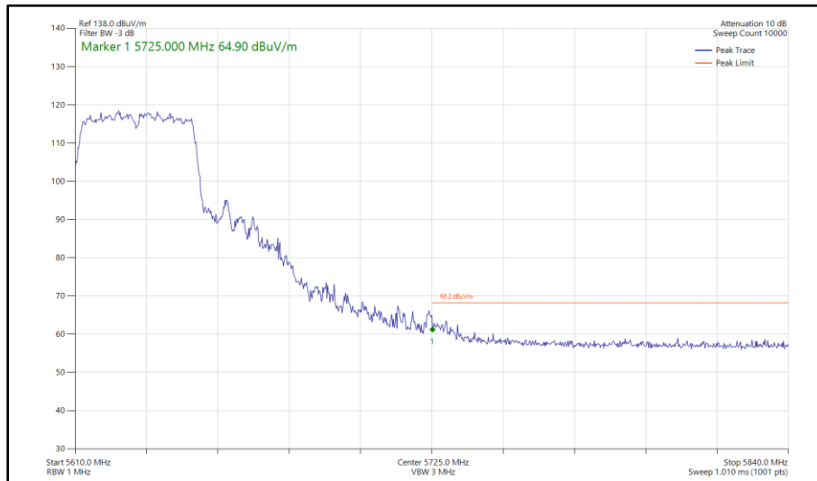
Figure 553 - 802.11ac VHT40, TxBF, Core 0 - Core 1 - 5630 MHz Band Edge Frequency 5725 MHz
