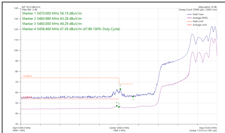
Figure 512 - 802.11ax HE40, RU 52-44, CDD, Core 0 - Core 1 - 5510 MHz Band Edge Frequency 5470 MHz
