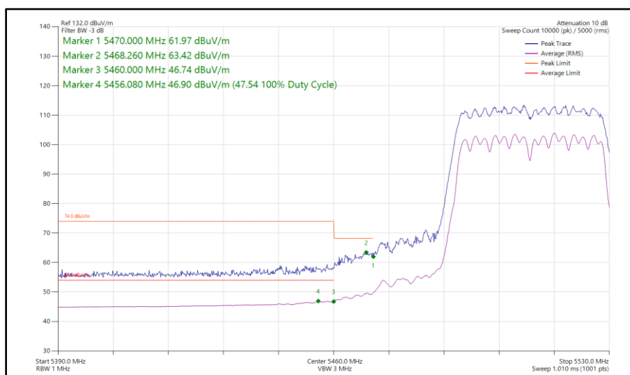
Figure 509 - 802.11n HT40, CDD, Core 0 - Core 1 - 5510 MHz Band Edge Frequency 5470 MHz
