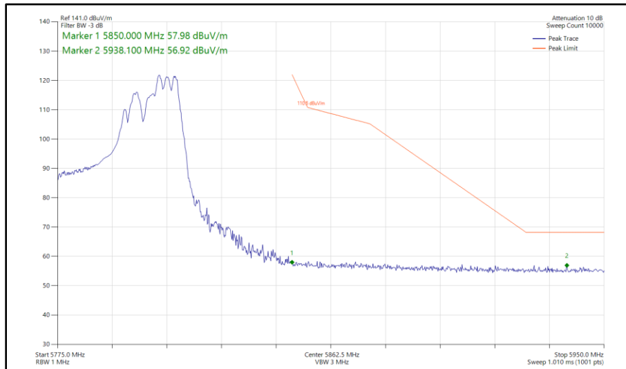
Figure 528 - 802.11ax HE40, RU 106-56, CDD, Core 0 - Core 1 - 5795 MHz Band Edge Frequency 5850 MHz
