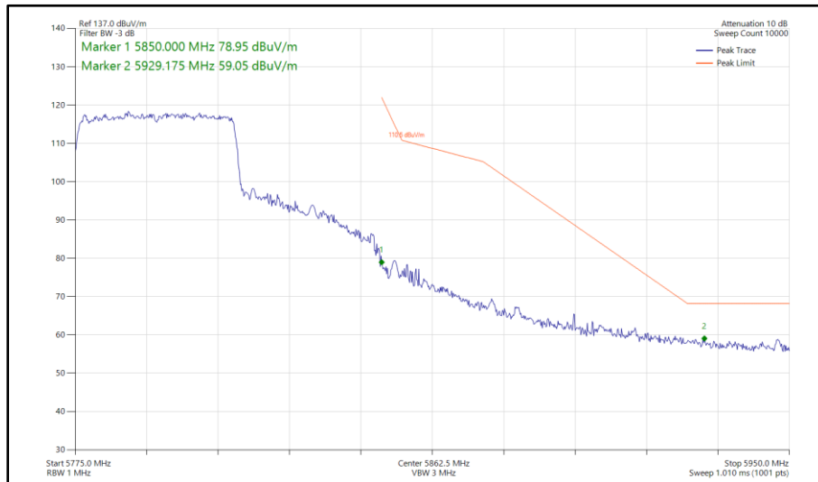
Figure 507 - 802.11ax HE40, SU, SISO, Core 1 - 5795 MHz Band Edge Frequency 5850 MHz
