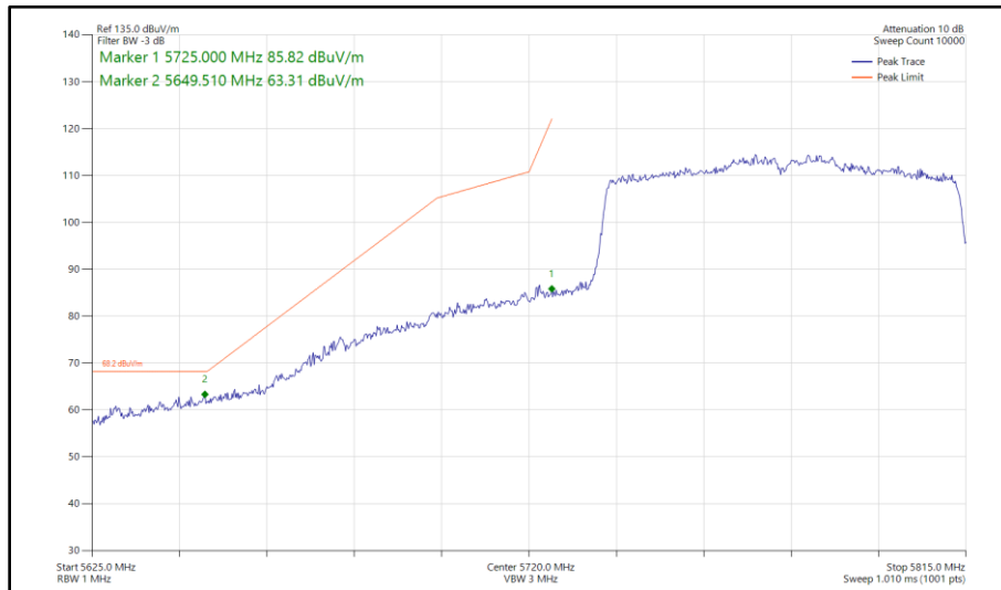
Figure 560 - 802.11ac VHT80, SISO, Core 0 - 5775 MHz Band Edge Frequency 5725 MHz
