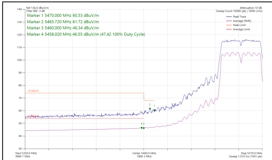
Figure 530 - 802.11n HT40, SDM, Core 0 - Core 1 - 5550 MHz Band Edge Frequency 5470 MHz
