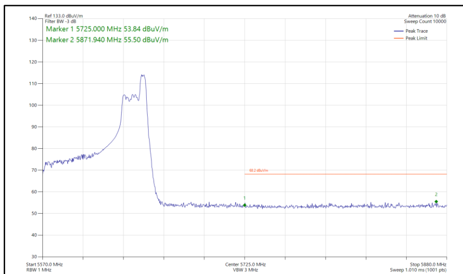
Figure 565 - 802.11ax HE80, RU 52-52, SISO, Core 0 - 5610 MHz Band Edge Frequency 5725 MHz
