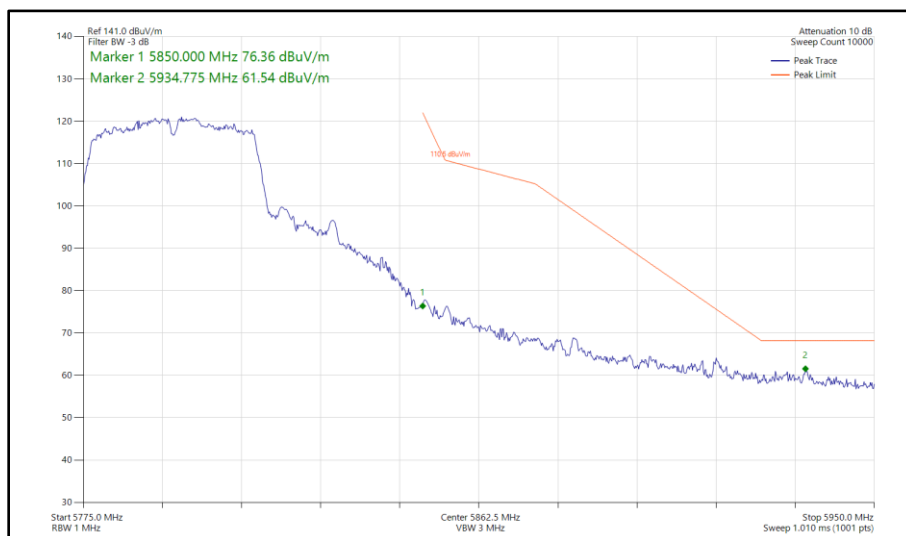
Figure 545 - 802.11n HT40, SDM, Core 0 - Core 1 - 5795 MHz Band Edge Frequency 5850 MHz
