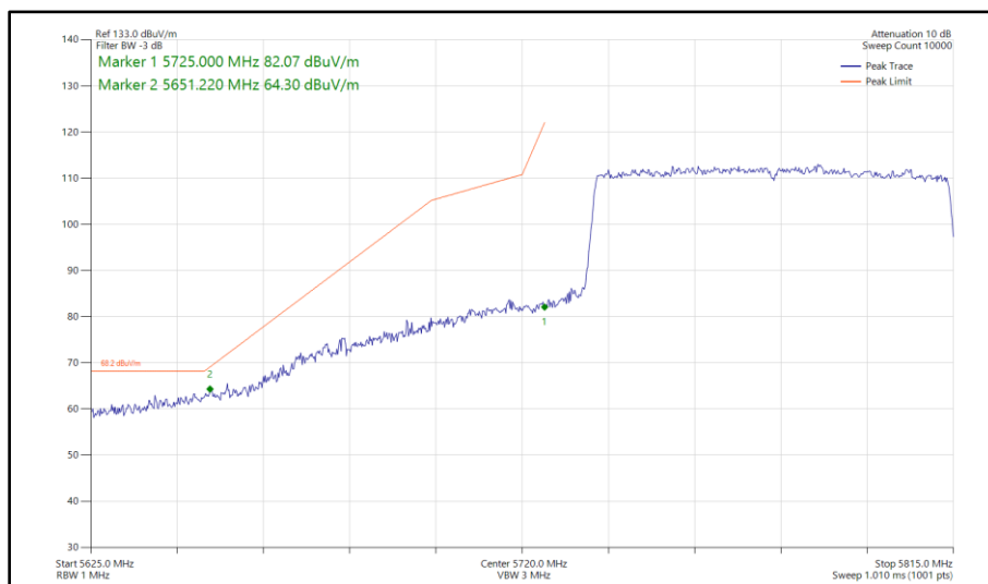
Figure 576 - 802.11ax HE80, SU, SISO, Core 1 - 5775 MHz Band Edge Frequency 5725 MHz
