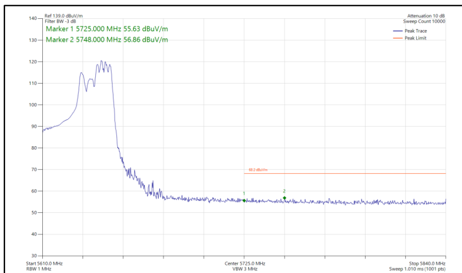
Figure 541 - 802.11ax HE40, RU 106-56, SDM, Core 0 - Core 1 - 5630 MHz Band Edge Frequency 5725 MHz
