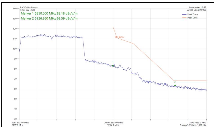
Figure 582 - 802.11ac VHT80, SISO, Core 1 - 5775 MHz Band Edge Frequency 5850 MHz
