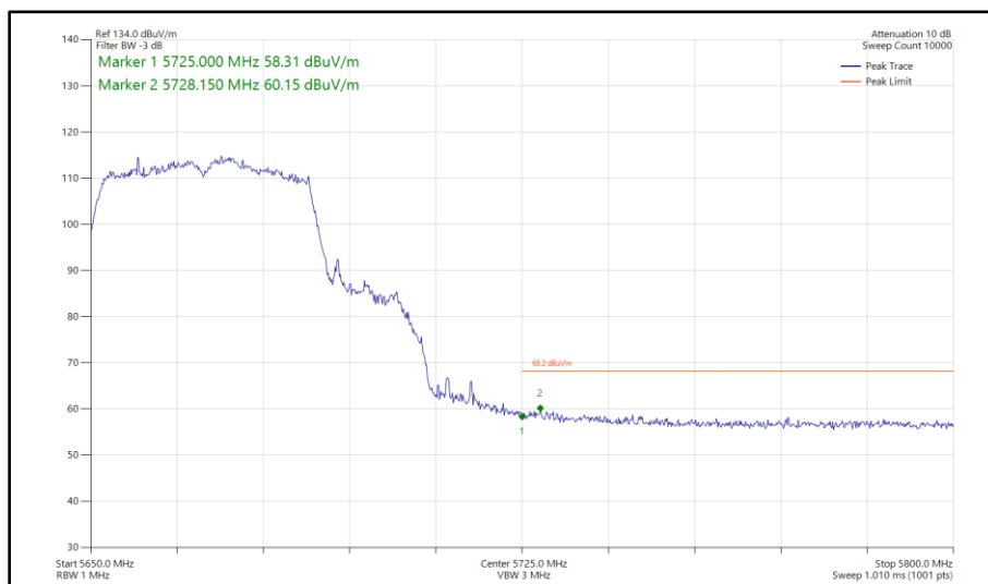
Figure 554 - 802.11ac VHT40, TxBF, Core 0 - Core 1 - 5670 MHz Band Edge Frequency 5725 MHz
