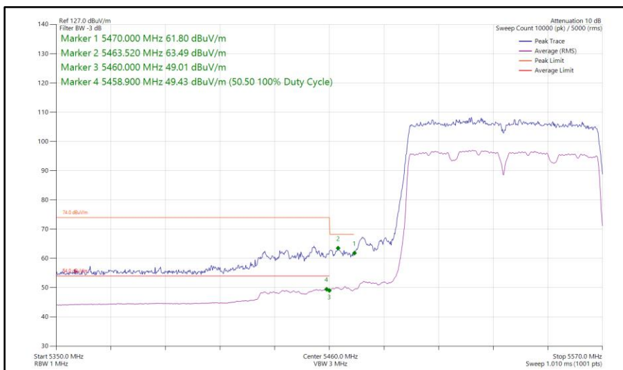
Figure 572 - 802.11ac VHT80, SISO, Core 1 - 5530 MHz Band Edge Frequency 5470 MHz
