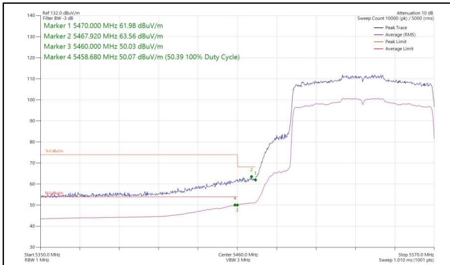
Figure 558 - 802.11ax HE80, SU, SISO, Core 0 - 5530 MHz Band Edge Frequency 5470 MHz
