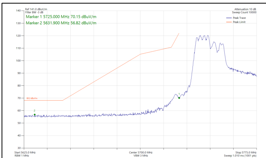
Figure 537 - 802.11ax HE40, RU 106-53, SDM, Core 0 - Core 1 - 5755 MHz Band Edge Frequency 5725 MHz
