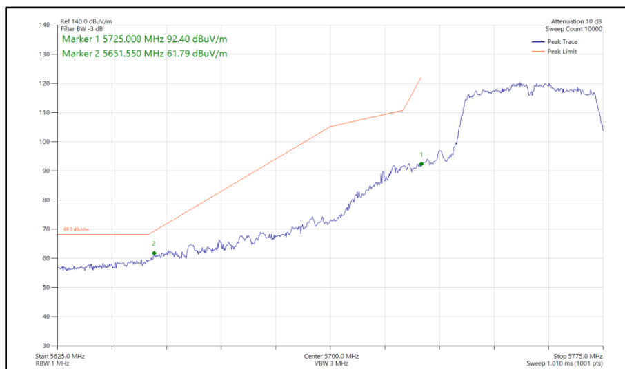
Figure 535 - 802.11n HT40, SDM, Core 0 - Core 1 - 5755 MHz Band Edge Frequency 5725 MHz
