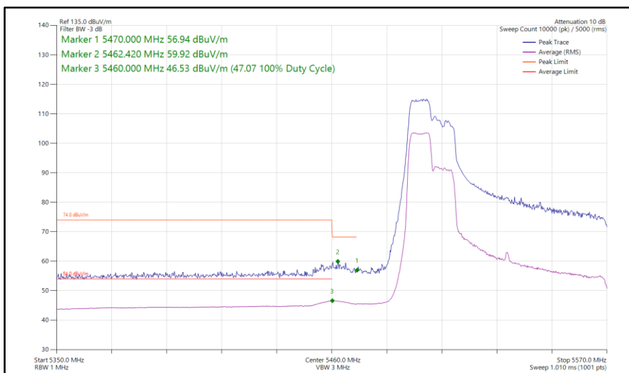
Figure 559 - 802.11ax HE80, RU 106-53, SISO, Core 0 - 5530 MHz Band Edge Frequency 5470 MHz
