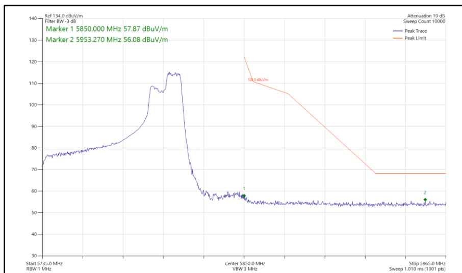
Figure 571 - 802.11ax HE80, RU 106-60, SISO, Core 0 - 5775 MHz Band Edge Frequency 5850 MHz
