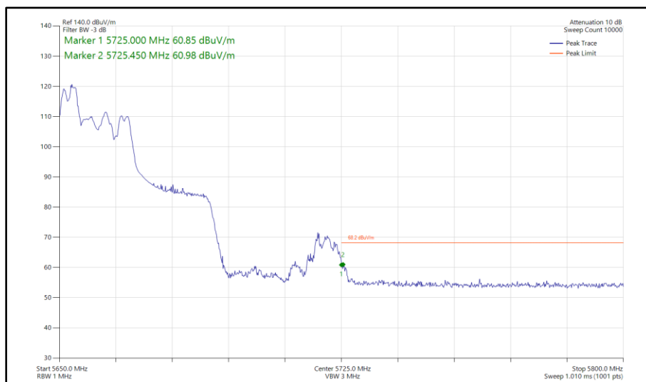
Figure 543 - 802.11ax HE40, RU 52-37, SDM, Core 0 - Core 1 - 5670 MHz Band Edge Frequency 5725 MHz
