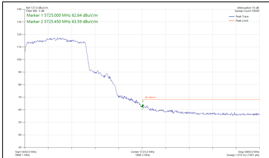
Figure 542 - 802.11ax HE40, SU, SDM, Core 0 - Core 1 - 5670 MHz Band Edge Frequency 5725 MHz
