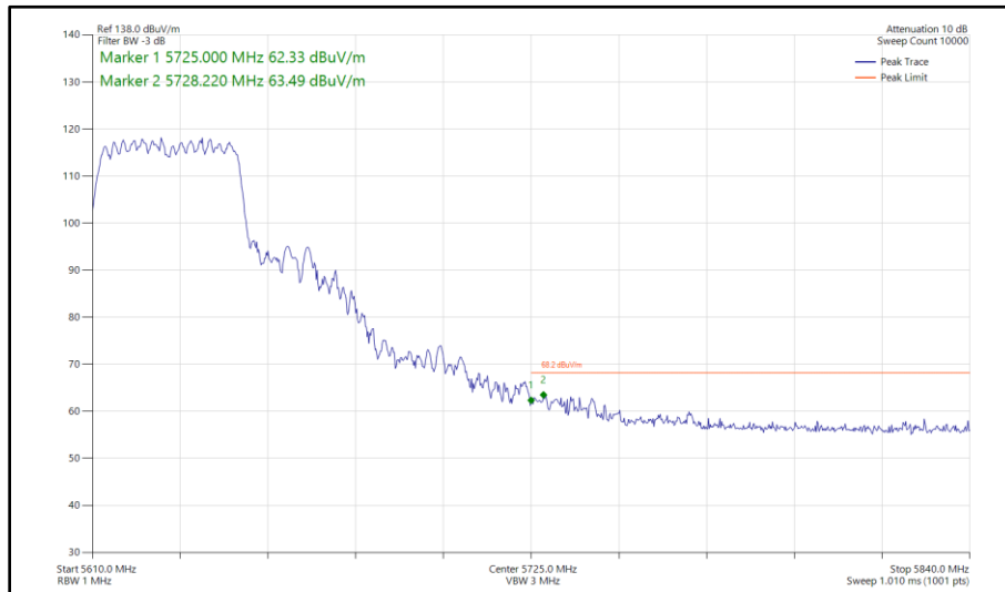
Figure 518 - 802.11n HT40, CDD, Core 0 - Core 1 - 5630 MHz Band Edge Frequency 5725 MHz
