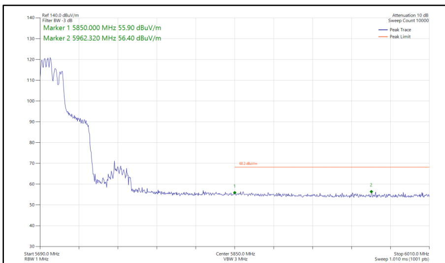
Figure 547 - 802.11ax HE40, RU 106-53, SDM, Core 0 - Core 1 - 5710 MHz Band Edge Frequency 5850 MHz
