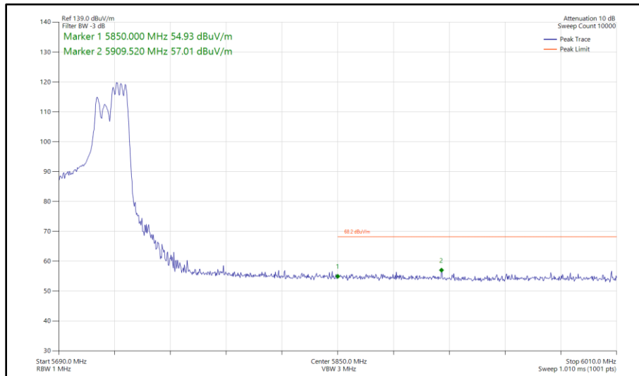
Figure 526 - 802.11ax HE40, RU 106-56, CDD, Core 0 - Core 1 - 5710 MHz Band Edge Frequency 5850 MHz
