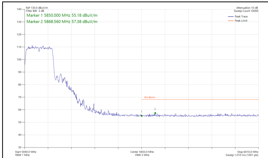
Figure 555 - 802.11ac VHT40, TxBF, Core 0 - Core 1 - 5710 MHz Band Edge Frequency 5850 MHz
