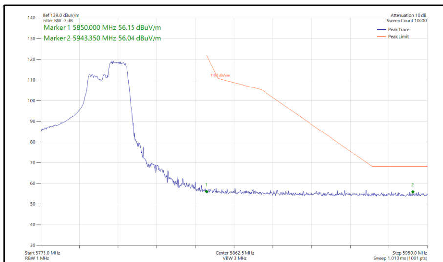
Figure 508 - 802.11ax HE40, RU 106-56, SISO, Core 1 - 5795 MHz Band Edge Frequency 5850 MHz
