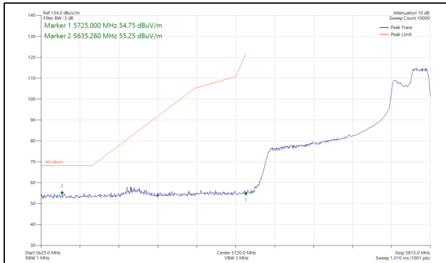
Figure 562 - 802.11ax HE80, RU 106-60, SISO, Core 0 - 5775 MHz Band Edge Frequency 5725 MHz
