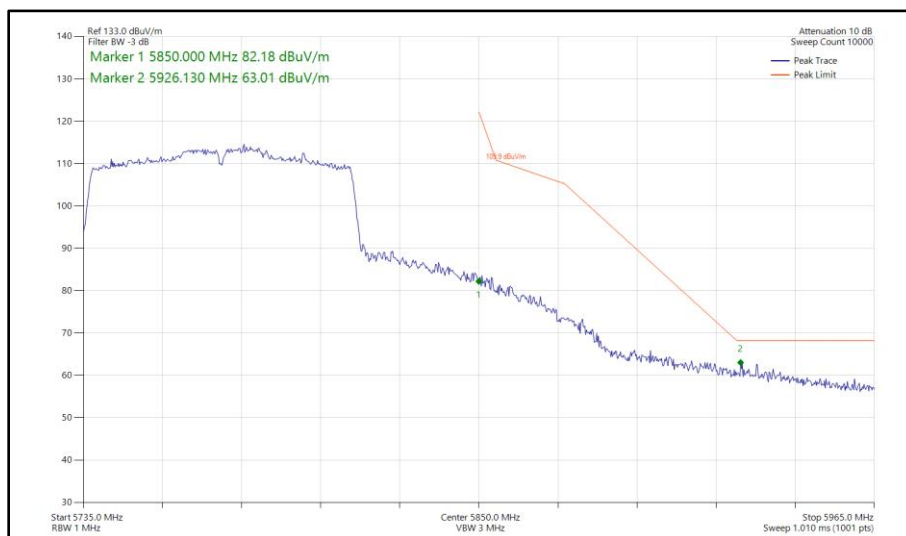
Figure 567 - 802.11ac VHT80, SISO, Core 0 - 5775 MHz Band Edge Frequency 5850 MHz
