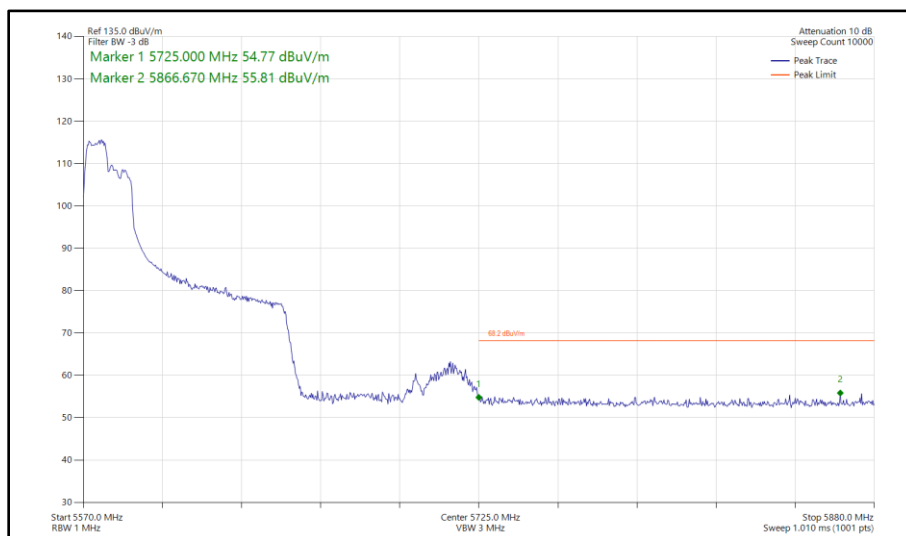
Figure 580 - 802.11ax HE80, RU 106-53, SISO, Core 1 - 5610 MHz Band Edge Frequency 5725 MHz
