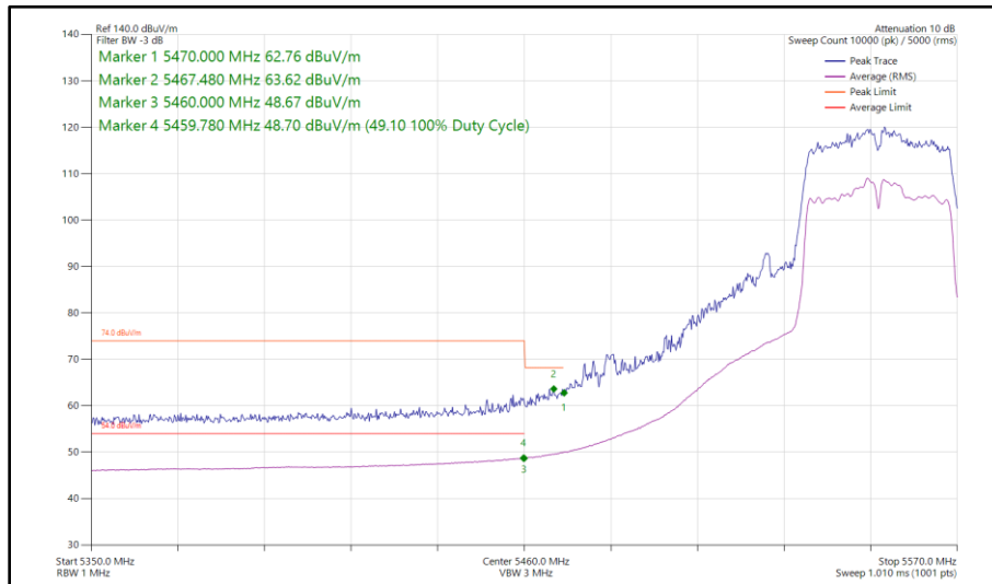
Figure 551 - 802.11ac VHT40, TxBF, Core 0 - Core 1 - 5550 MHz Band Edge Frequency 5470 MHz
