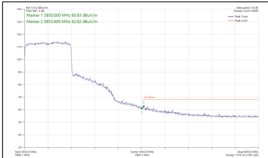
Figure 583 - 802.11ax HE80, SU, SISO, Core 1 - 5690 MHz Band Edge Frequency 5850 MHz
