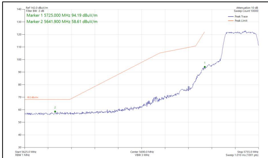
Figure 441 - 802.11n HT20, SDM, Core 0 - Core 1 - 5745 MHz Band Edge Frequency 5725 MHz
