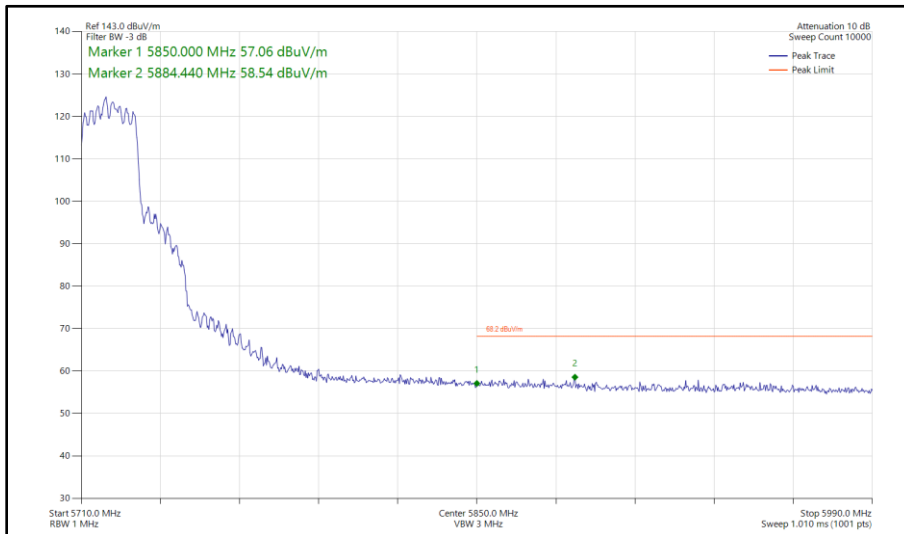
Figure 430 - 802.11ax HE20, SU, CDD, Core 0 - Core 1 - 5720 MHz Band Edge Frequency 5850 MHz
