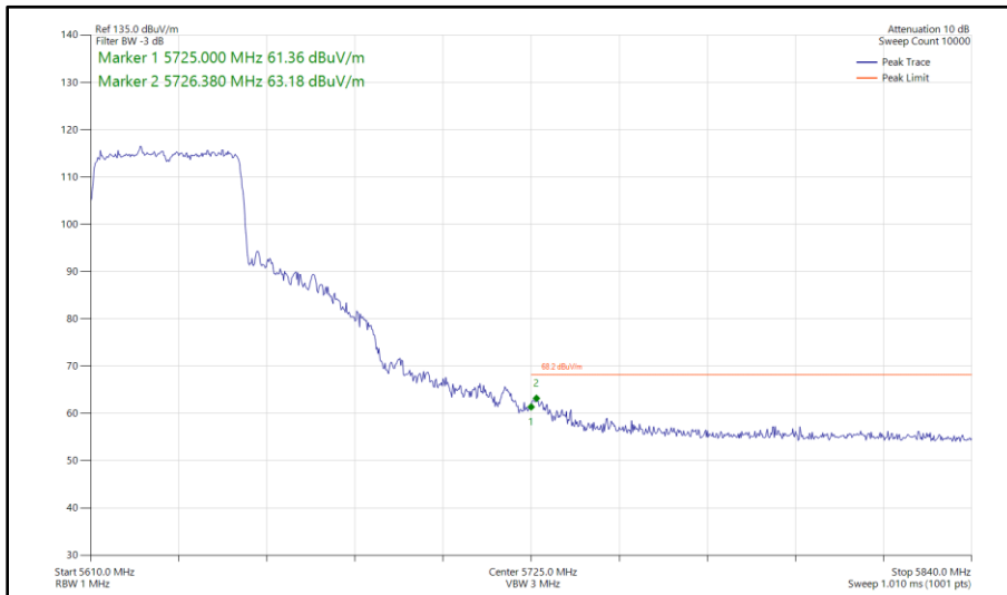
Figure 499 - 802.11ax HE40, SU, SISO, Core 1 - 5630 MHz Band Edge Frequency 5725 MHz
