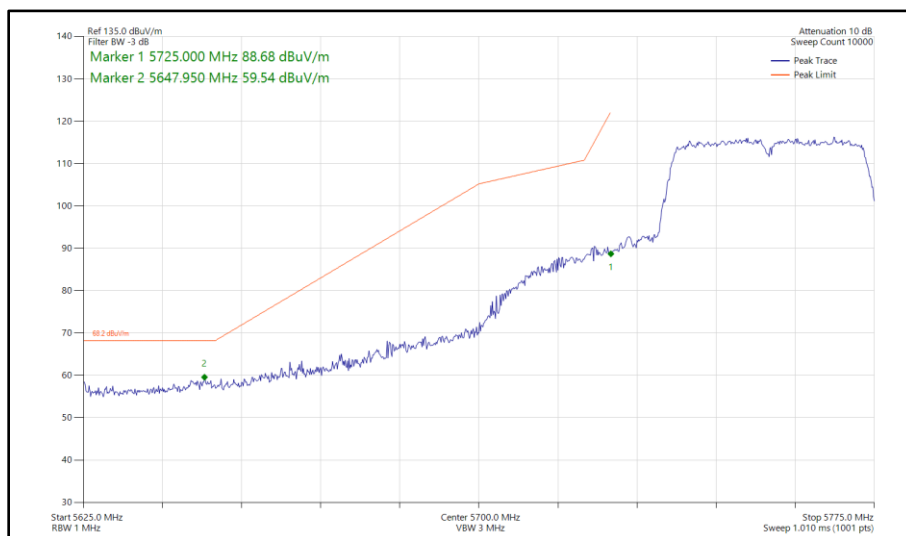
Figure 473 - 802.11n HT40, SISO, Core 0 - 5755 MHz Band Edge Frequency 5725 MHz
