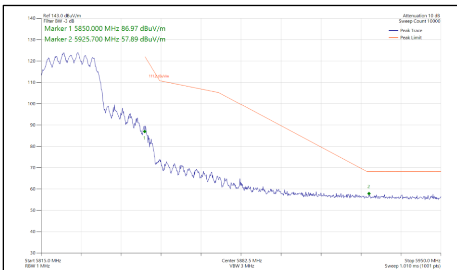
Figure 433 - 802.11ax HE20, SU, CDD, Core 0 - Core 1 - 5825 MHz Band Edge Frequency 5850 MHz
