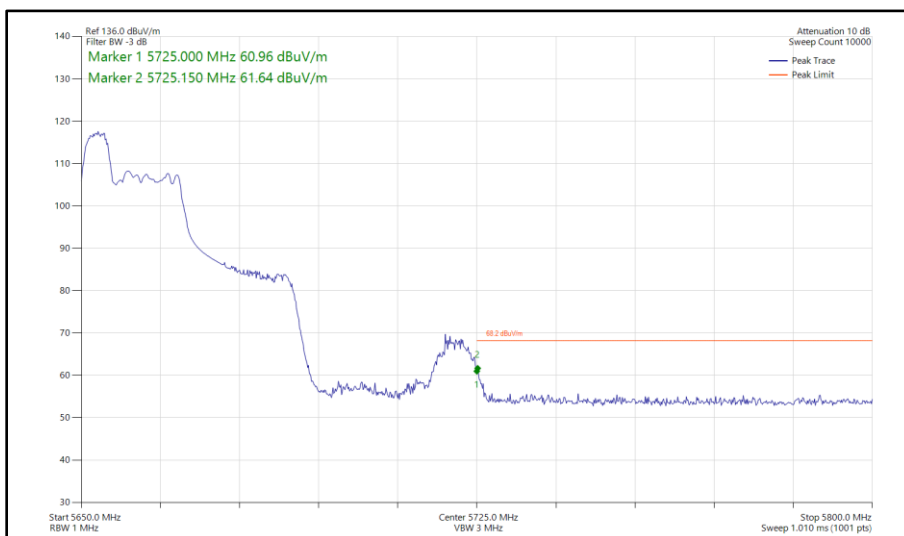
Figure 502 - 802.11ax HE40, RU 52-37, SISO, Core 1 - 5670 MHz Band Edge Frequency 5725 MHz
