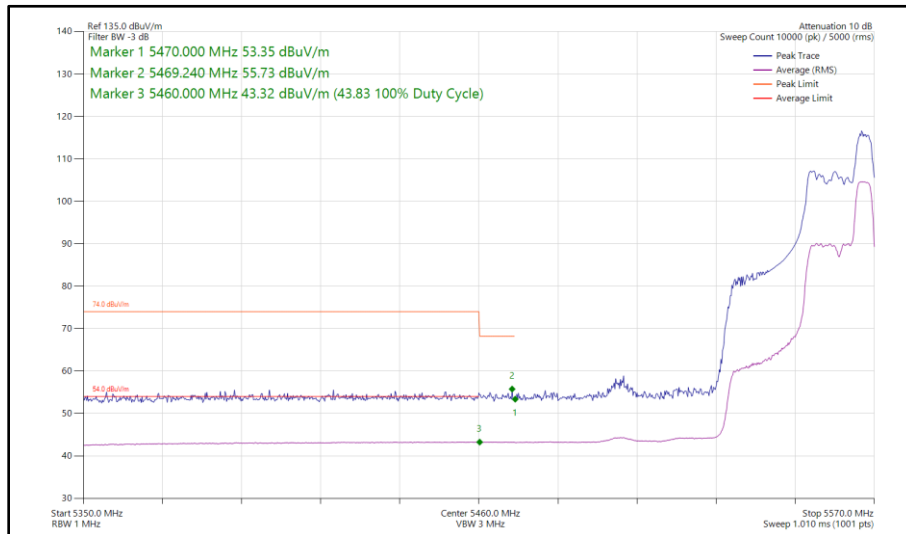
Figure 493 - 802.11ax HE40, RU 52-44, SISO, Core 1 - 5550 MHz Band Edge Frequency 5470 MHz
