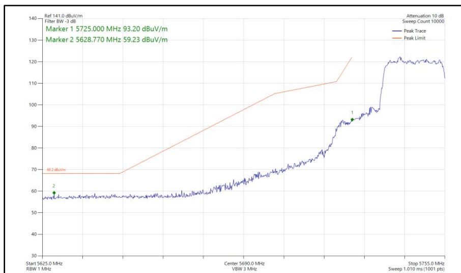
Figure 442 - 802.11ax HE20, SU, SDM, Core 0 - Core 1 - 5745 MHz Band Edge Frequency 5725 MHz
