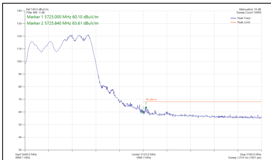
Figure 450 - 802.11ax HE20, RU 106-54, SDM, Core 0 - Core 1 - 5700 MHz Band Edge Frequency 5725 MHz
