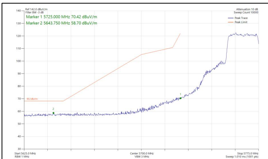
Figure 444 - 802.11ax HE20, SU, SDM, Core 0 - Core 1 - 5765 MHz Band Edge Frequency 5725 MHz
