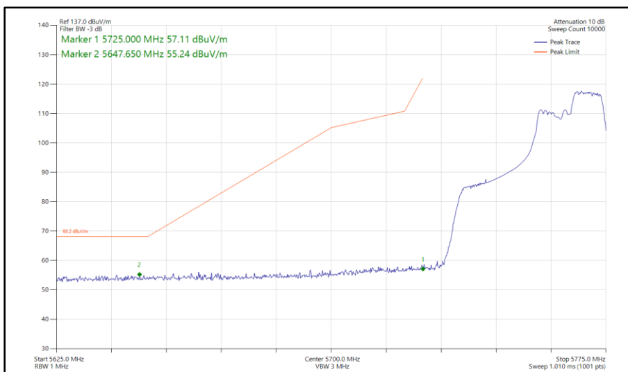
Figure 475 - 802.11ax HE40, RU 106-56, SISO, Core 0 - 5755 MHz Band Edge Frequency 5725 MHz
