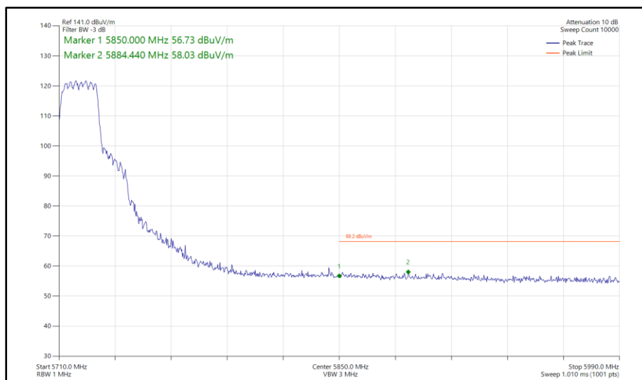
Figure 427 - 802.11n HT20, CDD, Core 0 - Core 1 - 5720 MHz Band Edge Frequency 5850 MHz
