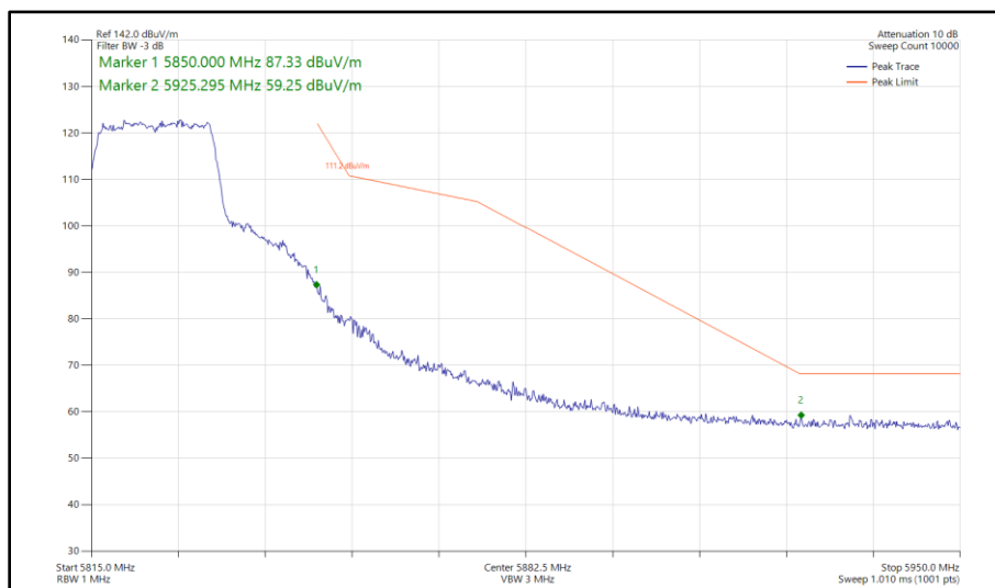
Figure 452 - 802.11n HT20, SDM, Core 0 - Core 1 - 5825 MHz Band Edge Frequency 5850 MHz
