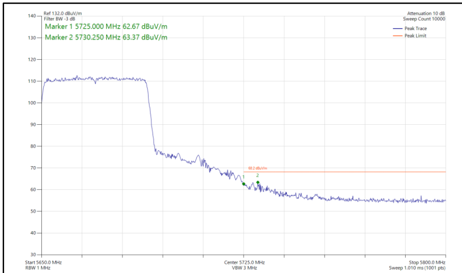
Figure 501 - 802.11ax HE40, SU, SISO, Core 1 - 5670 MHz Band Edge Frequency 5725 MHz
