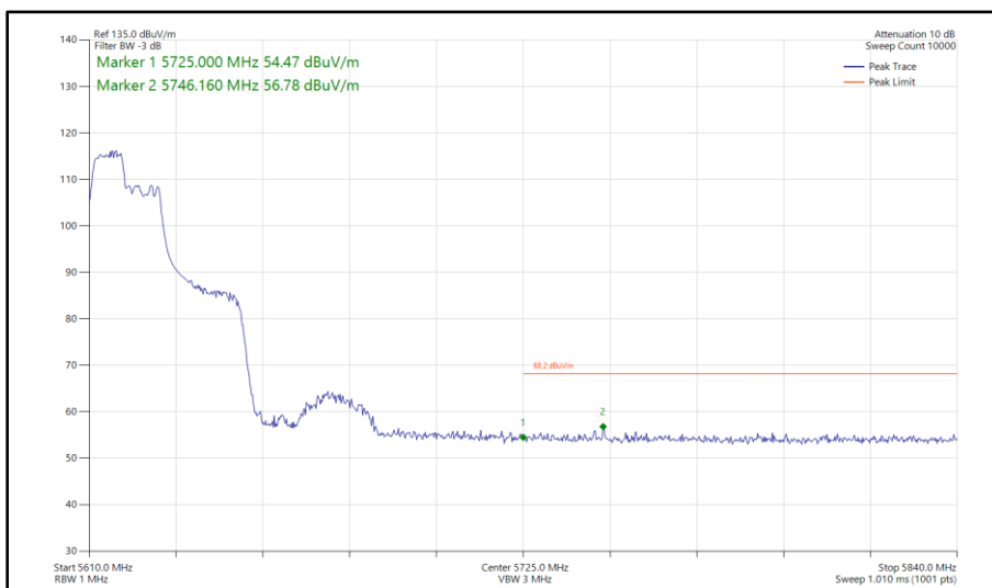
Figure 500 - 802.11ax HE40, RU 106-53, SISO, Core 1 - 5630 MHz Band Edge Frequency 5725 MHz
