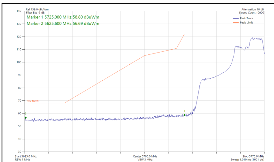
Figure 496 - 802.11ax HE40, RU 106-56, SISO, Core 1 - 5755 MHz Band Edge Frequency 5725 MHz
