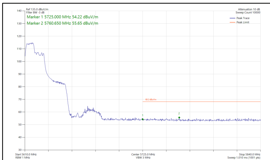
Figure 479 - 802.11ax HE40, RU 106-53, SISO, Core 0 - 5630 MHz Band Edge Frequency 5725 MHz
