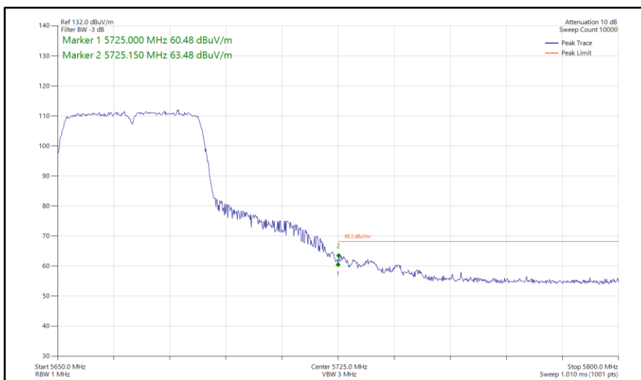
Figure 498 - 802.11n HT40, SISO, Core 1 - 5670 MHz Band Edge Frequency 5725 MHz
