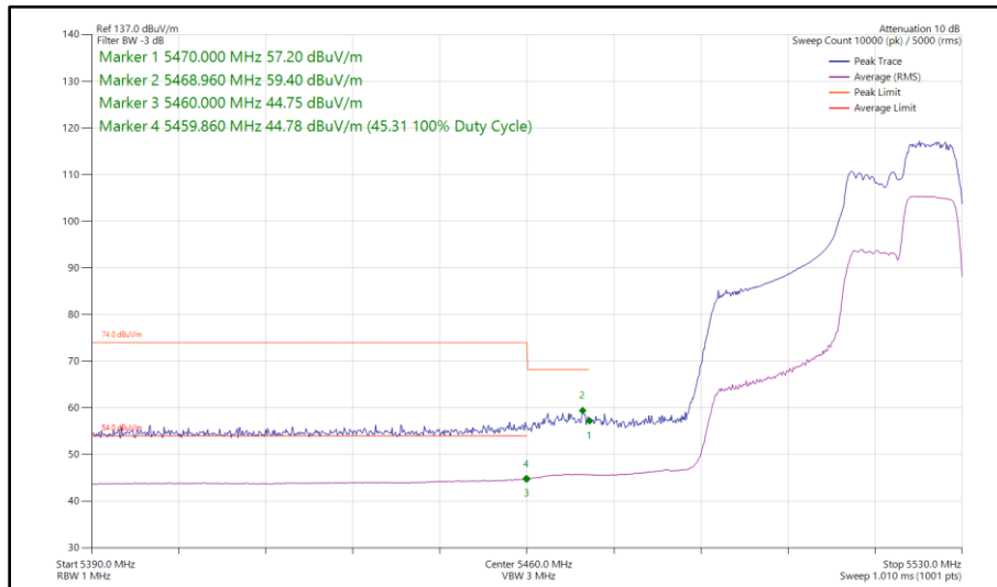
Figure 491 - 802.11ax HE40, RU 106-56, SISO, Core 1 - 5510 MHz Band Edge Frequency 5470 MHz
