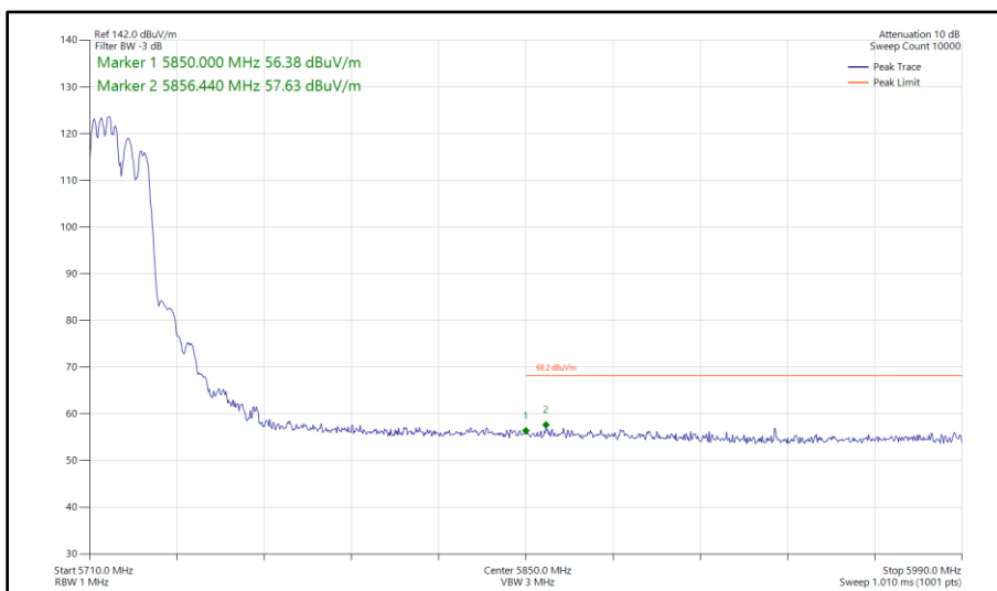
Figure 431 - 802.11ax HE20, RU 106-53, CDD, Core 0 - Core 1 - 5720 MHz Band Edge Frequency 5850 MHz
