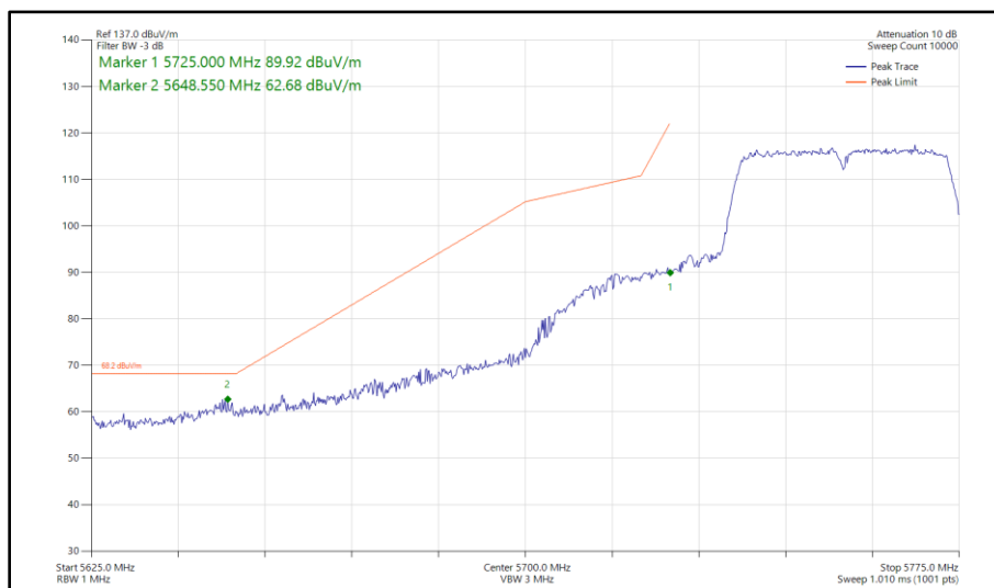
Figure 494 - 802.11n HT40, SISO, Core 1 - 5755 MHz Band Edge Frequency 5725 MHz
