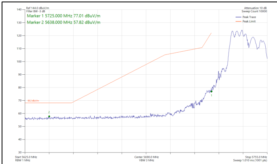
Figure 443 - 802.11ax HE20, RU 106-53, SDM, Core 0 - Core 1 - 5745 MHz Band Edge Frequency 5725 MHz
