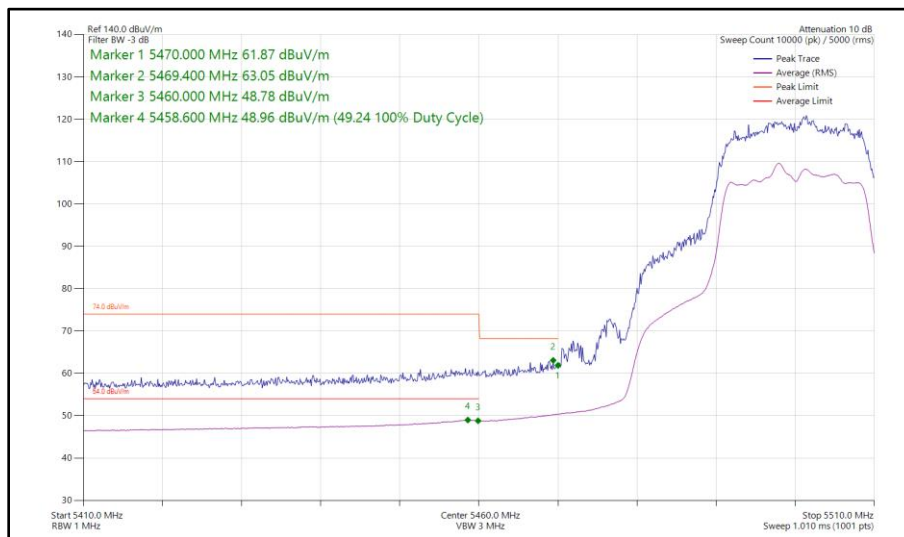
Figure 458 - 802.11ac VHT20, TxBF, Core 0 - Core 1 - 5500 MHz Band Edge Frequency 5470 MHz
