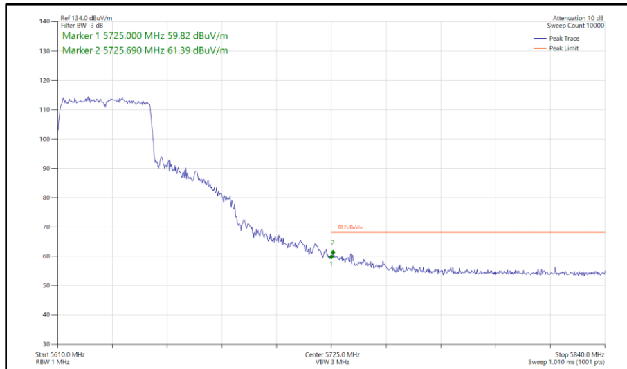
Figure 478 - 802.11ax HE40, SU, SISO, Core 0 - 5630 MHz Band Edge Frequency 5725 MHz
