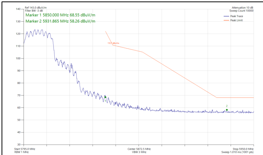
Figure 432 - 802.11ax HE20, SU, CDD, Core 0 - Core 1 - 5805 MHz Band Edge Frequency 5850 MHz
