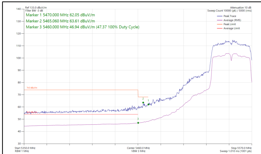
Figure 468 - 802.11n HT40, SISO, Core 0 - 5550 MHz Band Edge Frequency 5470 MHz
