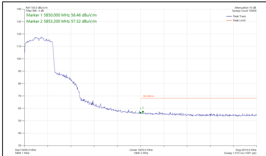
Figure 484 - 802.11ax HE40, SU, SISO, Core 0 - 5710 MHz Band Edge Frequency 5850 MHz
