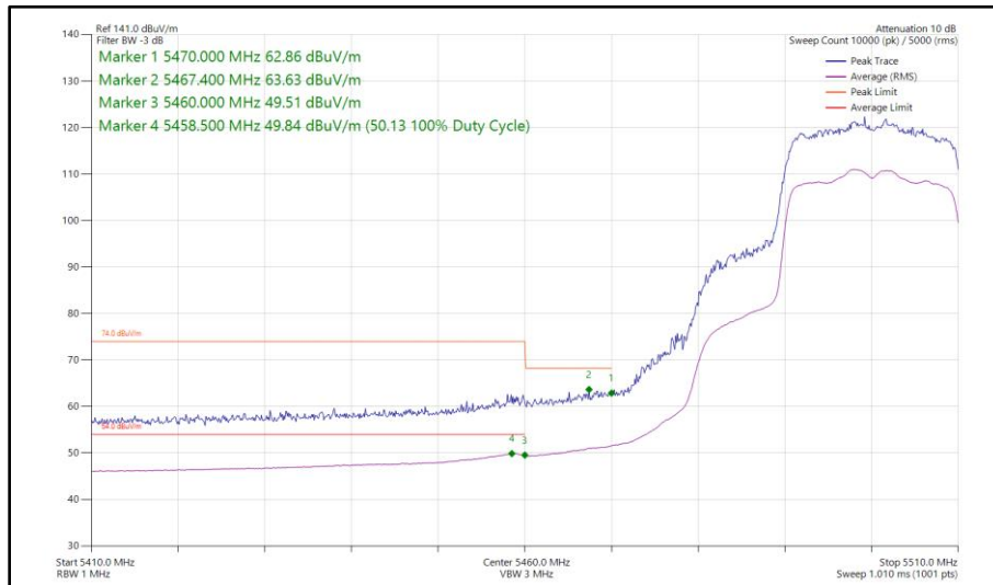
Figure 437 - 802.11ax HE20, SU, SDM, Core 0 - Core 1 - 5500 MHz Band Edge Frequency 5470 MHz
