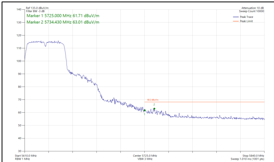
Figure 497 - 802.11n HT40, SISO, Core 1 - 5630 MHz Band Edge Frequency 5725 MHz
