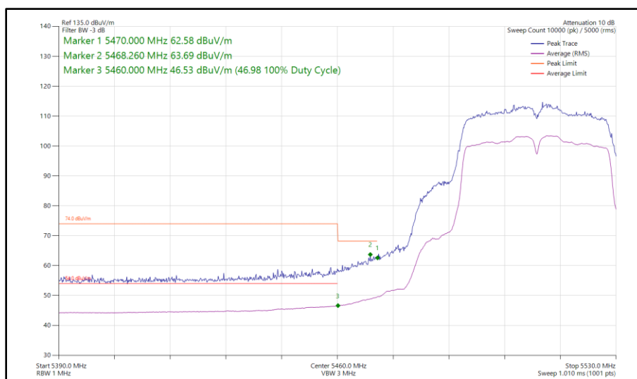
Figure 488 - 802.11n HT40, SISO, Core 1 - 5510 MHz Band Edge Frequency 5470 MHz
