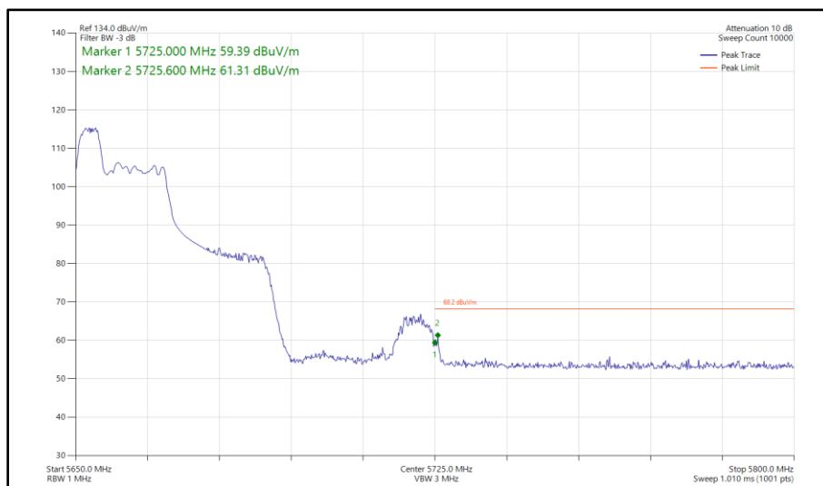
Figure 481 - 802.11ax HE40, RU 52-37, SISO, Core 0 - 5670 MHz Band Edge Frequency 5725 MHz
