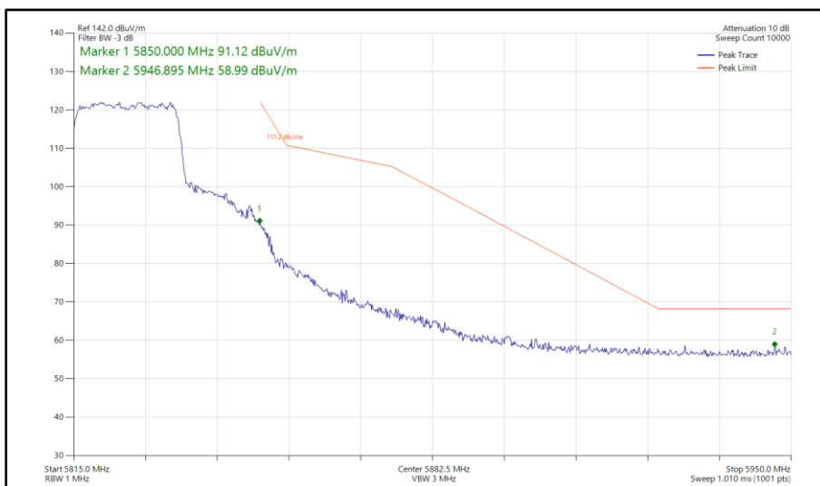
Figure 456 - 802.11ax HE20, SU, SDM, Core 0 - Core 1 - 5825 MHz Band Edge Frequency 5850 MHz
