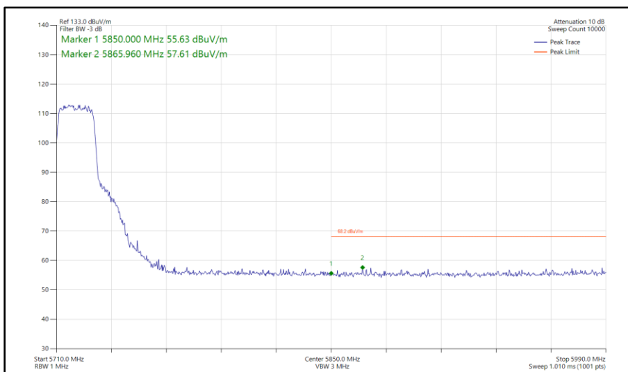
Figure 464 - 802.11ac VHT20, TxBF, Core 0 - Core 1 - 5720 MHz Band Edge Frequency 5850 MHz
