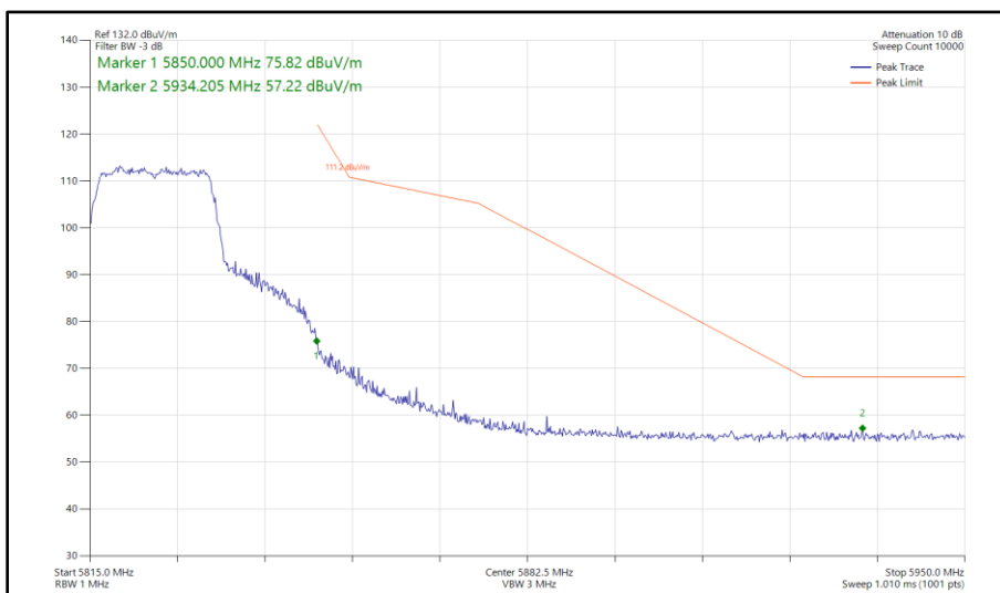
Figure 466 - 802.11ac VHT20, TxBF, Core 0 - Core 1 - 5825 MHz Band Edge Frequency 5850 MHz
