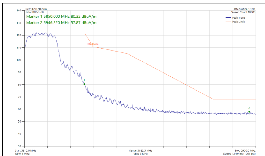
Figure 429 - 802.11n HT20, CDD, Core 0 - Core 1 - 5825 MHz Band Edge Frequency 5850 MHz
