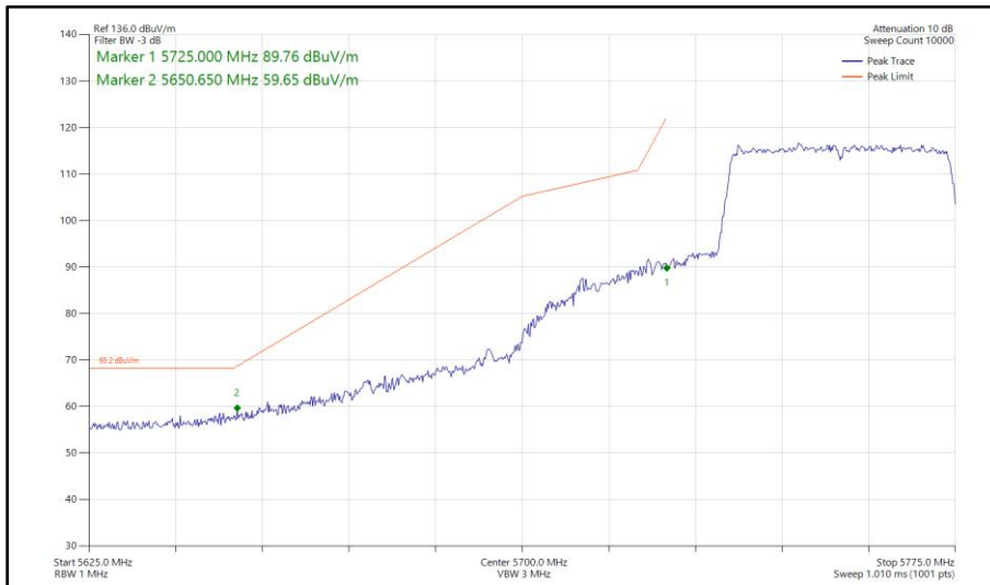
Figure 474 - 802.11ax HE40, SU, SISO, Core 0 - 5755 MHz Band Edge Frequency 5725 MHz
