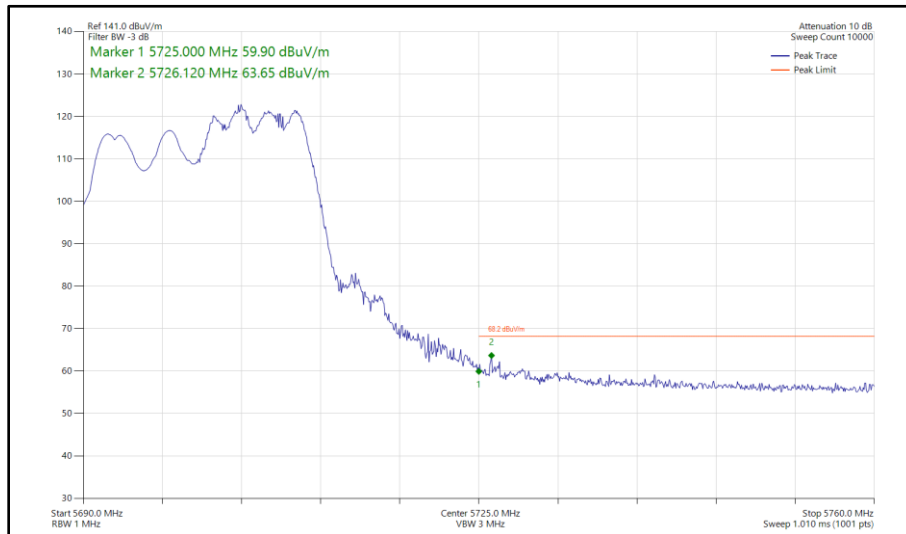
Figure 426 - 802.11ax HE20, RU 106-54, CDD, Core 0 - Core 1 - 5700 MHz Band Edge Frequency 5725 MHz
