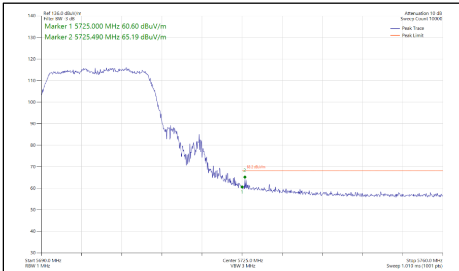
Figure 463 - 802.11ac VHT20, TxBF, Core 0 - Core 1 - 5700 MHz Band Edge Frequency 5725 MHz
