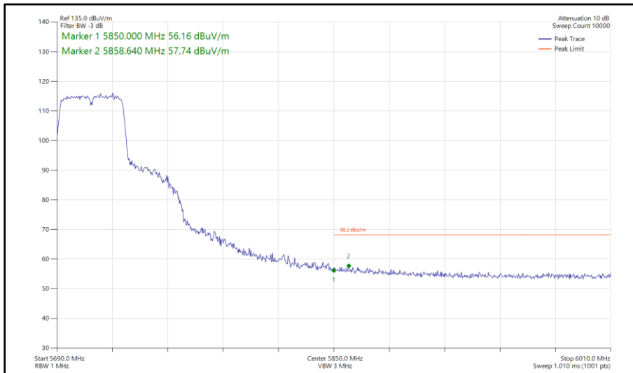
Figure 482 - 802.11n HT40, SISO, Core 0 - 5710 MHz Band Edge Frequency 5850 MHz
