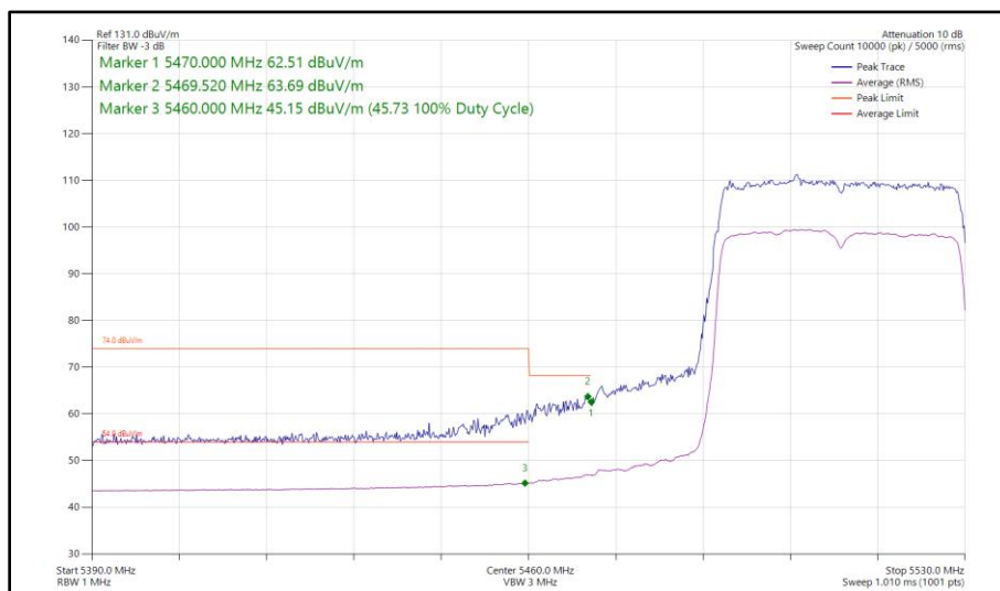
Figure 490 - 802.11ax HE40, SU, SISO, Core 1 - 5510 MHz Band Edge Frequency 5470 MHz
