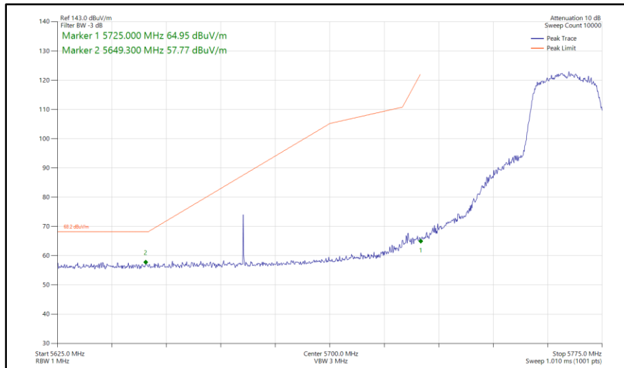
Figure 461 - 802.11ac VHT20, TxBF, Core 0 - Core 1 - 5765 MHz Band Edge Frequency 5725 MHz
