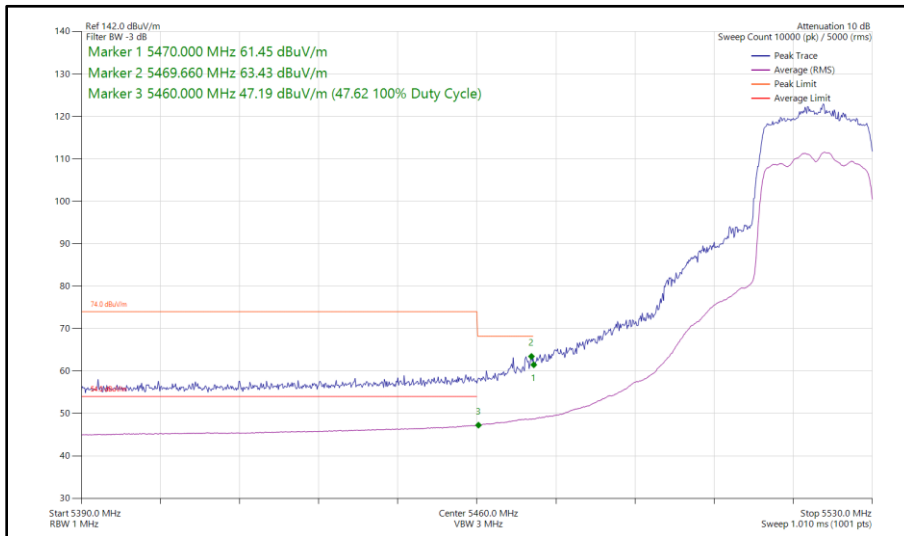
Figure 439 - 802.11ax HE20, SU, SDM, Core 0 - Core 1 - 5520 MHz Band Edge Frequency 5470 MHz
