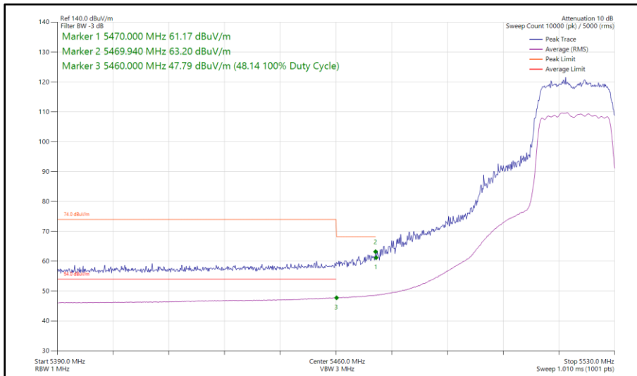
Figure 459 - 802.11ac VHT20, TxBF, Core 0 - Core 1 - 5520 MHz Band Edge Frequency 5470 MHz
