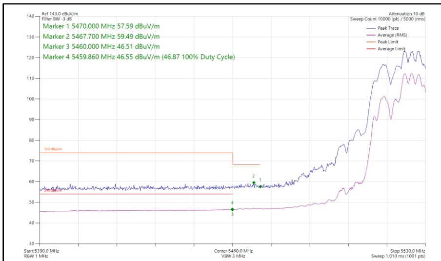
Figure 440 - 802.11ax HE20, RU 106-54, SDM, Core 0 - Core 1 - 5520 MHz Band Edge Frequency 5470 MHz
