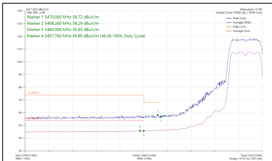
Figure 436 - 802.11n HT20, SDM, Core 0 - Core 1 - 5520 MHz Band Edge Frequency 5470 MHz
