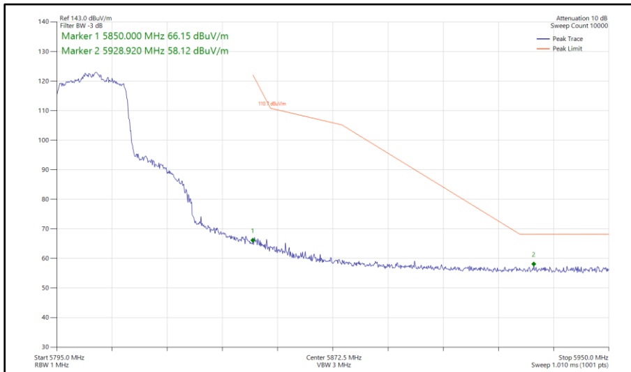
Figure 455 - 802.11ax HE20, SU, SDM, Core 0 - Core 1 - 5805 MHz Band Edge Frequency 5850 MHz
