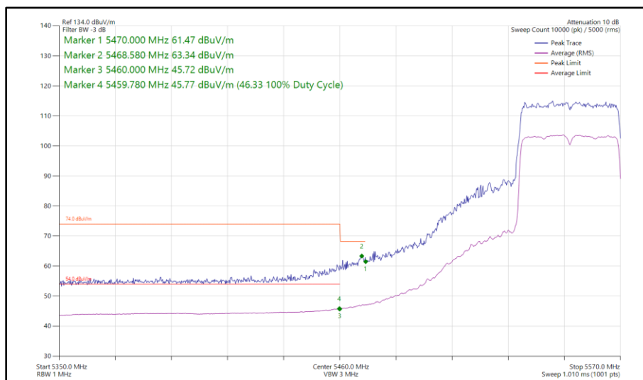
Figure 492 - 802.11ax HE40, SU, SISO, Core 1 - 5550 MHz Band Edge Frequency 5470 MHz
