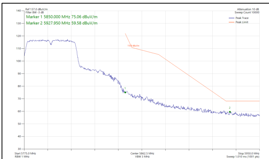
Figure 504 - 802.11n HT40, SISO, Core 1 - 5795 MHz Band Edge Frequency 5850 MHz
