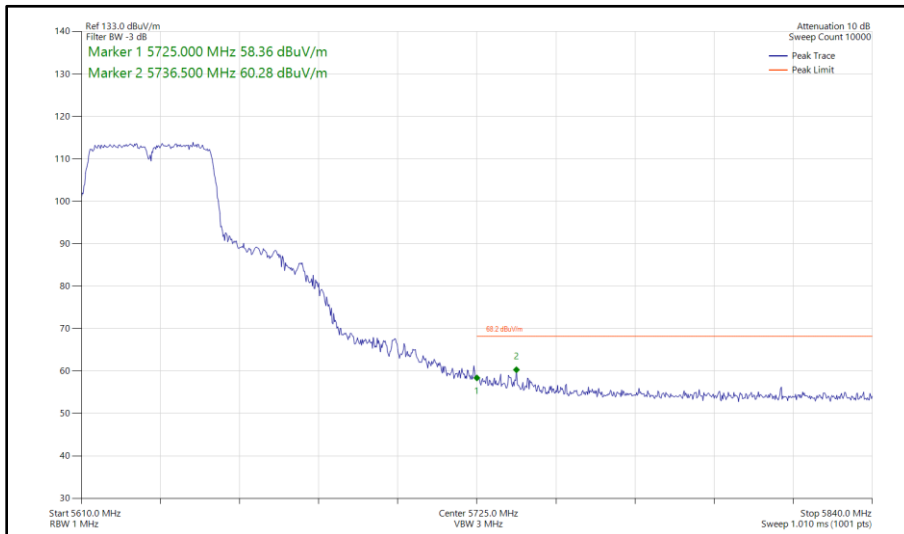
Figure 476 - 802.11n HT40, SISO, Core 0 - 5630 MHz Band Edge Frequency 5725 MHz
