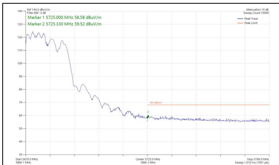
Figure 448 - 802.11ax HE20, RU 106-53, SDM, Core 0 - Core 1 - 5680 MHz Band Edge Frequency 5725 MHz
