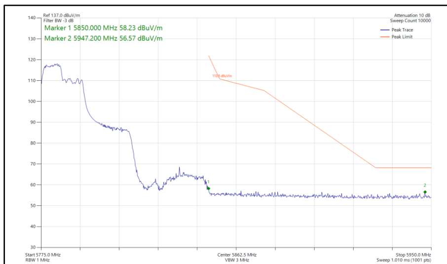
Figure 487 - 802.11ax HE40, RU 106-53, SISO, Core 0 - 5795 MHz Band Edge Frequency 5850 MHz
