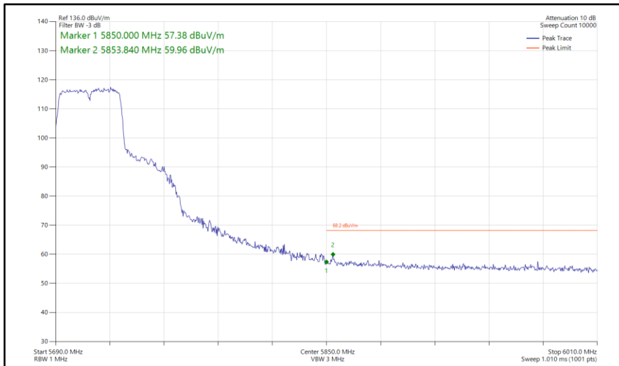
Figure 503 - 802.11n HT40, SISO, Core 1 - 5710 MHz Band Edge Frequency 5850 MHz
