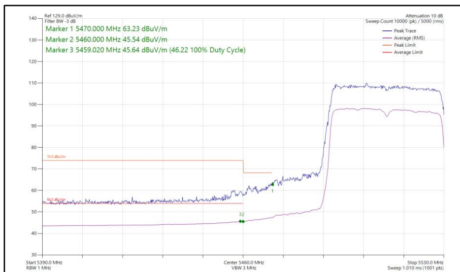
Figure 469 - 802.11ax HE40, SU, SISO, Core 0 - 5510 MHz Band Edge Frequency 5470 MHz
