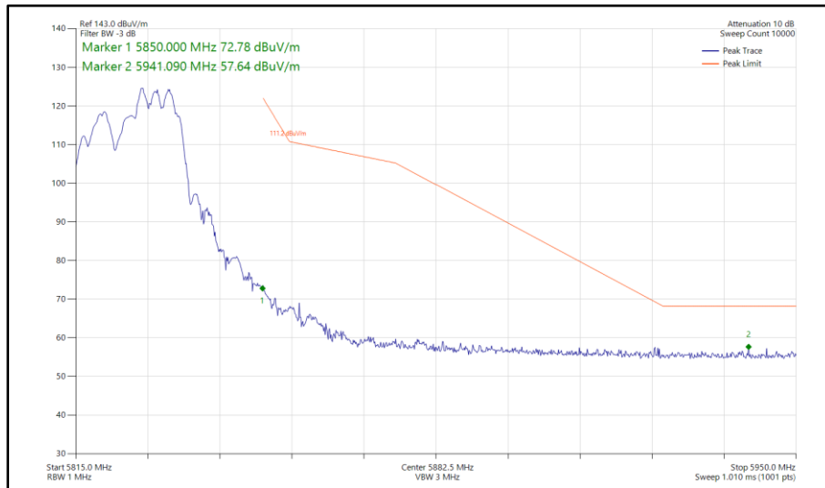
Figure 434 - 802.11ax HE20, RU 106-54, CDD, Core 0 - Core 1 - 5825 MHz Band Edge Frequency 5850 MHz
