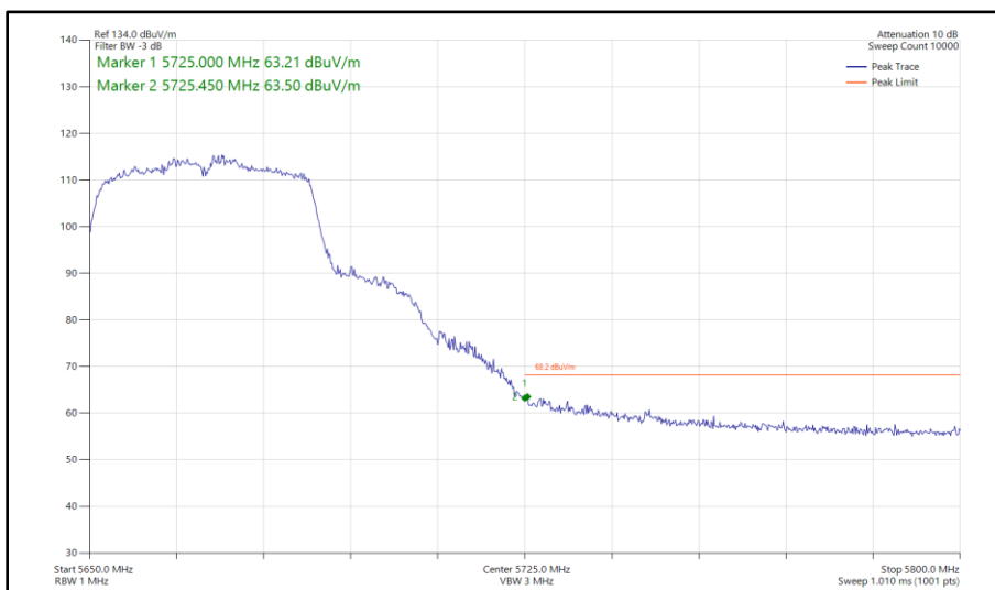
Figure 477 - 802.11n HT40, SISO, Core 0 - 5670 MHz Band Edge Frequency 5725 MHz
