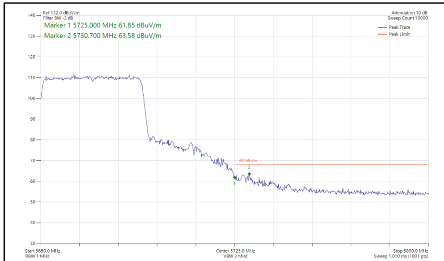
Figure 480 - 802.11ax HE40, SU, SISO, Core 0 - 5670 MHz Band Edge Frequency 5725 MHz
