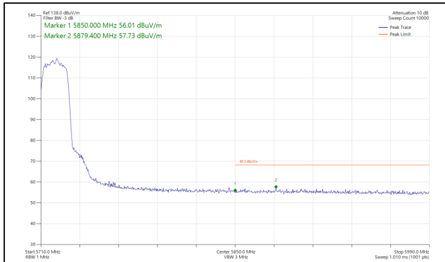
Figure 451 - 802.11n HT20, SDM, Core 0 - Core 1 - 5720 MHz Band Edge Frequency 5850 MHz
