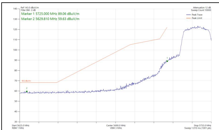
Figure 460 - 802.11ac VHT20, TxBF, Core 0 - Core 1 - 5745 MHz Band Edge Frequency 5725 MHz
