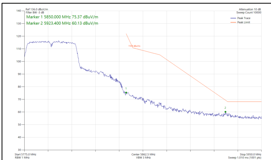
Figure 483 - 802.11n HT40, SISO, Core 0 - 5795 MHz Band Edge Frequency 5850 MHz
