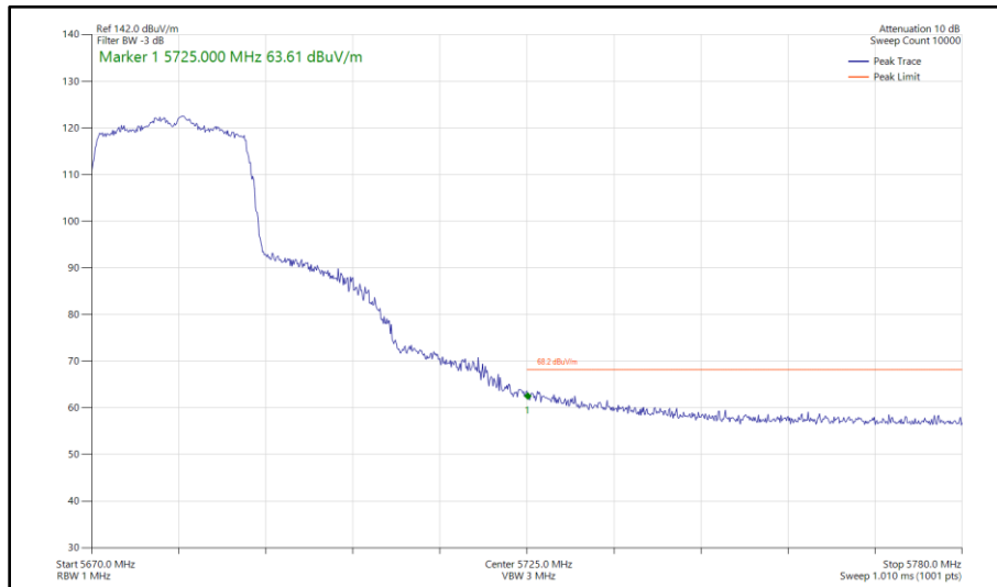
Figure 447 - 802.11ax HE20, SU, SDM, Core 0 - Core 1 - 5680 MHz Band Edge Frequency 5725 MHz
