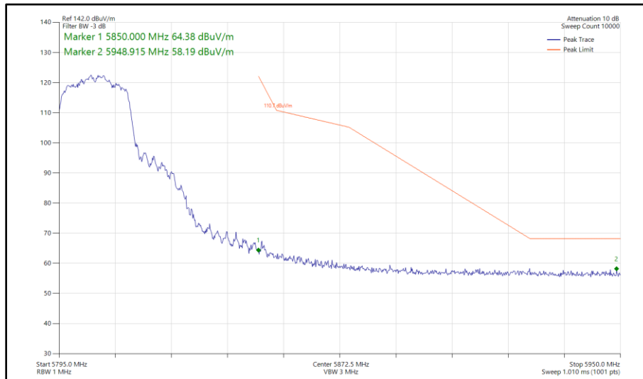
Figure 428 - 802.11n HT20, CDD, Core 0 - Core 1 - 5805 MHz Band Edge Frequency 5850 MHz
