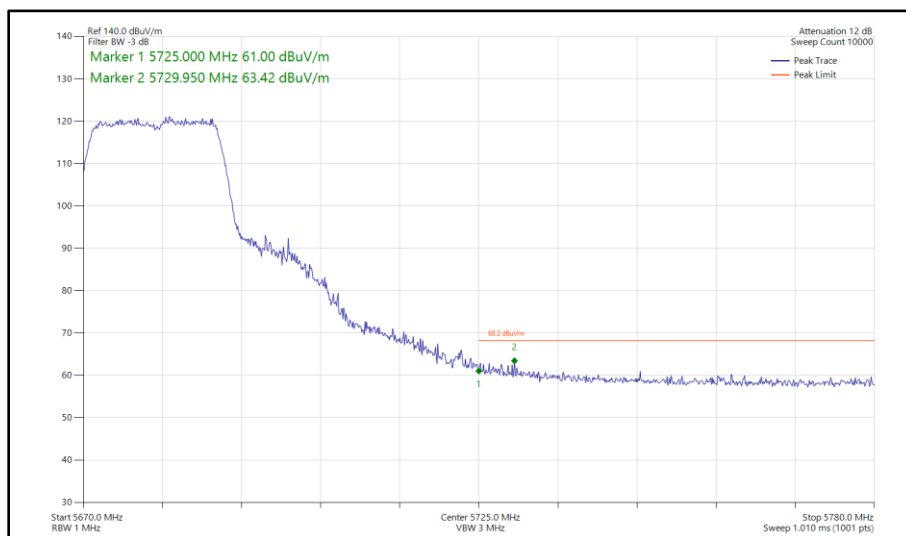
Figure 462 - 802.11ac VHT20, TxBF, Core 0 - Core 1 - 5680 MHz Band Edge Frequency 5725 MHz
