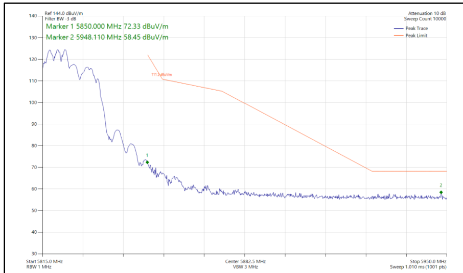
Figure 457 - 802.11ax HE20, RU 106-53, SDM, Core 0 - Core 1 - 5825 MHz Band Edge Frequency 5850 MHz
