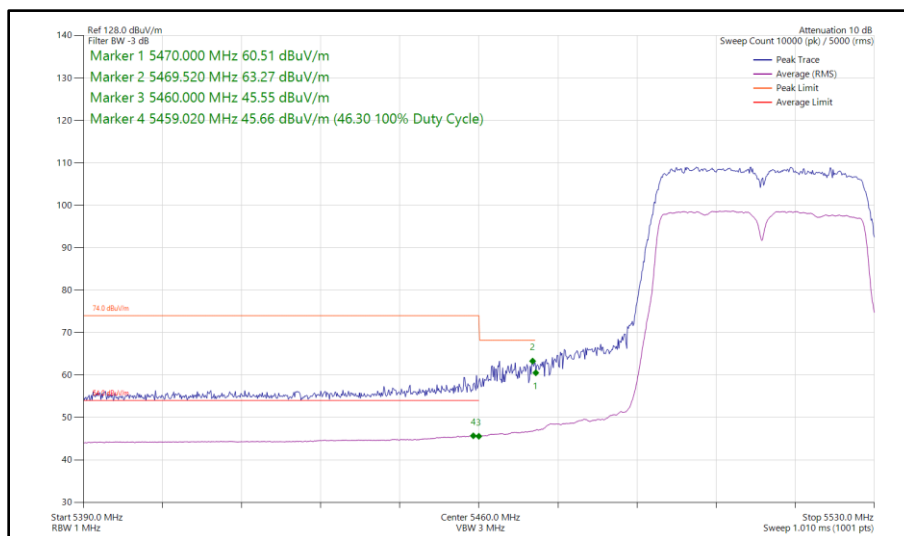
Figure 467 - 802.11n HT40, SISO, Core 0 - 5510 MHz Band Edge Frequency 5470 MHz
