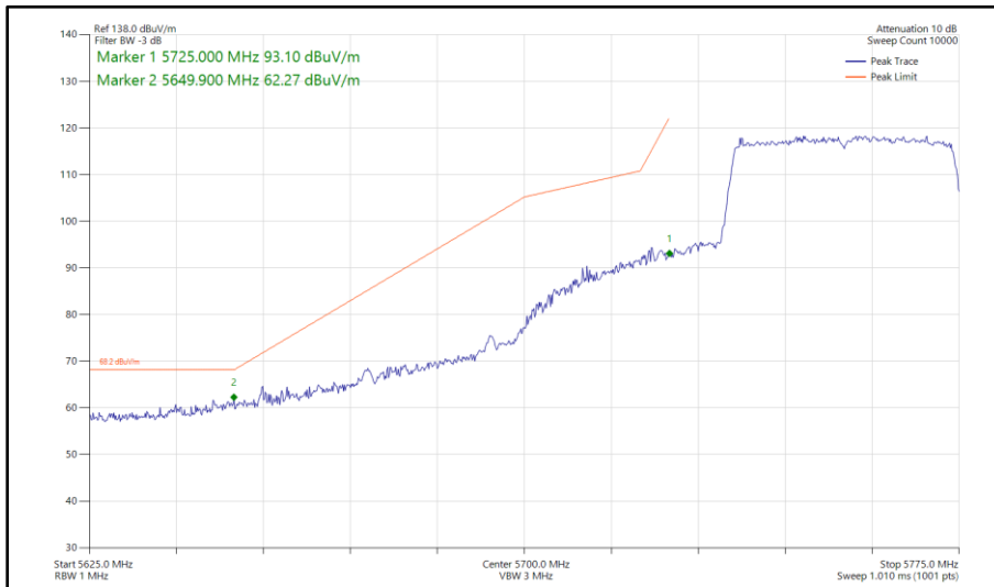
Figure 495 - 802.11ax HE40, SU, SISO, Core 1 - 5755 MHz Band Edge Frequency 5725 MHz
