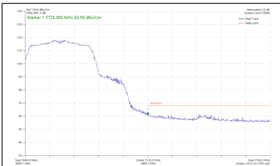
Figure 446 - 802.11n HT20, SDM, Core 0 - Core 1 - 5700 MHz Band Edge Frequency 5725 MHz
