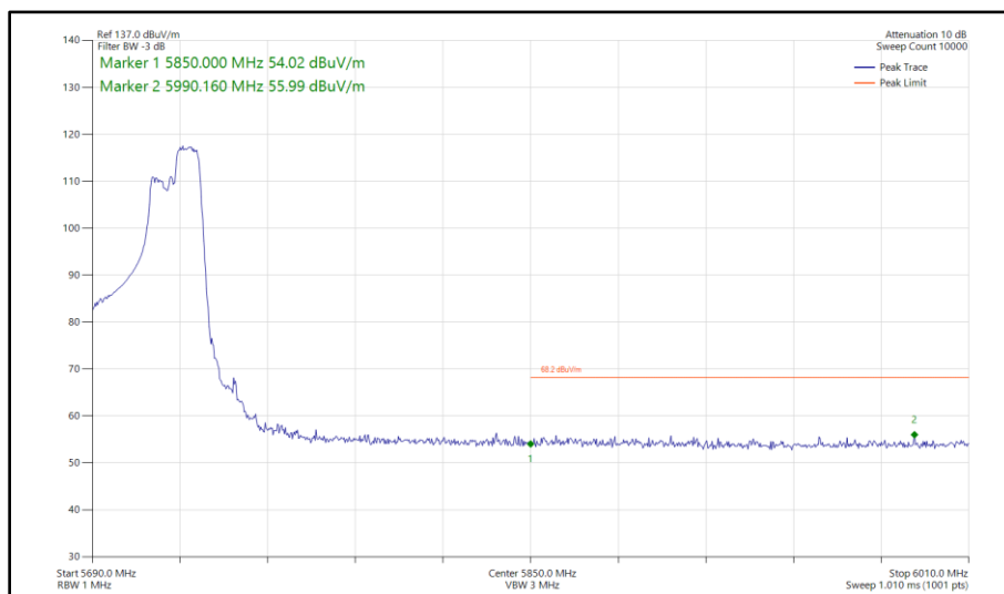
Figure 485 - 802.11ax HE40, RU 106-56, SISO, Core 0 - 5710 MHz Band Edge Frequency 5850 MHz
