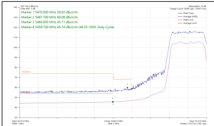
Figure 435 - 802.11n HT20, SDM, Core 0 - Core 1 - 5500 MHz Band Edge Frequency 5470 MHz
