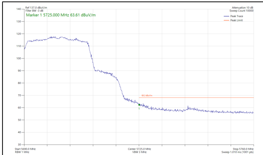
Figure 449 - 802.11ax HE20, SU, SDM, Core 0 - Core 1 - 5700 MHz Band Edge Frequency 5725 MHz
