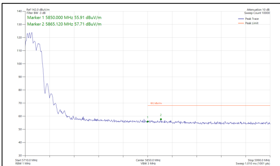
Figure 454 - 802.11ax HE20, RU 106-53, SDM, Core 0 - Core 1 - 5720 MHz Band Edge Frequency 5850 MHz
