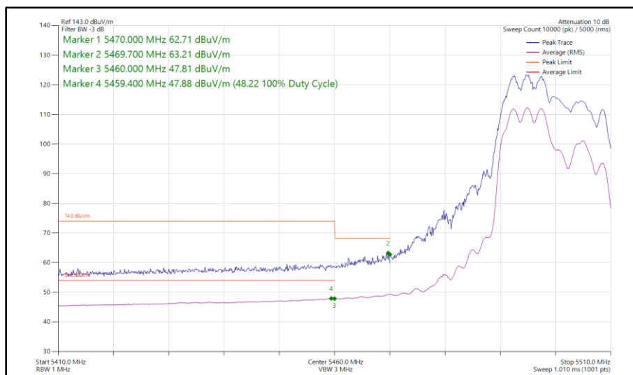
Figure 438 - 802.11ax HE20, RU 106-53, SDM, Core 0 - Core 1 - 5500 MHz Band Edge Frequency 5470 MHz
