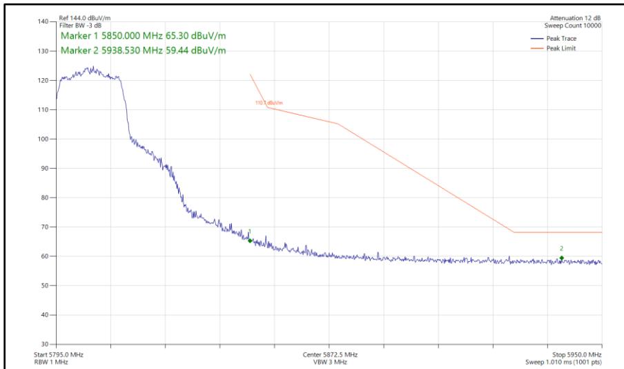
Figure 465 - 802.11ac VHT20, TxBF, Core 0 - Core 1 - 5805 MHz Band Edge Frequency 5850 MHz
