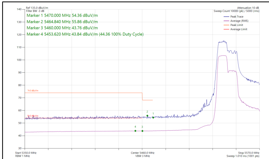
Figure 472 - 802.11ax HE40, RU 106-53, SISO, Core 0 - 5550 MHz Band Edge Frequency 5470 MHz
