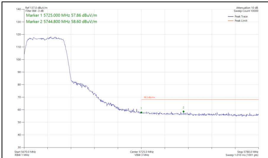
Figure 445 - 802.11n HT20, SDM, Core 0 - Core 1 - 5680 MHz Band Edge Frequency 5725 MHz
