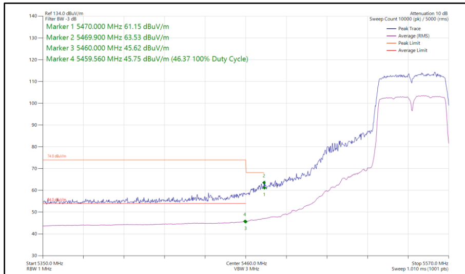
Figure 489 - 802.11n HT40, SISO, Core 1 - 5550 MHz Band Edge Frequency 5470 MHz
