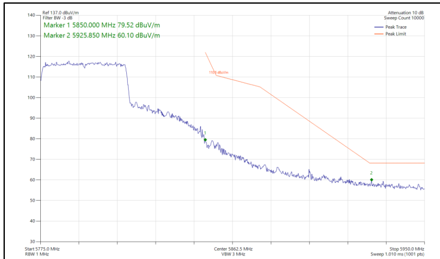
Figure 486 - 802.11ax HE40, SU, SISO, Core 0 - 5795 MHz Band Edge Frequency 5850 MHz
