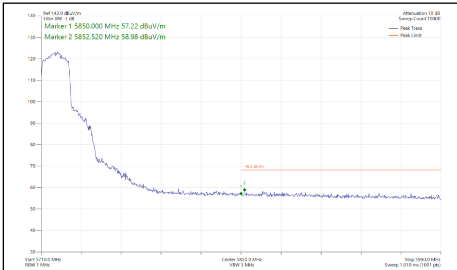
Figure 453 - 802.11ax HE20, SU, SDM, Core 0 - Core 1 - 5720 MHz Band Edge Frequency 5850 MHz
