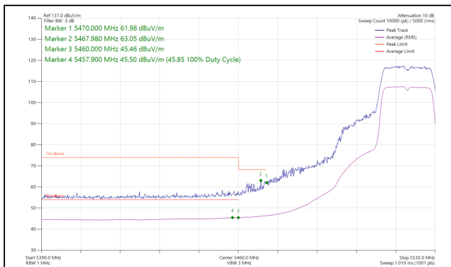
Figure 379 - 802.11n HT20, SISO, Core 1 - 5520 MHz Band Edge Frequency 5470 MHz
