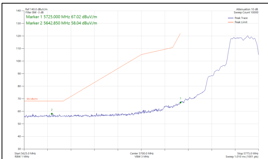
Figure 385 - 802.11a, SISO, Core 1 - 5765 MHz Band Edge Frequency 5725 MHz
