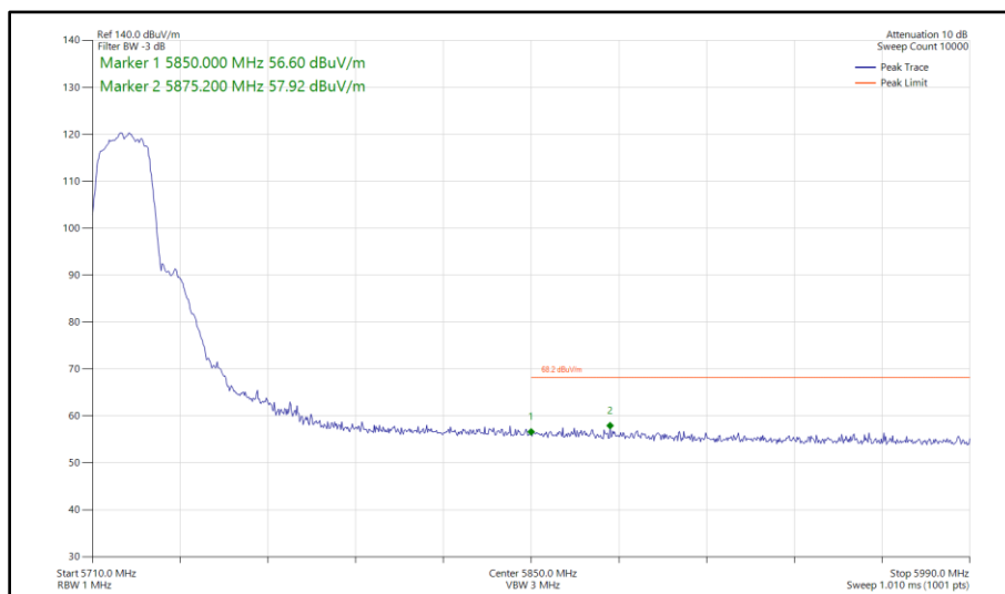
Figure 399 - 802.11a, SISO, Core 1 - 5720 MHz Band Edge Frequency 5850 MHz
