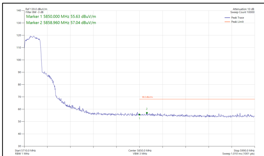
Figure 371 - 802.11ax HE20, SU, SISO, Core 0 - 5720 MHz Band Edge Frequency 5850 MHz
