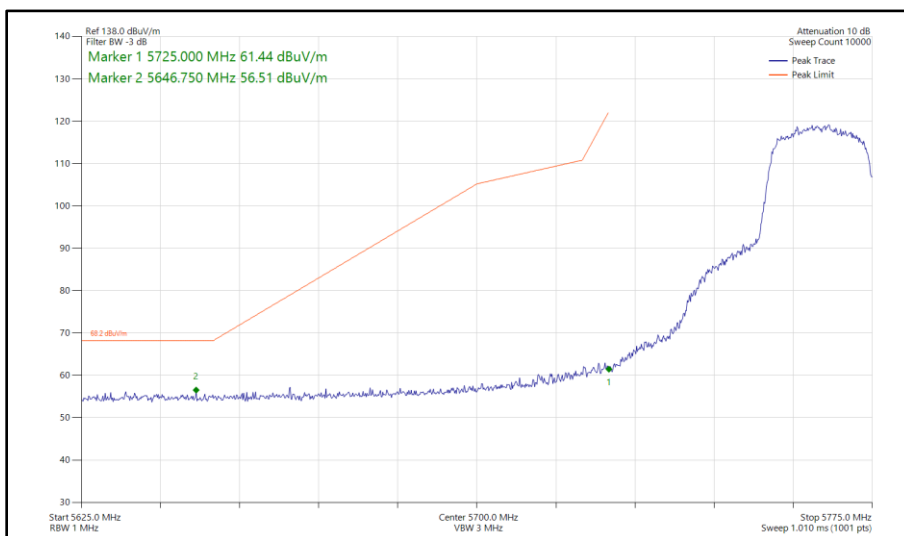
Figure 353 - 802.11n HT20, SISO, Core 0 - 5765 MHz Band Edge Frequency 5725 MHz
