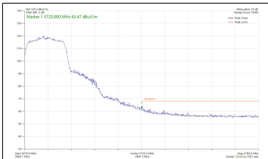
Figure 393 - 802.11n HT20, SISO, Core 1 - 5680 MHz Band Edge Frequency 5725 MHz
