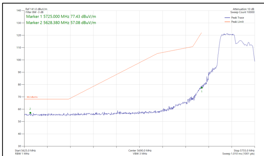
Figure 389 - 802.11ax HE20, RU 106-53, SISO, Core 1 - 5745 MHz Band Edge Frequency 5725 MHz
