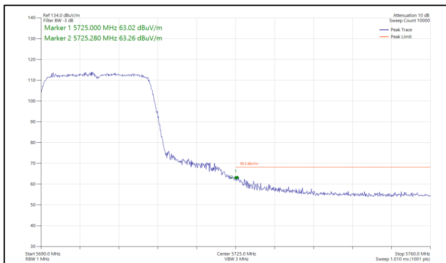
Figure 397 - 802.11ax HE20, SU, SISO, Core 1 - 5700 MHz Band Edge Frequency 5725 MHz
