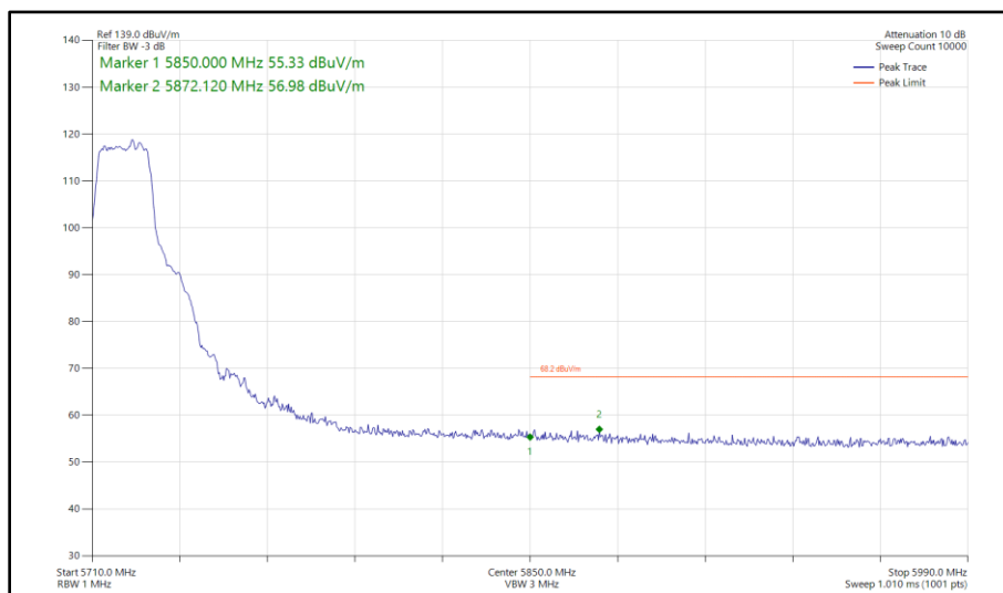
Figure 365 - 802.11a, SISO, Core 0 - 5720 MHz Band Edge Frequency 5850 MHz
