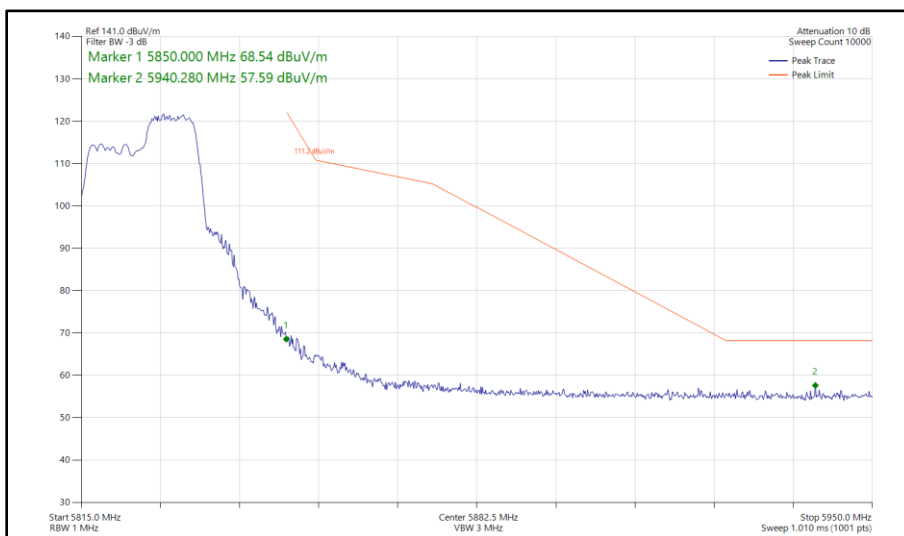
Figure 409 - 802.11ax HE20, RU 106-54, SISO, Core 1 - 5825 MHz Band Edge Frequency 5850 MHz
