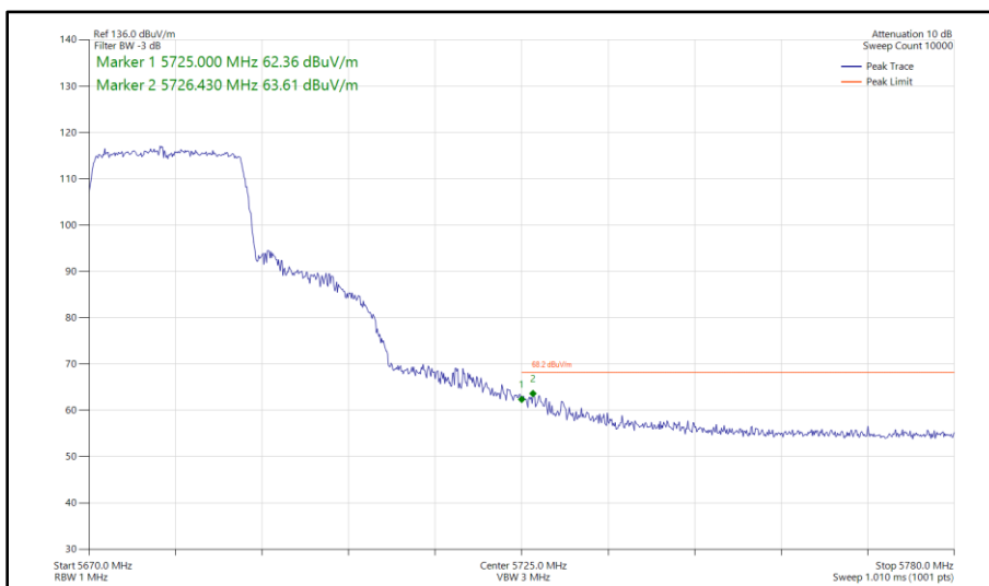
Figure 361 - 802.11ax HE20, SU, SISO, Core 0 - 5680 MHz Band Edge Frequency 5725 MHz
