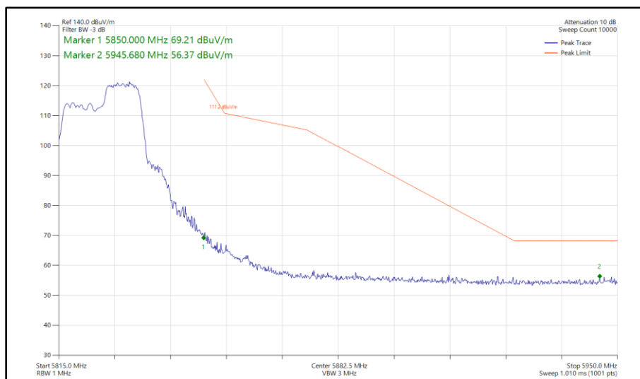
Figure 375 - 802.11ax HE20, RU 106-54, SISO, Core 0 - 5825 MHz Band Edge Frequency 5850 MHz
