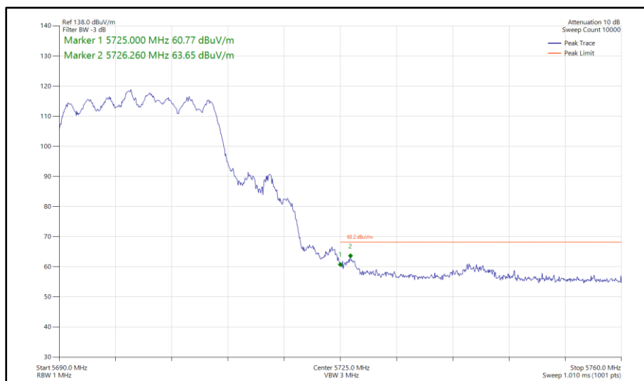
Figure 425 - 802.11ax HE20, SU, CDD, Core 0 - Core 1 - 5700 MHz Band Edge Frequency 5725 MHz
