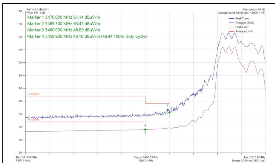
Figure 413 - 802.11ax HE20, RU 106-53, CDD, Core 0 - Core 1 - 5500 MHz Band Edge Frequency 5470 MHz
