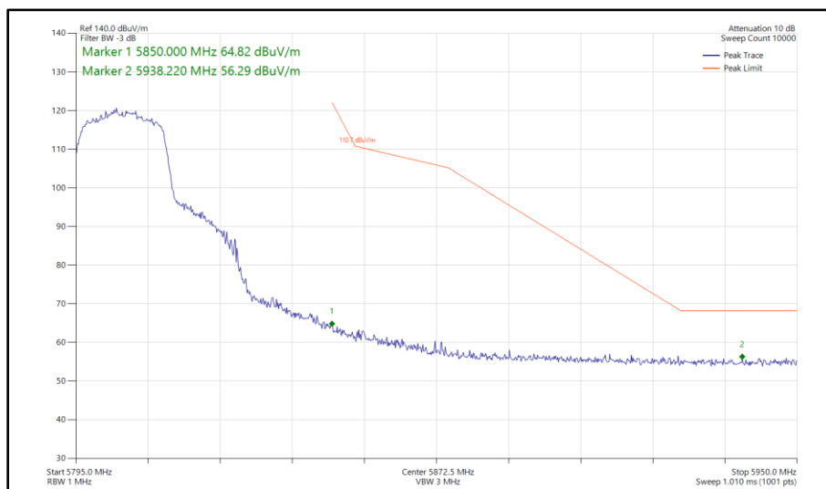
Figure 369 - 802.11n HT20, SISO, Core 0 - 5805 MHz Band Edge Frequency 5850 MHz
