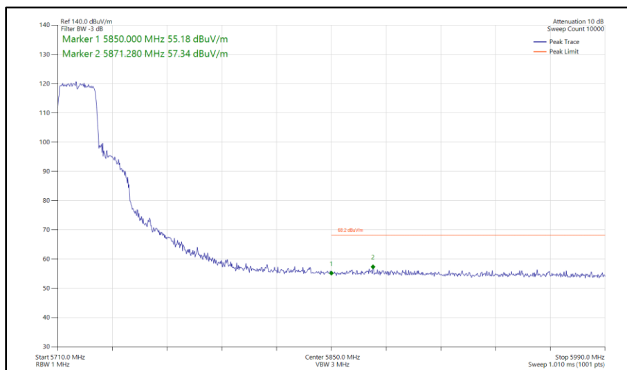
Figure 405 - 802.11ax HE20, SU, SISO, Core 1 - 5720 MHz Band Edge Frequency 5850 MHz
