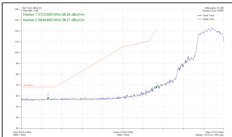
Figure 417 - 802.11n HT20, CDD, Core 0 - Core 1 - 5765 MHz Band Edge Frequency 5725 MHz
