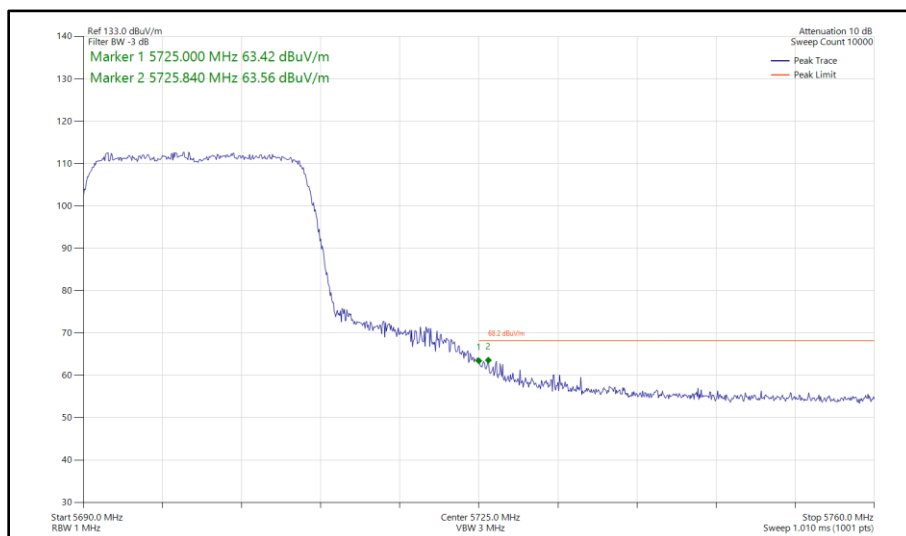
Figure 363 - 802.11ax HE20, SU, SISO, Core 0 - 5700 MHz Band Edge Frequency 5725 MHz
