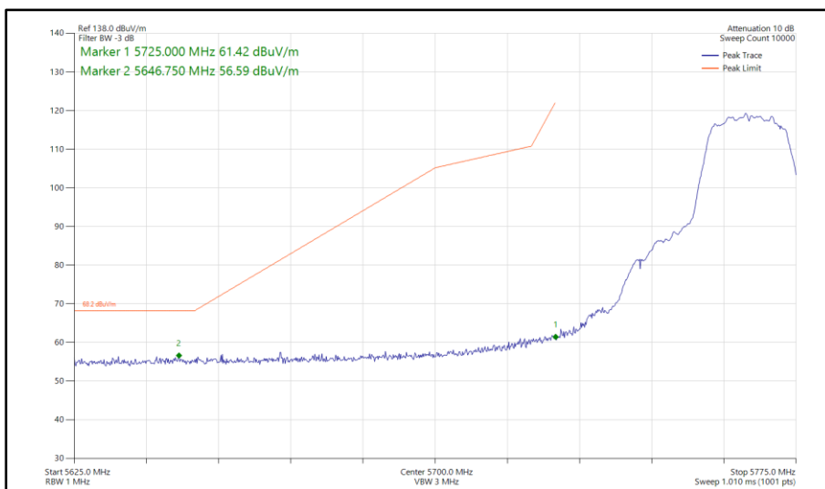
Figure 351 - 802.11a, SISO, Core 0 - 5765 MHz Band Edge Frequency 5725 MHz
