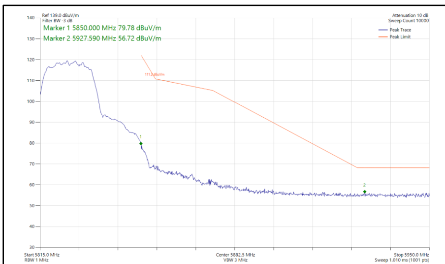
Figure 367 - 802.11a, SISO, Core 0 - 5825 MHz Band Edge Frequency 5850 MHz
