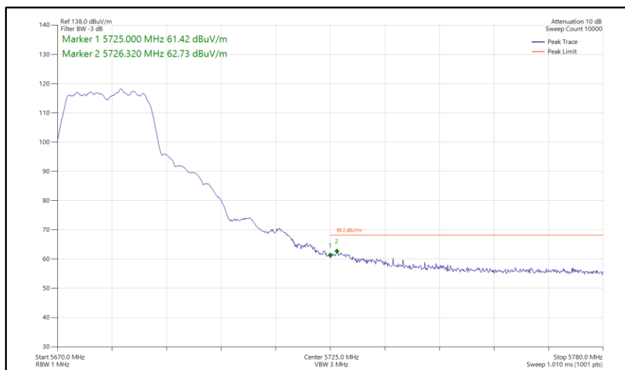
Figure 391 - 802.11a, SISO, Core 1 - 5680 MHz Band Edge Frequency 5725 MHz
