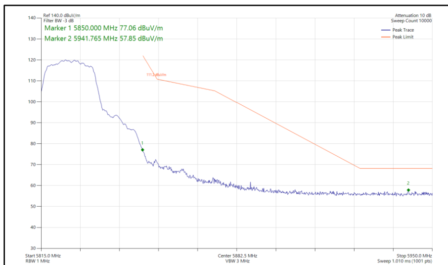
Figure 401 - 802.11a, SISO, Core 1 - 5825 MHz Band Edge Frequency 5850 MHz
