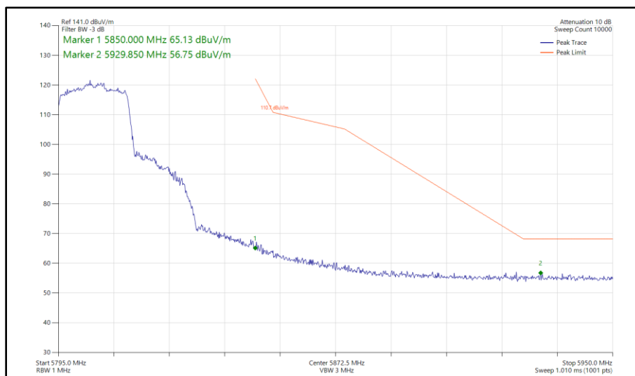
Figure 373 - 802.11ax HE20, SU, SISO, Core 0 - 5805 MHz Band Edge Frequency 5850 MHz
