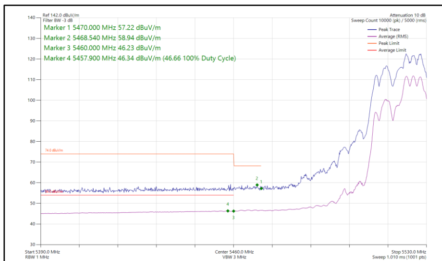
Figure 415 - 802.11ax HE20, RU 106-54, CDD, Core 0 - Core 1 - 5520 MHz Band Edge Frequency 5470 MHz
