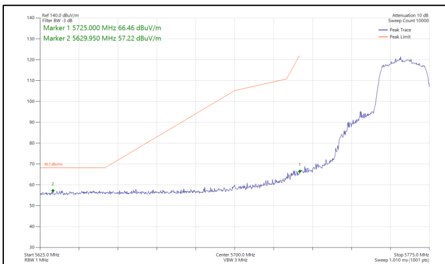
Figure 387 - 802.11n HT20, SISO, Core 1 - 5765 MHz Band Edge Frequency 5725 MHz
