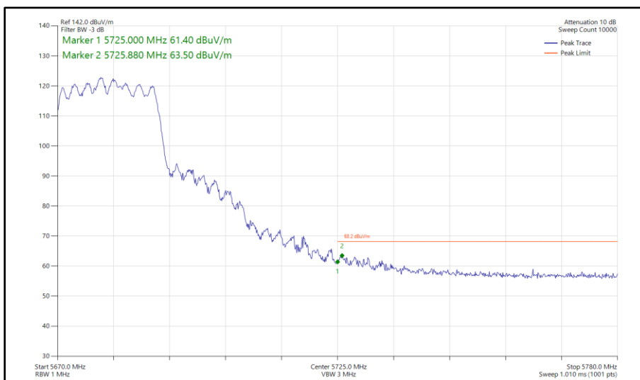
Figure 423 - 802.11ax HE20, SU, CDD, Core 0 - Core 1 - 5680 MHz Band Edge Frequency 5725 MHz
