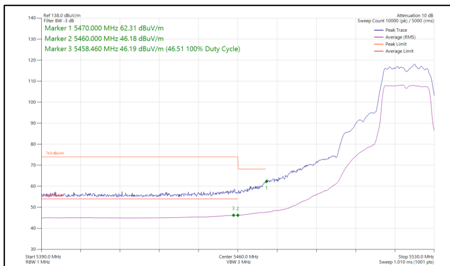
Figure 377 - 802.11a, SISO, Core 1 - 5520 MHz Band Edge Frequency 5470 MHz
