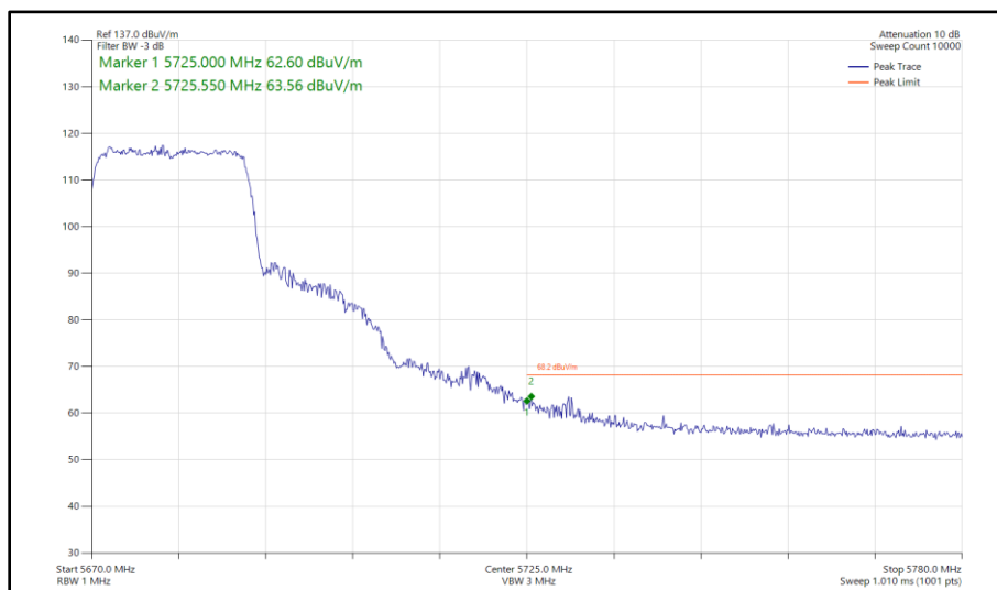
Figure 395 - 802.11ax HE20, SU, SISO, Core 1 - 5680 MHz Band Edge Frequency 5725 MHz
