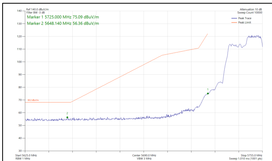
Figure 355 - 802.11ax HE20, RU 106-54, SISO, Core 0 - 5745 MHz Band Edge Frequency 5725 MHz
