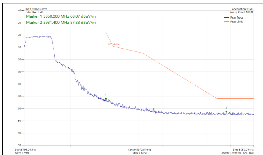
Figure 403 - 802.11n HT20, SISO, Core 1 - 5805 MHz Band Edge Frequency 5850 MHz
