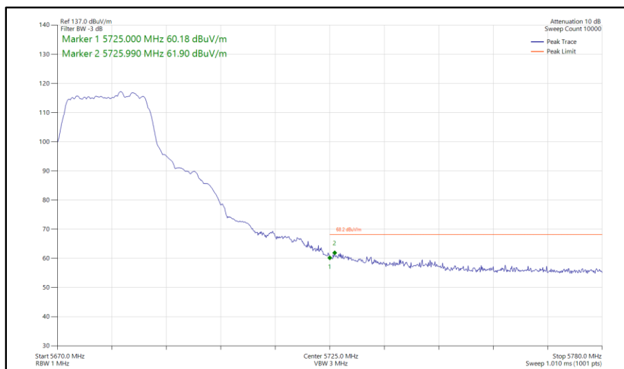
Figure 357 - 802.11a, SISO, Core 0 - 5680 MHz Band Edge Frequency 5725 MHz
