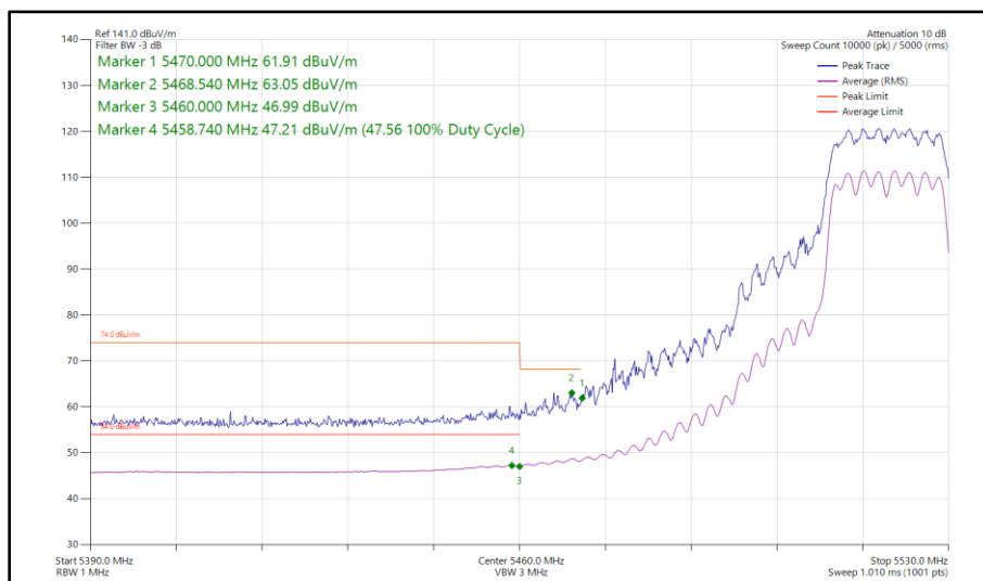
Figure 411 - 802.11n HT20, CDD, Core 0 - Core 1 - 5520 MHz Band Edge Frequency 5470 MHz
