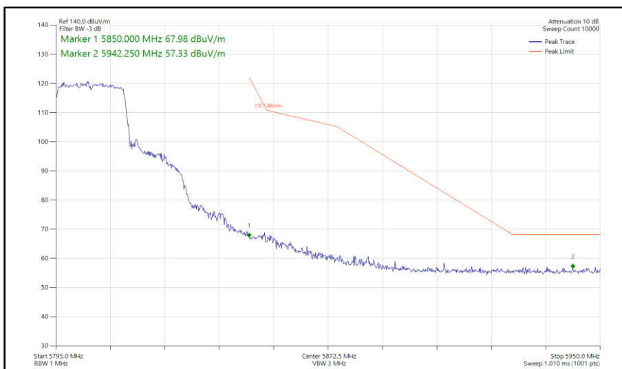
Figure 407 - 802.11ax HE20, SU, SISO, Core 1 - 5805 MHz Band Edge Frequency 5850 MHz
