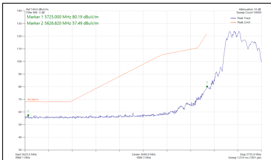
Figure 419 - 802.11ax HE20, RU 106-53, CDD, Core 0 - Core 1 - 5745 MHz Band Edge Frequency 5725 MHz
