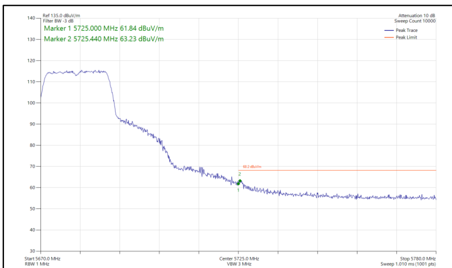
Figure 359 - 802.11n HT20, SISO, Core 0 - 5680 MHz Band Edge Frequency 5725 MHz
